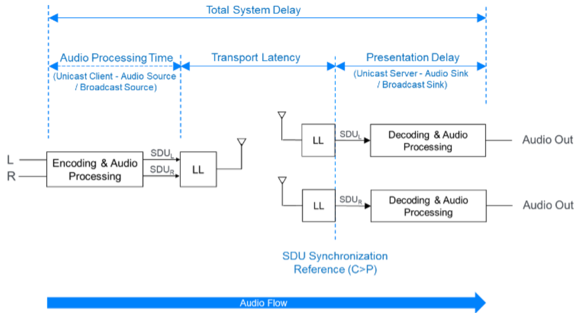
Figure 3.10: Unicast total system delay
