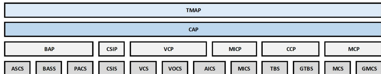
Figure 3.2: TMAP and LE Audio layers in detail
