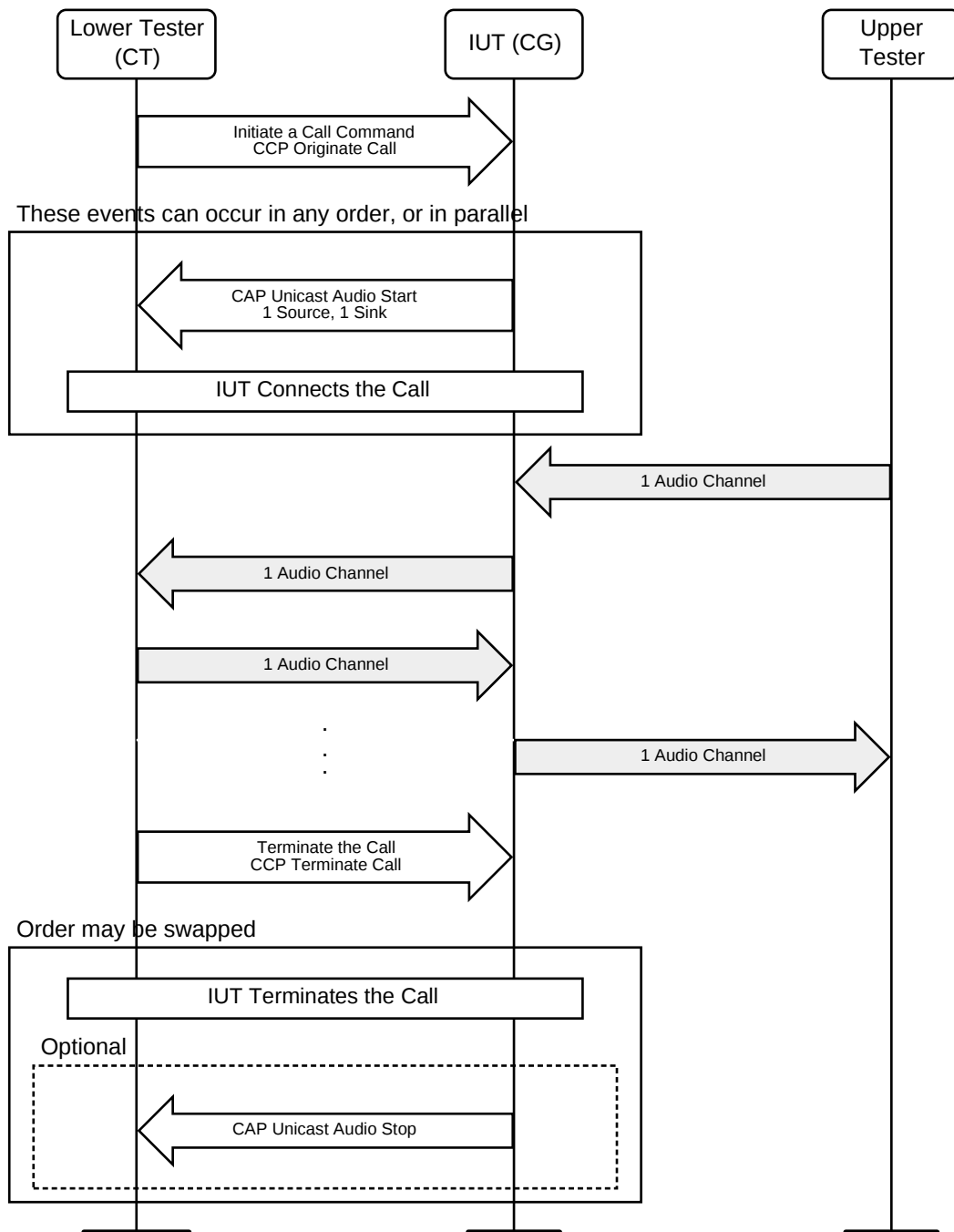
Figure 4.1: TMAP/CG/VRC/BV-07-C [Call Initiated from CT] MSC
