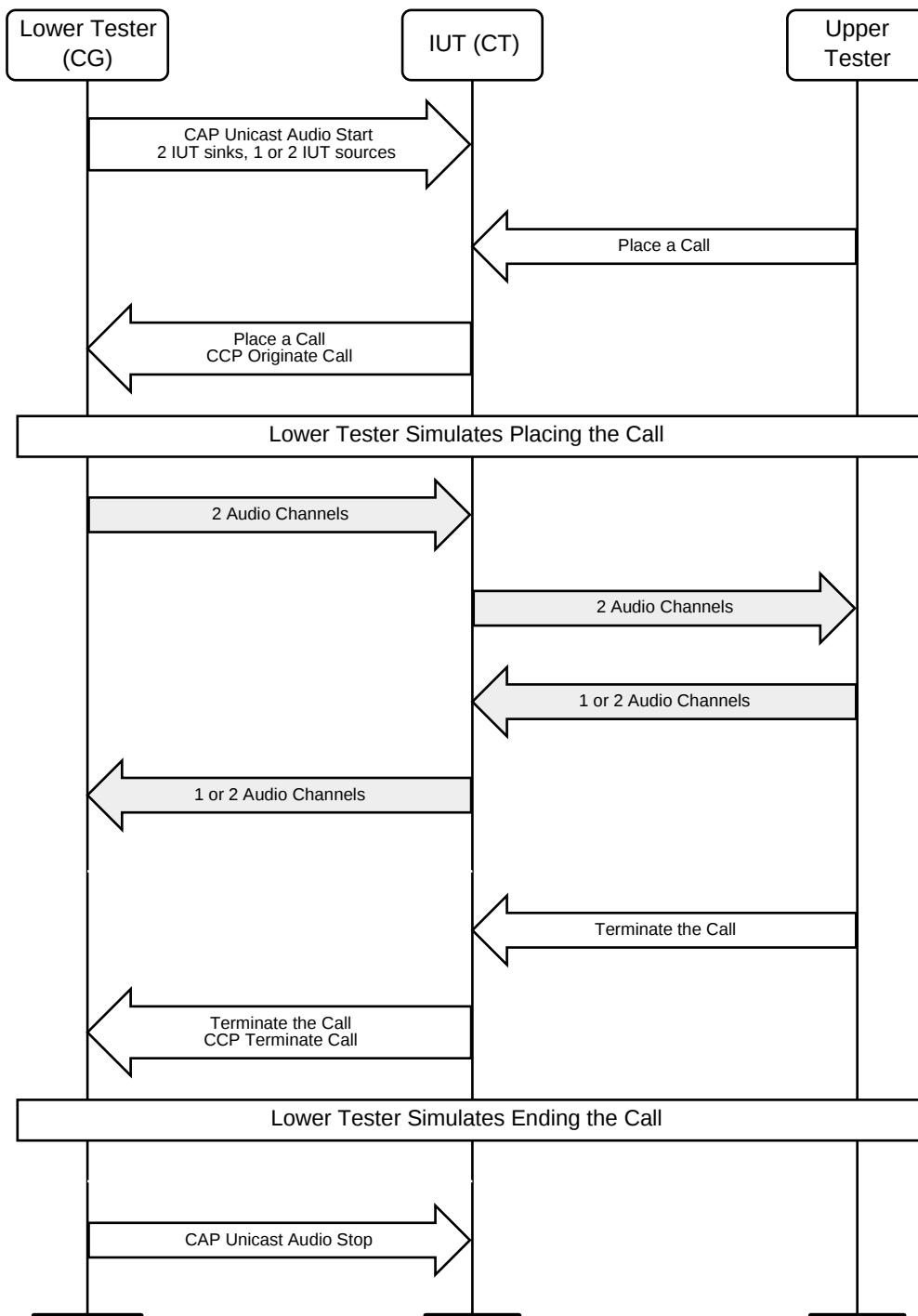
Figure 4.4: Call Initiated from CT MSC
