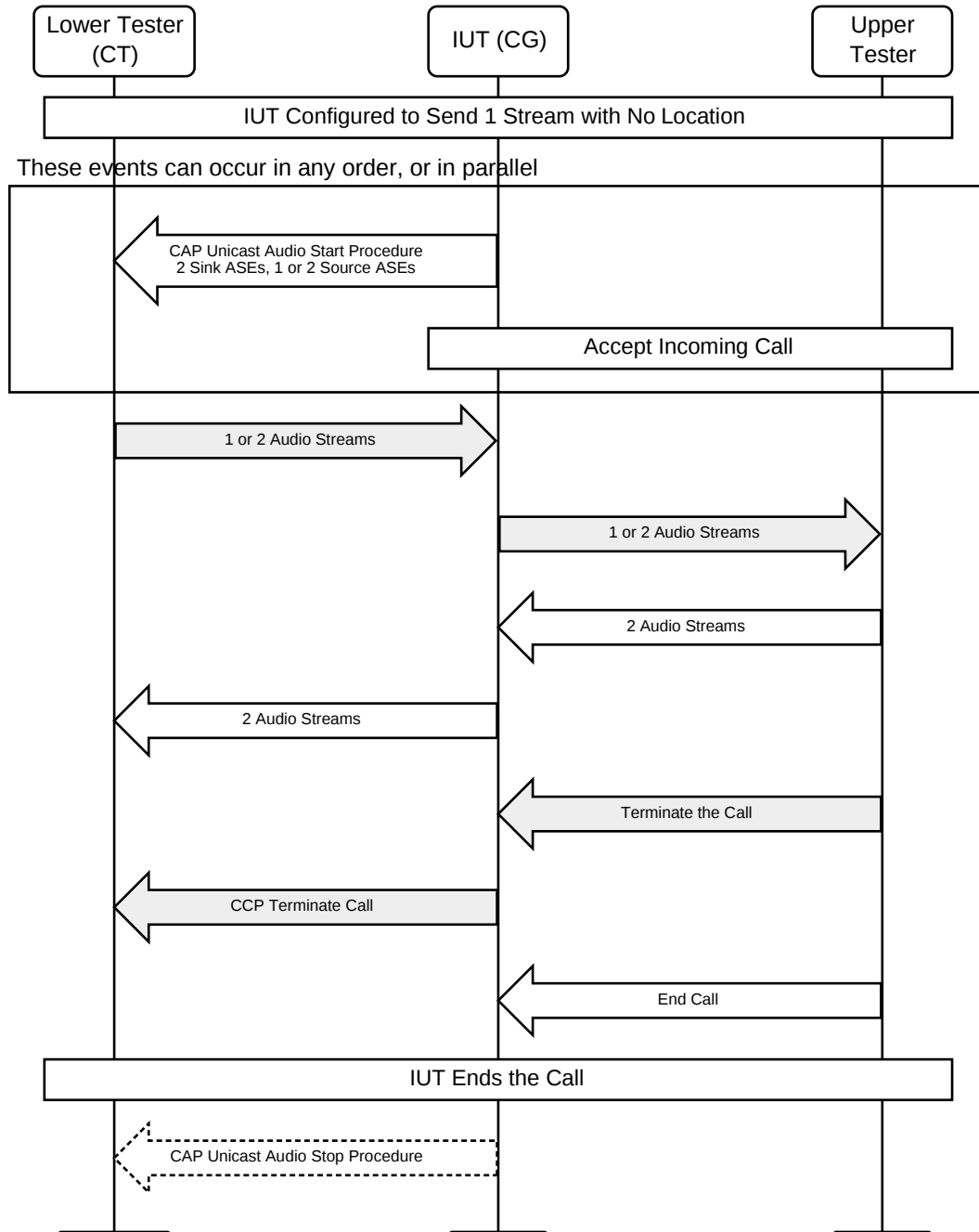
Figure 4.2: CG sends identical audio to Front Left and Front Right Audio Locations MSC
