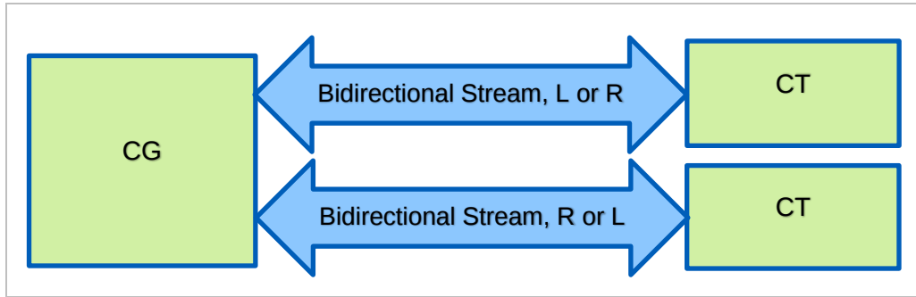
Figure 3.21: CG/CT Configuration G, single CG, two CTs, two bidirectional streams
