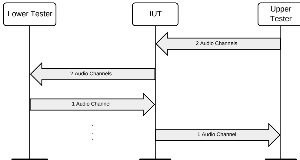
Figure 3.22: MSC describing the flow of audio channels
