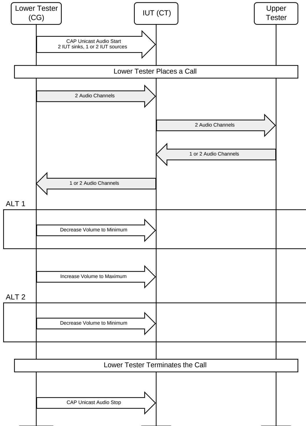
Figure 4.3: Call Initiated from CG, IUT is Audio Source and Sink MSC
