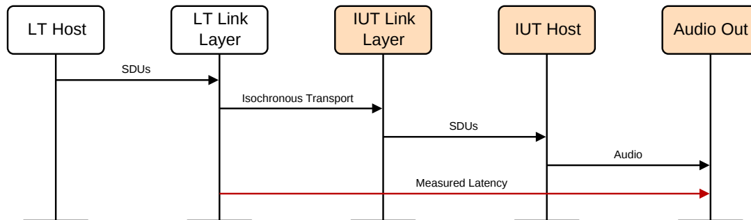
Figure 3.11: Multi-stream synchronization for two Acceptors latency measurement
