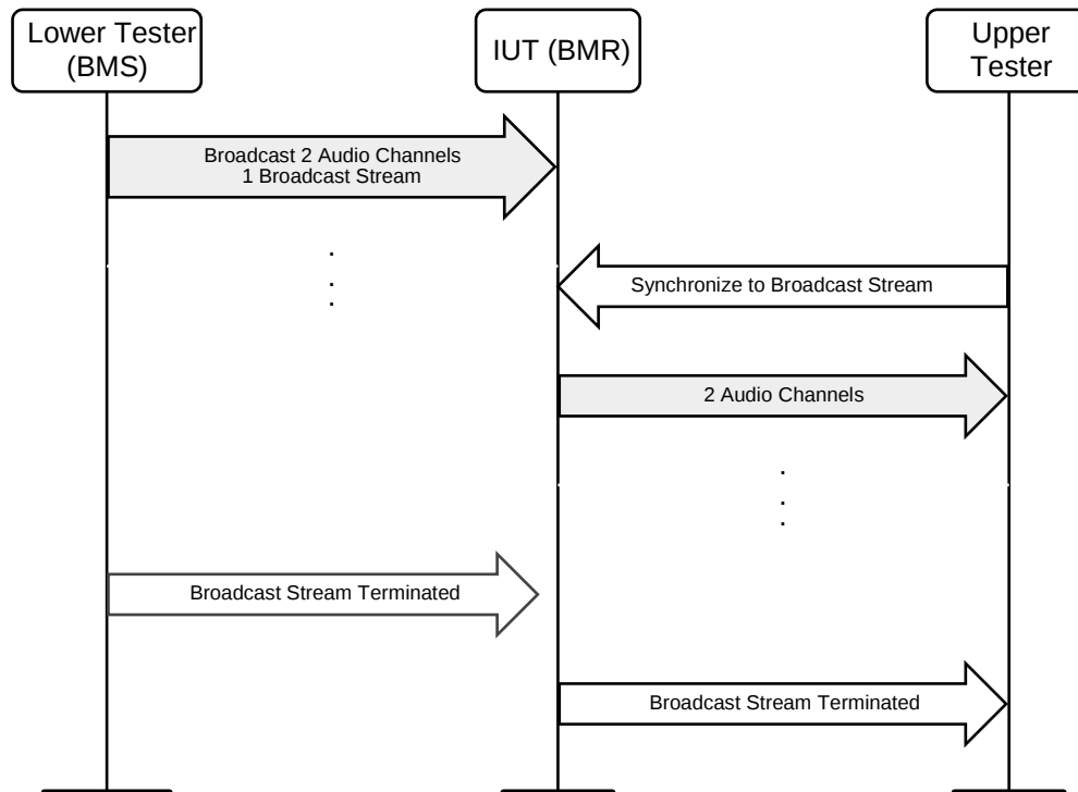
Figure 4.5: BMR in Audio Configuration 14 MSC
