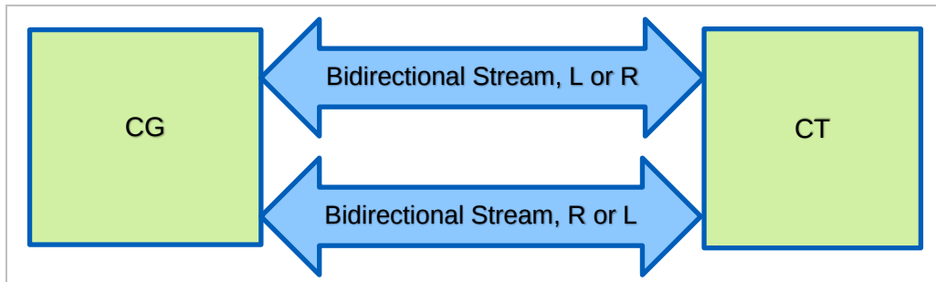
Figure 3.20: CG/CT Configuration F, single CG, single CT, two bidirectional streams
