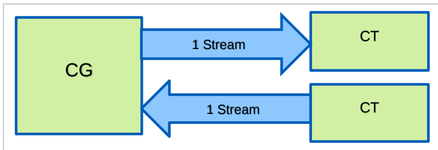
Figure 3.16: CG/CT Configuration B, two CTs, single streams
