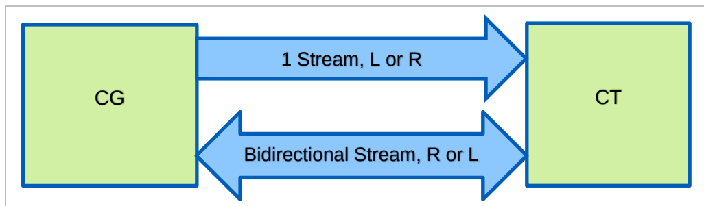
Figure 3.18: CG/CT Configuration D, single CG, single CT, two streams, Front Left and Front Right
