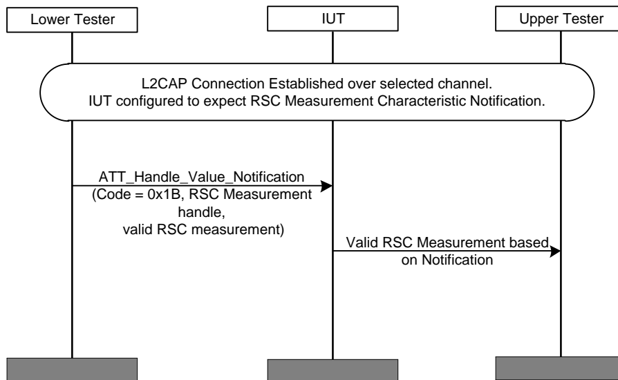
Figure 4.6: RSCP/COL/RSCF/BI-01-C [Receive RSC Measurement Notifications with reserved flags]
