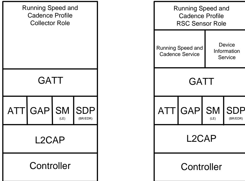
Figure 3.1: Running Speed and Cadence test model
