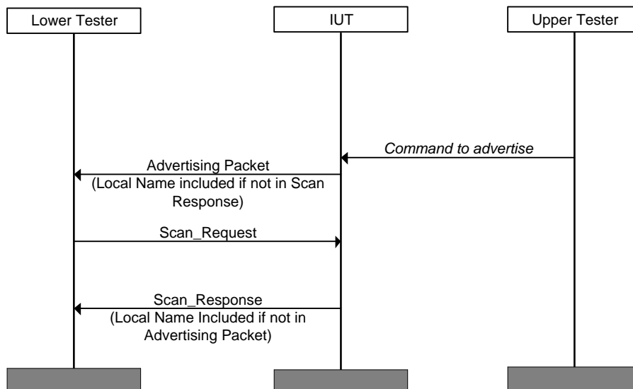
Figure 4.2: RSCP/SEN/RSCF/BV-02-C [Local Name included in AD or Scan Response]
