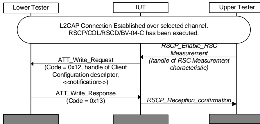
Figure 4.4: RSCP/COL/RSCF/BV-04-C [Configure RSC Measurement for Notification]
