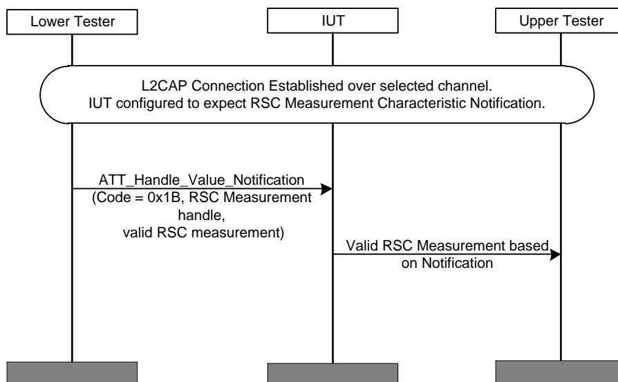
Figure 4.5: RSCP/COL/RSCF/BV-05-C [Receive RSC Measurement for Notifications]
