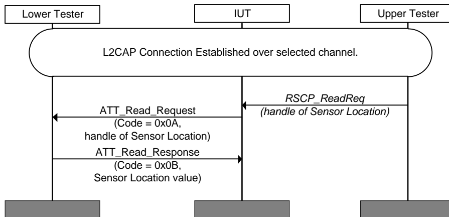
Figure 4.9: RSCP/COL/RSCF/BI-04-C [Read Sensor Location characteristic with reserved value]
