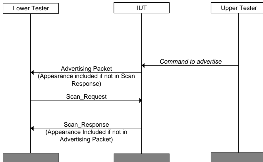
Figure 4.3: RSCP/SEN/RSCF/BV-03-C [Appearance included in AD or Scan Response]
