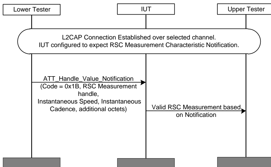
Figure 4.7: RSCP/COL/RSCF/BI-02-C [Receive RSC Measurement Notifications with additional octets not represented in the flags field]
