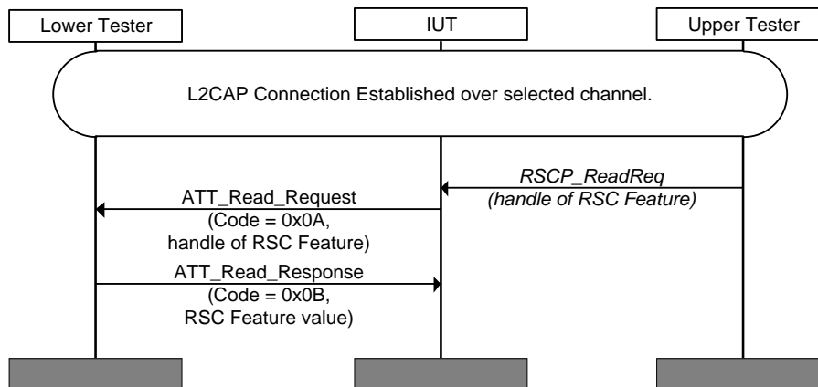
Figure 4.8: RSCP/COL/RSCF/BI-03-C [Read RSC Feature characteristic with reserved value]
