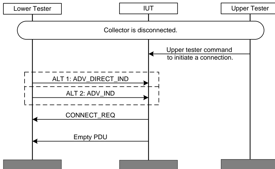
Figure 4.1: LE Collector: Scan to detect Sensor Advertisements preamble
