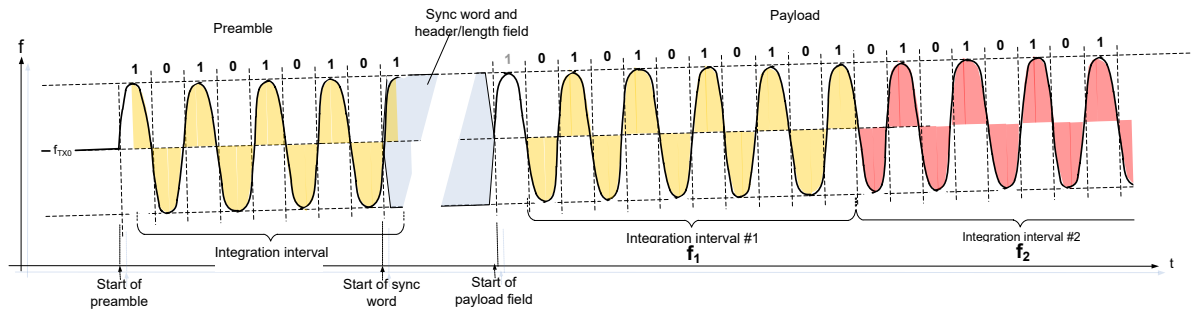
Figure 4.8: Frequency drift measurement principle
