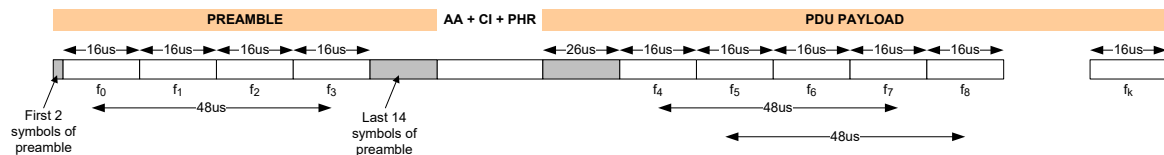
Figure 4.10: Frequency drift rate measurement principle for S=8
