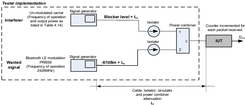
Figure 4.22: Blocking performance test setup
