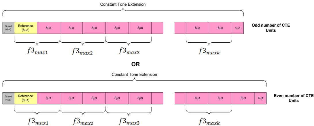
Figure 4.15: Average frequency deviation measurement principle
