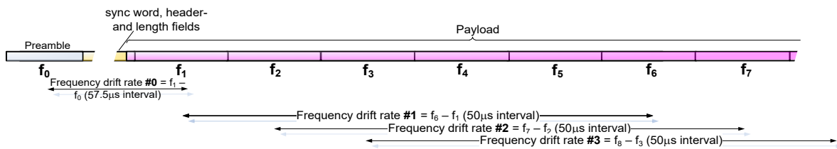
Figure 4.9: Frequency drift rate measurement principle
