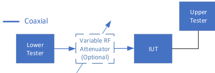
Figure 4.1: Test Equipment Setup for AoD Receiver
