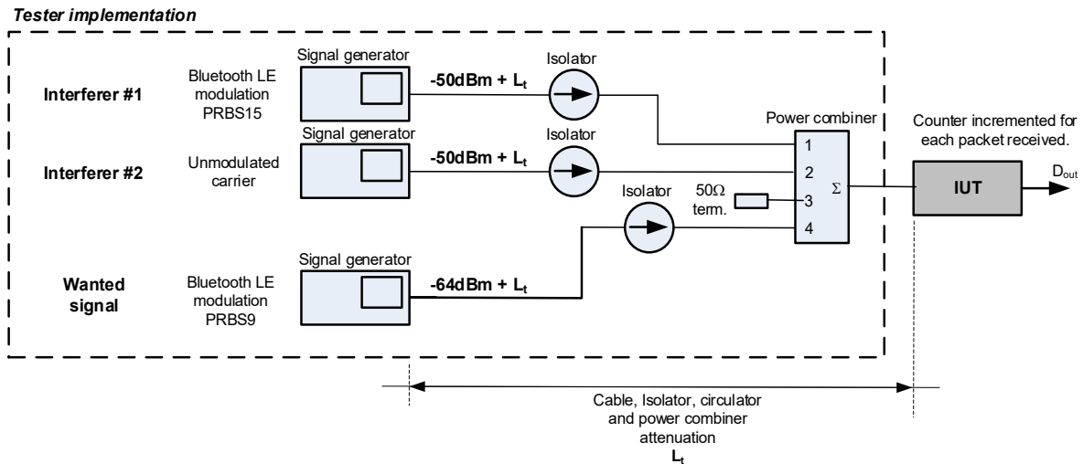
Figure 4.23: Test setup for intermodulation test
