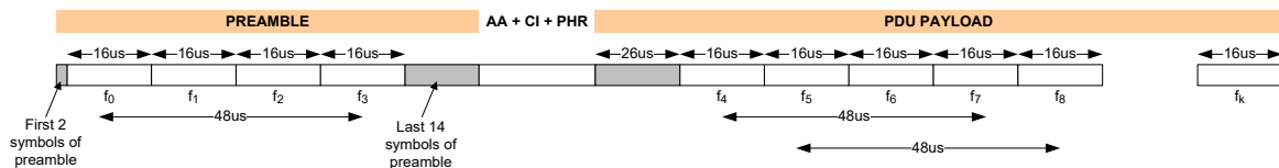
Figure 4.10: Frequency drift rate measurement principle for S=8
