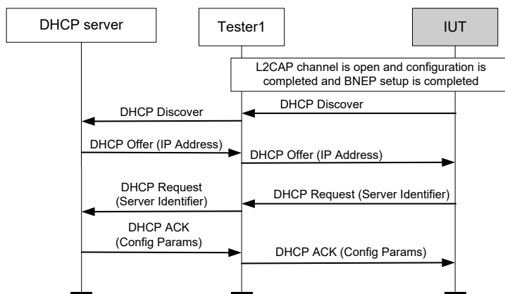
Figure 4.20: PAN/PANU/IP/DHCP/BV-03-C [IP Address Assignment – Infrastructure (DHCP)]
