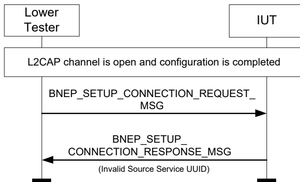
Figure 4.32: 128-Bit UUID processing
