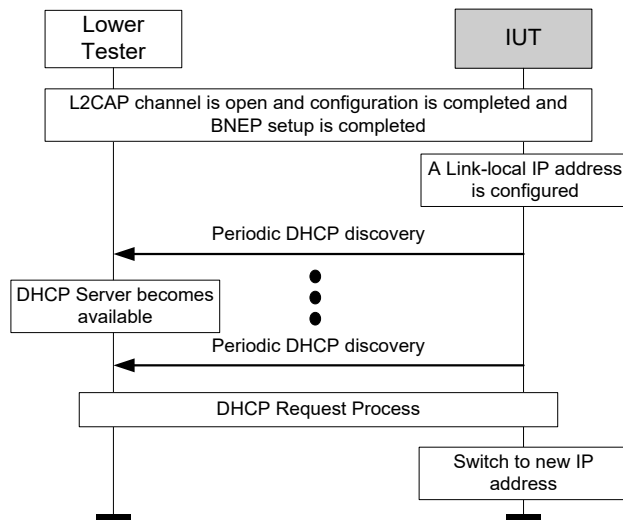
Figure 4.27: PAN/PANU/IP/APP/BV-04-C [Periodically Checking for DHCP Service]
