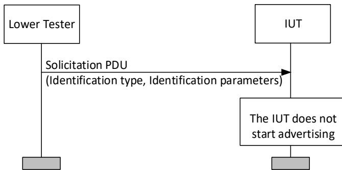
Figure 4.106: Test procedure for MESH/SR/MPXS/BV-13-C MSC
