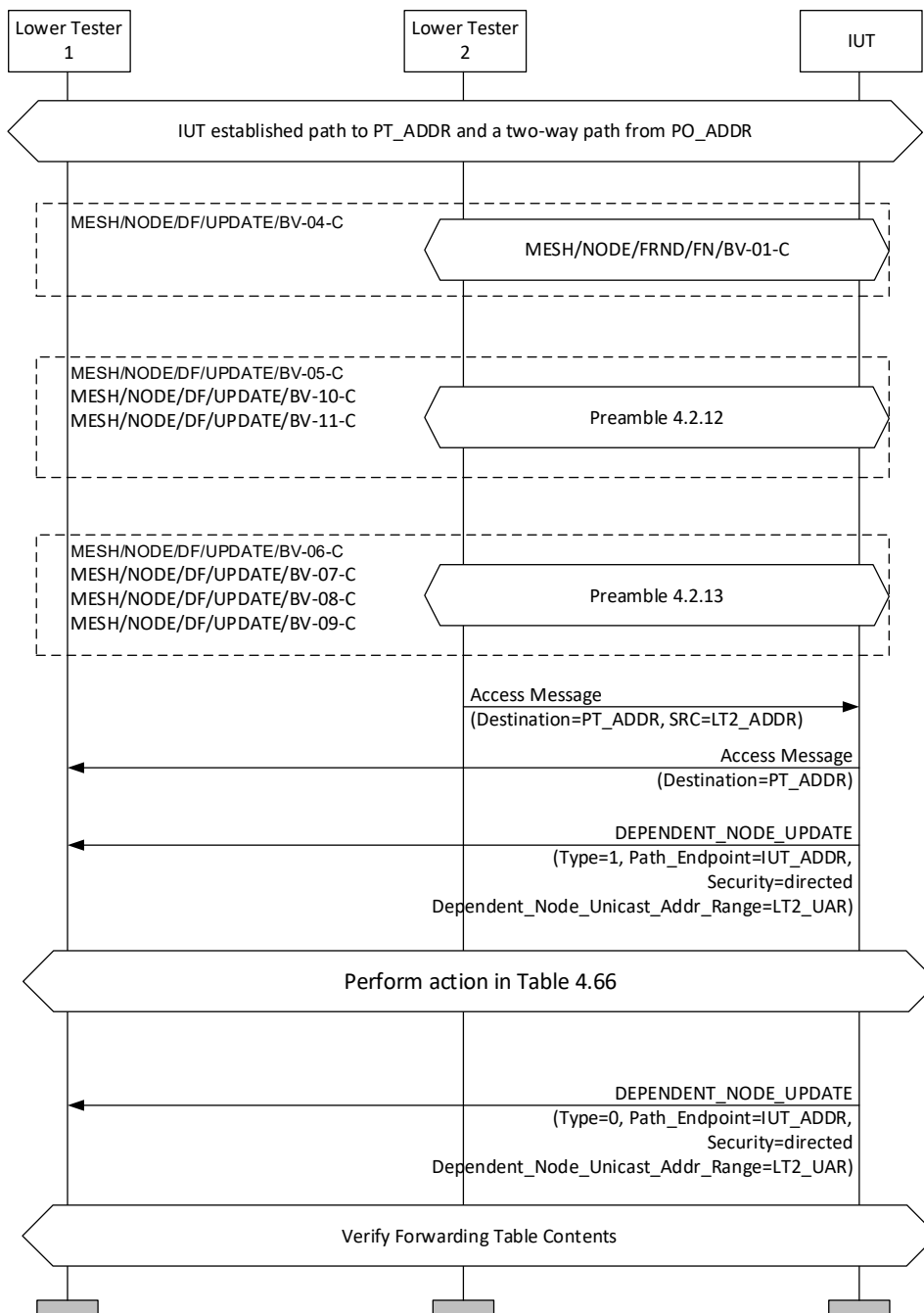
Figure 4.245: Remove Node Dependence MSC
