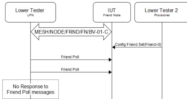
Figure 4.69: MESH/NODE/FRND/FN/BV-10-C [Friendship – Friend Node Config Friend Set Received] MSC
