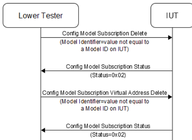
Figure 4.141: MESH/NODE/CFG/SL/BI-06-C [Respond to Config Model Subscription Delete / Virtual Address Delete Message (Invalid Model Identifier)] MSC
