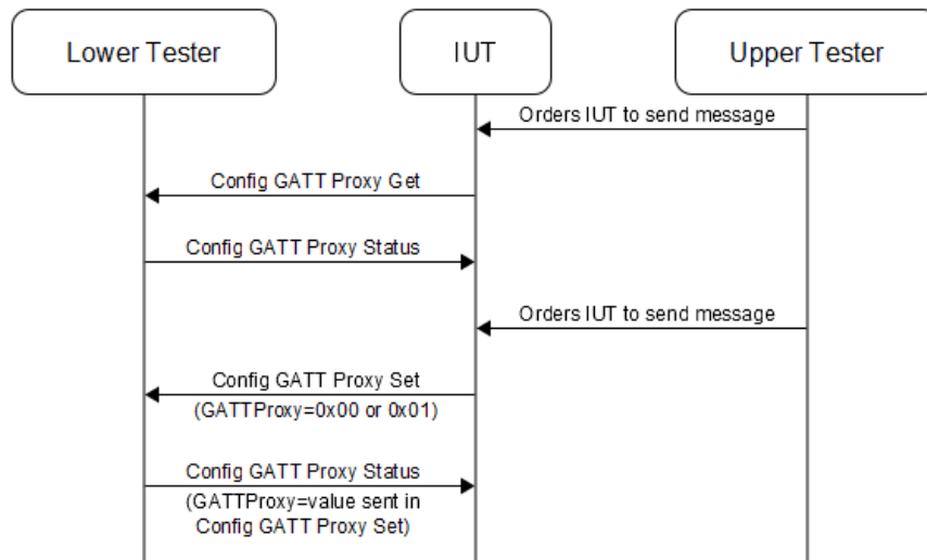
Figure 4.119: MESH/CFGCL/CFG/GPXY/BV-01-C [Send Config GATT Proxy Set/Get Messages] MSC
