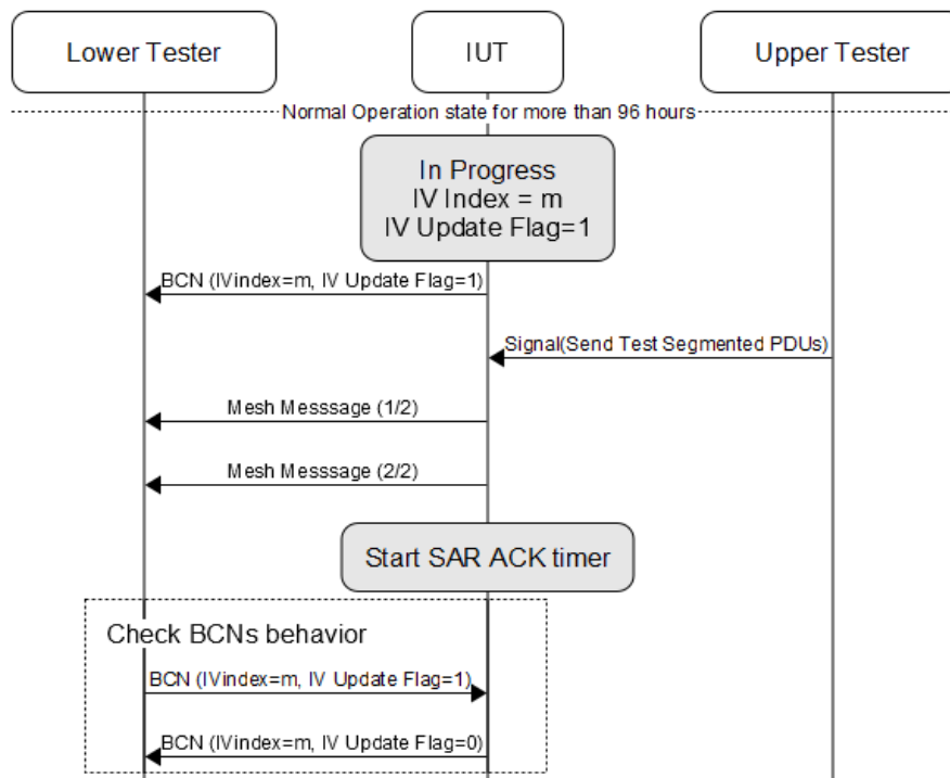
Figure 4.48: MESH/NODE/IVU/BV-04-C and MESH/NODE/IVU/BV-09-C MSC
