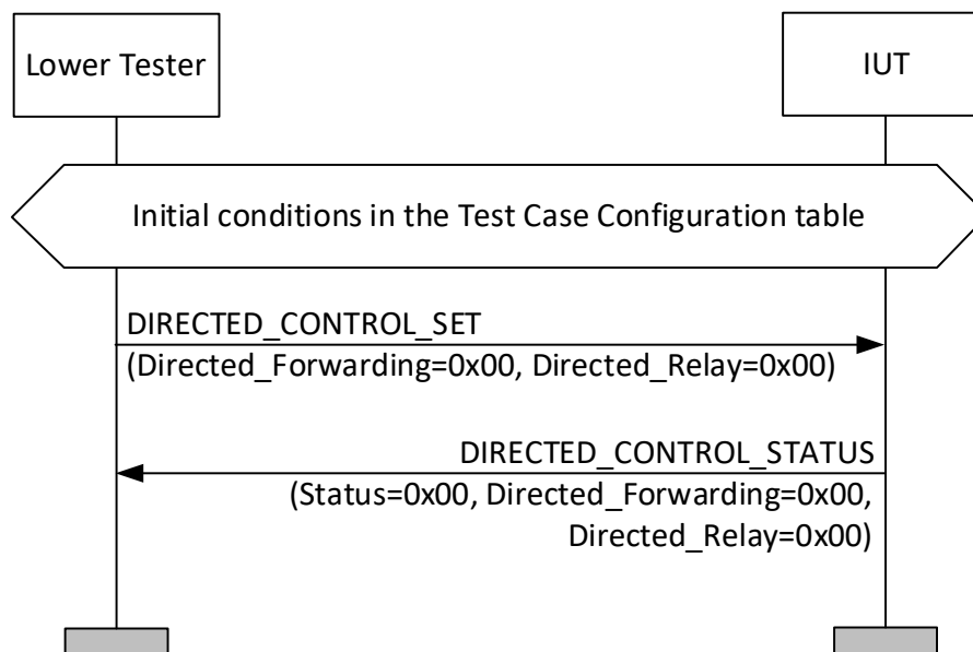
Figure 4.280: Directed Control Set Behavior – Bindings MSC
