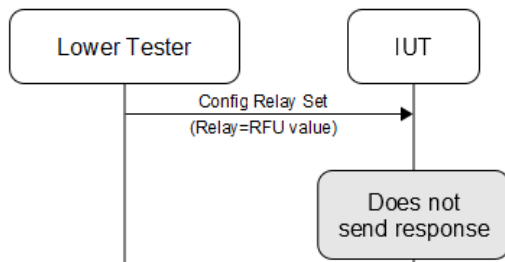
Figure 4.124: MESH/NODE/CFG/CFGR/BI-01-C [Respond to Config Relay Set Messages Invalid Parameters] MSC
