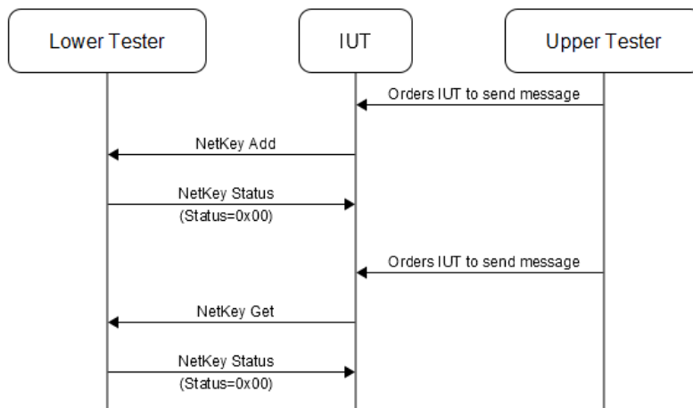
Figure 4.155: MESH/CFGCL/CFG/NKL/BV-01-C [Send Config NetKey Add/Get Messages] MSC
