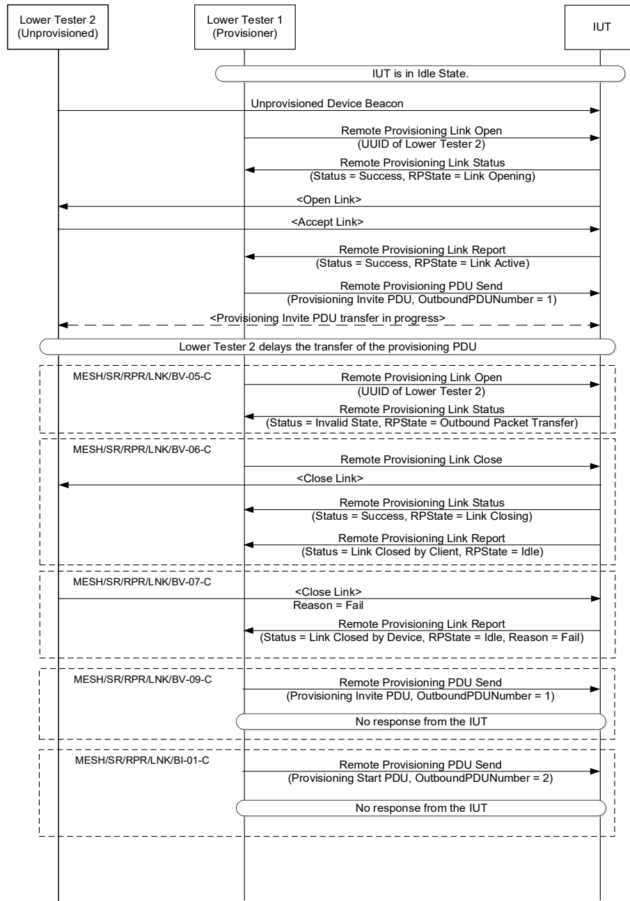
Figure 4.324: Test procedure – Handle Requests and Events in the Outbound Packet Transfer State MSC – Page 1 of 2
