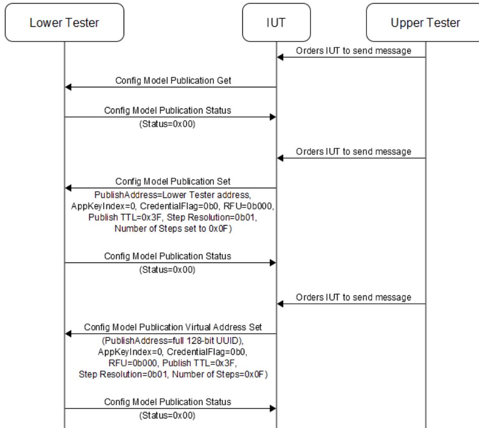
Figure 4.131: MESH/CFGCL/CFG/MP/BV-01-C [Send Config Model Publication Set/Get and Config Model Publication Virtual Address Set Messages] MSC
