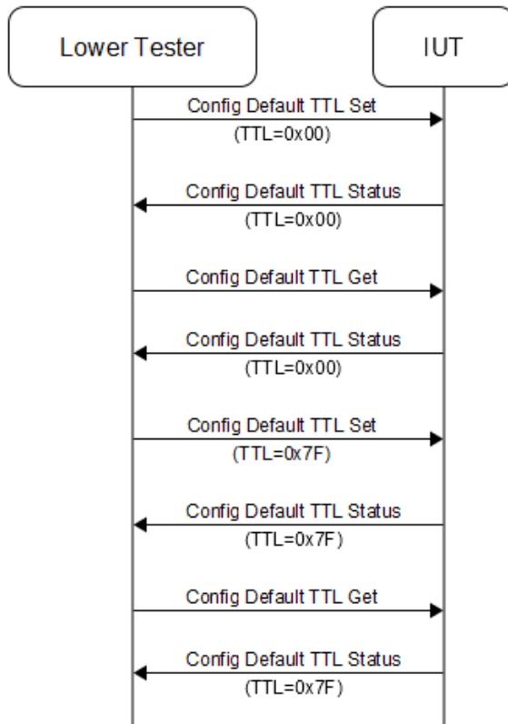
Figure 4.113: MESH/NODE/CFG/DTTL/BV-01-C [Respond to Config Default TTL Set/Get Messages] MSC
