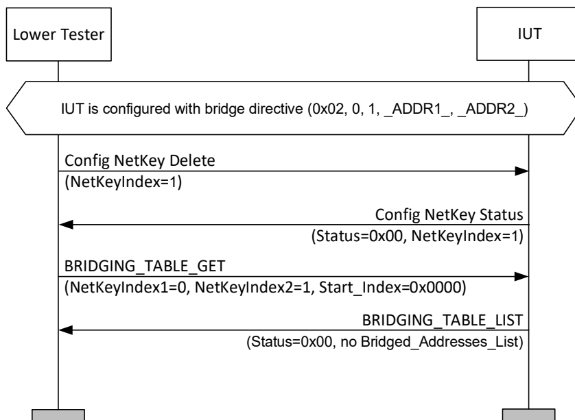
Figure 4.307: Test procedure for MESH/SR/BCM/BDS/BV-06-C [Bridging Table State – Binding with NetKey List State] MSC
