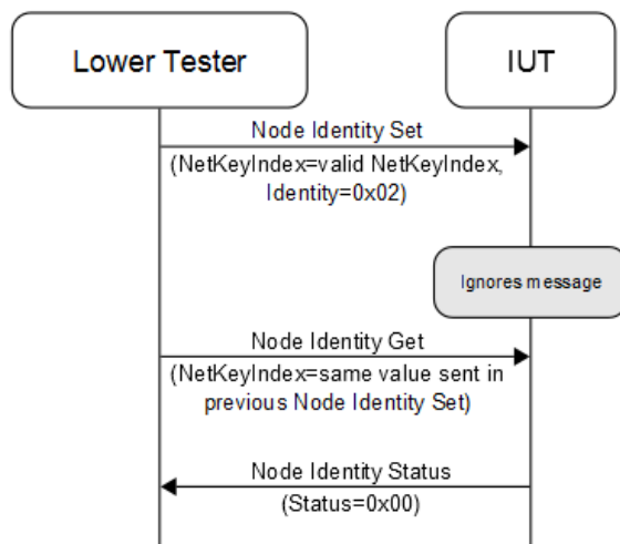
Figure 4.179: MESH/NODE/CFG/NID/BI-03-C [Receive Config Node Identity Set Message – Change to Not Supported] MSC
