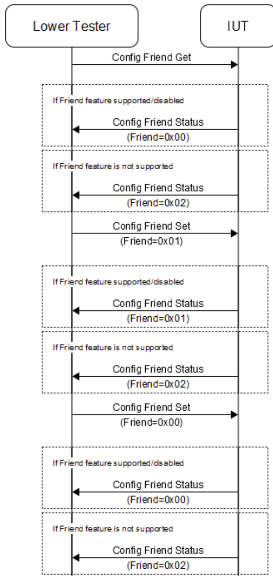
Figure 4.120: MESH/NODE/CFG/CFGF/BV-01-C [Respond to Config Friend Get/Set Messages] MSC
