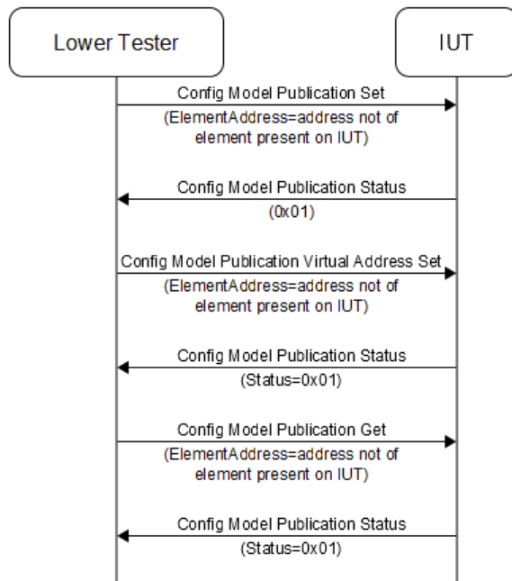
Figure 4.128: MESH/NODE/CFG/MP/BI-01-C [Respond to Config Model Publication Get/Set/Virtual Address Set Messages (Invalid ElementAddress)] MSC
