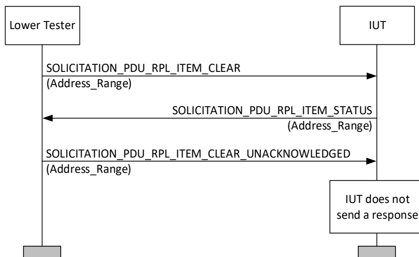
Figure 4.354: Test procedure for MESH/SR/SRPL/BV-01-C MSC
