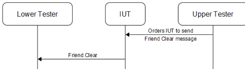
Figure 4.92: MESH/NODE/FRND/LPN/BV-08-C [Low Power Node Send Friend Clear Message] MSC
