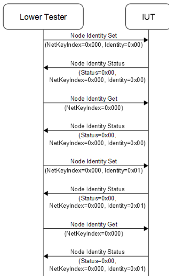
Figure 4.175: MESH/NODE/CFG/NID/BV-01-C [Receive Config Node Identity Get/Set Messages] MSC
