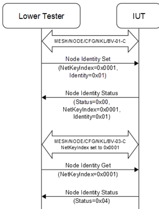
Figure 4.177: MESH/NODE/CFG/NID/BV-03-C [Node Identity Config NetKey Deleted] MSC
