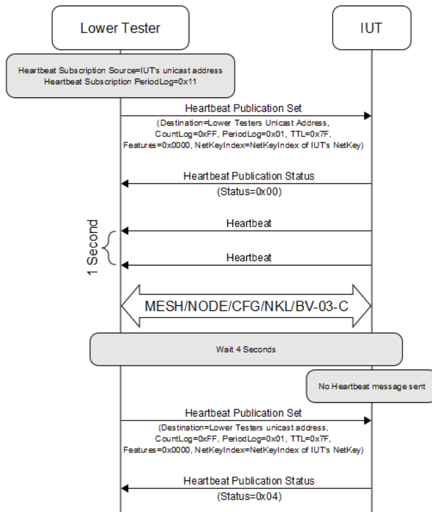
Figure 4.188: MESH/NODE/CFG/HBP/BV-06-C [Disabling publishing of Heartbeat messages – Config NetKey Deleted] MSC
