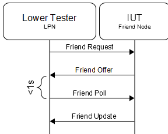
Figure 4.60: MESH/NODE/FRND/FN/BV-01-C [Friendship Establishment Mode – Friend Node] MSC
