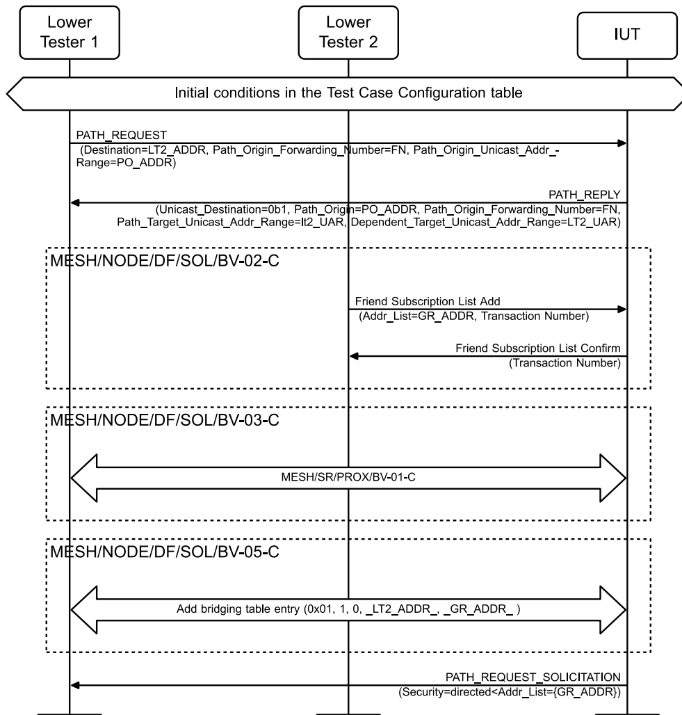
Figure 4.257: Send PATH_REQUEST_SOLICITATION for Dependent MSC
