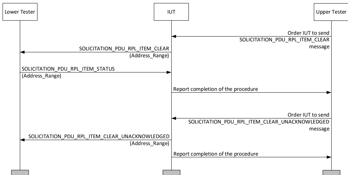
Figure 4.355: Test procedure for MESH/CL/SRPL/BV-01-C MSC
