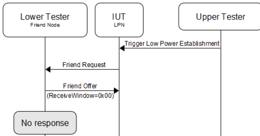
Figure 4.95: MESH/NODE/FRND/LPN/BI-03-C [Friendship Low Power Node – Friend Offer Invalid RFU Bits] MSC
