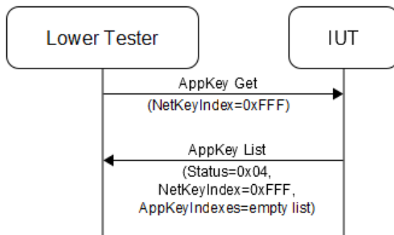
Figure 4.163: MESH/NODE/CFG/AKL/BI-03-C [Respond to Config AppKey Get Message with Invalid NetKey Index] MSC
