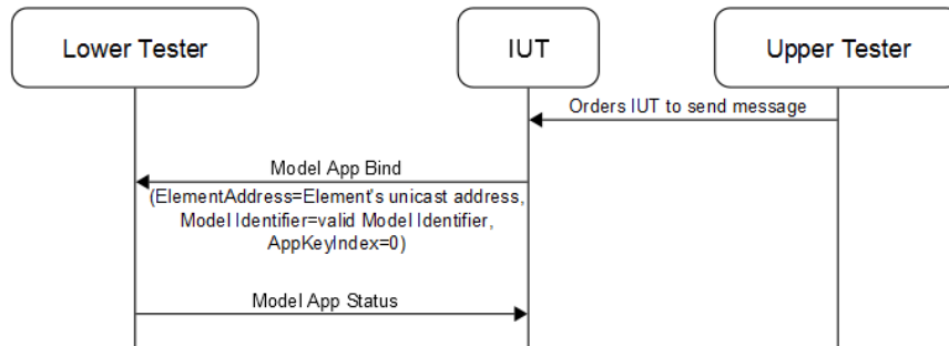
Figure 4.171: MESH/CFGCL/CFG/MAKL/BV-01-C [Send Config Model App Bind Messages] MSC
