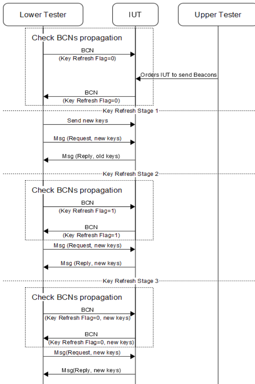
Figure 4.54: MESH/NODE/KR/BV-02-C and MESH/NODE/KR/BV-04-C MSC
