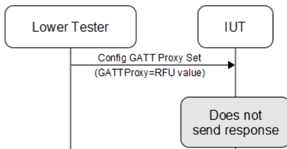
Figure 4.118: MESH/NODE/CFG/GPXY/BI-01-C [Respond to Config GATT Proxy Set Messages Invalid Parameters] MSC
