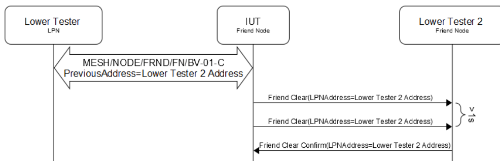
Figure 4.70: MESH/NODE/FRND/FN/BV-11-C [Friendship – Friend Node Friend Clear Send and Retry] MSC
