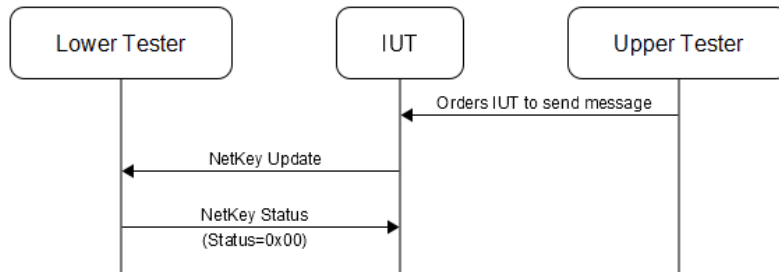
Figure 4.156: MESH/CFGCL/CFG/NKL/BV-02-C [Send Config NetKey Update Messages] MSC
