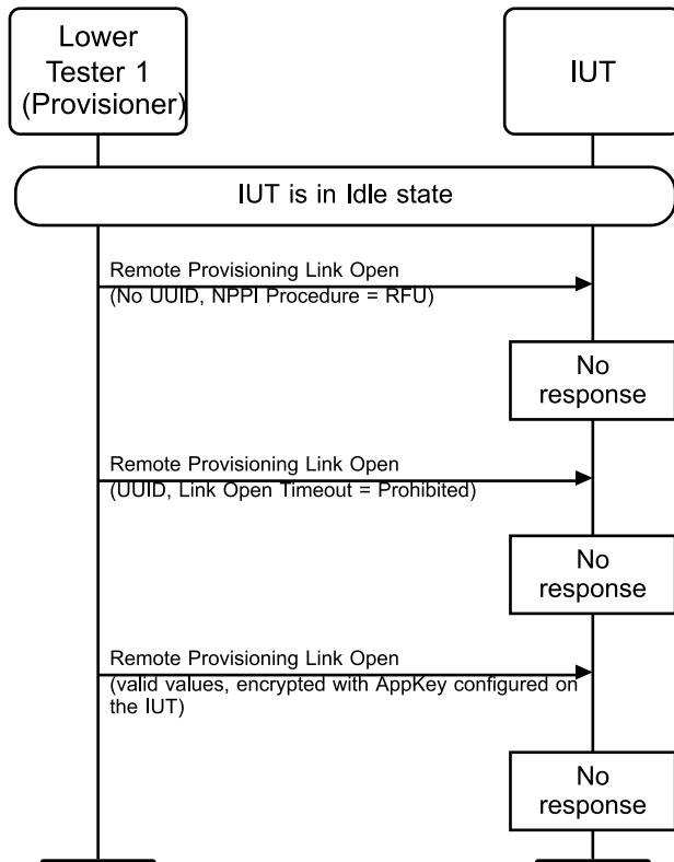
Figure 4.331: Test procedure for MESH/SR/RPR/LNK/BI-04-C MSC
