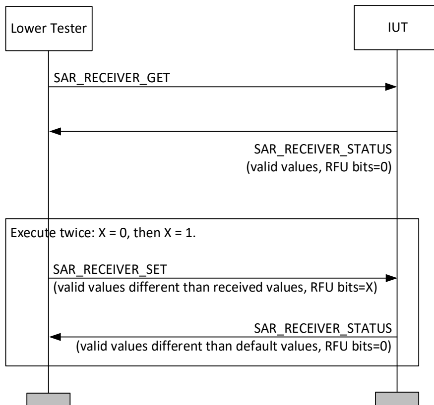
Figure 4.344: Test procedure for MESH/SR/SAR/BV-02-C MSC
