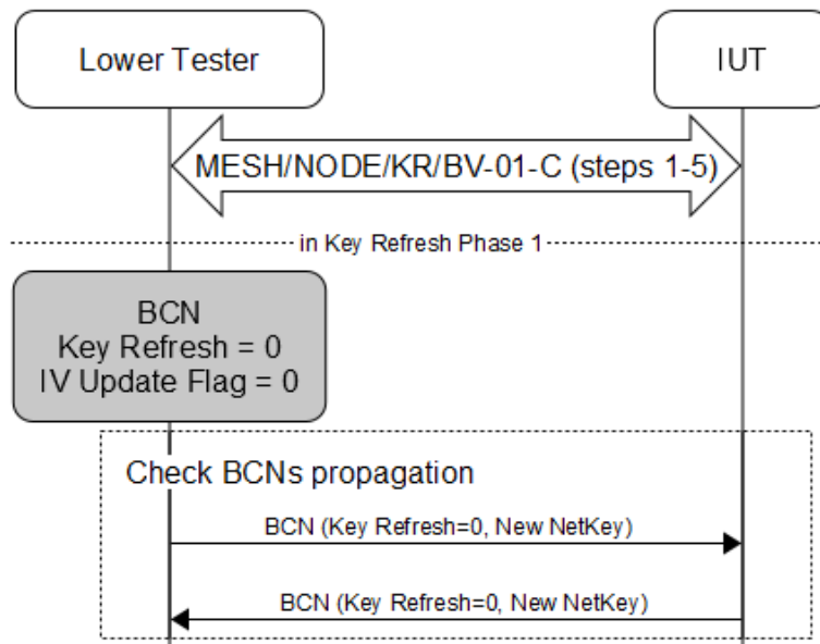
Figure 4.55: MESH/NODE/KR/BV-03-C and MESH/NODE/KR/BV-05-C MSC
