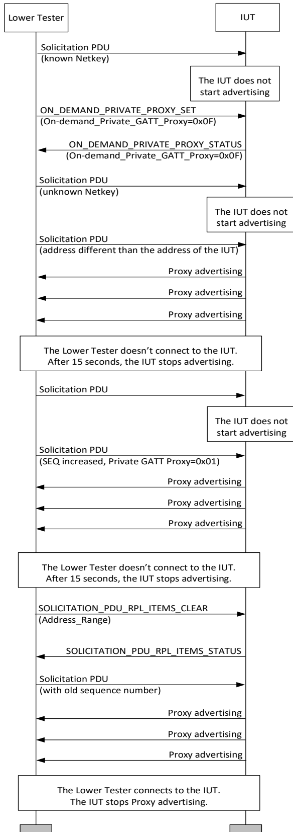
Figure 4.105: Test procedure for MESH/SR/MPXS/BV-12-C MSC
