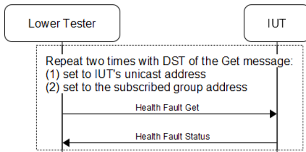
Figure 4.202: MESH/SR/HM/RFS/BV-01-C [Respond to Health Fault Get] MSC
