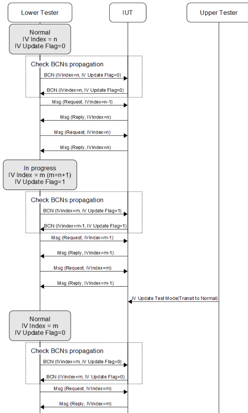
Figure 4.45: MESH/NODE/IVU/BV-01-C and MESH/NODE/IVU/BV-06-C MSC
