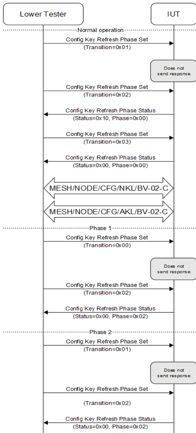
Figure 4.58: MESH/NODE/KR/BI-01-C [Receive Config Key Refresh Phase Set Messages with Valid and Invalid Transition Values] MSC
