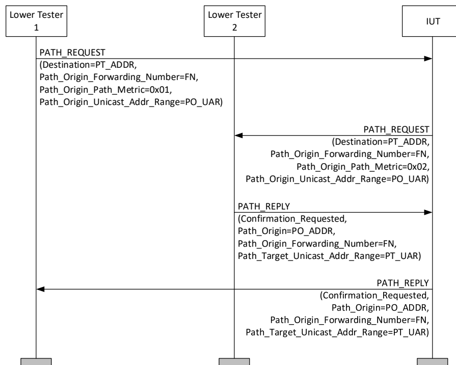
Figure 4.3: Preamble procedure for State: Path Established as Directed Relay, Unicast Address Destination MSC
