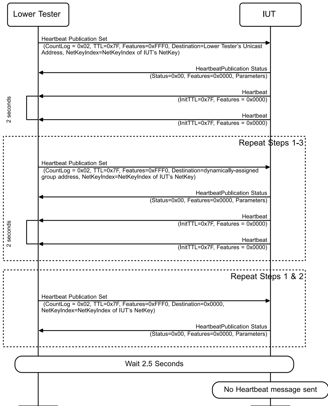
Figure 4.184: MESH/NODE/CFG/HBP/BV-02-C [Periodic publishing of Heartbeat messages] MSC
