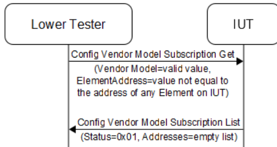
Figure 4.144: MESH/NODE/CFG/SL/BI-09-C [Respond to Config Vendor Model Subscription Get Message (Invalid ElementAddress)] MSC
