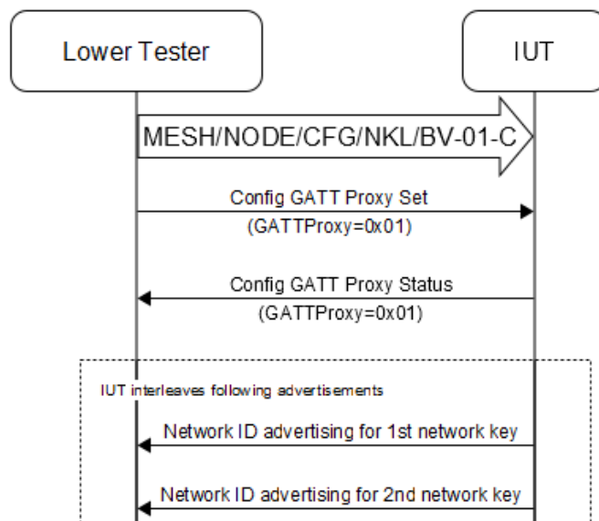
Figure 4.117: MESH/NODE/CFG/GPXY/BV-02-C [Network ID Advertising on Multiple Subnets] MSC
