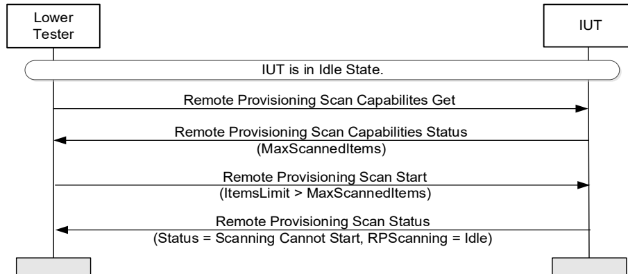
Figure 4.319: Test procedure for MESH/SR/RPR/SCN/BI-02-C MSC
