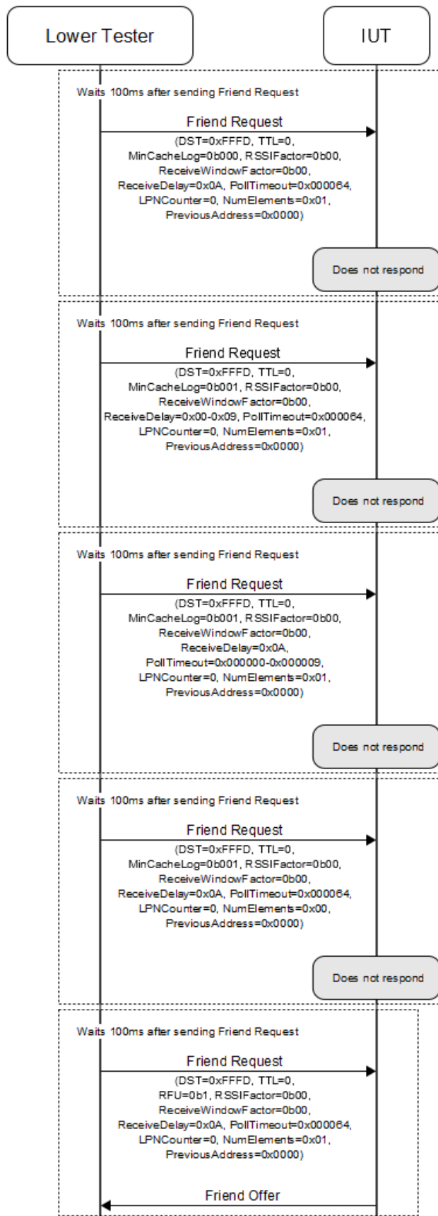
Figure 4.84: MESH/NODE/FRND/FN/BI-03-C [Friendship – Friend Node – Friend Request Invalid RFU Bits] MSC
