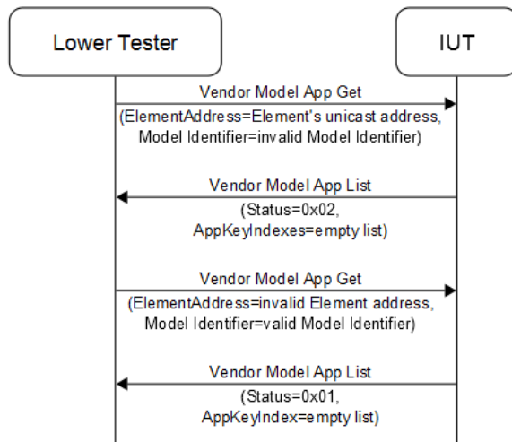
Figure 4.170: MESH/NODE/CFG/MAKL/BI-04-C [Respond to Config Vendor Model App Get Message with Invalid Values] MSC
