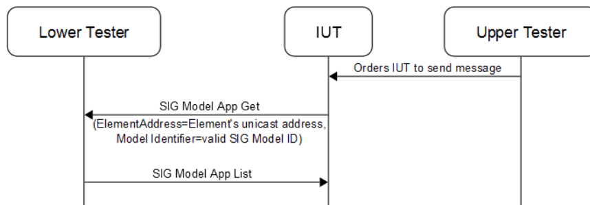
Figure 4.173: MESH/CFGCL/CFG/MAKL/BV-03-C [Send Config SIG Model App Get Messages] MSC
