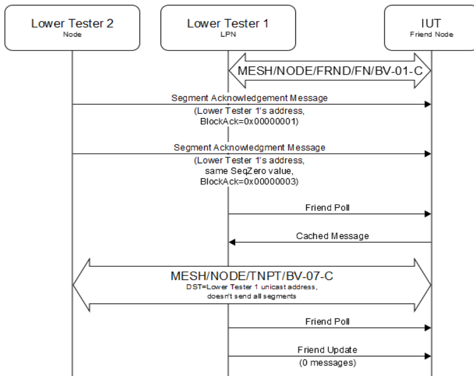
Figure 4.75: MESH/NODE/FRND/FN/BV-17-C [Friendship – Friend Node – SAR Interruption] MSC
