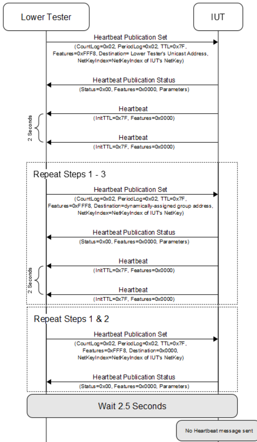
Figure 4.184: MESH/NODE/CFG/HBP/BV-02-C [Periodic publishing of Heartbeat messages] MSC
