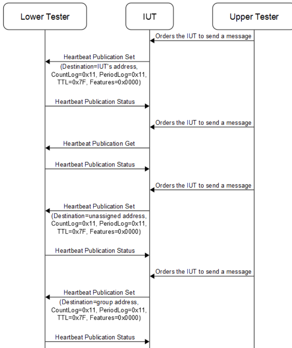
Figure 4.192: MESH/CFGCL/CFG/HBP/BV-01-C [Send Config Heartbeat Publication Set/Get Messages] MSC
