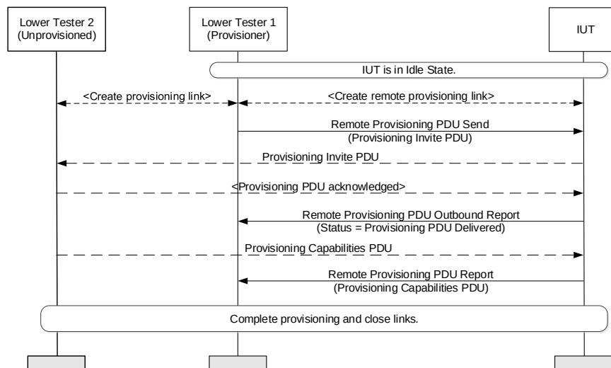
Figure 4.334: Test procedure – Provision an Unprovisioned Device MSC
