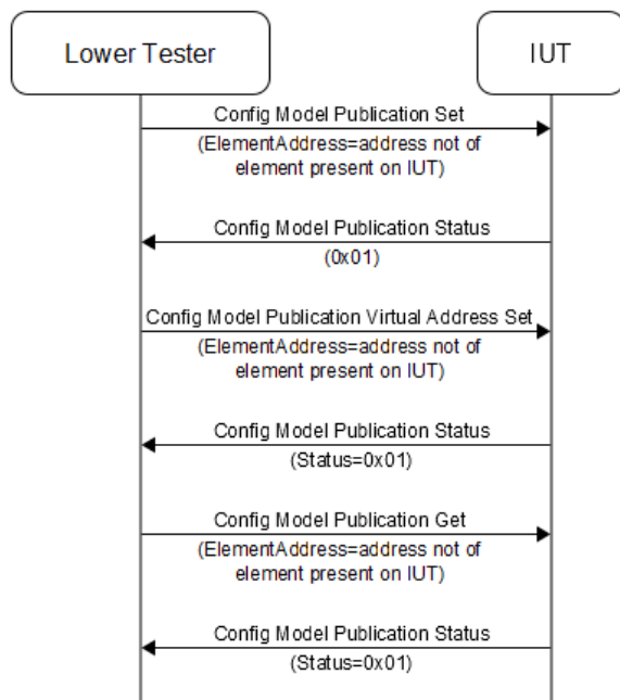
Figure 4.128: MESH/NODE/CFG/MP/BI-01-C [Respond to Config Model Publication Get/Set/Virtual Address Set Messages (Invalid ElementAddress)] MSC
