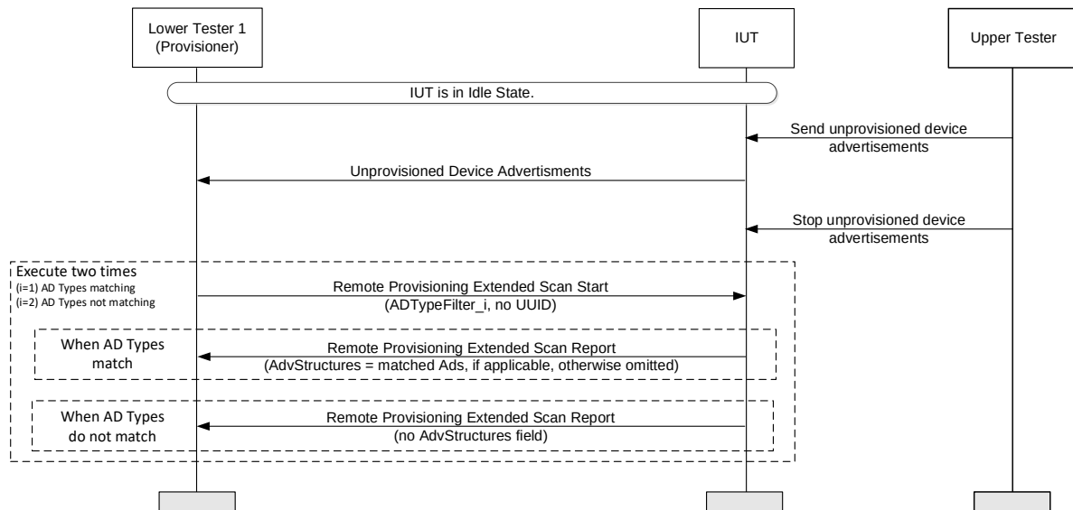
Figure 4.315: Test procedure for MESH/SR/RPR/SCN/BV-06-C MSC
