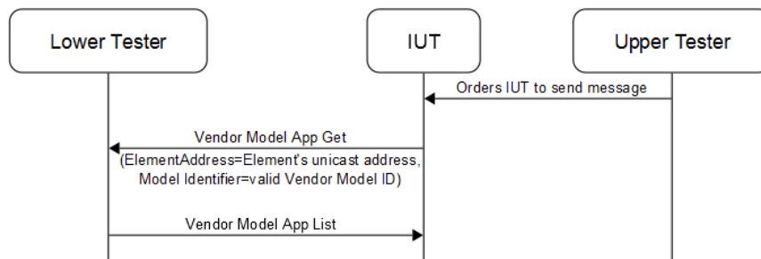
Figure 4.174: MESH/CFGCL/CFG/MAKL/BV-04-C [Send Config Vendor Model App Get Messages] MSC
