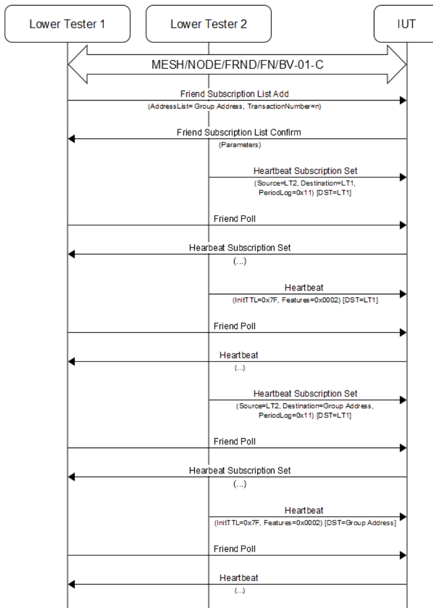
Figure 4.197: MESH/NODE/CFG/HBS/BV-05-C [Receive Heartbeat messages – Friendship] MSC
