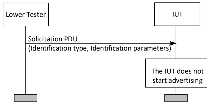
Figure 4.106: Test procedure for MESH/SR/MPXS/BV-13-C MSC
