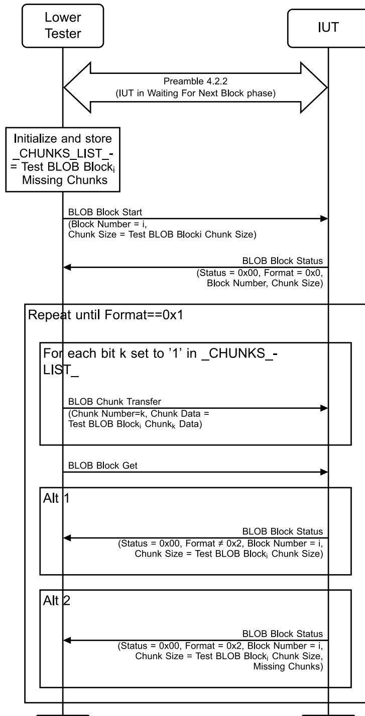
Figure 4.5: MBTM/SR/BT/BV-01-C [Transfer Block Sequence, Push BLOB Transfer Mode]
