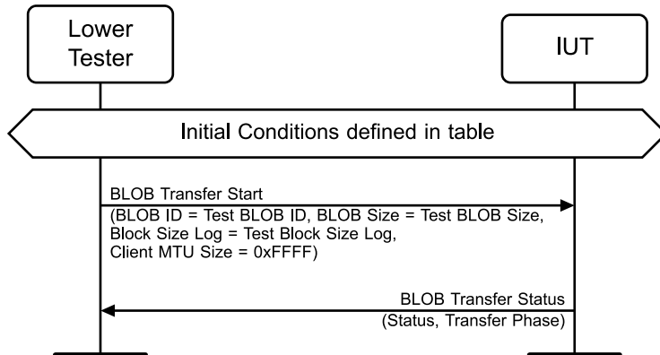
Figure 4.16: Receive BLOB Transfer Start
