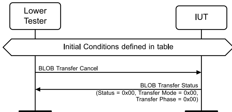
Figure 4.15: Receive BLOB Transfer Cancel
