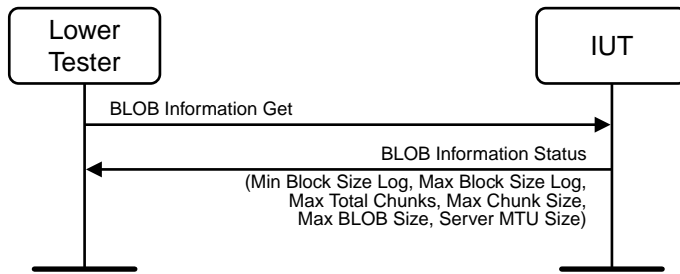
Figure 4.7: MBTM/SR/BT/BV-03-C [BLOB Capabilities]
