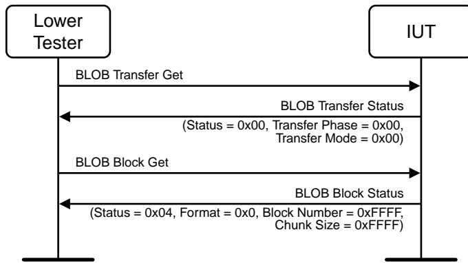
Figure 4.23: MBTM/SR/BT/BV-35-C [BLOB Transfer Server State – Default Values]
