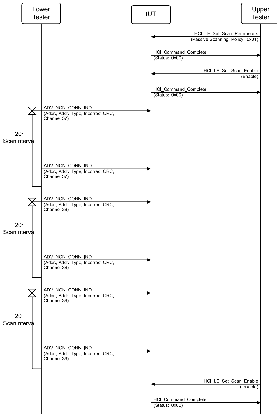
Figure 4.2-109: LL/DDI/SCN/BI-02-C [Passive Scanning: Invalid CRC] MSC
