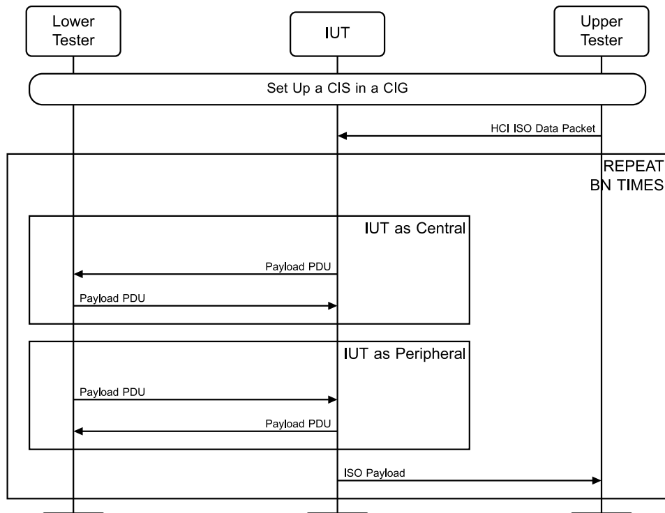
Figure 4.10-50: Sending and Receiving Data in Bidirectional CIS MSC
