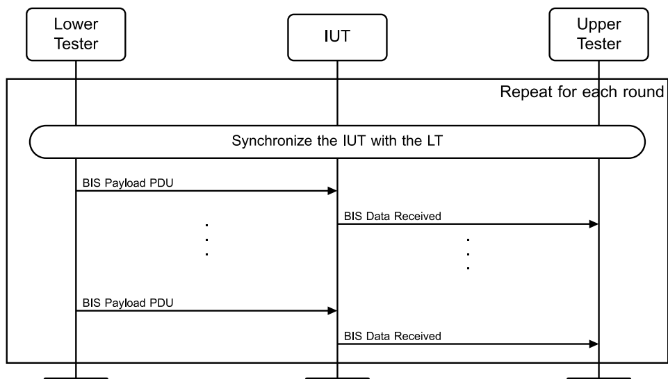
Figure 4.11-17: LL/BIS/SNC/BV-07-C [Bursting of Packets in Broadcast Isochronous Stream] MSC
