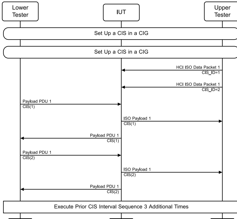
Figure 4.10-40: LL/CIS/PER/BV-32-C [Sending and Receiving Data in Multiple CIsEs, Single CIG, Single Connection, Interleaved CIG, Peripheral, BN=1] MSC
