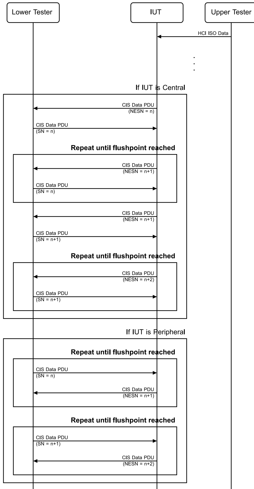
Figure 4.10-61: CIS ACK Scheme and FlushTimeout MSC
