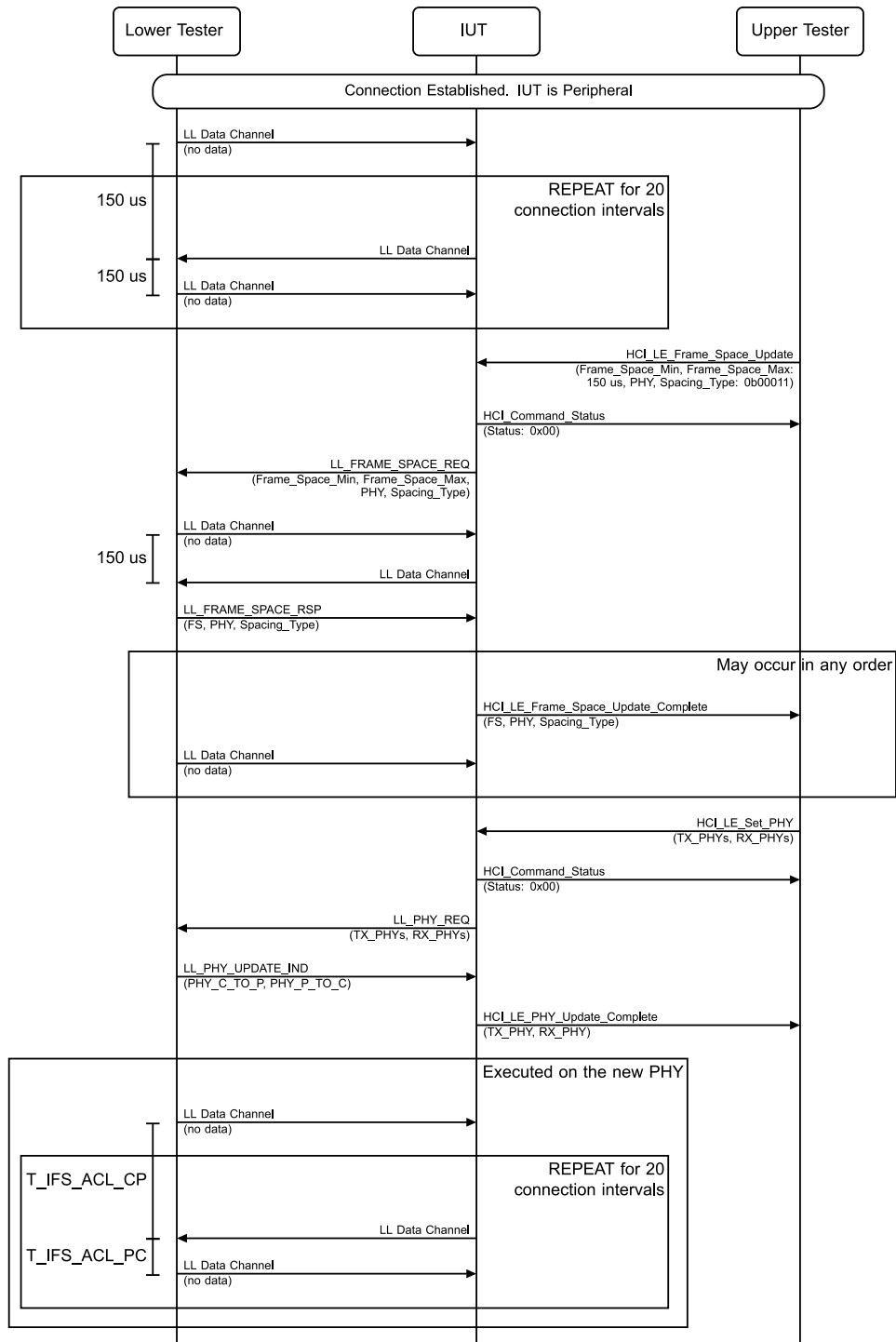
Figure 4.4-20: Initiate Inter Frame Space Change on a Different PHY, Peripheral MSC
