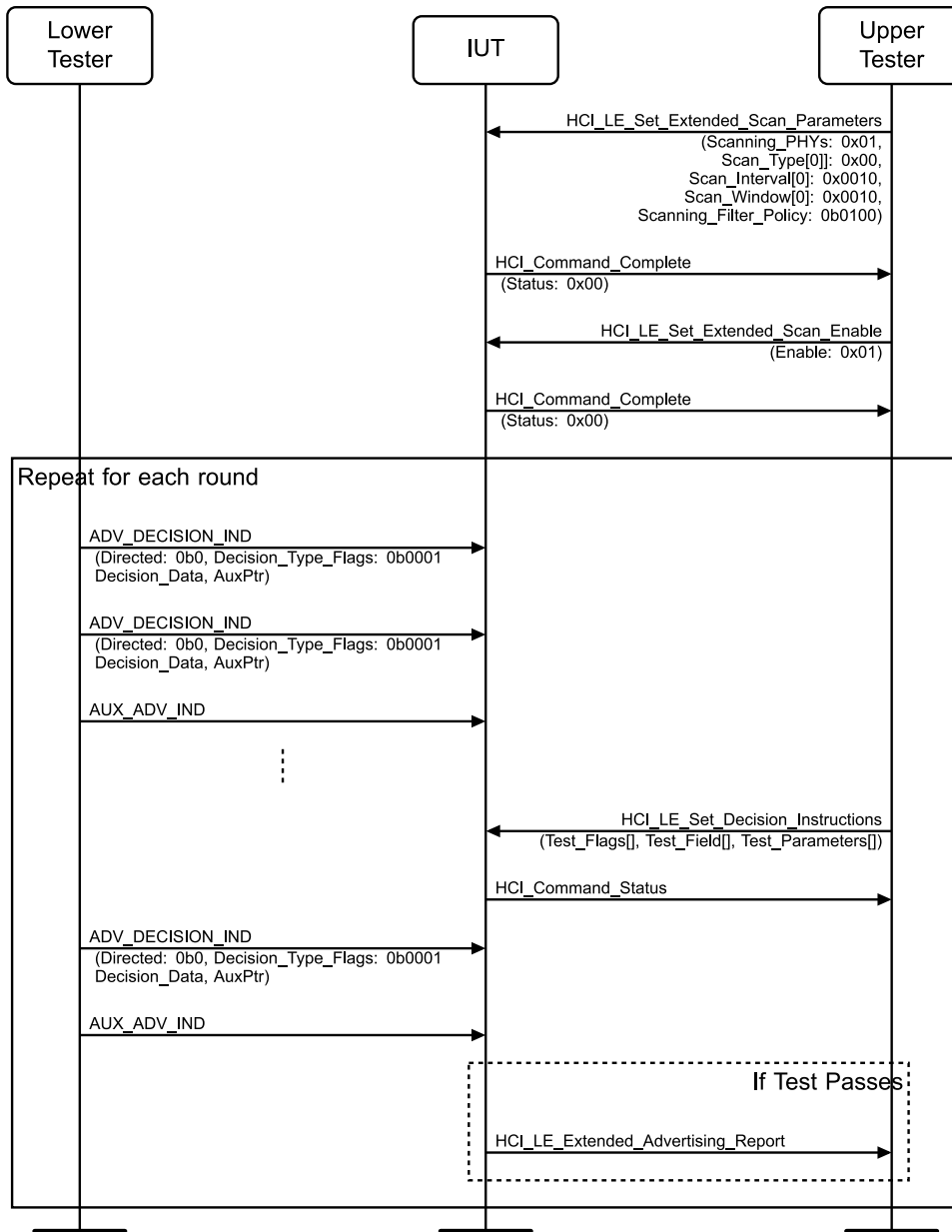
Figure 4.2-138: Decision-Based Advertisements, RSSI and Path Loss MSC
