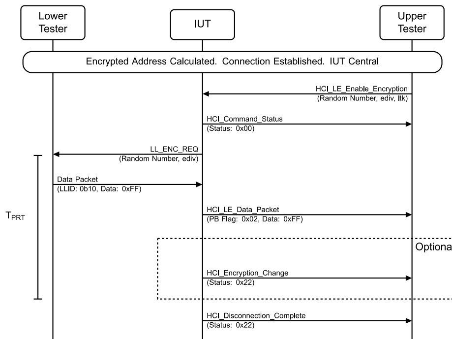
Figure 4.8-59: LL/SEC/CEN/BI-08-C [Central Encryption: Sending Data and Not Response] MSC
