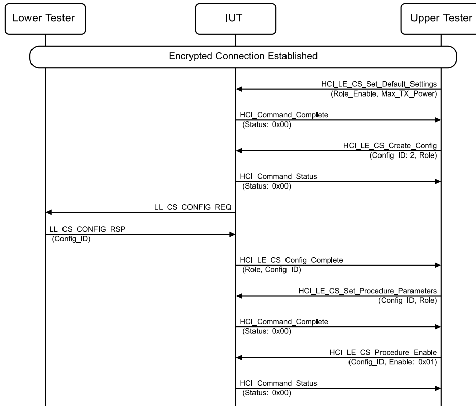
Figure 4.14-19: Initiate CS Start Procedure MSC – Page 1 of 2
