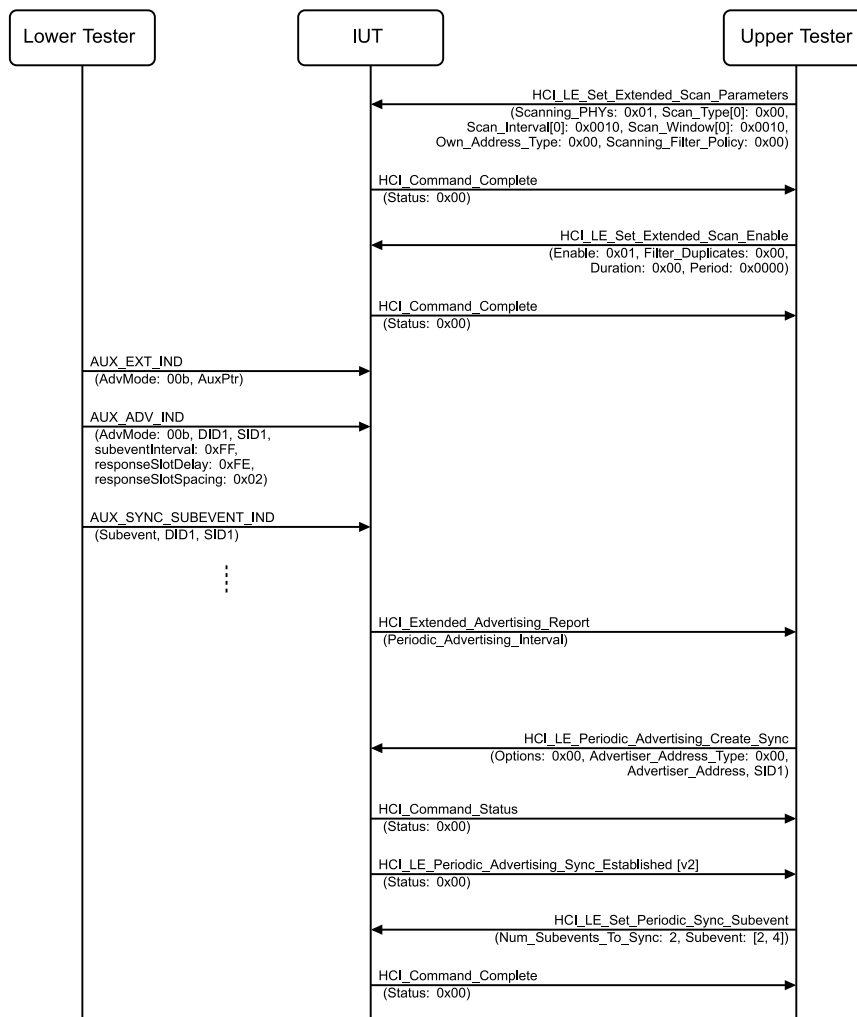
Figure 4.2-132: Sync with a Periodic Advertiser, Send Response Data in Future Subevent, Scanner MSC – Page 1 of 2
