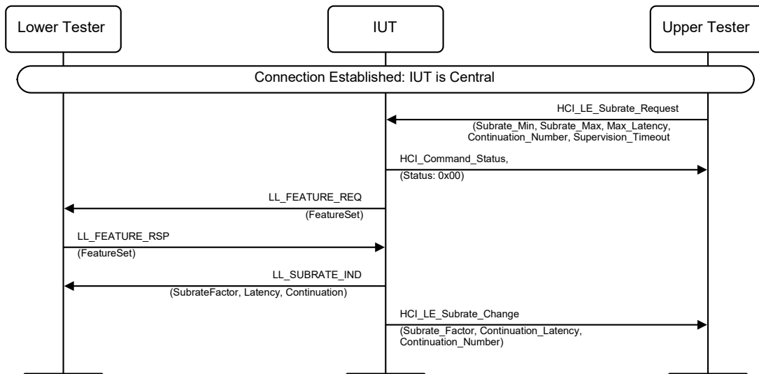
Figure 4.3-197: LL/CON/CEN/BV-136-C [Feature Exchange Before a Subrate Request] MSC
