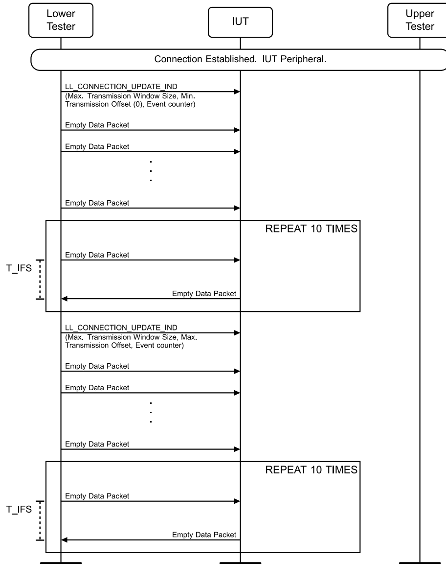
Figure 4.4-4: LL/TIM/PER/BV-01-C [Adjusting Anchor Point] MSC
