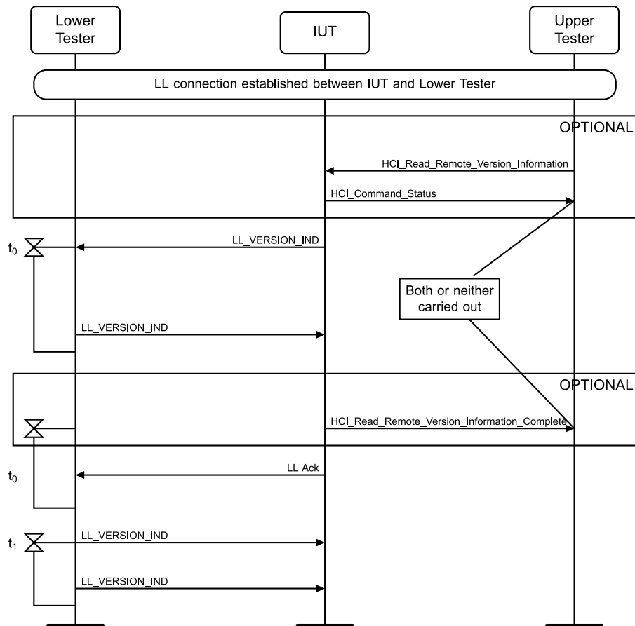
Figure 4.3-253: Version Exchange, IUT Requesting MSC
