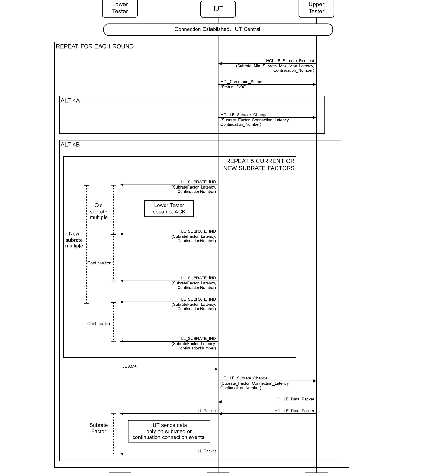
Figure 4.3-199: LL/CON/CEN/BV-138-C [Central Retransmission on Old and New Subrate when Connection Subrate Update Not Acknowledged] MSC
