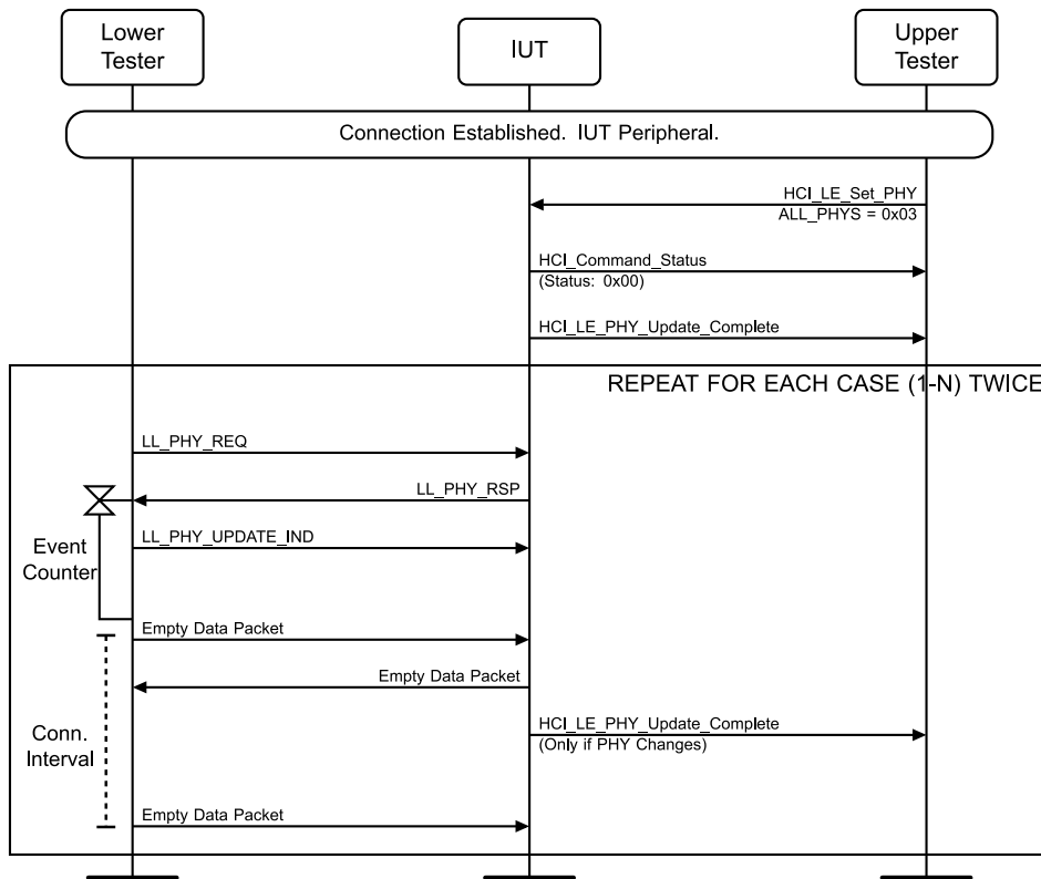
Figure 4.3-77: LL/CON/PER/BV-42-C [Responding to PHY Update Procedure] MSC
