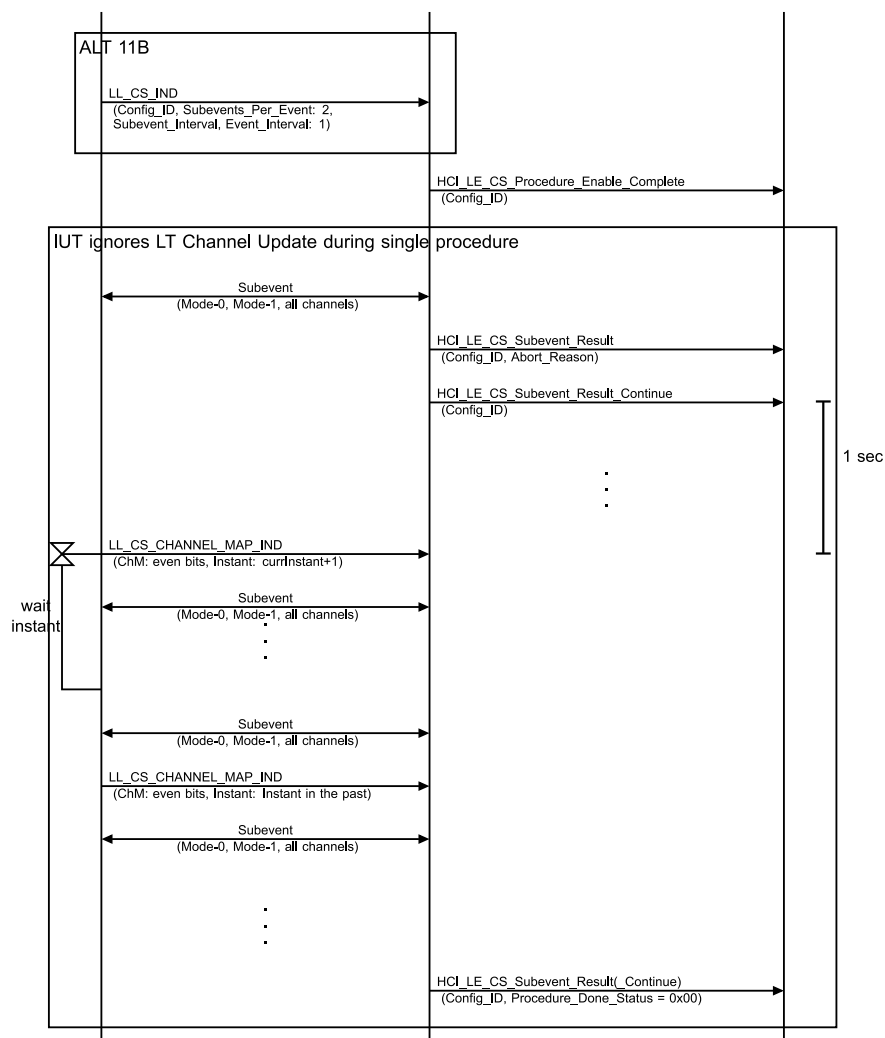
Figure 4.14-34: Channel Sounding Procedure Terminate, Channel Map Update in the Past, Initiating CS Procedure MSC – Page 2 of 4
