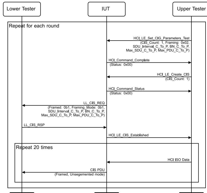
Figure 4.10-24: Max PDU Value, Framed, Unsegmented Mode MSC
