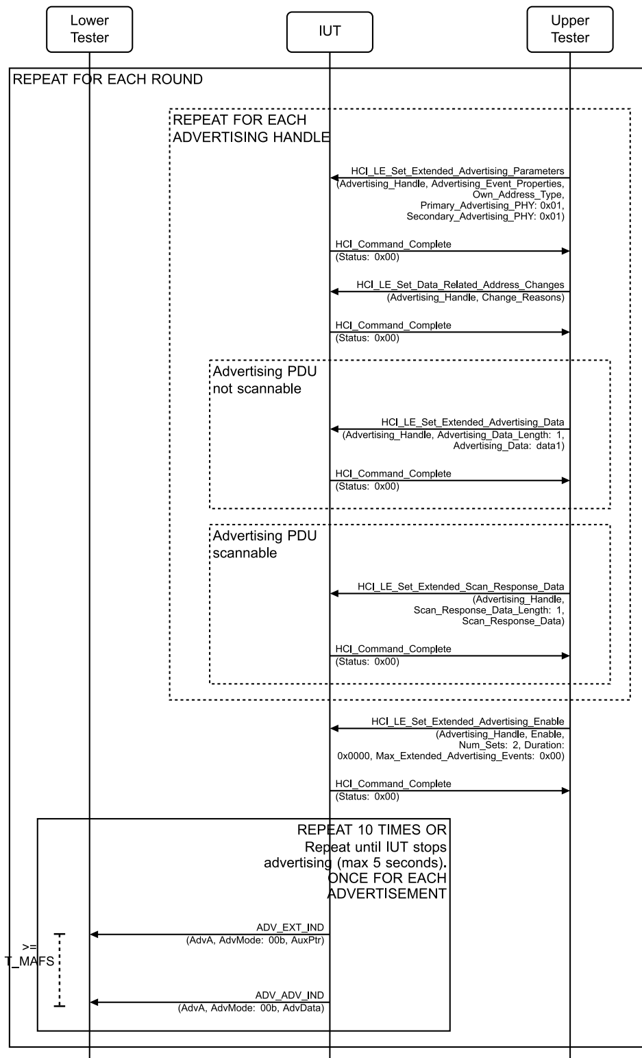
Figure 4.2-56: Extended Advertising, Multiple Sets, New RPA on AdvData Change MSC – Page 1 of 4
