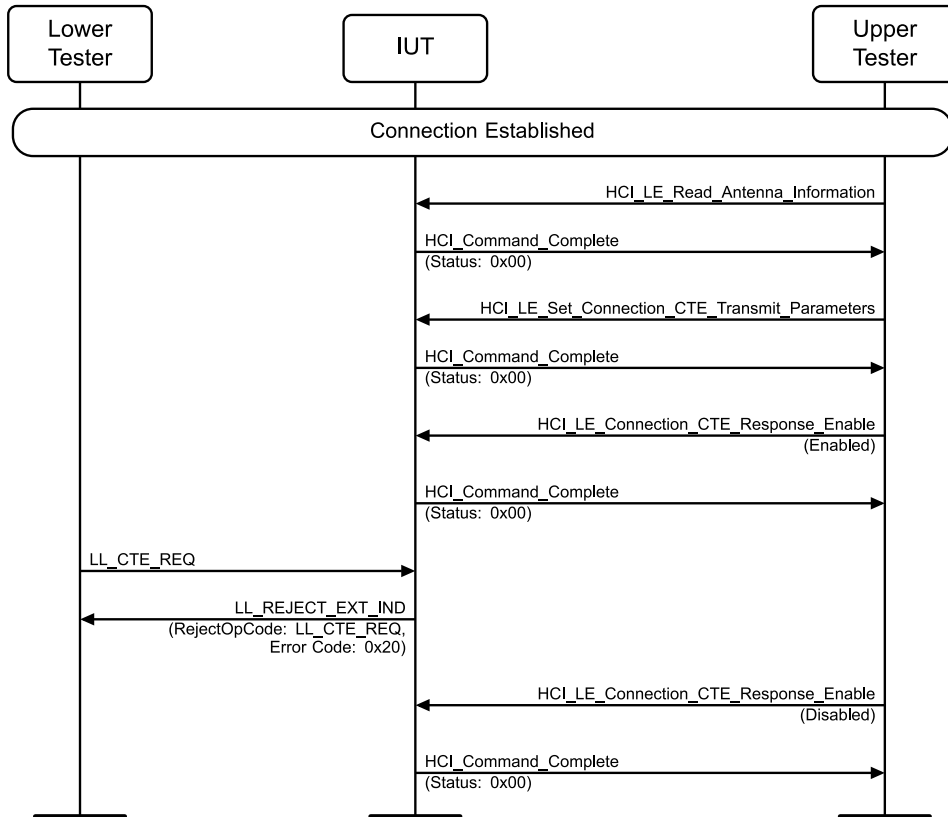
Figure 4.3-213: Constant Tone Extension Request Procedure, IUT Responding, Unsupported MSC
