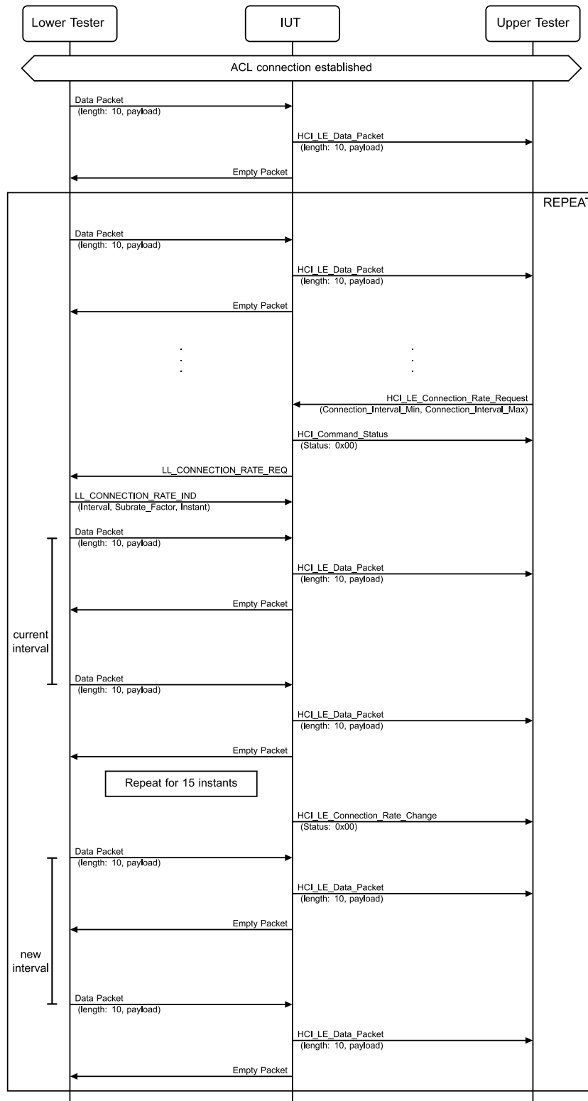
Figure 4.3-130: LL/CON/PER/BV-178-C [Initiate a Connection Rate Request, Peripheral] MSC
