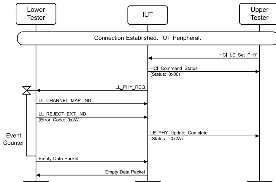
Figure 4.3-80: LL/CON/PER/BV-46-C [Handling Protocol Collision – Different Procedure – Channel Map] MSC
