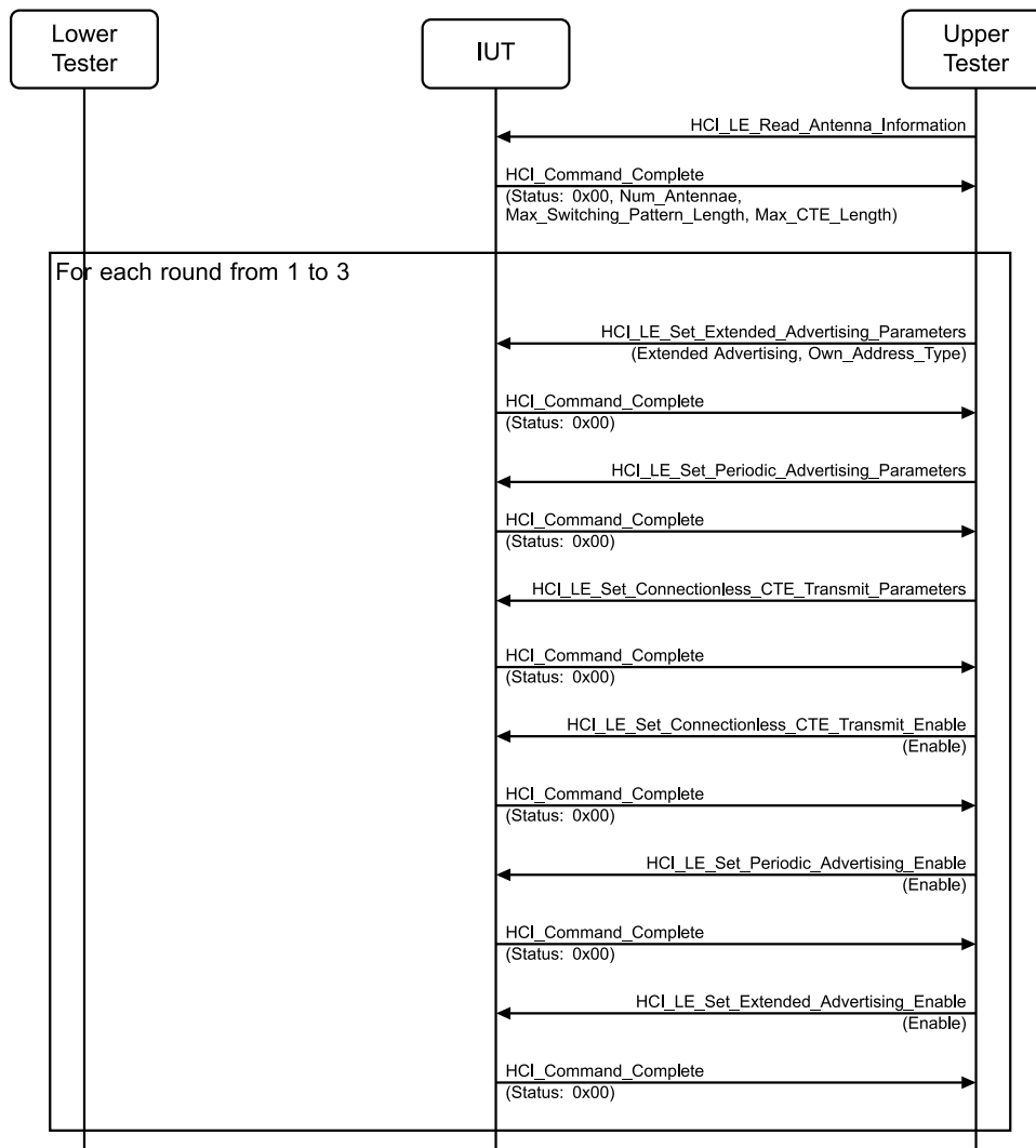
Figure 4.2-37: AoA Connectionless CTE Advertising MSC – Page 1 of 2
