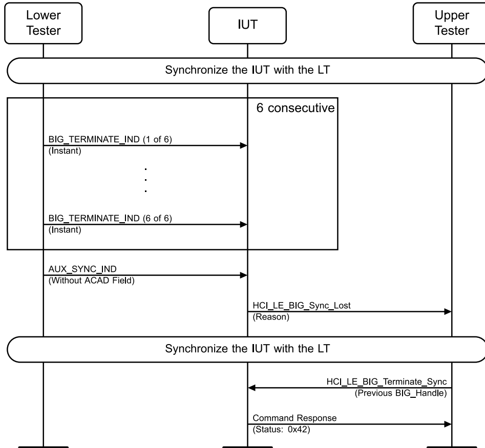
Figure 4.11-20: Broadcast Isochronous Stream Termination MSC
