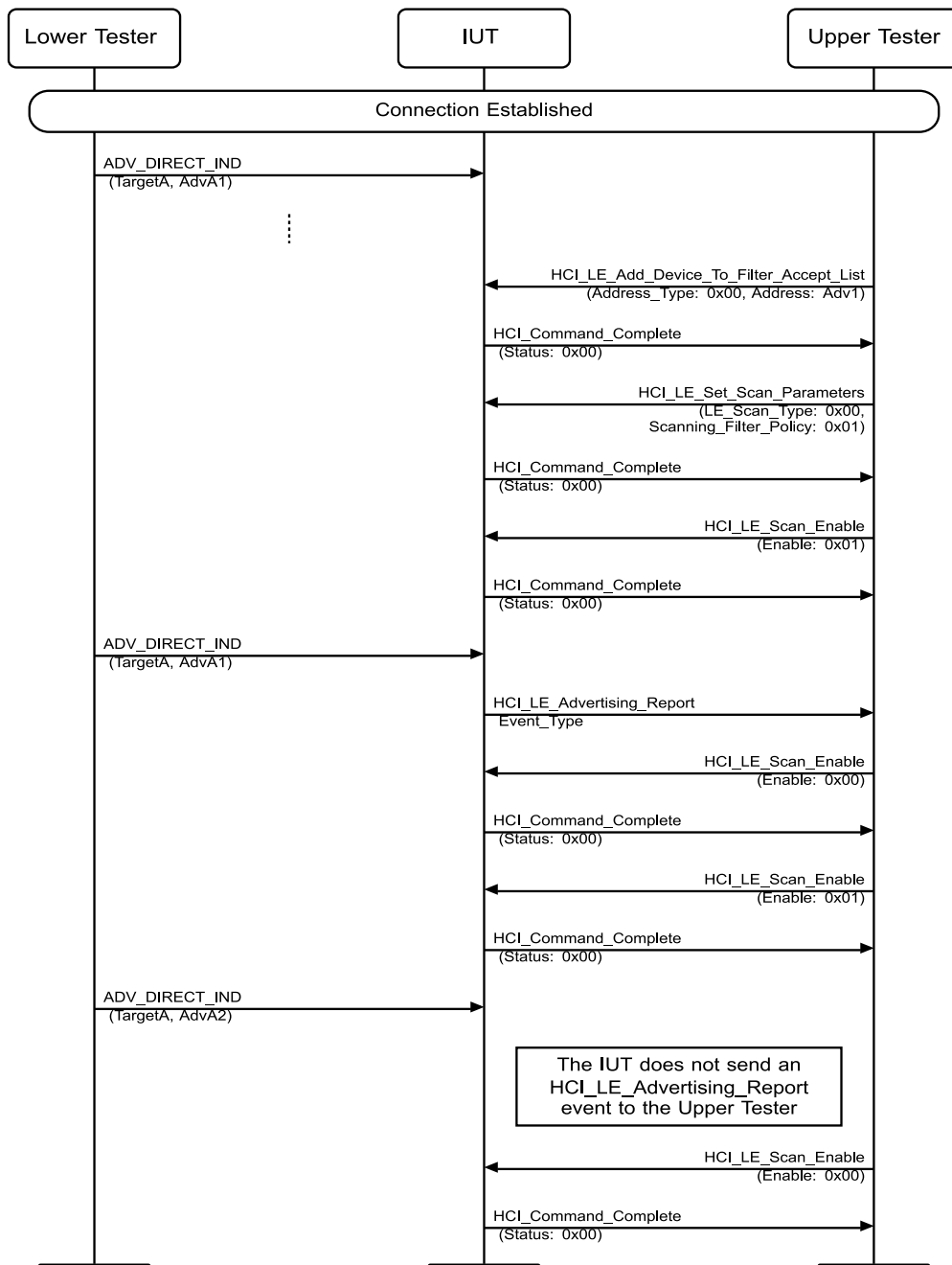
Figure 4.2-125: LL/DDI/SCN/BV-90-C [Ignore Directed Advertising, Address Not In Filter Accept List] MSC
