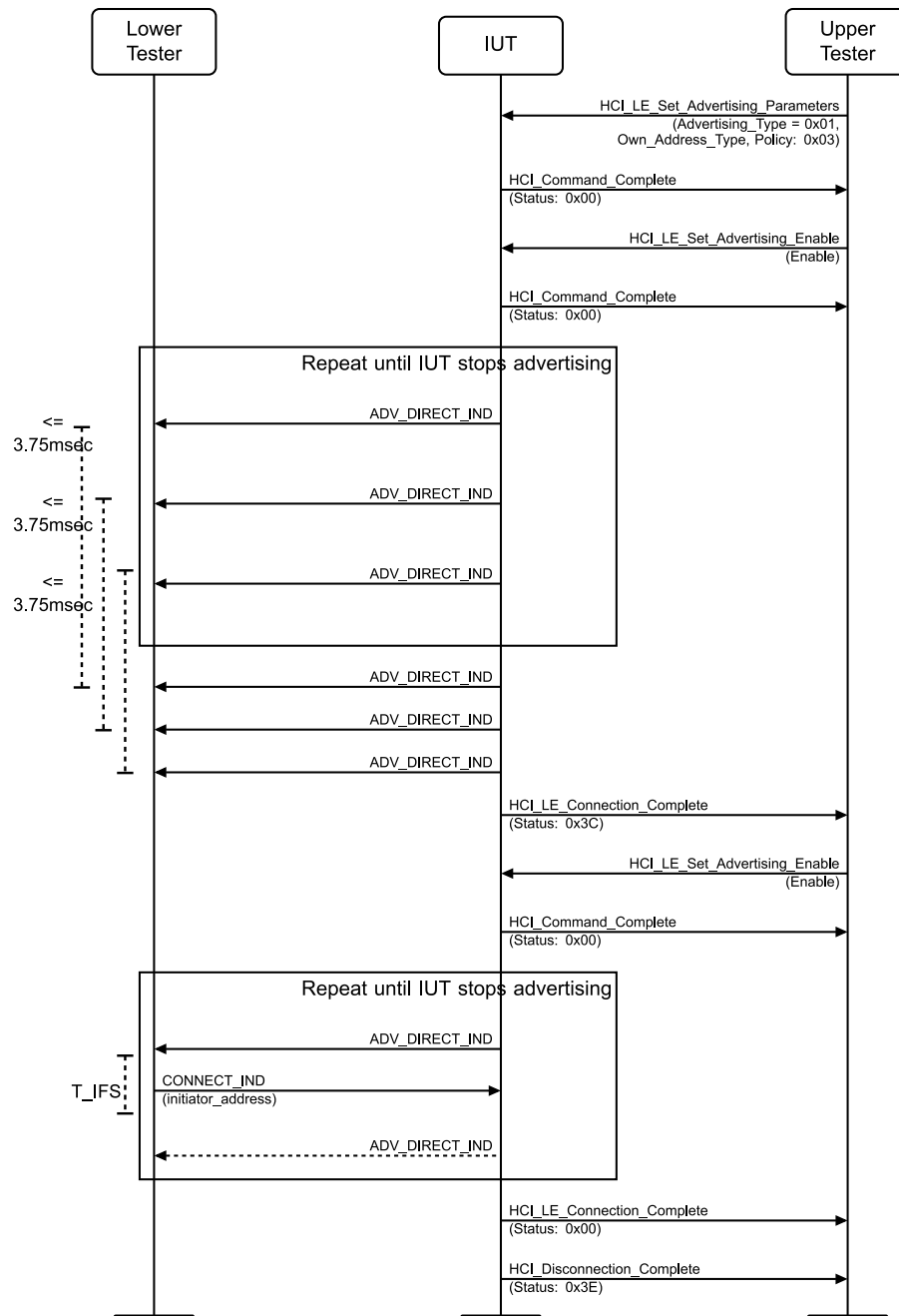
Figure 4.2-8: LL/DDI/ADV/BV-11-C [Directed Advertising Events, Extended Advertising not supported] MSC
