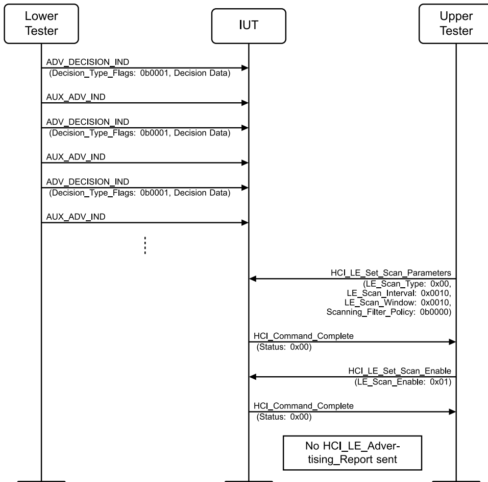
Figure 4.2-140: LL/DDI/SCN/BV-104-C [Decision-Based Advertisements Ignored, Legacy Scanning] MSC
