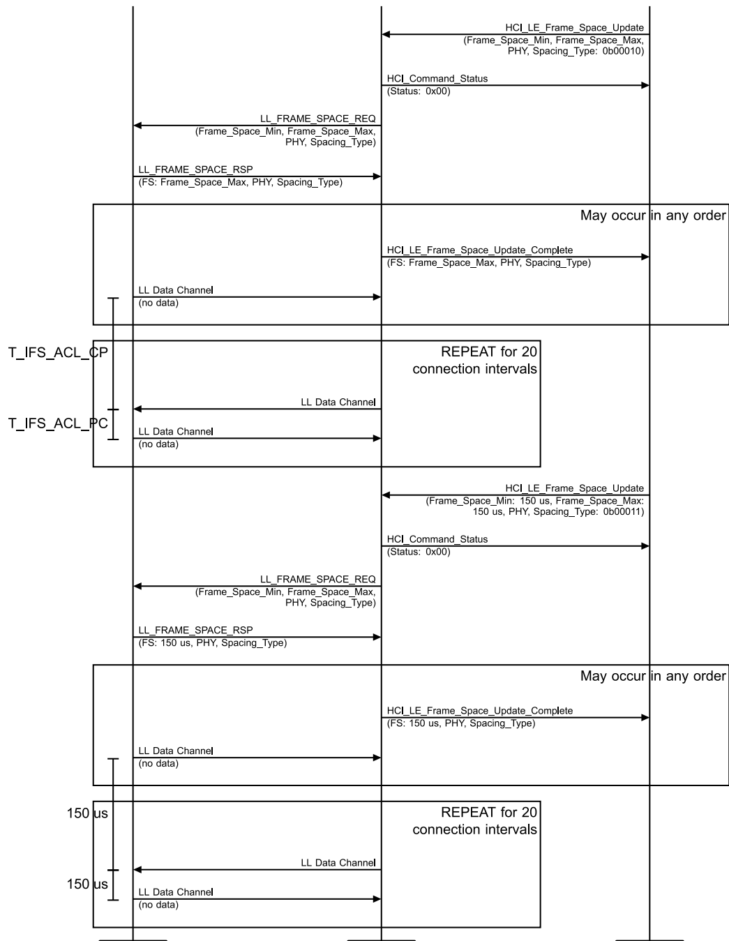
Figure 4.4-14: Initiate Inter Frame Space Change in the current ACL connection, Symmetric PHYs, Peripheral MSC – Page 2 of 2
