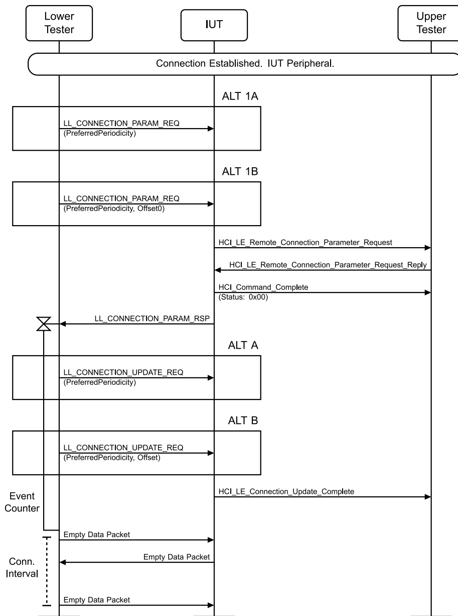
Figure 4.3-73: Accepting Connection Parameter Request – Preferred_Periodicity MSC
