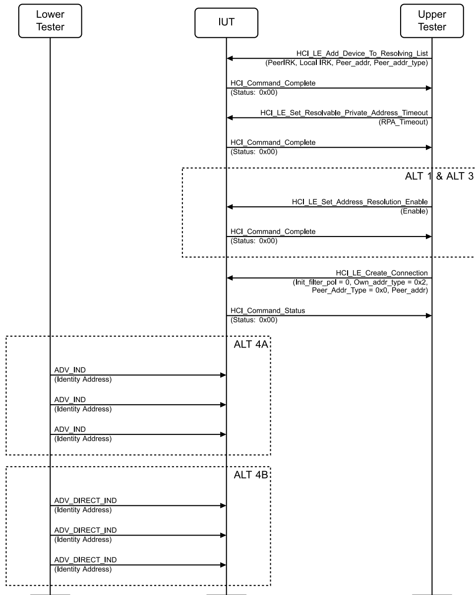
Figure 4.3-34: Network Privacy – Connection Establishment using resolving list, Initiator, Ignore Identity Address MSC
