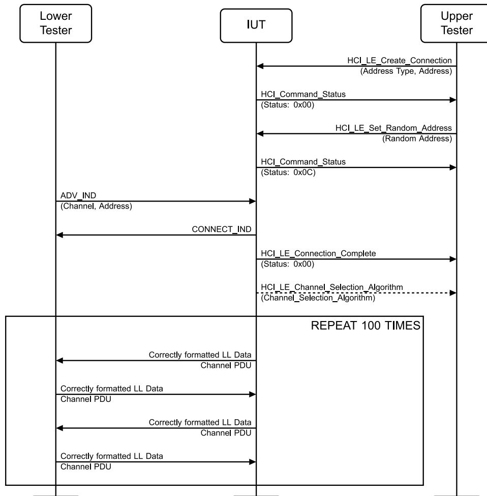
Figure 4.3-21: Connection Initiation MSC
