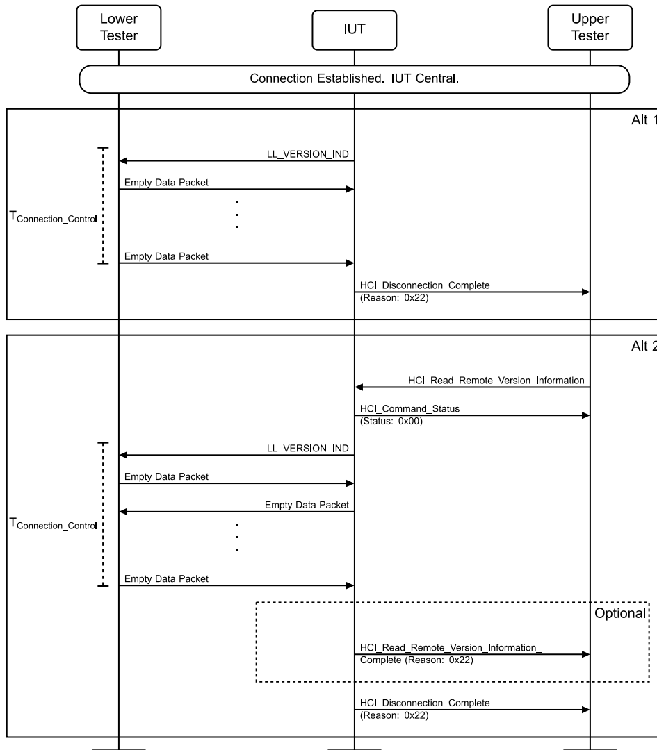
Figure 4.3-191: LL/CON/CEN/BI-04-C [Central Connection Control Timer] MSC
