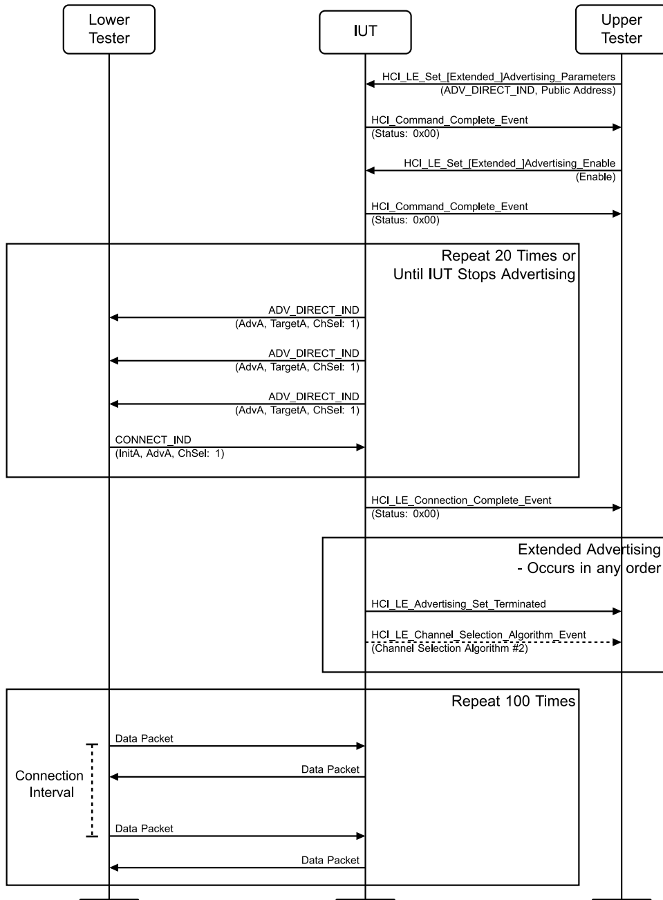
Figure 4.3-12: Directed Advertising Connection, Channel Selection Algorithm #2 MSC
