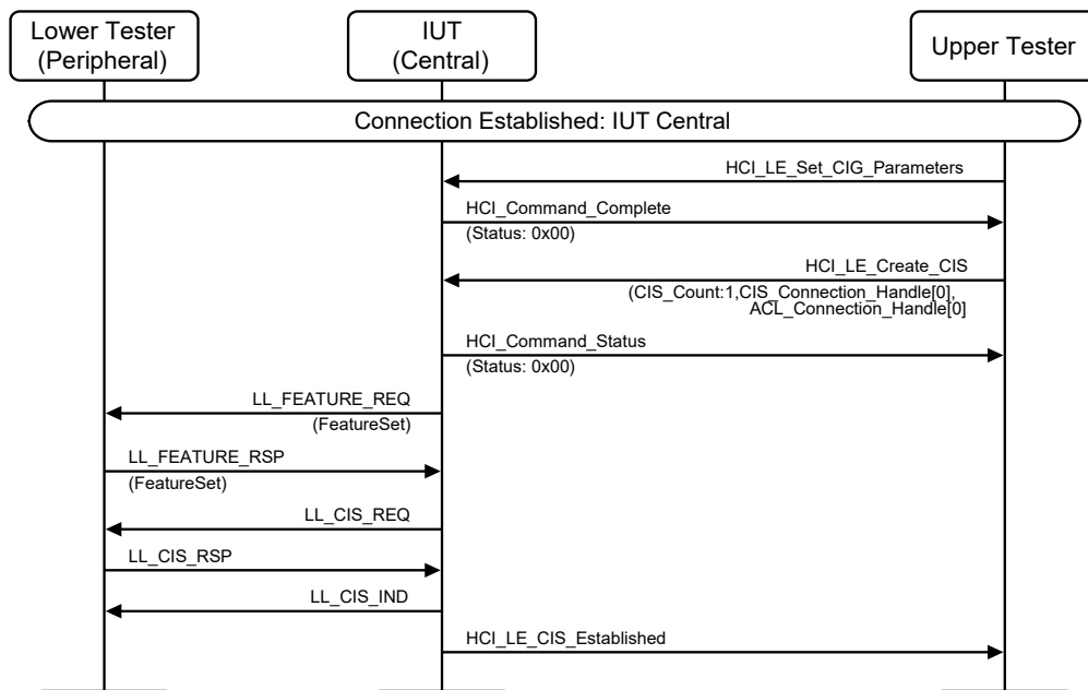
Figure 4.10-23 LL/CIS/CEN/BV-56-C [Feature Exchange Before a CIS Connect Request] MSC
