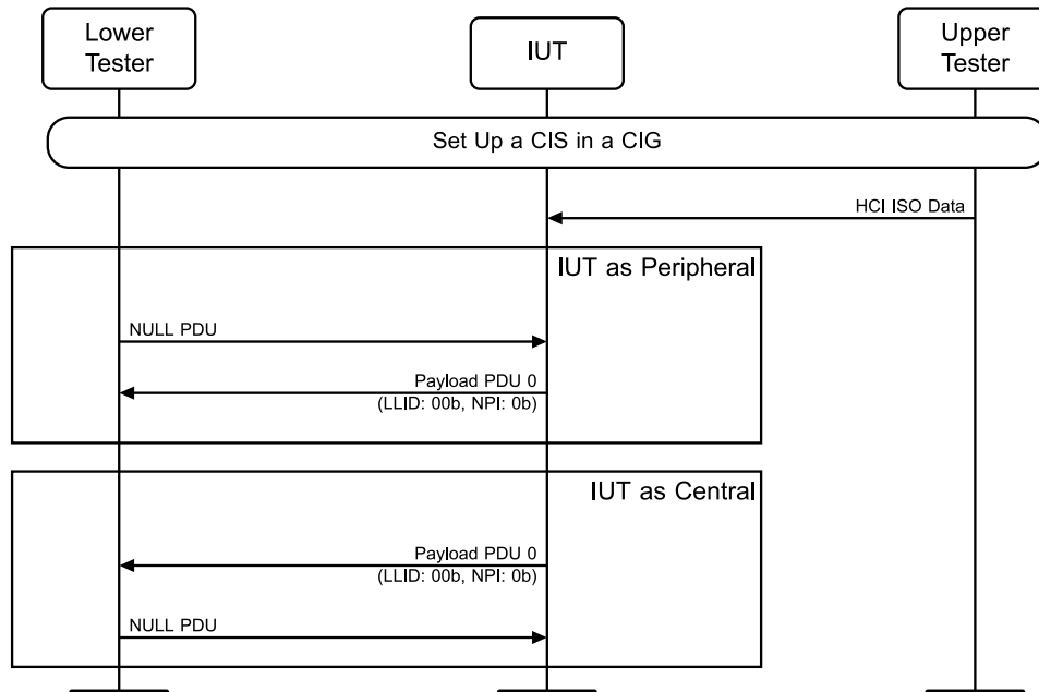
Figure 4.10-57: Sending Data in Unidirectional CIS, BN = 1 MSC
