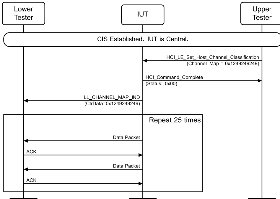
Figure 4.10-4: New Channel Map MSC
