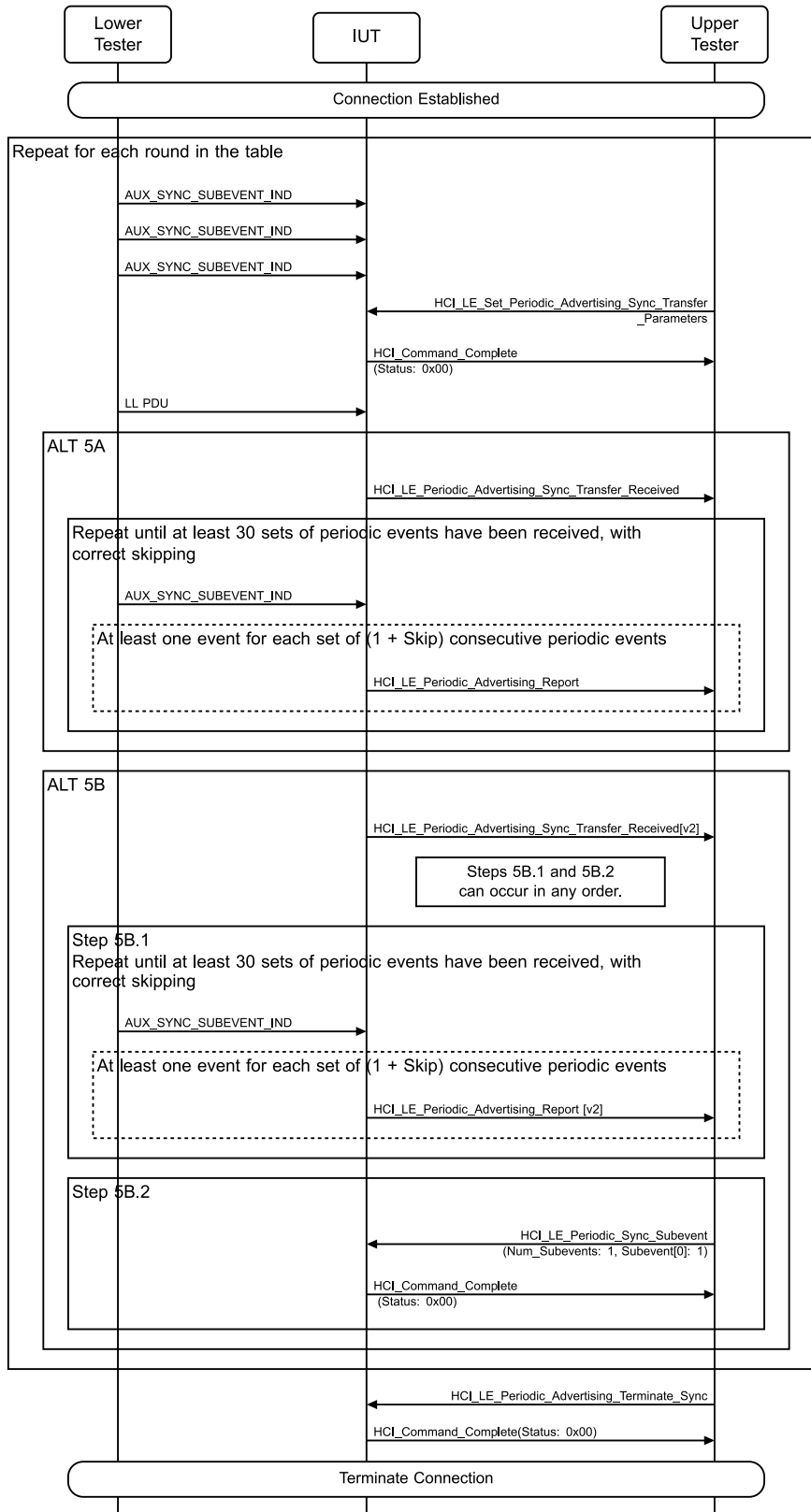
Figure 4.3-217: Periodic Advertising Sync Transfer Procedure, Accepting – Skipping Events MSC
