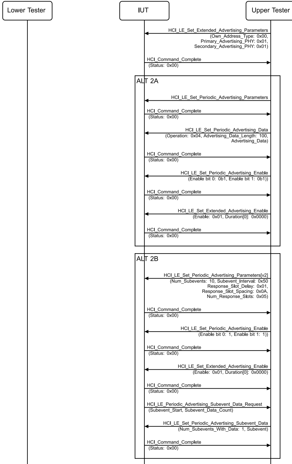
Figure 4.2-46: ADI in Periodic Advertising when supporting Periodic Advertising Filtering MSC – Page 1 of 2
