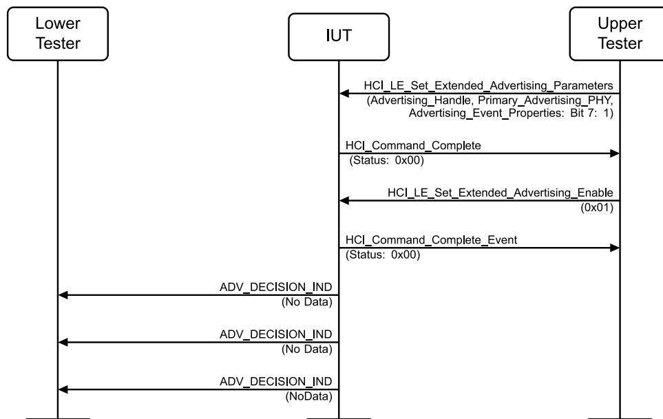
Figure 4.2-74: Decision Advertisements With No Data, Enable Extended Advertisement MSC
