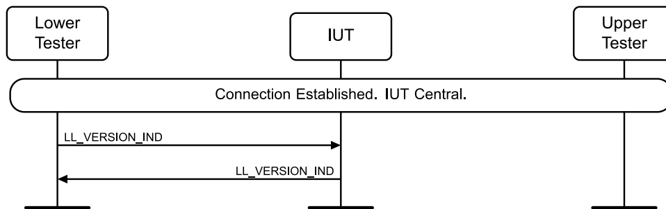
Figure 4.3-150: LL/CON/CEN/BV-21-C [Central Respond Version] MSC
