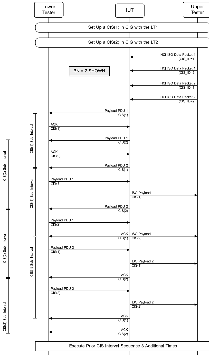
Figure 4.10-10: Sending and Receiving Data in Multiple CISes, Single CIG, Single Connection, Interleaved CIG, Central MSC
