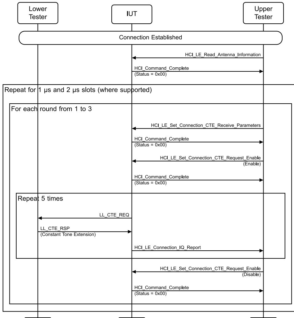
Figure 4.3-234: Constant Tone Extension Request Procedure, IUT Initiated, Periodic MSC
