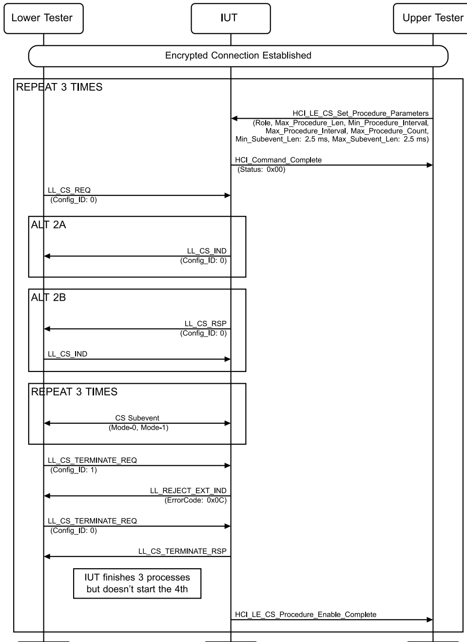
Figure 4.14-32: CS Procedure, Receive Repeat Termination MSC
