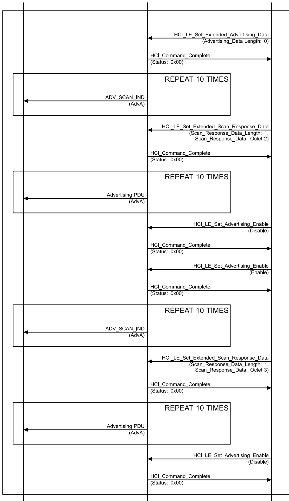
Figure 4.2-55: LL/DDI/ADV/BV-76-C [Extended Scannable Advertising, New RPA on Change Reasons] MSC – Page 2 of 2
