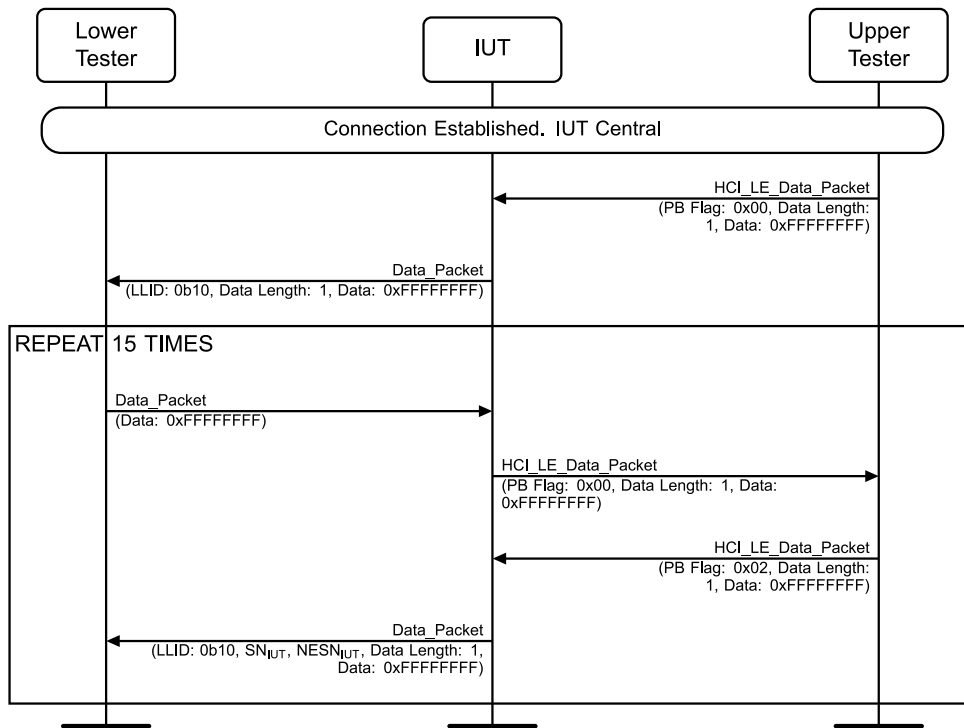
Figure 4.3-151: LL/CON/CEN/BV-22-C [Central Acknowledgement Scheme] MSC
