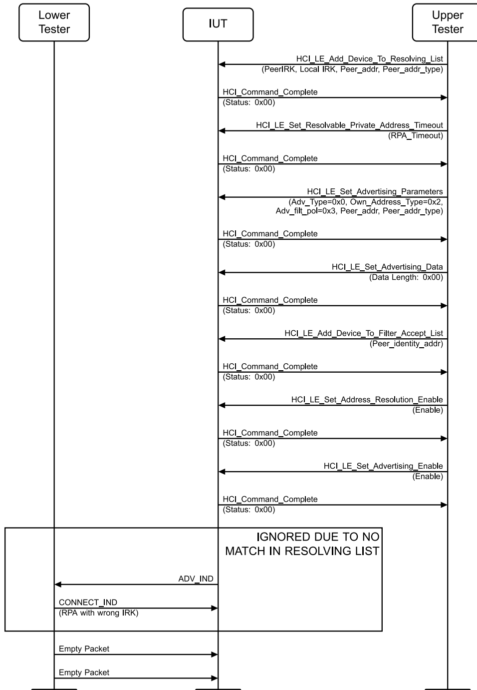
Figure 4.8-10: LL/SEC/ADV/BV-10-C [Network Privacy - Undirected Connectable Advertising using Resolving List and Peer Device Identity not in the List] MSC
