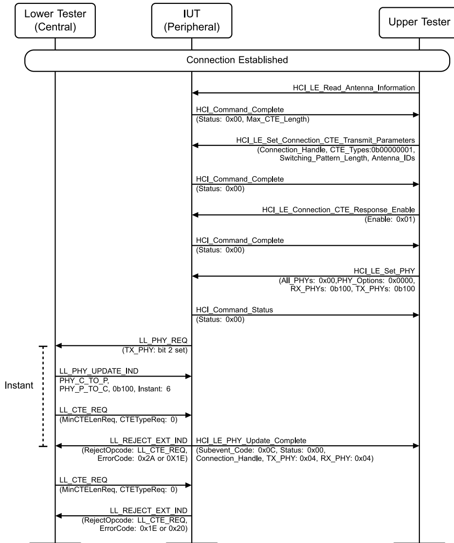
Figure 4.3-126: LL/CON/PER/BV-150-C [Reject Constant Tone Extension Request Procedure for LE Coded PHY, IUT Responding, AoA, Peripheral] MSC
