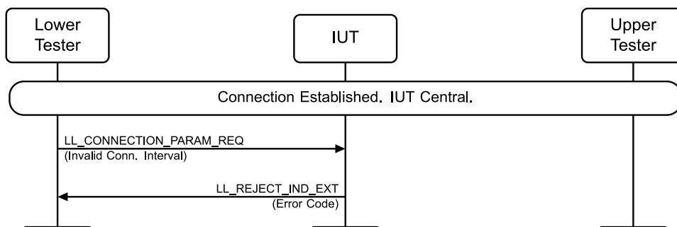
Figure 4.3-193: LL/CON/CEN/BI-06-C [Accepting Connection Parameter Request – illegal parameters] MSC
