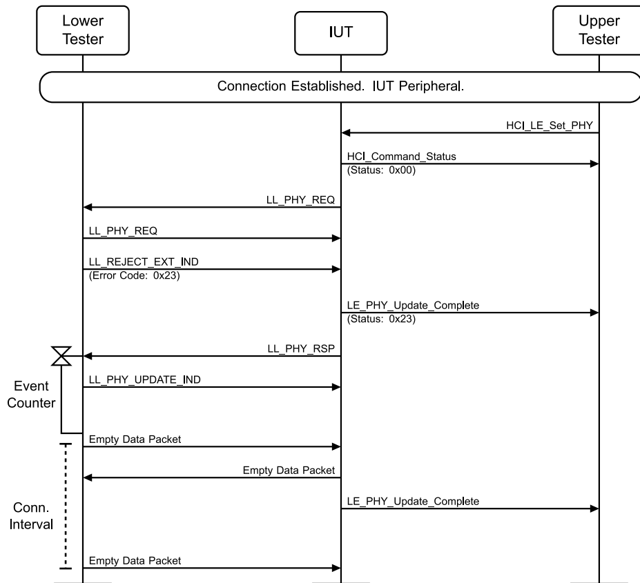
Figure 4.3-78: LL/CON/PER/BV-44-C [Handling Protocol Collision – Same Procedure] MSC
