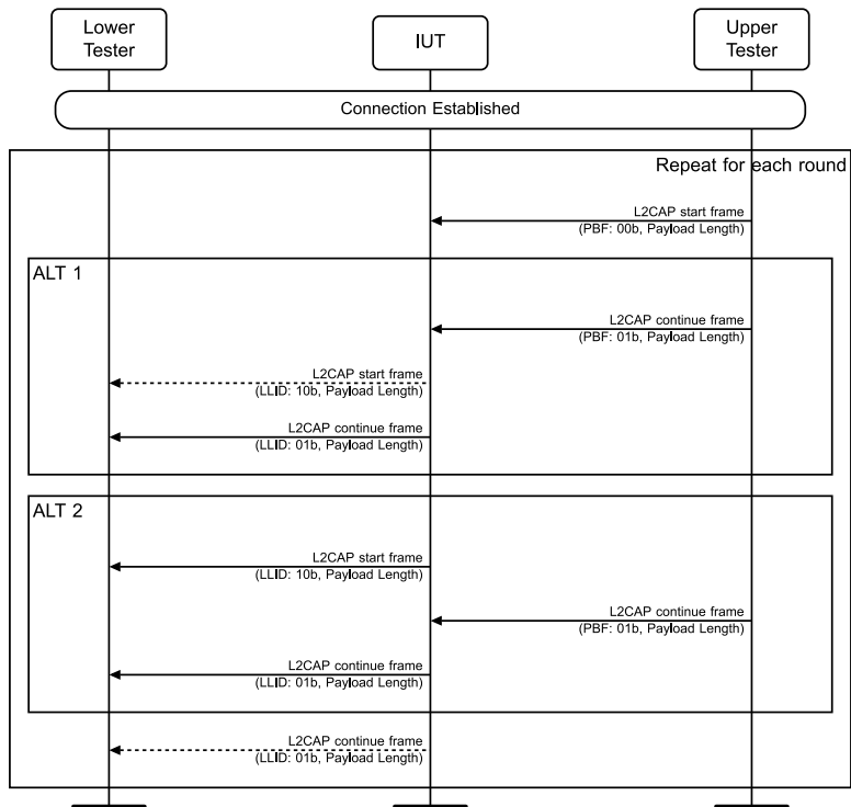
Figure 4.9-1: Transmit Fragmented L2CAP Header MSC
