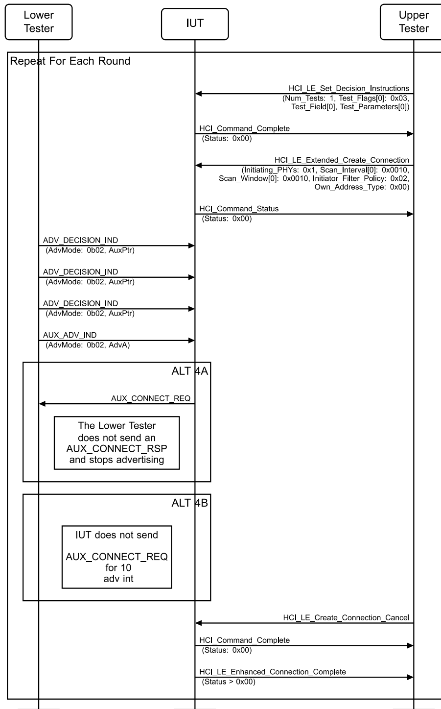
Figure 4.3-45: Extended Scanning, Connection Initiation, Decision-Based Advertising MSC
