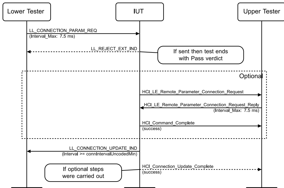
Figure 4.4-44: Frame Space Change, Connection Parameters Request, insufficient time MSC
