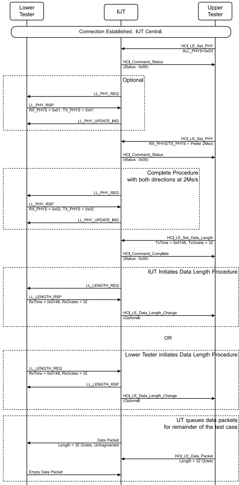
Figure 4.3-171: LL/CON/CEN/BV-49-C [Initiating PHY Update Procedure – Packet Time Restrictions] MSC – Page 1 of 2
