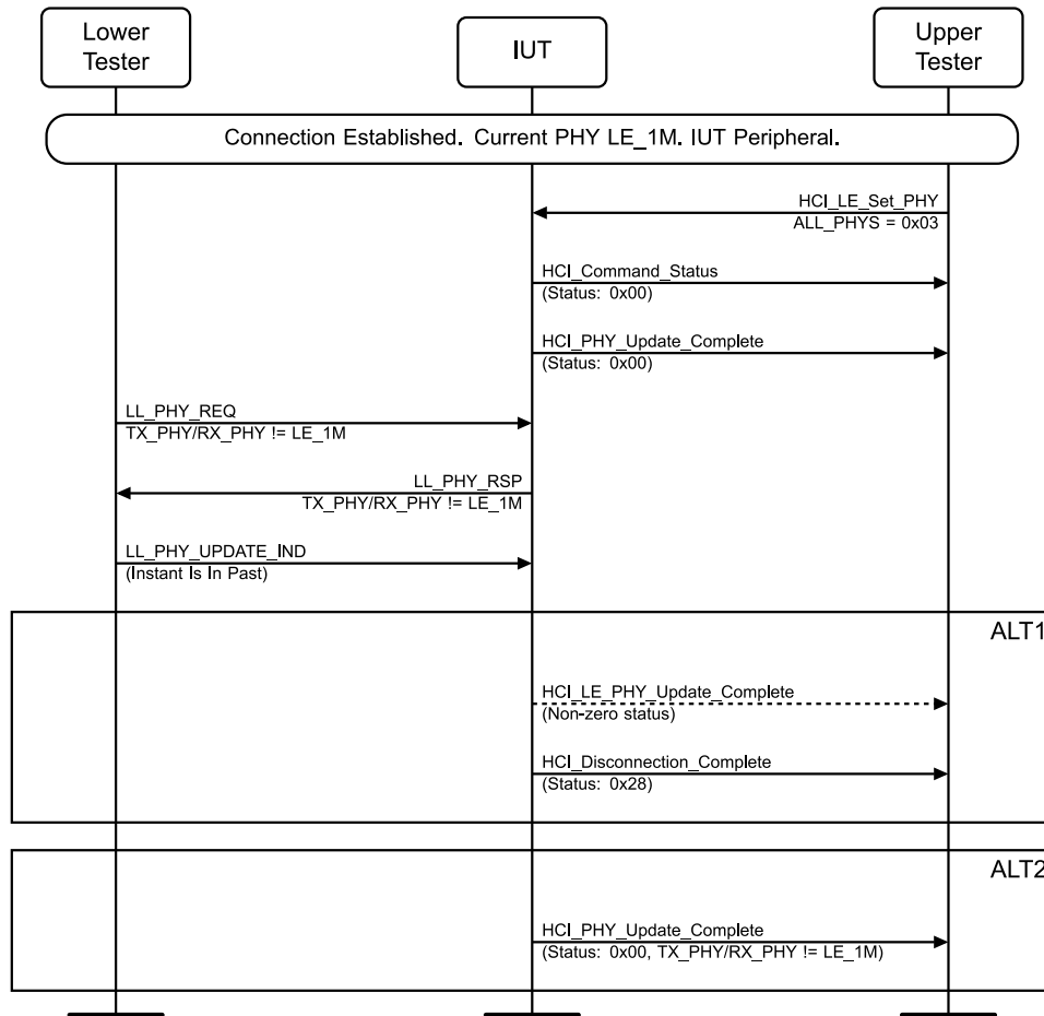
Figure 4.3-111: LL/CON/PER/BI-09-C [Responding to PHY Update Procedure – Instant In the Past] MSC
