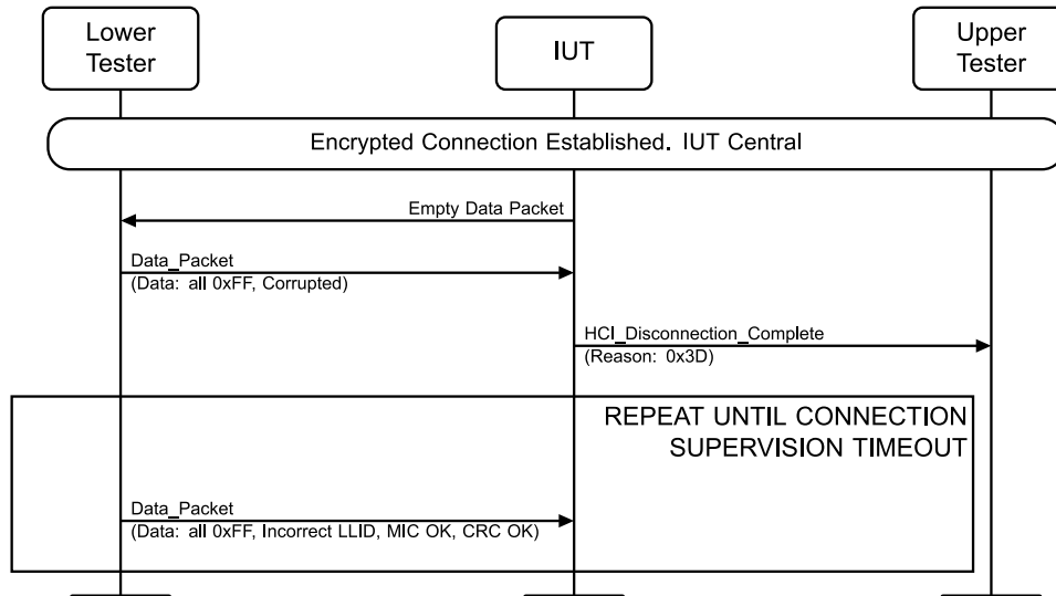
Figure 4.8-57: LL/SEC/CEN/BI-05-C [Central MIC Failure: Corrupt MIC] MSC
