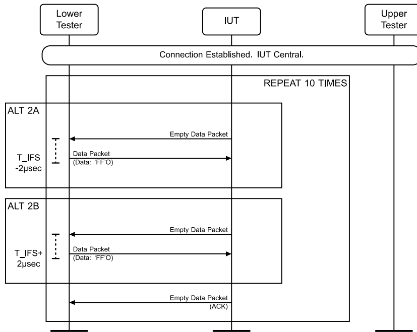
Figure 4.4-26: Earliest/Latest Transmission to Central MSC
