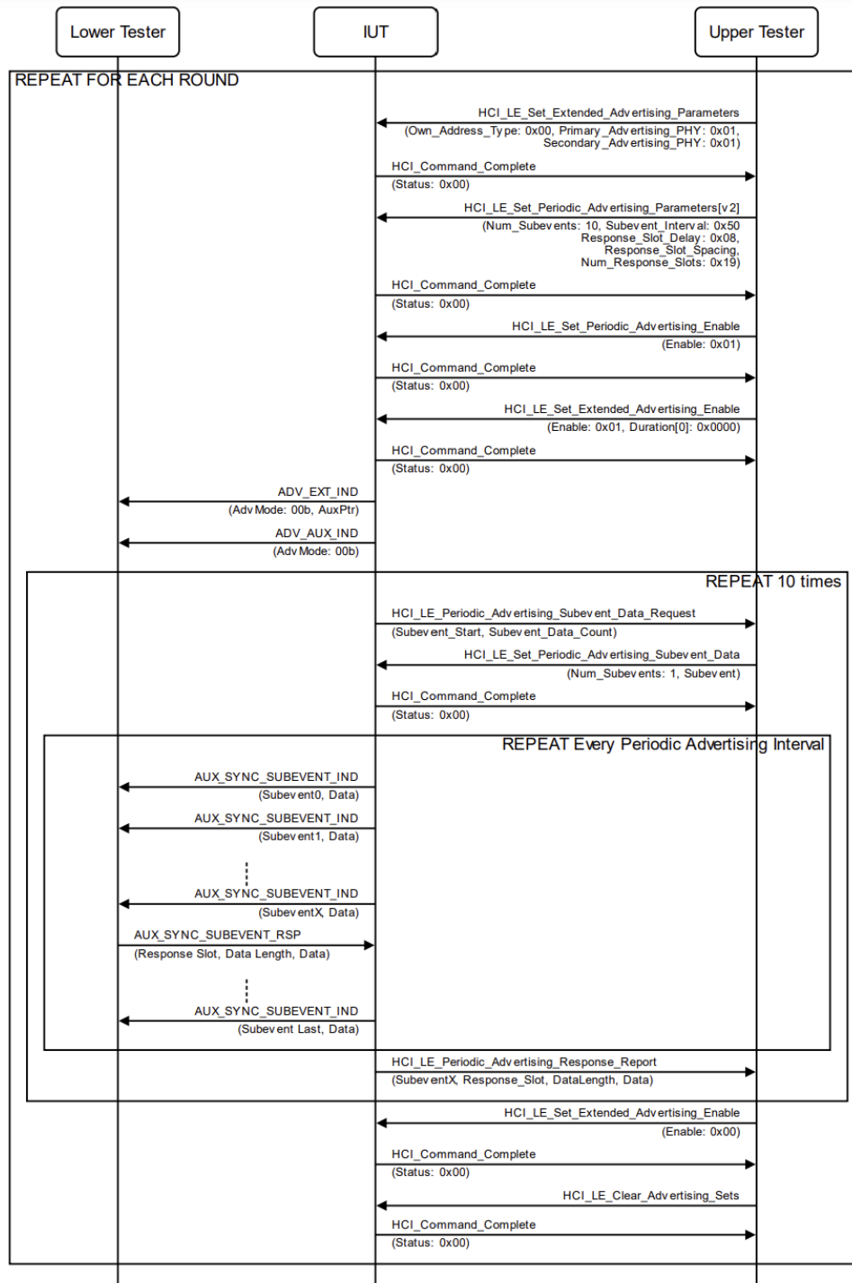
Figure 4.2-63: Transmit Periodic Advertising with Responses MSC
