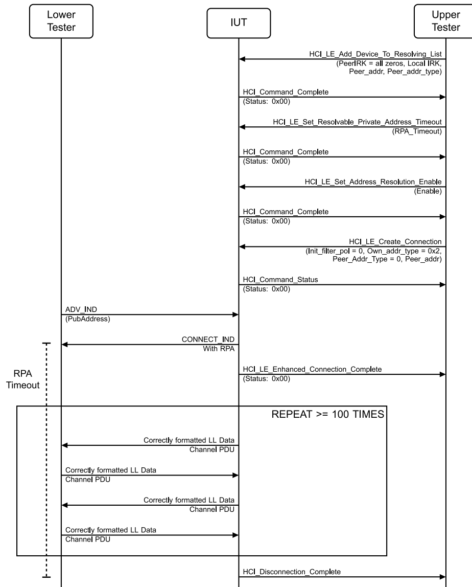
Figure 4.3-26: Network Privacy – Connection Establishment responding to connectable undirected advertising, Initiator MSC
