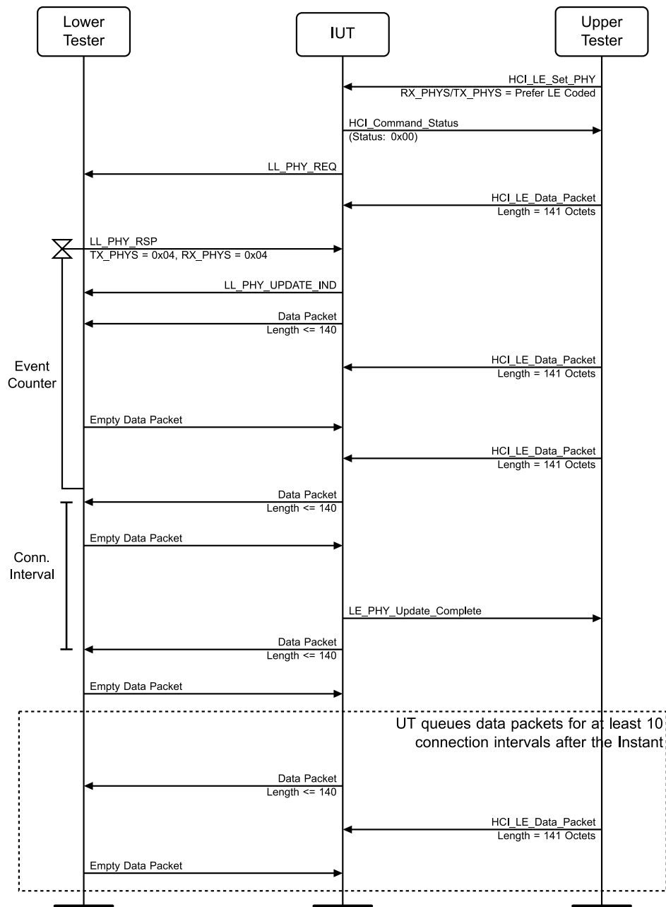
Figure 4.3-178: LL/CON/CEN/BV-53-C [Initiating PHY Update Procedure – Packet Time Restrictions, LE Coded] MSC – Page 2 of 2
