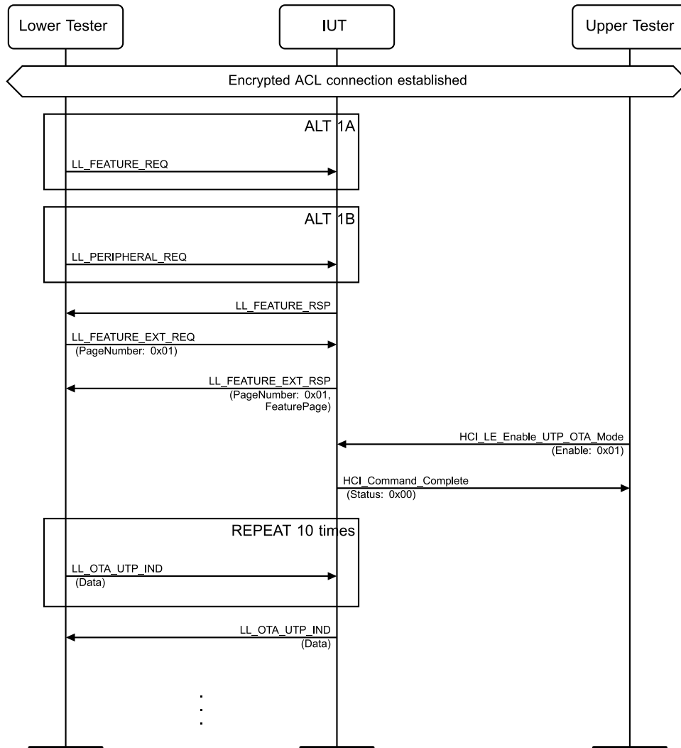
Figure 4.7-5: Receive UTP OTA Mode Maximum Length MSC
