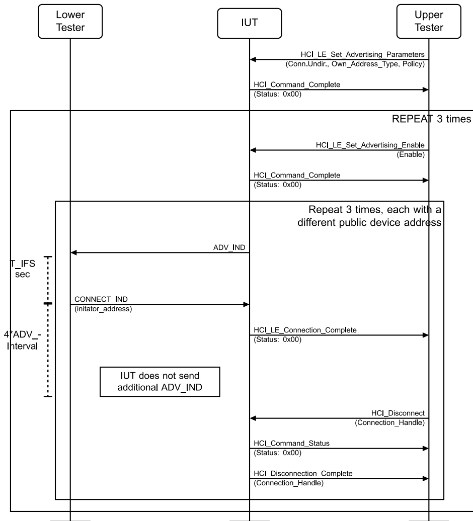
Figure 4.2-4: LL/DDI/ADV/BV-06-C [Connection Request] MSC
