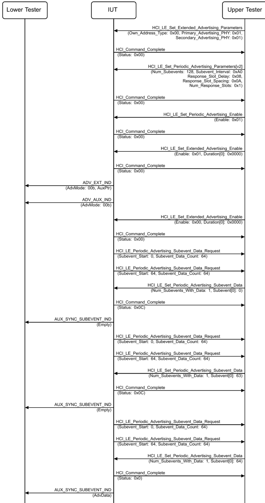
Figure 4.2-76: LL/DDI/ADV/BI-11-C [Periodic Advertising with Responses, Reject Subevent Data With Invalid Subevent] MSC
