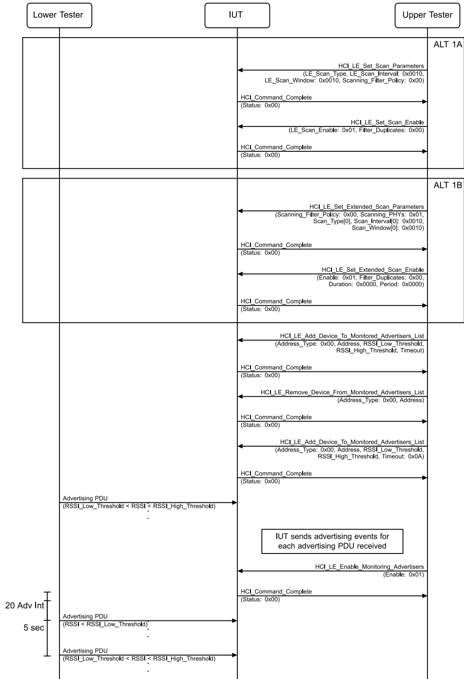
Figure 4.2-147: Monitoring Advertisers MSC – Page 1 of 2
