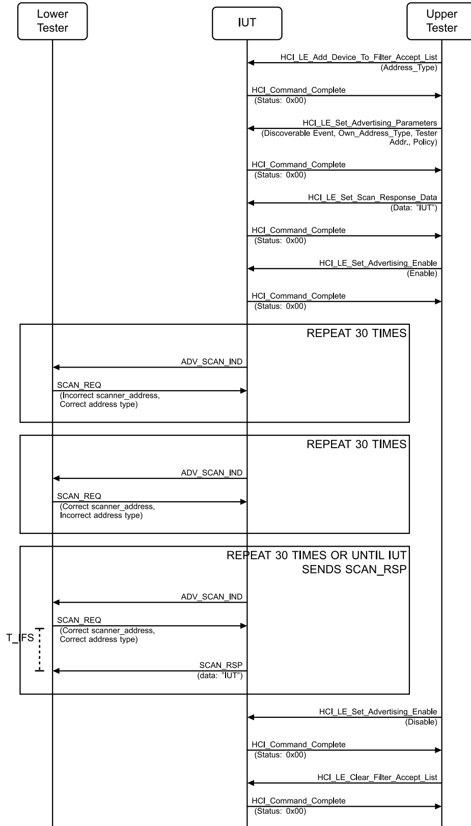
Figure 4.2-12: LL/DDI/ADV/BV-18-C [Device Filtering: Discoverable] MSC
