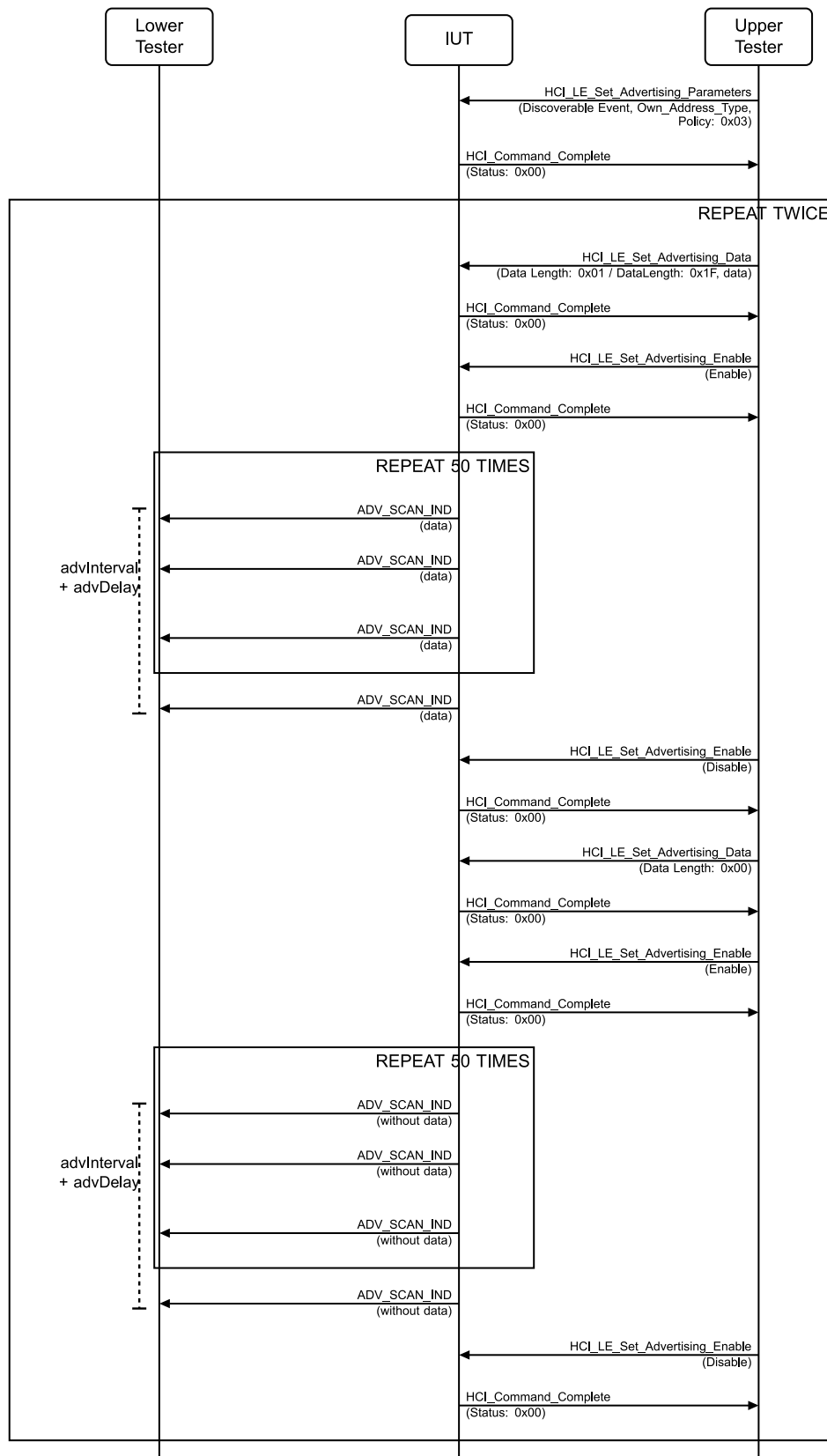
Figure 4.2-10: LL/DDI/ADV/BV-16-C [Advertising Data: Discoverable] MSC
