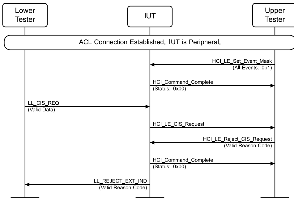
Figure 4.10-28: LL/CIS/PER/BV-02-C [CIS Setup Procedure, Peripheral Responding, Reject Response] MSC
