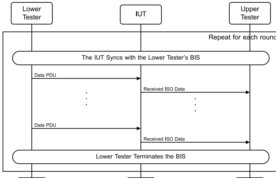
Figure 4.11-18: LL/BIS/SNC/BV-08-C [Pre-transmissions in Broadcast Isochronous Stream] MSC
