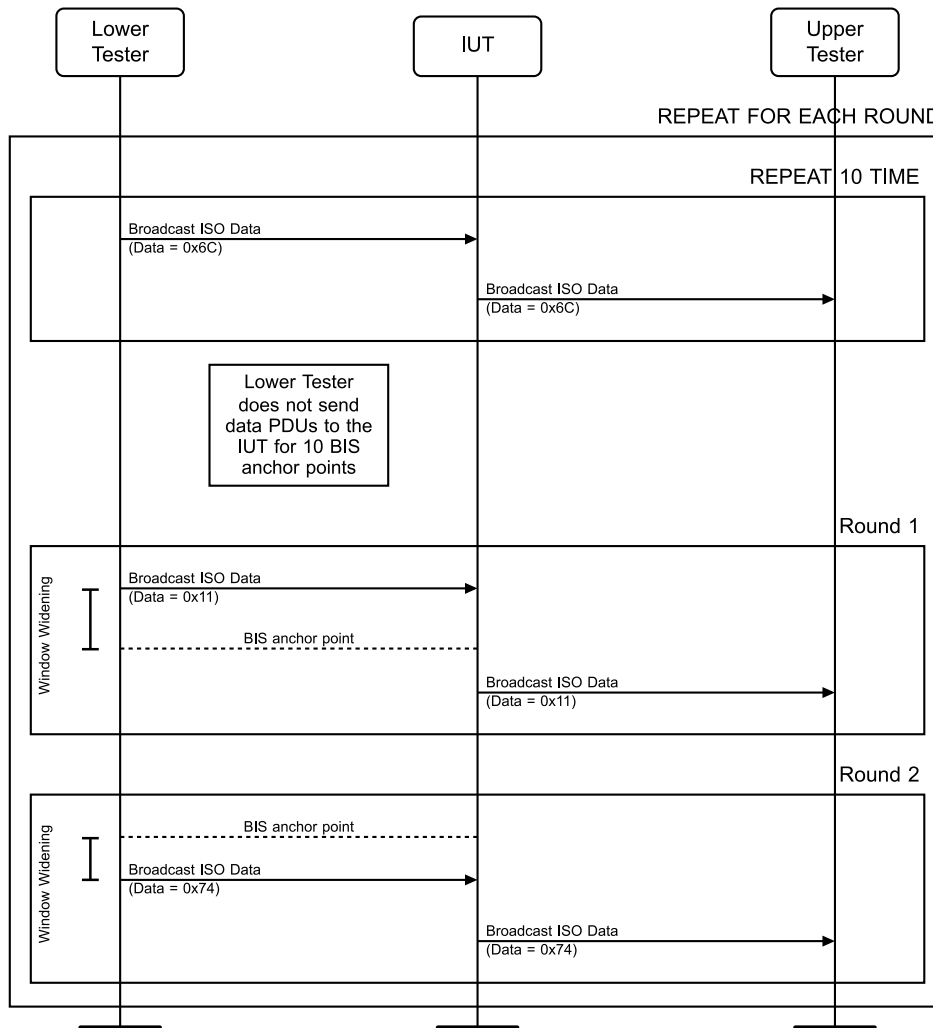
Figure 4.11-25: LL/BIS/SNC/BV-19-C [Listening for Packet With Window Widening, BIS] MSC
