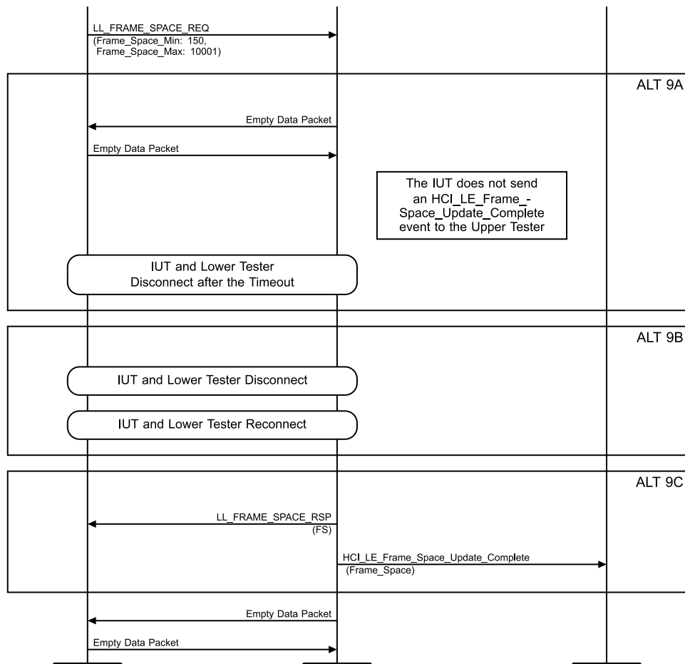
Figure 4.4-48: Frame Space Change, Invalid Parameters MSC – Page 2 of 2
