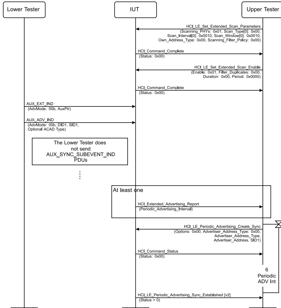
Figure 4.2-129: Transition to Standby State, no AUX_SYNC_SUBEVENT_IND MSC
