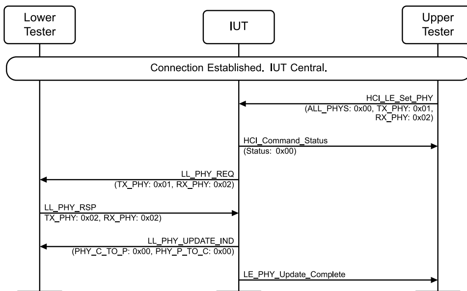
Figure 4.3-189: LL/CON/CEN/BV-117-C [PHY Update Procedure – Central Requests Asymmetrical, Peripheral Symmetrical] MSC
