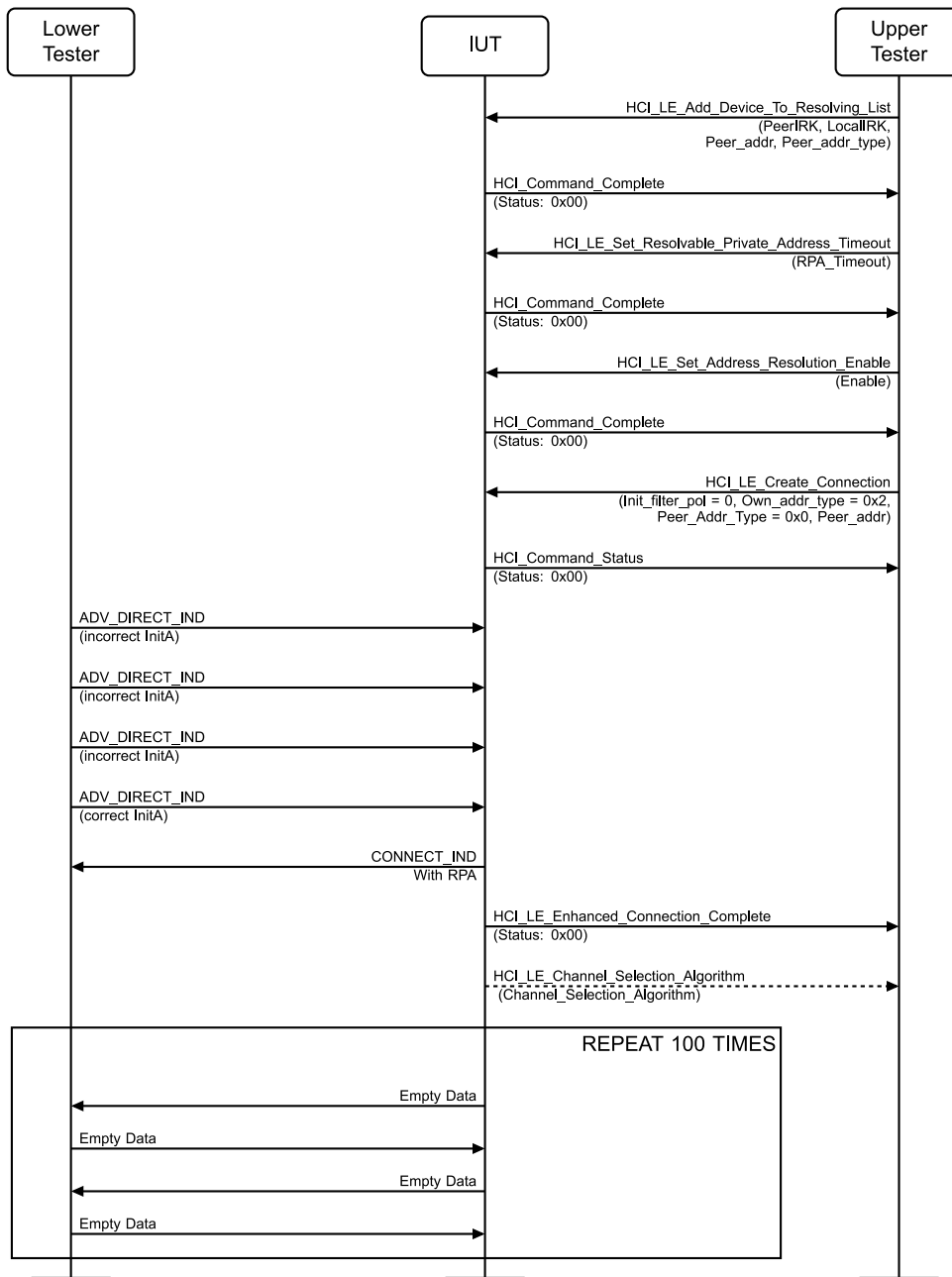
Figure 4.3-29: Network Privacy – Connection Establishment using directed advertising with wrong address and resolving list, Initiator MSC
