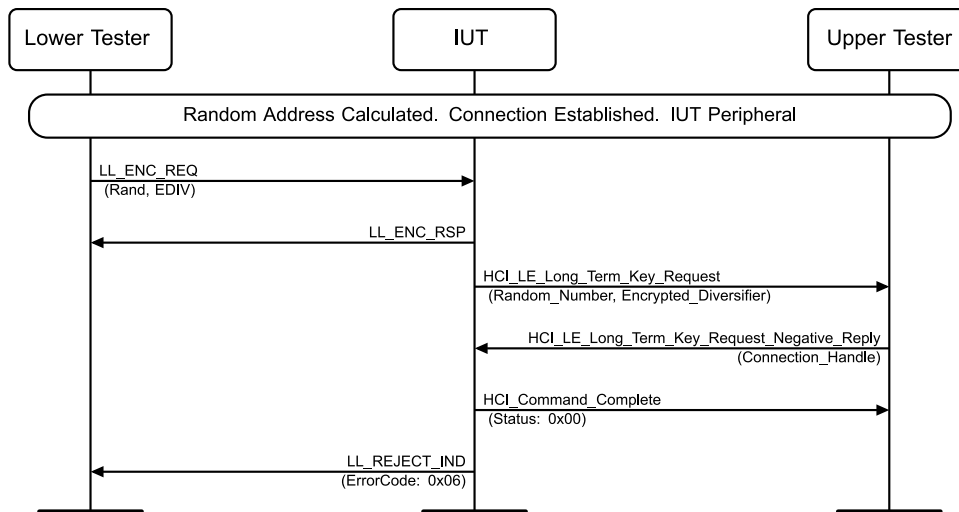
Figure 4.8-30: LL/SEC/PER/BV-04-C [Peripheral Sending LL_REJECT_IND] MSC
