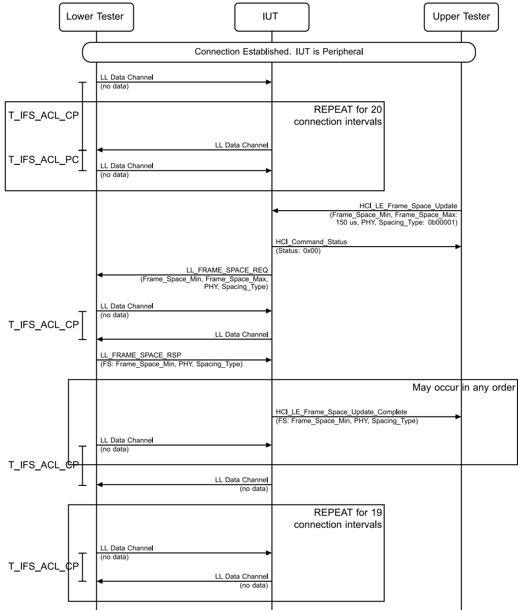
Figure 4.4-13: Initiate Inter Frame Space Change in the current ACL connection, Symmetric PHYs, Peripheral MSC – Page 1 of 2
