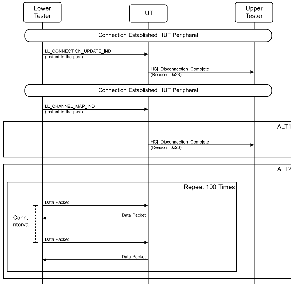
Figure 4.3-107: LL/CON/PER/BI-04-C [Rejecting Connection Change] MSC
