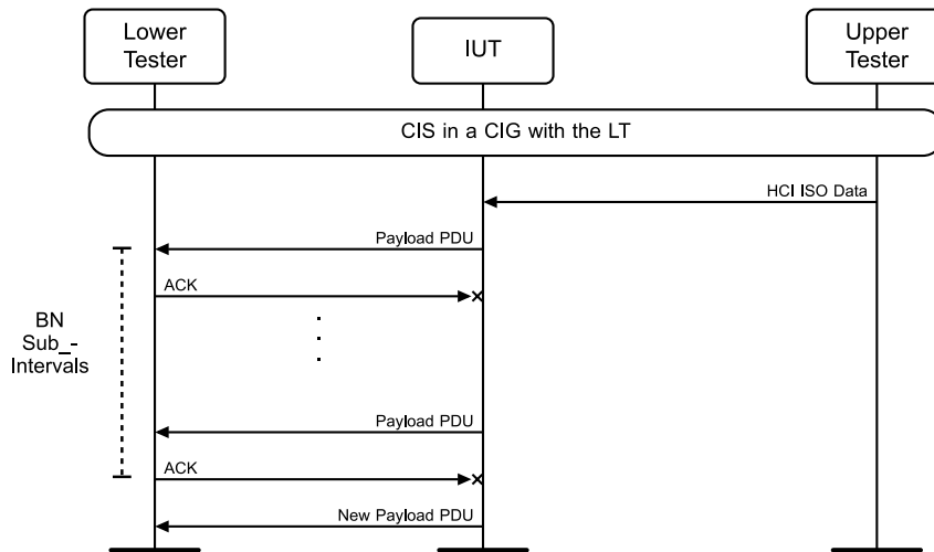
Figure 4.10-13: LL/CIS/CEN/BV-17-C [Flushing of Packets in CIS, Central] MSC
