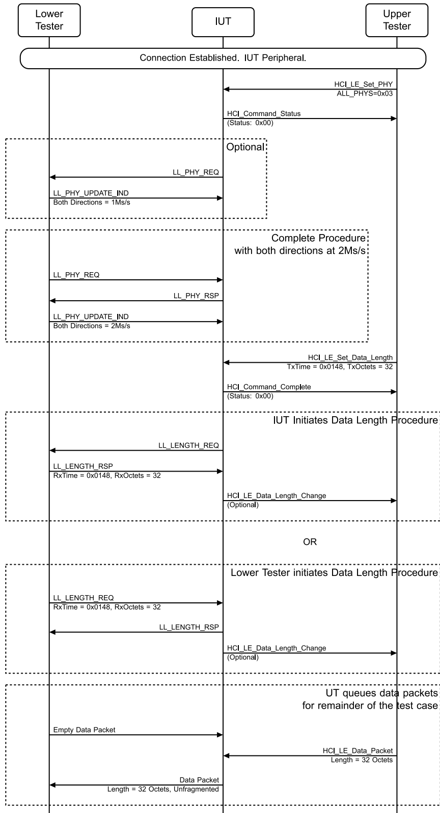
Figure 4.3-90: LL/CON/PER/BV-53-C [Responding to PHY Update Procedure – Packet Time Restrictions, No Change] MSC – Page 1 of 2
