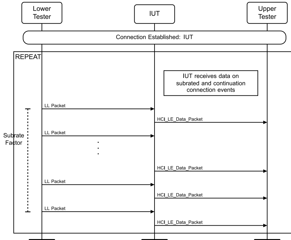
Figure 4.3-252: Receive Data on Continuation events MSC
