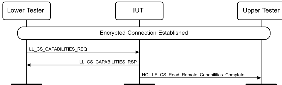
Figure 4.14-12: Verify Capabilities Bit MSC
