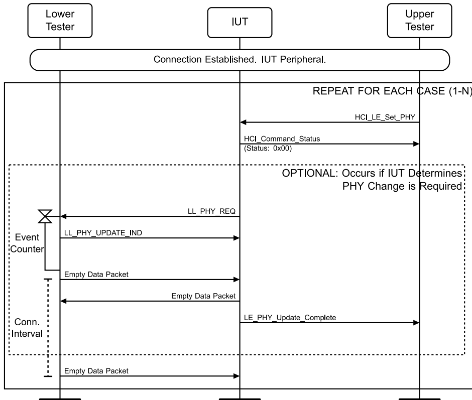
Figure 4.3-76: LL/CON/PER/BV-40-C [Initiating PHY Update Procedure] MSC
