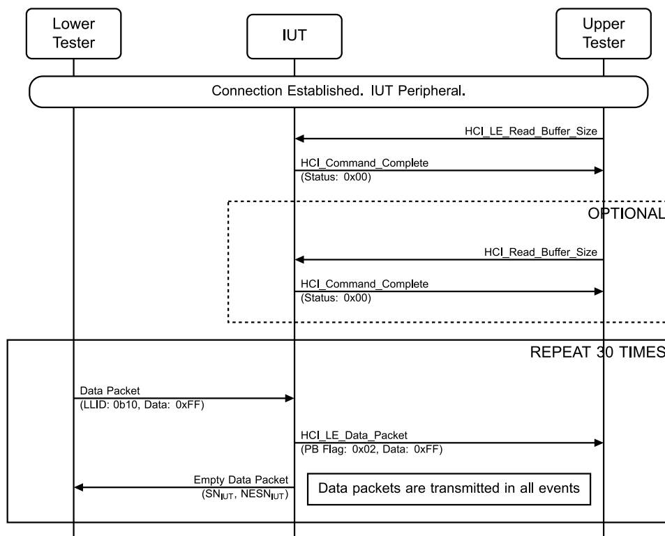
Figure 4.3-47: LL/CON/PER/BV-02-C [Peripheral asymmetric connections] MSC
