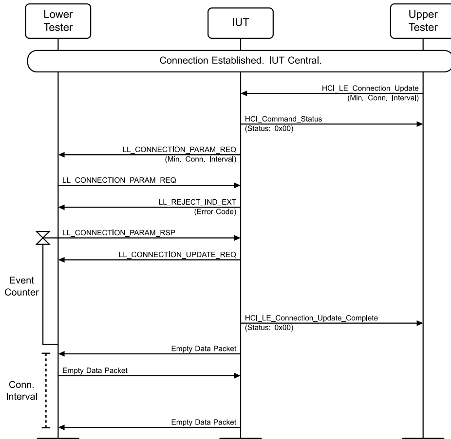
Figure 4.3-156: LL/CON/CEN/BV-26-C [Initiating Connection Parameter Request – same procedure collision] MSC
