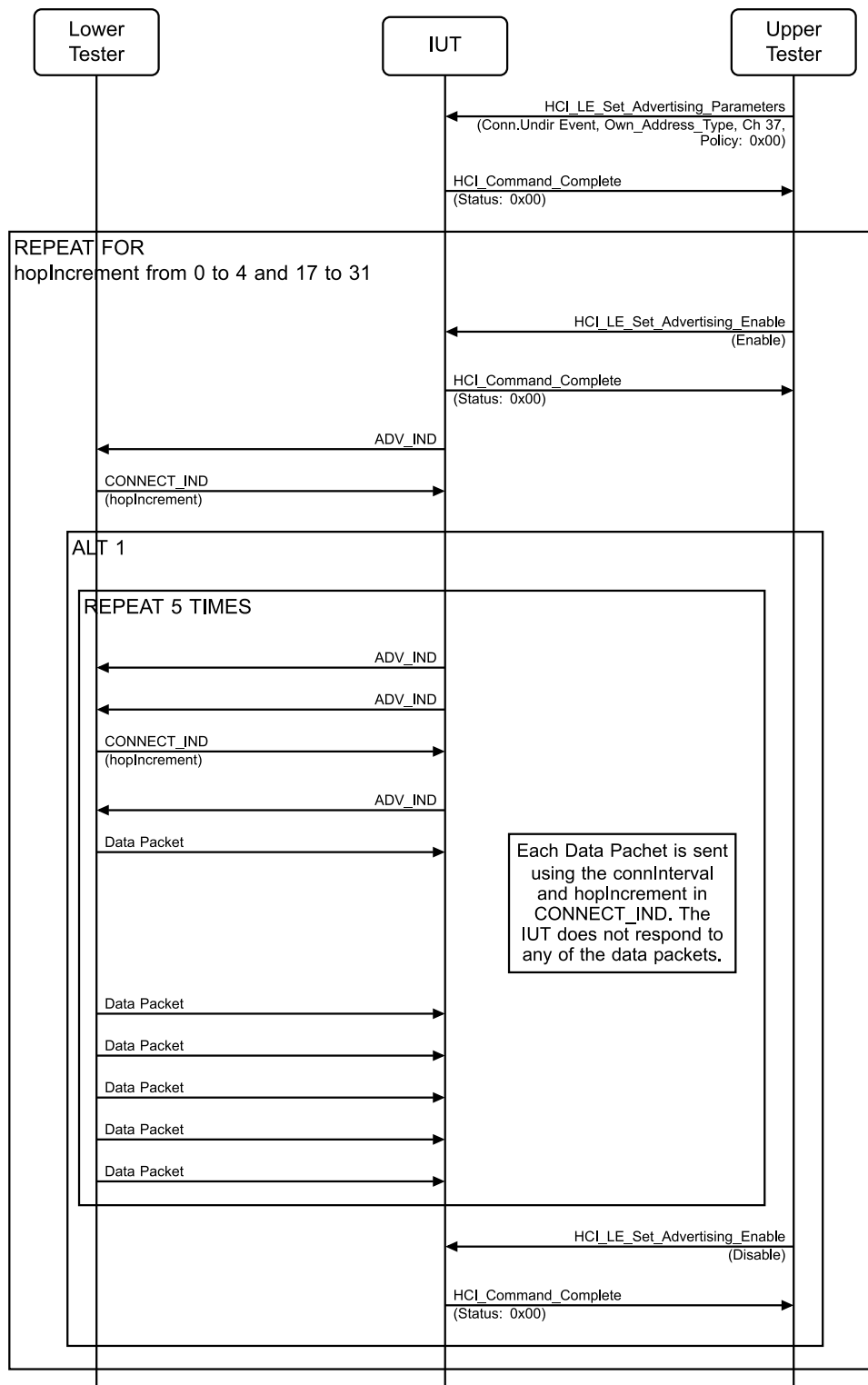
Figure 4.2-48: LL/DDI/ADV/BI-07-C [Connection Request Invalid hopIncrement] MSC – Page 1 of 2
