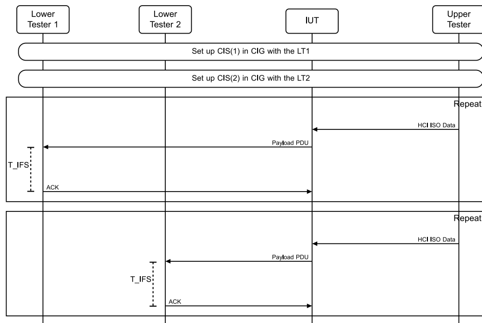
Figure 4.10-6: LL/CIS/CEN/BV-11-C [Sending Data in Multiple CISes, Single CIG, Multiple Connections, Sequential] MSC
