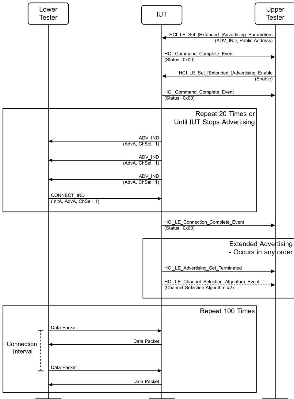
Figure 4.3-11: Accepting Connections, Channel Selection Algorithm #2 MSC
