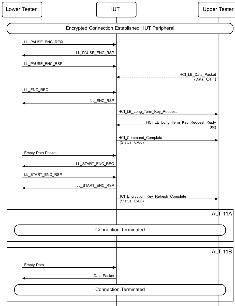
Figure 4.8-29: LL/SEC/PER/BV-02-C [Peripheral Pause Encryption] MSC
