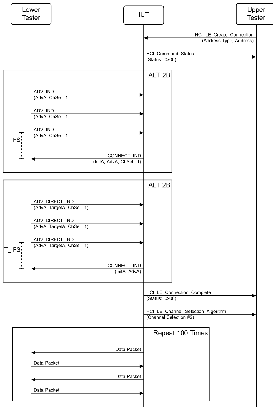
Figure 4.3-33: LL/CON/INI/BV-16-C [Connection Initiation, Channel Selection Algorithm #2] MSC
