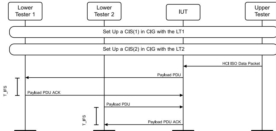
Figure 4.10-5: Sending and Receiving Data in Multiple CISes, Single CIG, Multiple Connections, Interleaved CIG MSC
