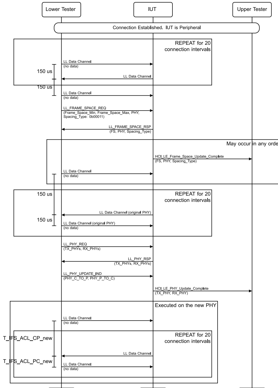
Figure 4.4-21: Respond to Inter Frame Space Change Request on a Different PHY, Peripheral MSC
