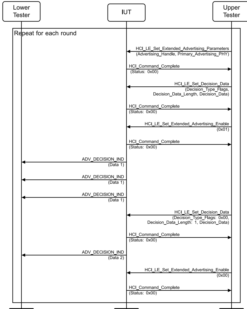
Figure 4.2-72: Decision-Based Advertisements, Set Before and After Extended Advertising Enabled MSC
