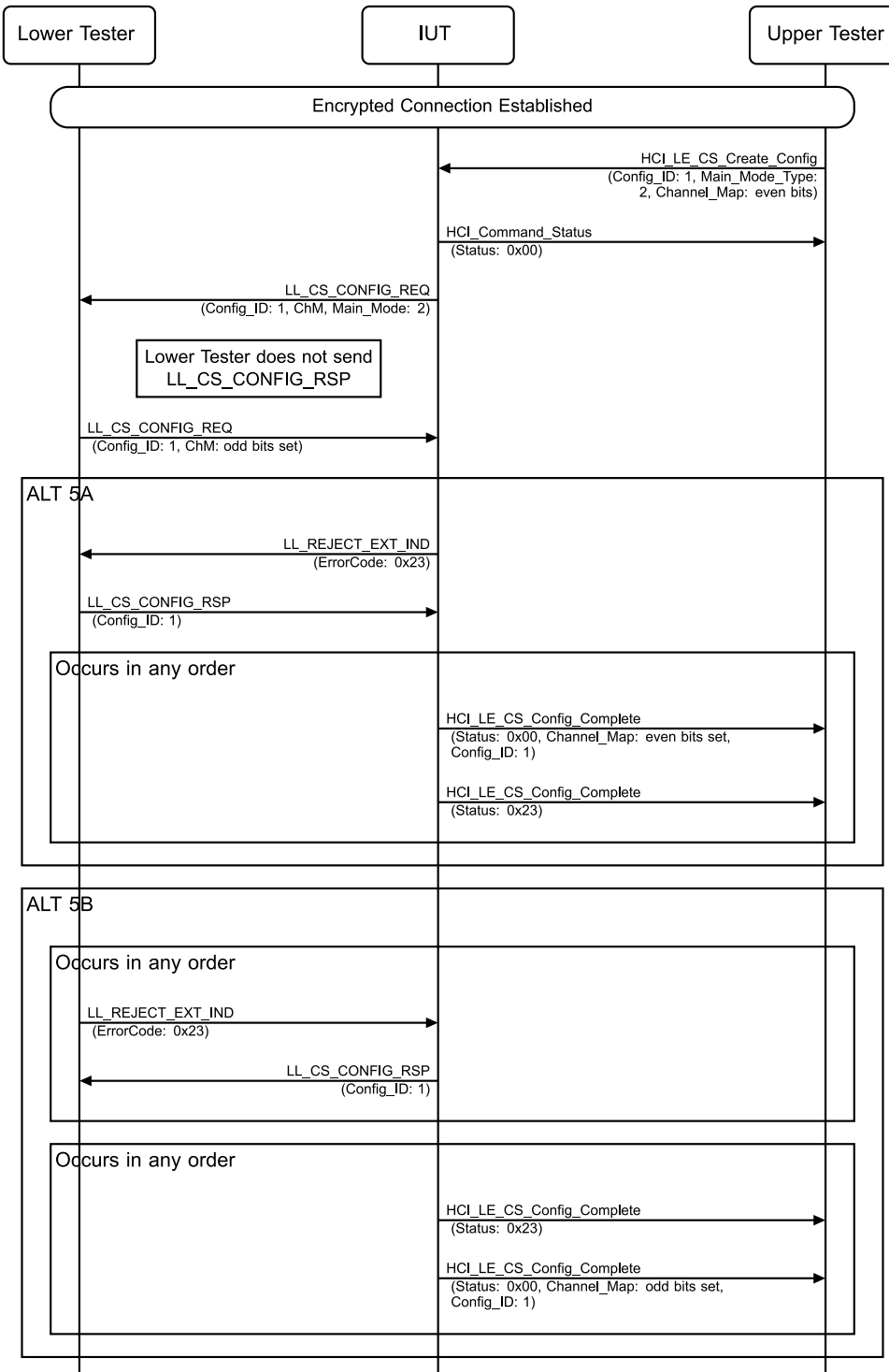
Figure 4.14-41: Channel Sounding Configuration Procedure Collision MSC – Page 1 of 2
