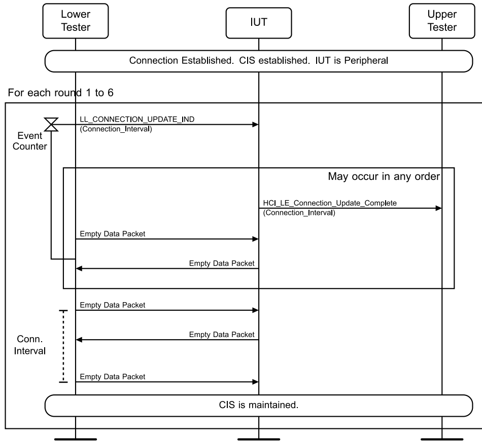
Figure 4.10-47: LL/CIS/PER/BV-54-C [Accepting an Update to an ACL while Maintaining a CIS] MSC
