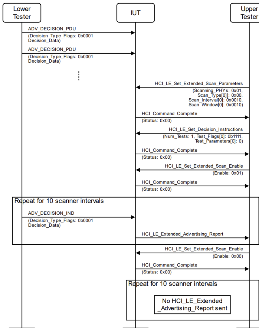
Figure 4.2-142: Decision-Based Advertisements Ignored, Disabled Scanning MSC
