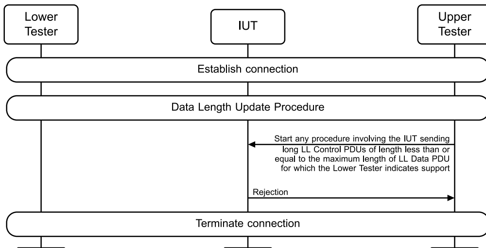
Figure 4.3-228: Rejecting Request to Send Long Control PDUs before Feature Exchange but after Data Length Update Procedure MSC
