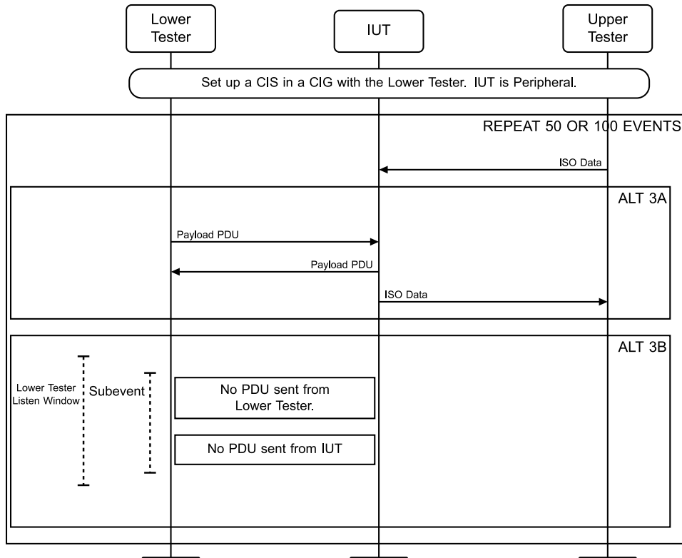
Figure 4.10-38: LL/CIS/PER/BV-28-C [CIS Peripheral Response, No PDU Received in Subevent] MSC
