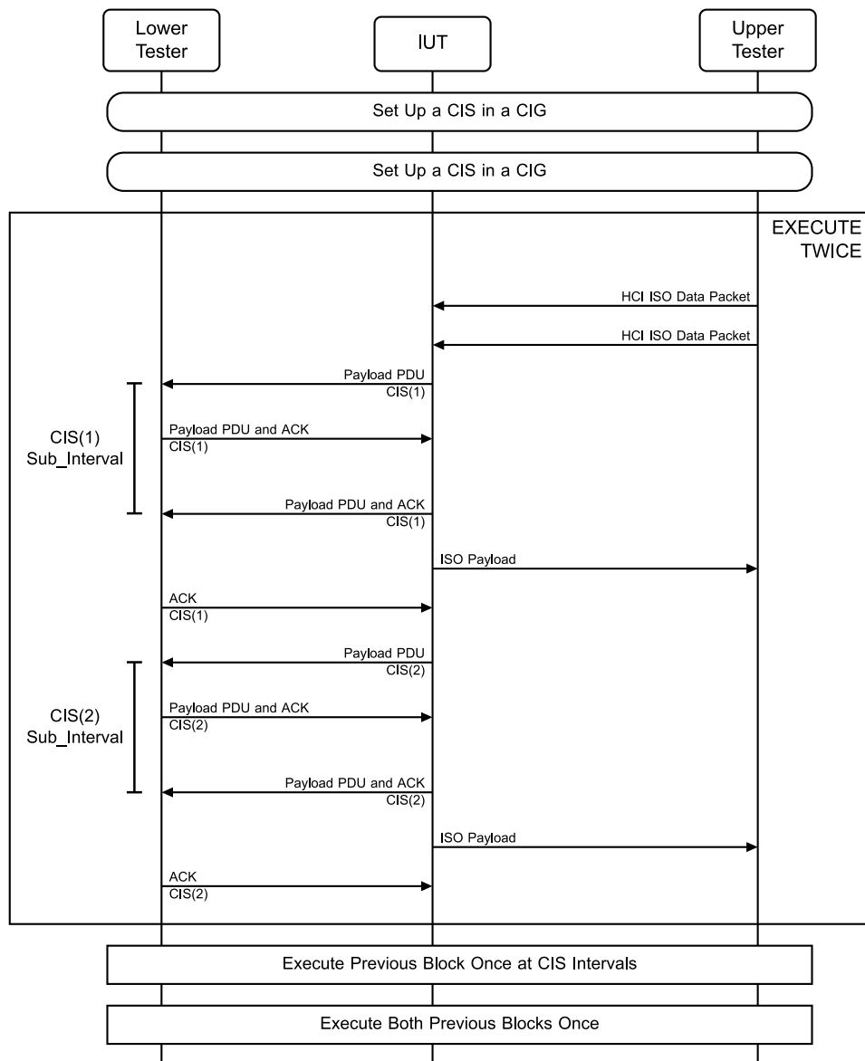
Figure 4.10-11: LL/CIS/CEN/BV-09-C [Sending and Receiving Data in Multiple CISes, Single CIG, Single Connection, Sequential, Central] MSC
