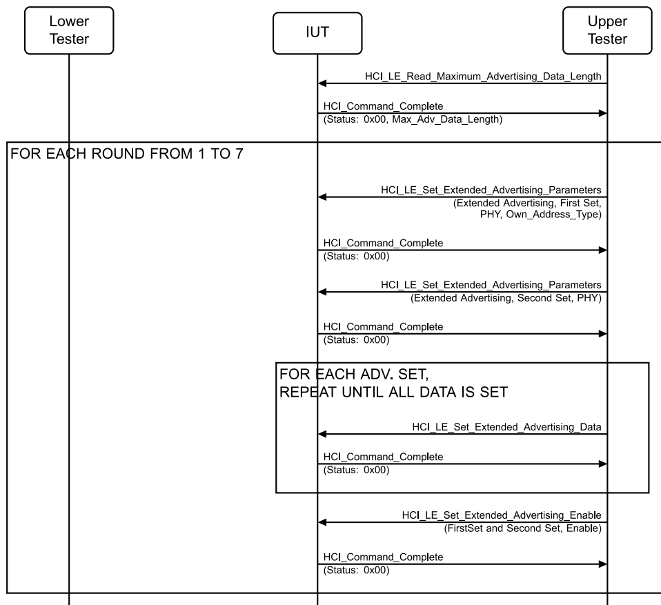
Figure 4.2-27: Extended Advertising, Multiple Sets MSC – Page 1 of 2
