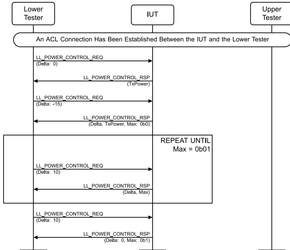
Figure 4.13-16: Power Control Response, Max Power MSC
