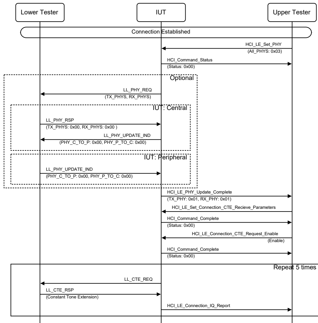
Figure 4.3-247: Constant Tone Extension Request Procedure, IUT Initiated, Periodic MSC – Page 1 of 2
