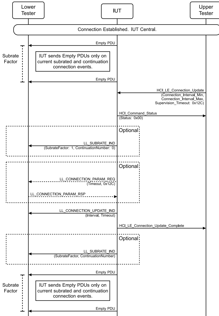
Figure 4.3-200: LL/CON/CEN/BV-139-C [Subrate Set to 1 After Requesting Connection Interval Change] MSC – Page 1 of 2
