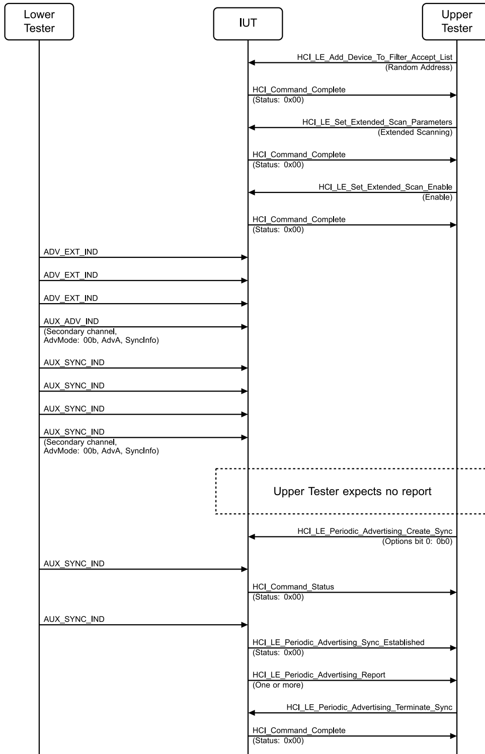
Figure 4.2-102: LL/DDI/SCN/BV-34-C [Extended Scanning, Periodic Advertising Reception, Filter Policies] MSC – Page 1 of 2
