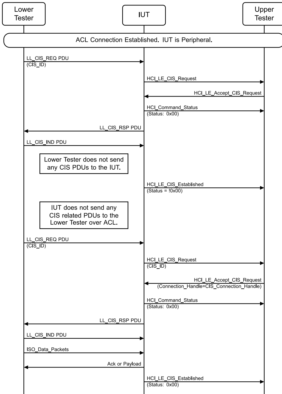
Figure 4.10-37: LL/CIS/PER/BV-25-C [CIS Considered Lost before Establishment, Peripheral] MSC
