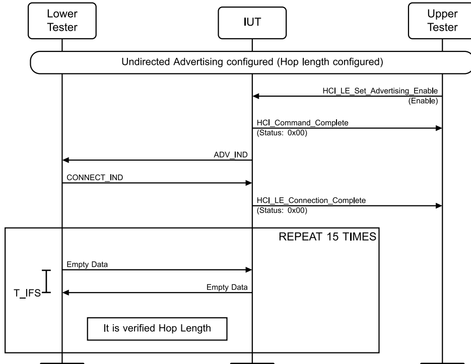
Figure 4.6-1: LL/FRH/ADV/BV-01-C [Accepting Connections with Hop Lengths] MSC
