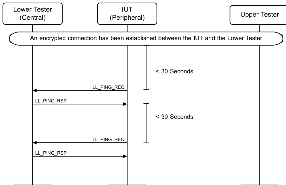
Figure 4.8-32: LL/SEC/PER/BV-06-C [Initiate LE Ping procedure when encryption is enabled] MSC
