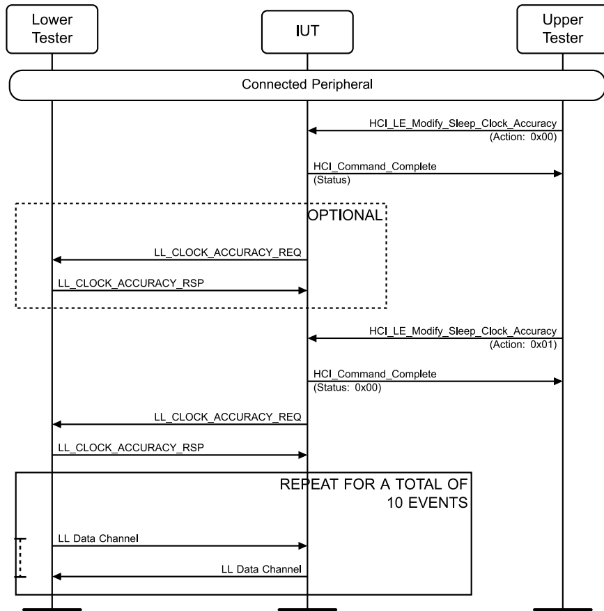
Figure 4.4-10: LL/TIM/PER/BV-08-C [Initiate Sleep Clock Accuracy Update] MSC
