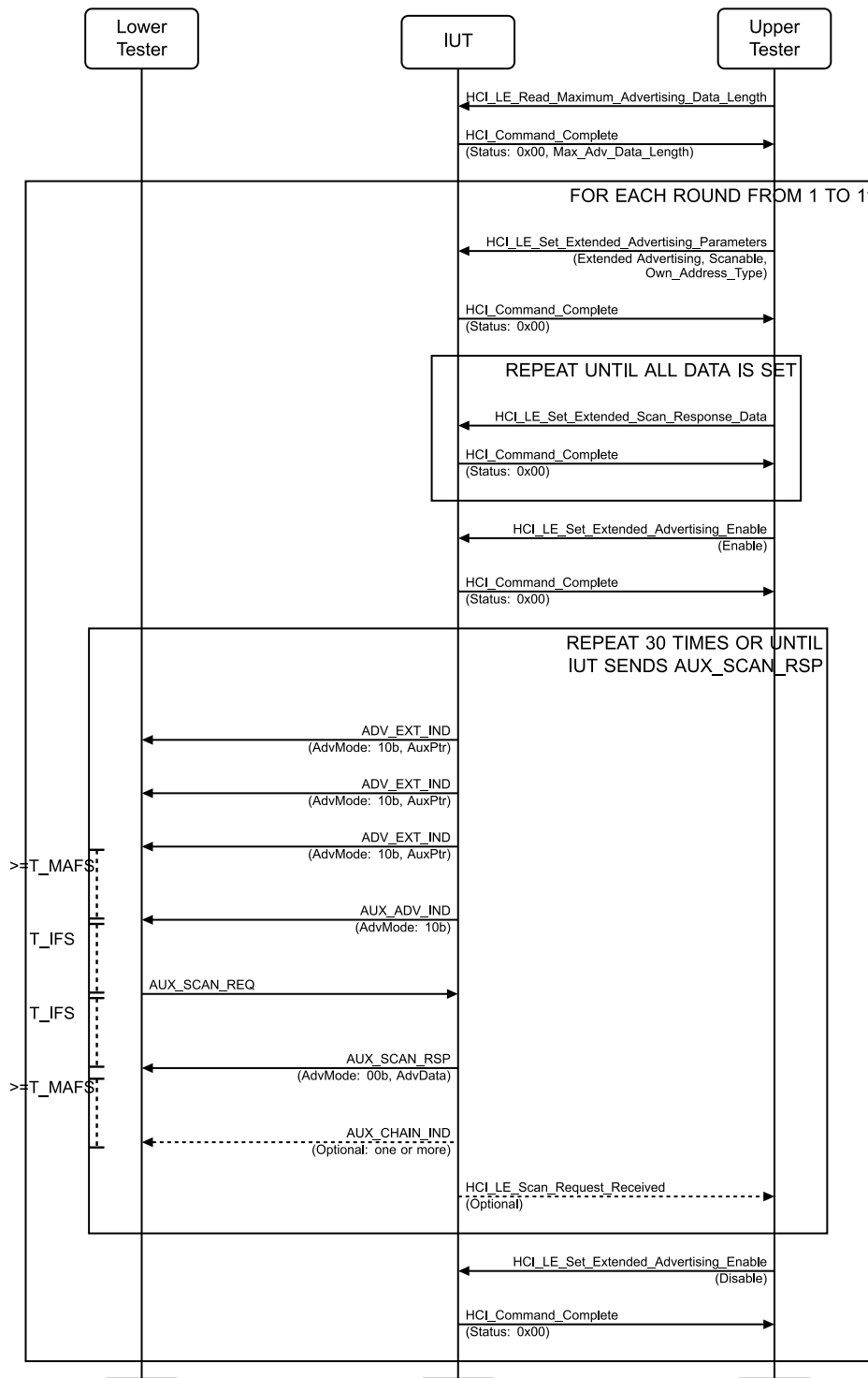
Figure 4.2-20: Extended Advertising, Secondary Channel, Scannable MSC
