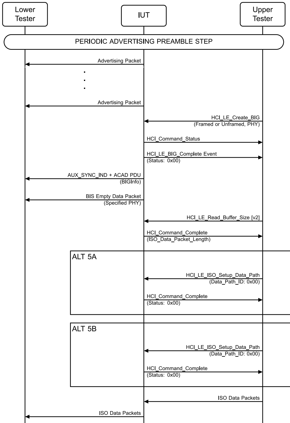
Figure 4.11-7: Broadcast Isochronous Stream Using Non-Test Command – MSC Page 1 of 2
