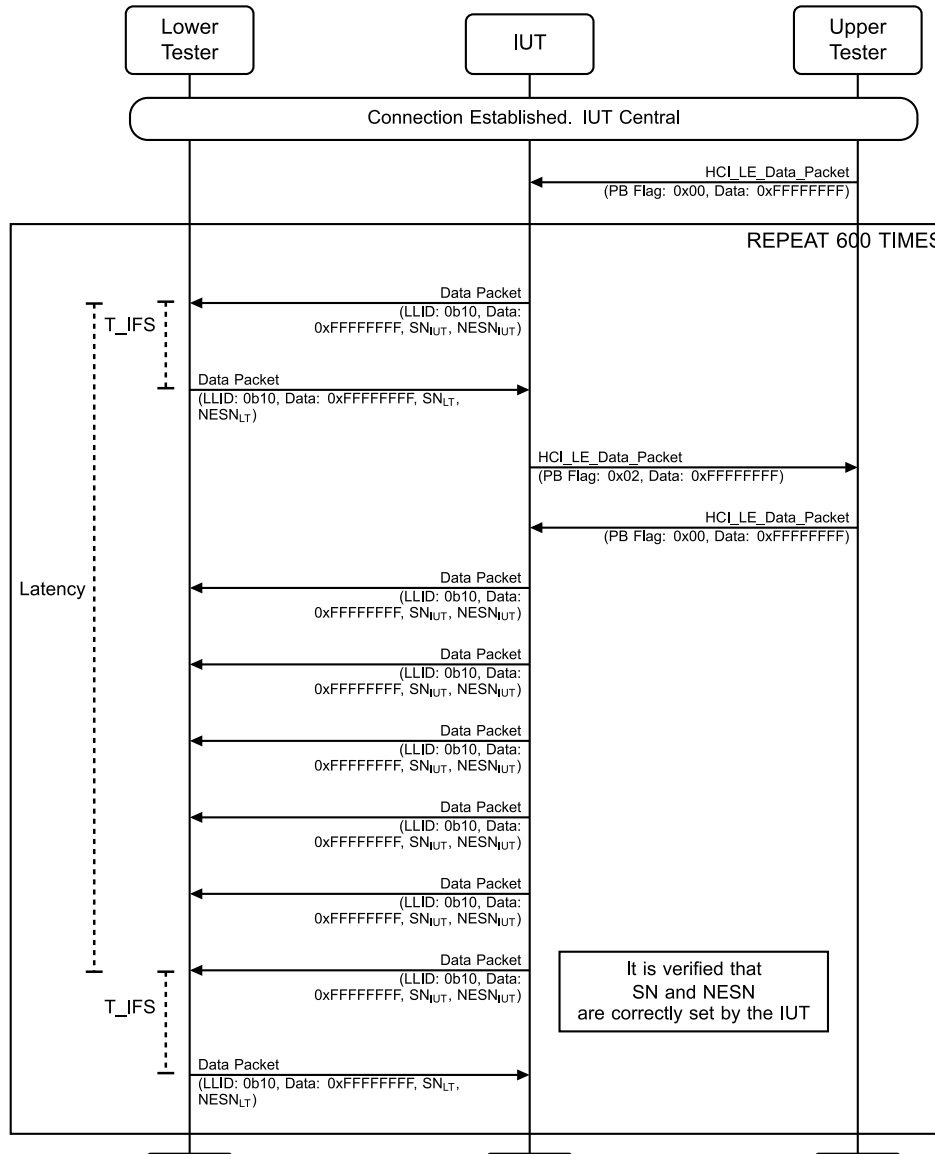
Figure 4.3-134: LL/CON/CEN/BV-02-C [Events with Peripheral Latency] MSC
