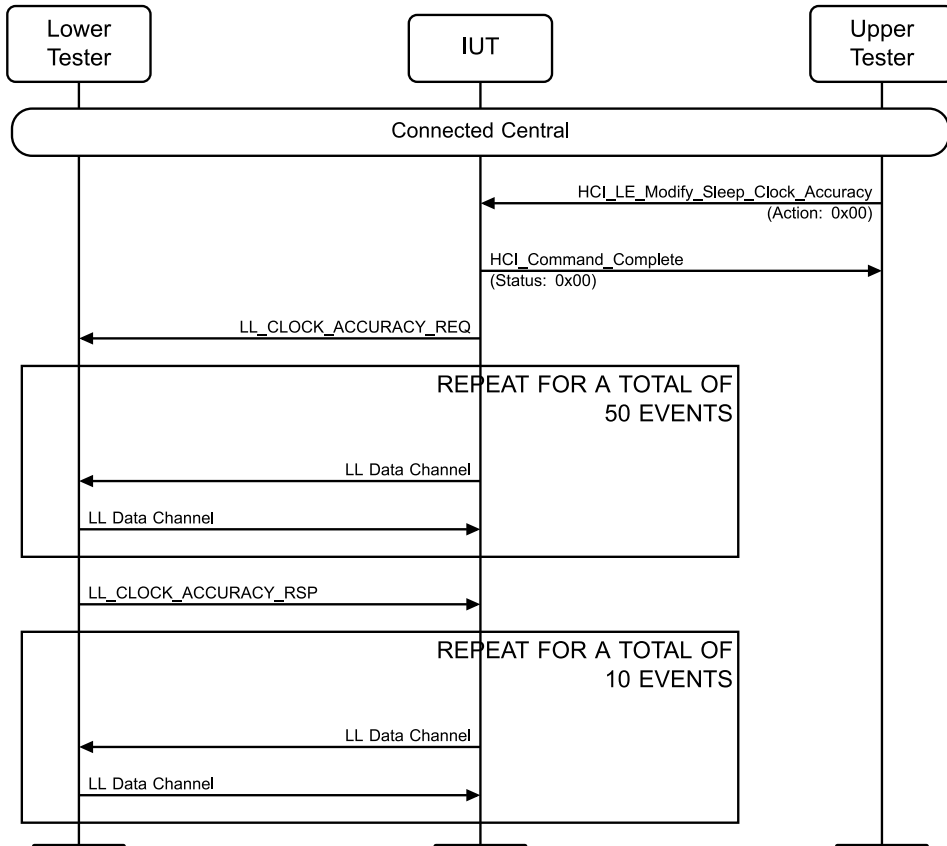
Figure 4.4-31: LL/TIM/CEN/BV-07-C [Change Accuracy before Update] MSC
