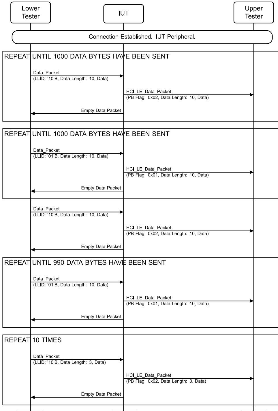
Figure 4.3-49: LL/CON/PER/BV-05-C [Peripheral receiving data] MSC
