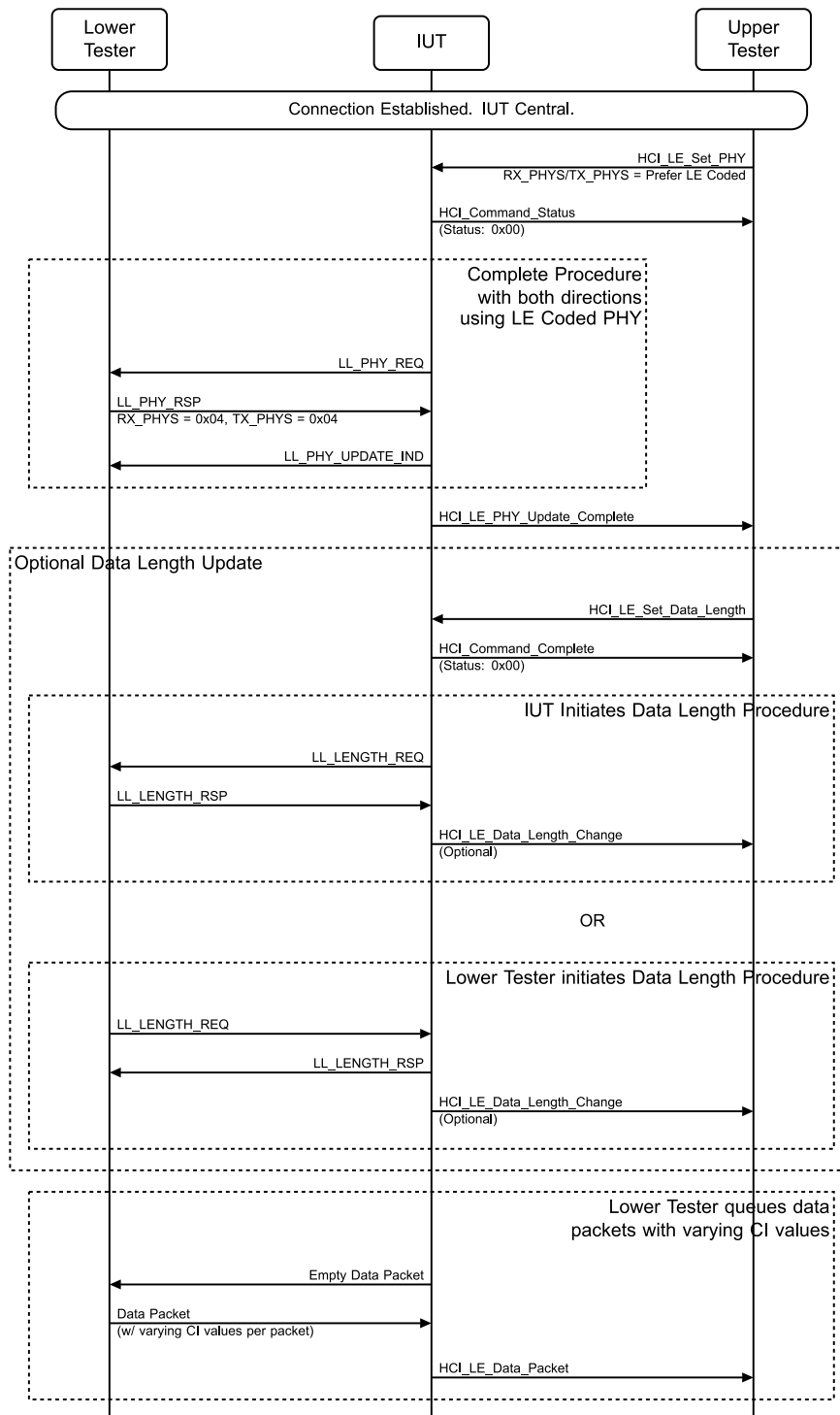
Figure 4.3-176: LL/CON/CEN/BV-52-C [Central Receiving Data, LE Coded, CI Change] MSC
