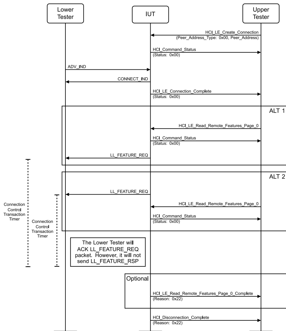
Figure 4.3-148: LL/CON/CEN/BV-19-C [Connection Control Timeout] MSC
