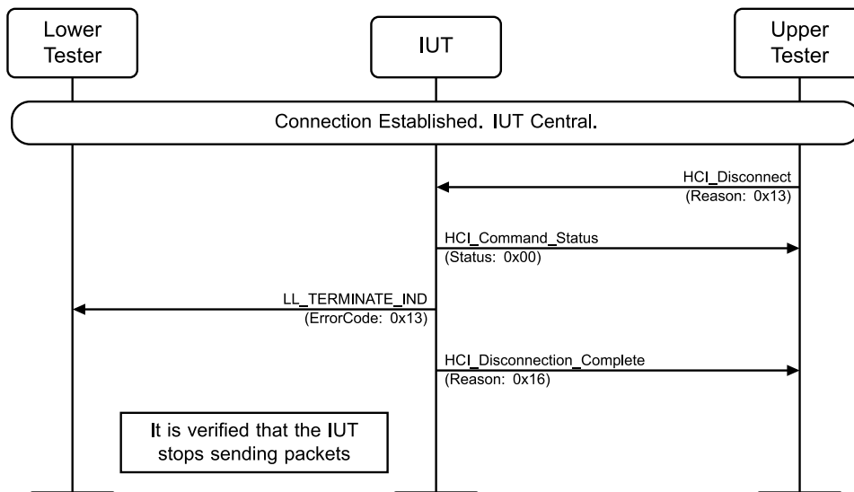
Figure 4.3-139: LL/CON/CEN/BV-08-C [Central Sending Termination] MSC
