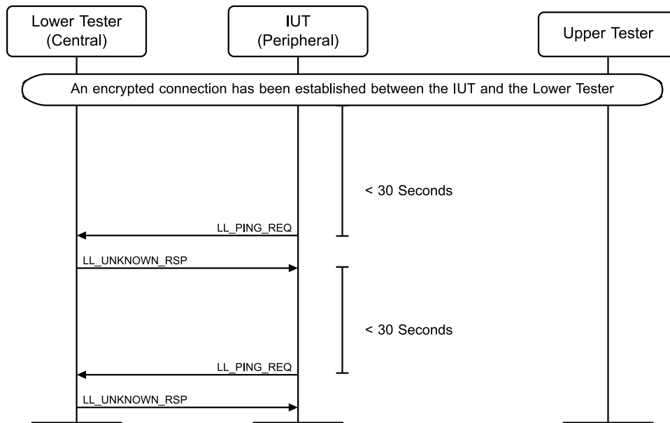
Figure 4.8-36: LL/SEC/PER/BV-10-C [Initiate LE Ping procedure when the other side does not support the procedure] MSC
