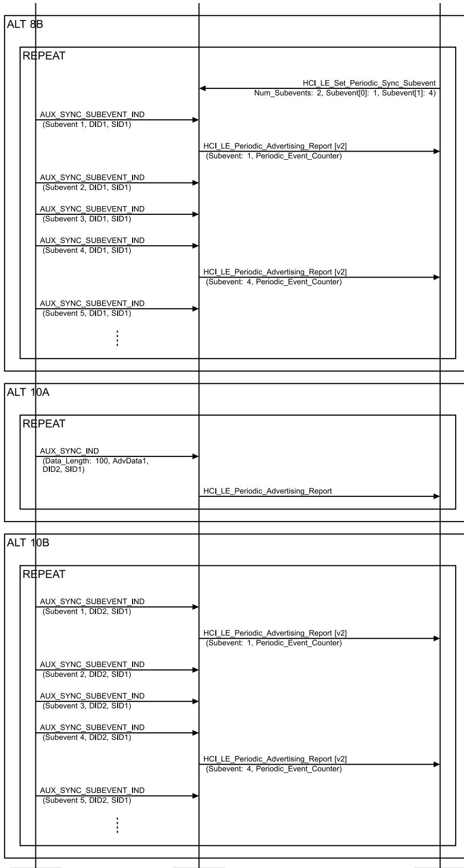
Figure 4.2-113: Scanner not supporting Periodic Advertising ADI accepts Advertising PDU with ADI Set MSC – Page 2 of 2
