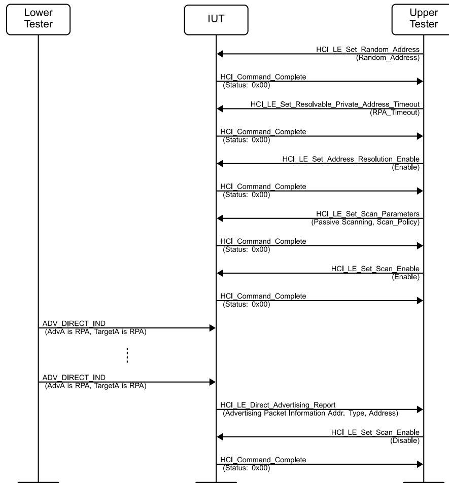
Figure 4.2-85: LL/DDI/SCN/BV-14-C [Network Privacy - Passive Scanning: Directed Events to an address different from the scanner's address] MSC
