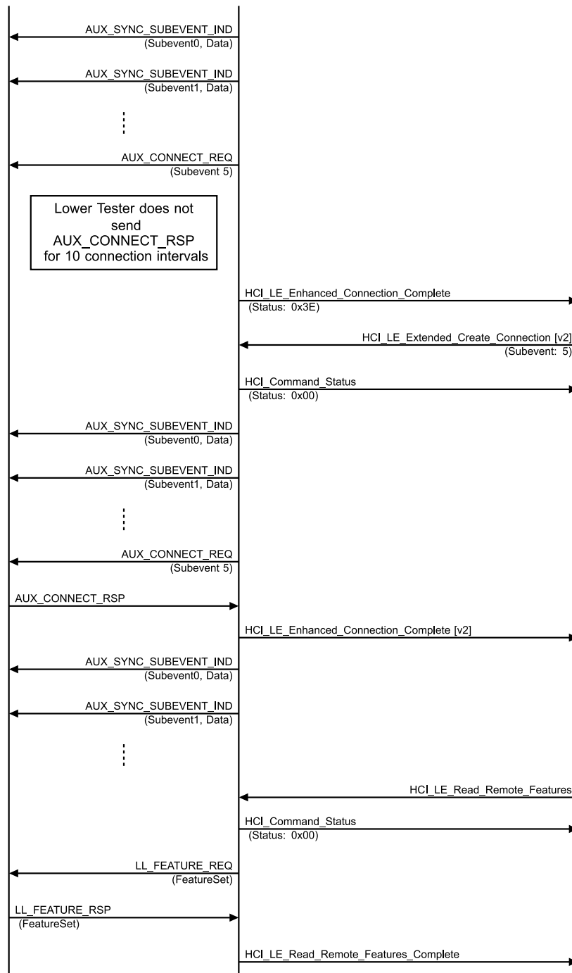
Figure 4.2-65: Reconnect with a Synchronized Device using Periodic Advertising with Responses MSC – Page 2 of 3
