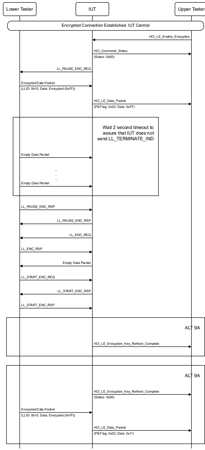
Figure 4.8-42: Central Pause Encryption MSC
