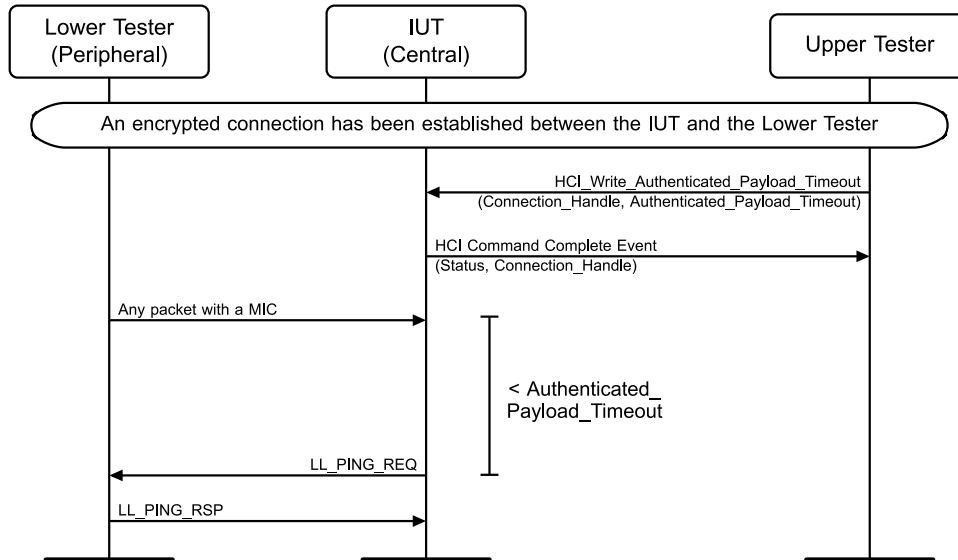
Figure 4.8-48: LL/SEC/CEN/BV-09-C [Modified Authentication Payload Timeout] MSC
