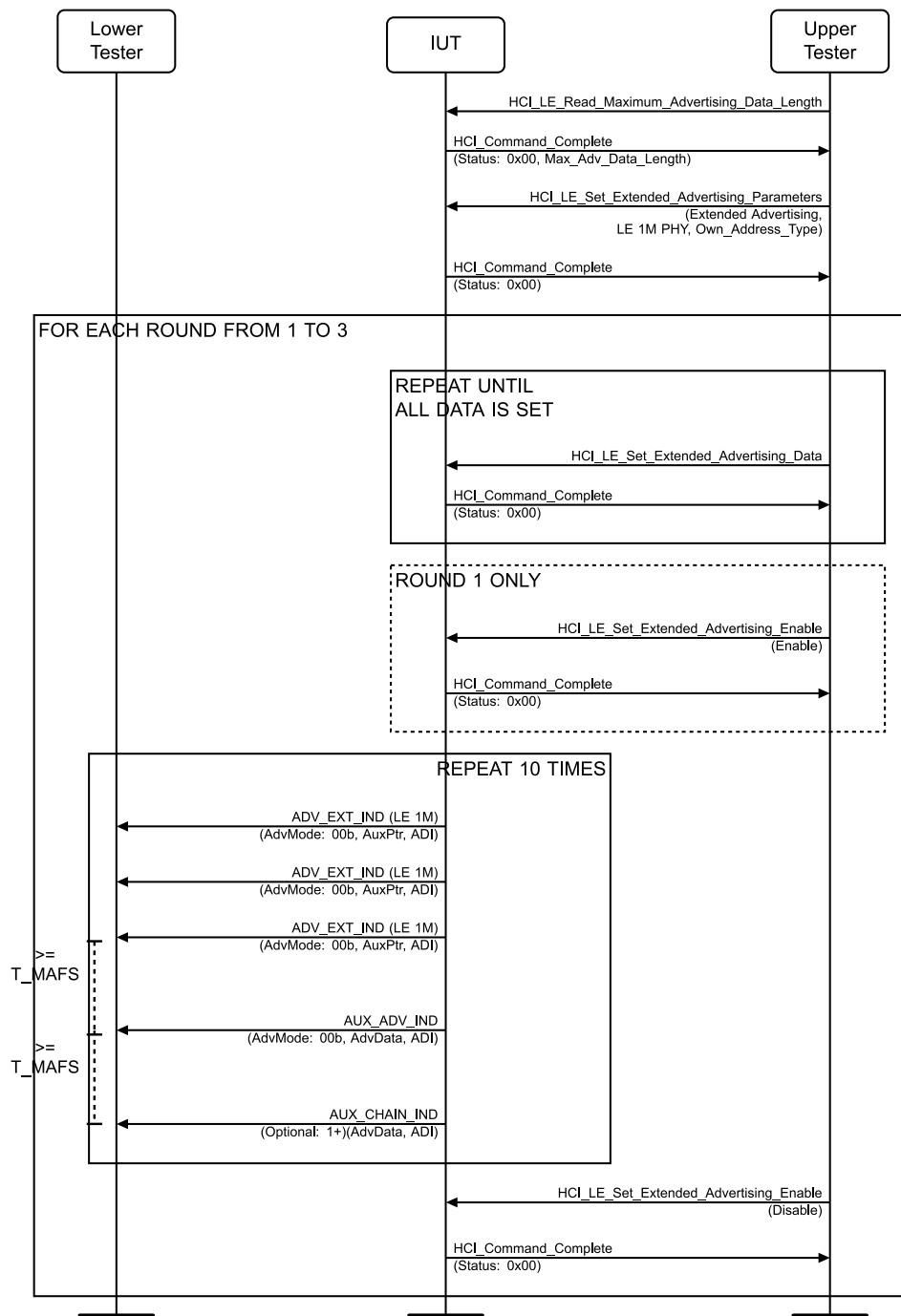
Figure 4.2-23: LL/DDI/ADV/BV-27-C [Extended Advertising, Host Modifying Data and ADI] MSC
