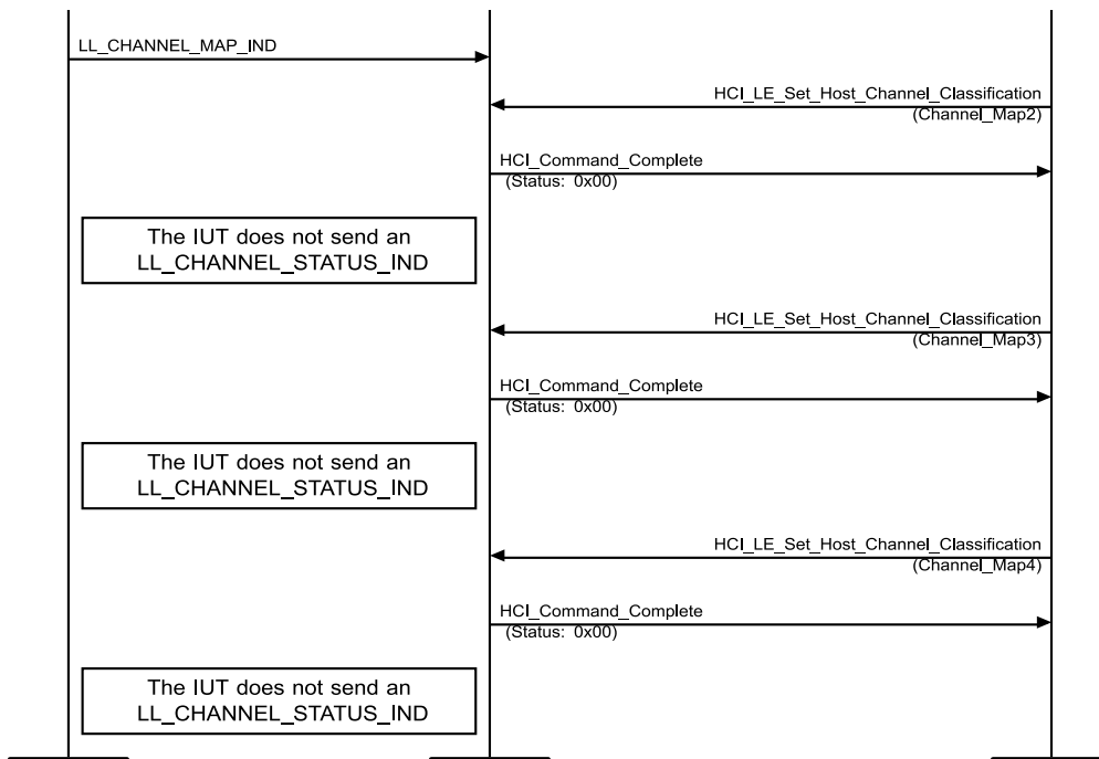
Figure 4.6-4: LL/FRH/PER/BV-03-C [Send Channel Status Update] – MSC Page 2 of 2
