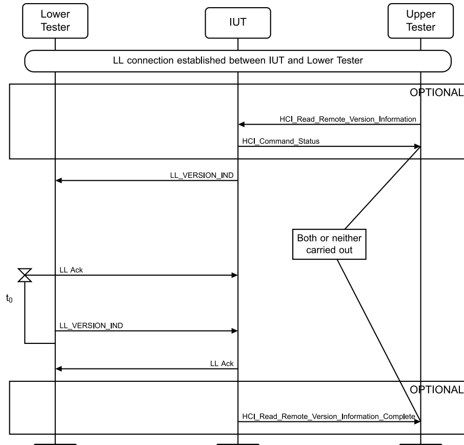
Figure 4.3-256: Version Exchange, IUT Requesting, Delayed Response MSC
