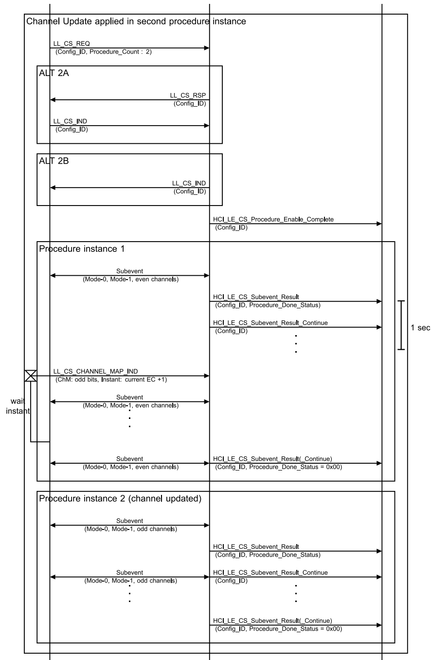
Figure 4.14-48: Channel Map Update during CS Procedure MSC – Page 3 of 4
