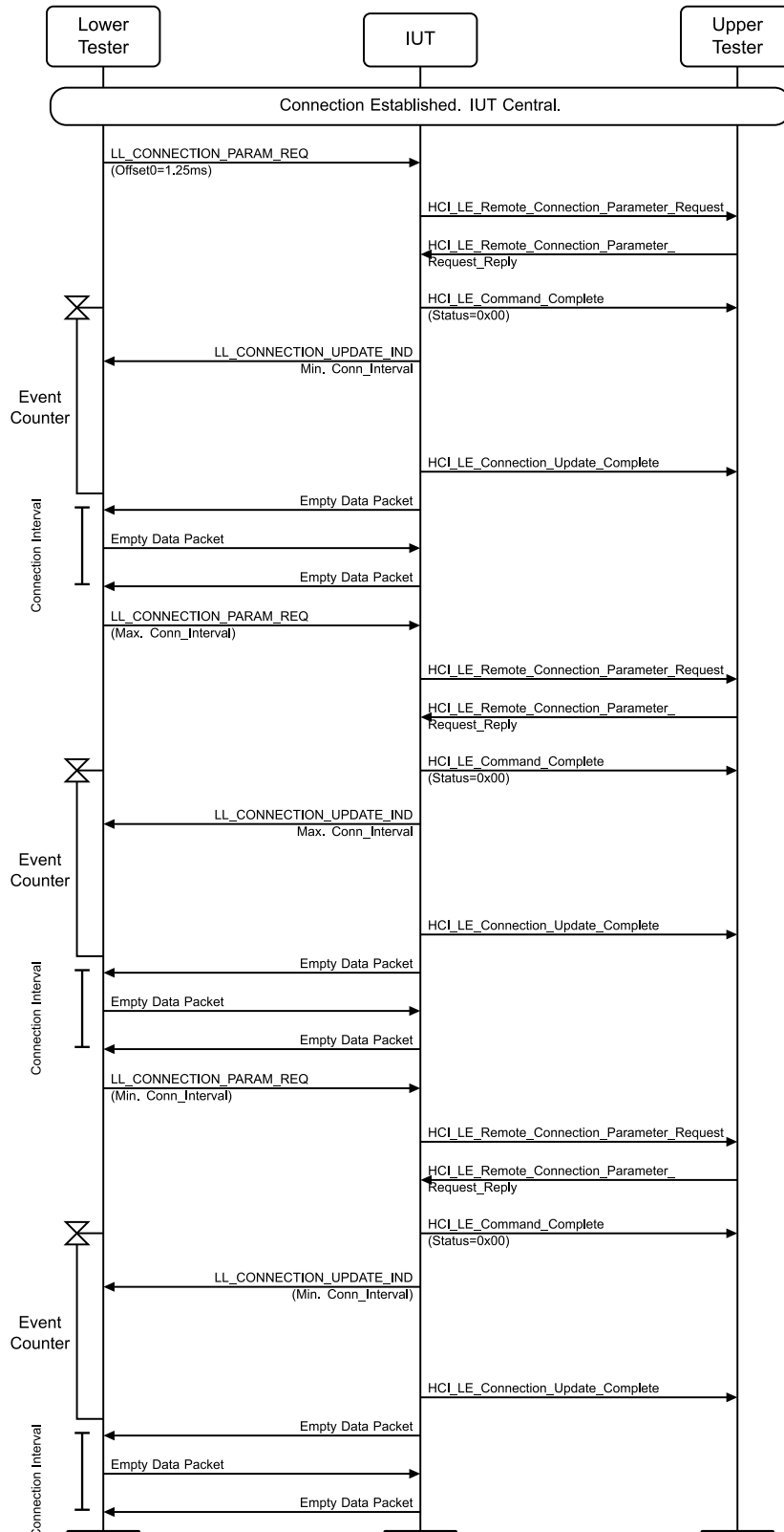
Figure 4.3-161: LL/CON/CEN/BV-31-C [Accepting Connection Parameter Request – preferred anchor points only] MSC
