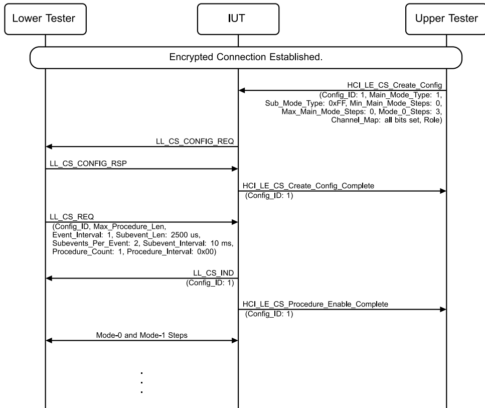
Figure 4.14-56: Reject Connection Subrate During CS Procedure MSC – Page 1 of 2
