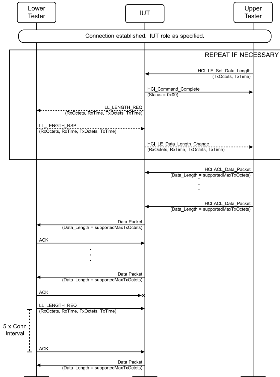
Figure 4.3-243: Data Length Update – Retransmission During an Update MSC
