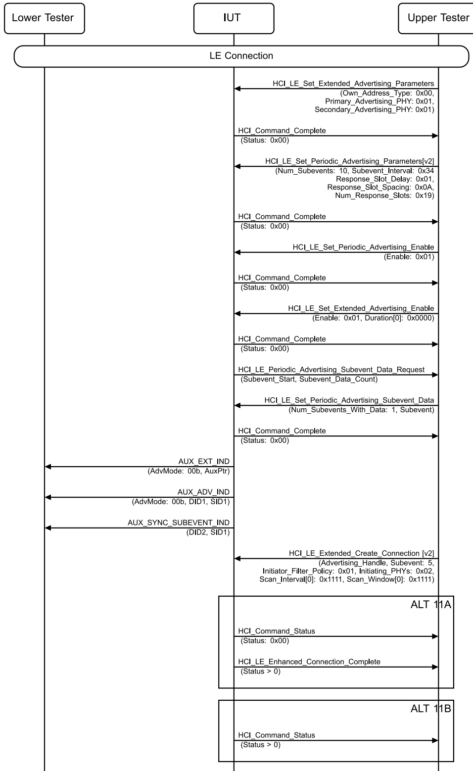
Figure 4.2-68: Reject Connection Request When Connected to a Peer, Periodic Advertising with Responses MSC
