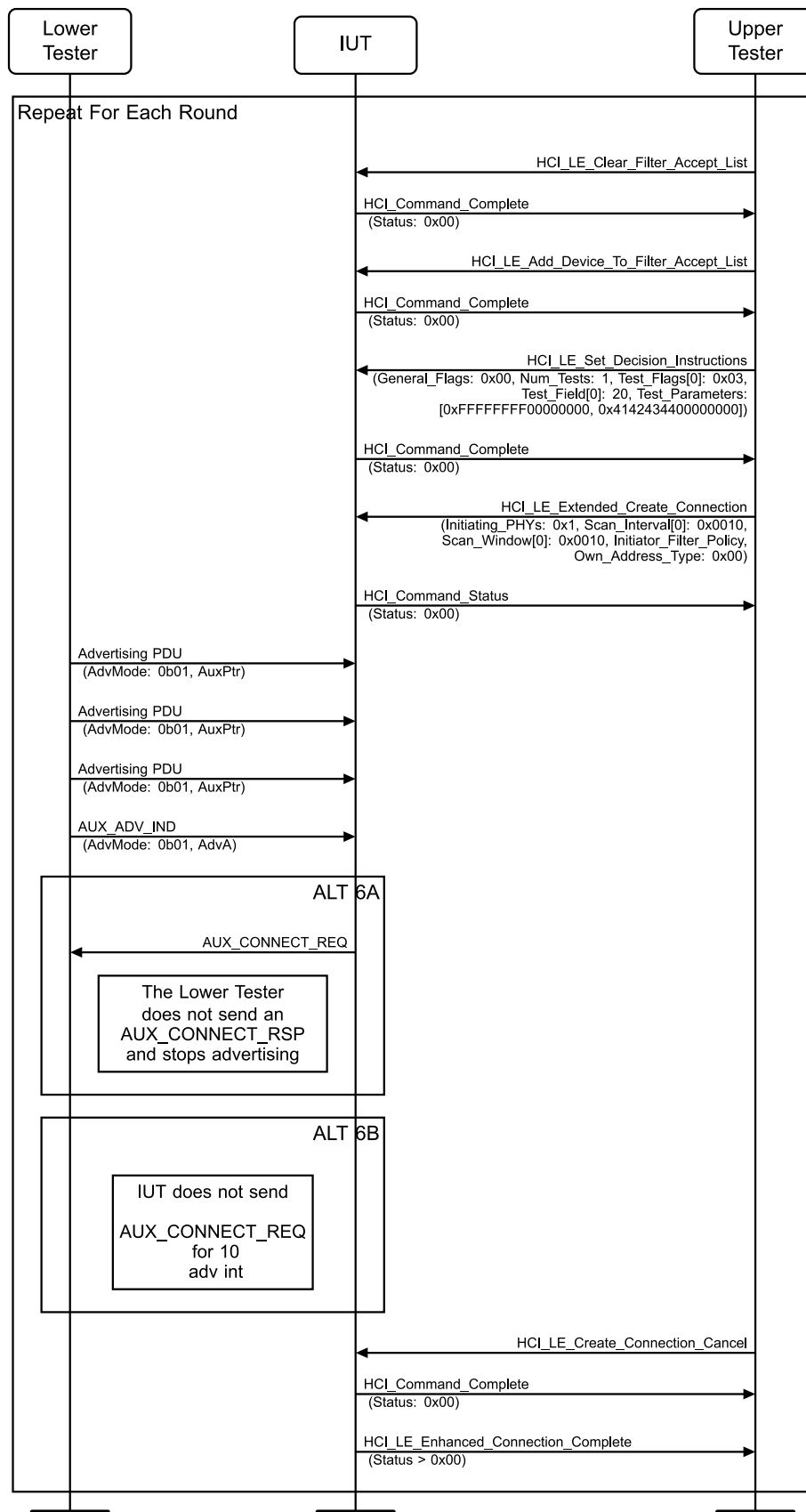
Figure 4.3-46: Extended Scanning, Connection Initiation, Decision-Based Advertising, Initiator Filter Policy MSC
