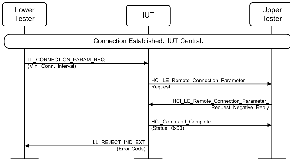
Figure 4.3-164: LL/CON/CEN/BV-35-C [Accepting Connection Parameter Request – Host rejects] MSC
