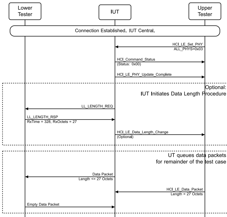
Figure 4.3-181: LL/CON/CEN/BV-55-C [Mandatory Minimum PDU Length, LE Coded] MSC – Page 1 of 2
