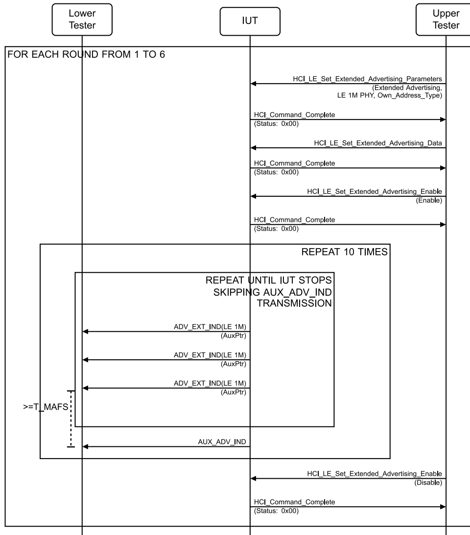
Figure 4.2-24: Extended Advertising, Overlapping Extended Advertising Events MSC
