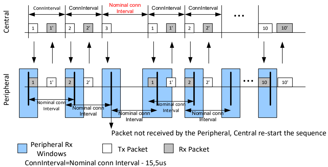
Figure 4.4-7: LL/TIM/PER/BV-04-C Timing sequence
