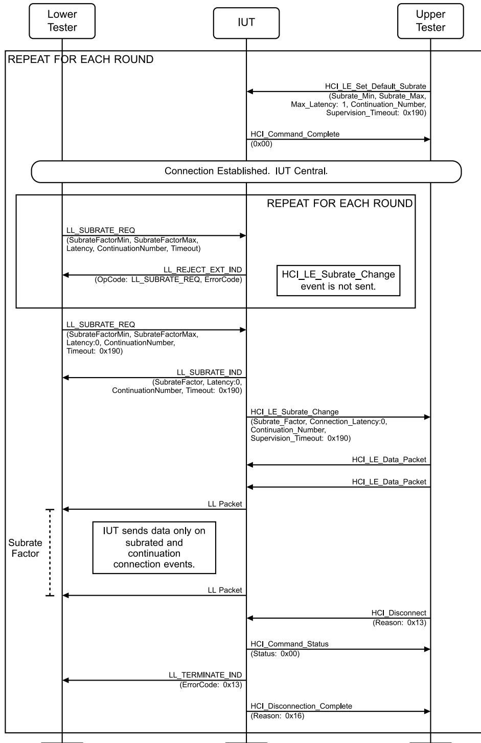
Figure 4.3-198: LL/CON/CEN/BV-137-C [Set the Default Subrate Factor] MSC
