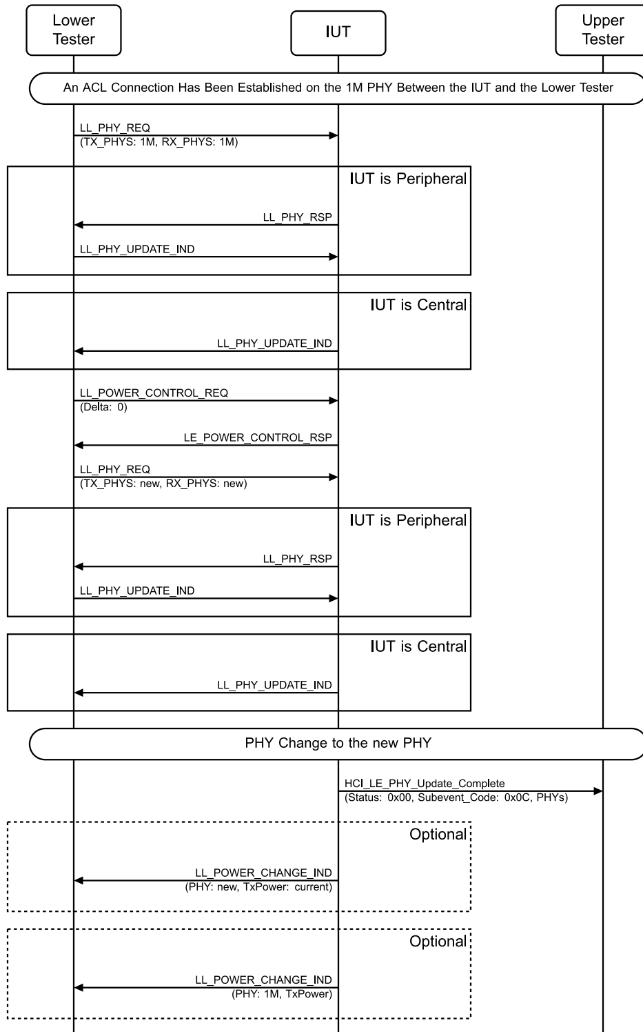
Figure 4.13-8: Power Change Indication on PHY Change MSC
