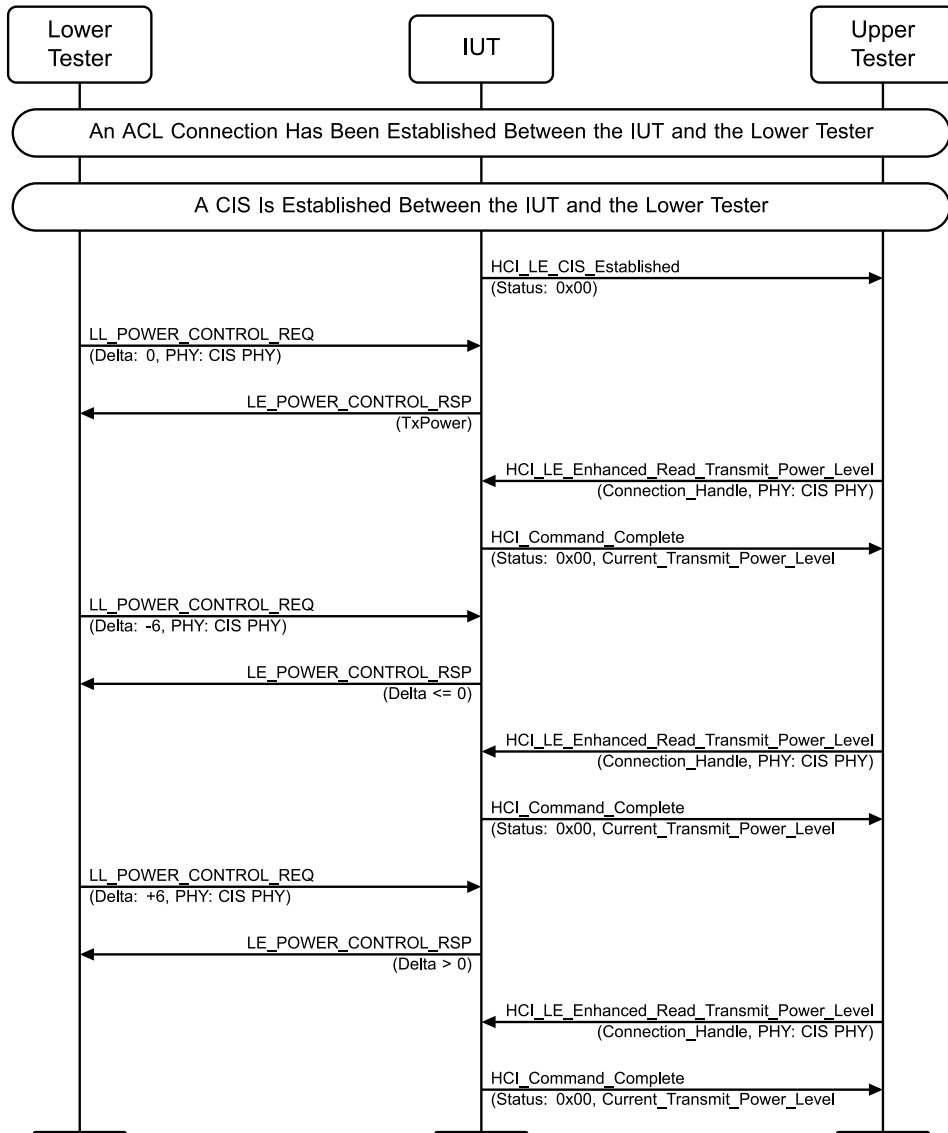
Figure 4.13-10: Power Control Response when a CIS has been established MSC
