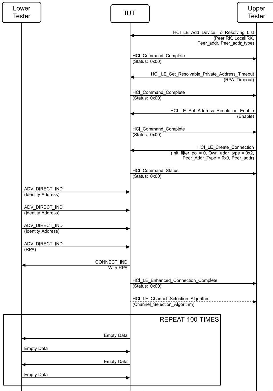
Figure 4.3-30: Network Privacy – Connection Establishment using directed advertising with identity address and resolving list, Initiator MSC
