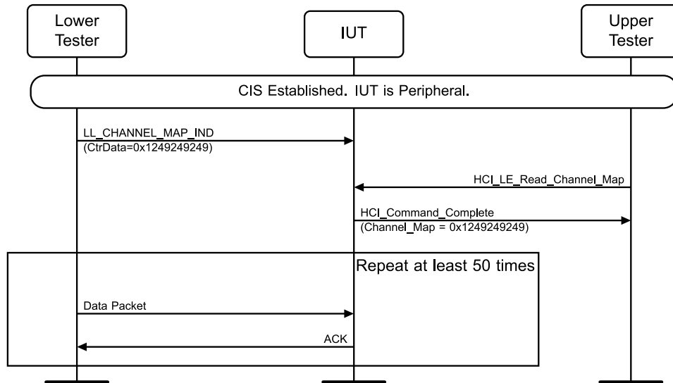
Figure 4.10-29: CIS Map Update MSC
