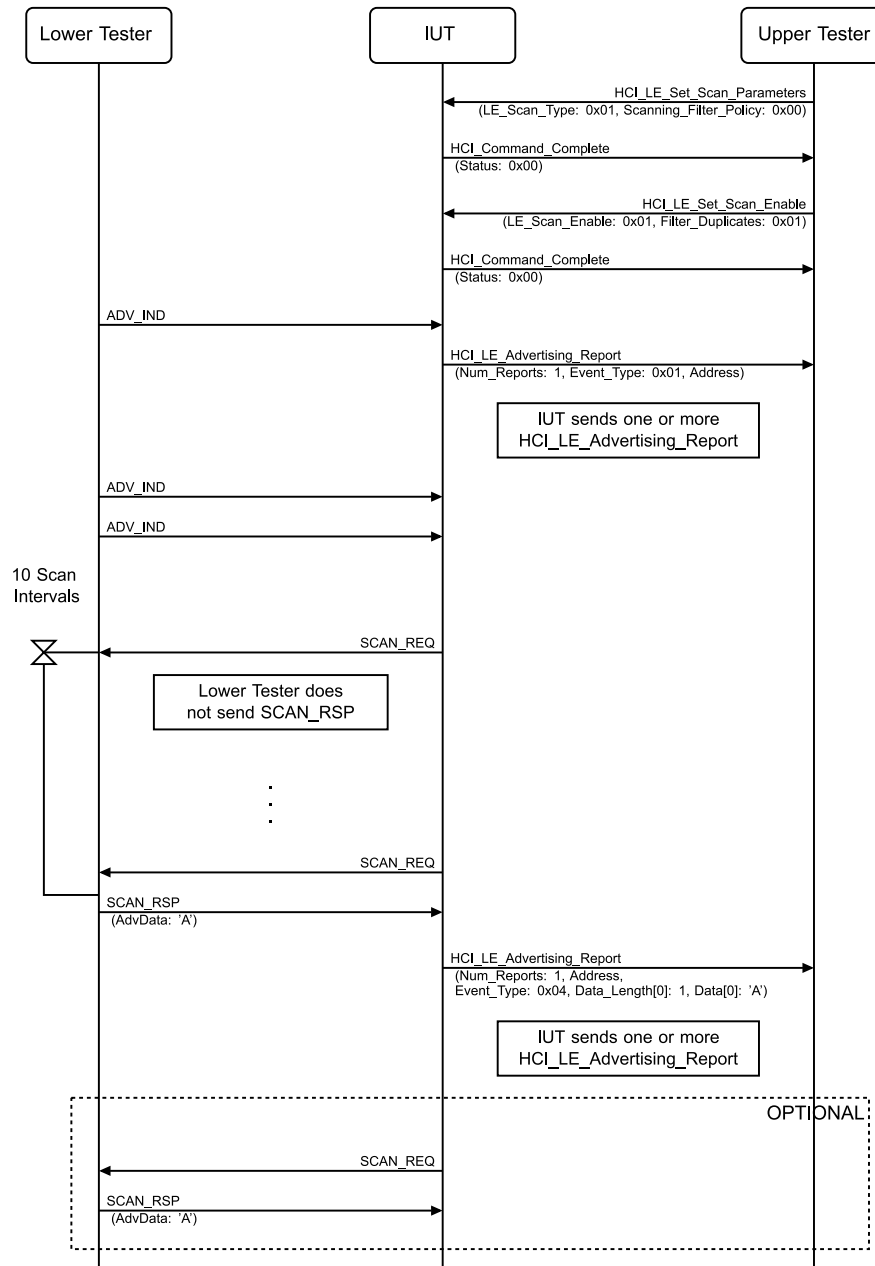
Figure 4.2-152: LL/DDI/SCN/BV-127-C [Active Scanning, Duplicate Filtering] MSC
