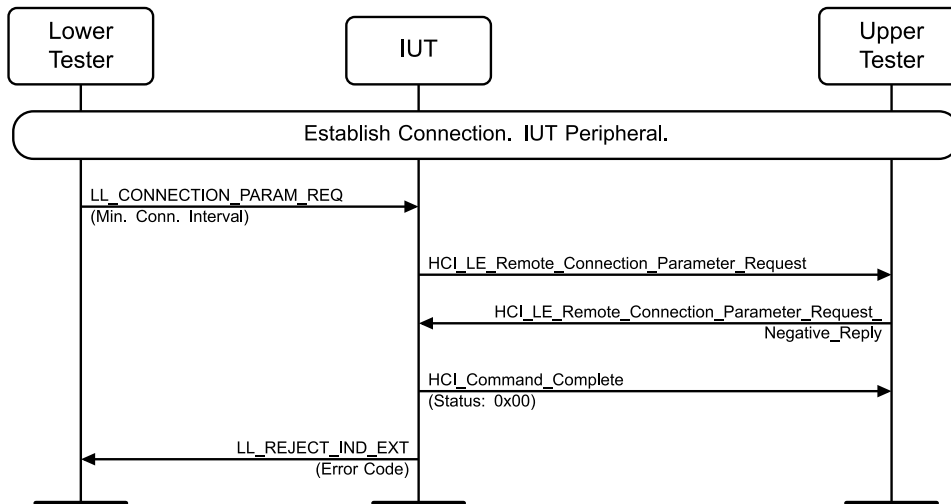
Figure 4.3-75: LL/CON/PER/BV-34-C [Accepting Connection Parameter Request – Host rejects] MSC
