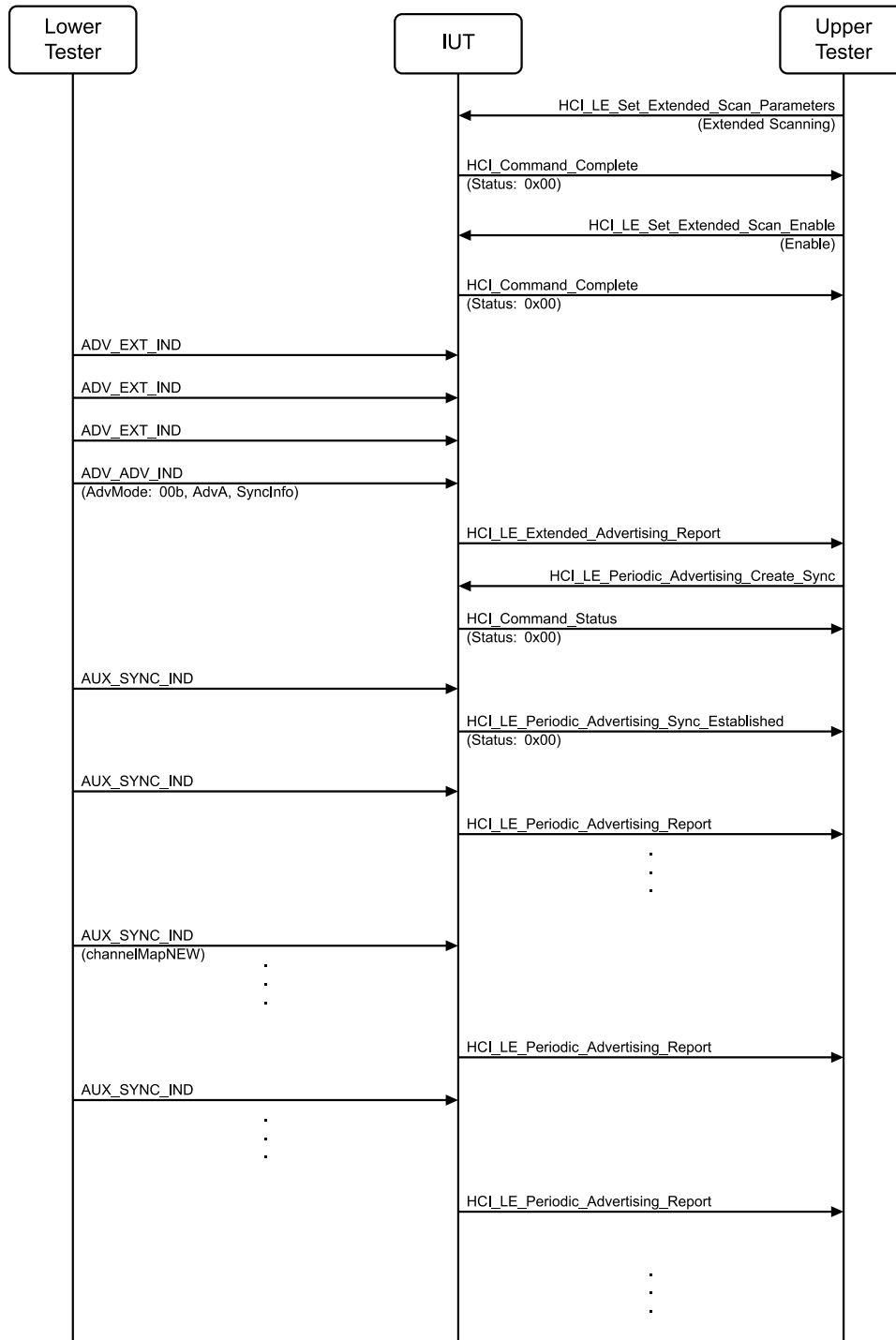
Figure 4.2-111: LL/DDI/SCN/BV-67-C [Periodic Advertising Reception, Channel Map Update] MSC
