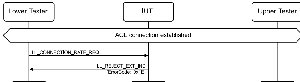
Figure 4.3-212: LL/CON/CEN/BI-23-C [Reject Peer Connection Rate Request, invalid parameters] MSC
