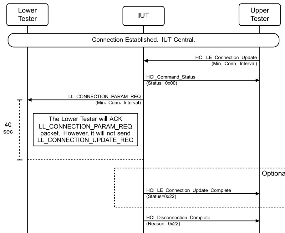
Figure 4.3-192: LL/CON/CEN/BI-05-C [Initiating Connection Parameter Request – Timeout] MSC
