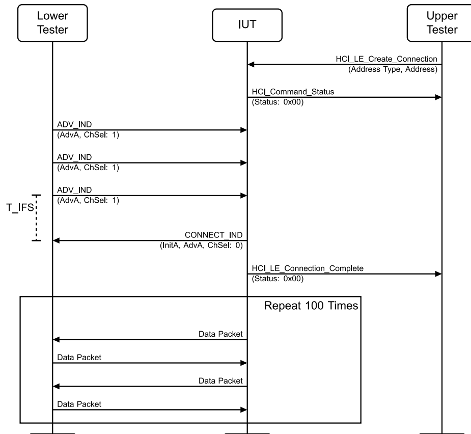
Figure 4.3-39: LL/CON/INI/BV-22-C [Connection Initiation, Channel Selection Algorithm #1] MSC
