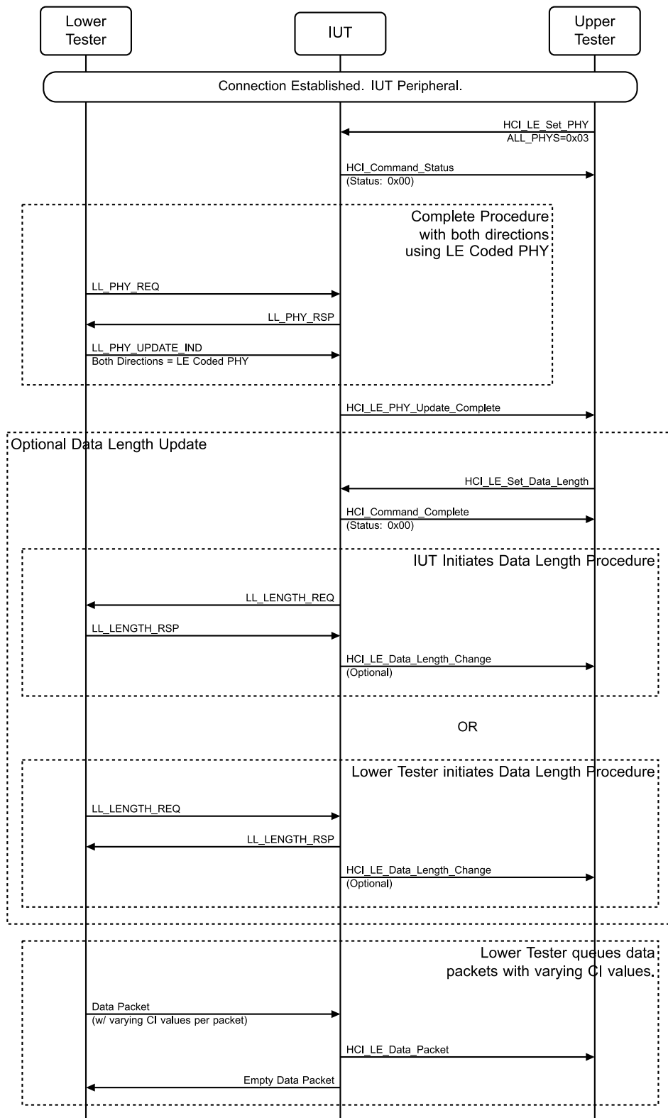
Figure 4.3-92: LL/CON/PER/BV-54-C [Peripheral Receiving Data, LE Coded, CI Change] MSC
