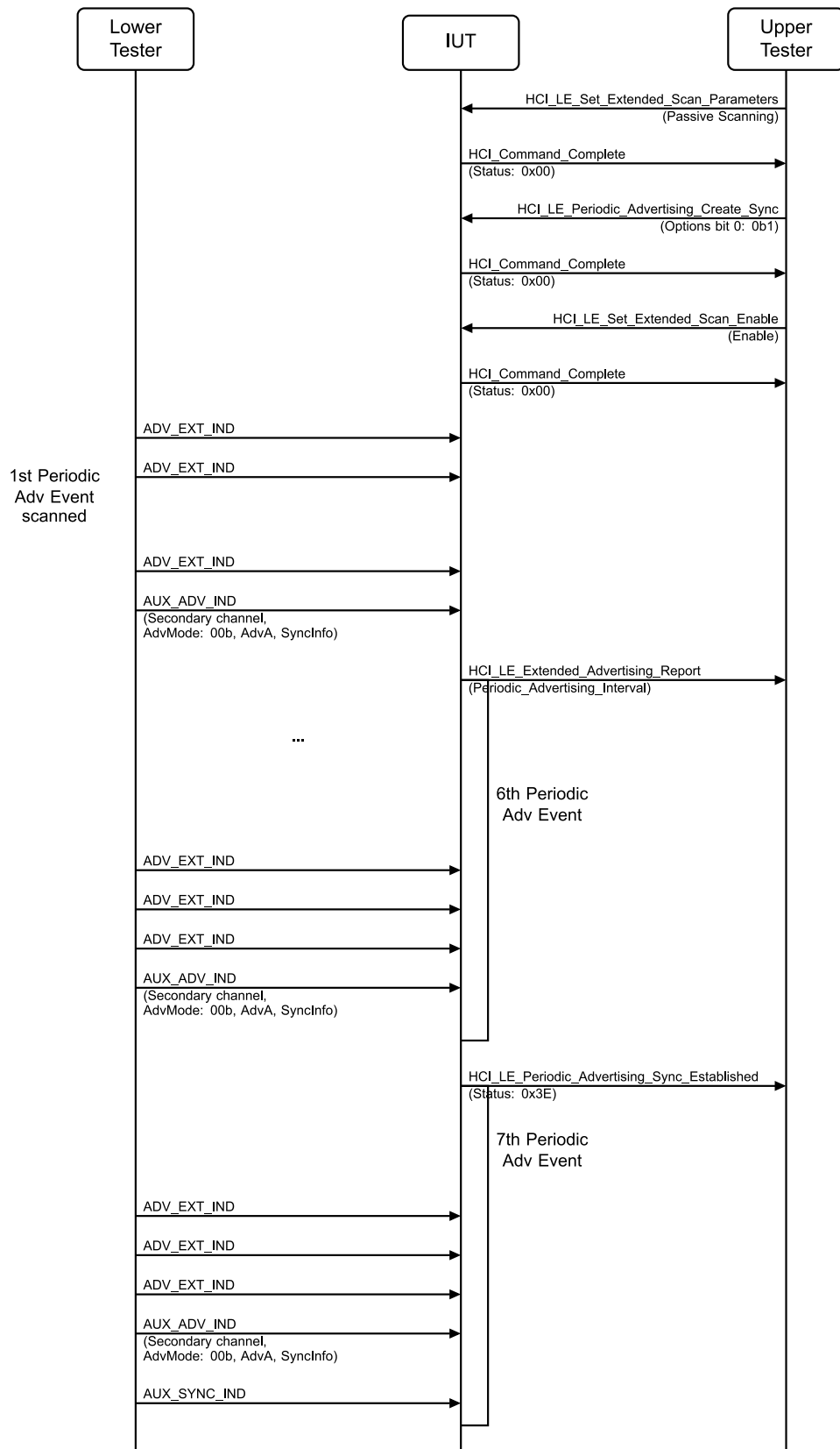
Figure 4.2-106: LL/DDI/SCN/BV-37-C [First AUX_SYNC_IND Never Received] MSC
