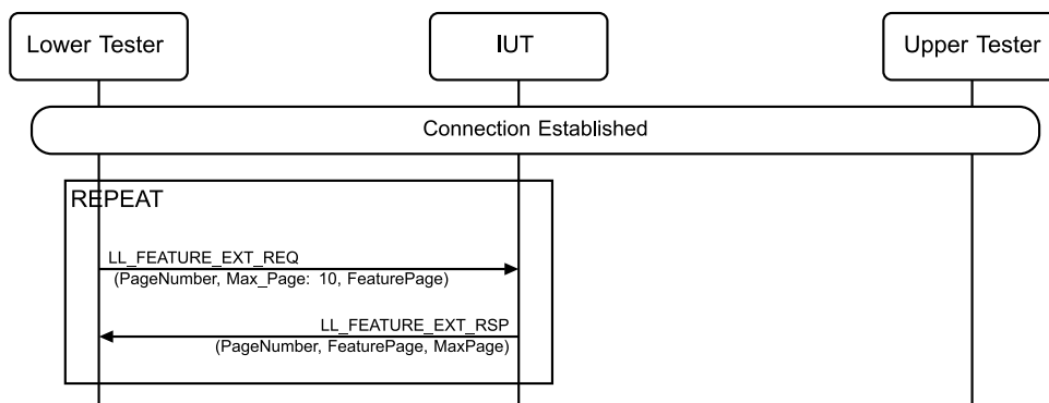
Figure 4.3-262: LL Extended Feature Set Response MSC
