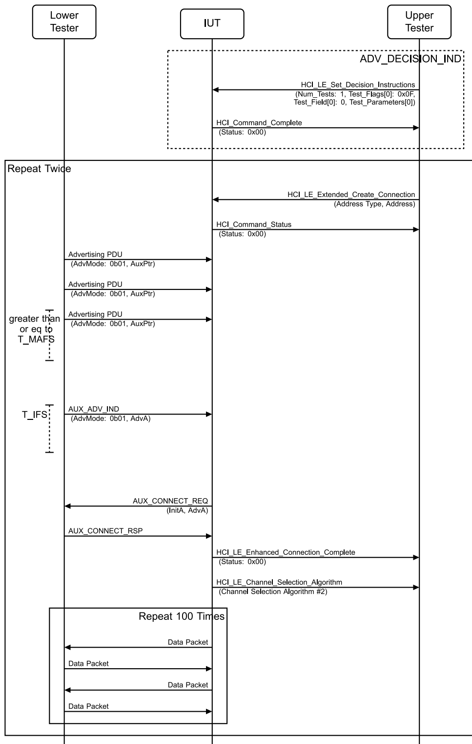
Figure 4.3-31: Extended Scanning, Connection Initiation MSC
