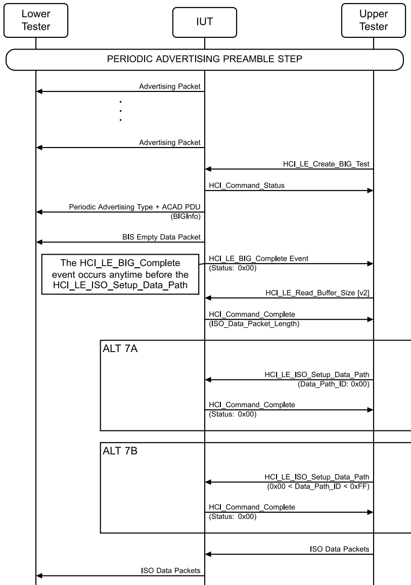
Figure 4.11-1: Broadcast Isochronous Stream Setup MSC
