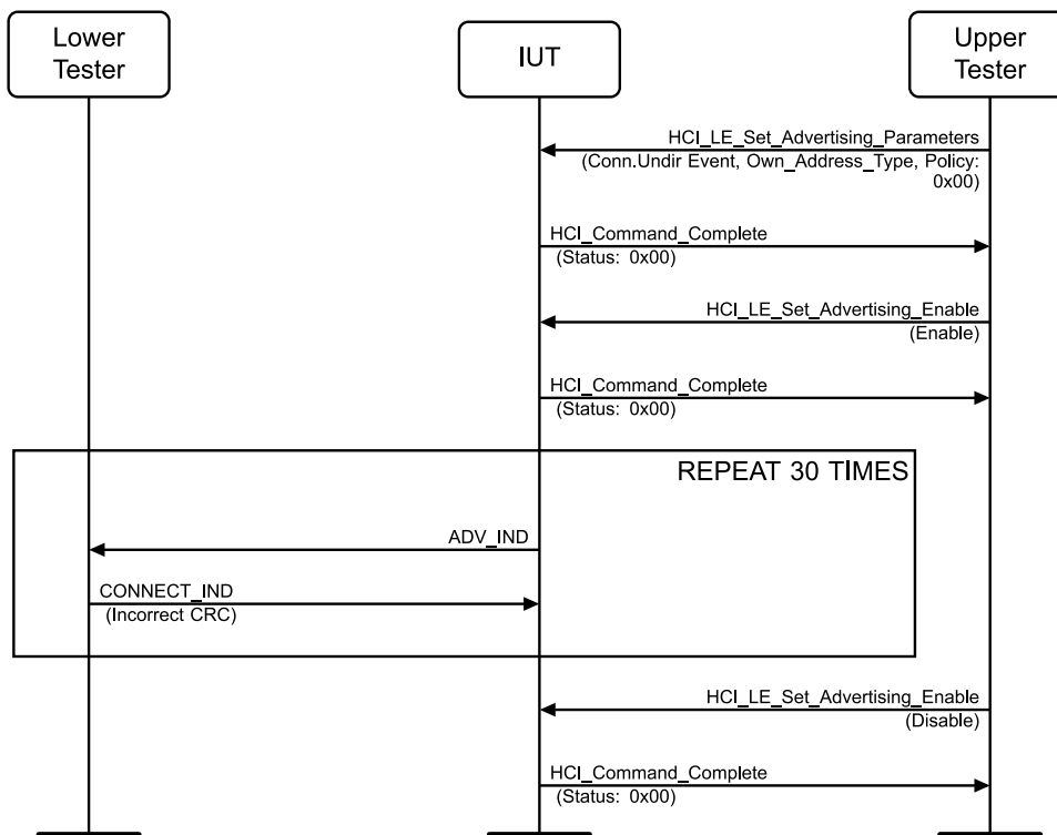
Figure 4.2-14: LL/DDI/ADV/BI-02-C [Connection Request Invalid CRC] MSC
