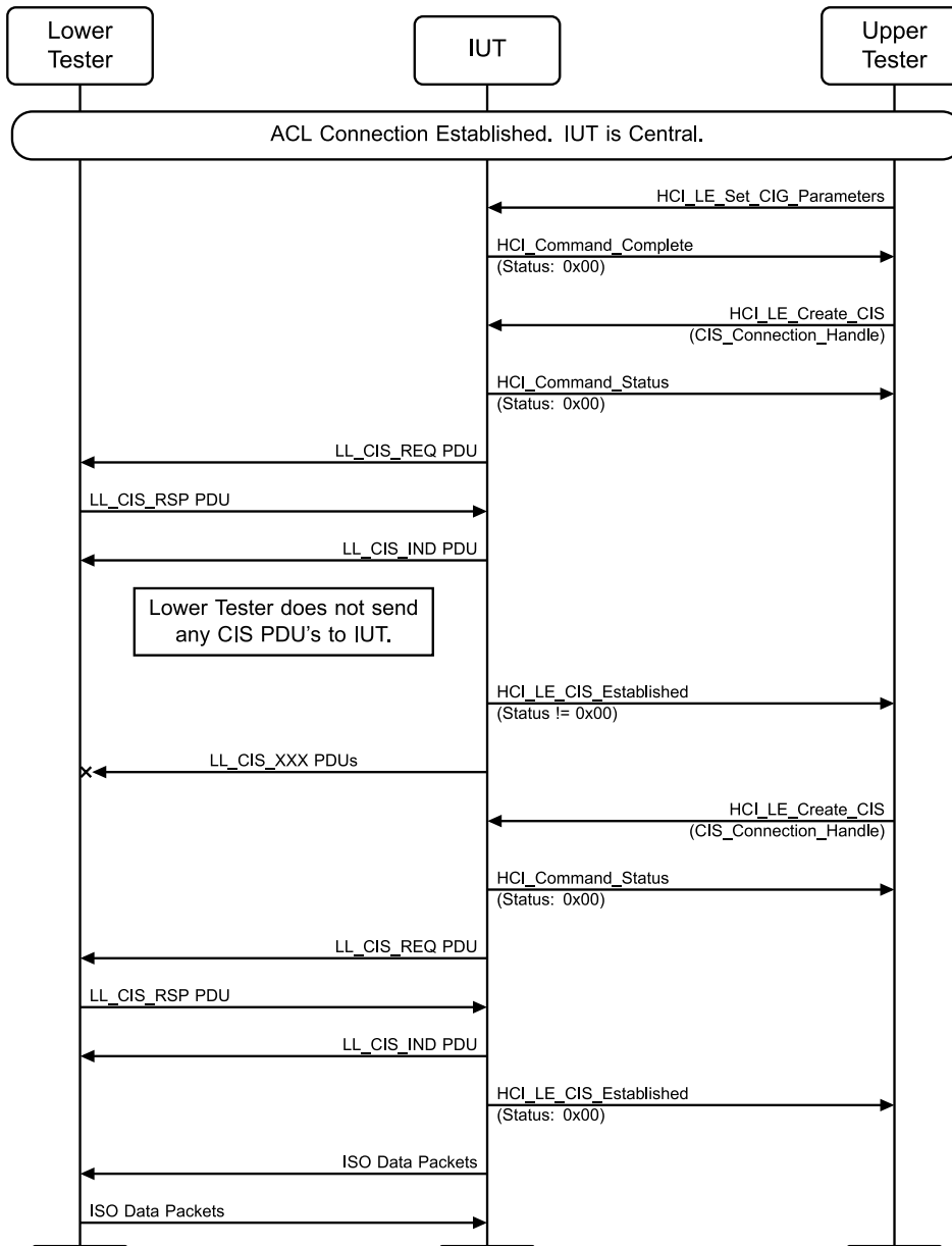
Figure 4.10-16: LL/CIS/CEN/BV-33-C [CIS Considered Lost before Establishment, Central] MSC
