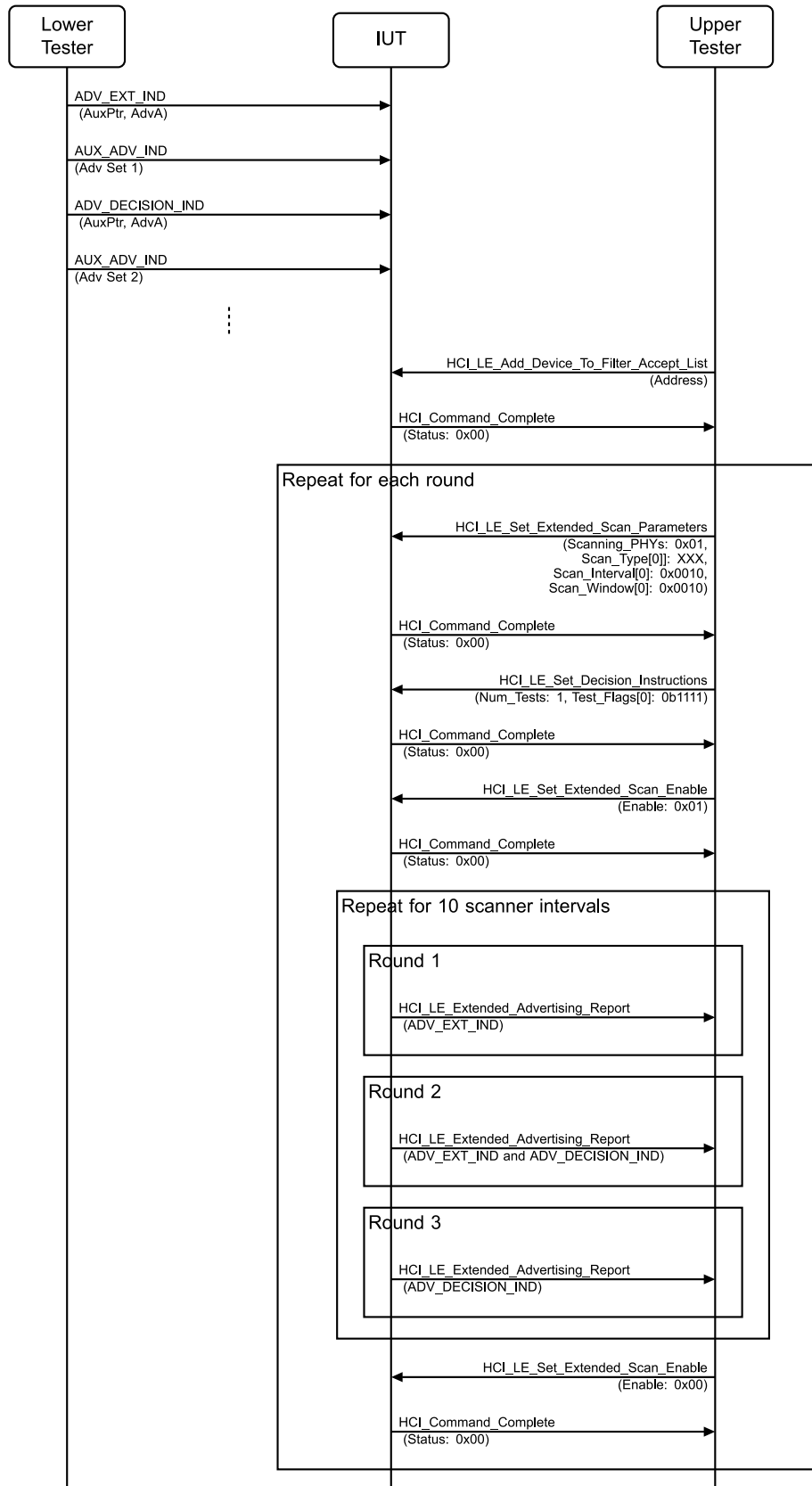
Figure 4.2-143: Decision-Based Advertisements, Ignore Non-Decision PDUs MSC
