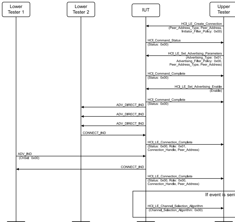
Figure 4.3-42: Parallel connection requests, incoming connect indication first MSC
