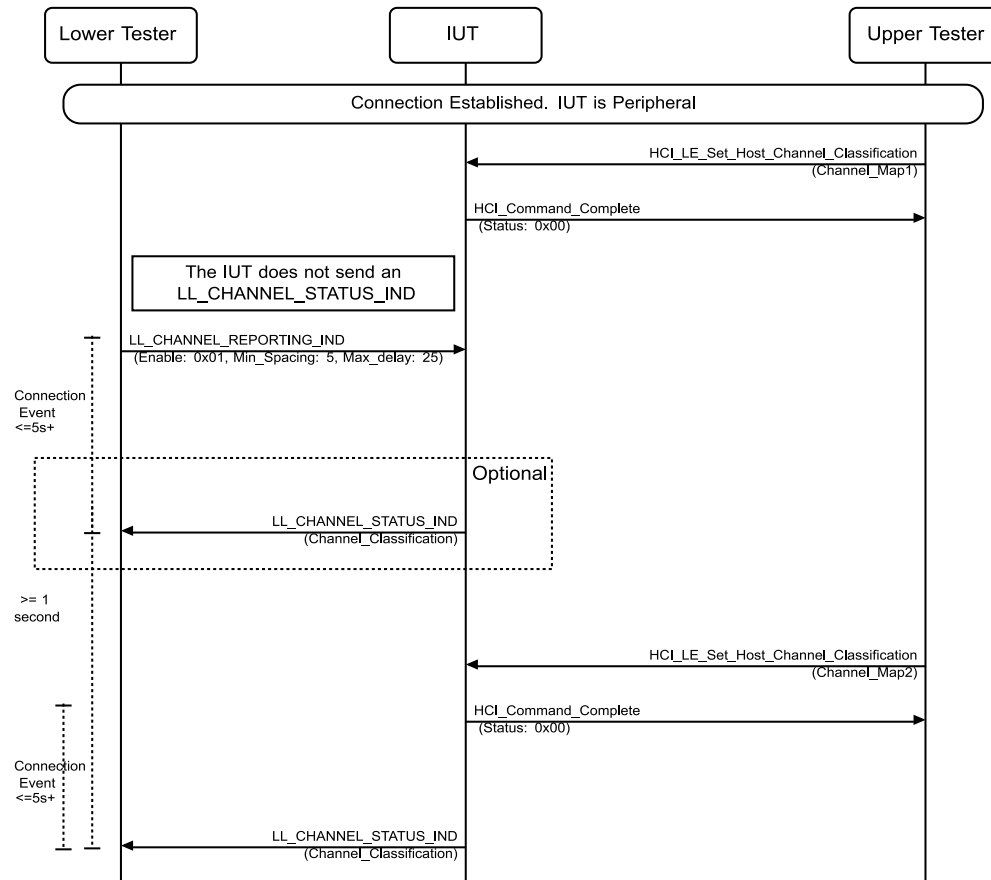
Figure 4.6-3: LL/FRH/PER/BV-03-C [Send Channel Status Update] – MSC Page 1 of 2
