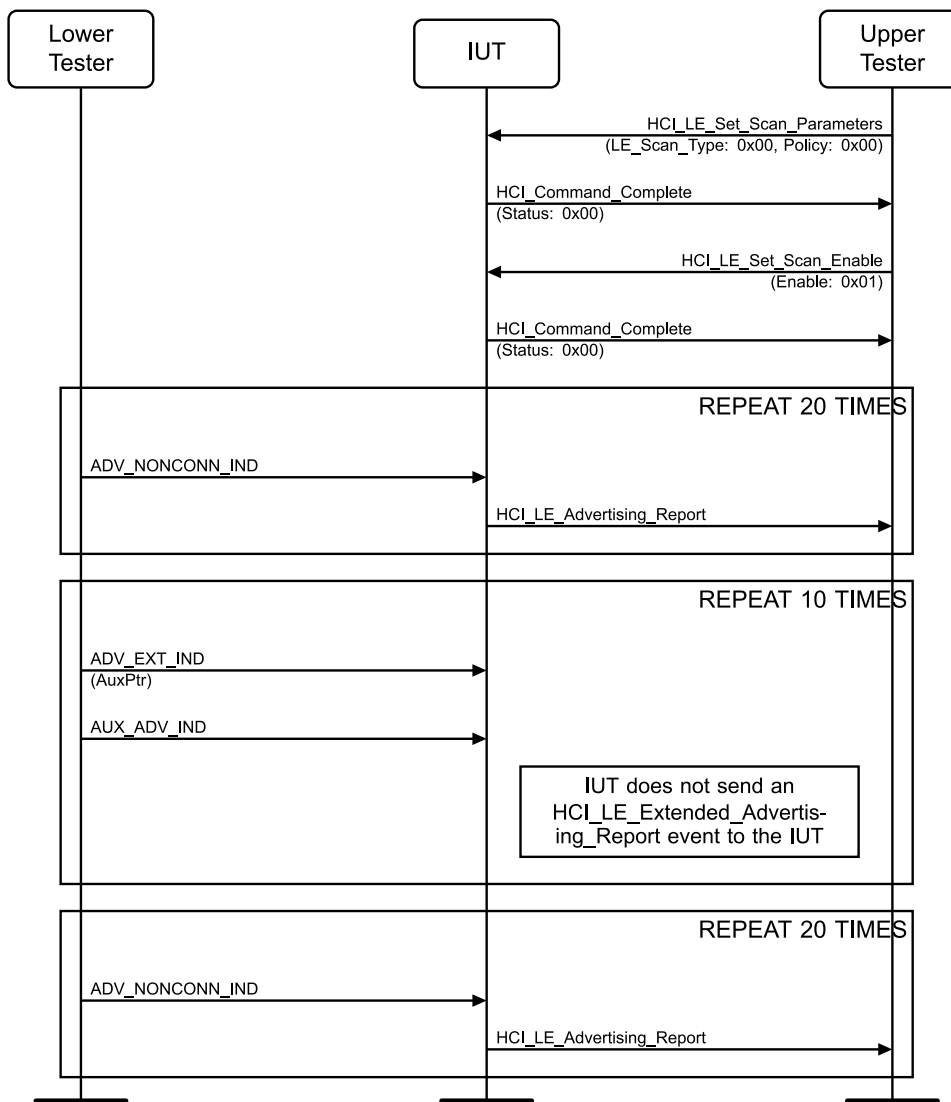
Figure 4.2-121: LL/DDI/SCN/BV-74-C [Legacy Scanning Ignore Extended Advertising Packets] MSC
