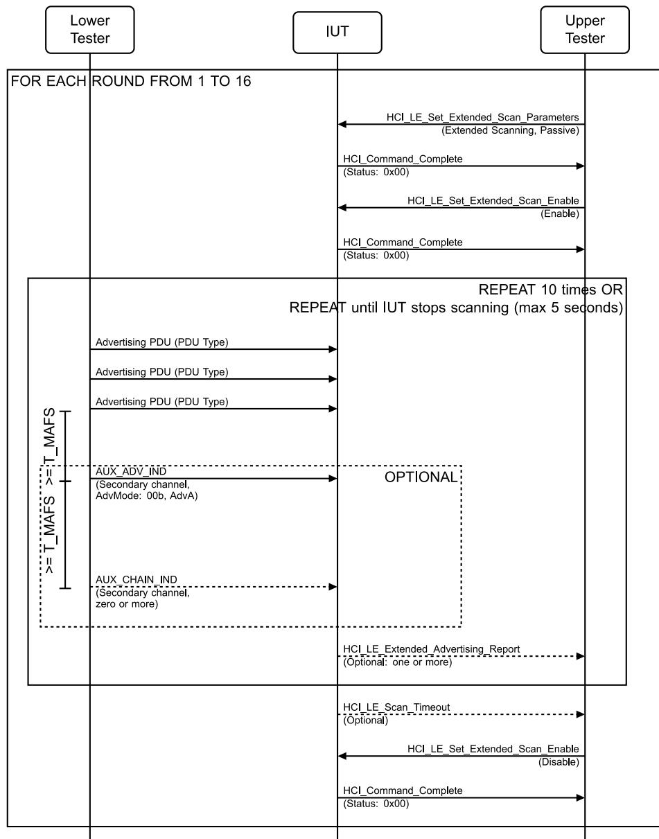
Figure 4.2-88: Extended Scanning, Passive MSC
