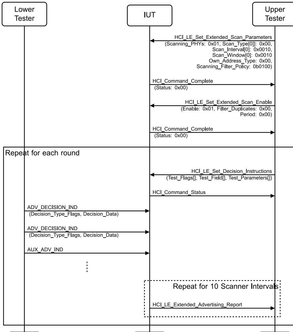
Figure 4.2-139: Decision-Based Advertisements, Test Groups MSC
