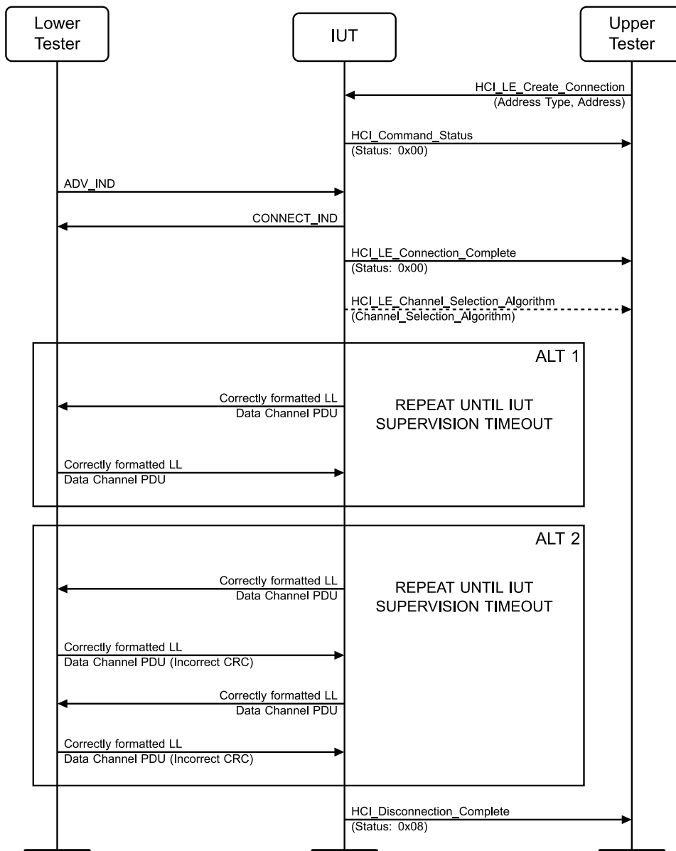
Figure 4.3-38: Peripheral packets Invalid CRC MSC
