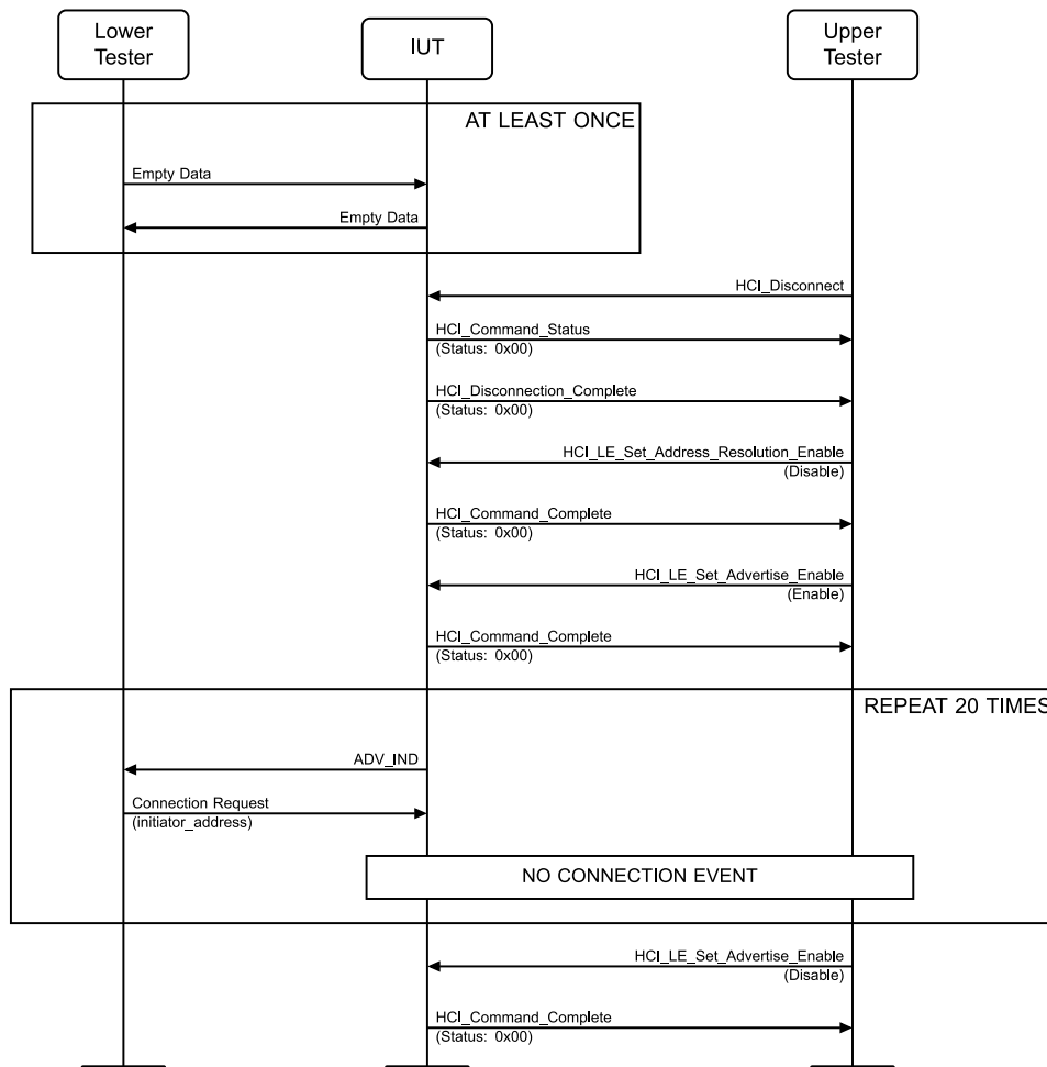
Figure 4.8-8: Network Privacy - Undirected Connectable Advertising with Local IRK and Peer IRK MSC – Page 2 of 2
