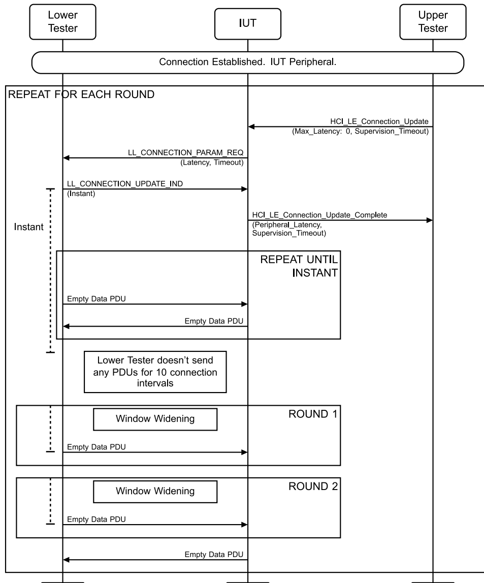
Figure 4.3-127: LL/CON/PER/BV-158-C [Listening for Packet With Window Widening, ACL] MSC
