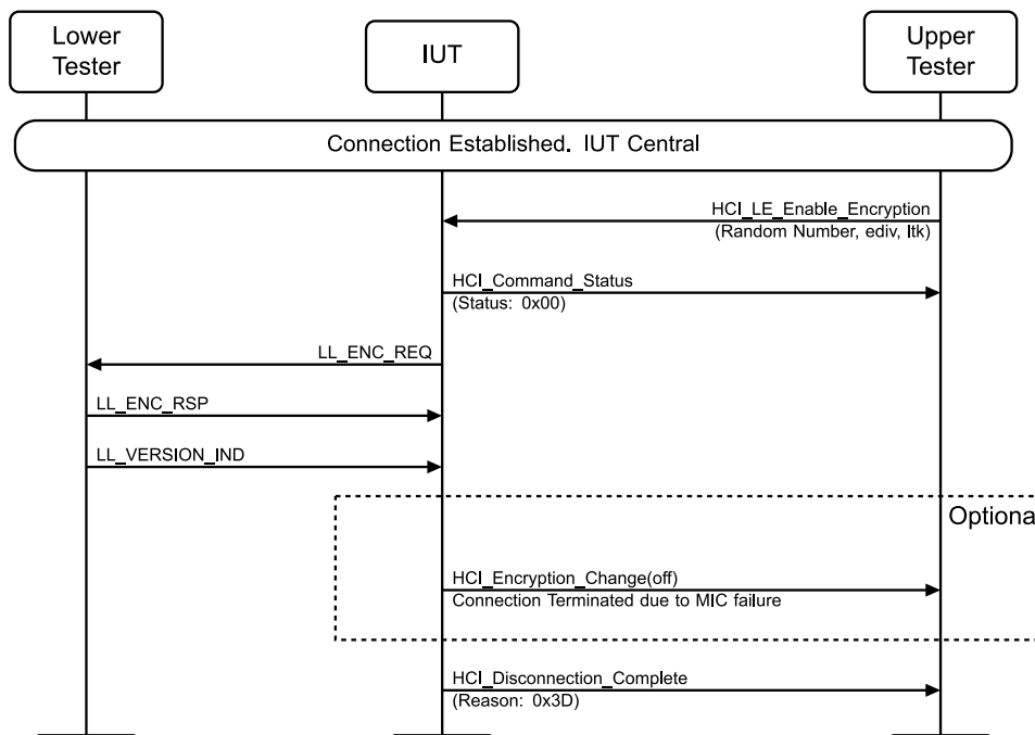
Figure 4.8-53: LL/SEC/CEN/BV-14-C [Central Receiving unexpected Data Channel PDU during encryption start] MSC
