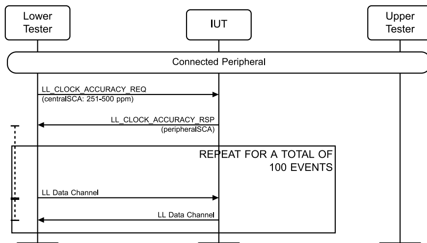
Figure 4.4-11: LL/TIM/PER/BV-09-C [Response to Sleep Clock Accuracy Update] MSC
