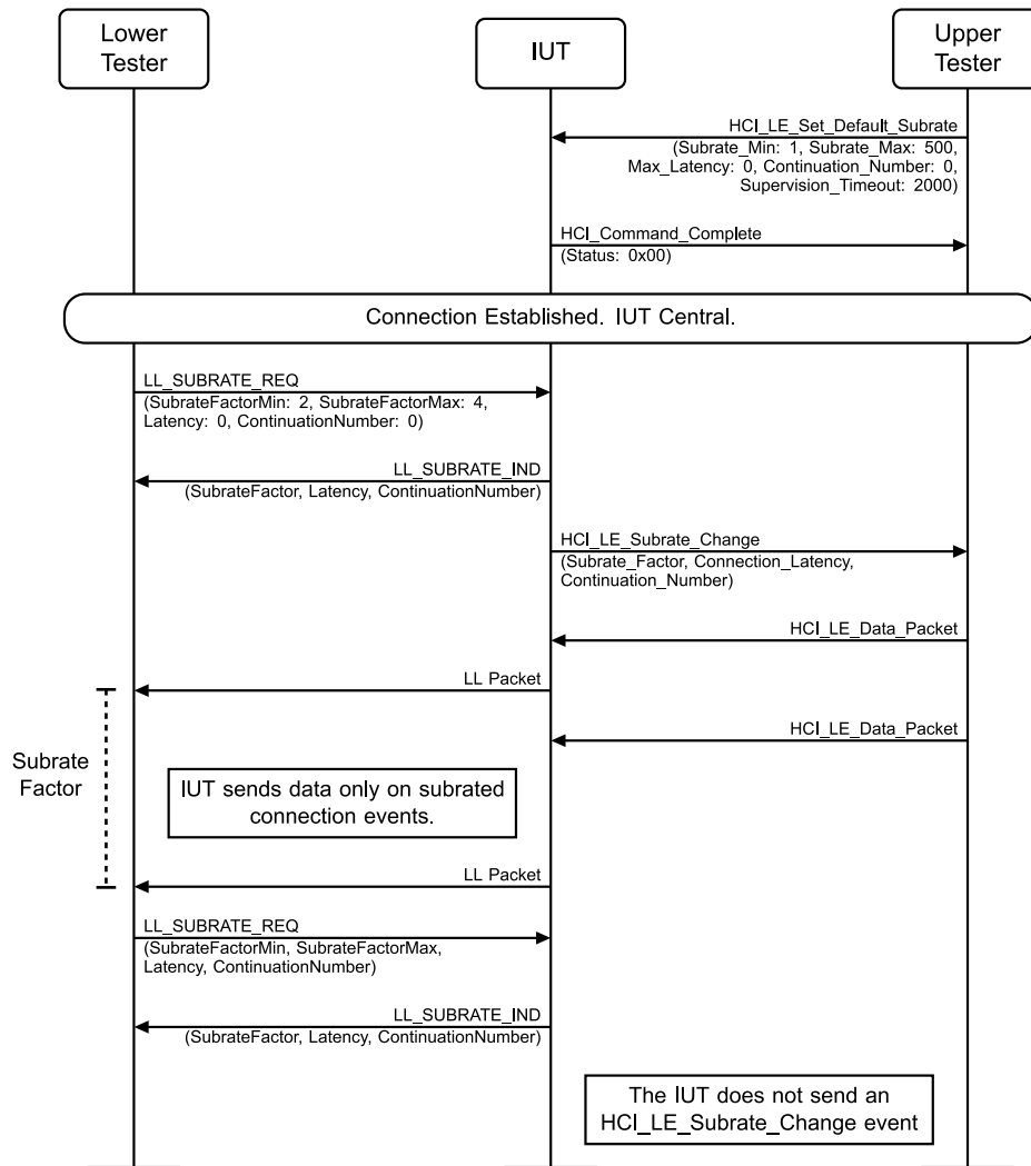
Figure 4.3-195: LL/CON/CEN/BV-135-C [Accept an Incoming Subrate Change Request] MSC
