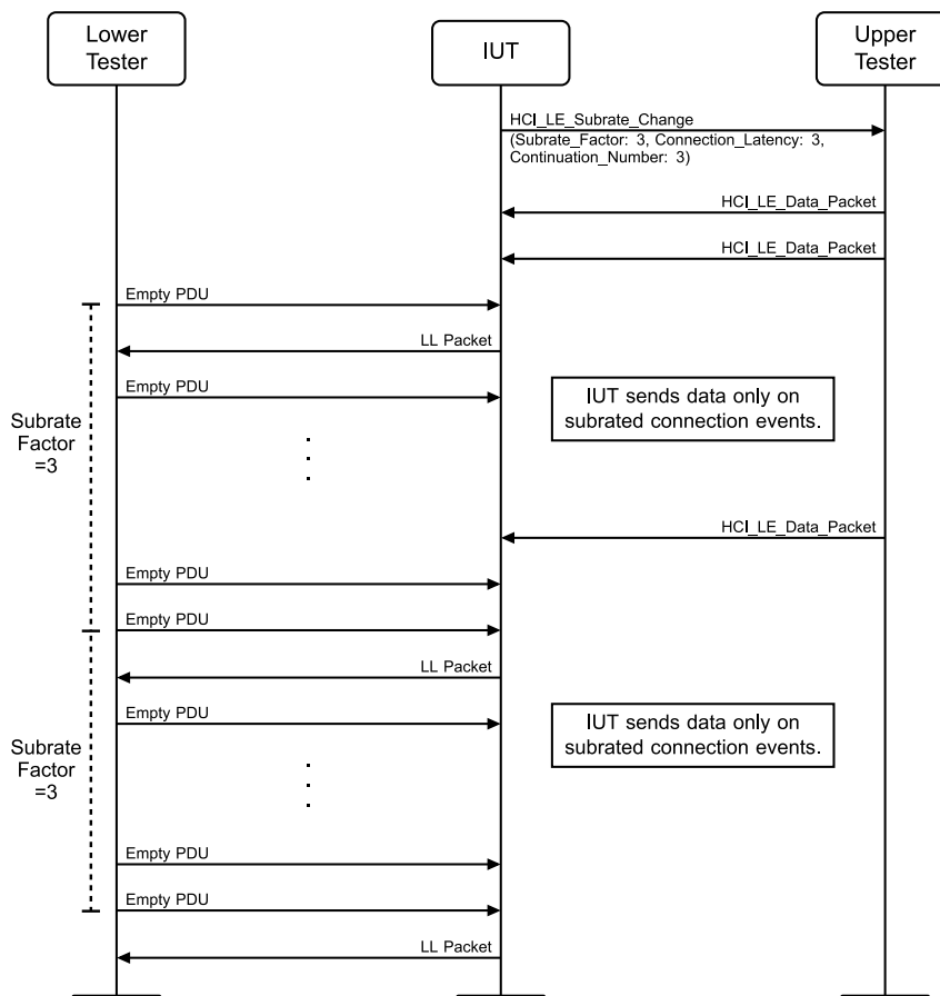
Figure 4.3-120: LL/CON/PER/BV-144-C [Receiving a Delayed Connection Change Update After the Event Counter Wraps] MSC – Page 2 of 2
