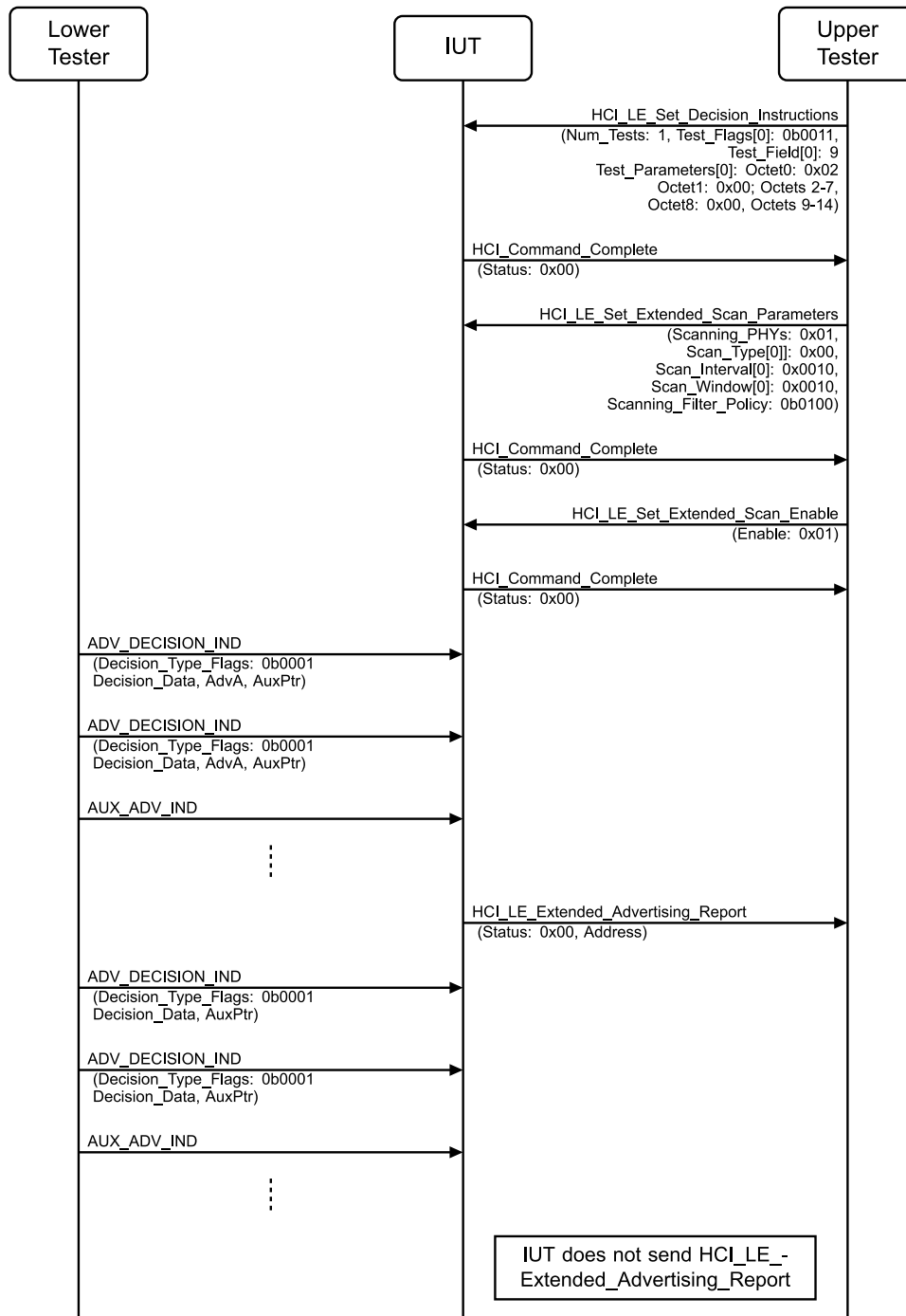
Figure 4.2-145: Decision-Based Advertisements, AdvA in Decision PDU MSC – Page 1 of 2
