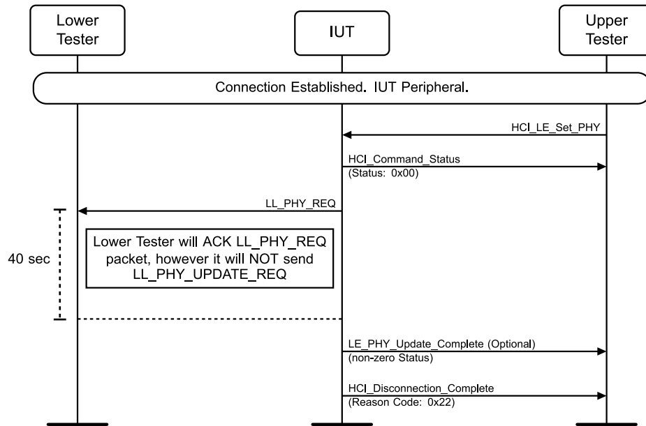
Figure 4.3-79: LL/CON/PER/BV-45-C [Protocol Timeout for PHY Update Procedure] MSC
