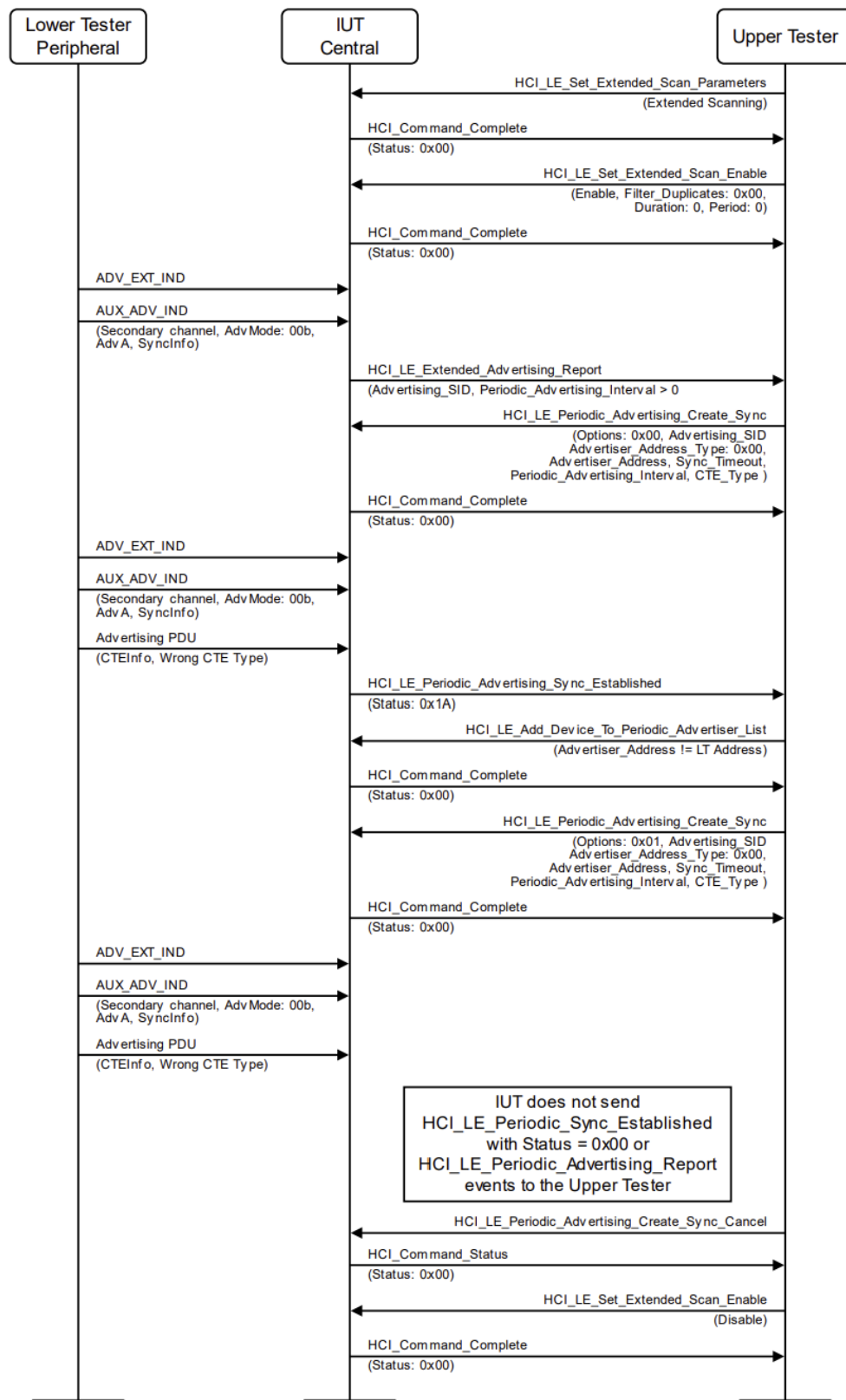
Figure 4.2-104: Connectionless CTE Scanning, Filter Wrong CTE Types on Synchronization MSC
