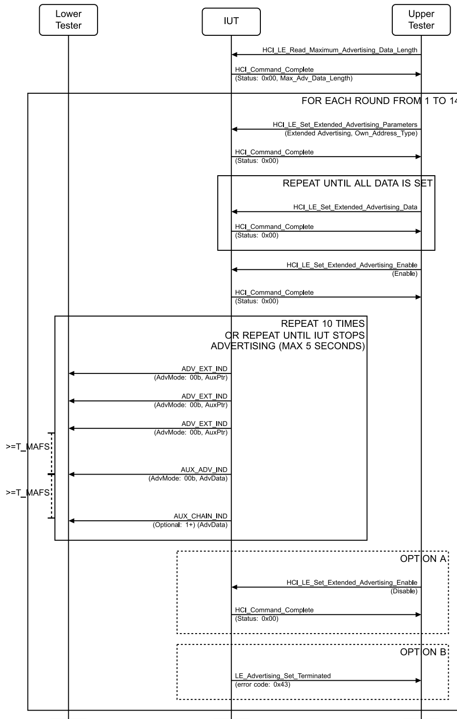
Figure 4.2-19: Extended Advertising, Secondary Channel, Non-Connectable MSC
