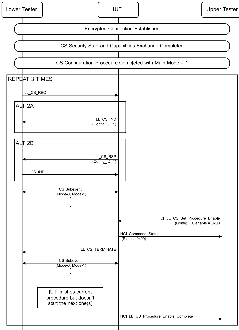
Figure 4.14-53: CS Procedure, Send Repeat Termination MSC
