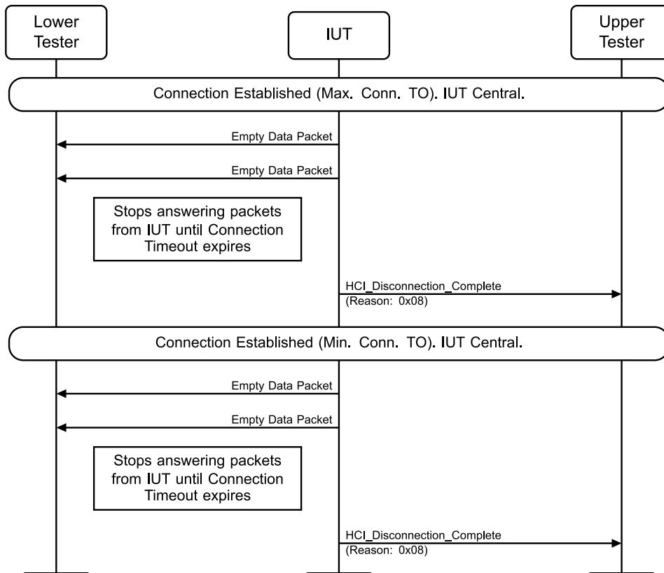
Figure 4.3-141: LL/CON/CEN/BV-10-C [Central Supervision Timer] MSC
