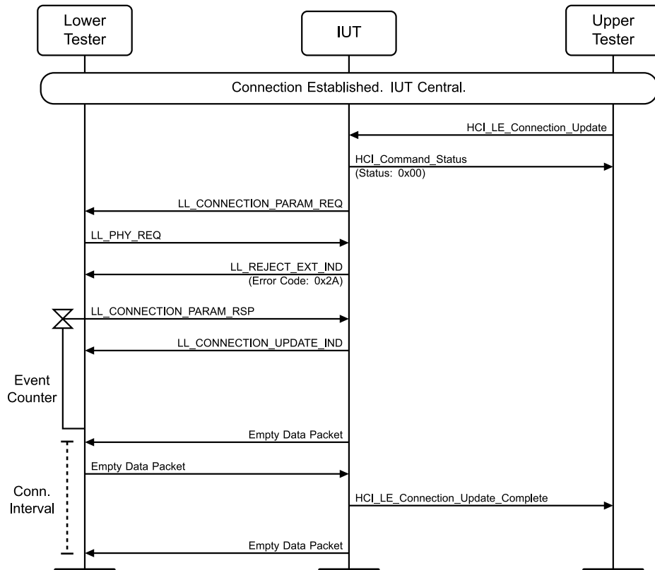
Figure 4.3-170: LL/CON/CEN/BV-48-C [Handling Protocol Collision – Different Procedure – Connection Parameters] MSC
