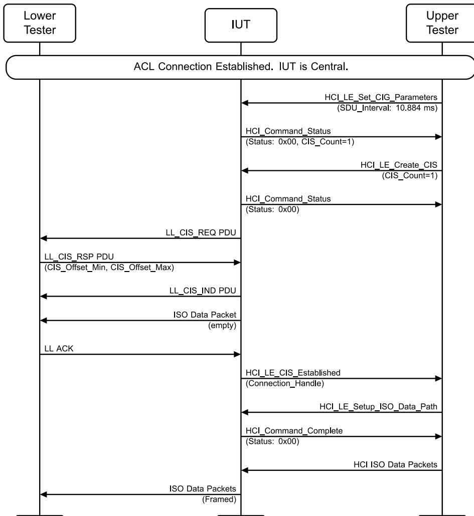
Figure 4.10-17: Connected Isochronous Stream Using Non-Test Command, Force Framed PDUs MSC
