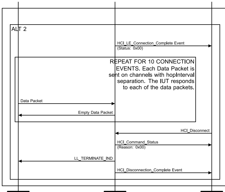
Figure 4.2-49: LL/DDI/ADV/BI-07-C [Connection Request Invalid hopIncrement] MSC – Page 2 of 2
