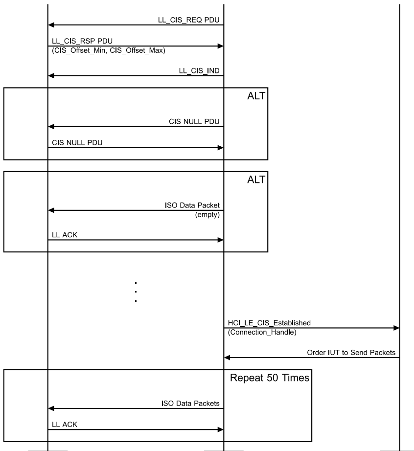
Figure 4.10-2: CIS Setup Procedure, Central Initiated MSC – Page 2 of 2
