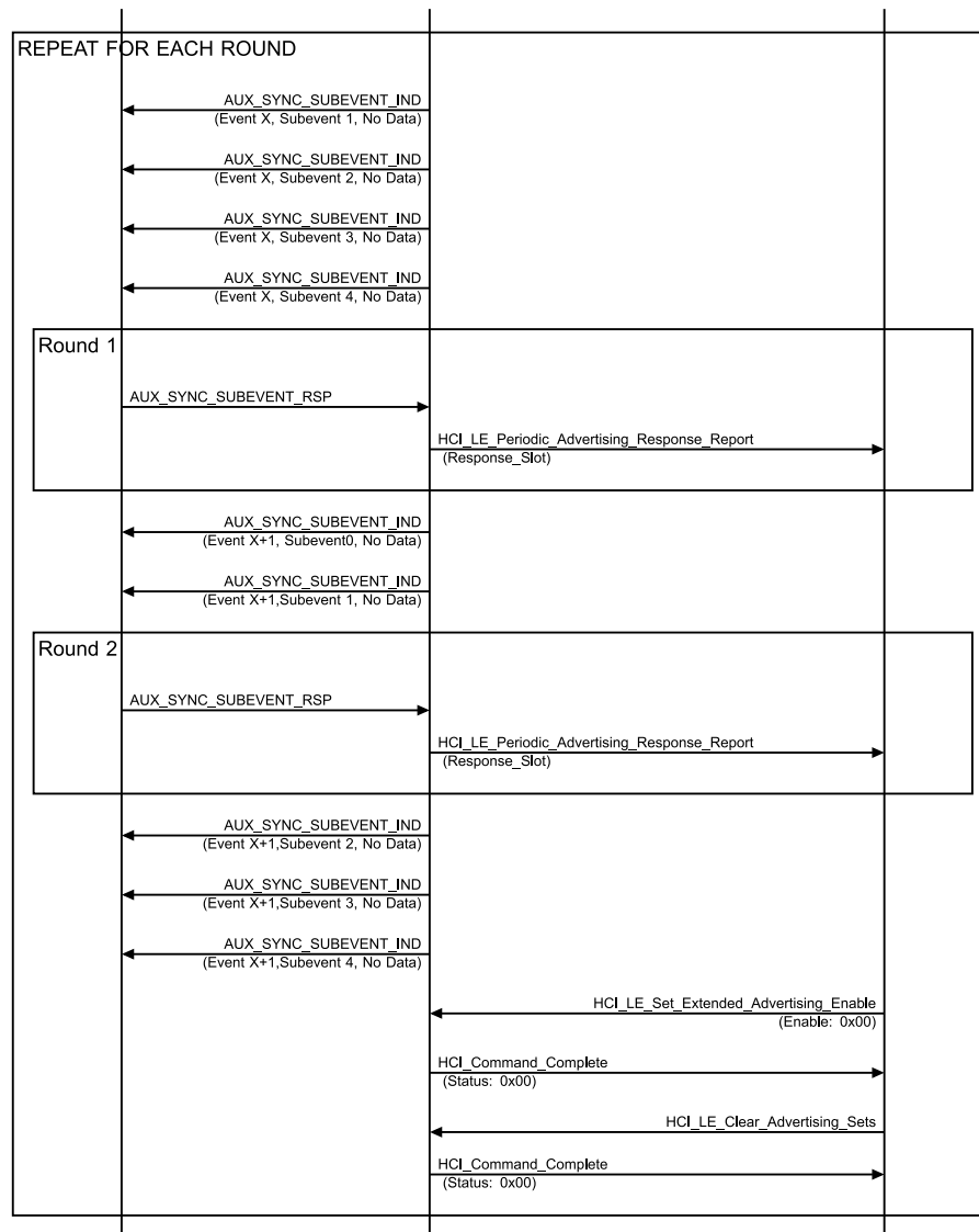
Figure 4.2-71: Receive Subevent Response Data in Future Subevent, Advertiser MSC – Page 2 of 2
