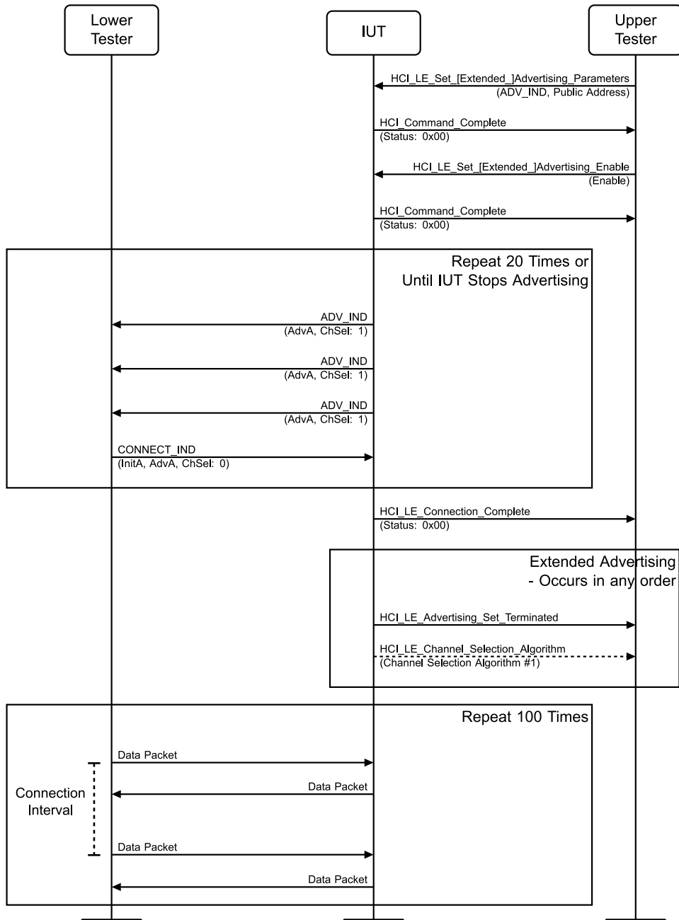
Figure 4.3-9: Accepting Connections, Channel Selection Algorithm #1 MSC
