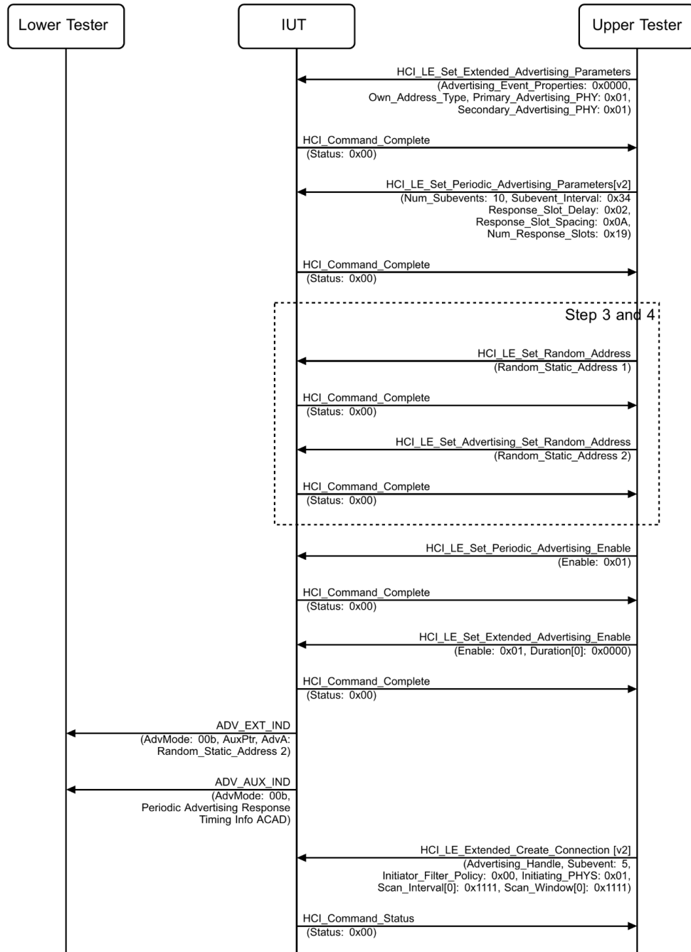
Figure 4.2-64: Reconnect with a Synchronized Device using Periodic Advertising with Responses MSC – Page 1 of 3
