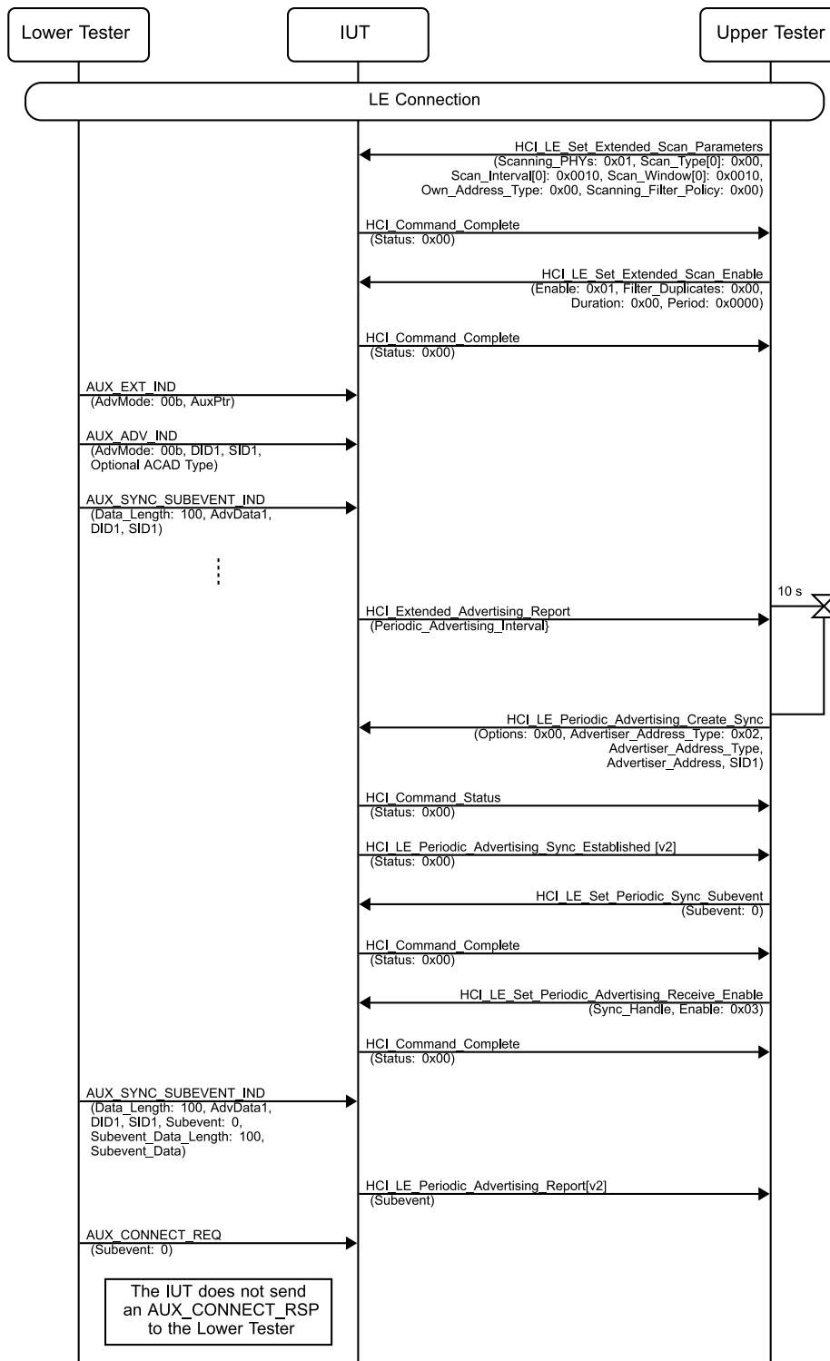
Figure 4.2-134: Reject Connection Request When Connected to a Peer, Periodic Advertising with Responses MSC
