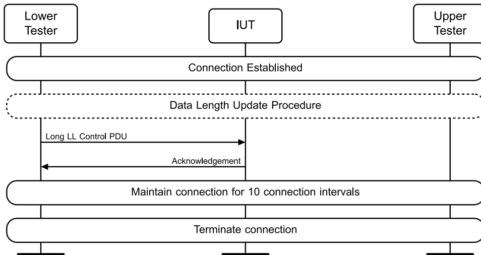
Figure 4.3-226: Acknowledging Long Control PDUs MSC
