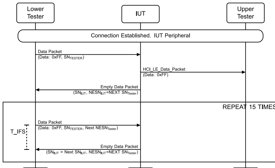
Figure 4.3-59: LL/CON/PER/BV-17-C [Peripheral acknowledgement repetition] MSC
