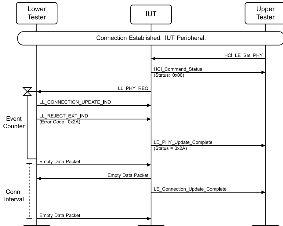
Figure 4.3-82: LL/CON/PER/BV-48-C [Handling Protocol Collision – Different Procedure – Connection Update] MSC
