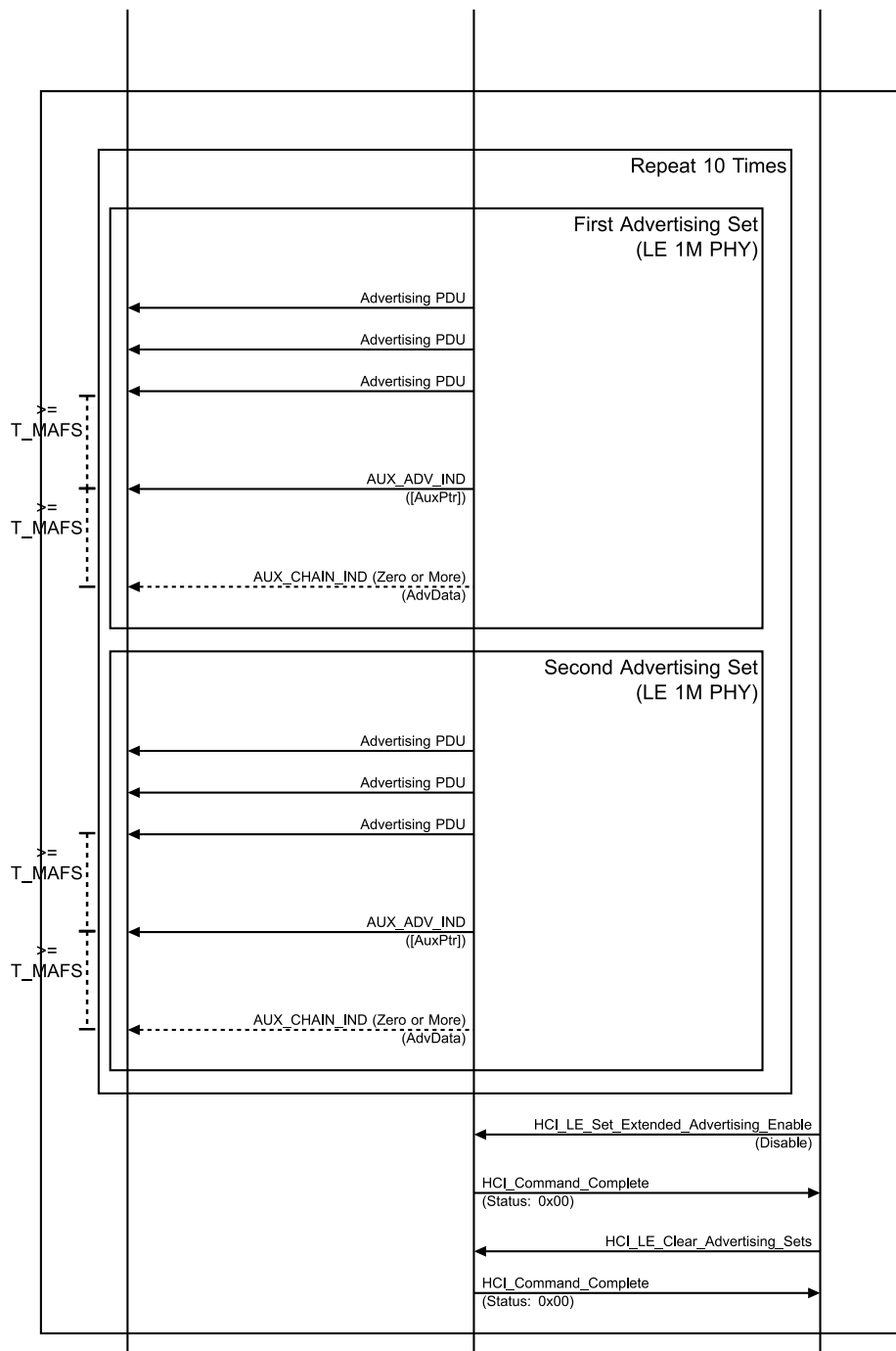
Figure 4.2-26: Extended Advertising, Multiple Sets, Single PHY, LE 1M PHY MSC – Page 2 of 2
