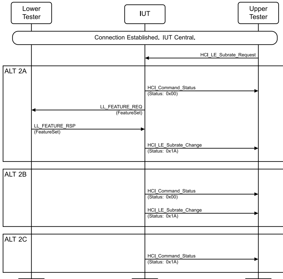
Figure 4.3-205: LL/CON/CEN/BV-143-C [Reject Subrate Request when Peripheral Feature Bit is not set] MSC
