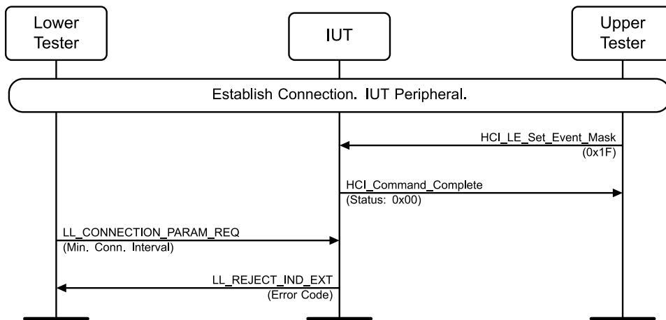
Figure 4.3-74: LL/CON/PER/BV-33-C [Accepting Connection Parameter Request – event masked] MSC
