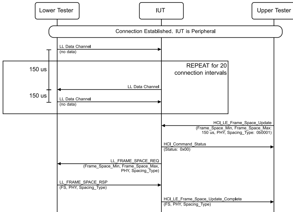
Figure 4.4-22: Initiate Inter Frame Space Change on a Different Asymmetric PHY for TX and RX, Peripheral MSC – Page 1 of 2
