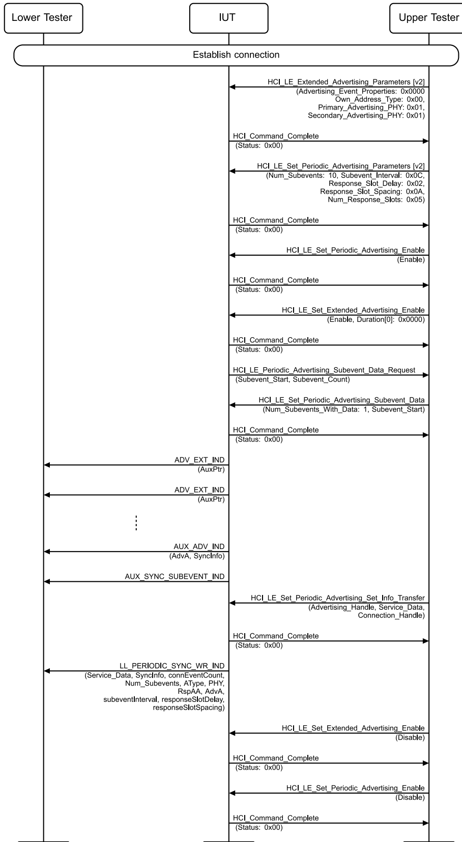
Figure 4.3-261: Periodic Advertising Sync Transfer Procedure, Advertising IUT Initiated, Periodic Advertising with Responses MSC
