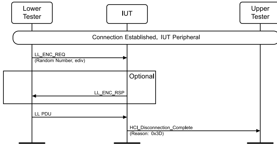
Figure 4.8-40: Peripheral Receiving unexpected Data Channel PDU during encryption start MSC
