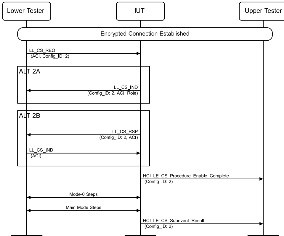
Figure 4.14-21: Respond to a CS Start Procedure MSC
