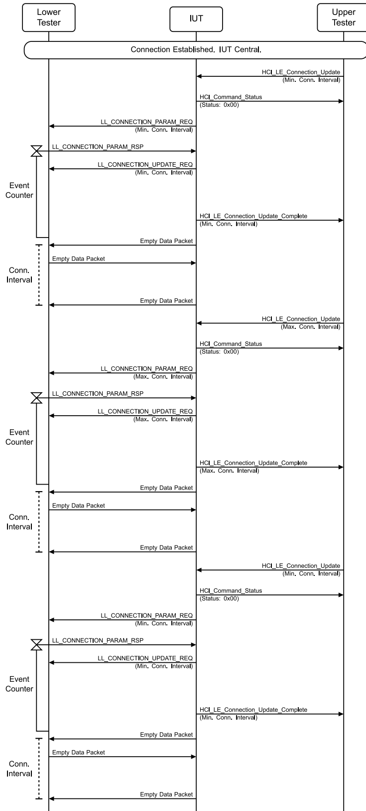
Figure 4.3-153: LL/CON/CEN/BV-24-C [Initiating Connection Parameter Request – Accept] MSC – Page 1 of 2
