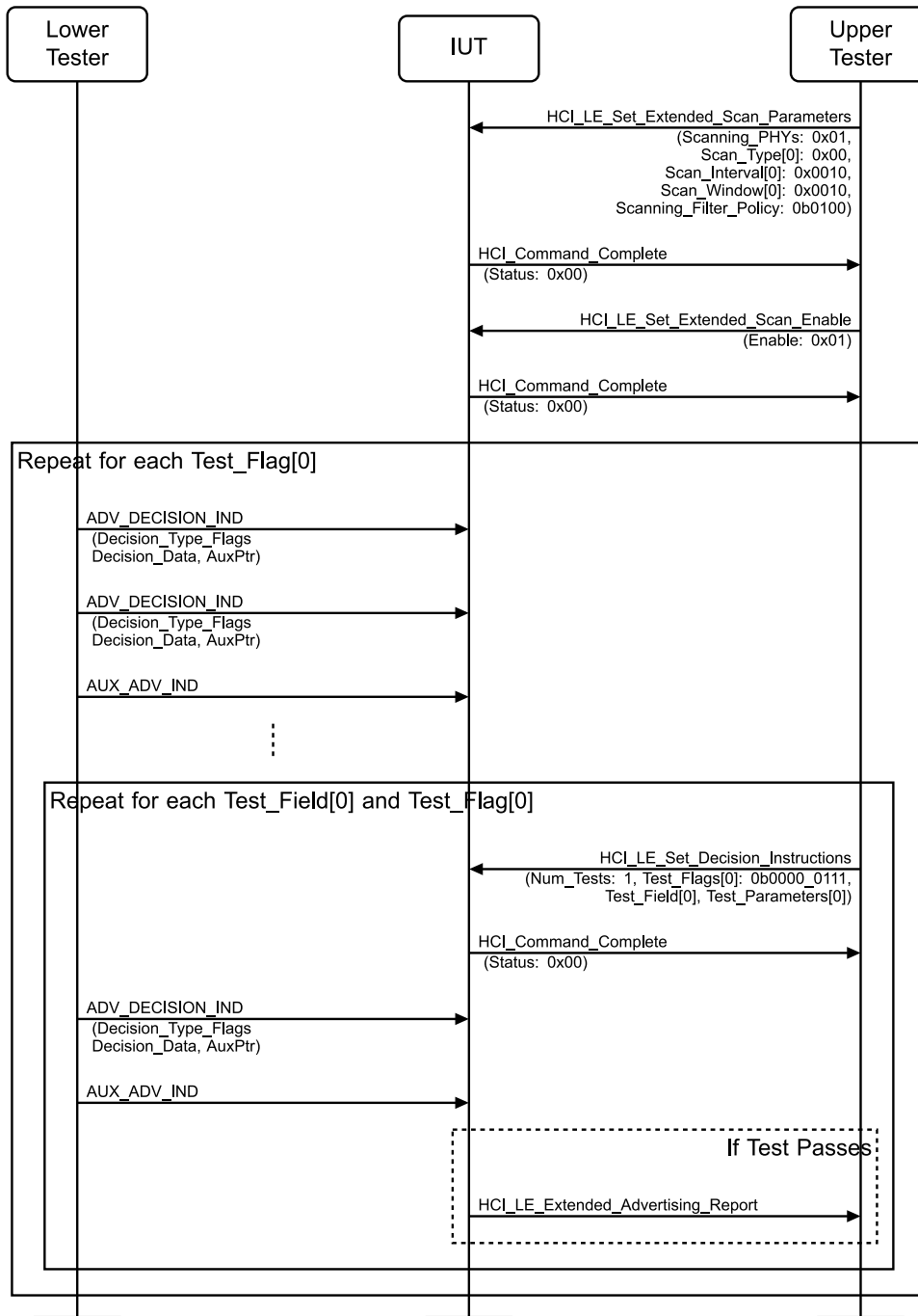
Figure 4.2-144: Decision-Based Advertisements, Arbitrary Data Test Flags MSC
