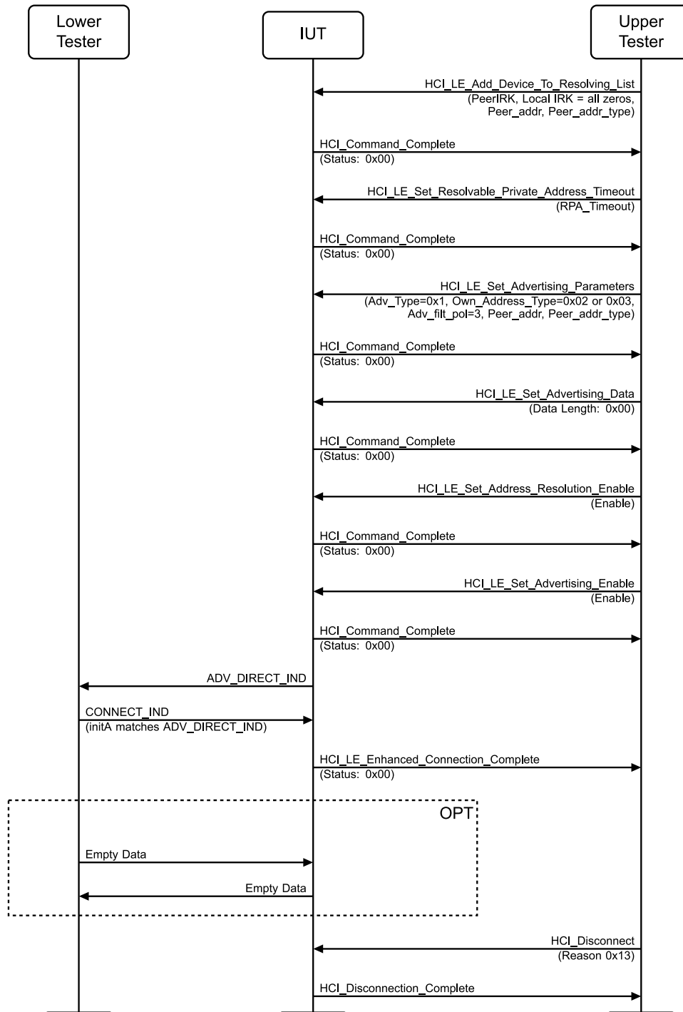
Figure 4.8-22: LL/SEC/ADV/BV-22-C [Network Privacy – Directed Connectable Advertising using Target RPA as InitA] MSC
