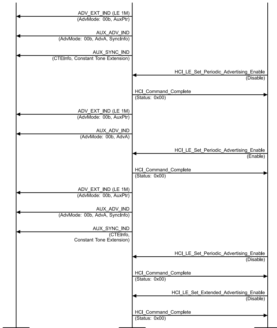
Figure 4.2-40: LL/DDI/ADV/BV-39-C [Connectionless CTE Advertising - Maintain CTE Configuration] MSC – Page 2 of 2
