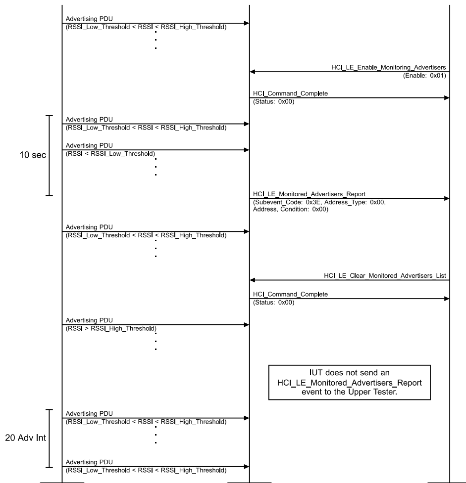
Figure 4.2-151: Monitoring Advertisers, Clear List MSC – Page 2 of 2
