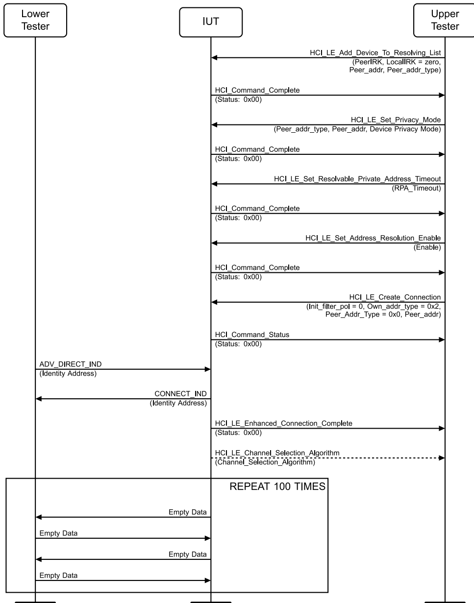
Figure 4.3-35: Device Privacy – Connection Establishment using resolving list, Initiator, Accept Identity Address MSC
