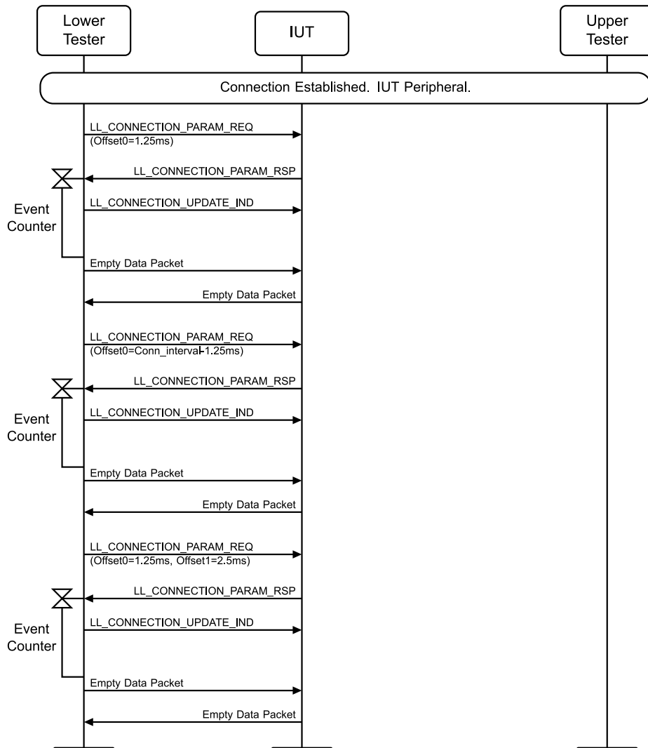
Figure 4.3-72: LL/CON/PER/BV-30-C [Accepting Connection Parameter Request – preferred anchor points only] MSC
