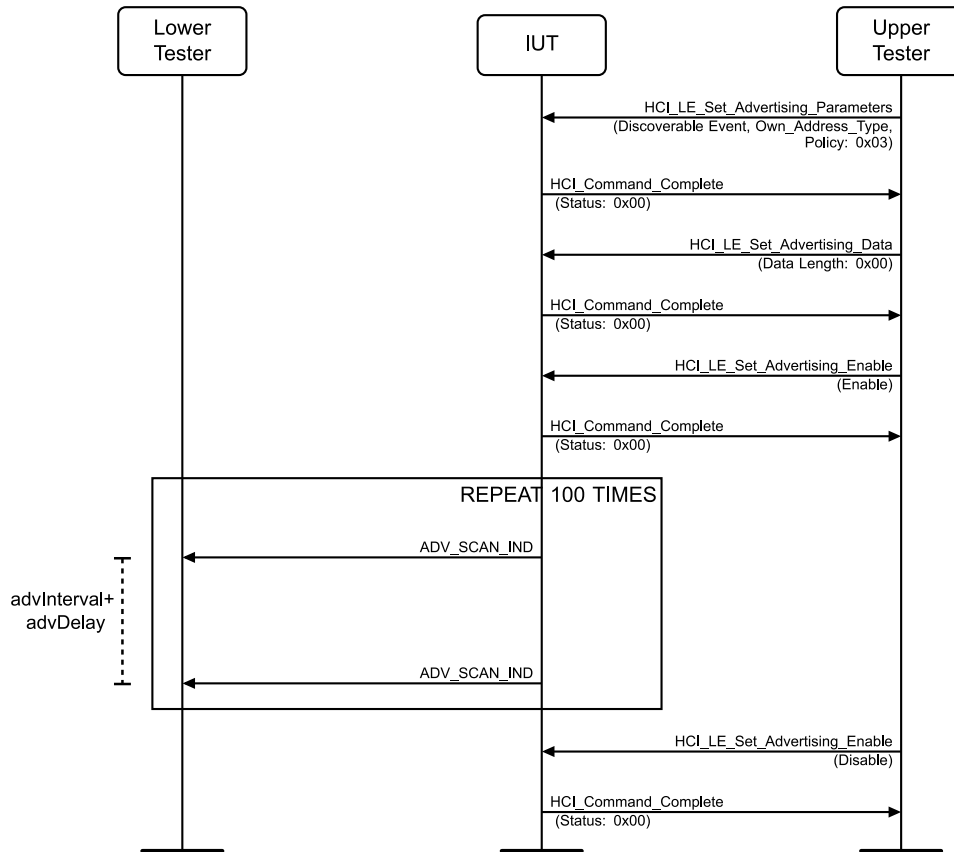
Figure 4.2-9: LL/DDI/ADV/BV-15-C [Discoverable Advertising Events] MSC
