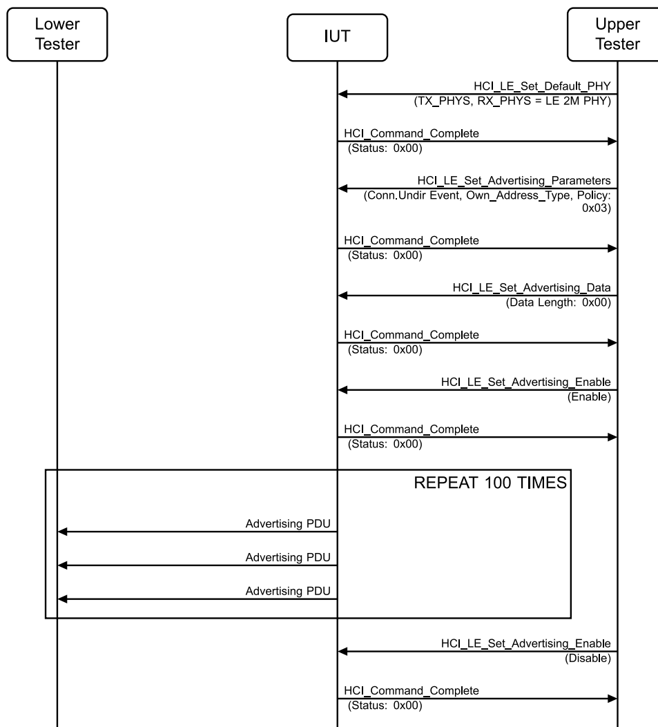
Figure 4.2-16: Advertising Always Using the LE 1M PHY MSC
