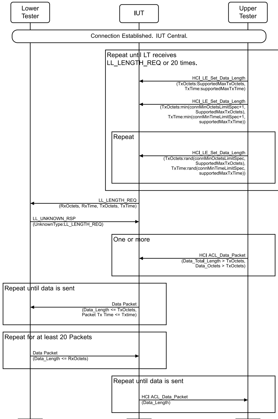
Figure 4.3-185: LL/CON/CEN/BV-75-C [Central Data Length Update – Peripheral does not support; LE 1M PHY] MSC
