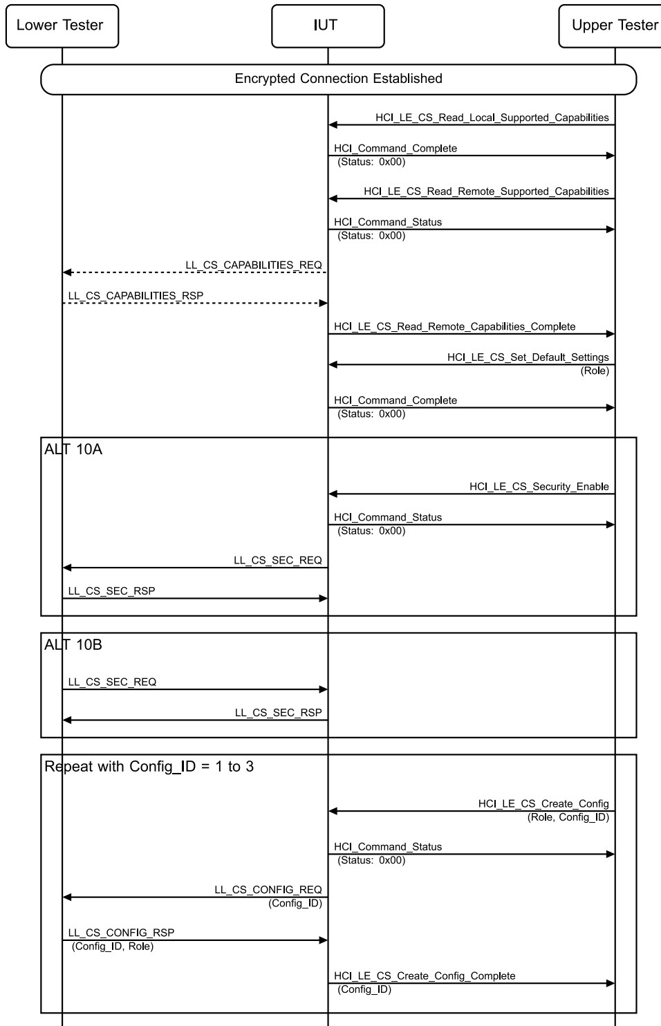
Figure 4.14-14: Initiate Configuration Procedure MSC
