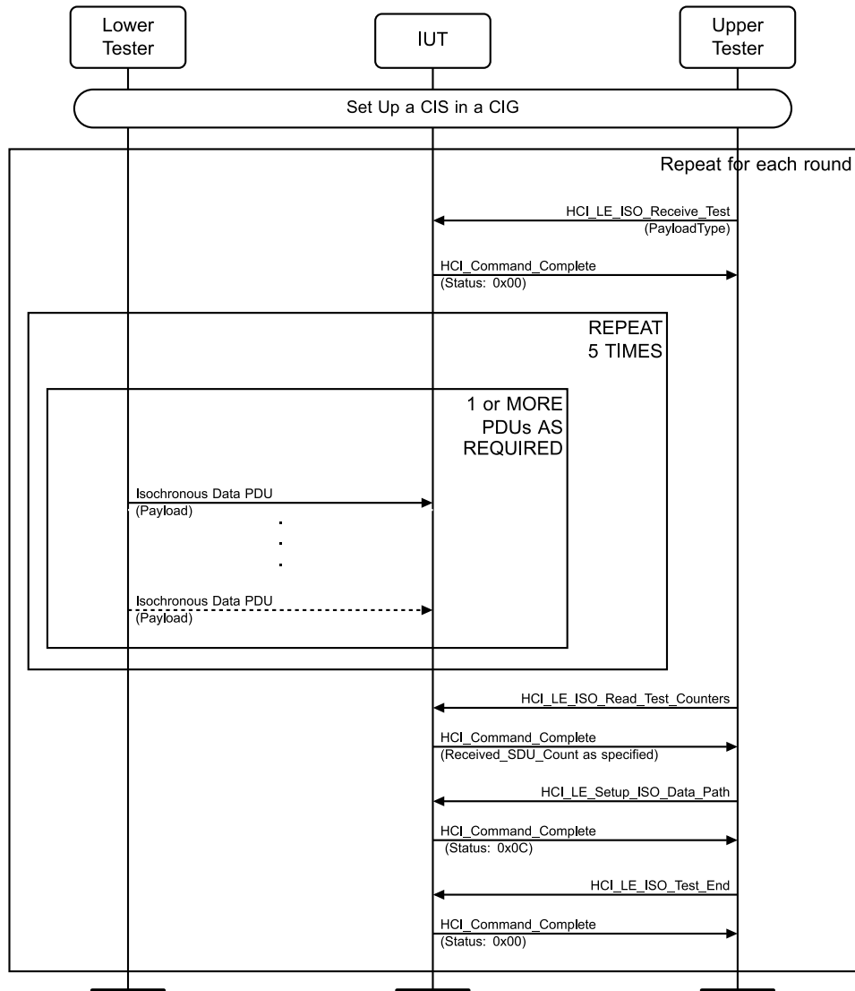
Figure 4.12-3: ISO Receive Test Mode, CIS MSC
