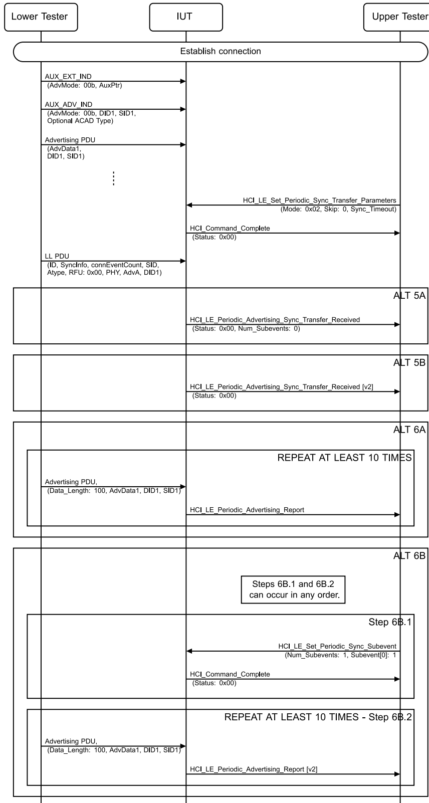
Figure 4.3-249: Periodic Advertising Sync Transfer Procedure, Accepting, Enabling Duplicate Filter when already synchronized MSC – Page 1 of 2
