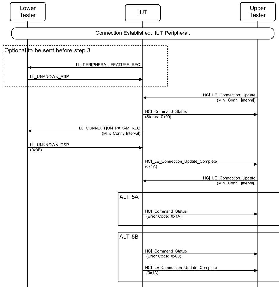
Figure 4.3-103: LL/CON/PER/BV-85-C [Initiating Connection Parameter Request – Unsupported Without Feature Exchange] MSC
