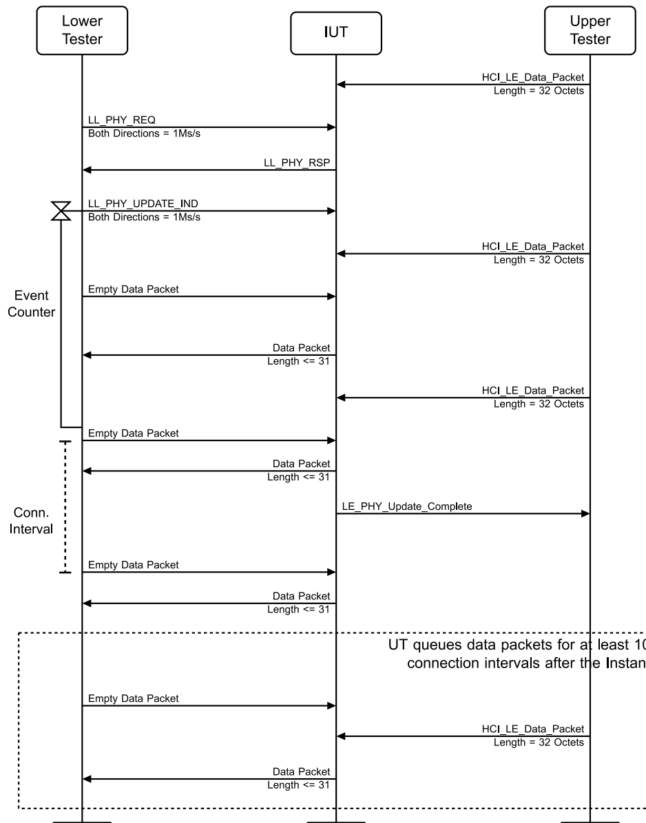
Figure 4.3-86: LL/CON/PER/BV-50-C [Responding to PHY Update Procedure – Packet Time Restrictions] MSC – Page 2 of 2
