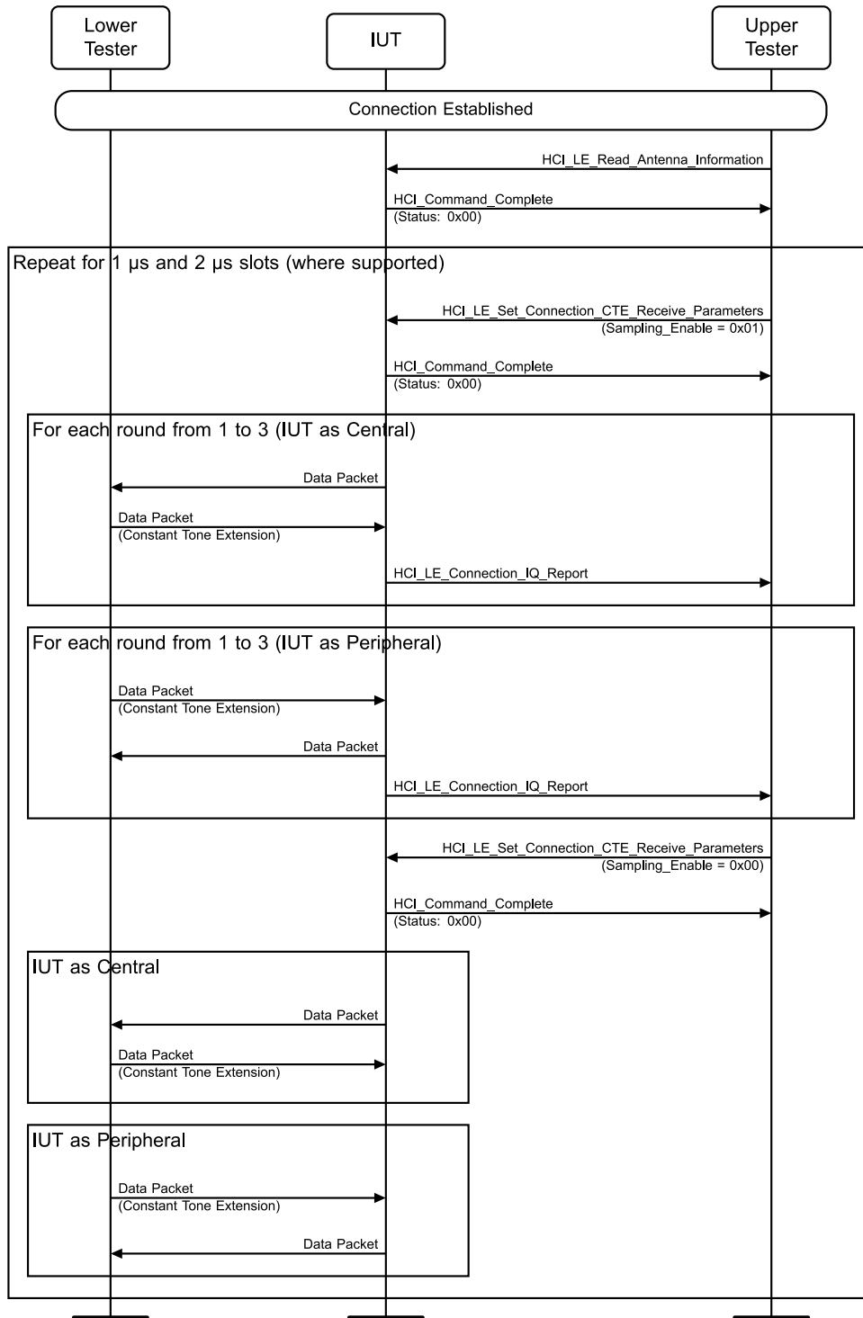
Figure 4.3-232: Unrequested Constant Tone Extension, IUT Receiving, AoD MSC
