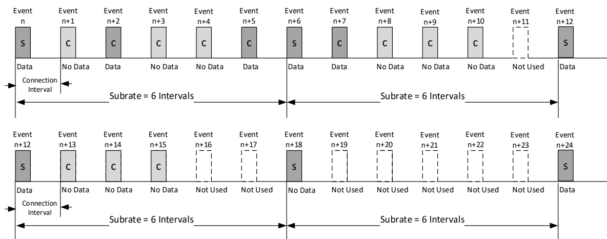
Figure 4.3-118: Continuation Interval Test Timeline
