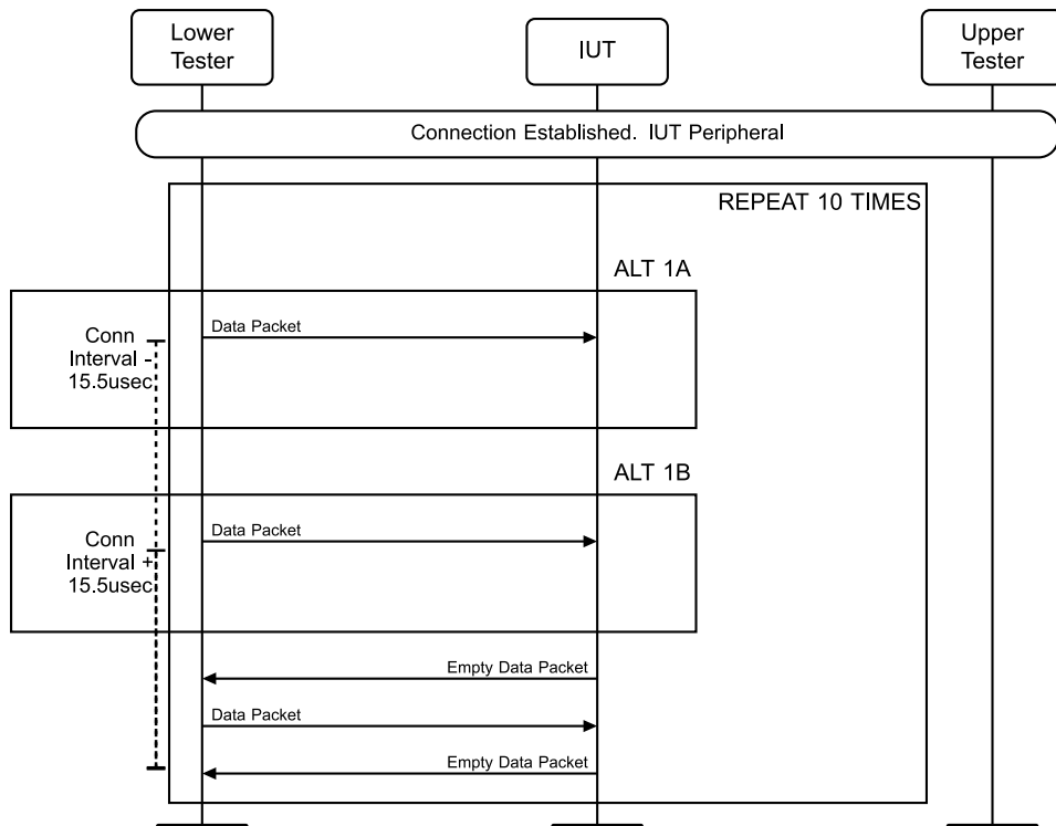
Figure 4.4-6: Shortest/Longest Connection Interval MSC
