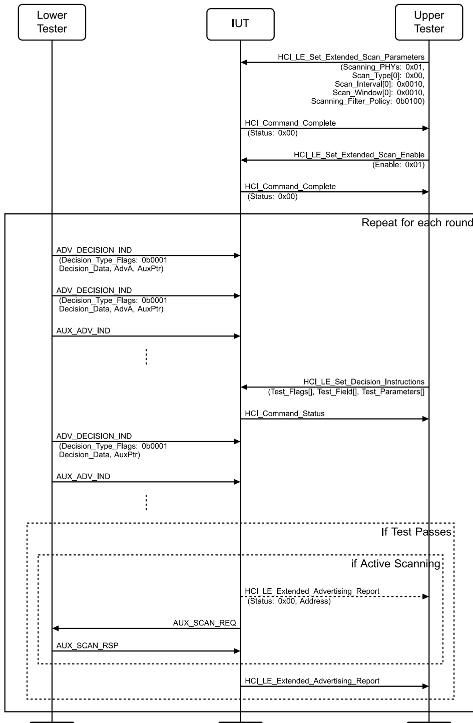
Figure 4.2-137: Decision-Based Advertisements, Test Flags MSC
