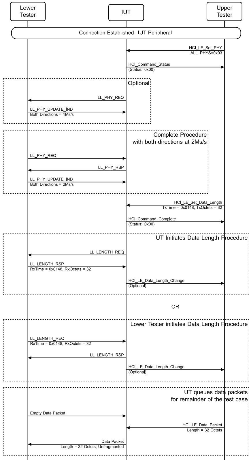
Figure 4.3-85: LL/CON/PER/BV-50-C [Responding to PHY Update Procedure – Packet Time Restrictions] MSC – Page 1 of 2
