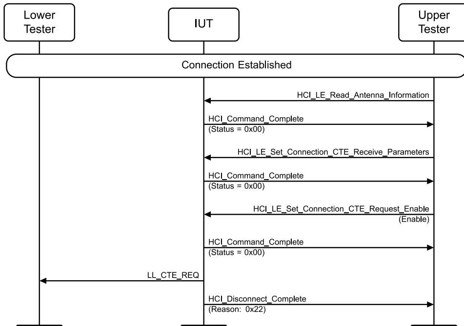
Figure 4.3-236: Constant Tone Extension Request Procedure, IUT Initiated, Timeout MSC
