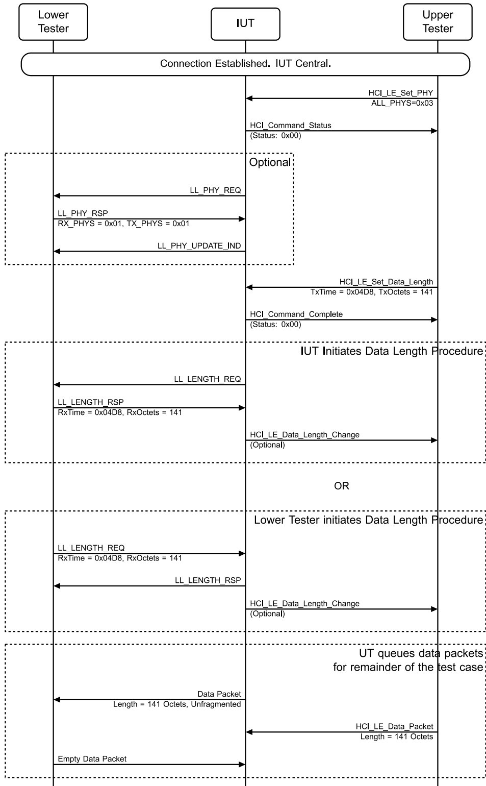
Figure 4.3-177: LL/CON/CEN/BV-53-C [Initiating PHY Update Procedure – Packet Time Restrictions, LE Coded] MSC – Page 1 of 2
