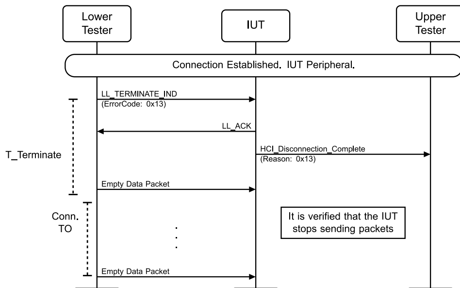
Figure 4.3-54: LL/CON/PER/BV-12-C [Peripheral accepting termination] MSC
