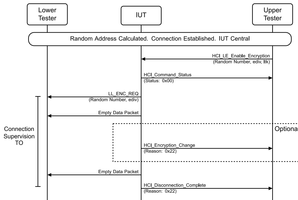
Figure 4.8-54: LL/SEC/CEN/BI-01-C [Central Encryption Setup: Missing Response] MSC
