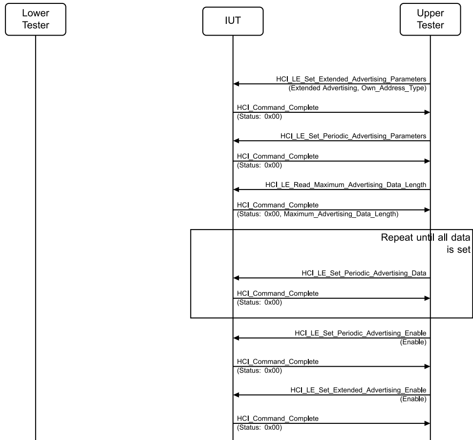
Figure 4.2-43: LL/DDI/ADV/BV-61-C [Extended Advertising, Periodic Advertising with TxPower] MSC – Page 1 of 2
