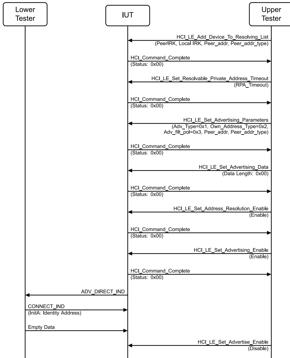
Figure 4.8-17: LL/SEC/ADV/BV-17-C [Network Privacy - Directed Connectable Advertising using local and remote IRK, Ignore Identity Address] MSC
