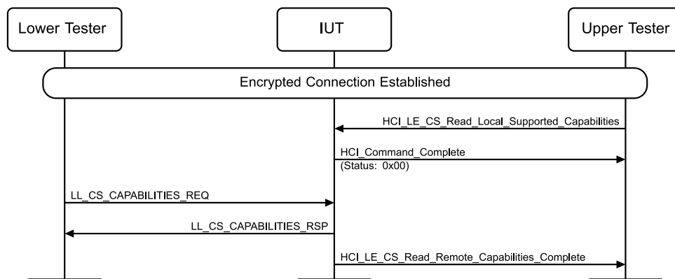
Figure 4.14-11: Respond to Capabilities Exchange MSC
