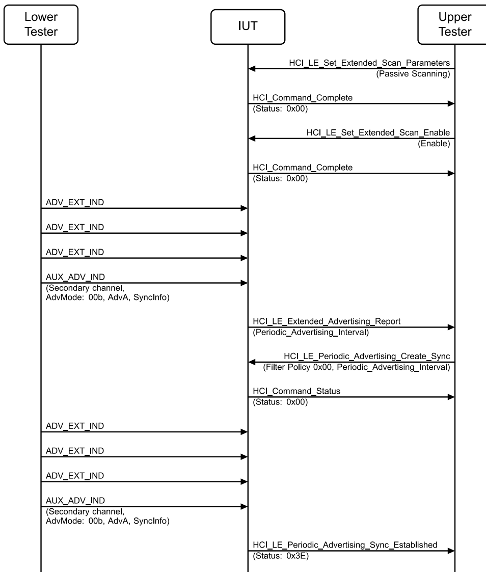
Figure 4.2-107: Extended Scanning, Periodic Advertising Reception, Reporting Initially Disabled MSC
