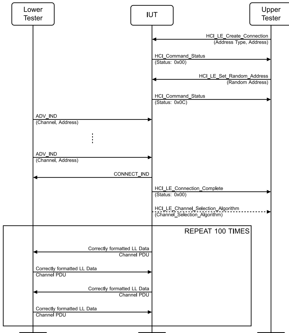
Figure 4.3-22: Connecting to Directed Advertising MSC
