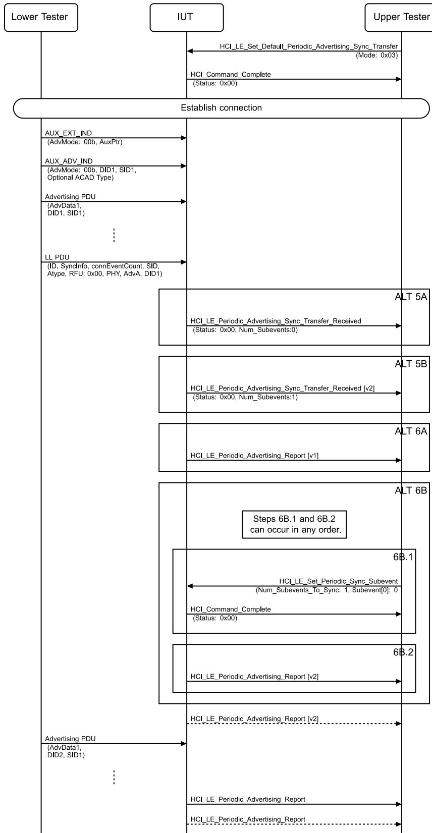
Figure 4.3-251: Periodic Advertising Sync Transfer Procedure, Accepting, Enabling Default Duplicate Filter MSC
