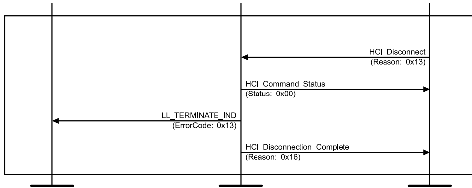
Figure 4.3-16: Extended Advertising, Accepting Connections MSC – Page 2 of 2
