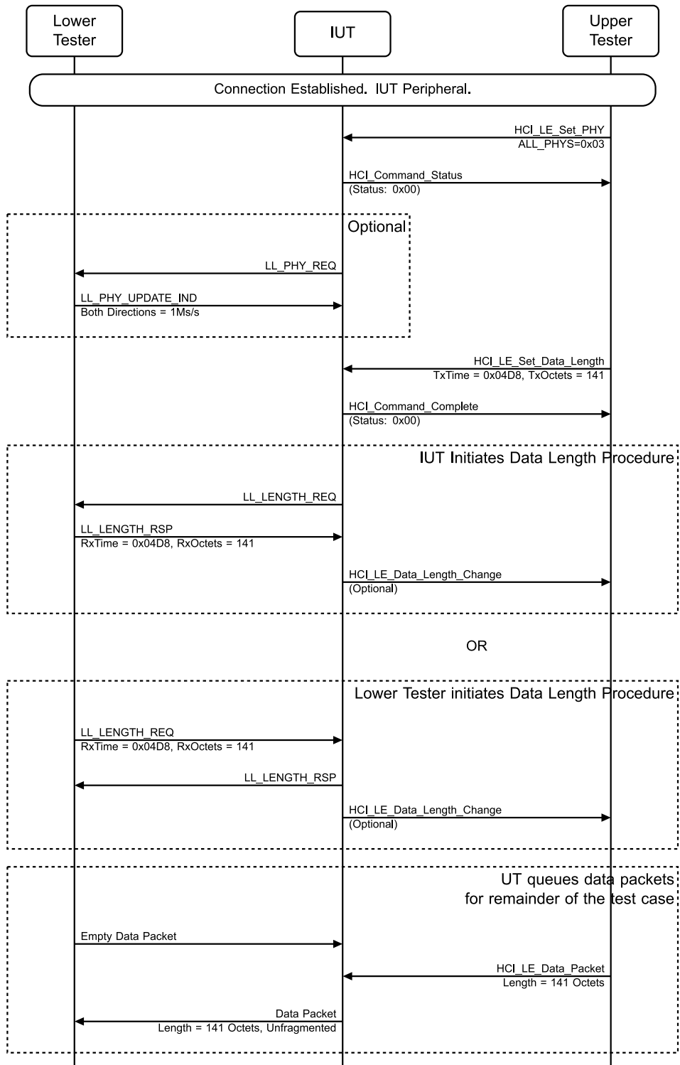
Figure 4.3-93: LL/CON/PER/BV-55-C [Initiating PHY Update Procedure – Packet Time Restrictions, LE Coded] MSC – Page 1 of 2
