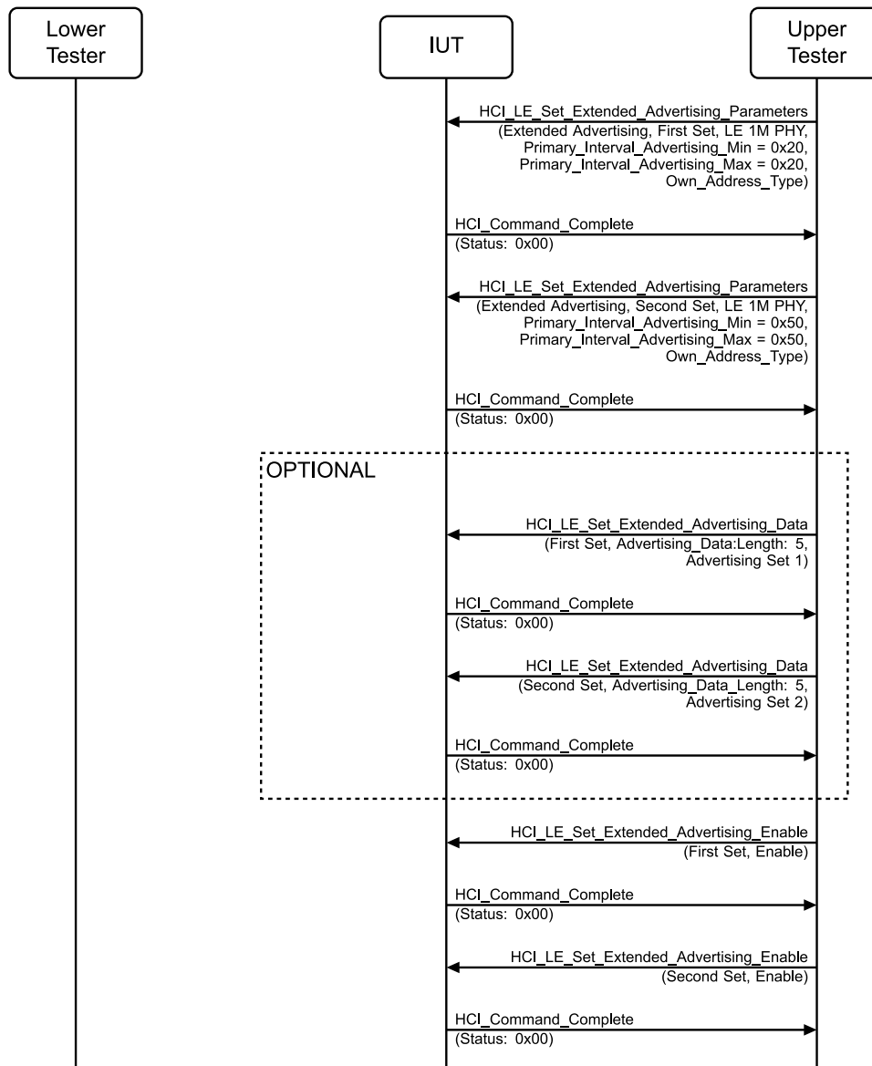
Figure 4.2-50: Extended Advertising, Multiple Sets, Legacy and Extended, Primary Advertising PDU MSC – Page 1 of 2
