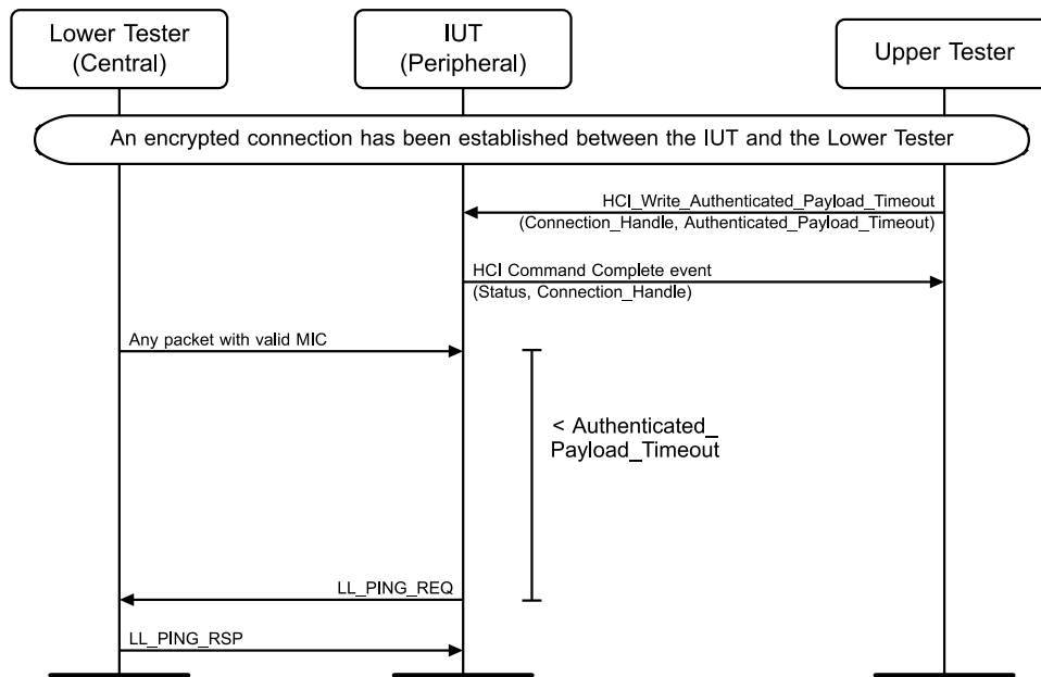
Figure 4.8-35: LL/SEC/PER/BV-09-C [Modified Authentication Payload Timeout] MSC
