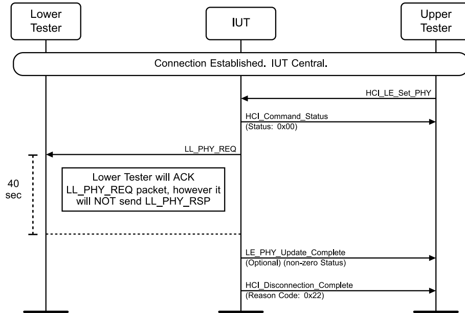
Figure 4.3-168: LL/CON/CEN/BV-46-C [Protocol Timeout for PHY Update Procedure] MSC
