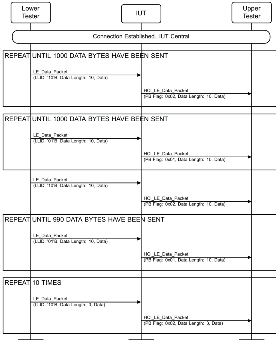
Figure 4.3-136: LL/CON/CEN/BV-04-C [Central Receiving Data] MSC
