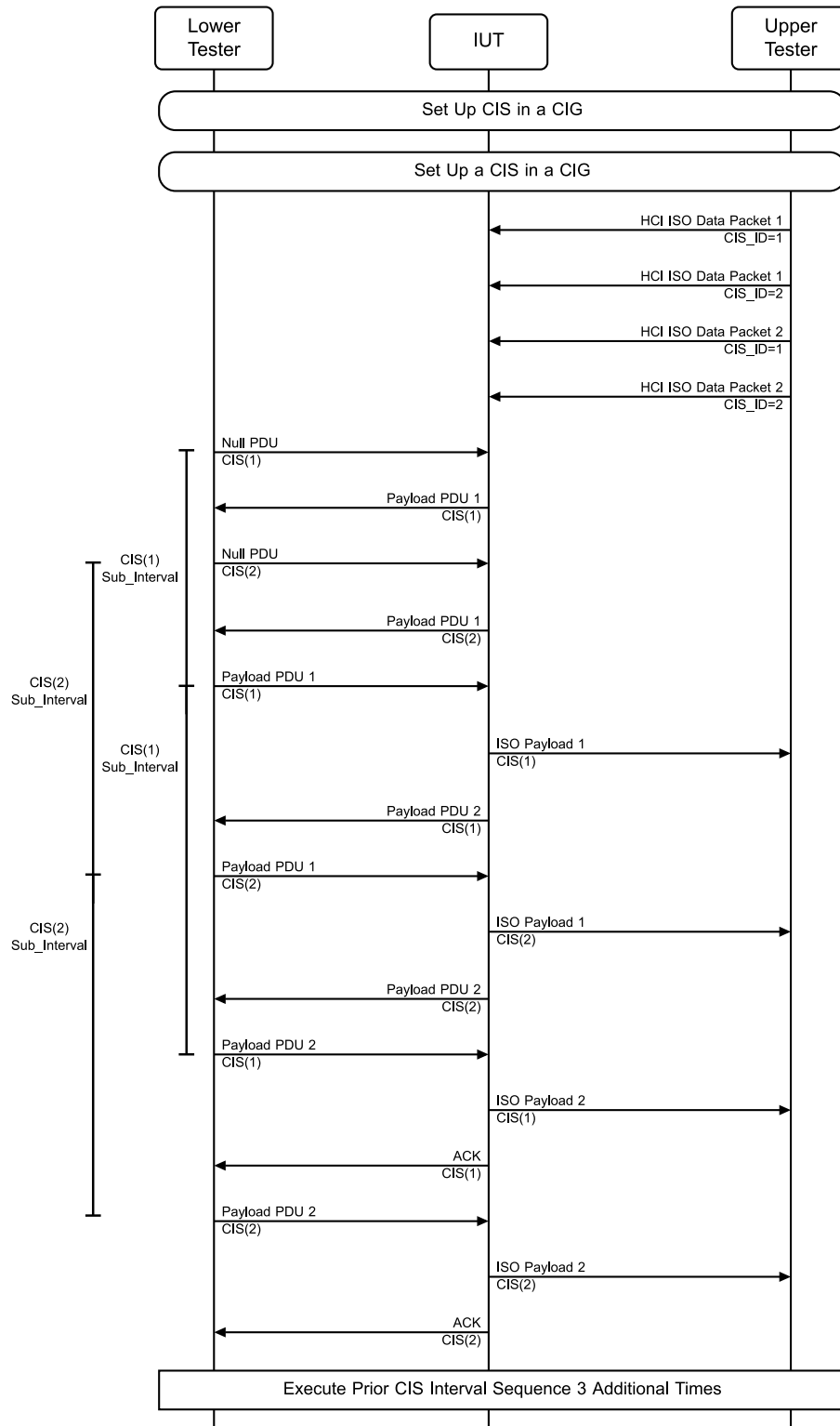
Figure 4.10-31: LL/CIS/PER/BV-07-C [Sending and Receiving Data in Multiple CISes, Single CIG, Single Connection, Interleaved CIG, Peripheral] MSC
