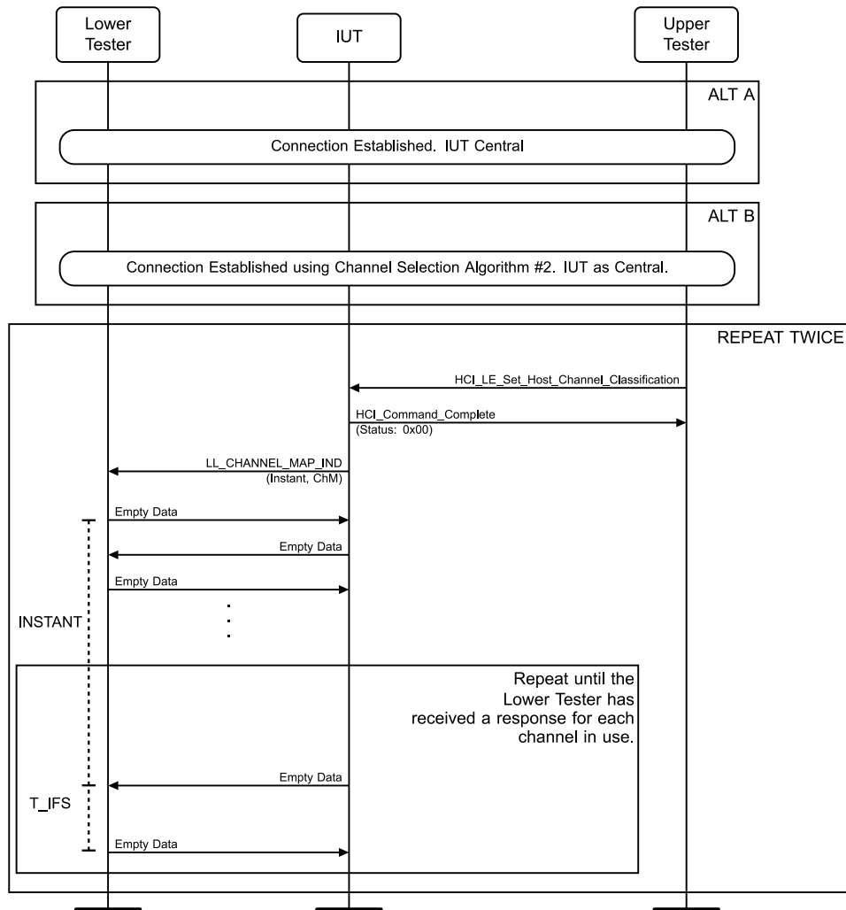
Figure 4.6-6: Requesting Channel Map Update MSC
