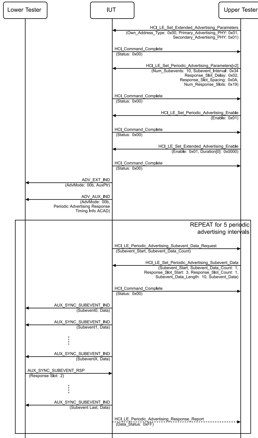
Figure 4.2-67: Ignore Periodic Advertising Response Data, Incorrect Response Slot MSC
