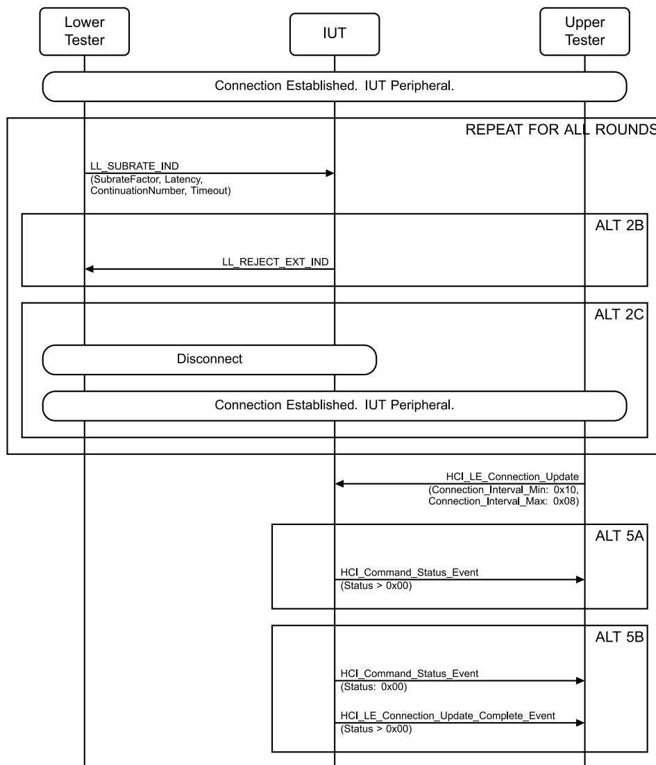
Figure 4.3-121: LL/CON/PER/BI-13-C [Reject Invalid Subrate Updates] MSC
