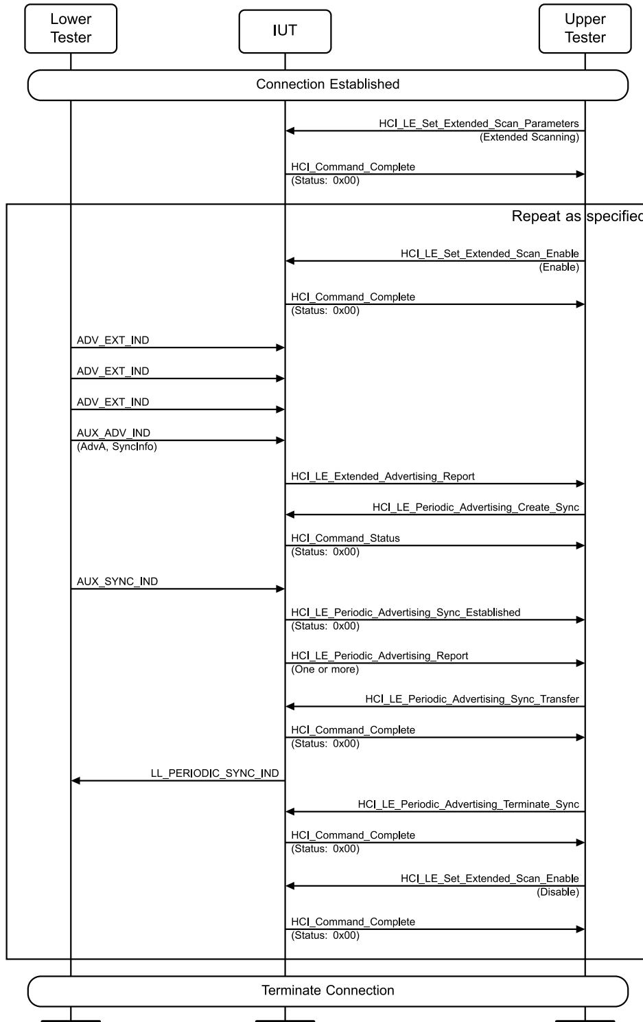
Figure 4.3-260: Periodic Advertising Sync Transfer Procedure, Synchronized IUT Initiated – Multiple Resolvable Private Addresses MSC
