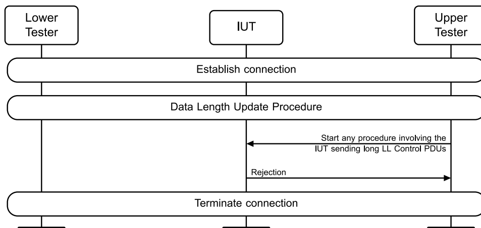
Figure 4.3-227: Rejecting Request to Send Long Control PDUs before Feature Exchange MSC
