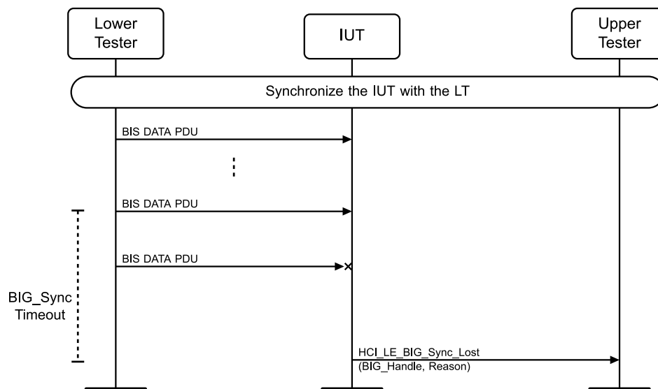
Figure 4.11-21: LL/BIS/SNC/BV-11-C [Loss of Sync with an Isochronous Broadcaster] MSC
