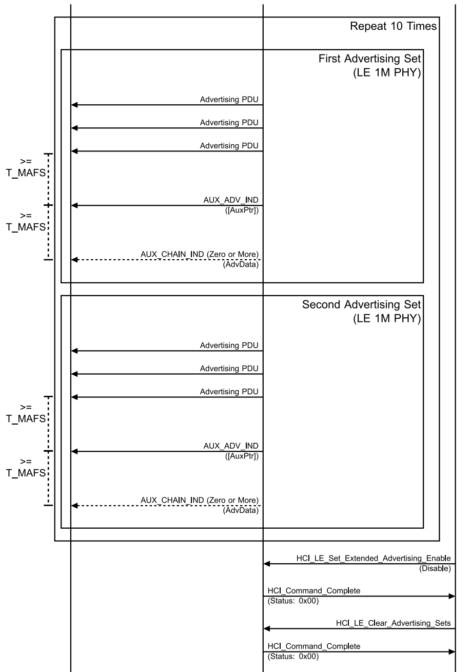
Figure 4.2-30: Extended Advertising, Multiple Sets, Legacy and Extended MSC – Page 2 of 2
