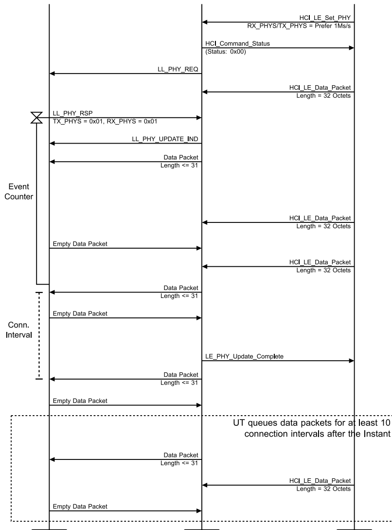
Figure 4.3-172: LL/CON/CEN/BV-49-C [Initiating PHY Update Procedure – Packet Time Restrictions] MSC – Page 2 of 2
