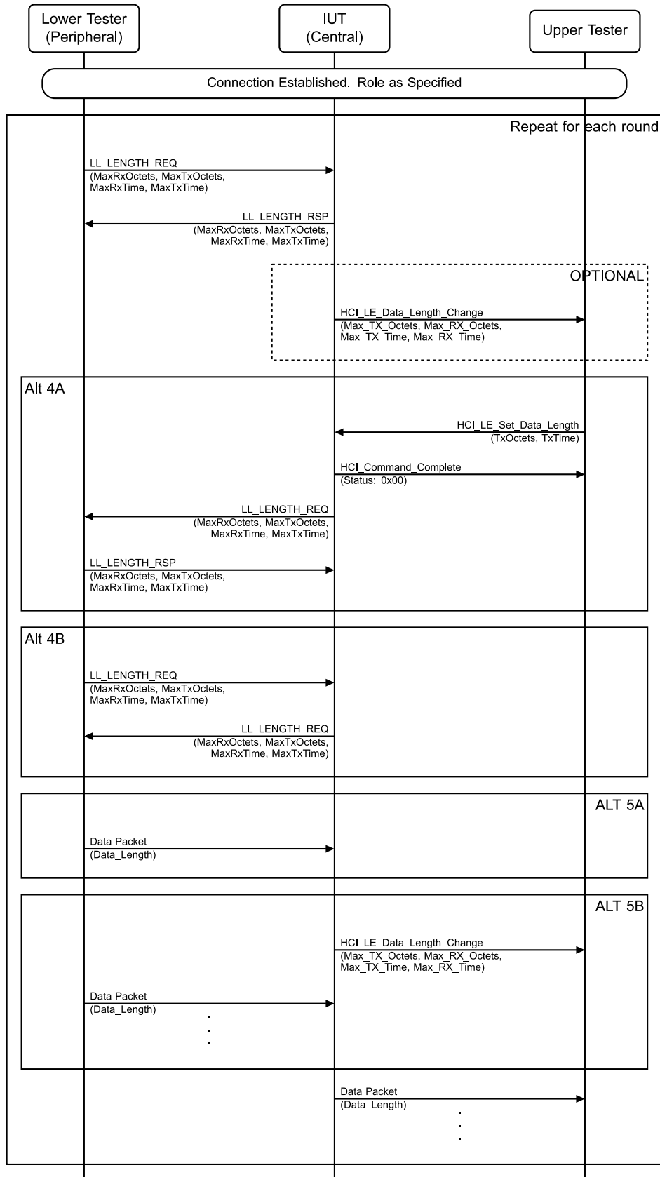
Figure 4.3-244: Data Length Update – Handling Invalid Data Length Responses MSC
