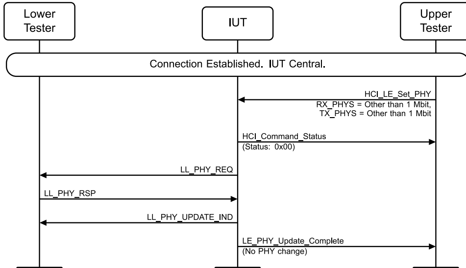
Figure 4.3-175: LL/CON/CEN/BV-51-C [Initiating PHY Update Procedure – No Common PHY] MSC
