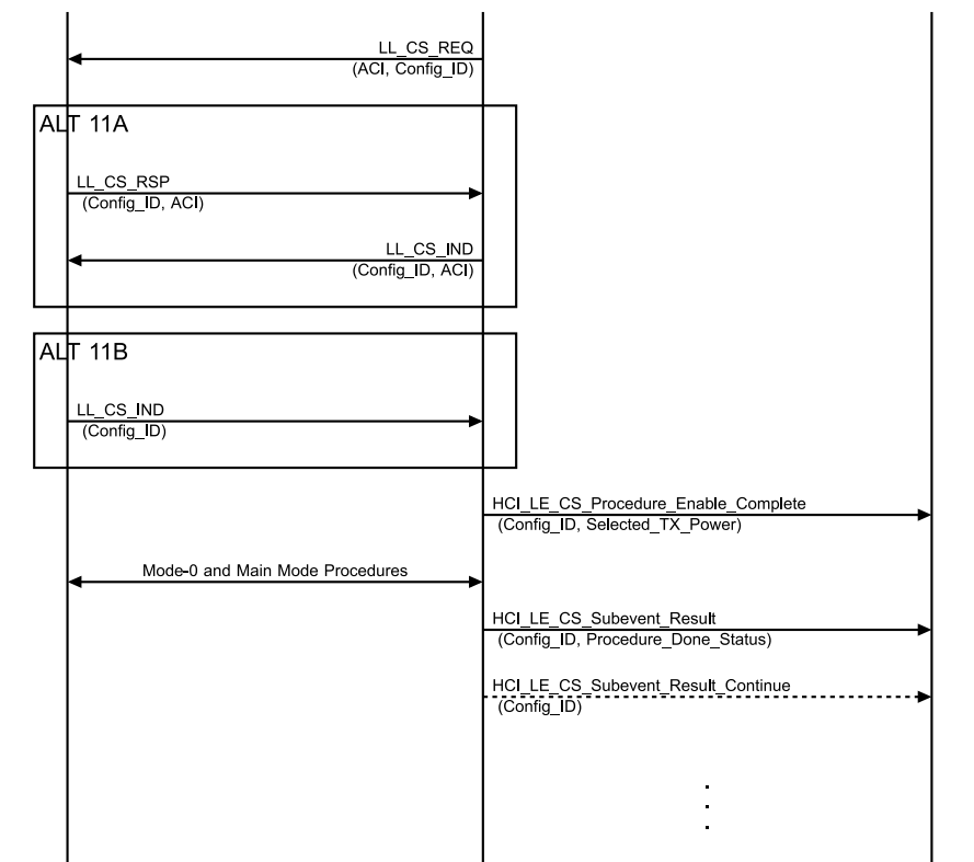
Figure 4.14-20: Initiate CS Start Procedure MSC – Page 2 of 2
