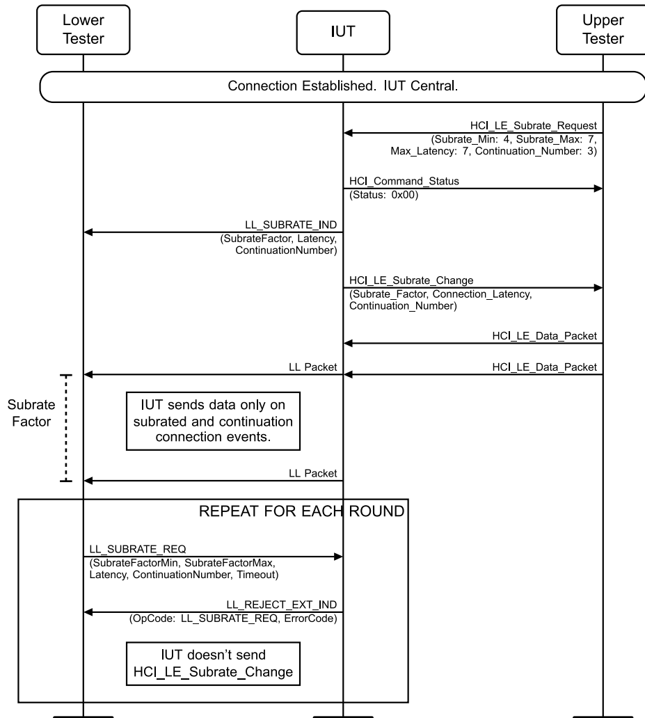
Figure 4.3-196: LL/CON/CEN/BI-10-C [Reject an Incoming Subrate Change Request] MSC
