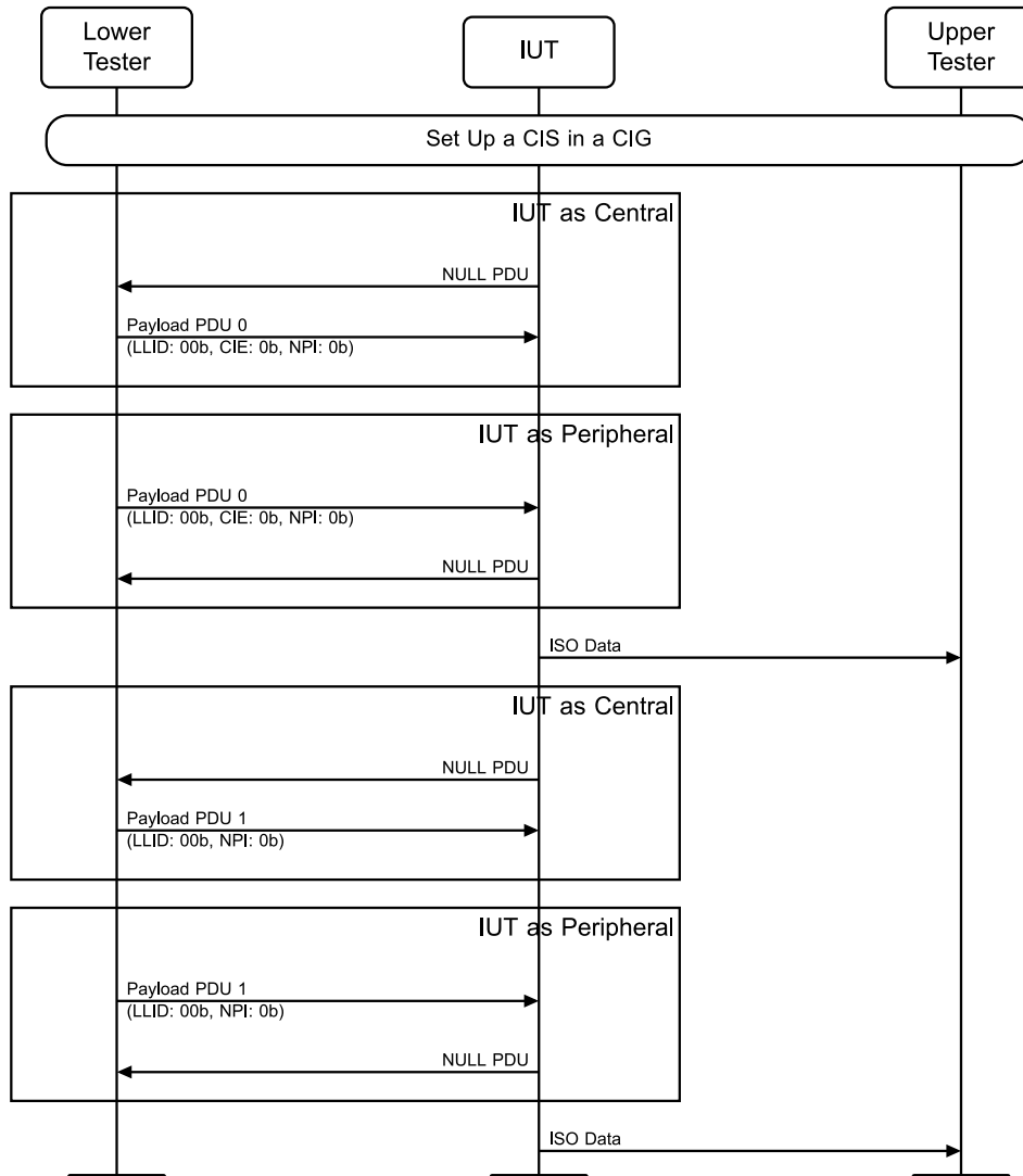
Figure 4.10-49: Receiving data in Unidirectional CIS MSC
