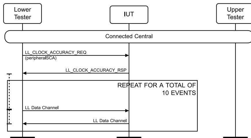
Figure 4.4-28: LL/TIM/CEN/BV-04-C [Response to Sleep Clock Accuracy Update] MSC
