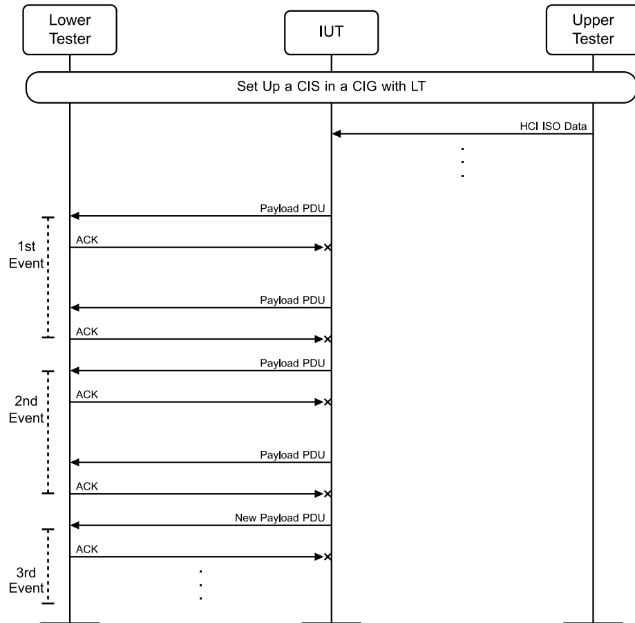
Figure 4.10-19: LL/CIS/CEN/BV-49-C [Flushing of Packets in CIS, Central, BN = 1] MSC
