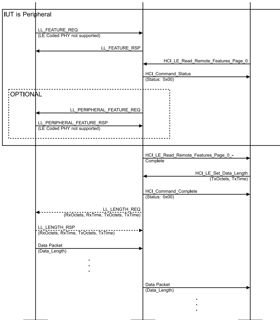
Figure 4.3-246: Data Length Update – Peer Does Not Support LE Coded PHY MSC – Page 2 of 2
