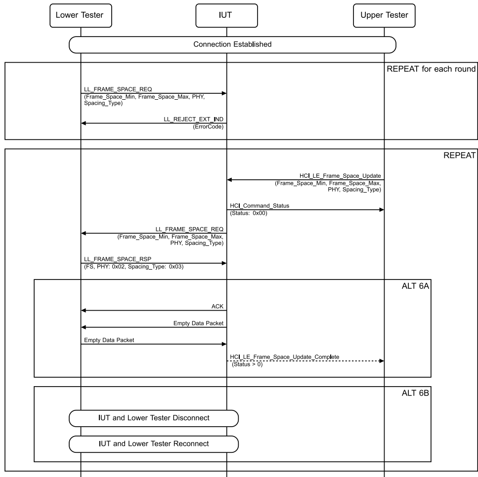
Figure 4.4-47: Frame Space Change, Invalid Parameters MSC – Page 1 of 2
