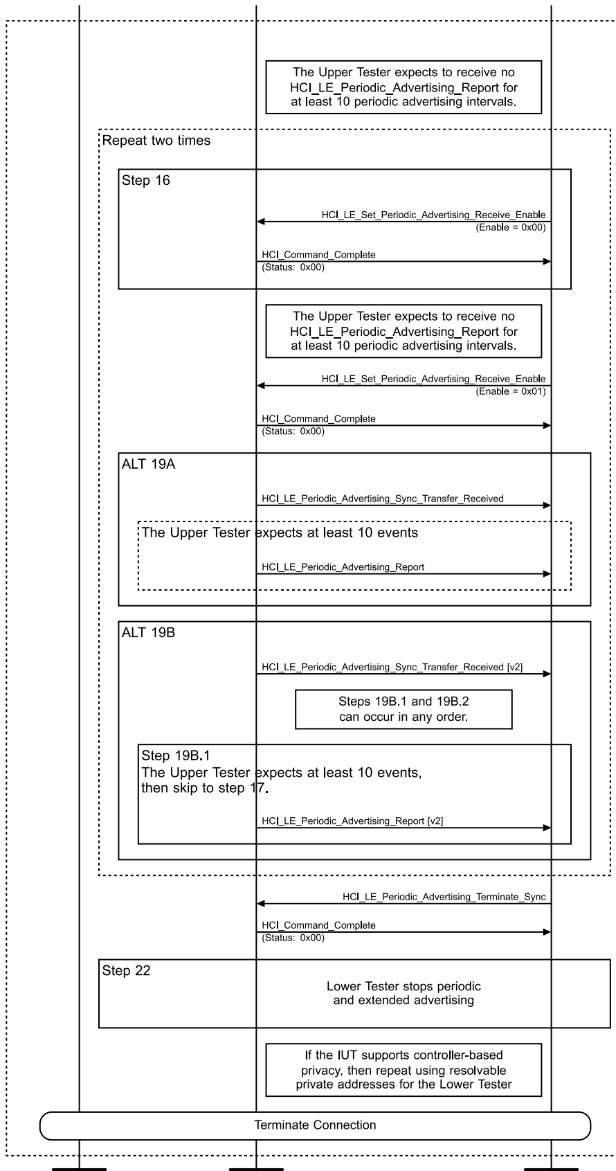
Figure 4.3-224: Periodic Advertising Sync Transfer Procedure, Accepting – Different Modes and Addresses MSC – Page 3 of 3
