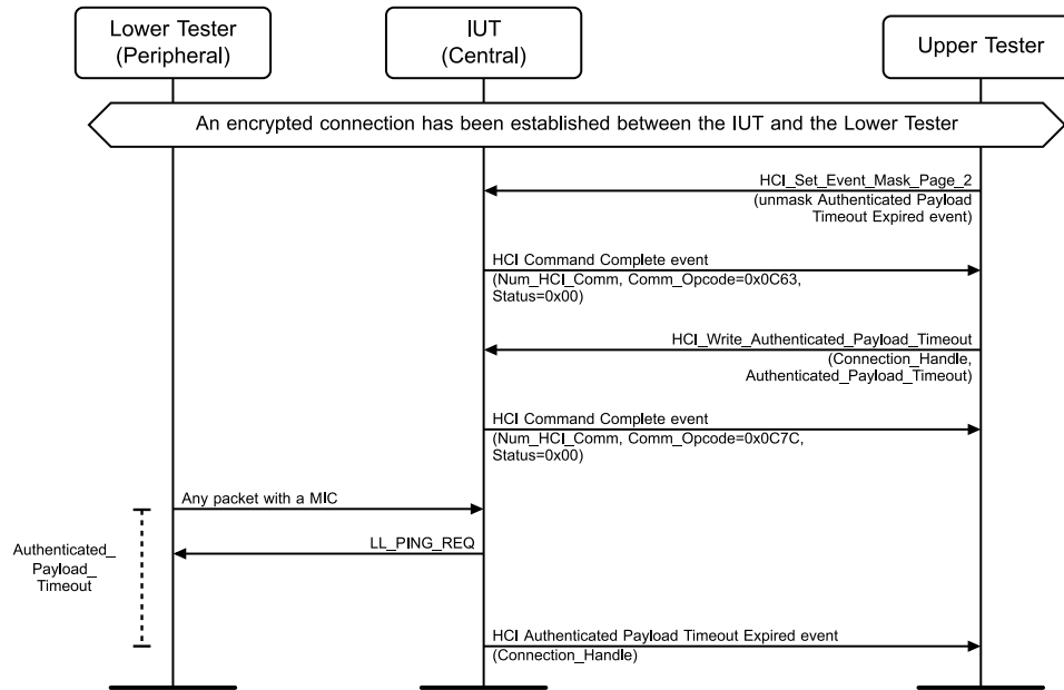
Figure 4.8-47: LL/SEC/CEN/BV-08-C [No response to LL_PING_REQ] MSC
