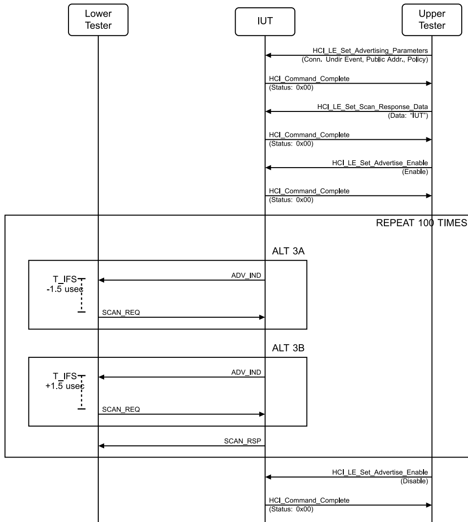
Figure 4.4-1: Earliest/Latest Transmission to Advertiser MSC
