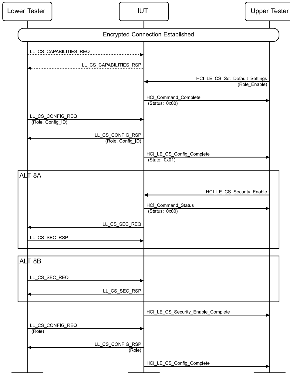
Figure 4.14-15: Respond to a Configuration Procedure MSC
