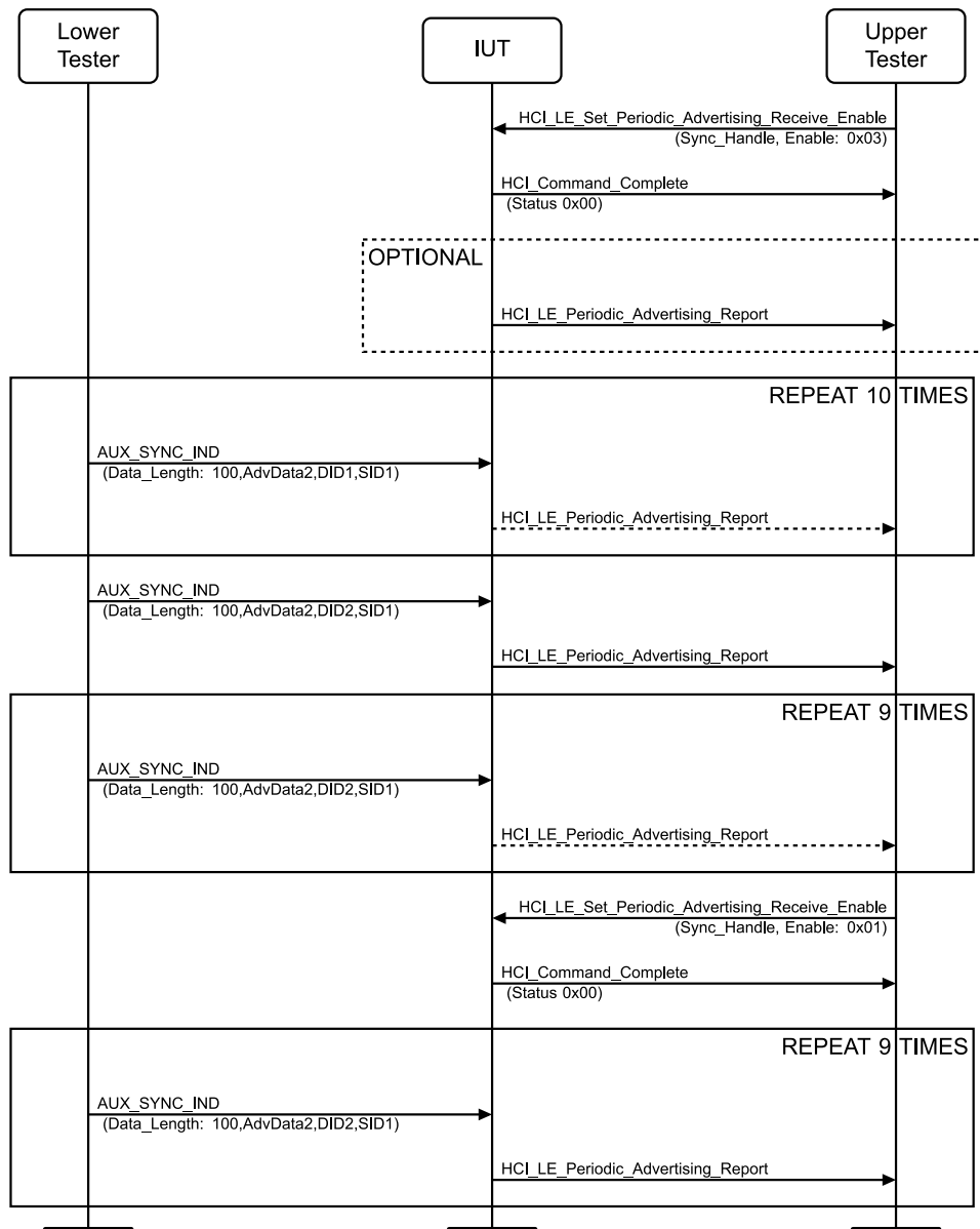
Figure 4.2-116: LL/DDI/SCN/BV-70-C [Scanner enables Duplicate Filtering after initially disabled] MSC – Page 2 of 2
