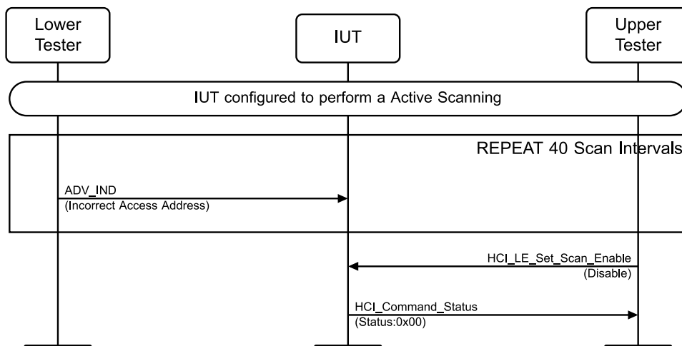
Figure 4.5-4: LL/ENC/SCN/BI-02-C [Active Scanning Invalid Address] MSC
