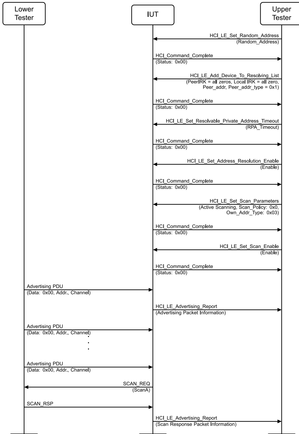
Figure 4.2-86: Network Privacy – Active Scanning MSC
