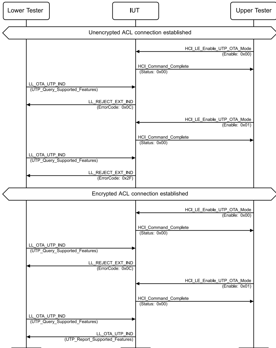
Figure 4.7-4: LL/PAC/BI-01-C [Reject UTP OTA Mode PDU, Unencrypted ACL or UTP OTA Mode disabled] MSC
