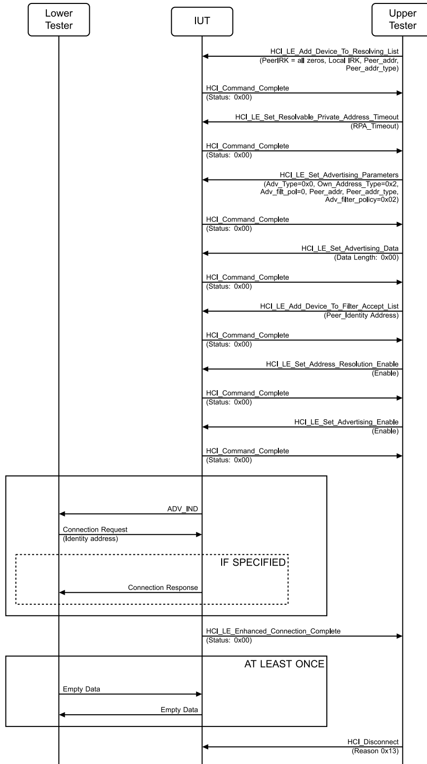
Figure 4.8-6: Network Privacy – Undirected Connectable Advertising with Local IRK, no peer IRK MSC
