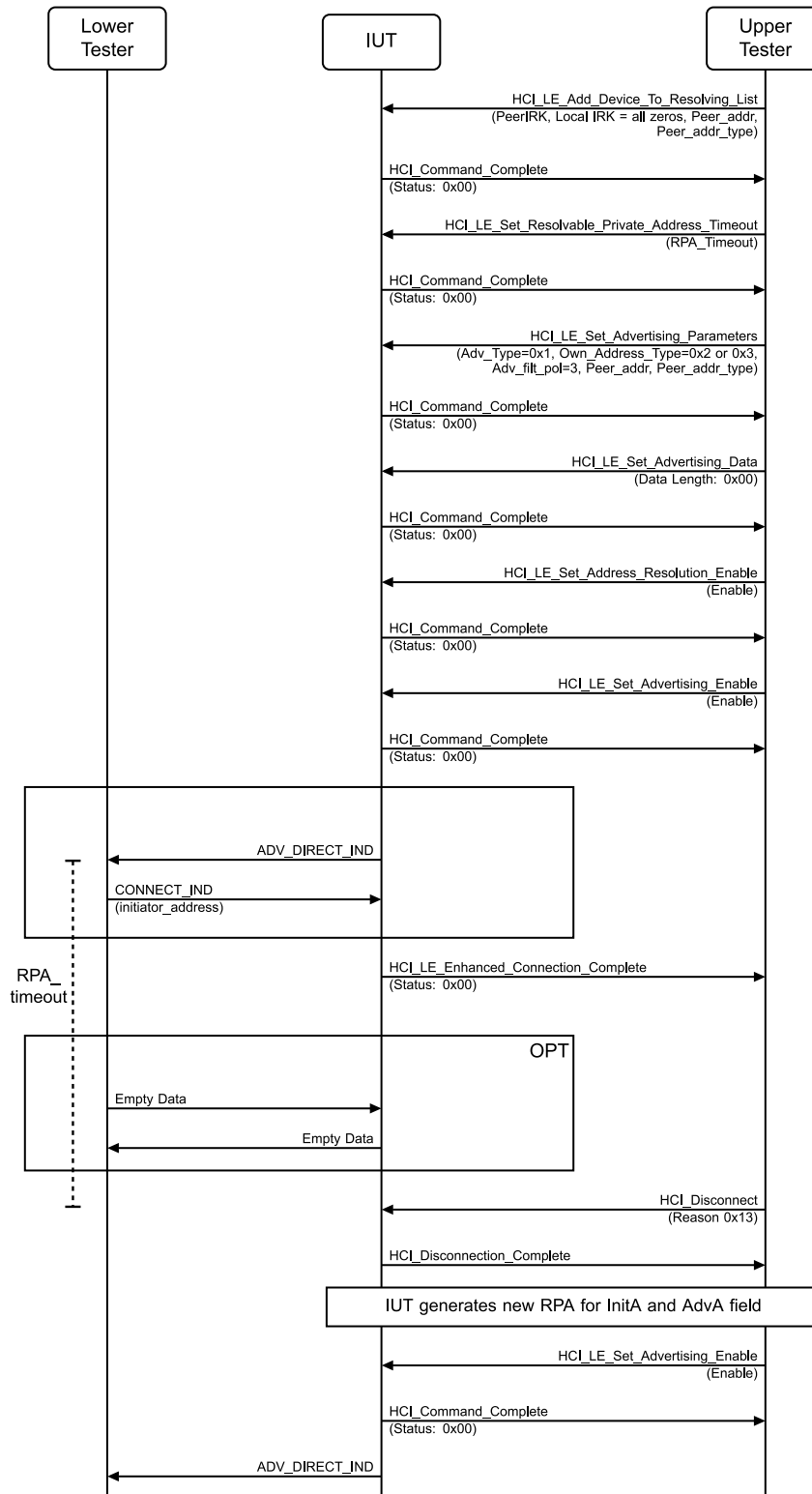
Figure 4.8-13: LL/SEC/ADV/BV-13-C [Network Privacy - Directed Connectable Advertising without local IRK but with remote IRK] MSC
