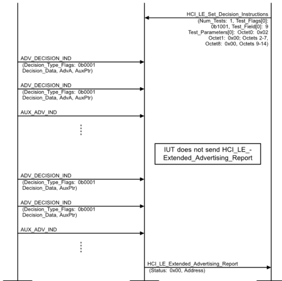
Figure 4.2-146: Decision-Based Advertisements, AdvA in Decision PDU MSC – Page 2 of 2
