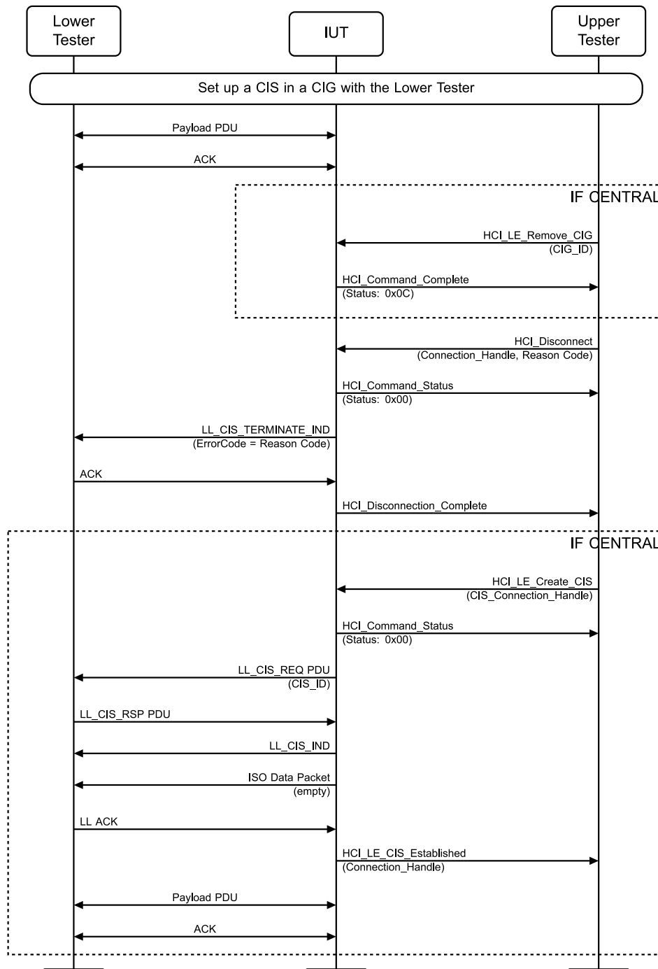
Figure 4.10-52: CIS Terminate Procedure, Initiated MSC
