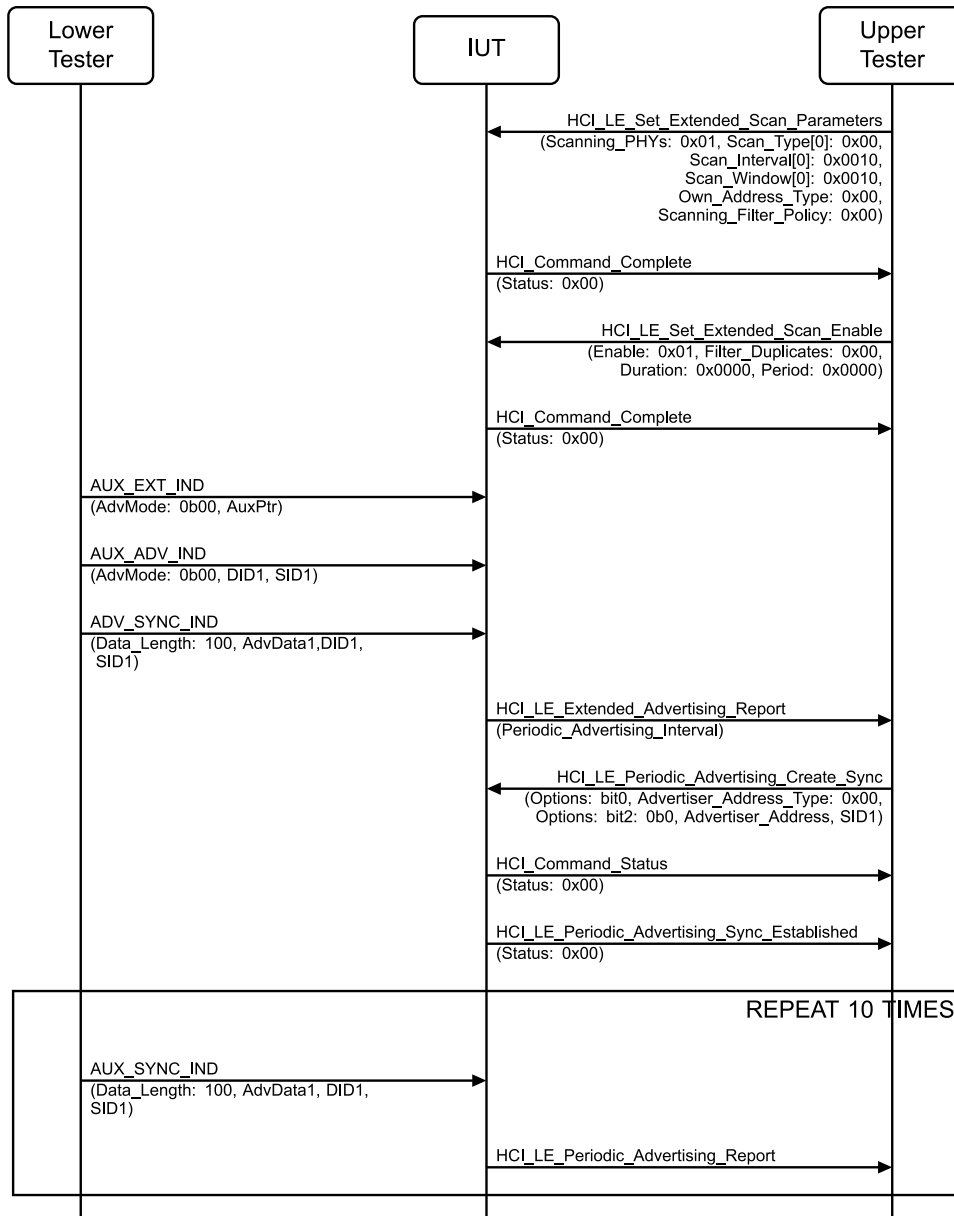
Figure 4.2-115: LL/DDI/SCN/BV-70-C [Scanner enables Duplicate Filtering after initially disabled] MSC – Page 1 of 2
