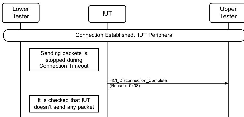
Figure 4.3-55: LL/CON/PER/BV-13-C [Peripheral supervision timer] MSC
