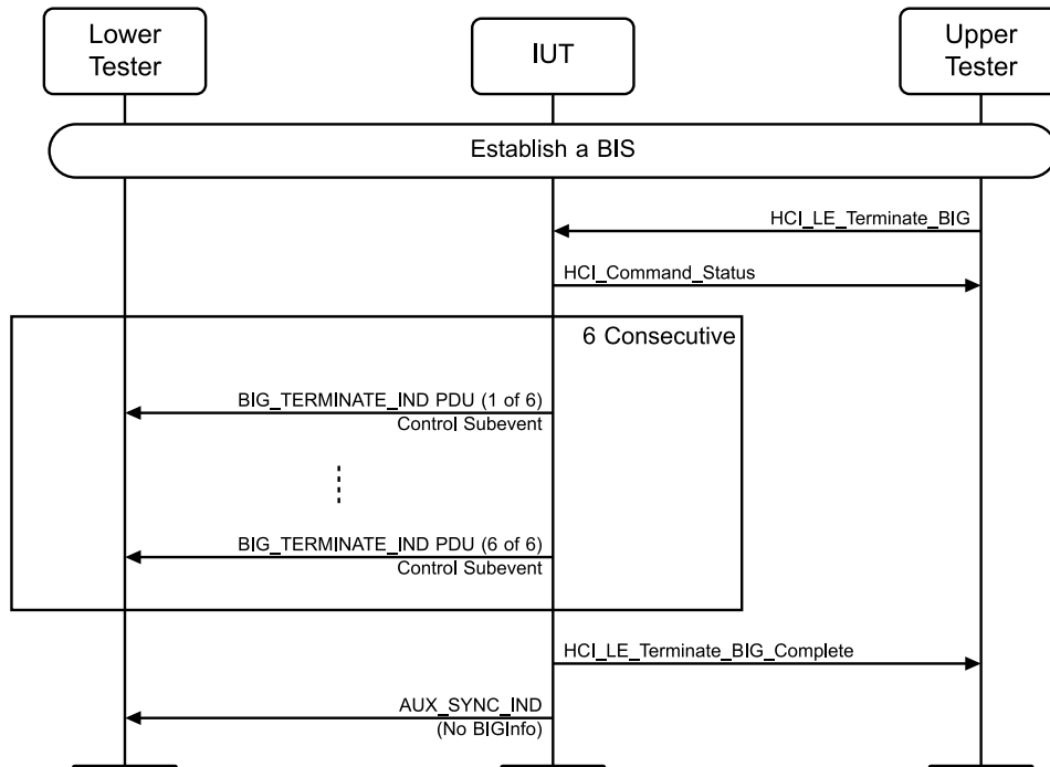
Figure 4.11-6: Isochronous Broadcaster Terminates BIS Stream MSC
