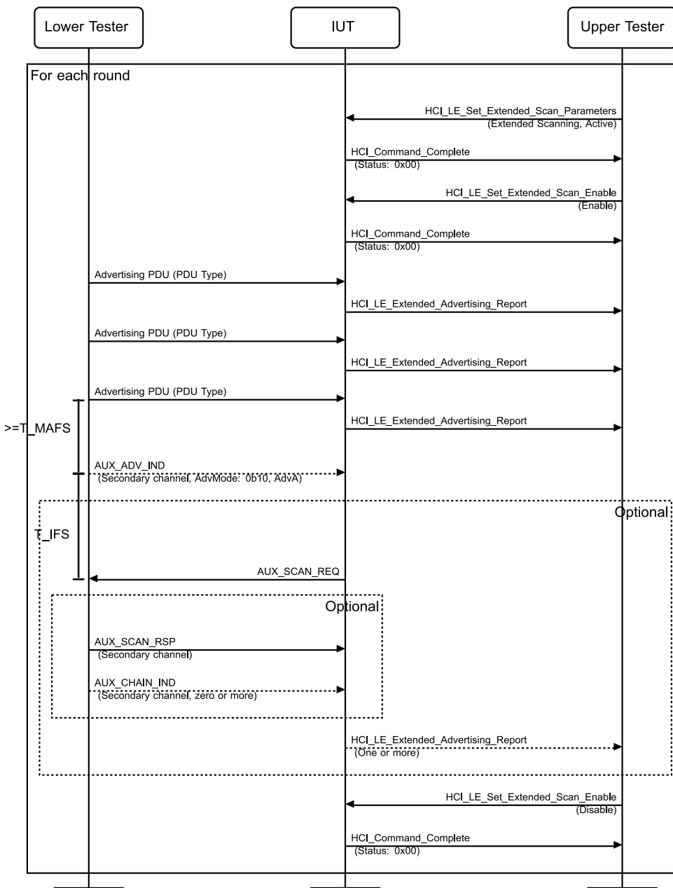
Figure 4.2-123: Extended Scanning, Properly Ignore RFU Fields, Extended Advertising MSC
