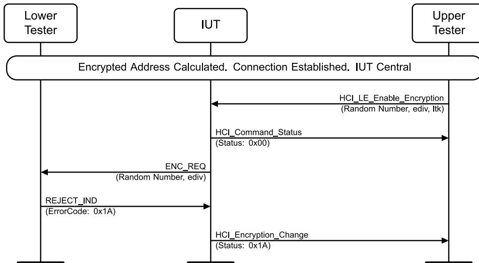
Figure 4.8-43: LL/SEC/CEN/BV-03-C [Central Receiving Reject_Ind] MSC
