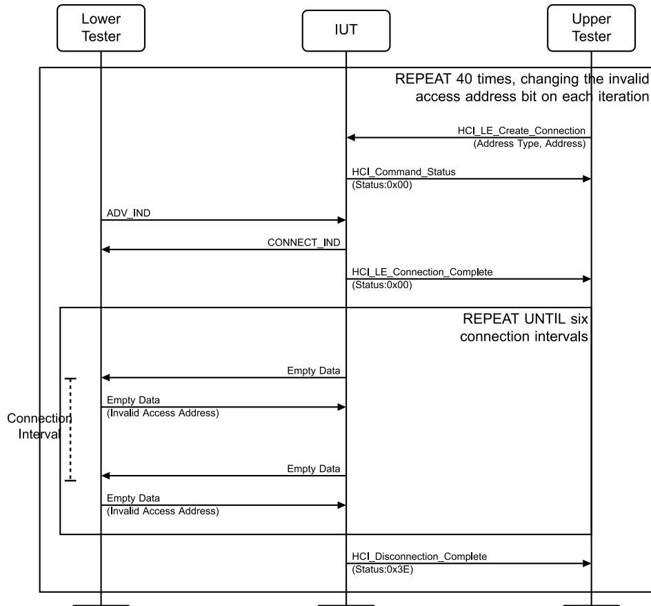
Figure 4.5-5: LL/ENC/INI/BI-01-C [Peripheral Packets Invalid Address] MSC
