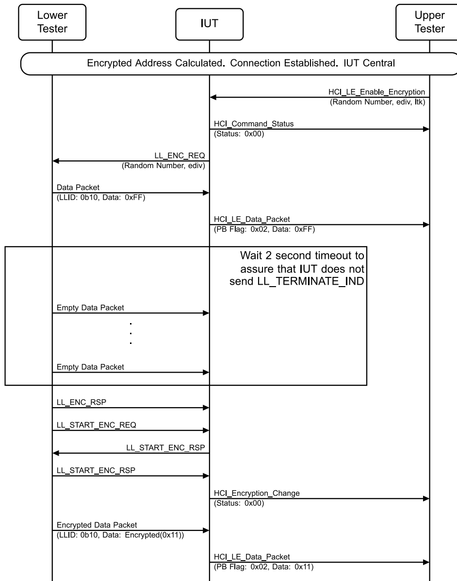
Figure 4.8-44: LL/SEC/CEN/BV-04-C [Central Encryption: Sending Data before LL_ENC_RSP] MSC
