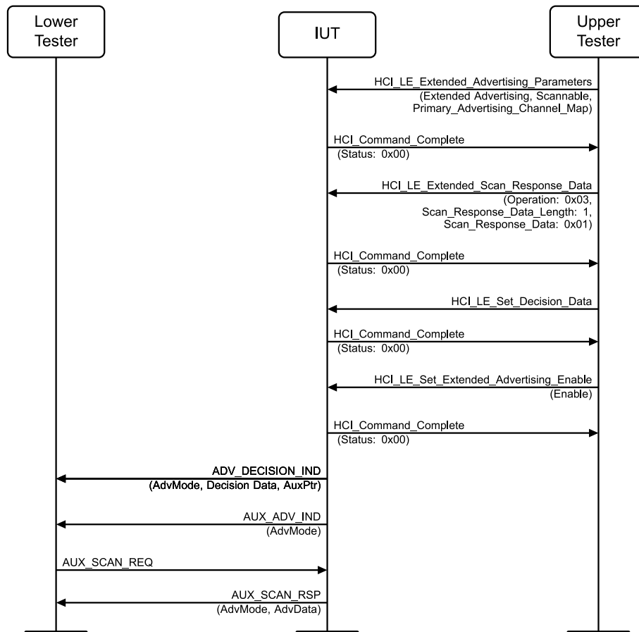
Figure 4.2-73: Decisions-Based Advertisements, Scannable MSC
