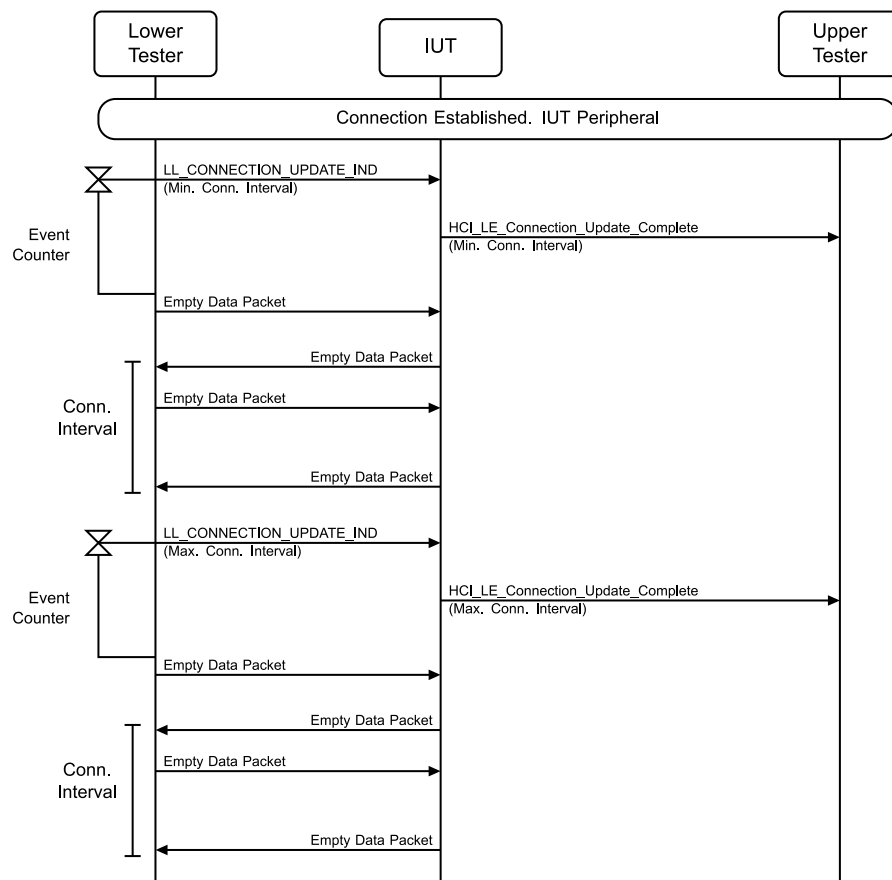
Figure 4.3-51: LL/CON/PER/BV-10-C [Accepting parameter update] MSC – Page 1 of 2
