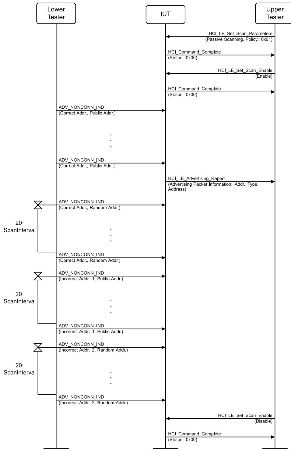
Figure 4.2-78: LL/DDI/SCN/BV-02-C [Passive Scanning Device Filtering] MSC
