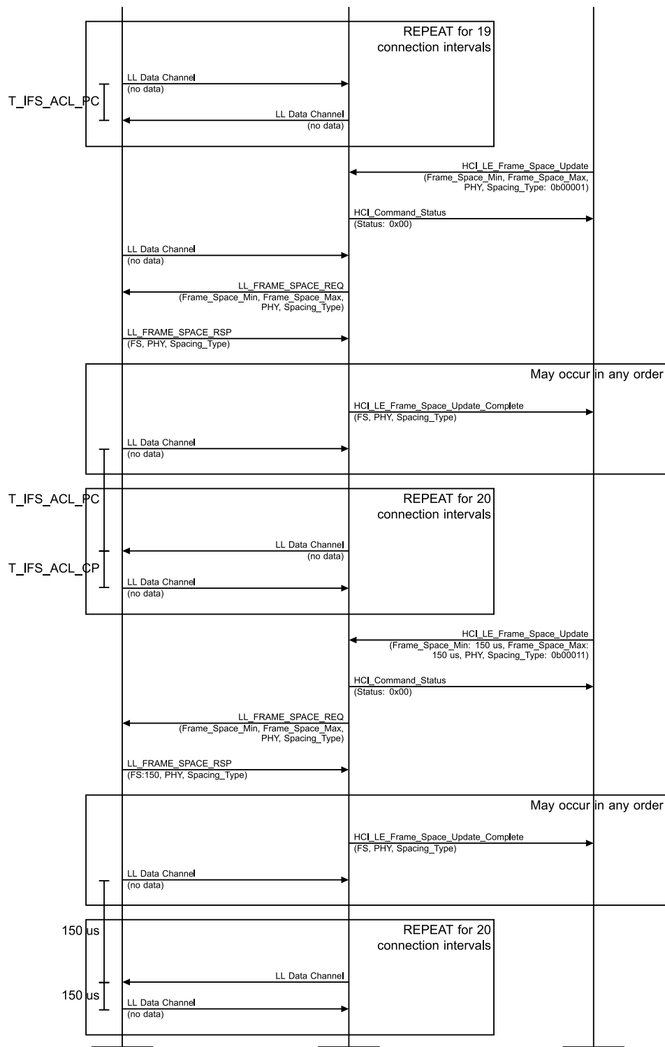
Figure 4.4-34: Initiate Inter Frame Space Change Request in the current ACL connection, Asymmetric PHYs, Peripheral Transmit, Central MSC – Page of 2 of 2
