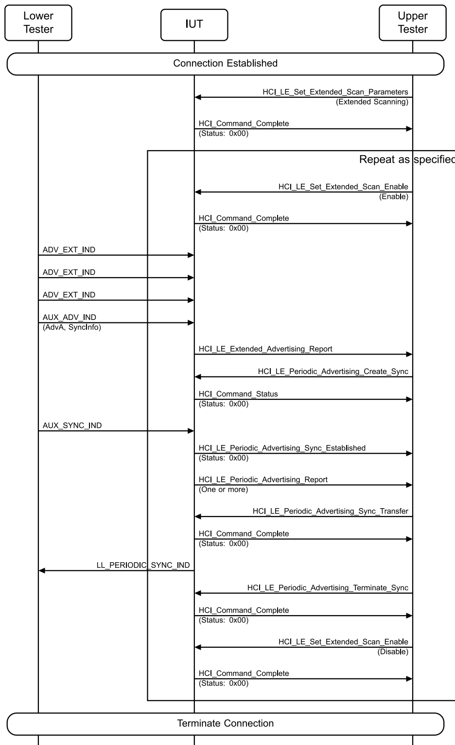
Figure 4.3-215: Periodic Advertising Sync Transfer Procedure, Synchronized IUT Initiated MSC
