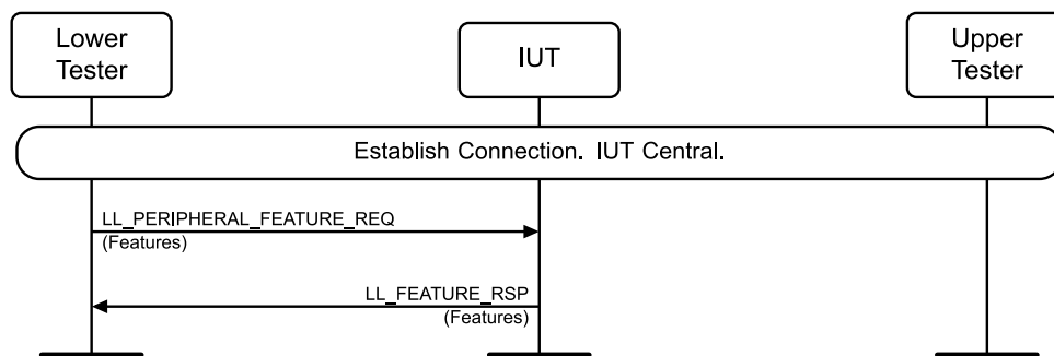
Figure 4.3-152: LL/CON/CEN/BV-23-C [Responding to Feature Exchange] MSC
