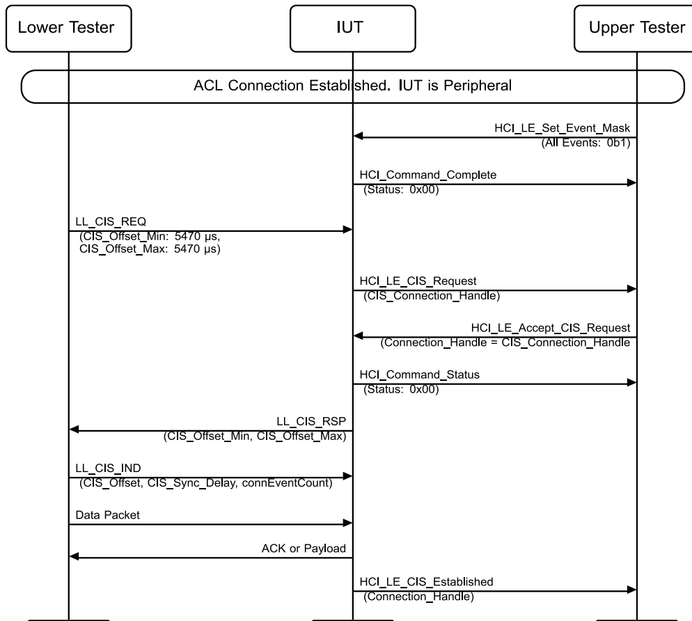
Figure 4.10-44: LL/CIS/PER/BV-48-C [CIS Setup Response Procedure, Peripheral] MSC
