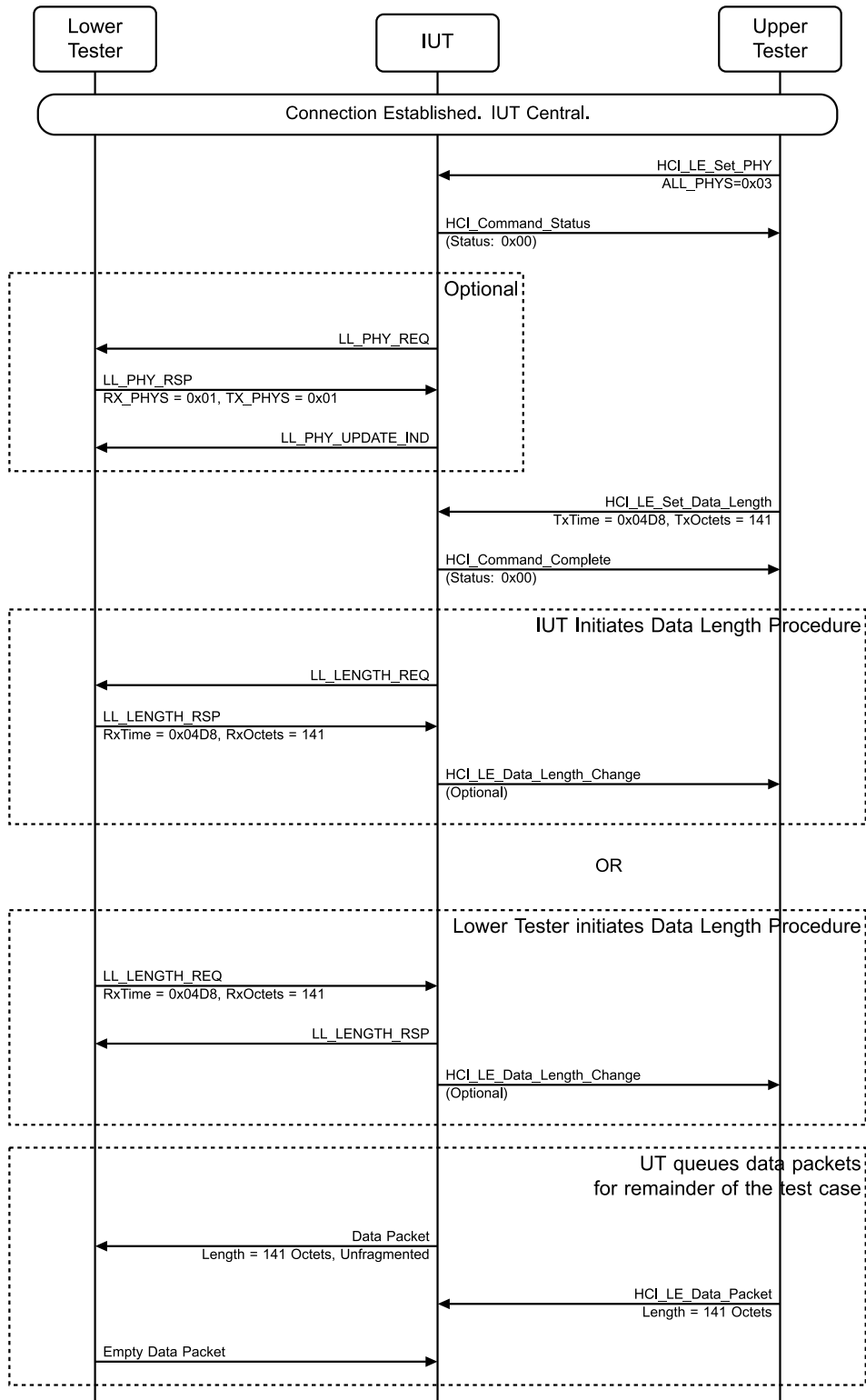
Figure 4.3-179: LL/CON/CEN/BV-54-C [Responding to PHY Update Procedure – Packet Time Restrictions, LE Coded] MSC – Page 1 of 2
