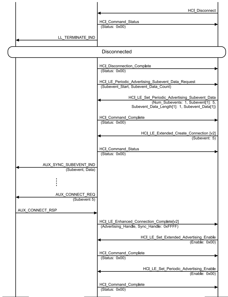
Figure 4.2-66: Reconnect with a Synchronized Device using Periodic Advertising with Responses MSC – Page 3 of 3
