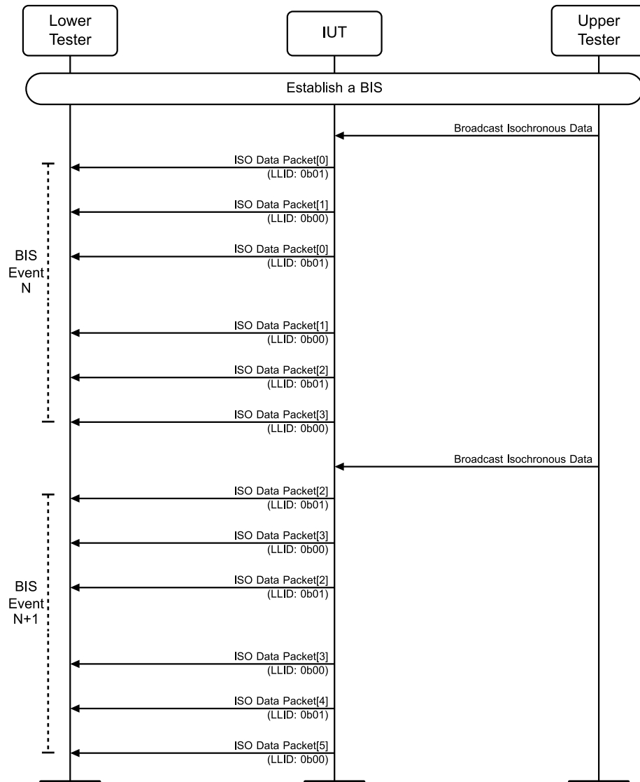
Figure 4.11-11: LL/BIS/BRD/BV-26-C [Pre-transmissions in Broadcast Isochronous Stream, Verify LLID] MSC
