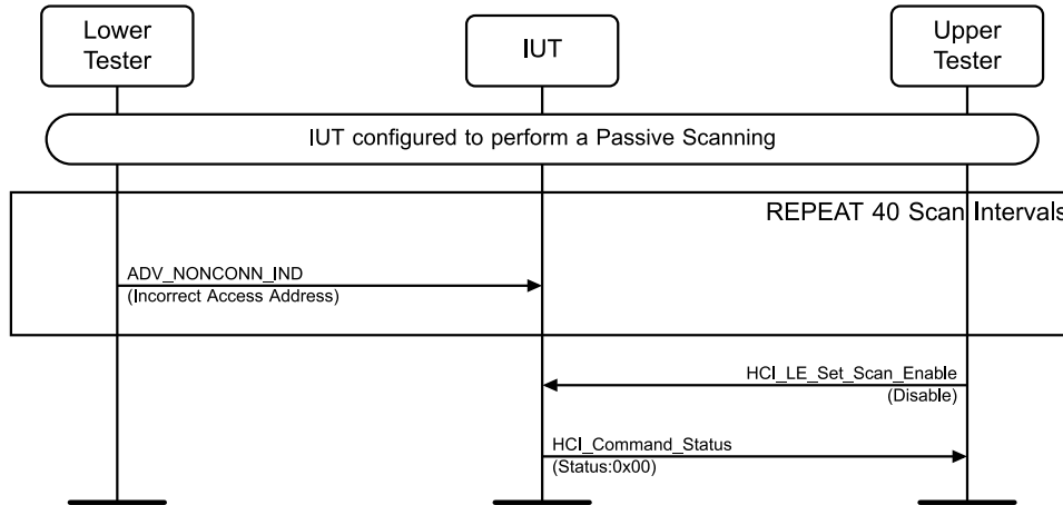
Figure 4.5-3: LL/ENC/SCN/BI-01-C [Passive Scanning Invalid Address] MSC
