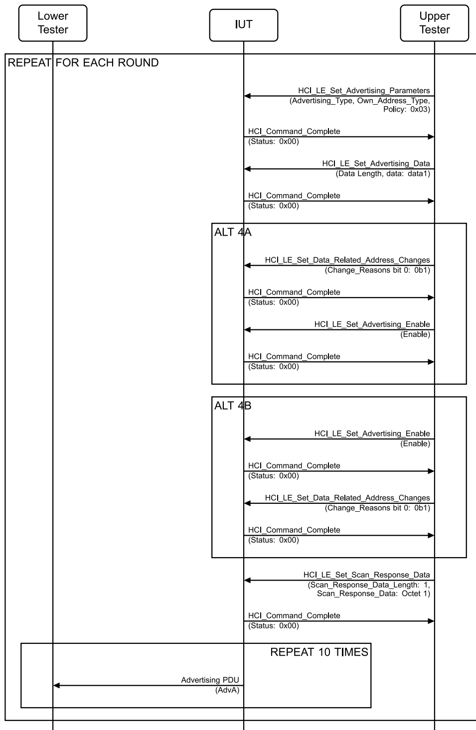
Figure 4.2-52: Advertising Data, New RPA on Change Reasons MSC – Page 1 of 2
