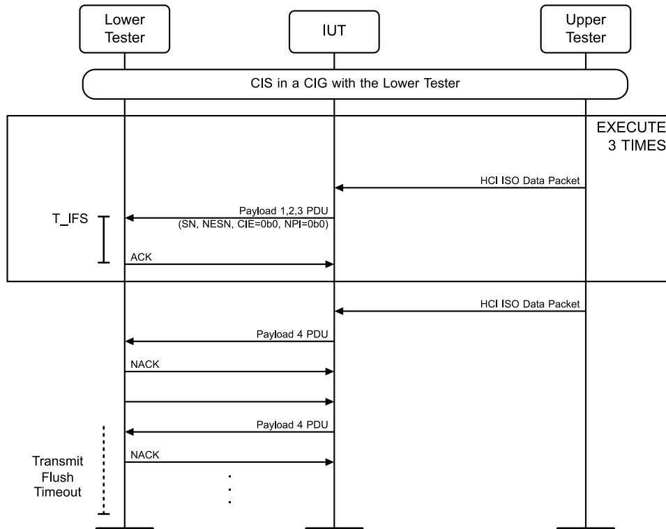
Figure 4.10-12: Acknowledgement Scheme, Central MSC
