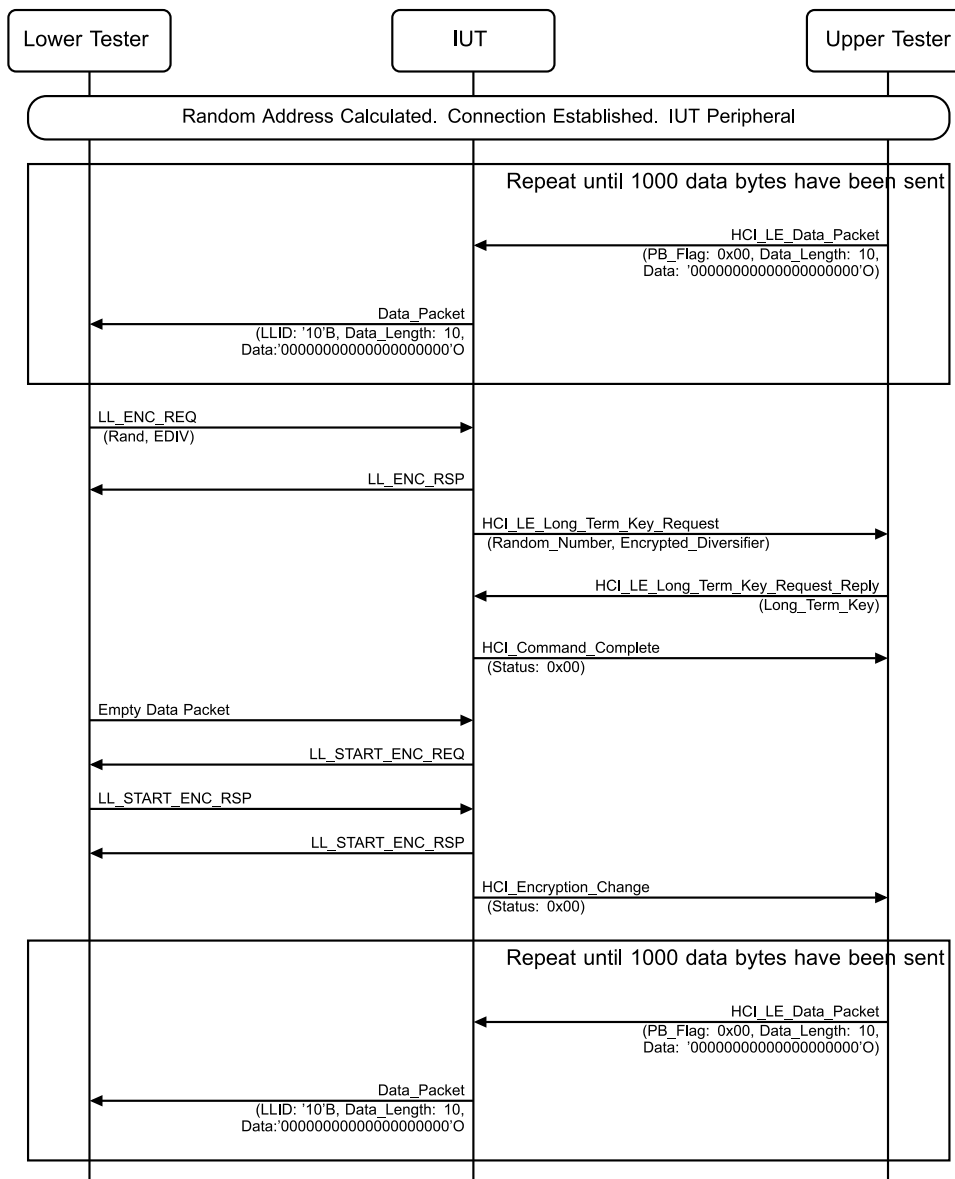
Figure 4.8-28: LL/SEC/PER/BV-01-C [Peripheral Encryption Mode Setup] MSC
