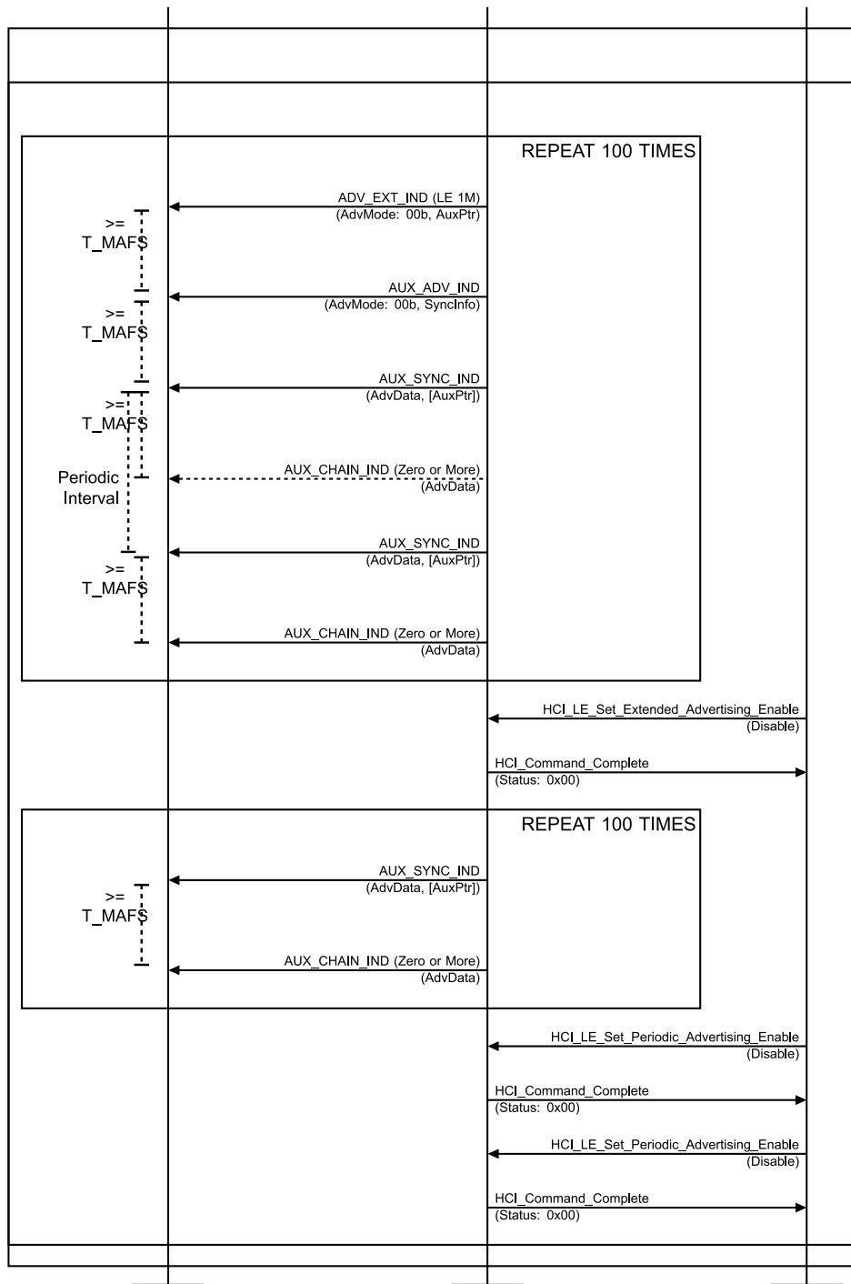
Figure 4.2-22: Extended Advertising, Periodic Advertising MSC – Page 2 of 2
