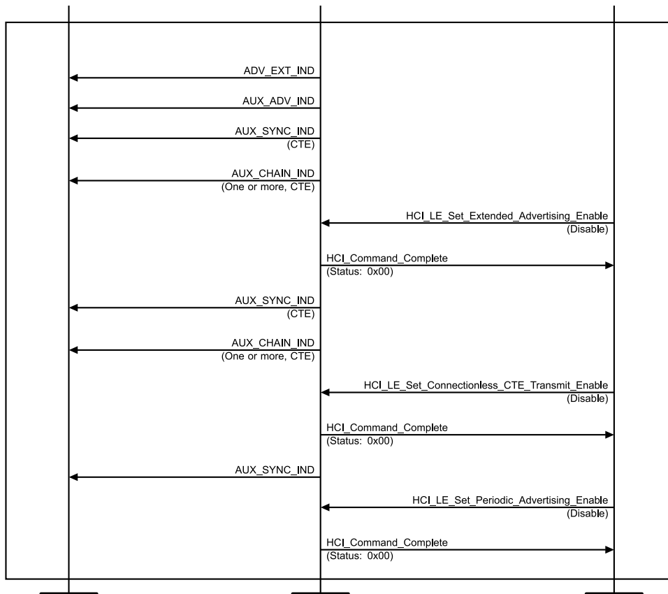
Figure 4.2-38: AoA Connectionless CTE Advertising MSC – Page 2 of 2
