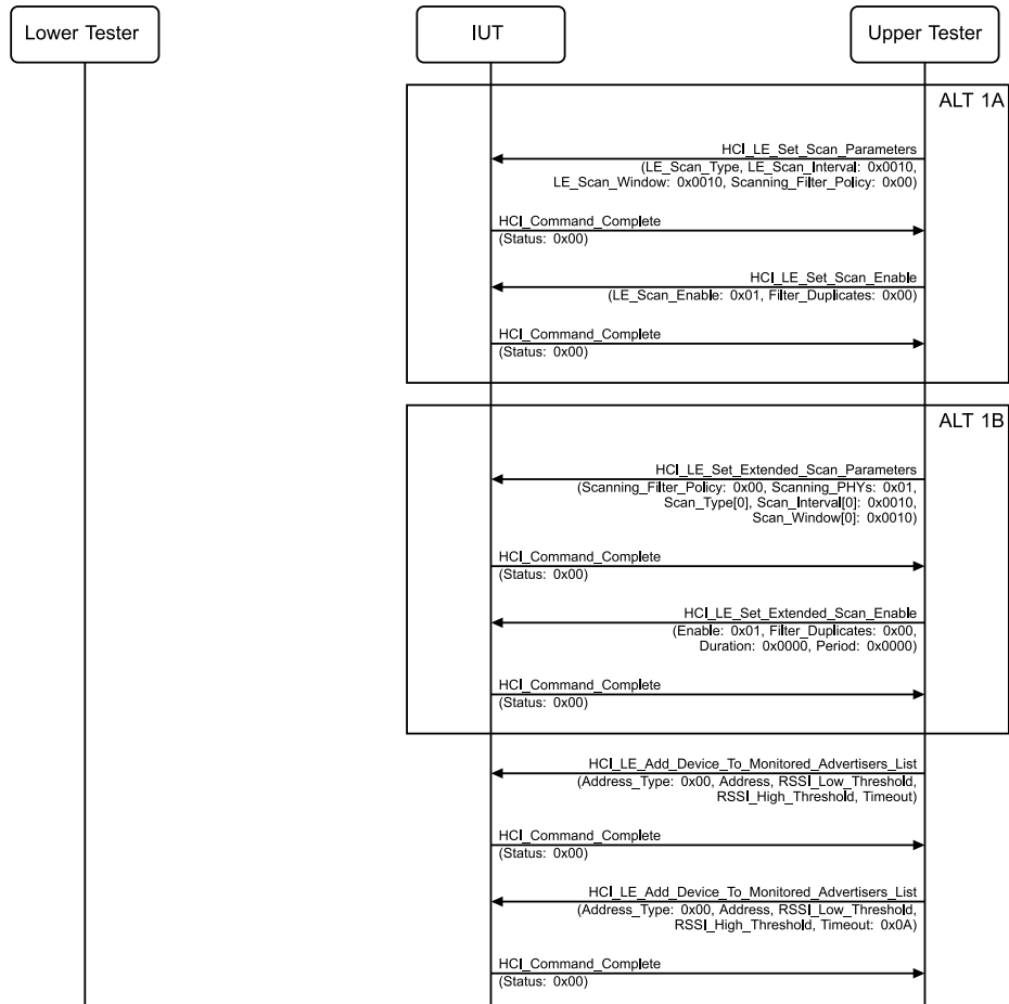
Figure 4.2-150: Monitoring Advertisers, Clear List MSC – Page 1 of 2
