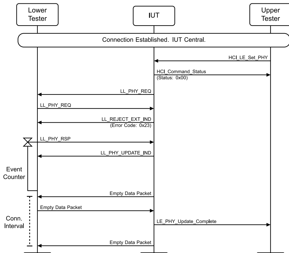
Figure 4.3-167: LL/CON/CEN/BV-45-C [Handling Protocol Collision – Same Procedure] MSC
