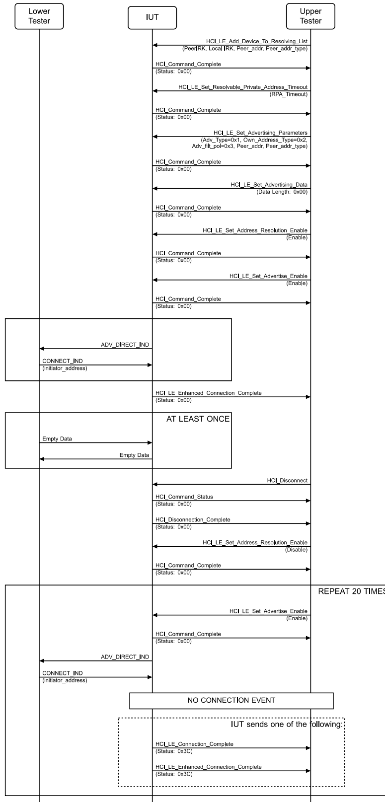
Figure 4.8-11: LL/SEC/ADV/BV-11-C [Network Privacy - Directed Connectable Advertising using local and remote IRK] MSC
