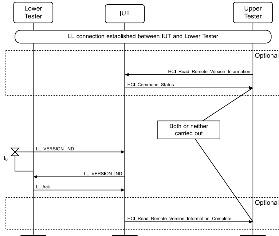
Figure 4.3-255: Version Exchange, IUT Requesting, Collision MSC
