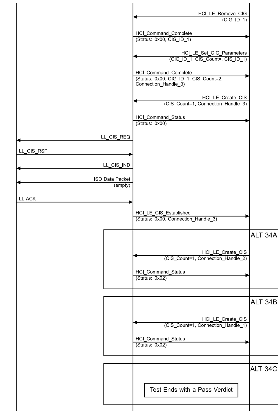
Figure 4.10-22: LL/CIS/CEN/BV-51-C [CIS Setup Procedure, Central Initiated, CIG ID Reuse] MSC – Page 2 of 2
