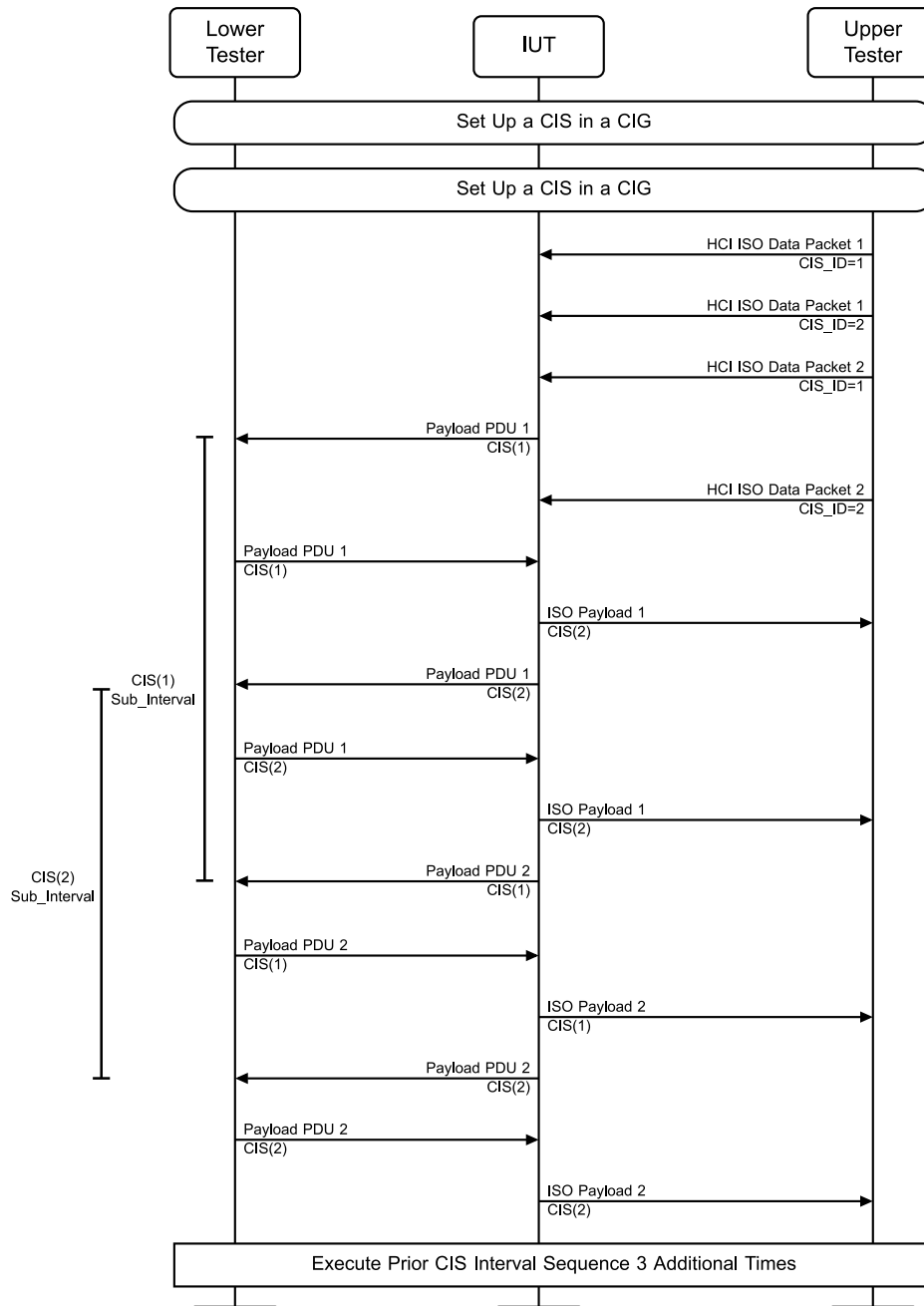
Figure 4.10-18: LL/CIS/CEN/BV-44-C [Sending and Receiving Data in Multiple CISes, Single CIG, Single Connection, Interleaved CIG, Central, BN > 1, NSE = 2] MSC
