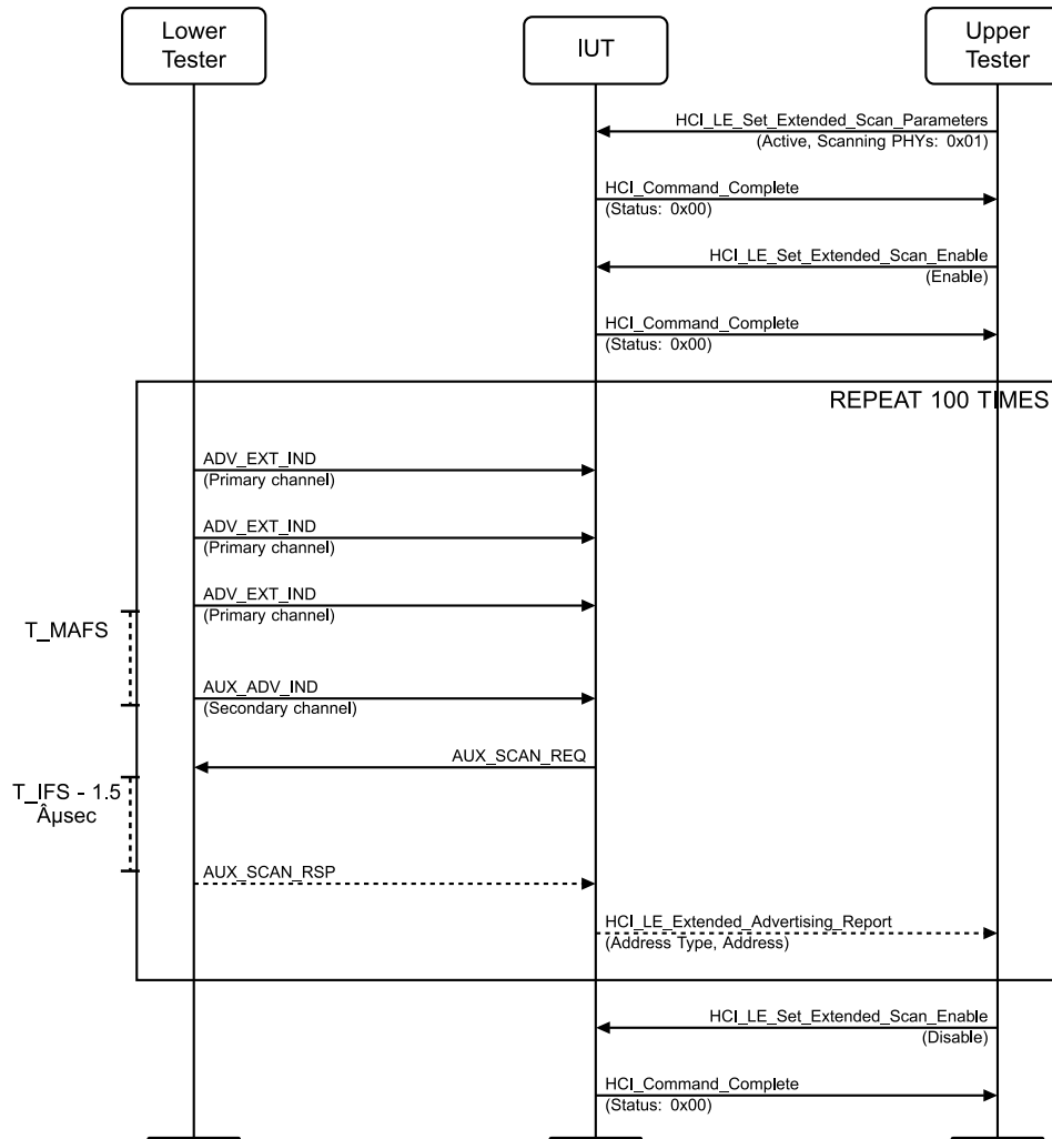
Figure 4.4-52: Extended Scanning, Secondary Channel, Earliest Transmission to Scanner MSC
