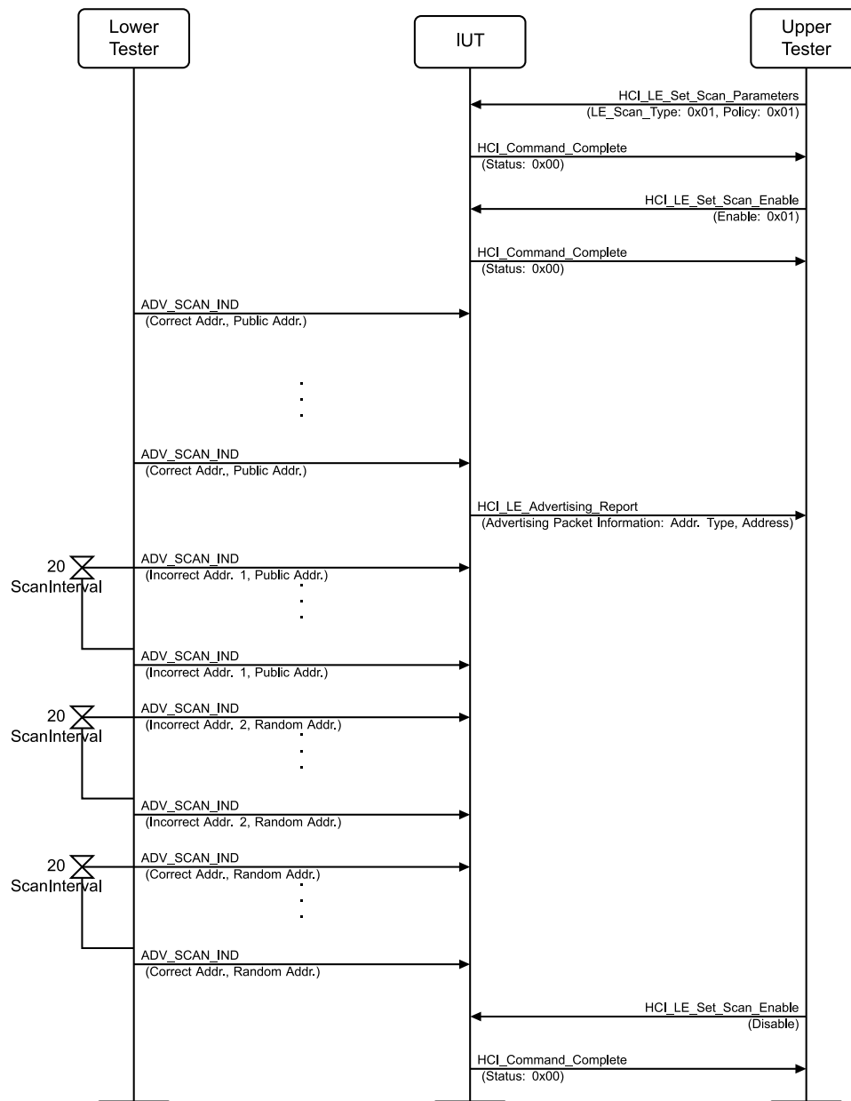
Figure 4.2-83: LL/DDI/SCN/BV-12-C [Passive Scanning: Discoverable events] MSC
