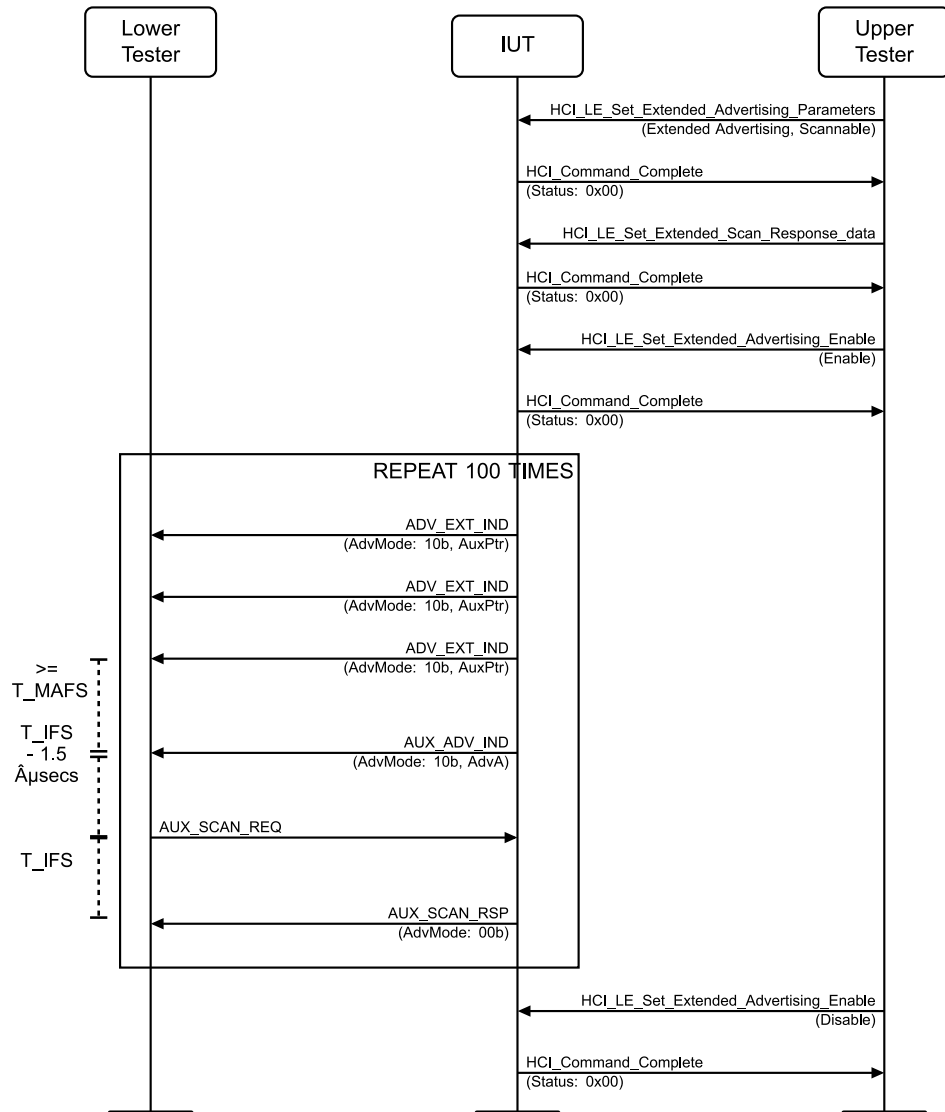
Figure 4.4-2: Extended Advertising, Secondary Channel, Earliest Transmission to Advertiser MSC
