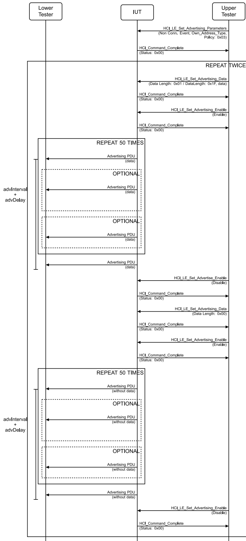
Figure 4.2-2: Advertising Data: Non-Connectable or Undirected MSC
