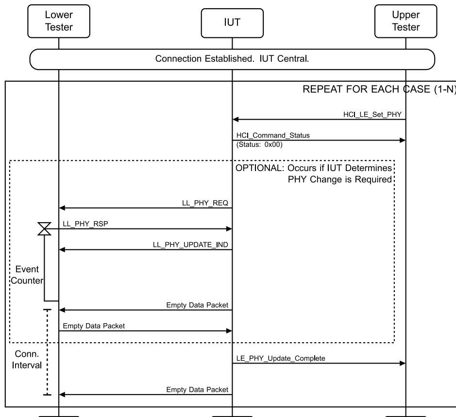
Figure 4.3-165: LL/CON/CEN/BV-41-C [Initiating PHY Update Procedure] MSC
