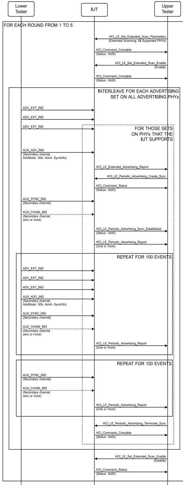
Figure 4.2-98: LL/DDI/SCN/BV-25-C [Extended Scanning, Multiple Sets, Periodic Advertising Reception, Multiple PHYs (All Supported PHYs)] MSC
