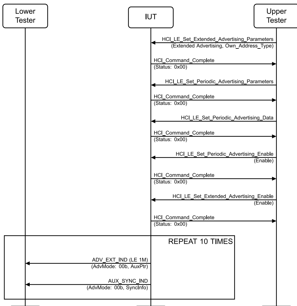
Figure 4.2-41: LL/DDI/ADV/BV-43-C [Periodic Advertising validating SyncInfo fields] MSC
