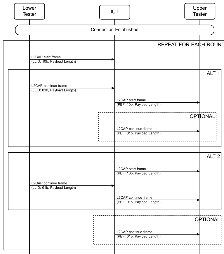
Figure 4.9-2: Receive Fragmented L2CAP Header MSC
