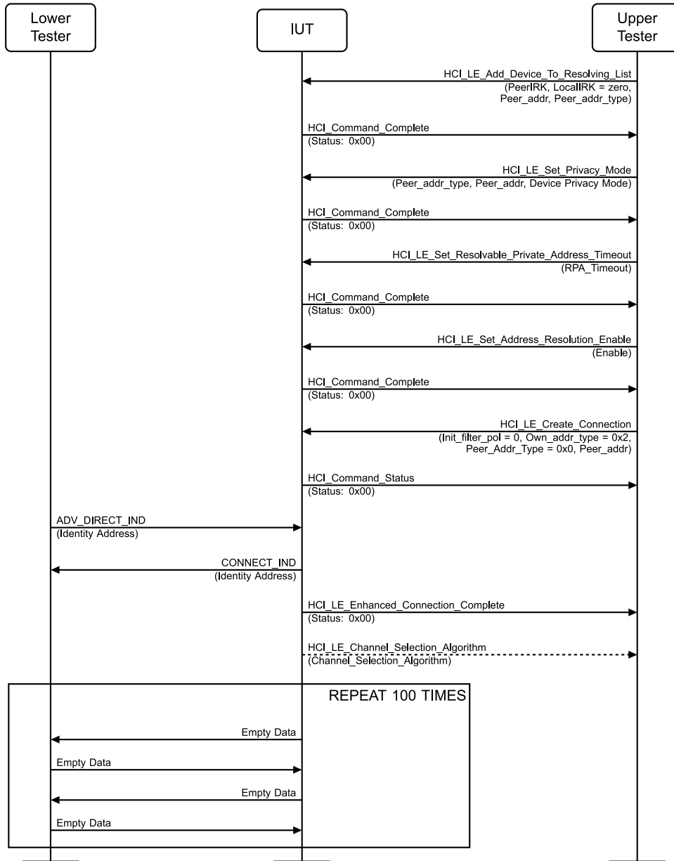
Figure 4.3-36: Device Privacy – Connection Establishment using directed advertising and resolving list, Initiator, Accept Identity Address MSC
