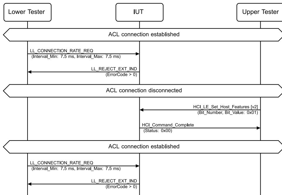
Figure 4.3-210: LL/CON/CEN/BI-20-C [Reject Connection Rate Request procedure, Connection Rate Host Bit not set]
