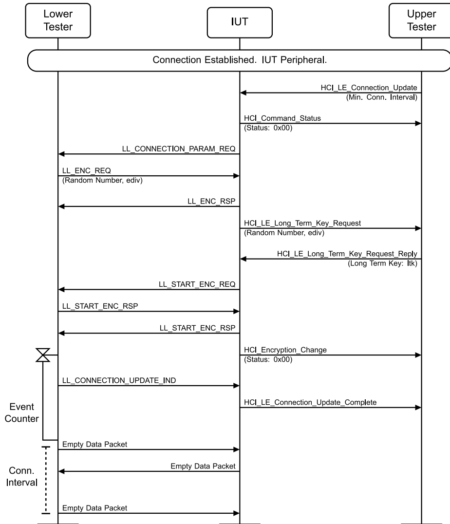
Figure 4.3-70: LL/CON/PER/BV-28-C [Initiating Connection Parameter Request – different procedure collision – encryption] MSC
