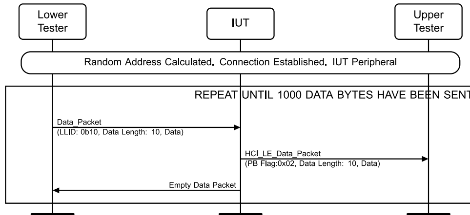
Figure 4.8-31: LL/SEC/PER/BV-05-C [Peripheral Receiving Encrypted Data] MSC
