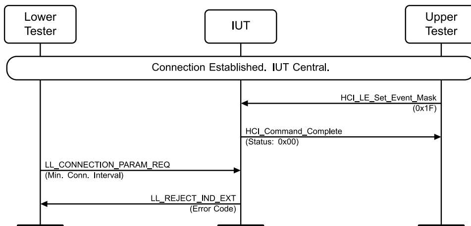
Figure 4.3-163: LL/CON/CEN/BV-34-C [Accepting Connection Parameter Request – event masked] MSC
