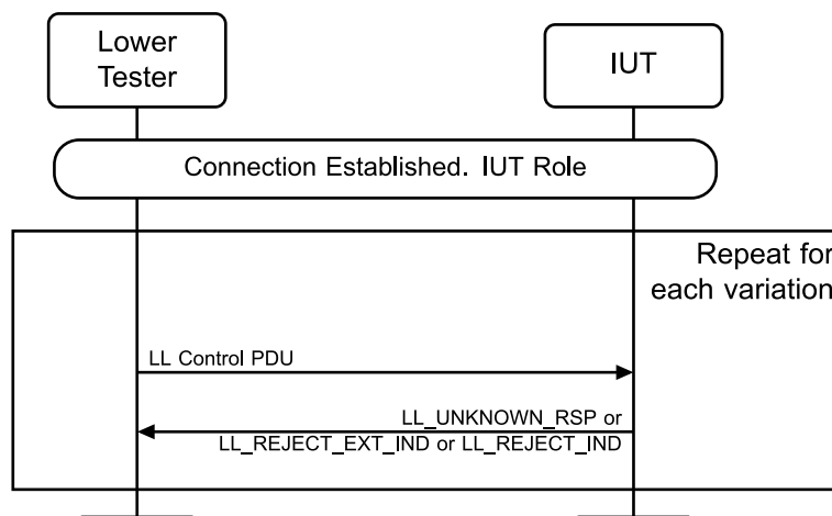
Figure 4.7-3: Control PDUs with Invalid CtrData MSC
