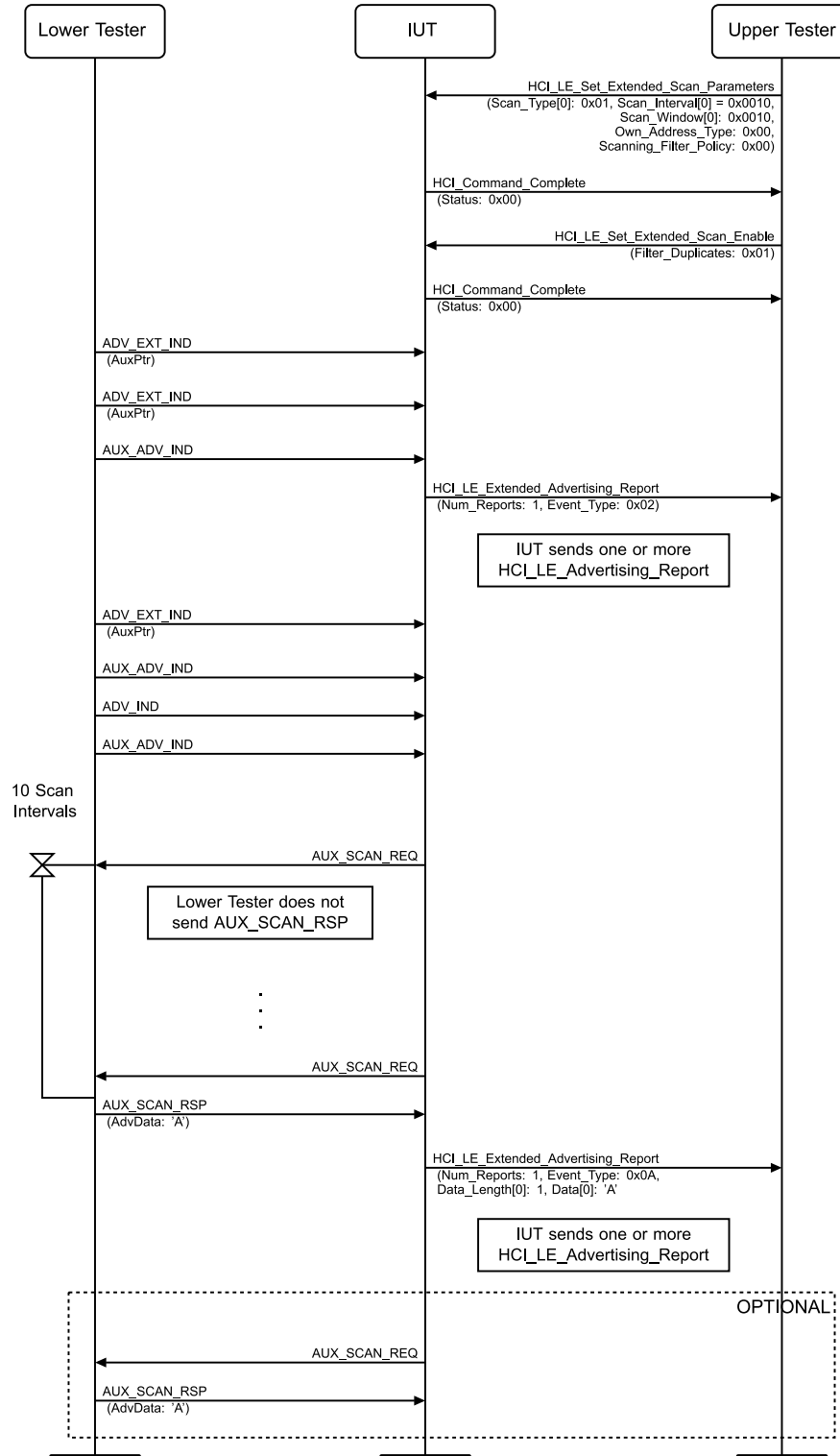
Figure 4.2-153: LL/DDI/SCN/BV-128-C [Extended Scanning, Active, Duplicate Filtering] MSC
