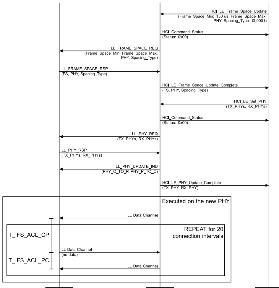
Figure 4.4-41: Initiate Inter Frame Space Change on a Different Asymmetric PHY for TX and RX, Central MSC – Page 2 of 2
