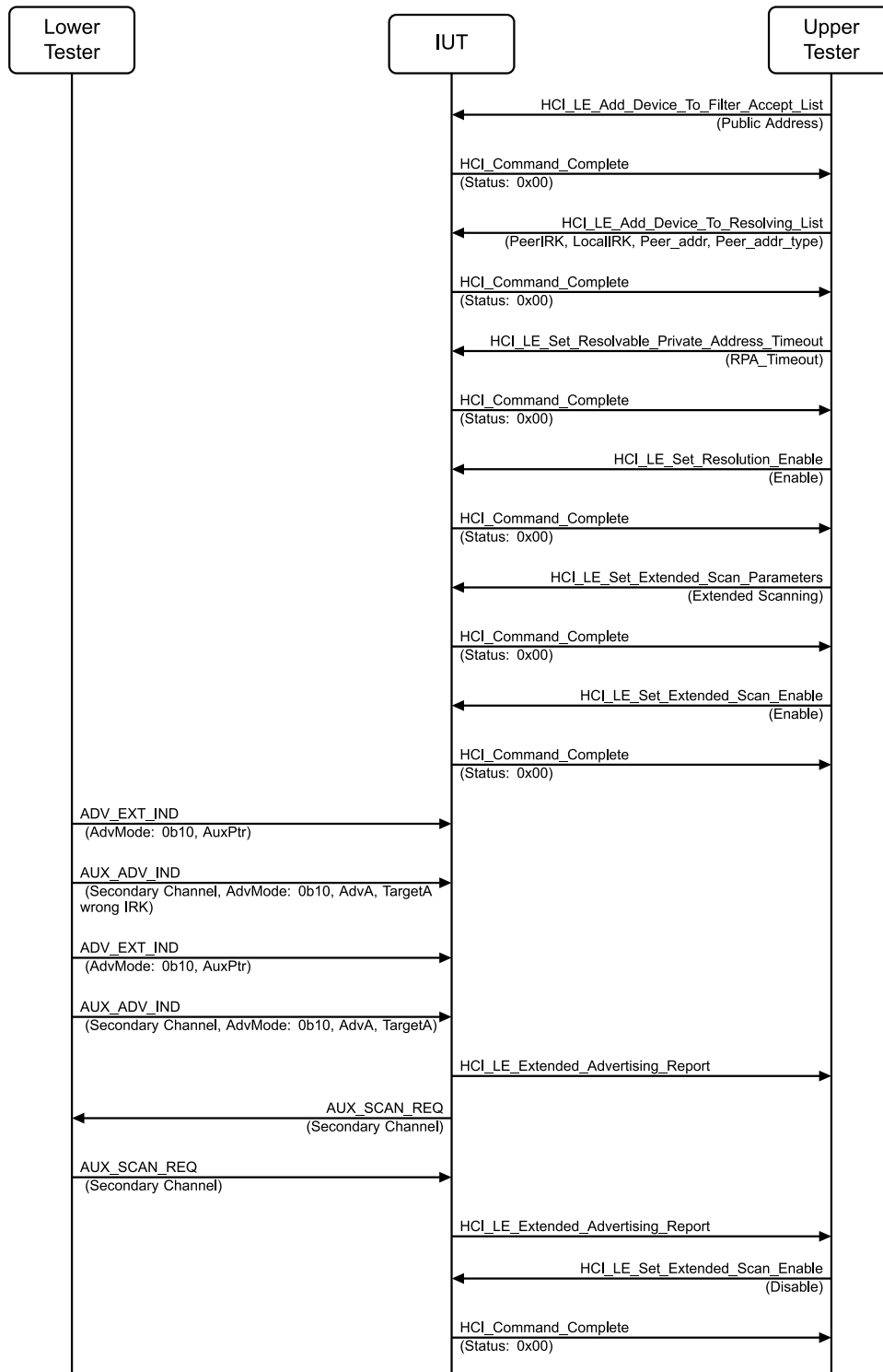
Figure 4.2-101: Privacy - Extended Scanning, Active MSC
