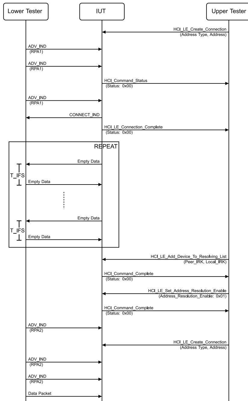
Figure 4.8-26: LL/SEC/INI/BI-01-C [Duplicate Connection Request, Different Peer RPA] MSC – Page 1 of 2
