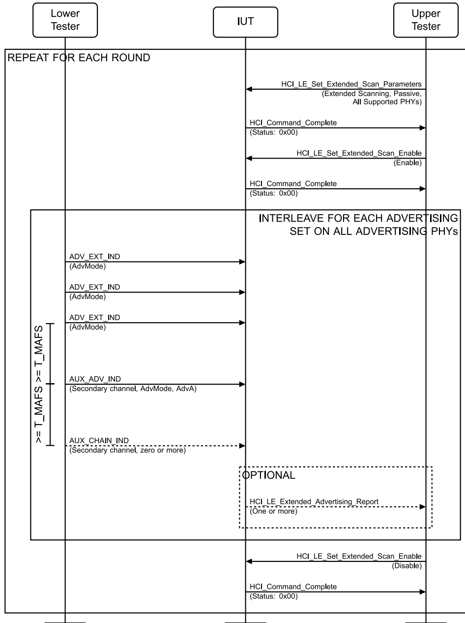
Figure 4.2-96: LL/DDI/SCN/BV-23-C [Extended Scanning, Multiple Sets, Passive, Multiple PHYs (All Supported PHYs)] MSC
