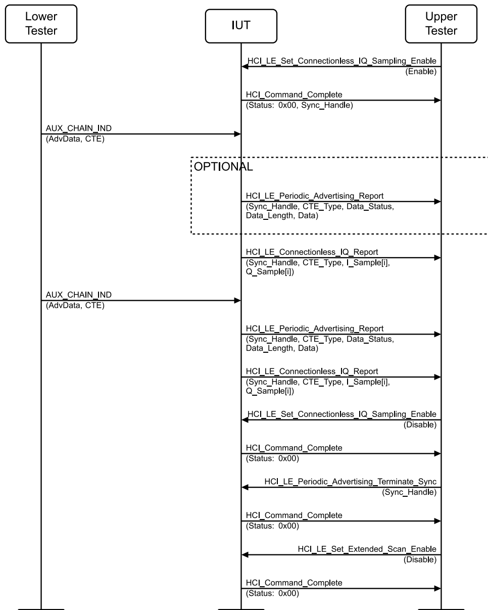
Figure 4.2-94: Connectionless CTE Scanning, Connectionless IQ Report MSC – Page 2 of 2
