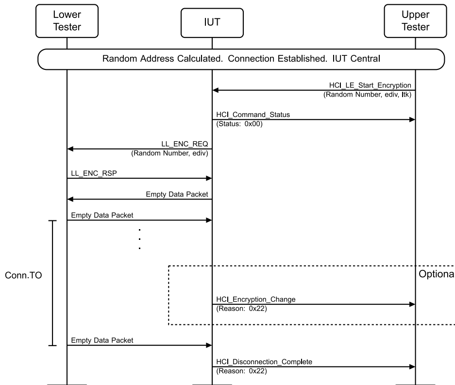
Figure 4.8-55: LL/SEC/CEN/BI-03-C [Central Encryption Setup: Missing Request] MSC
