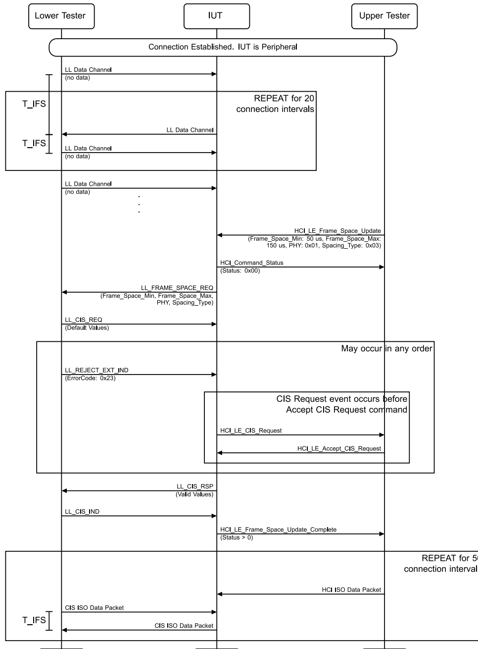
Figure 4.4-19: LL/TIM/PER/BV-28-C [Handling Frame Space Request Collision with CIS Creation, Peripheral] MSC
