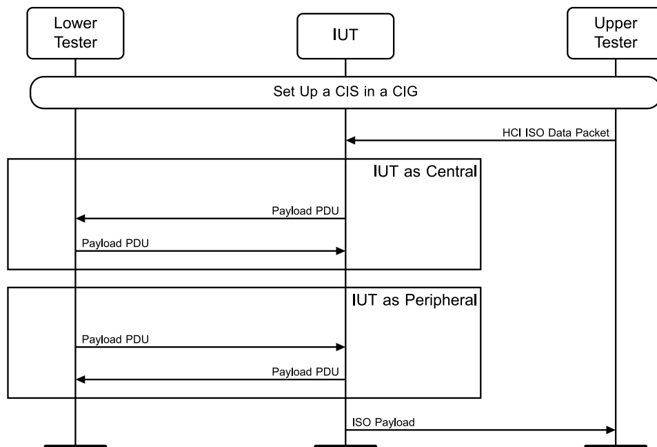
Figure 4.10-59: Sending and Receiving Data in Bidirectional CIS, BN = 1 MSC
