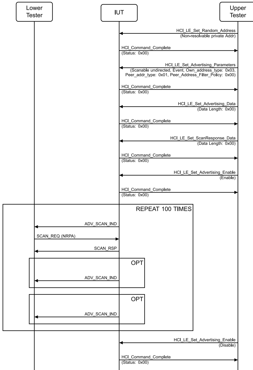
Figure 4.8-3: LL/SEC/ADV/BV-04-C [Network Privacy - Scannable Advertising, non-resolvable private address] MSC
