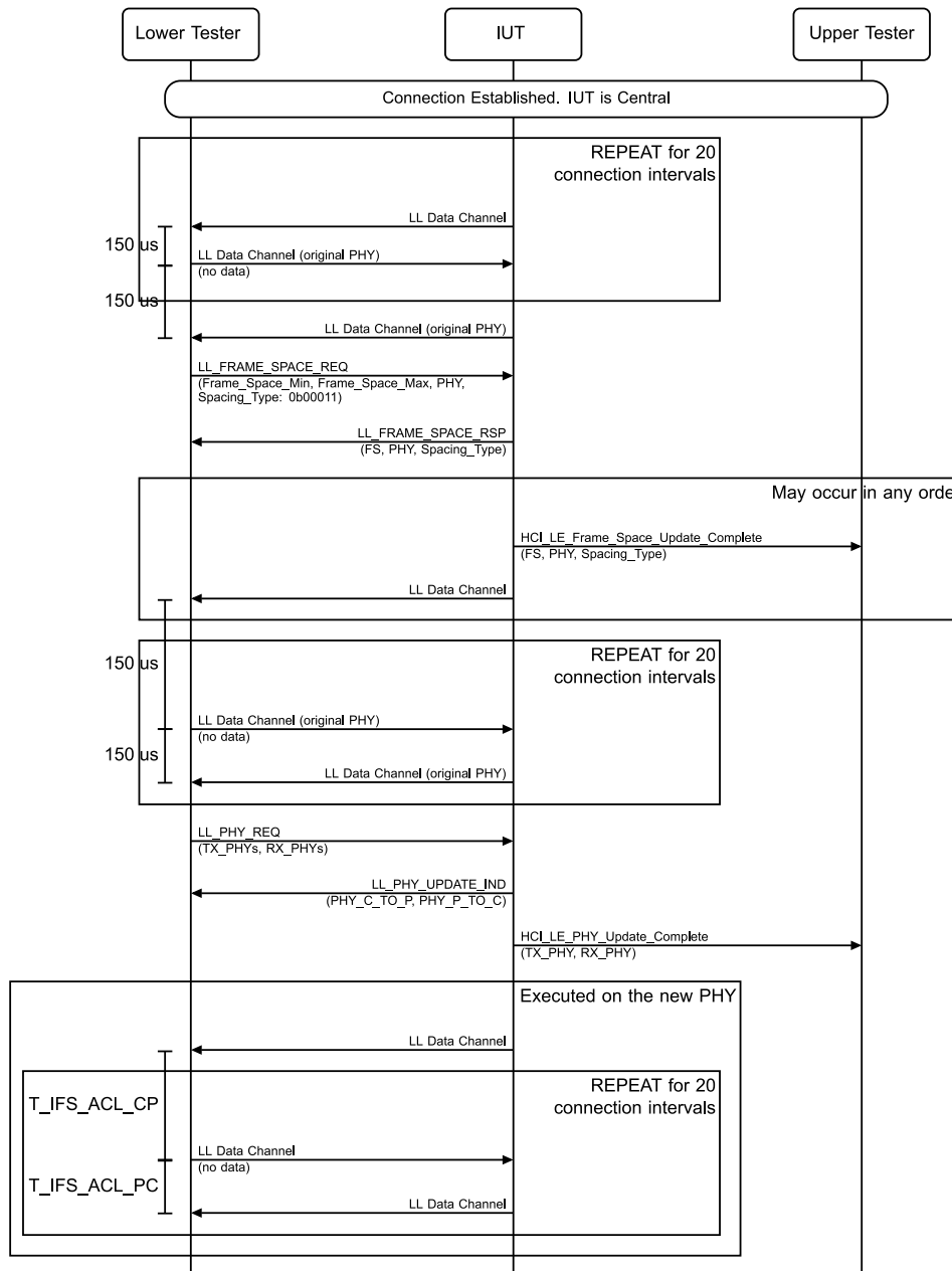
Figure 4.4-39: Respond to Inter Frame Space Change Request on a Different PHY, Central MSC
