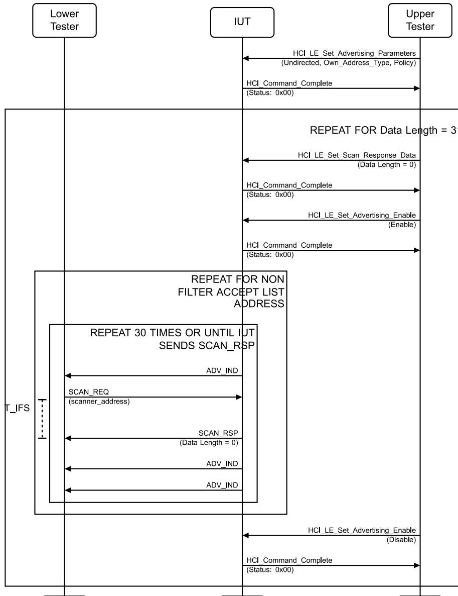
Figure 4.2-3: LL/DDI/ADV/BV-05-C [Scan Request: Undirected Connectable] MSC
