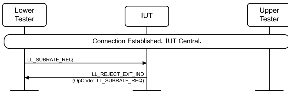
Figure 4.3-202: LL/CON/CEN/BV-140-C [Reject Subrate Request when Feature Bit is not set] MSC
