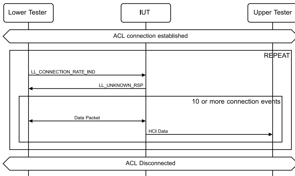
Figure 4.3-133: LL/CON/PER/BI-30-C [Reject Peer Connection Rate Update, invalid parameters] MSC
