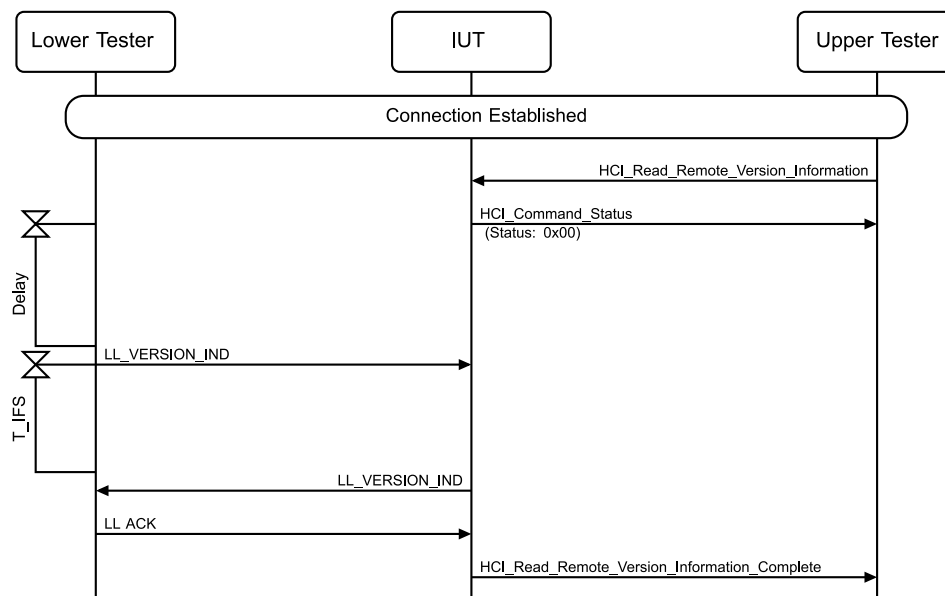
Figure 4.3-122: LL/CON/PER/BV-146-C [Version Exchange, IUT Requesting, Collision, Peripheral] MSC
