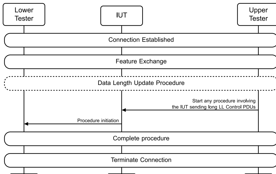
Figure 4.3-230: Sending Long Control PDUs after Feature Exchange MSC
