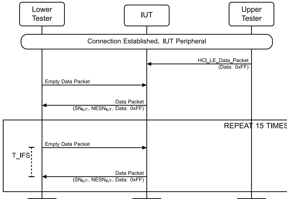
Figure 4.3-58: LL/CON/PER/BV-16-C [Peripheral retransmission] MSC
