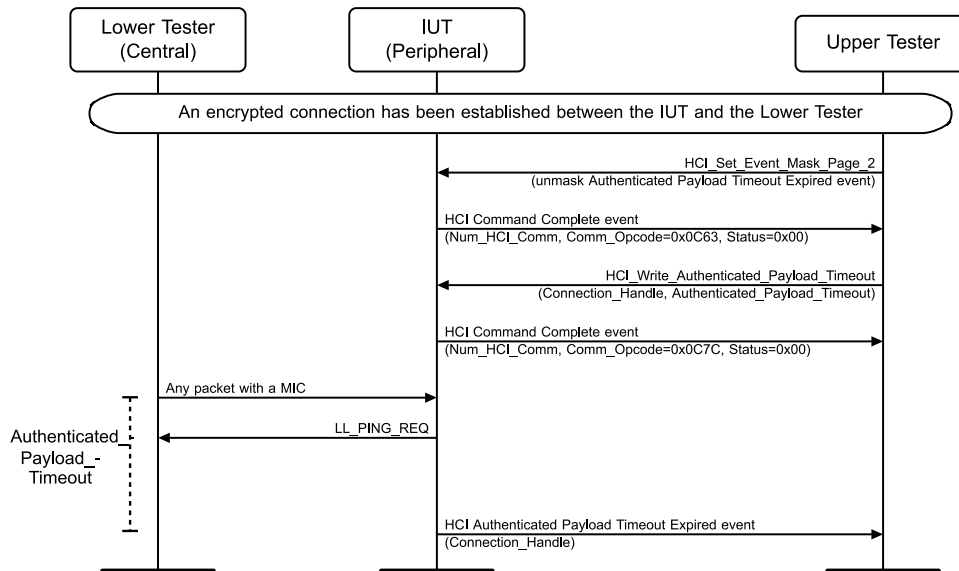
Figure 4.8-34: LL/SEC/PER/BV-08-C [No response to LL_PING_REQ] MSC
