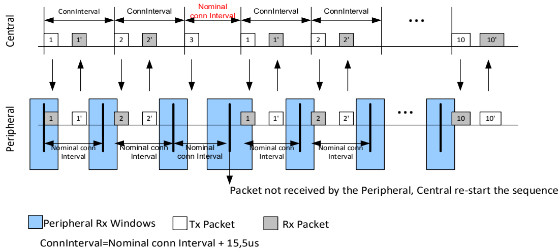
Figure 4.4-8: LL/TIM/PER/BV-05-C Timing sequence
