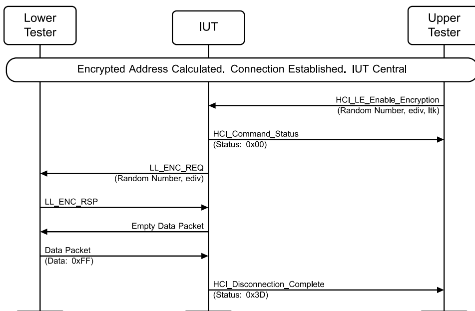
Figure 4.8-60: LL/SEC/CEN/BI-09-C [Central Encryption: Sending Data and Not Request] MSC
