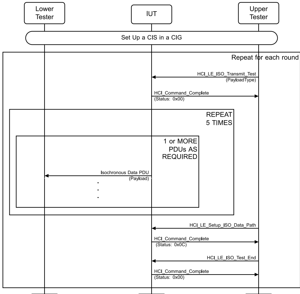
Figure 4.12-1: ISO Transmit Test Mode, CIS MSC
