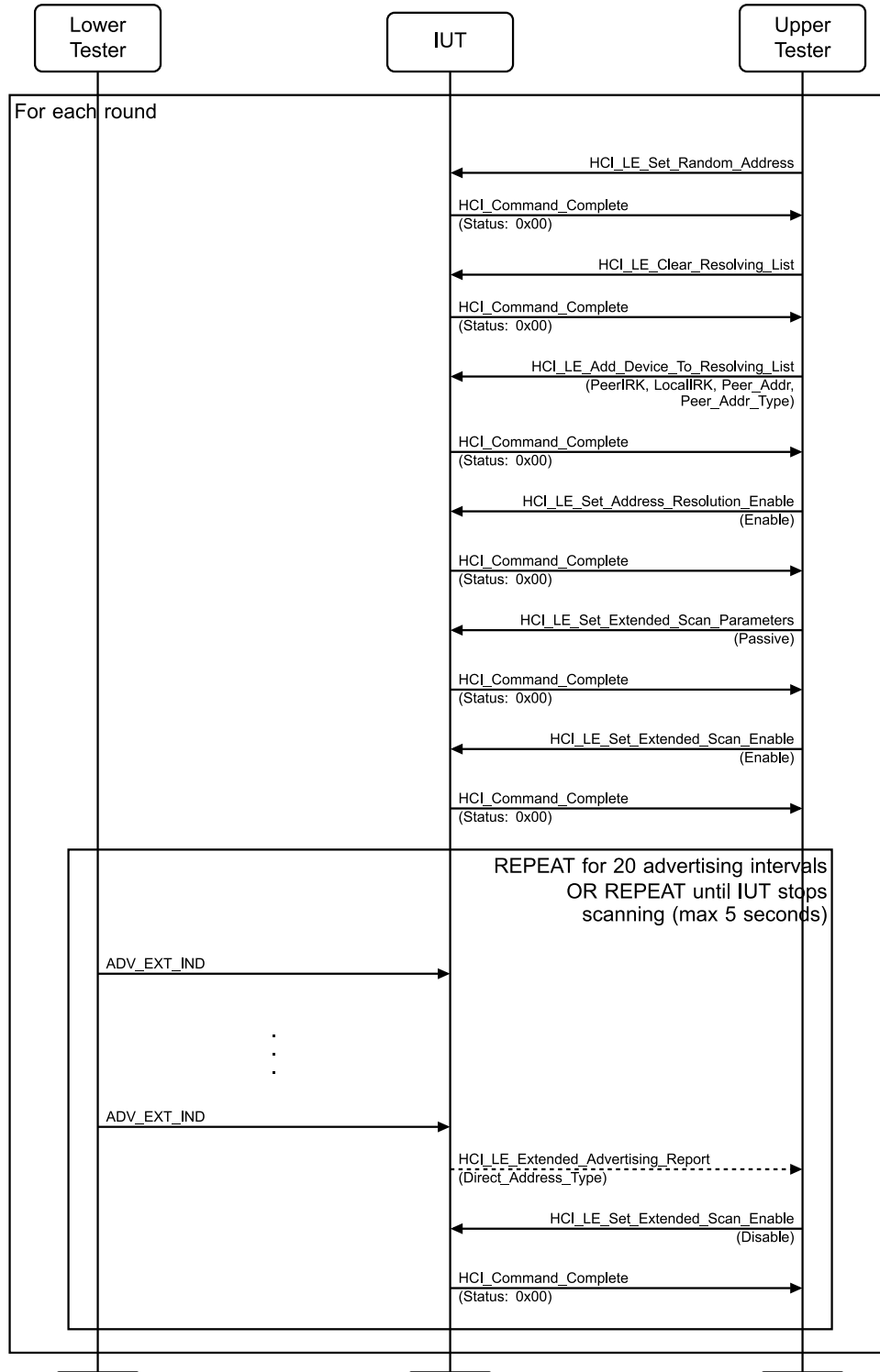
Figure 4.2-118: Extended Scanning, Passive, Scanning Filter Policy, Resolvable Private Addresses MSC
