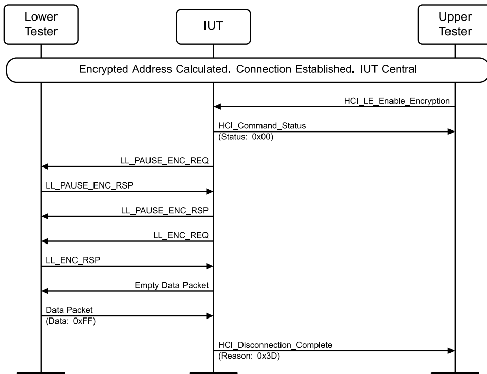
Figure 4.8-58: LL/SEC/CEN/BI-07-C [Central Pause Encryption Sending Data] MSC
