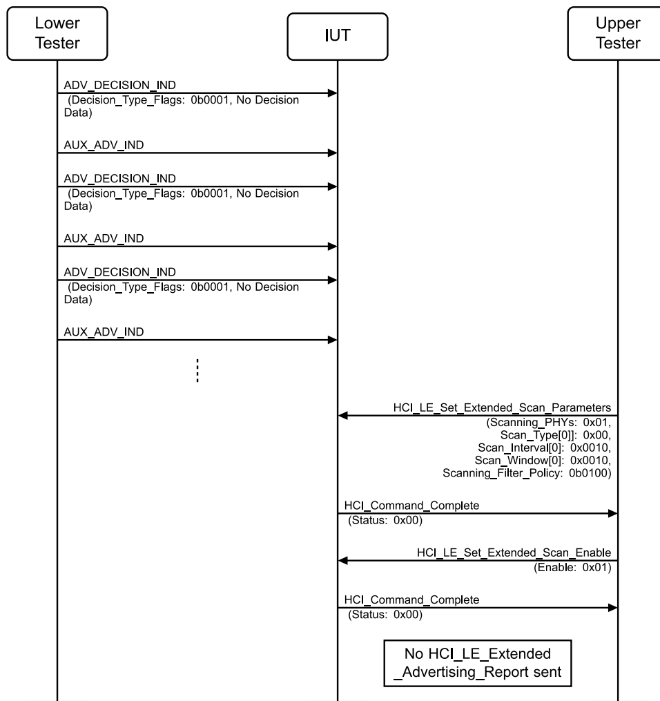
Figure 4.2-141: LL/DDI/SCN/BV-105-C [Decision-Based Advertisements Ignored, No Instructions Set] MSC
