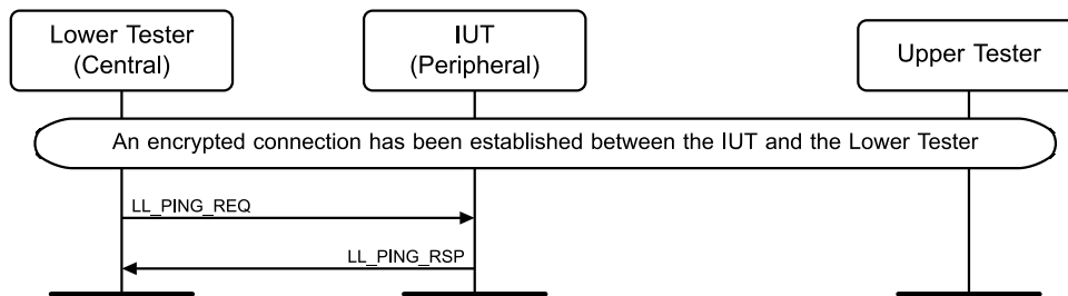
Figure 4.8-33: LL/SEC/PER/BV-07-C [Responding to LL_PING_REQ] MSC
