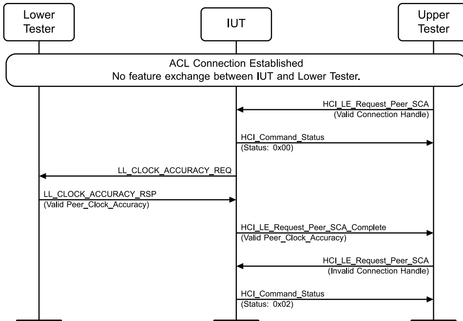
Figure 4.10-54: CIS Updating SCA MSC
