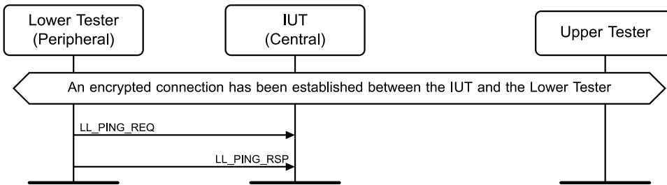
Figure 4.8-46: LL/SEC/CEN/BV-07-C [Responding to LL_PING_REQ] MSC
