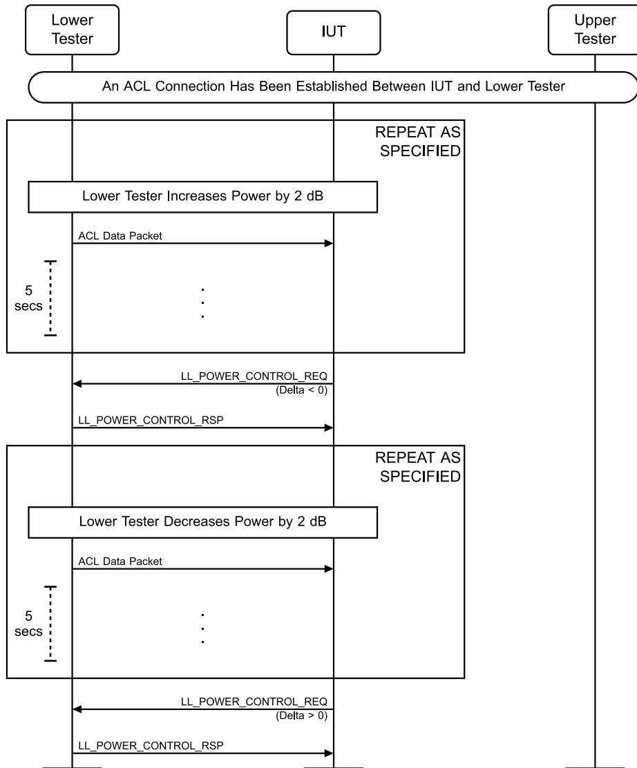
Figure 4.13-3: Power Control Request – Initiate MSC
