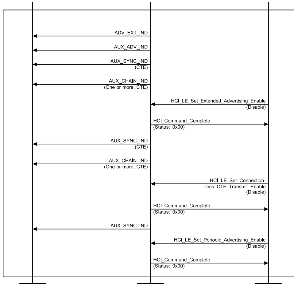
Figure 4.2-36: AoD Connectionless CTE Advertising MSC – Page 2 of 2
