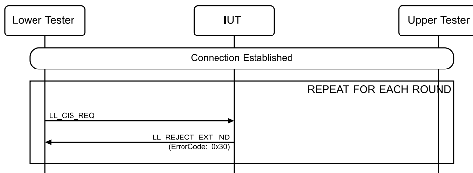
Figure 4.10-64: Reject LL_CS_REQ With Out of Range BN, FT, NSE MSC
