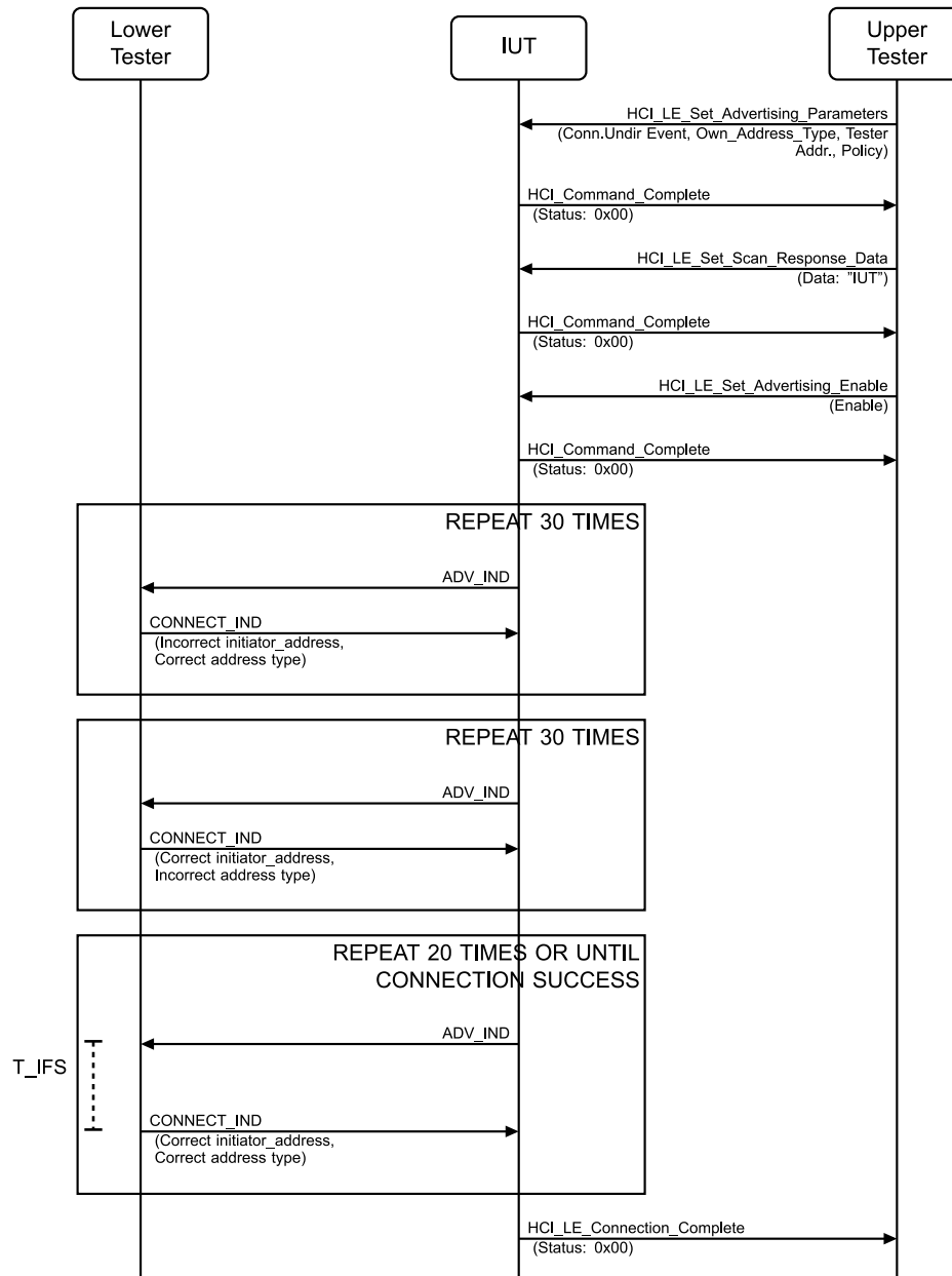
Figure 4.2-7: LL/DDI/ADV/BV-09-C [Connection Request Device Filtering, Extended Advertising not supported] MSC
