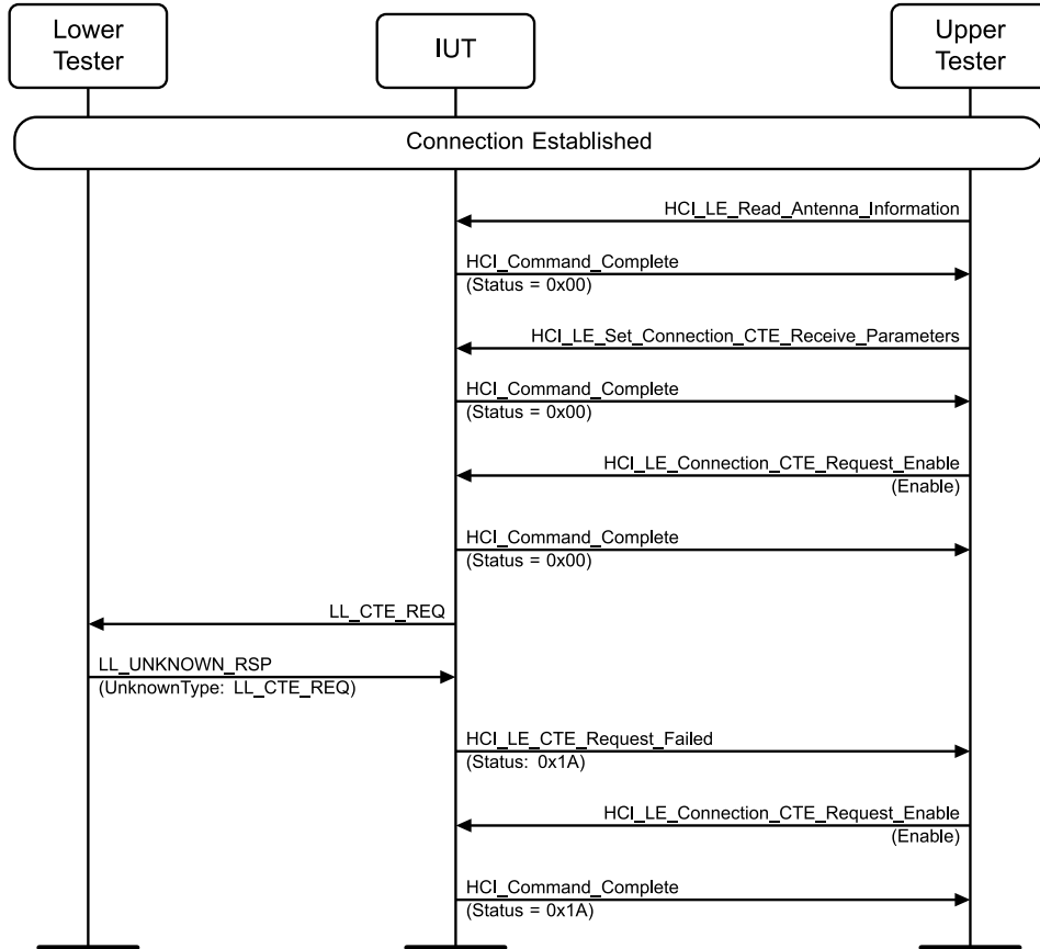
Figure 4.3-231: Constant Tone Extension Request Procedure, IUT Initiated, Unsupported MSC
