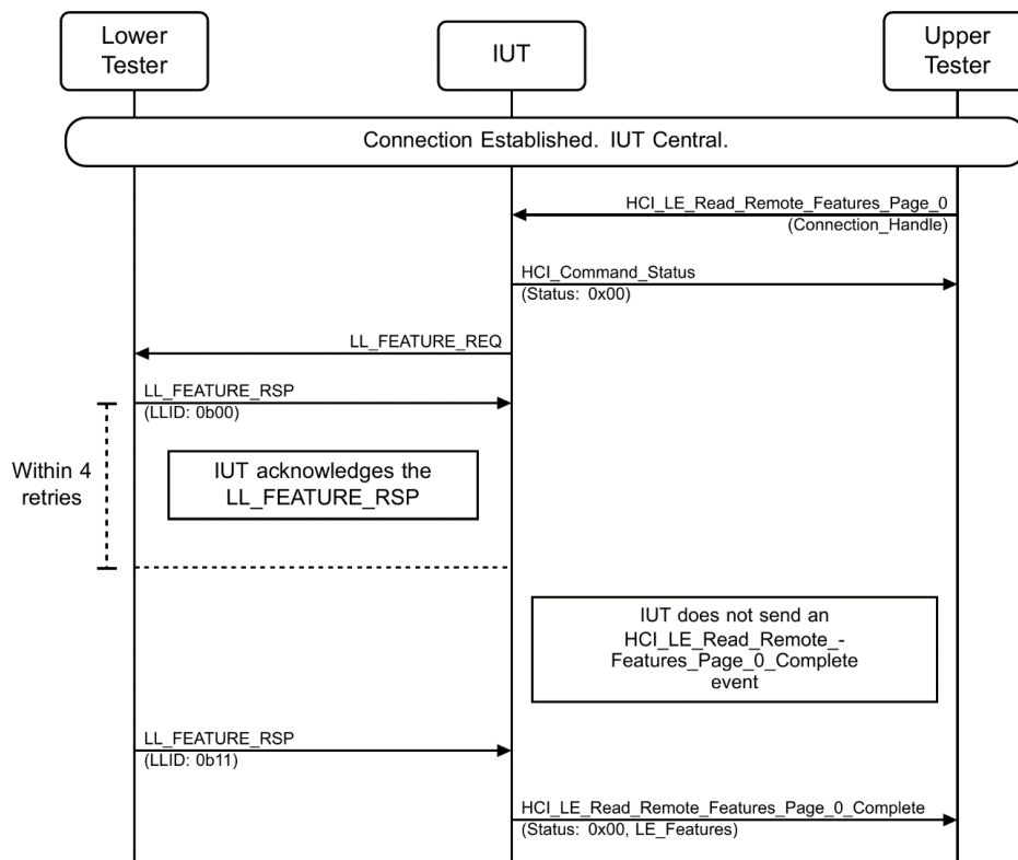
Figure 4.3-206: LL/CON/CEN/BI-14-C [Invalid LLID] MSC
