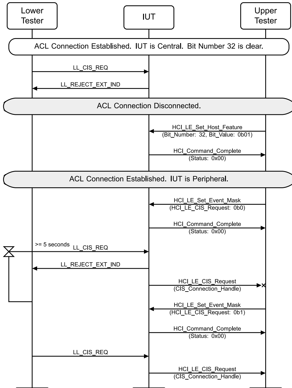
Figure 4.10-30: LL/CIS/PER/BV-22-C [CIS Request Event Not Set] MSC
