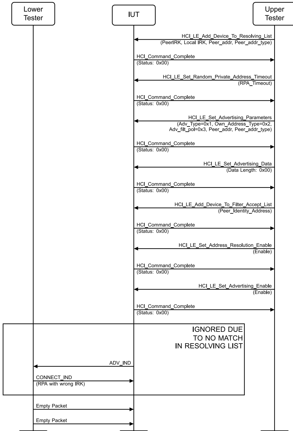
Figure 4.8-14: LL/SEC/ADV/BV-14-C [Network Privacy - Directed Connectable Advertising using Resolving List and Peer Device Identity not in the List] MSC
