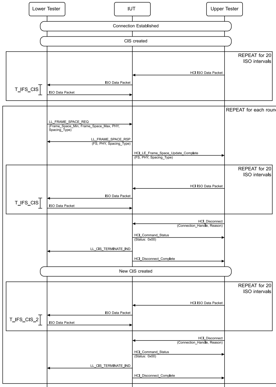
Figure 4.4-46: Respond to a Frame Space Change Request in a CIS MSC
