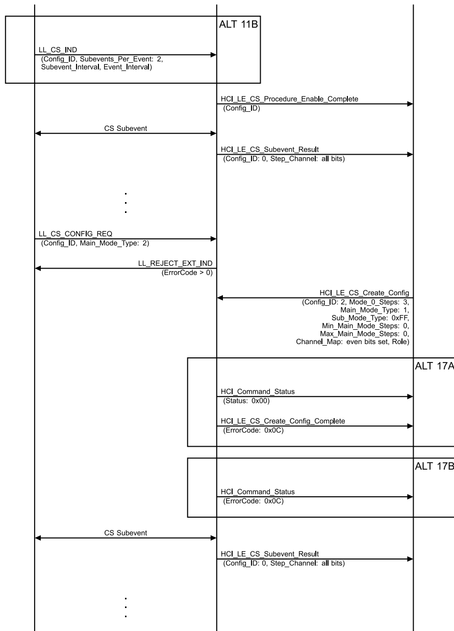
Figure 4.14-45: Reject a Config Request During an Active CS Procedure With the Same Config_ID MSC – Page 2 of 2
