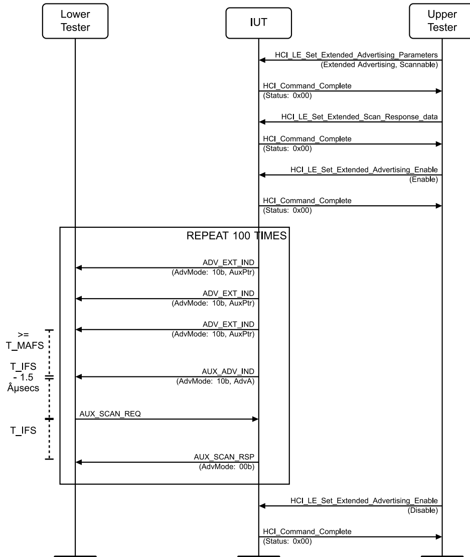
Figure 4.4-3: Extended Advertising, Secondary Channel, Latest Transmission to Advertiser MSC
