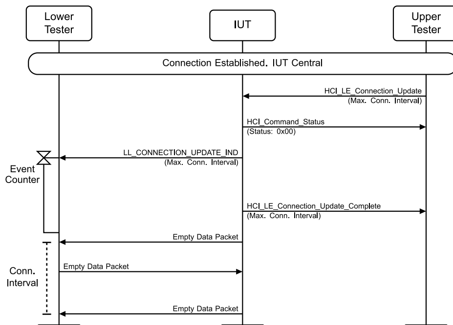
Figure 4.3-138: LL/CON/CEN/BV-07-C [Requesting parameter update] MSC
