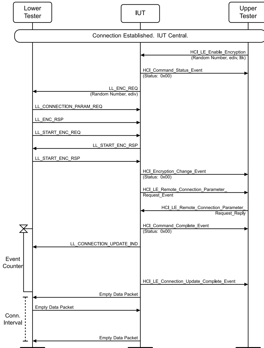
Figure 4.3-158: LL/CON/CEN/BV-28-C [Initiating Connection Parameter Request – different procedure collision – encryption] MSC
