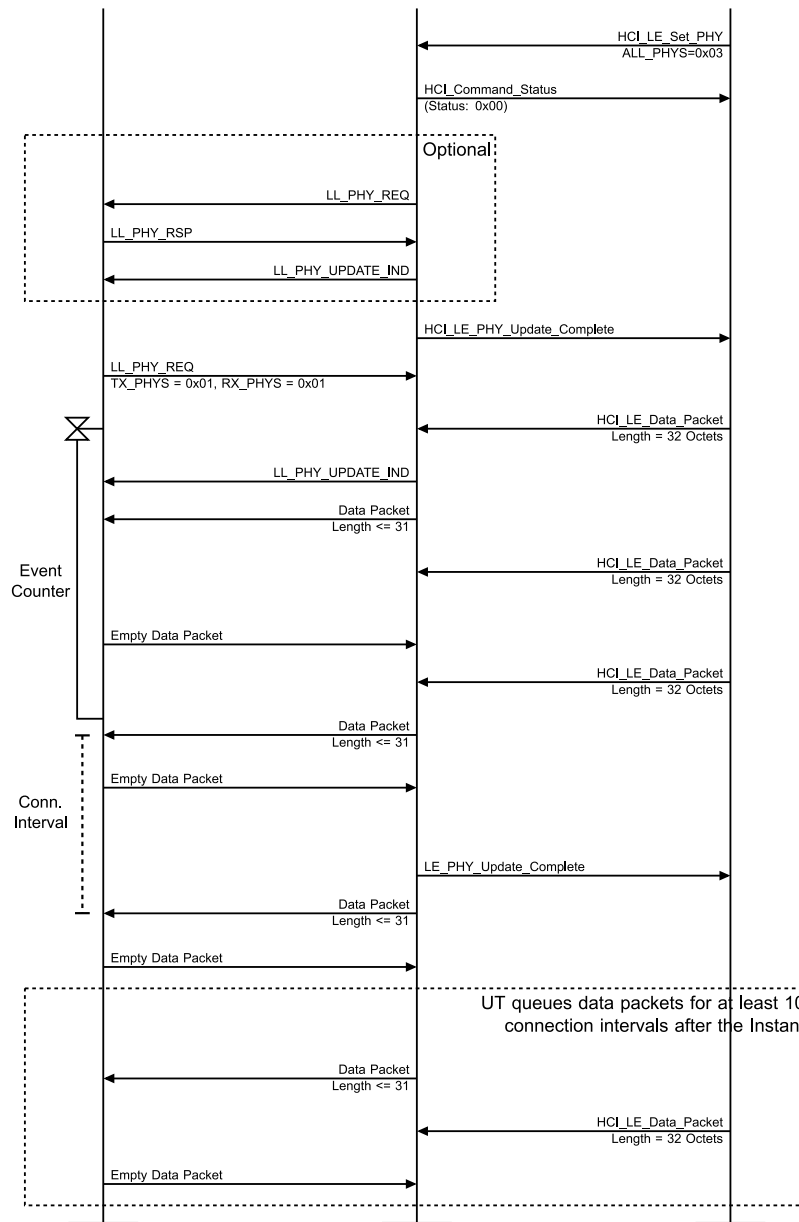
Figure 4.3-174: LL/CON/CEN/BV-50-C [Responding to PHY Update Procedure – Packet Time Restrictions] MSC – Page 2 of 2
