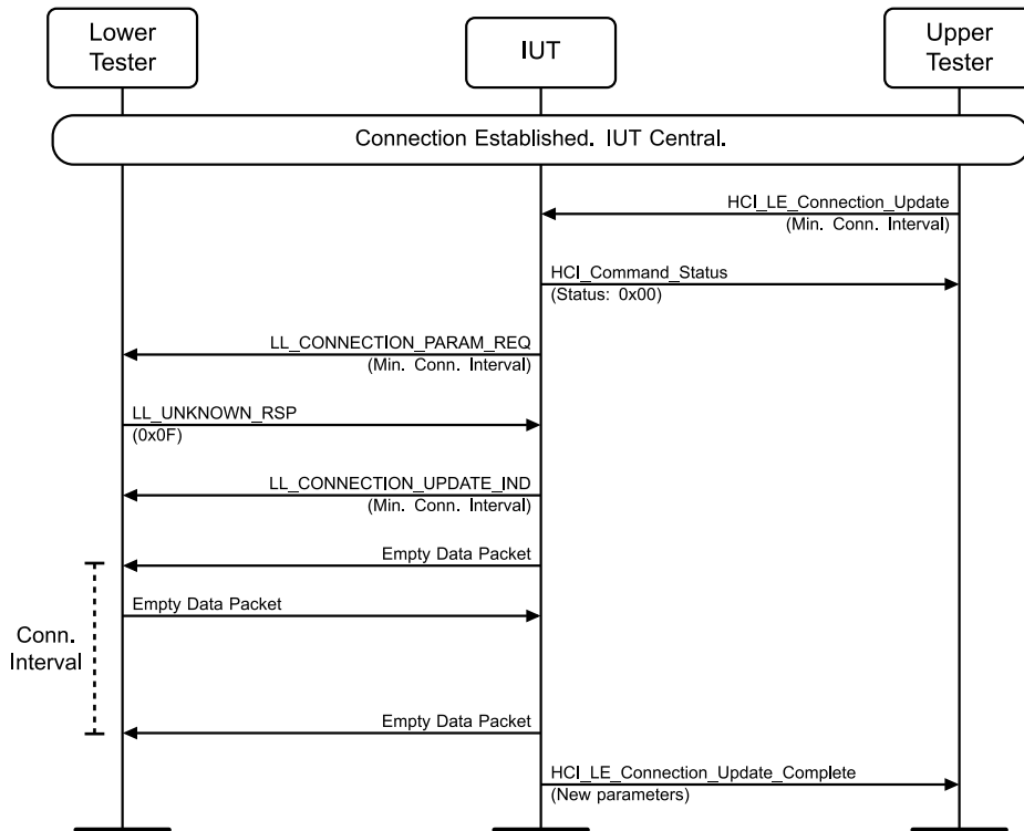
Figure 4.3-187: LL/CON/CEN/BV-81-C [Initiating Connection Parameter Request – Unsupported Without Feature Exchange] MSC
