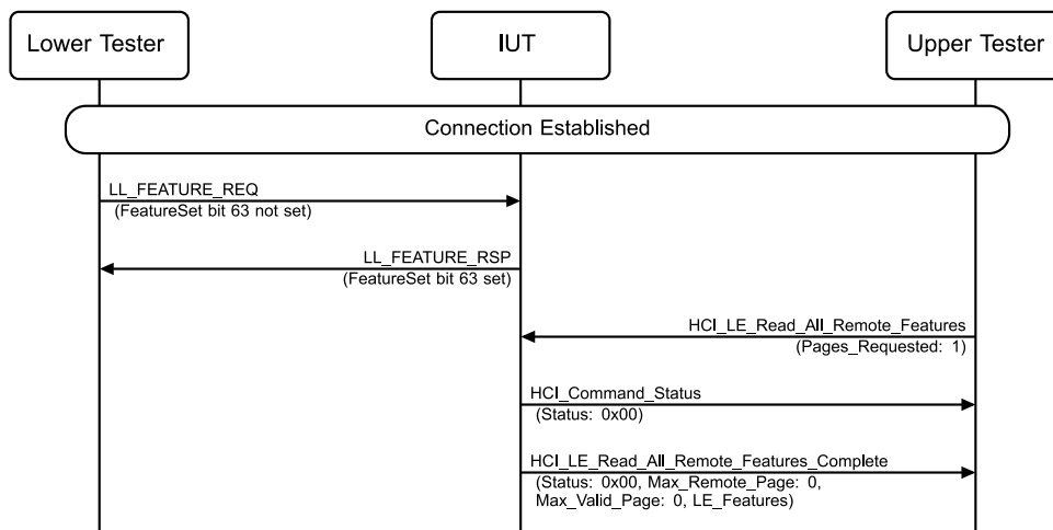
Figure 4.3-128: LL/CON/PER/BV-166-C [LL Extended Feature Set Not Supported by the Peer, Lower Tester Initiates Feature Exchange] MSC
