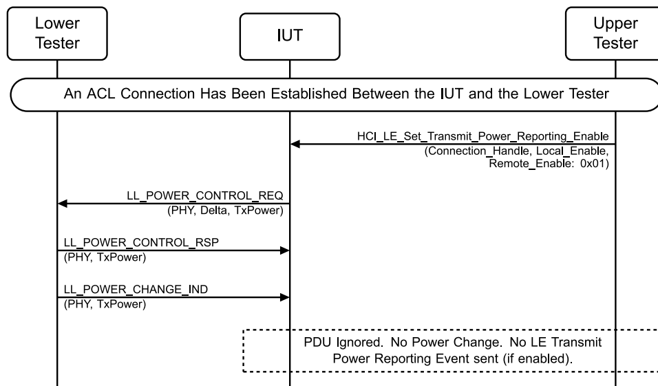
Figure 4.13-14: Power Change Request using an invalid or unsupported PHY MSC
