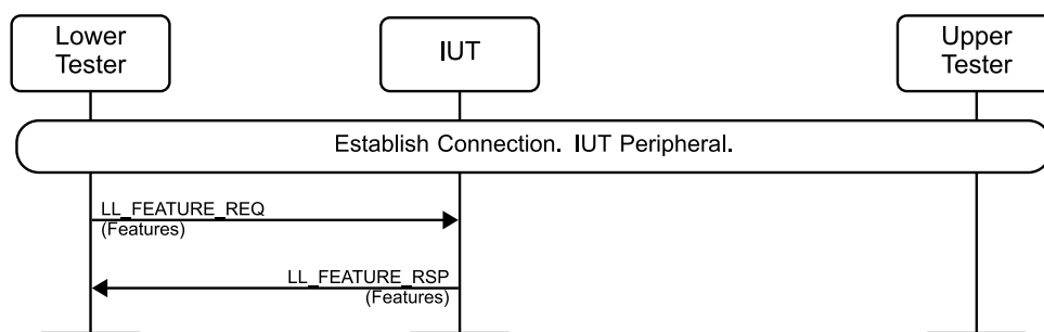
Figure 4.3-56: LL/CON/PER/BV-14-C [Feature Setup response] MSC
