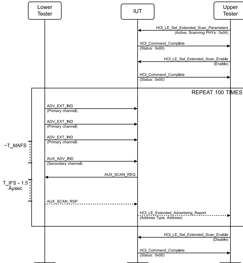
Figure 4.4-53: Extended Scanning, Secondary Channel, Earliest Transmission to Scanner, LE Coded PHY MSC
