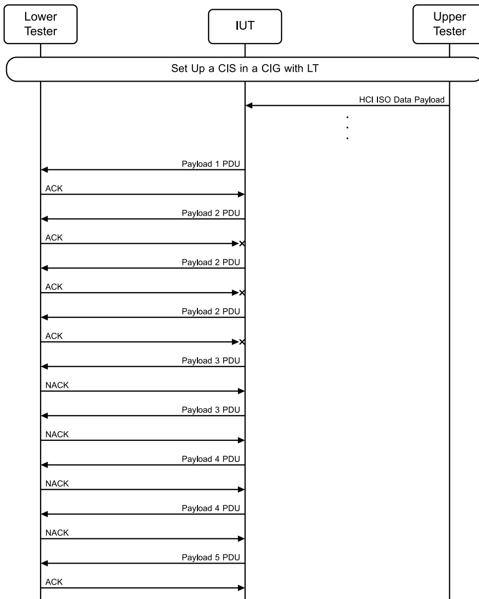
Figure 4.10-15: LL/CIS/CEN/BV-19-C [Deterministic Packet Transmission in CIS, Central] MSC
