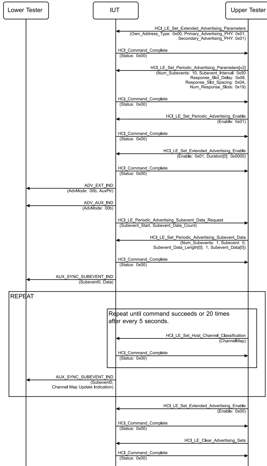
Figure 4.2-69: AUX_SYNC_SUBEVENT_IND PDU with Channel Map Update Indication MSC
