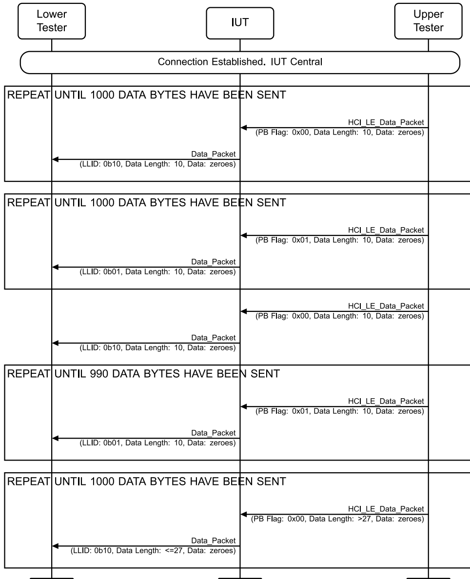
Figure 4.3-135: LL/CON/CEN/BV-03-C [Central Sending Data] MSC
