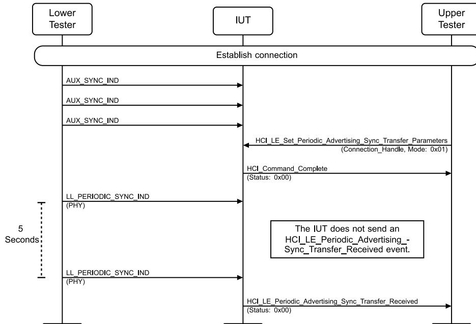
Figure 4.3-258: Periodic Advertising Sync Transfer Procedure, Invalid or Unsupported PHY MSC
