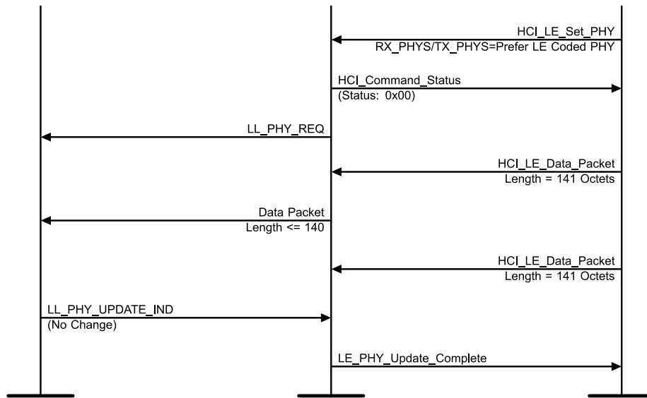
Figure 4.3-100: LL/CON/PER/BV-58-C [Initiating PHY Update Procedure – Packet Time Restrictions, No Change, LE Coded] MSC – Page 2 of 2
