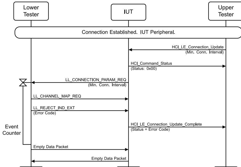
Figure 4.3-69: LL/CON/PER/BV-27-C [Initiating Connection Parameter Request – different procedure collision – channel map update] MSC
