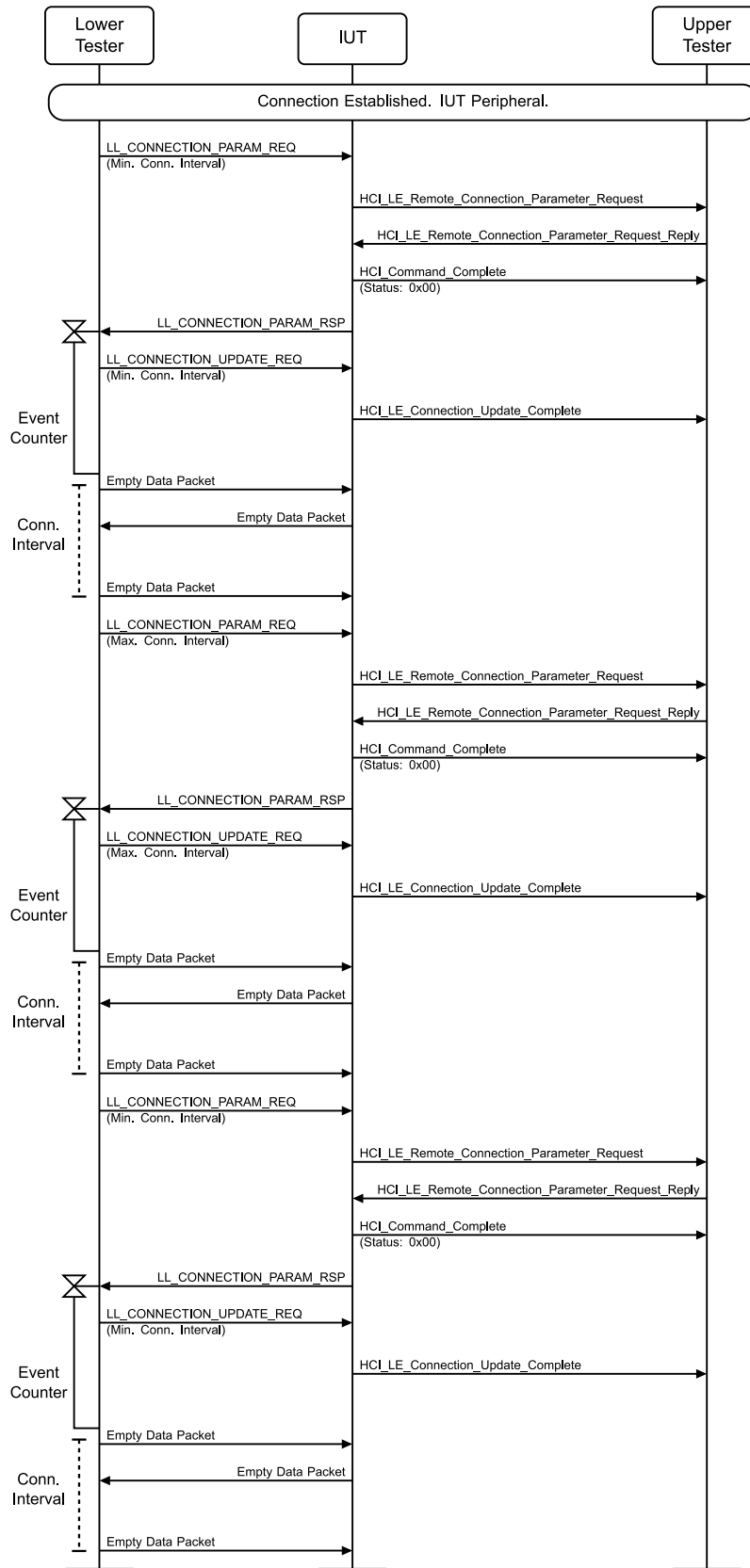
Figure 4.3-71: LL/CON/PER/BV-29-C [Accepting Connection Parameter Request – no Preferred_Periodicity] MSC
