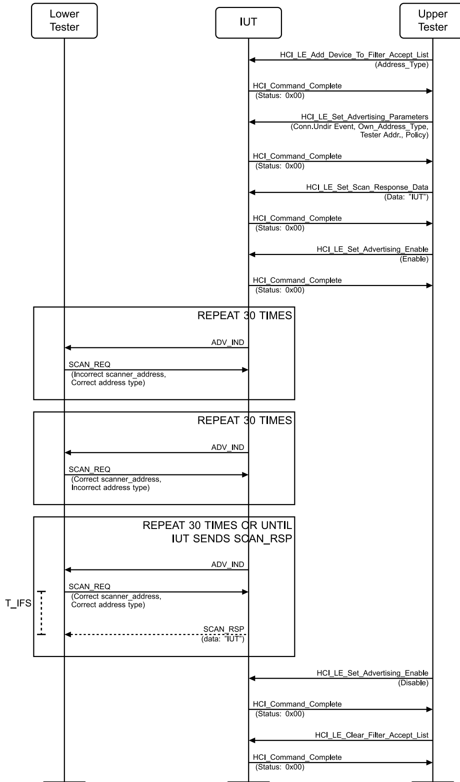
Figure 4.2-6: LL/DDI/ADV/BV-08-C [Scan Request Device filtering] MSC
