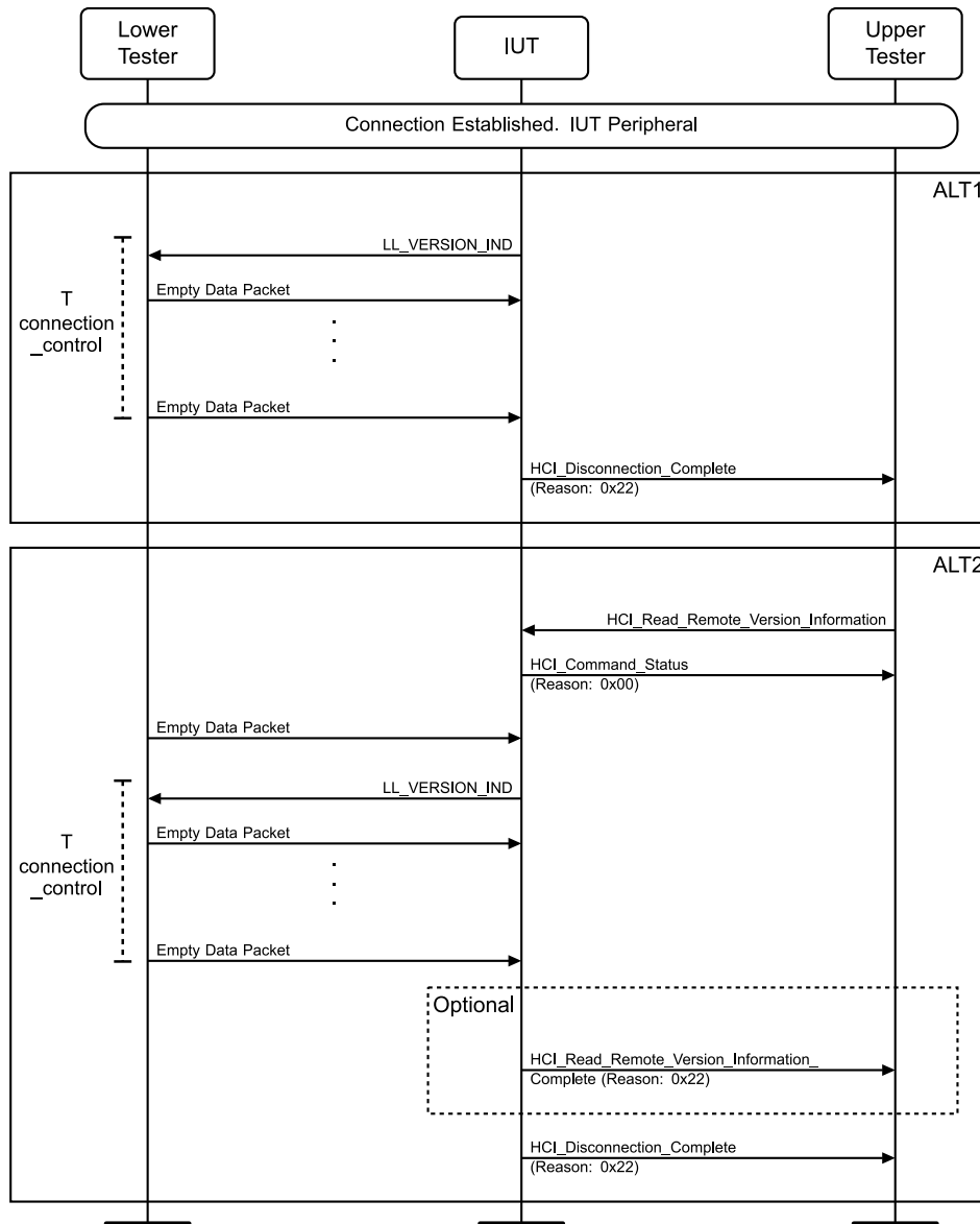
Figure 4.3-108: LL/CON/PER/BI-05-C [Peripheral Connection Control Timer] MSC
