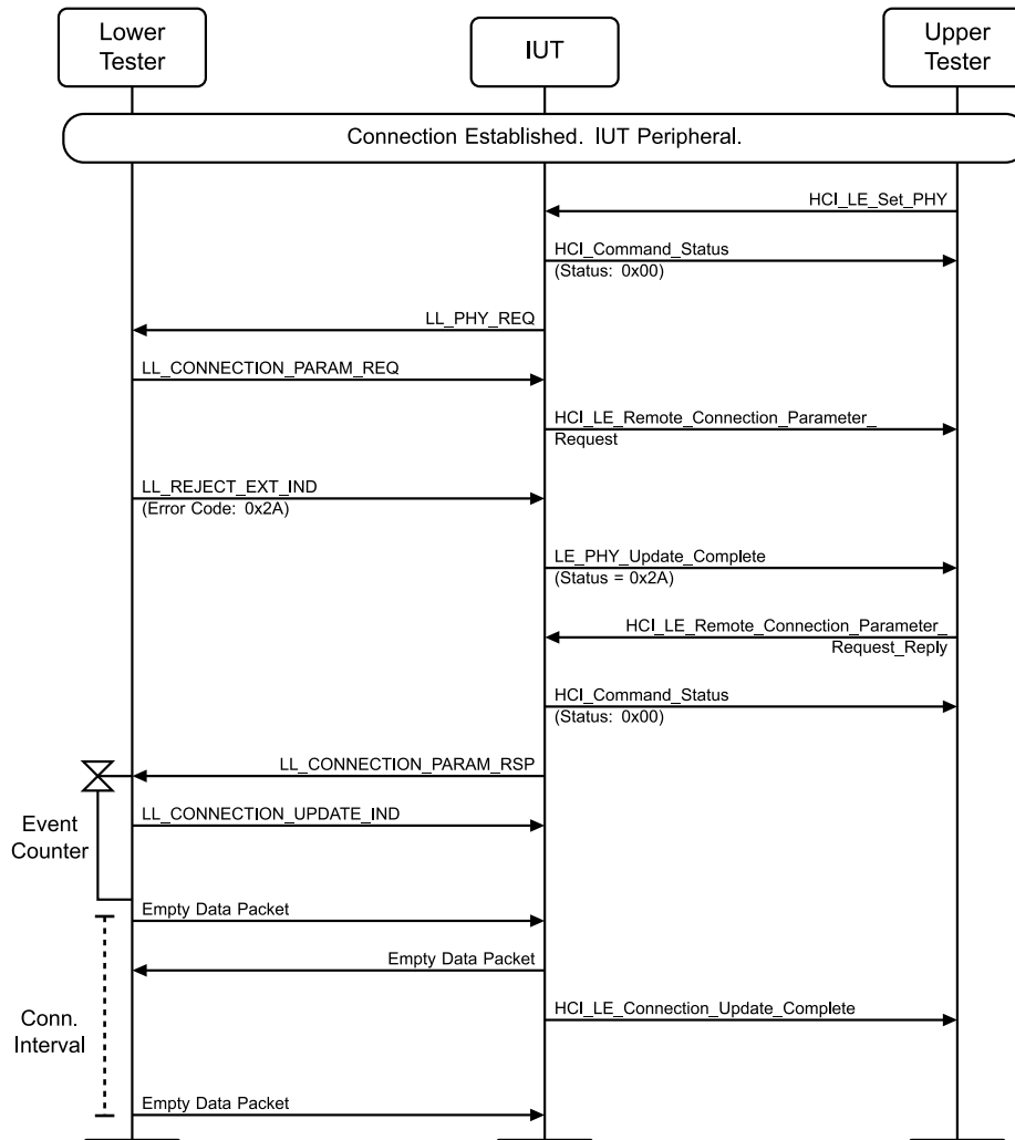
Figure 4.3-81: LL/CON/PER/BV-47-C [Handling Protocol Collision – Different Procedure – Connection Parameters] MSC
