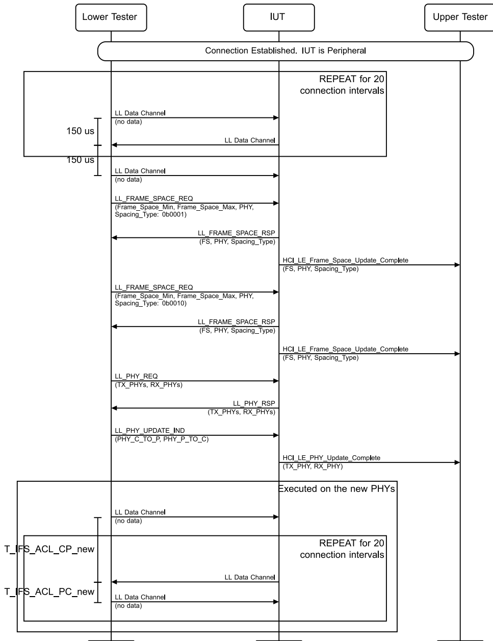
Figure 4.4-24: Respond to Inter Frame Space Change Request on a Different Asymmetric PHY for TX and RX, Peripheral MSC
