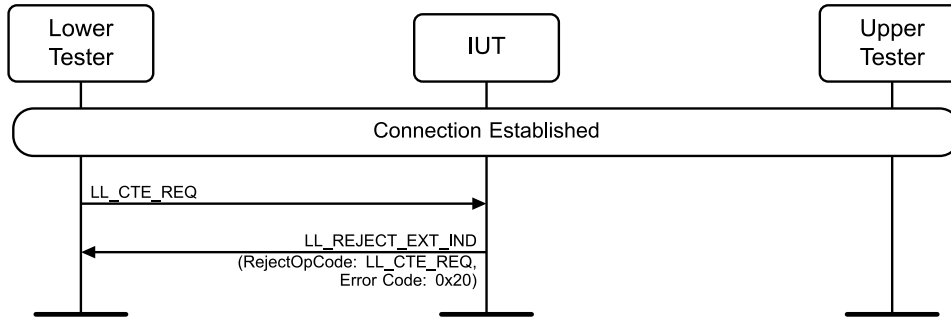
Figure 4.3-238: Constant Tone Extension Request Procedure, IUT Responding, Responses Disabled MSC
