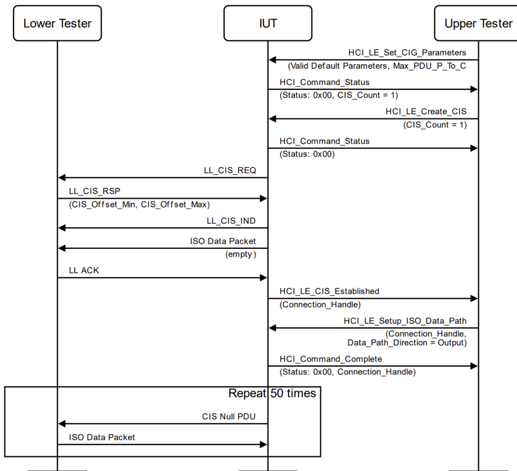
Figure 4.10-8: Connected Isochronous Stream Using Non-Test Command, Central Initiated – MSC Page 2 of 2
