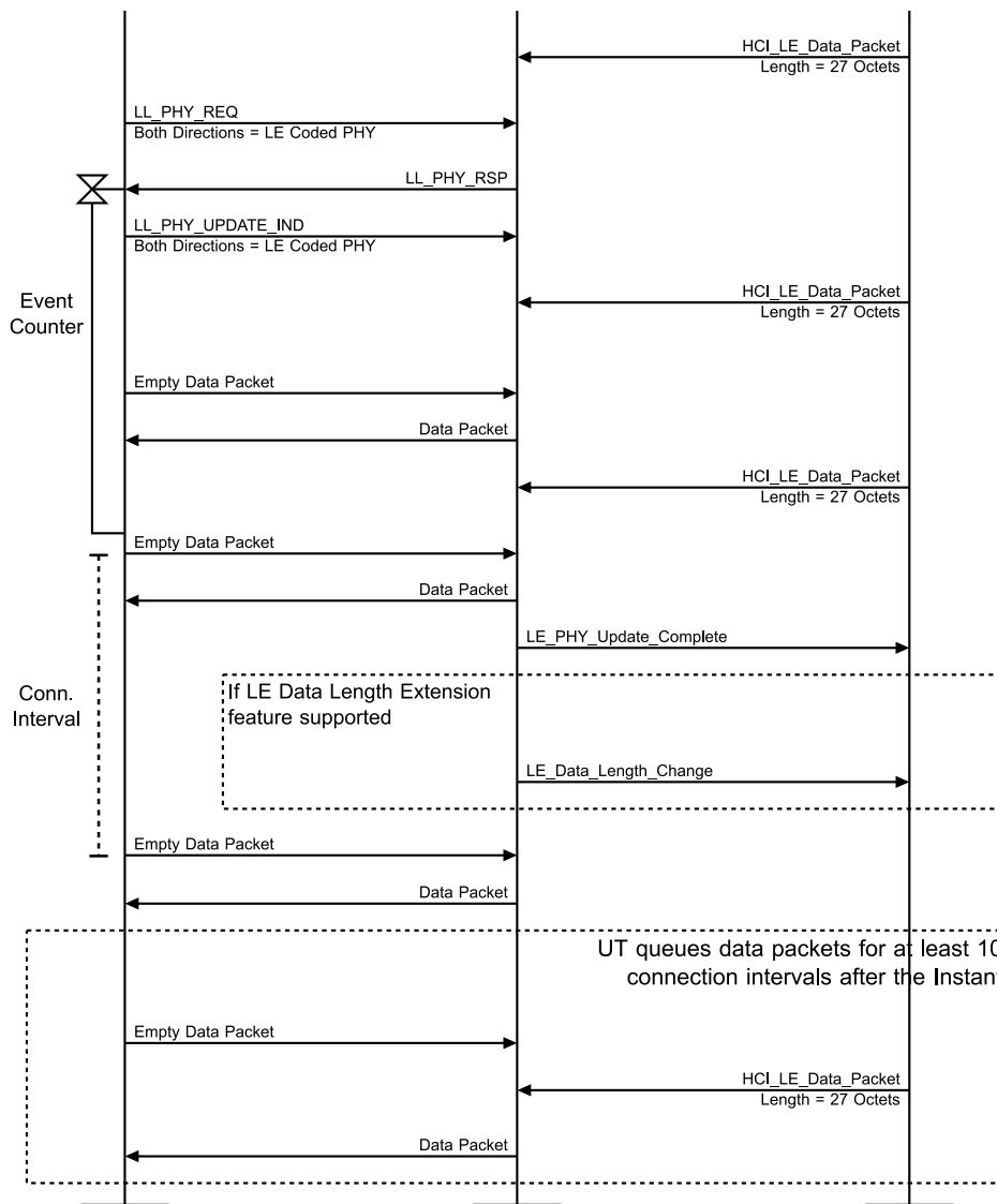
Figure 4.3-182: LL/CON/CEN/BV-55-C [Mandatory Minimum PDU Length, LE Coded] MSC – Page 2 of 2
