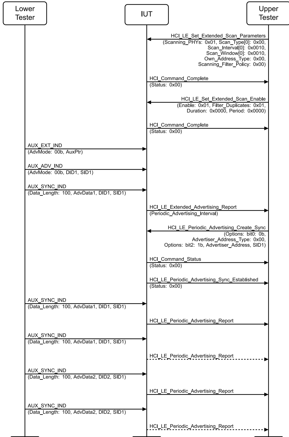
Figure 4.2-114: LL/DDI/SCN/BV-69-C [Scanner supporting Periodic Advertising Filtering accepts AUX_SYNC_IND with ADI] MSC
