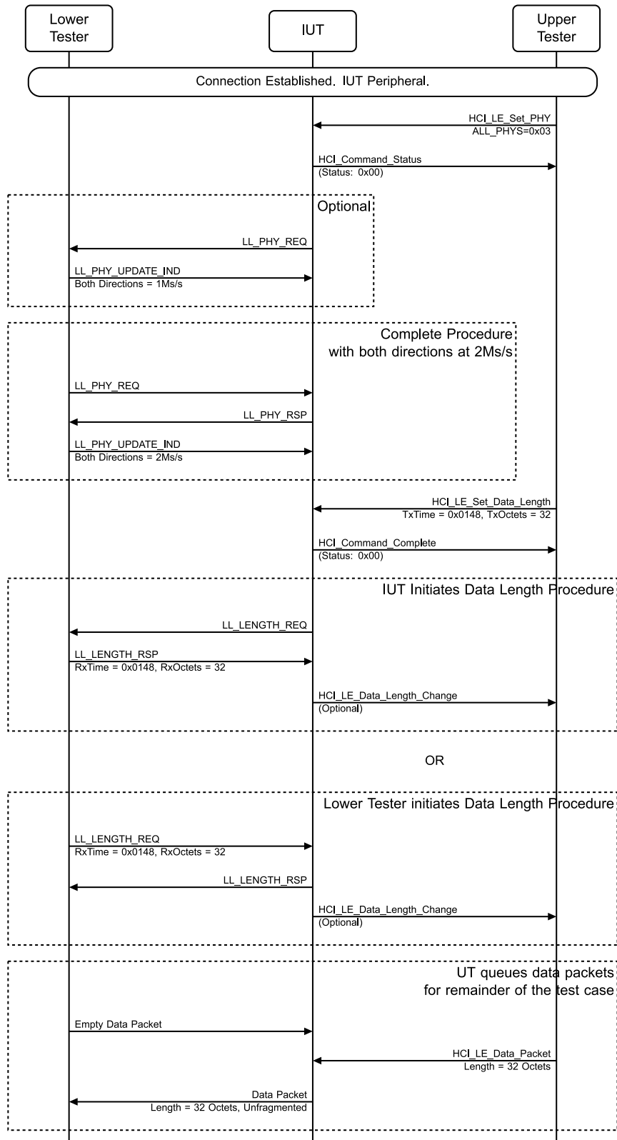
Figure 4.3-88: LL/CON/PER/BV-52-C [Initiating PHY Update Procedure – Packet Time Restrictions, No Change] MSC – Page 1 of 2
