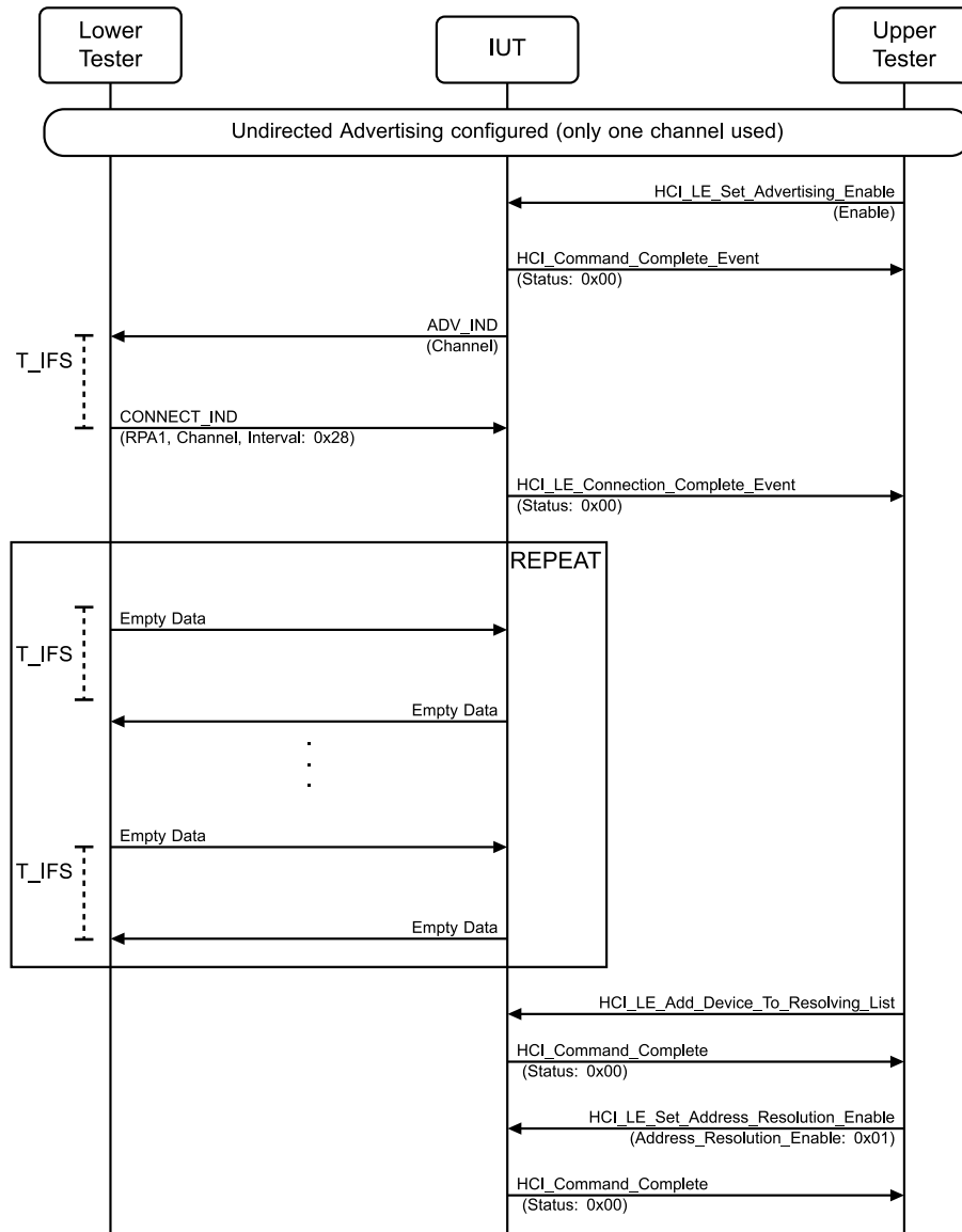
Figure 4.8-23: LL/SEC/ADV/BI-01-C [Reject Existing Connection Request, Different Peer RPA] MSC – Page 1 of 2
