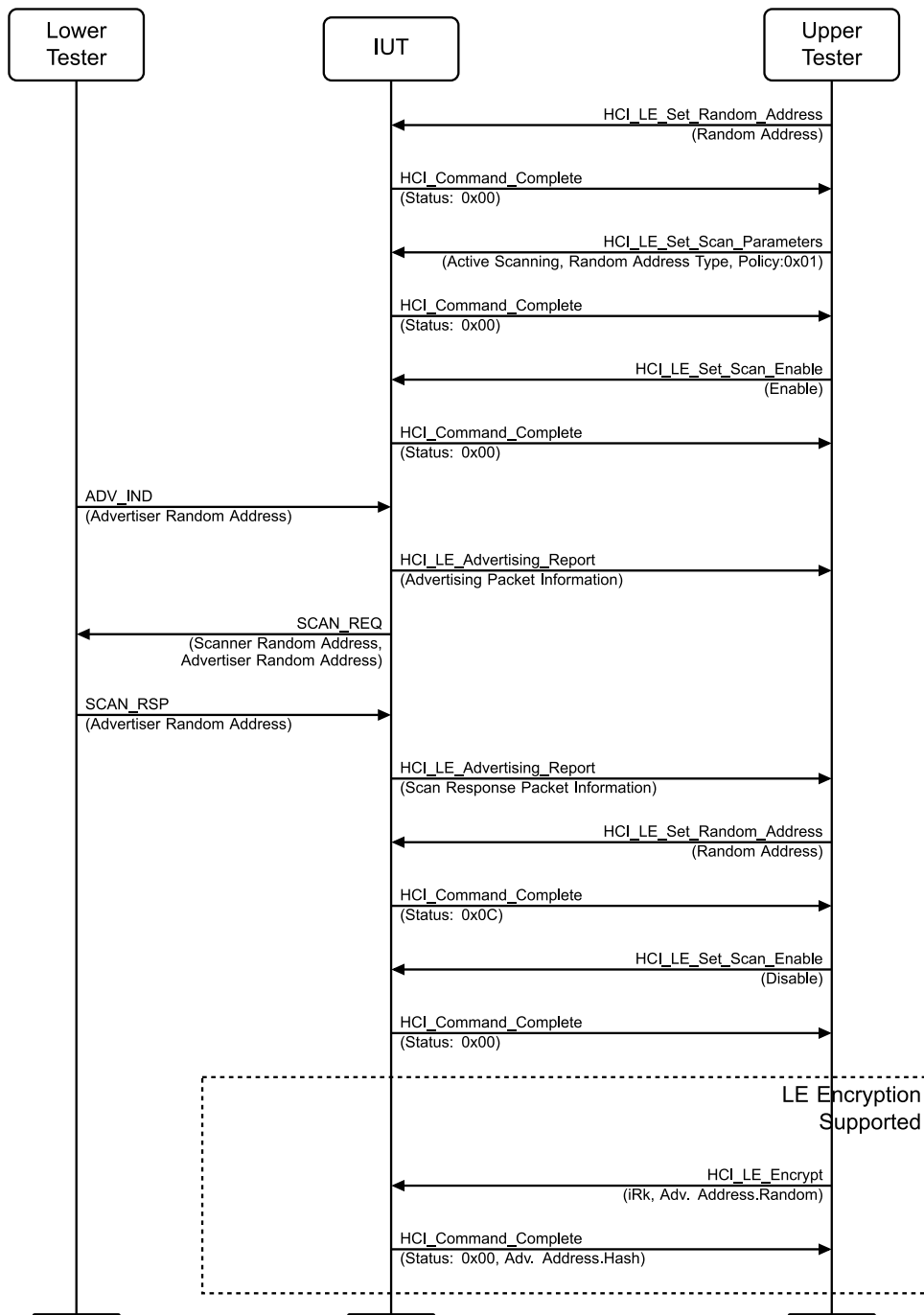
Figure 4.8-25: LL/SEC/SCN/BV-01-C [Random Address Scanning] MSC
