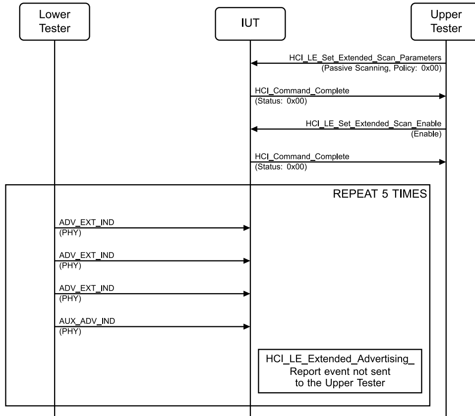
Figure 4.2-120: Passive Scanning, Invalid or Unsupported PHY MSC
