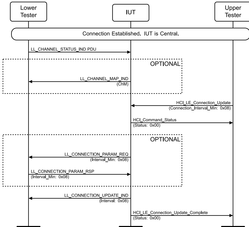
Figure 4.6-8: LL/FRH/CEN/BI-01-C [Channel Classification Disabled, Ignore Channel Classification PDU] MSC
