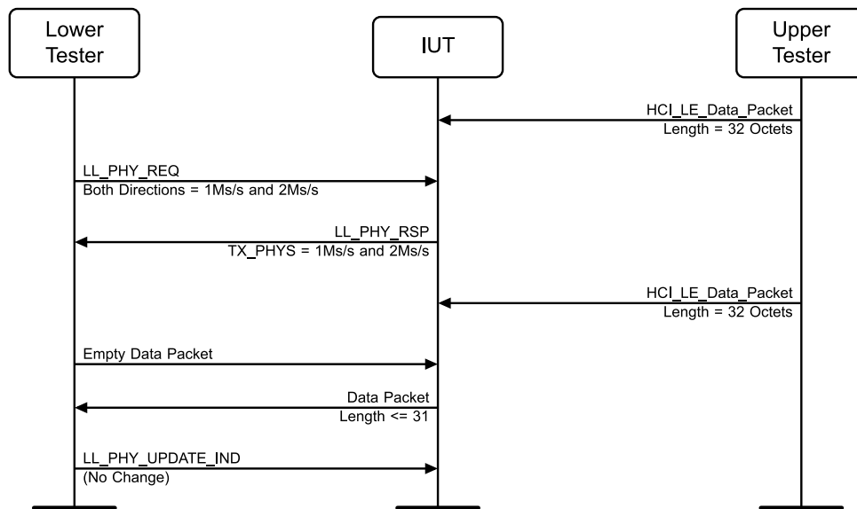
Figure 4.3-91: LL/CON/PER/BV-53-C [Responding to PHY Update Procedure – Packet Time Restrictions, No Change] MSC – Page 2 of 2
