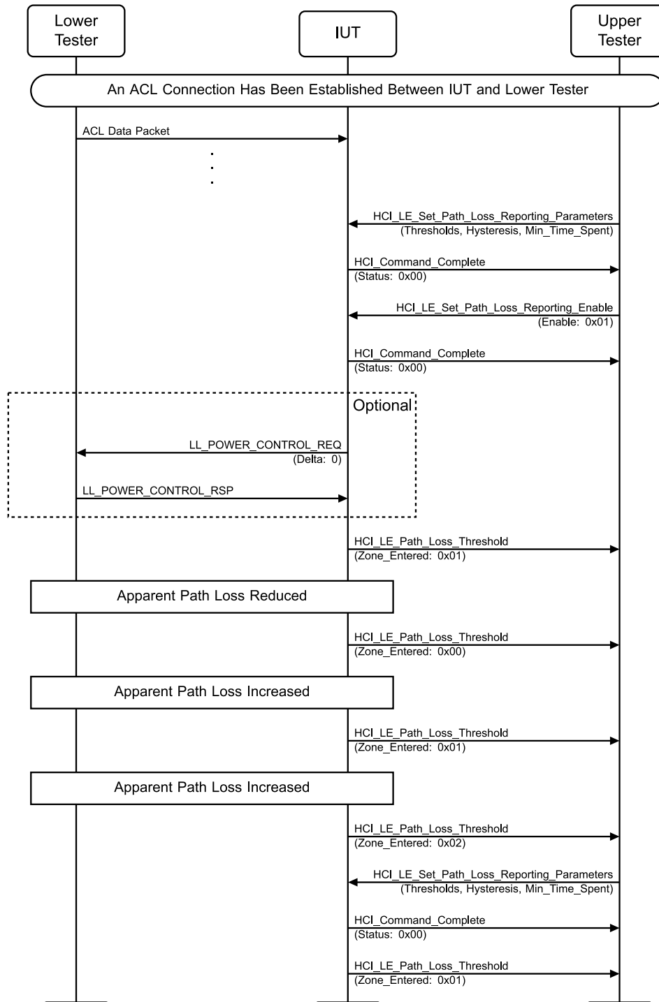
Figure 4.13-2: Path Loss Monitoring MSC
