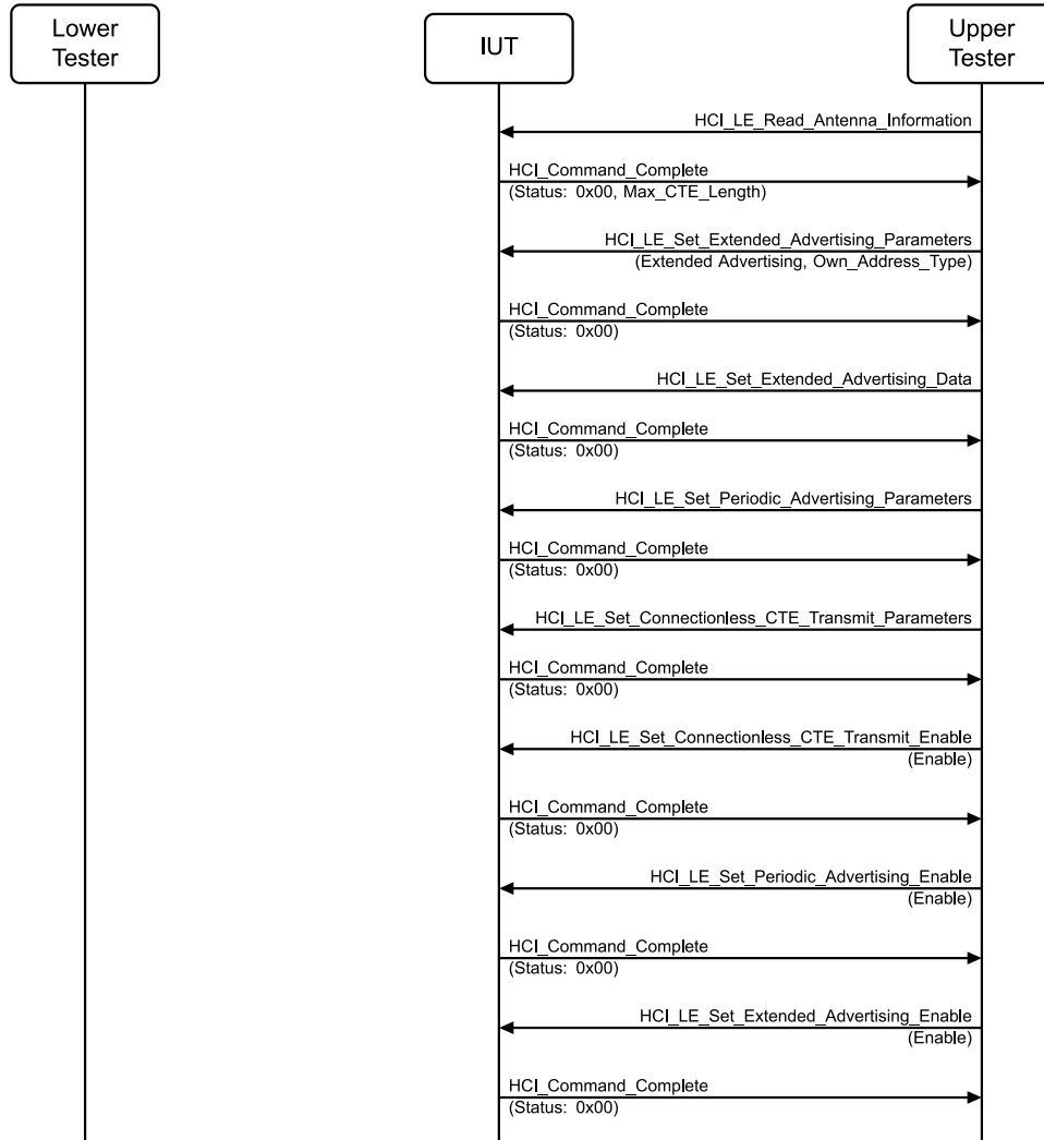
Figure 4.2-39: LL/DDI/ADV/BV-39-C [Connectionless CTE Advertising - Maintain CTE Configuration] MSC – Page 1 of 2
