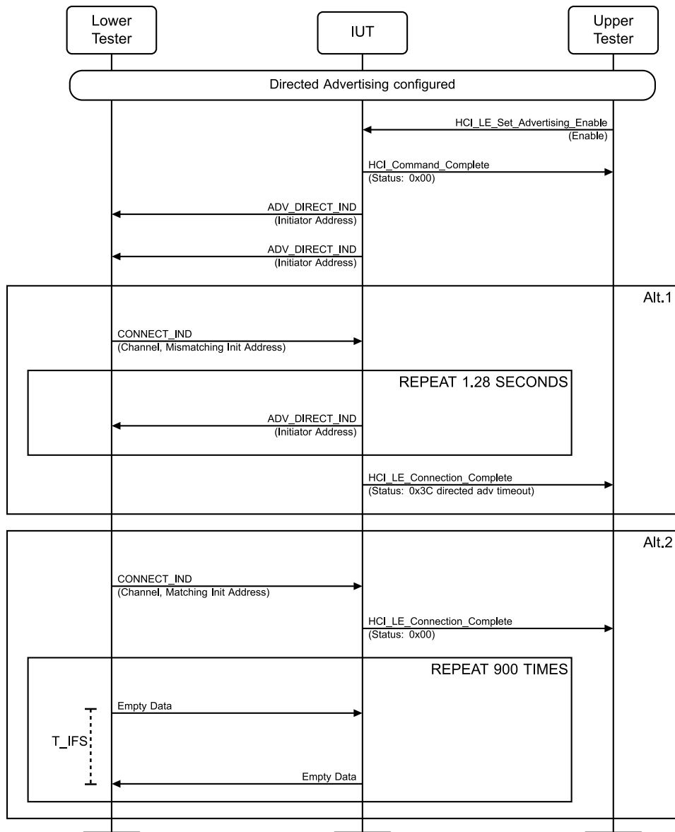
Figure 4.3-4: LL/CON/ADV/BV-04-C [Directed Advertising Connection] MSC
