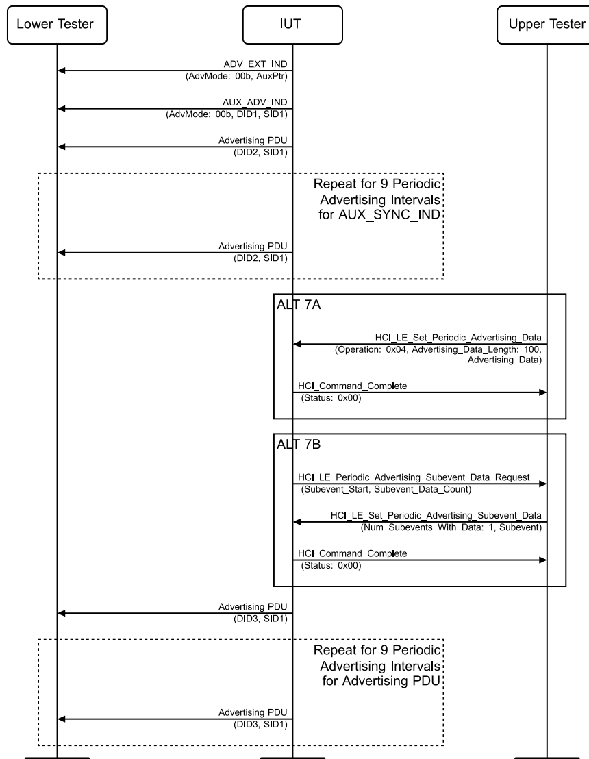
Figure 4.2-47: ADI in Periodic Advertising when supporting Periodic Advertising Filtering MSC – Page 2 of 2
