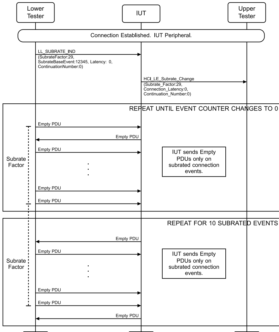
Figure 4.3-116: LL/CON/PER/BV-140-C [Subrate Factor, Event Counter Wrapping] MSC
