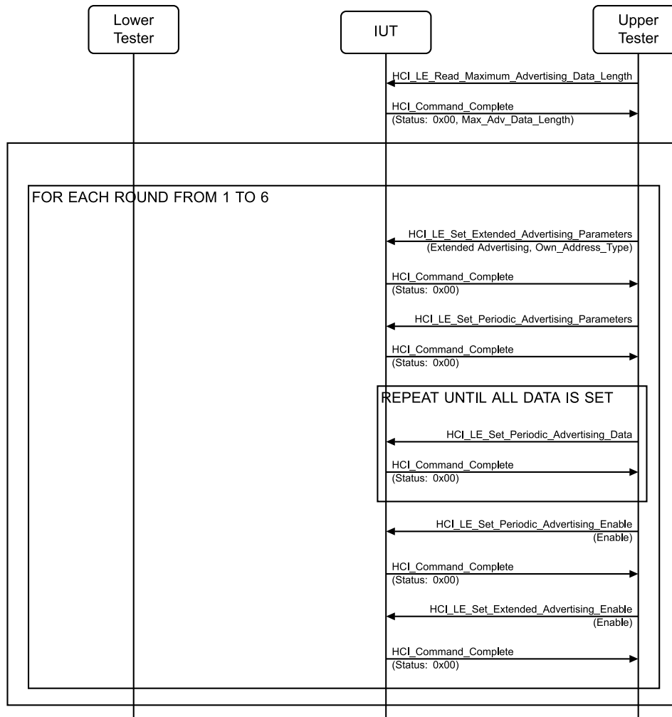
Figure 4.2-21: Extended Advertising, Periodic Advertising MSC – Page 1 of 2
