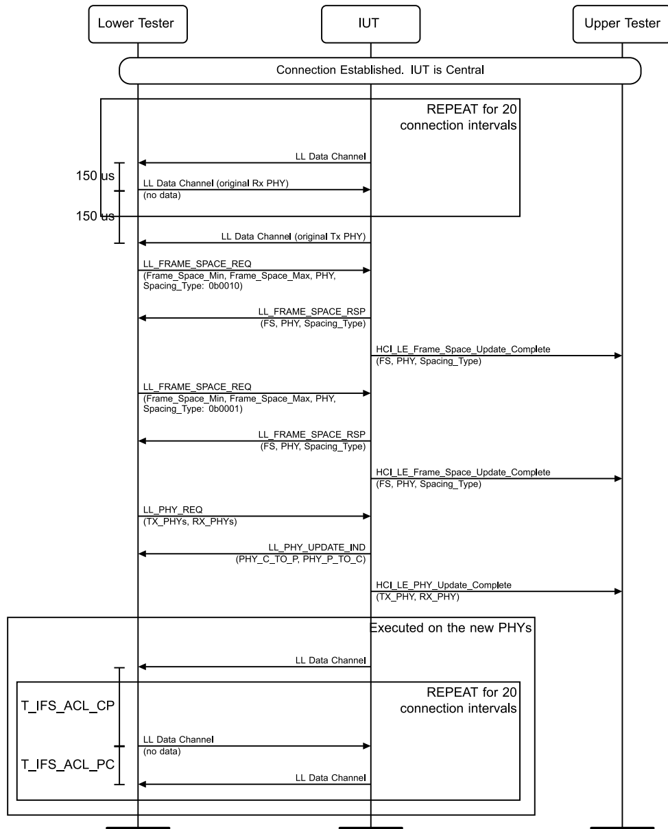
Figure 4.4-42: Respond to Inter Frame Space Change Request on a Different Asymmetric PHY for TX and RX, Central MSC
