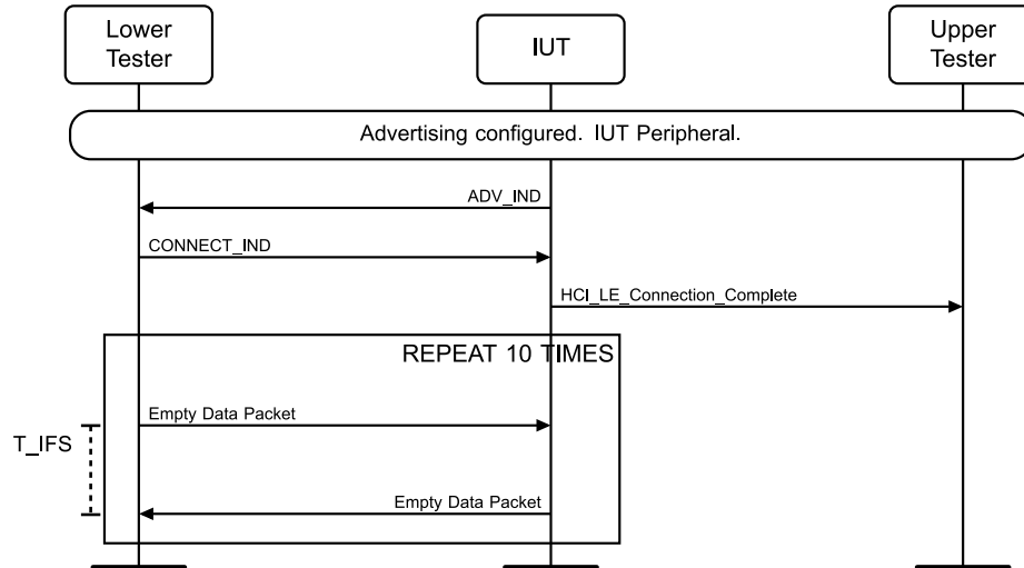
Figure 4.4-5: Earliest/Latest Transmission Start to Peripheral MSC
