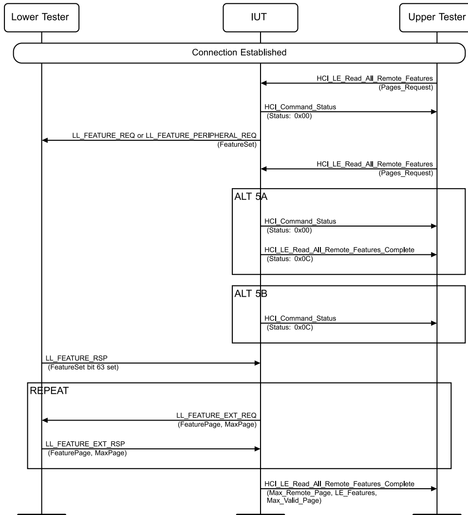
Figure 4.3-263: LL Extended Feature Set Request MSC
