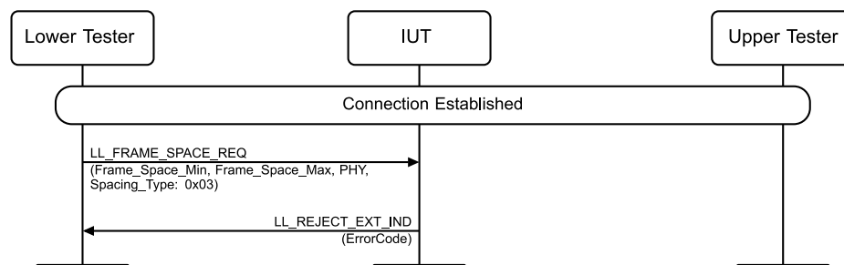
Figure 4.4-50: Frame Space Change, PHY not supported MSC
