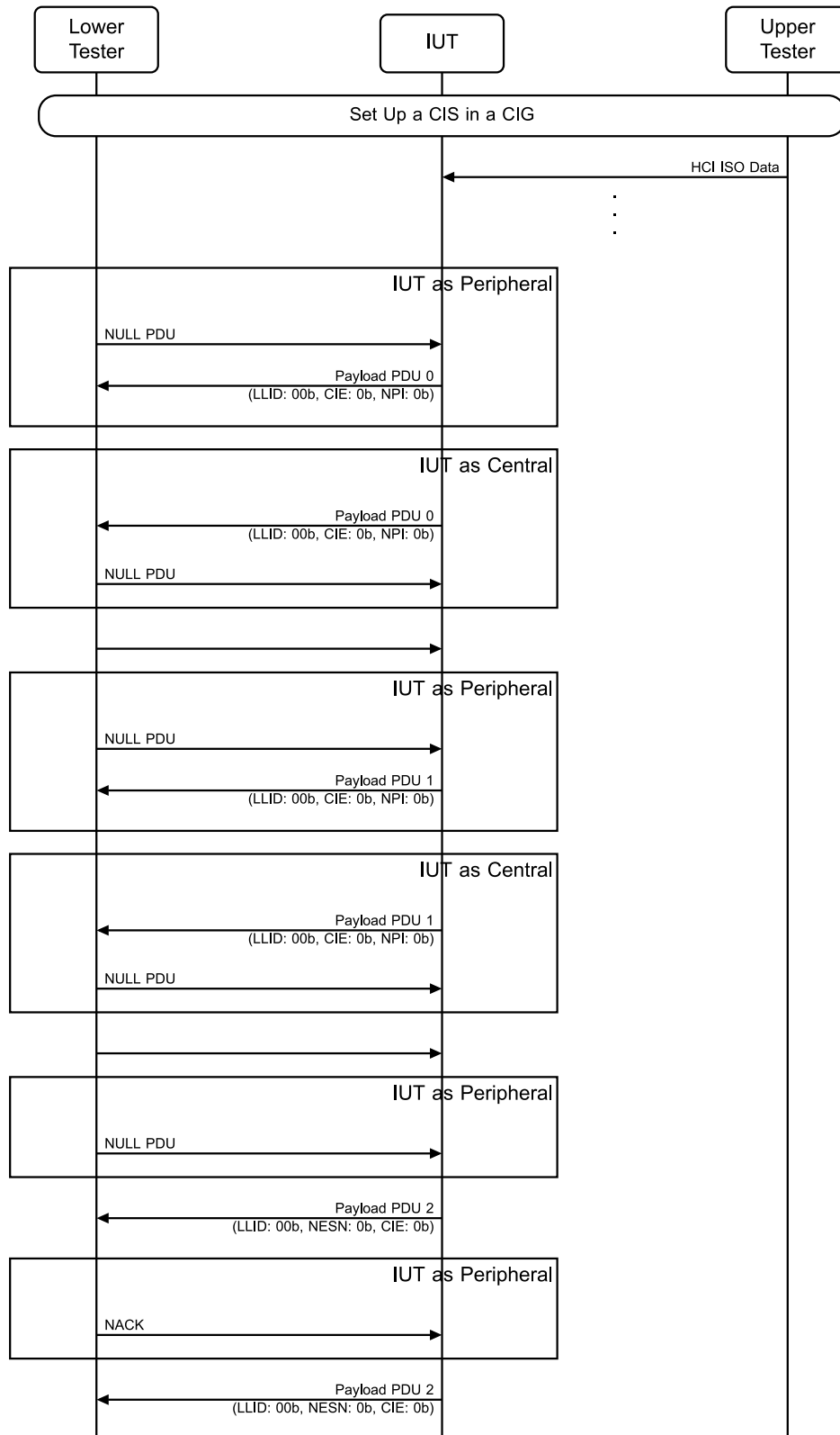
Figure 4.10-48: Sending data in Unidirectional CIS MSC
