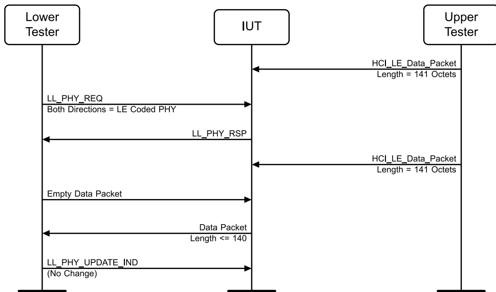
Figure 4.3-102: LL/CON/PER/BV-59-C [Responding to PHY Update Procedure – Packet Time Restrictions, No Change, LE Coded] MSC – Page 2 of 2
