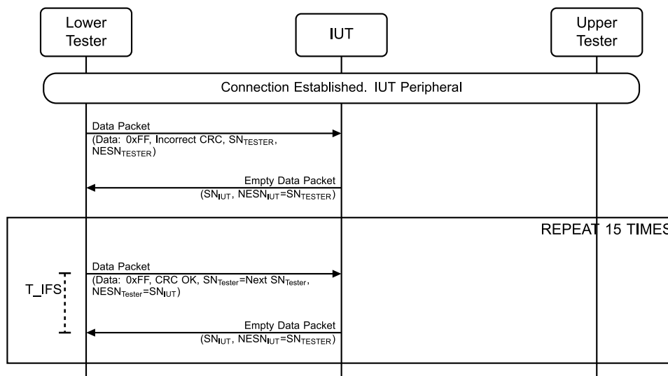
Figure 4.3-60: LL/CON/PER/BV-18-C [Peripheral lost negative acknowledgement] MSC
