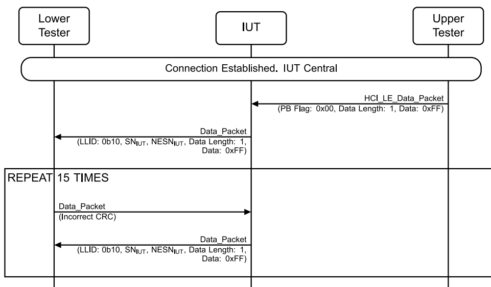
Figure 4.3-143: LL/CON/CEN/BV-14-C [Central Retransmission Request] MSC
