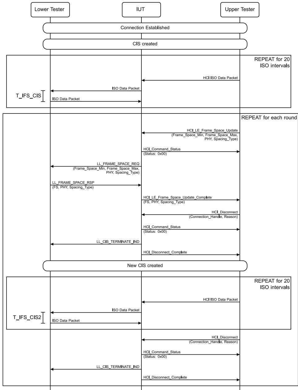
Figure 4.4-45: Initiate a Frame Space Change in a CIS MSC
