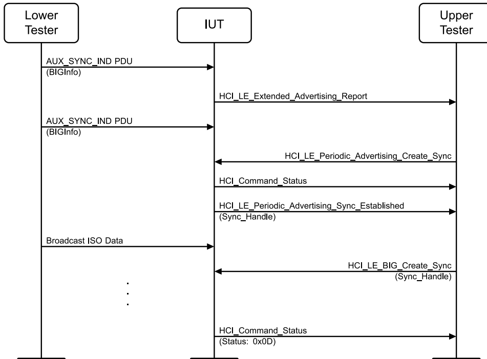
Figure 4.11-22: LL/BIS/SNC/BV-12-C [Broadcast Isochronous Stream Synchronization, Number of BISes Not Supported] MSC
