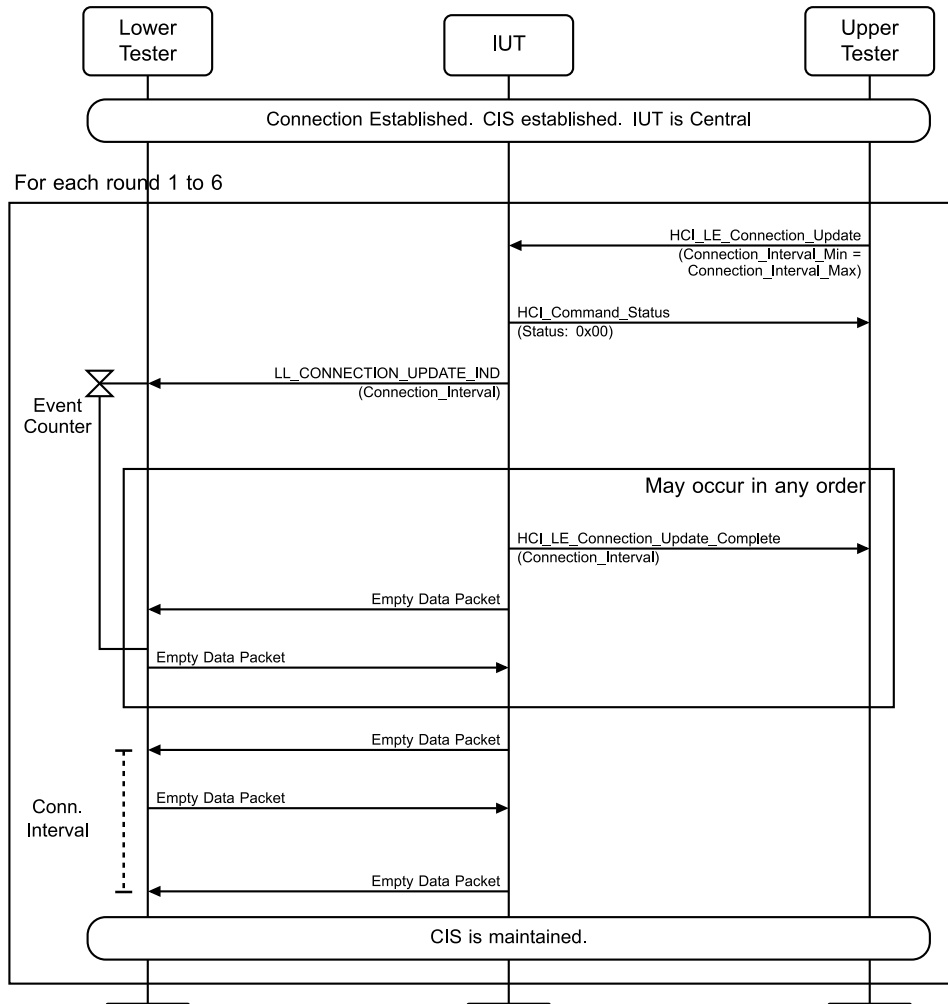
Figure 4.10-25: LL/CIS/CEN/BV-63-C [Updating an ACL while Maintaining a CIS]
