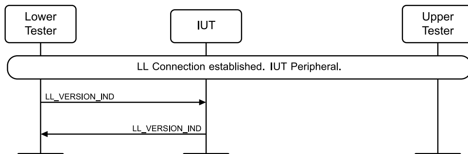
Figure 4.3-62: LL/CON/PER/BV-20-C [Peripheral Respond Version] MSC
