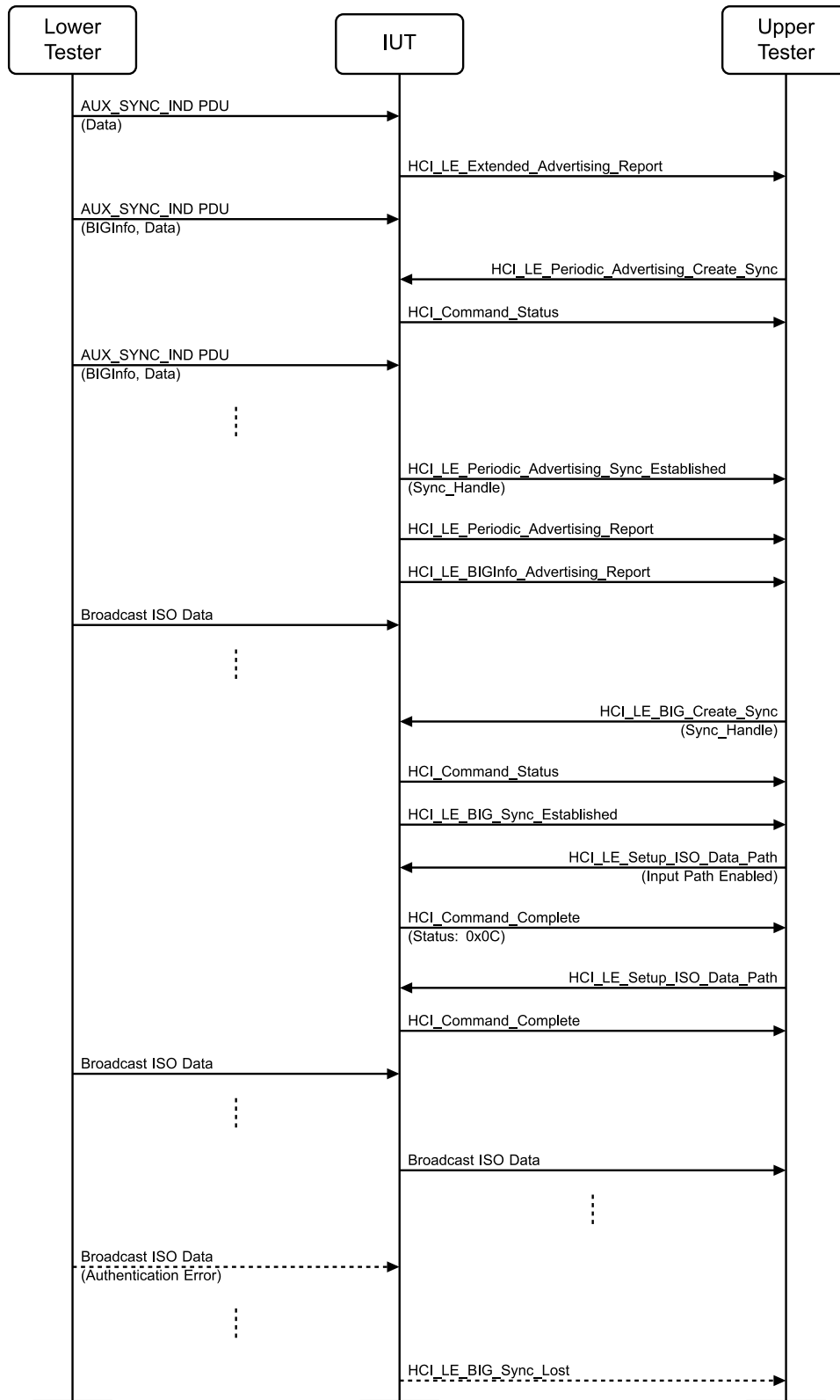
Figure 4.11-14: Broadcast Isochronous Stream Synchronization Setup MSC
