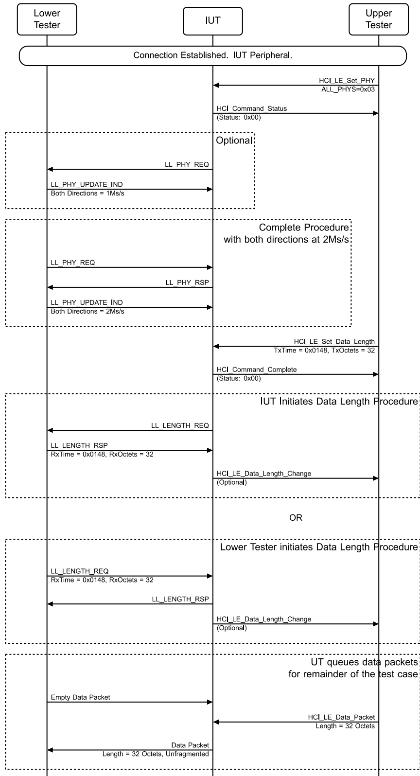
Figure 4.3-83: LL/CON/PER/BV-49-C [Initiating PHY Update Procedure – Packet Time Restrictions] MSC – Page 1 of 2
