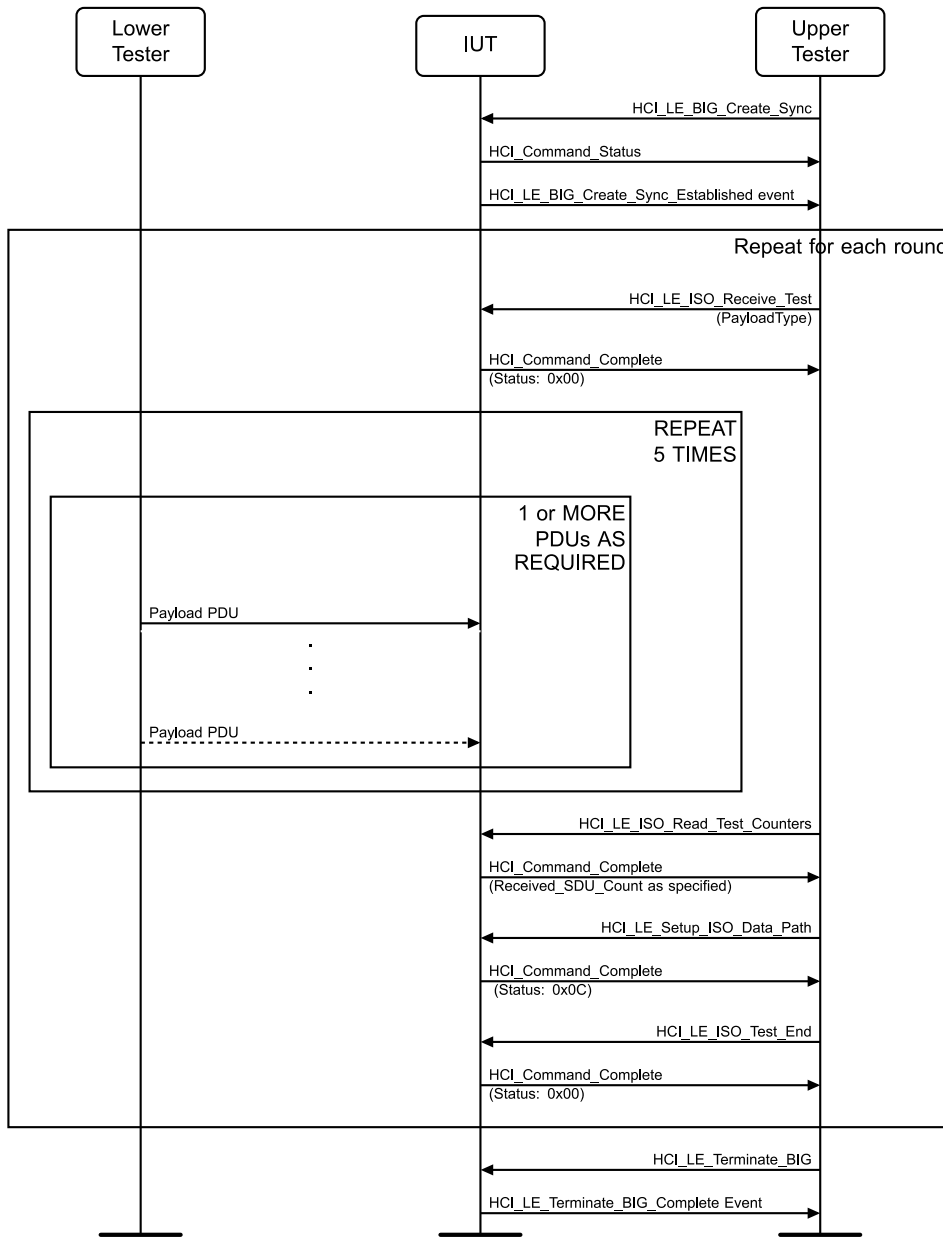
Figure 4.12-4: LL/IST/SNC/BV-01-C [ISO Receive Test Mode, BIS] MSC
