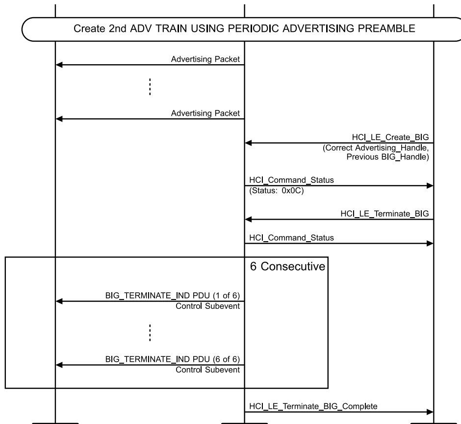
Figure 4.11-8: Broadcast Isochronous Stream Using Non-Test Command – MSC Page 2 of 2
