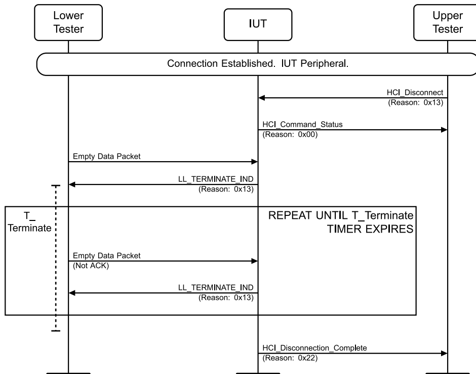
Figure 4.3-106: LL/CON/PER/BI-02-C [Peripheral T_Terminate Timer] MSC
