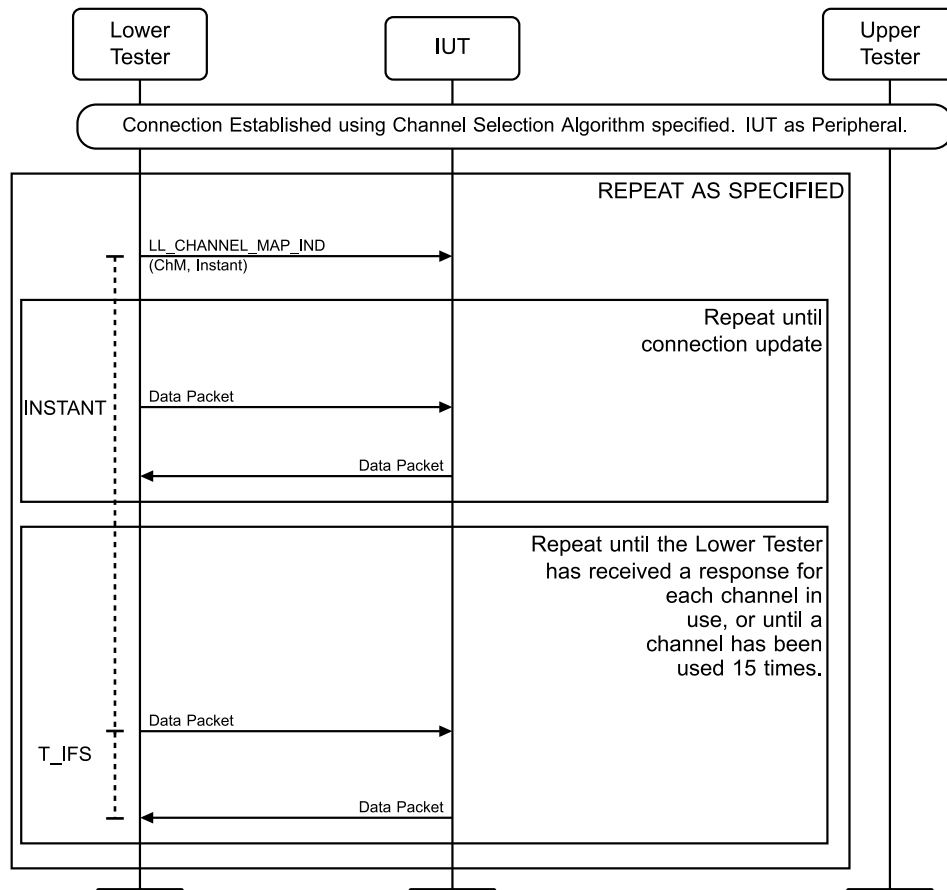
Figure 4.6-2: LL/FRH/PER/BV-02-C [Accepting Channel Map Update, Channel Selection Algorithm #2] MSC
