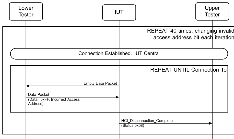
Figure 4.5-7: LL/ENC/CEN/BI-01-C [Packets to another Central] MSC
