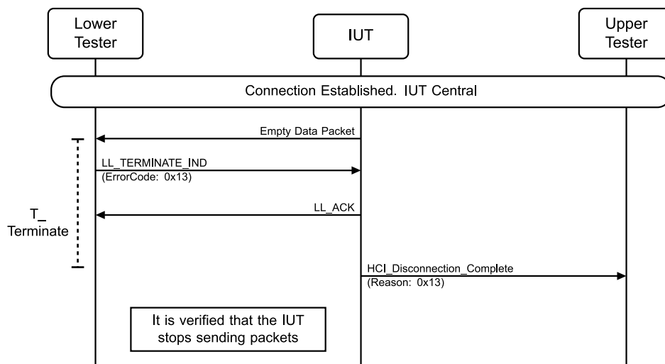
Figure 4.3-140: LL/CON/CEN/BV-09-C [Central Accepting Termination] MSC
