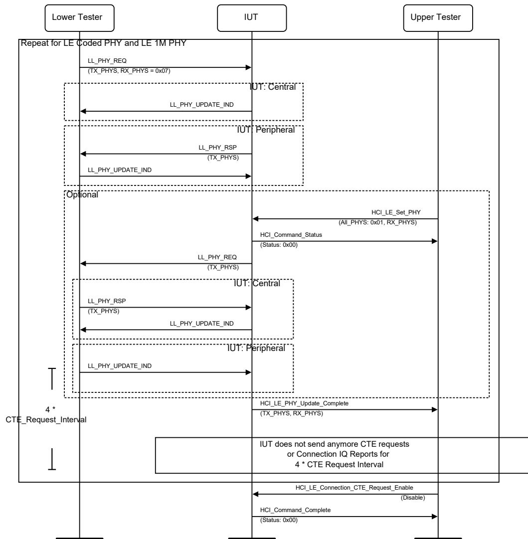
Figure 4.3-248: Constant Tone Extension Request Procedure, IUT Initiated, Periodic MSC – Page 2 of 2
