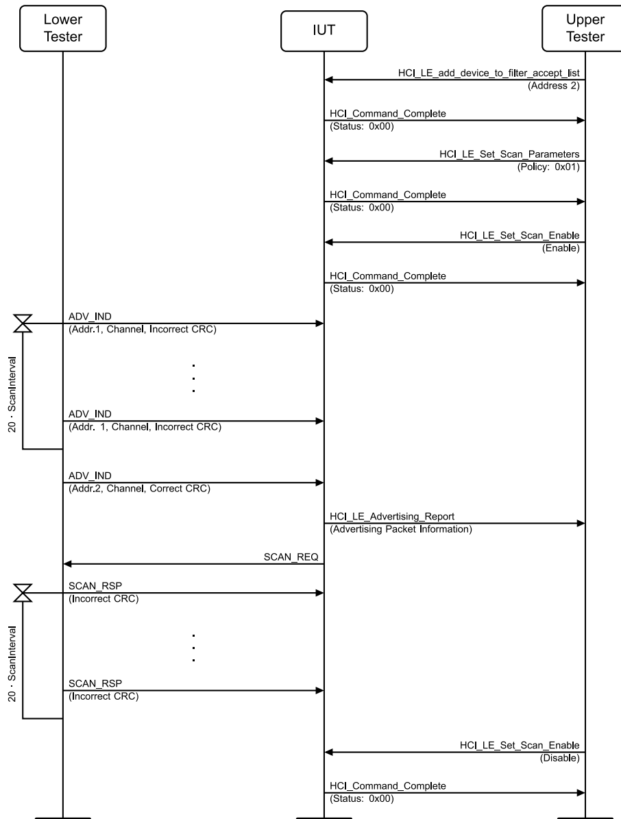
Figure 4.2-108: LL/DDI/SCN/BI-01-C [Active Scanning: Invalid CRC] MSC
