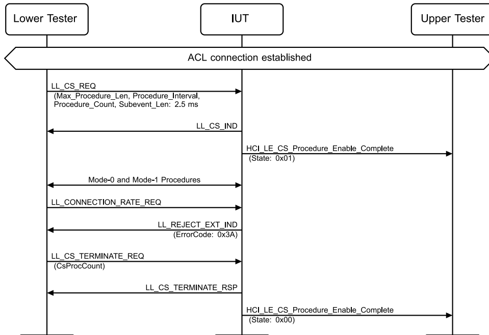
Figure 4.3-211: Reject Connection Rate Request, Channel Sounding procedure in progress MSC
