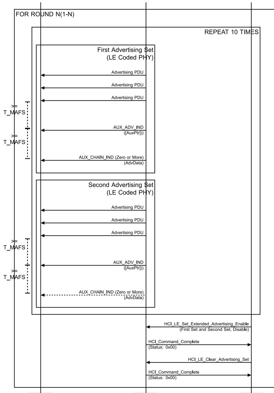
Figure 4.2-28: Extended Advertising, Multiple Sets MSC – Page 2 of 2
