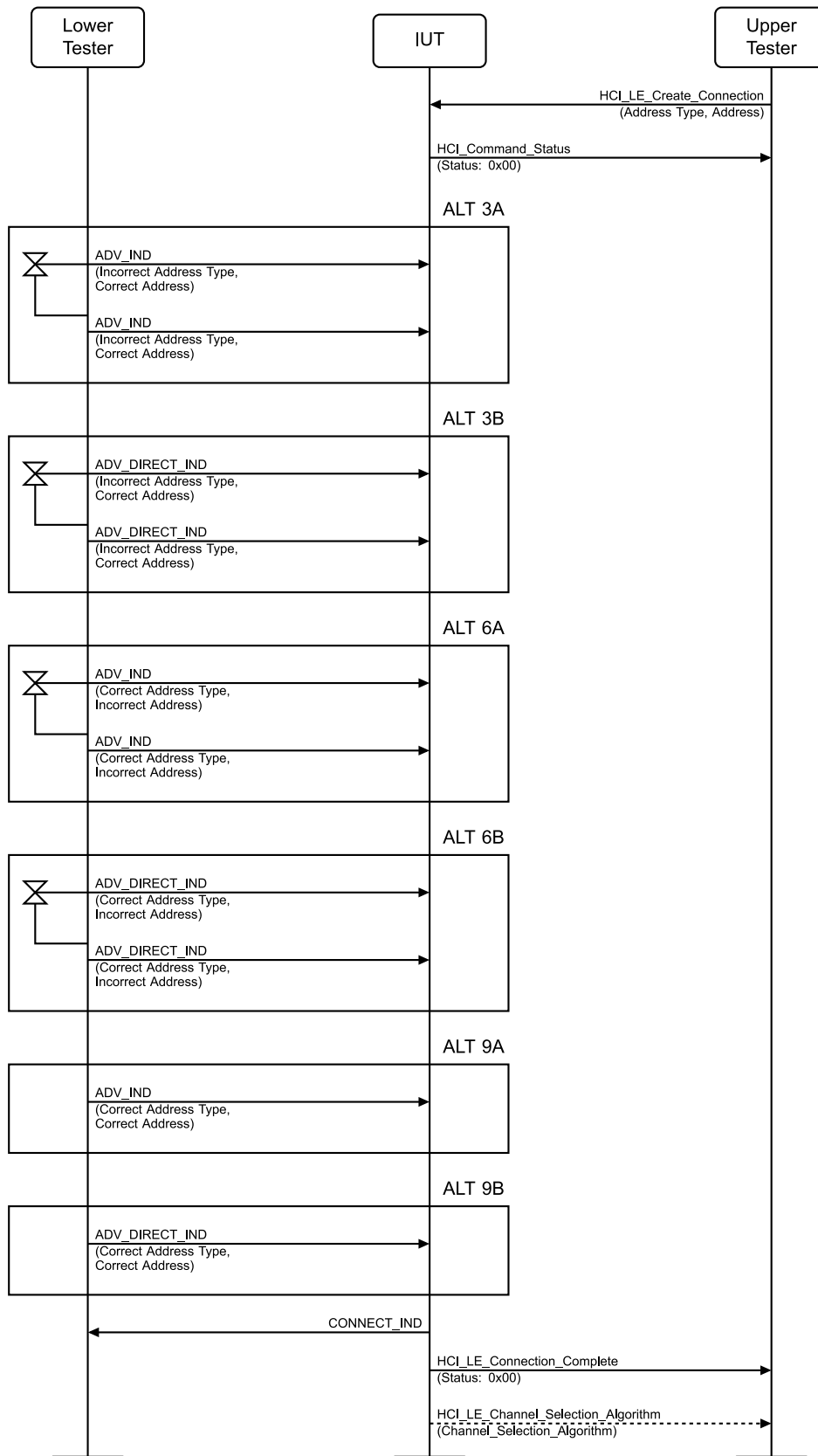
Figure 4.3-25: Initiation Device Filtering: MSC
