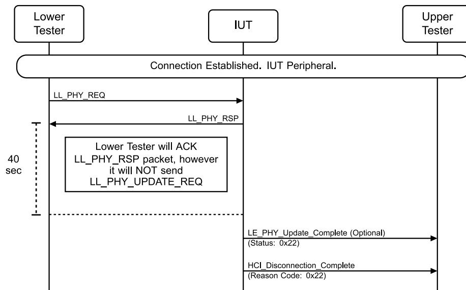
Figure 4.3-87: LL/CON/PER/BV-51-C [Protocol Timeout for PHY Update Procedure] MSC
