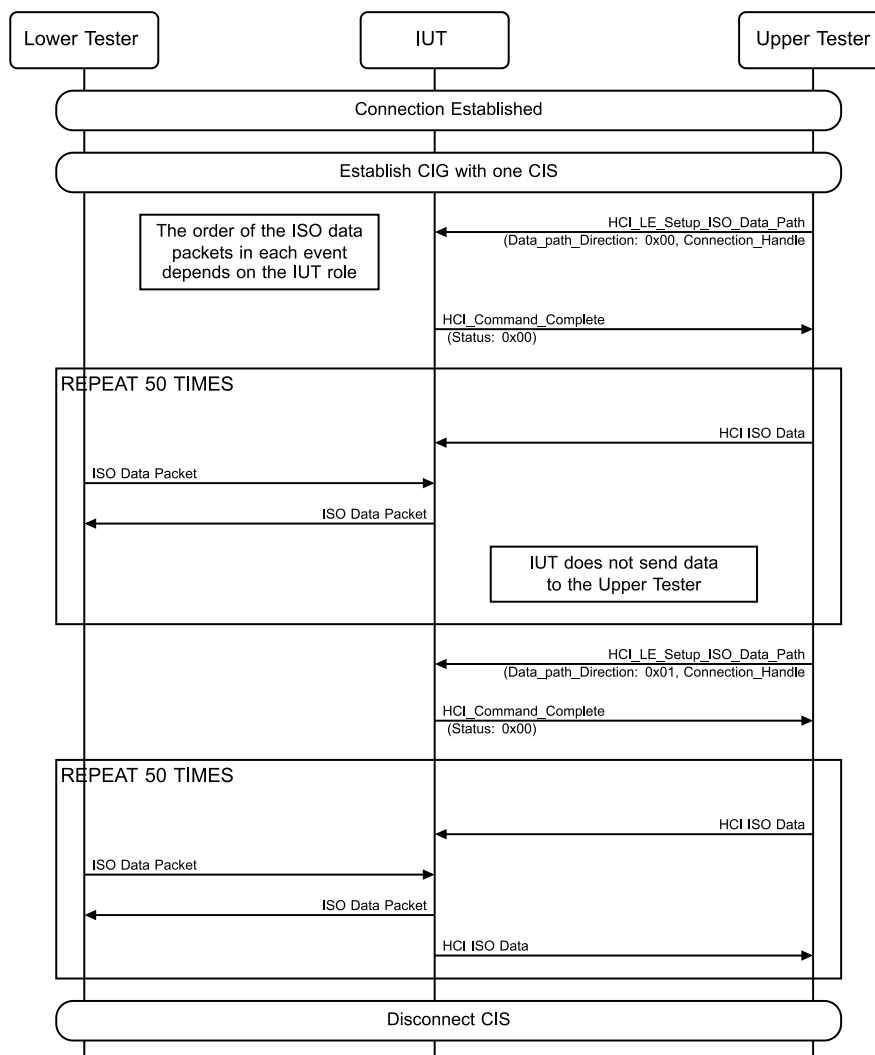
Figure 4.10-62: Incoming Data Path Setup MSC – Page 1 of 2
