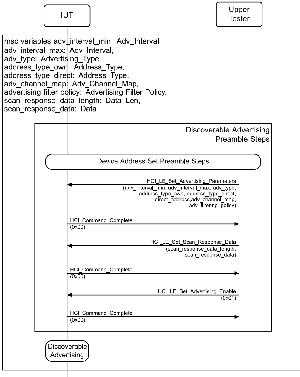
Figure 4.1-8: Discoverable Advertising preamble steps
