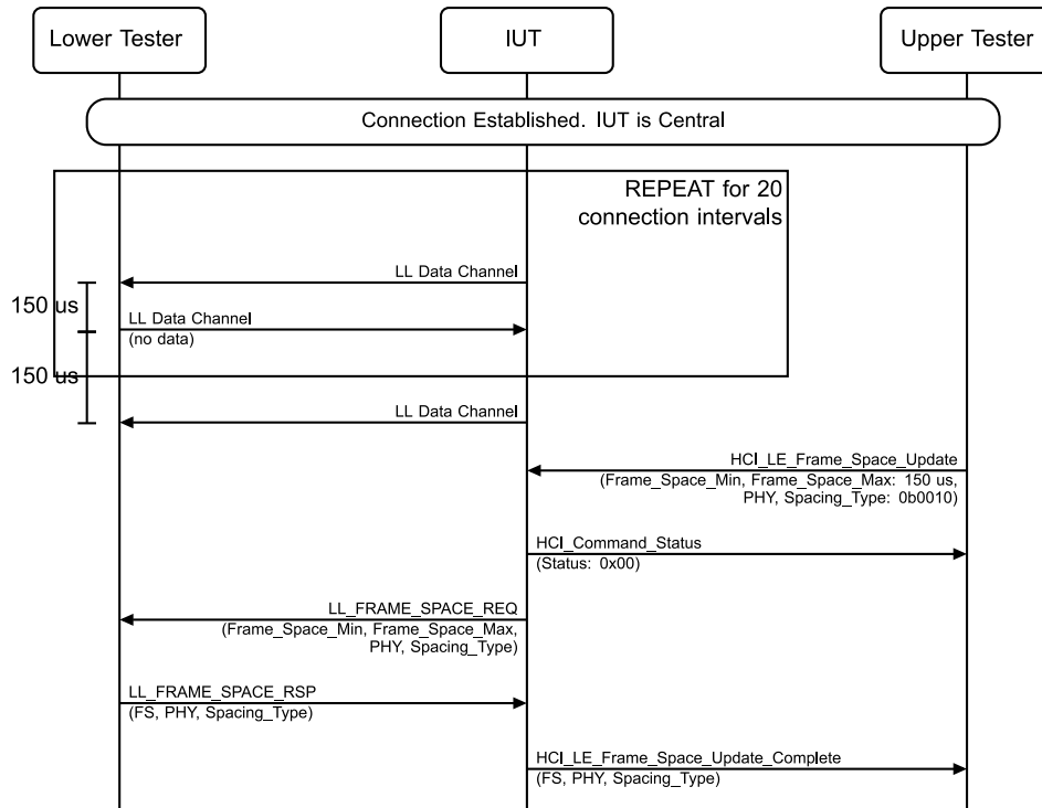
Figure 4.4-40: Initiate Inter Frame Space Change on a Different Asymmetric PHY for TX and RX, Central MSC – Page 1 of 2
