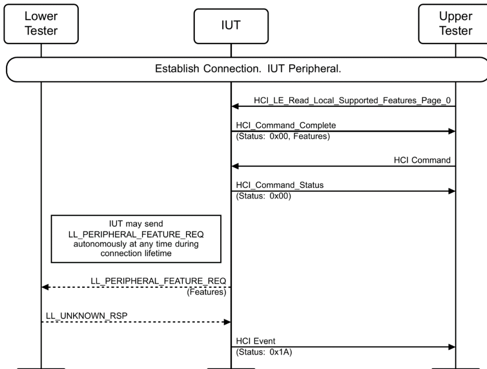
Figure 4.3-65: Initiate Feature Exchange – Central does not support MSC
