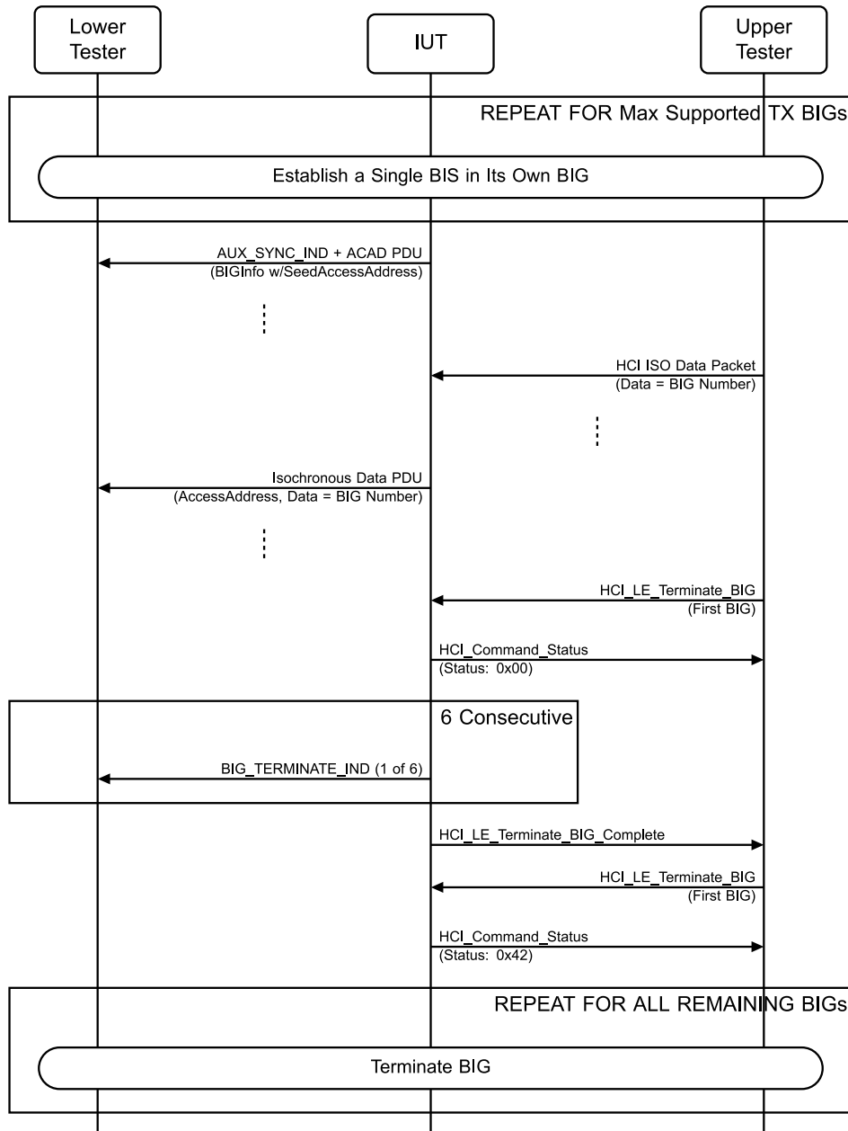
Figure 4.11-9: Maximum Supported Broadcast Isochronous Groups MSC
