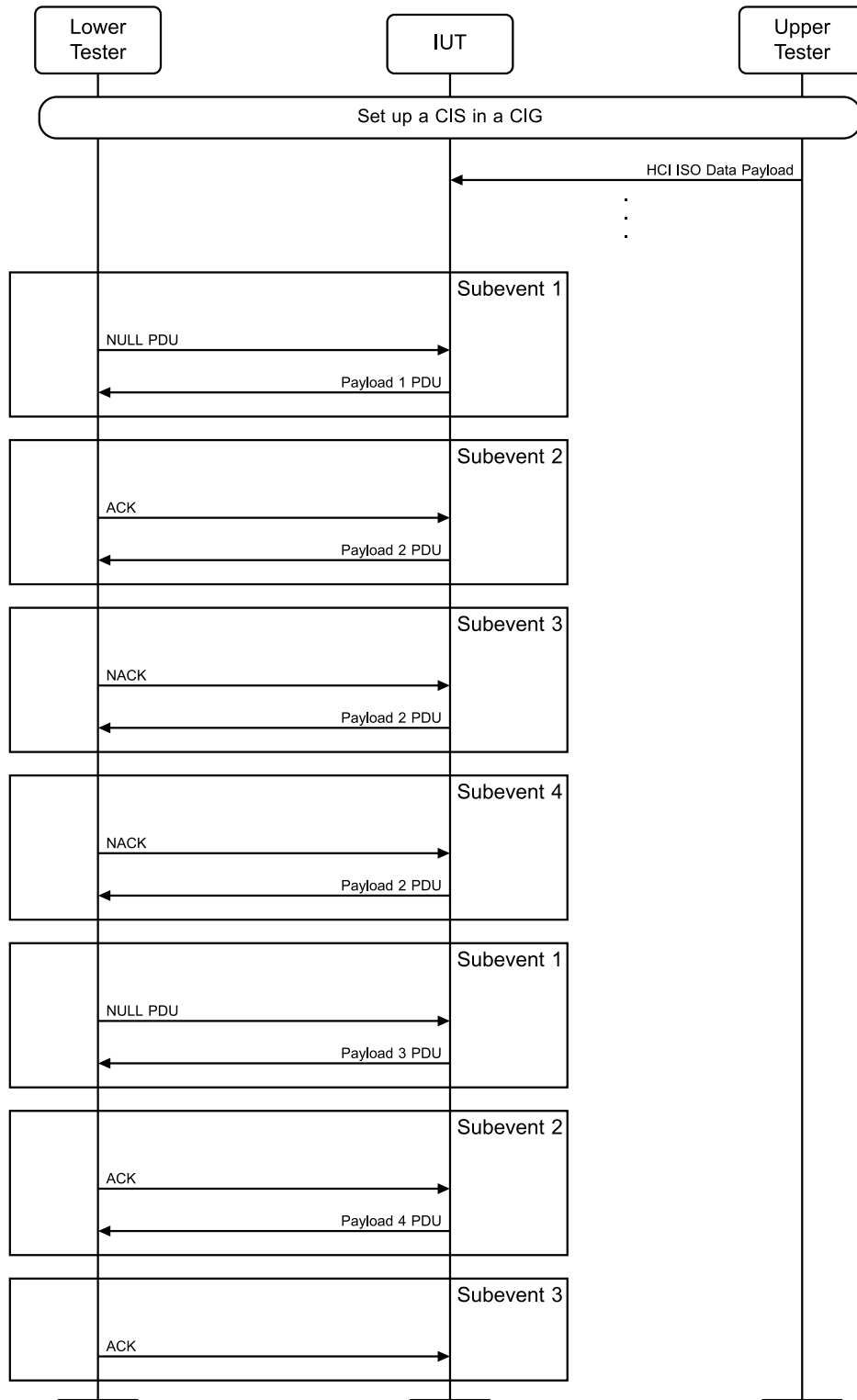
Figure 4.10-35: LL/CIS/PER/BV-15-C [Bursting of Payloads in CIS, Peripheral] MSC
