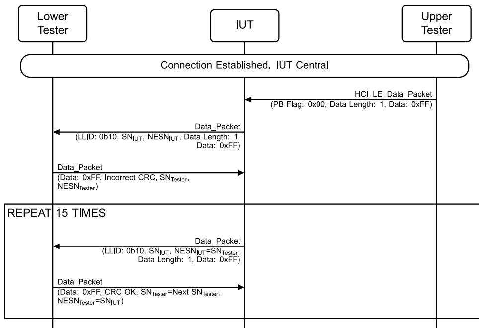
Figure 4.3-146: LL/CON/CEN/BV-17-C [Central Lost Negative Acknowledgement] MSC
