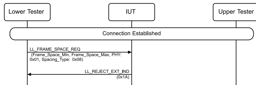
Figure 4.4-49: Frame Space Change, CIS not supported MSC
