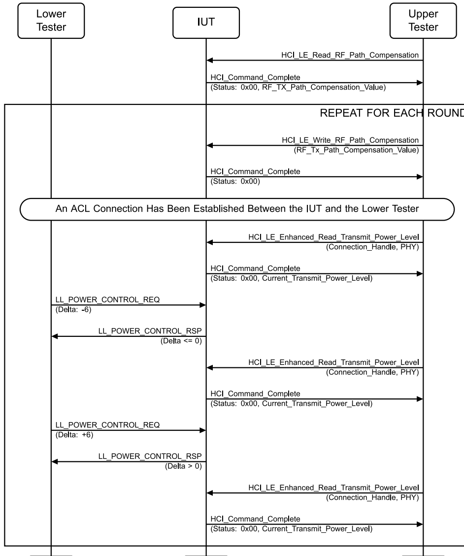
Figure 4.13-12: Power Control Response with RF Path Compensation MSC
