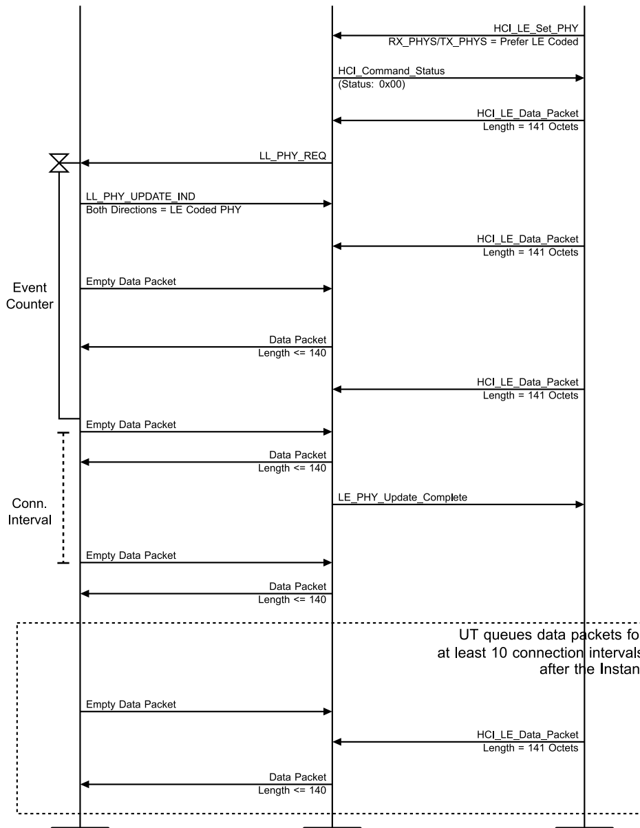
Figure 4.3-94: LL/CON/PER/BV-55-C [Initiating PHY Update Procedure – Packet Time Restrictions, LE Coded] MSC – Page 2 of 2
