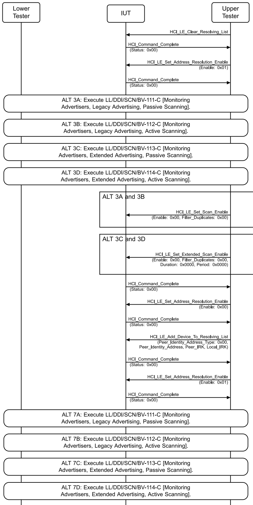
Figure 4.2-149: Monitoring Advertisers, Resolvable Addresses MSC
