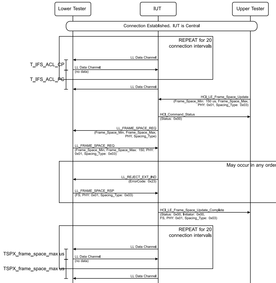
Figure 4.4-36: LL/TIM/CEN/BV-24-C [Handling Frame Space Request Collision – Same Procedure, Central] MSC
