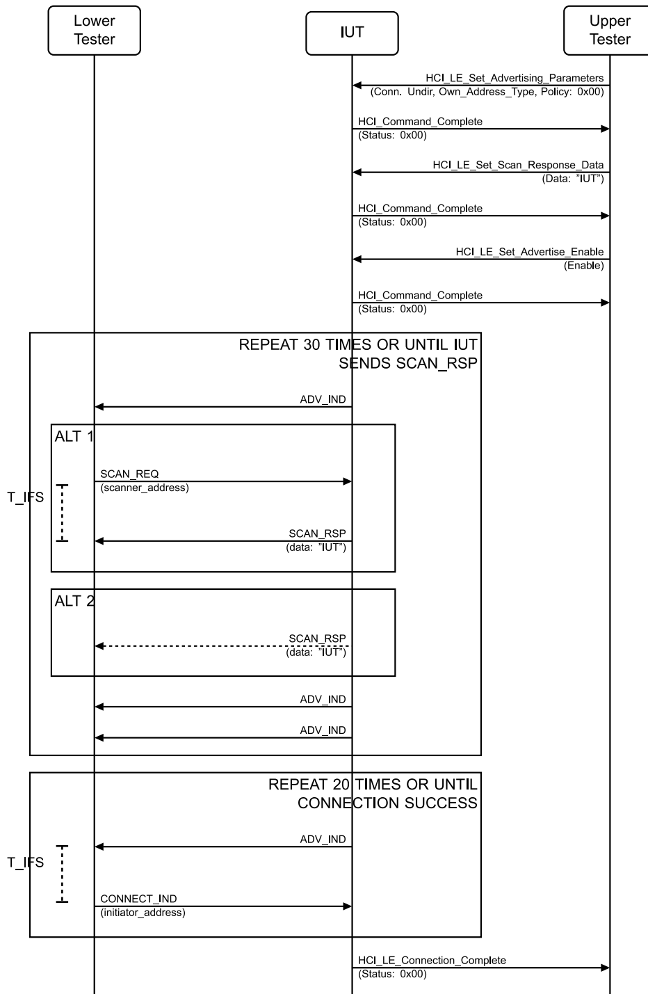
Figure 4.2-5: LL/DDI/ADV/BV-07-C [Scan Request Connection Request] MSC
