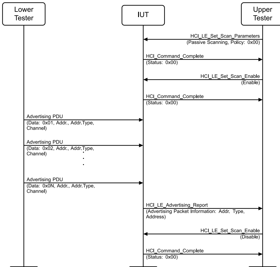
Figure 4.2-77: Passive Scanning MSC
