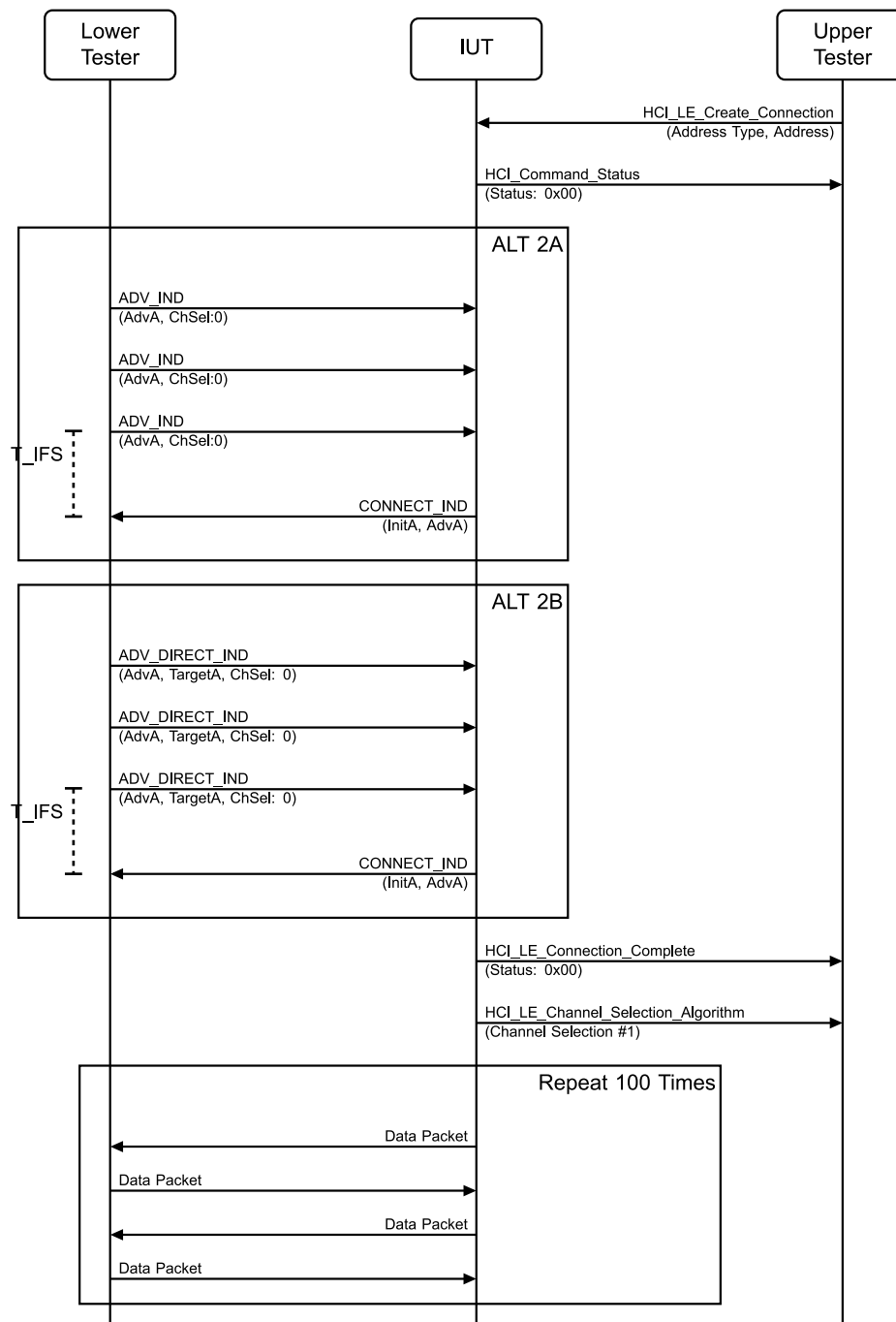
Figure 4.3-32: LL/CON/INI/BV-14-C [Connection Initiation, Channel Selection Algorithm #1] MSC
