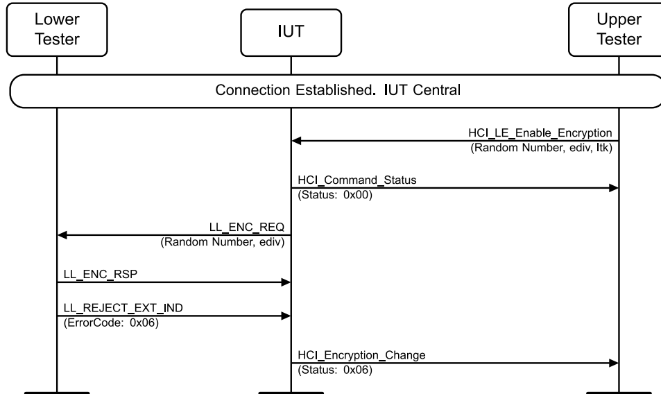
Figure 4.8-50: LL/SEC/CEN/BV-11-C [Central receiving LL_REJECT_EXT_IND] MSC
