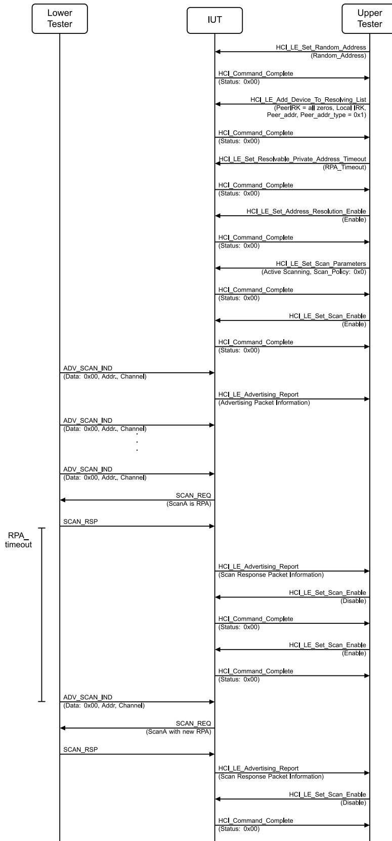
Figure 4.2-87: LL/DDI/SCN/BV-16-C [Network Privacy – Active Scanning, Local IRK, no Peer IRK] MSC
