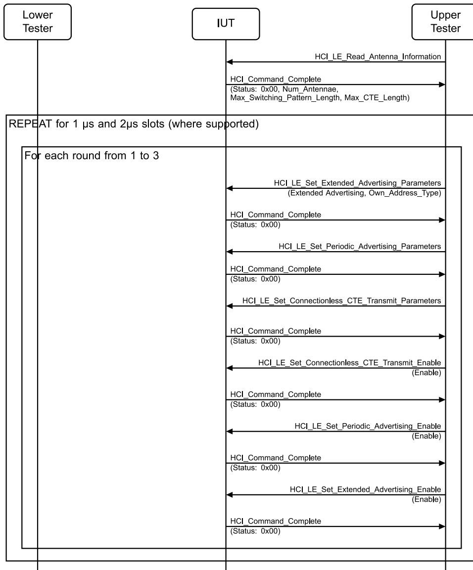
Figure 4.2-35: AoD Connectionless CTE Advertising MSC – Page 1 of 2
