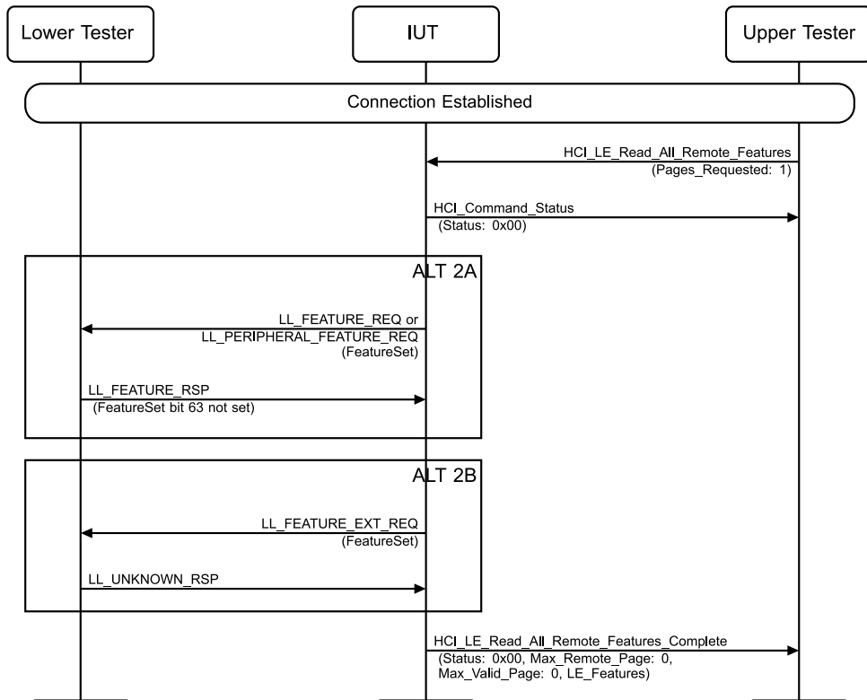
Figure 4.3-264: LL Extended Feature Set Not Supported by the Peer MSC
