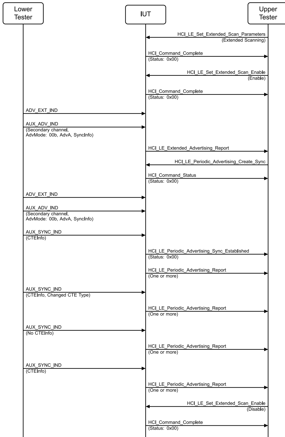
Figure 4.2-105: LL/DDI/SCN/BV-36-C [Connectionless CTE Scanning, CTE Type Change] MSC
