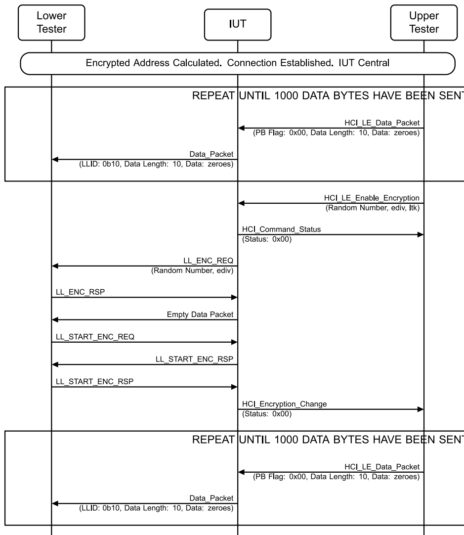
Figure 4.8-41: LL/SEC/CEN/BV-01-C [Central Encryption Mode Setup] MSC
