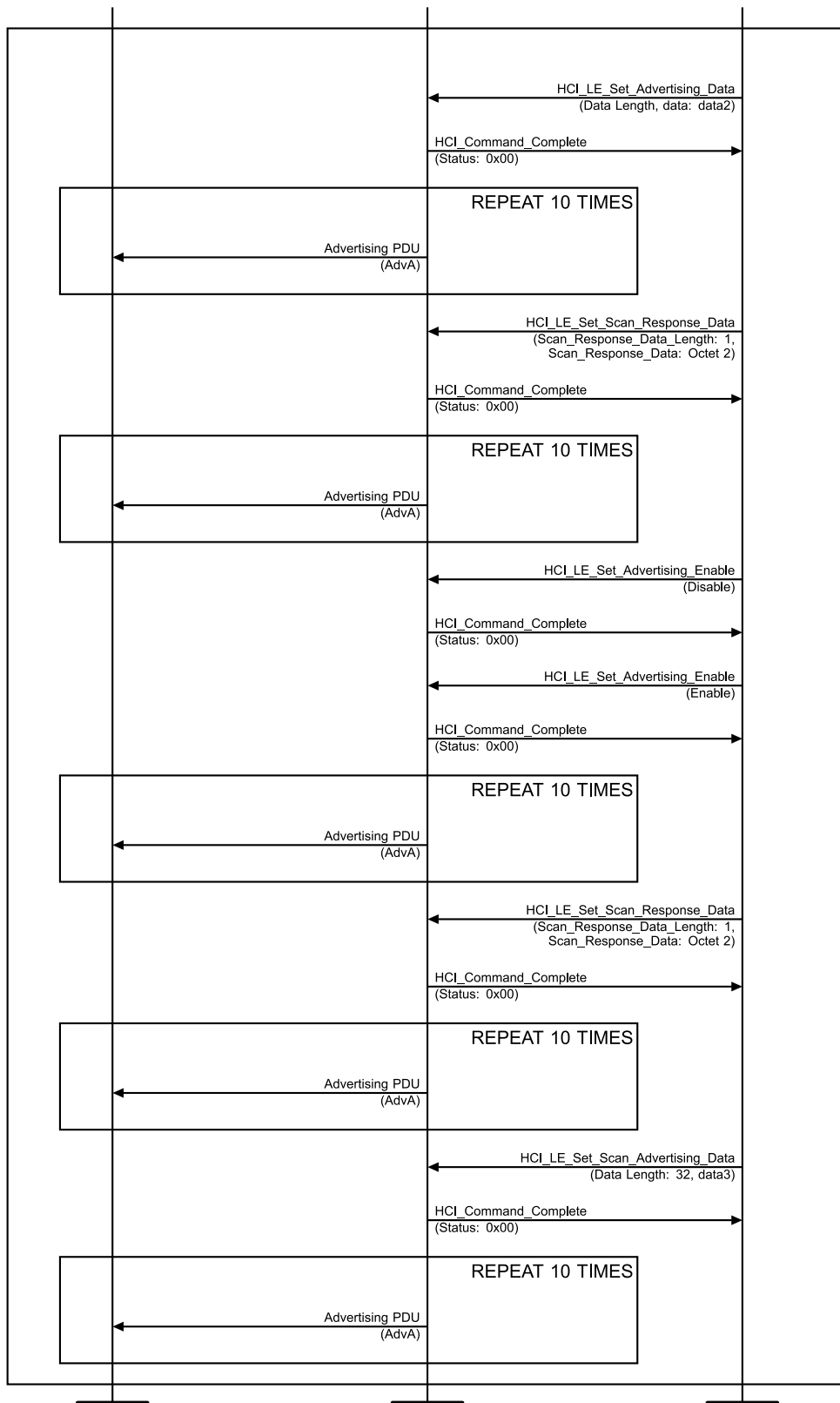
Figure 4.2-53: Advertising Data, New RPA on Change Reasons MSC – Page 2 of 2
