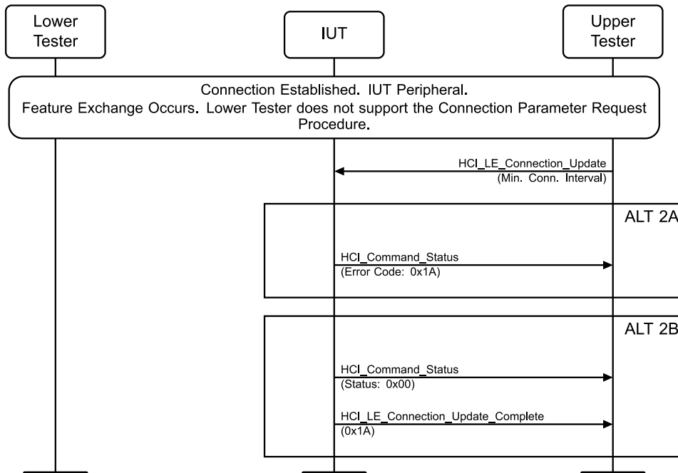
Figure 4.3-104: LL/CON/PER/BV-86-C [Initiating Connection Parameter Request – Unsupported With Feature Exchange] MSC
