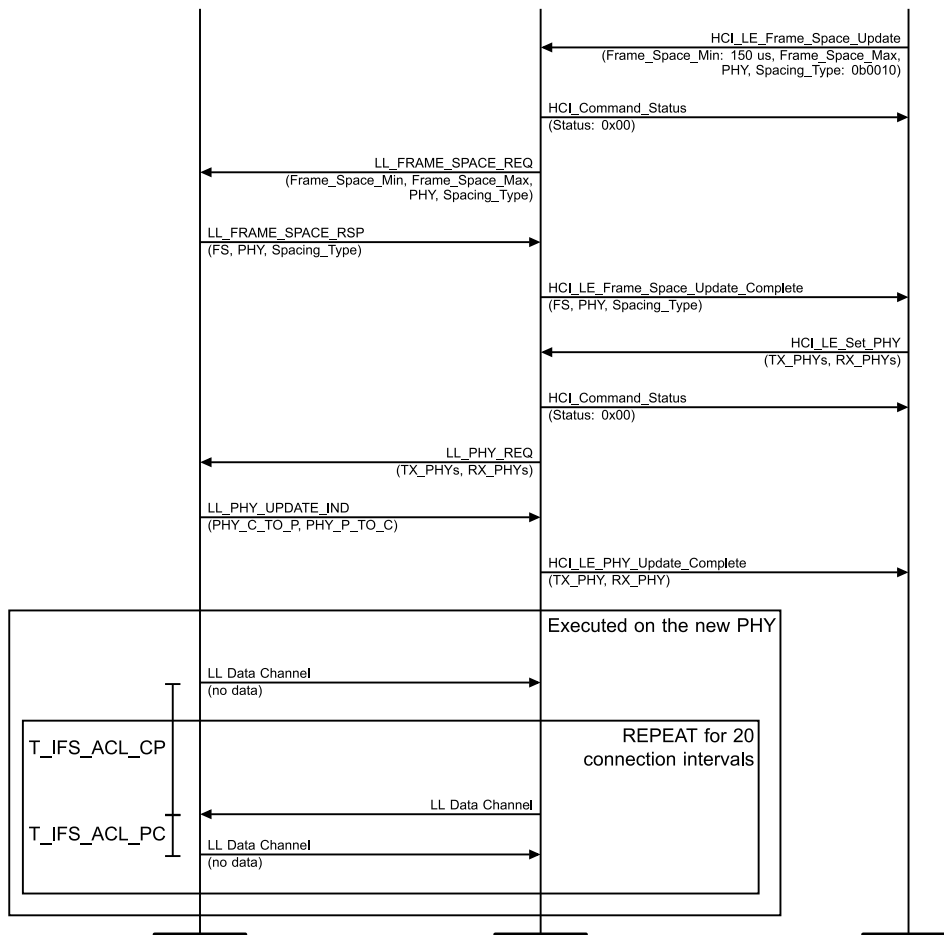
Figure 4.4-23: Initiate Inter Frame Space Change on a Different Asymmetric PHY for TX and RX, Peripheral MSC – Page 2 of 2
