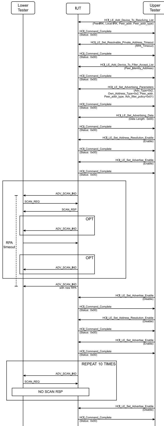
Figure 4.8-4: Network Privacy – Scannable Advertising, resolvable private address MSC
