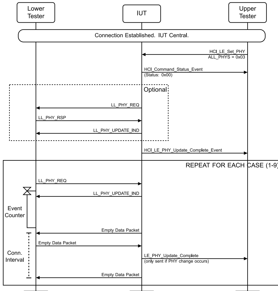
Figure 4.3-166: LL/CON/CEN/BV-43-C [Responding to PHY Update Procedure] MSC
