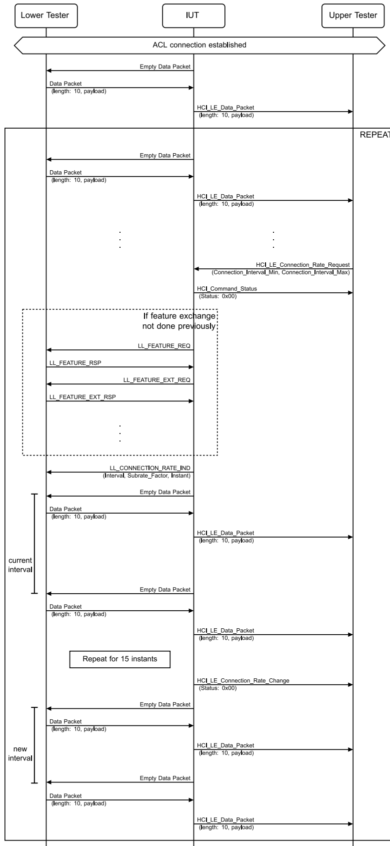
Figure 4.3-208: LL/CON/CEN/BV-174-C [Initiate a Connection Rate Update, Central] MSC
