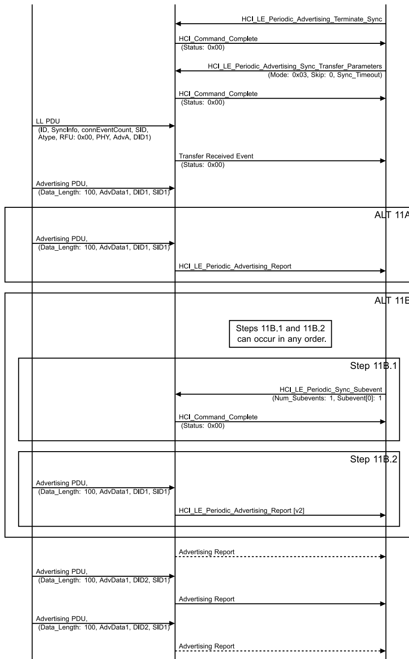
Figure 4.3-250: Periodic Advertising Sync Transfer Procedure, Accepting, Enabling Duplicate Filter when already synchronized MSC – Page 2 of 2
