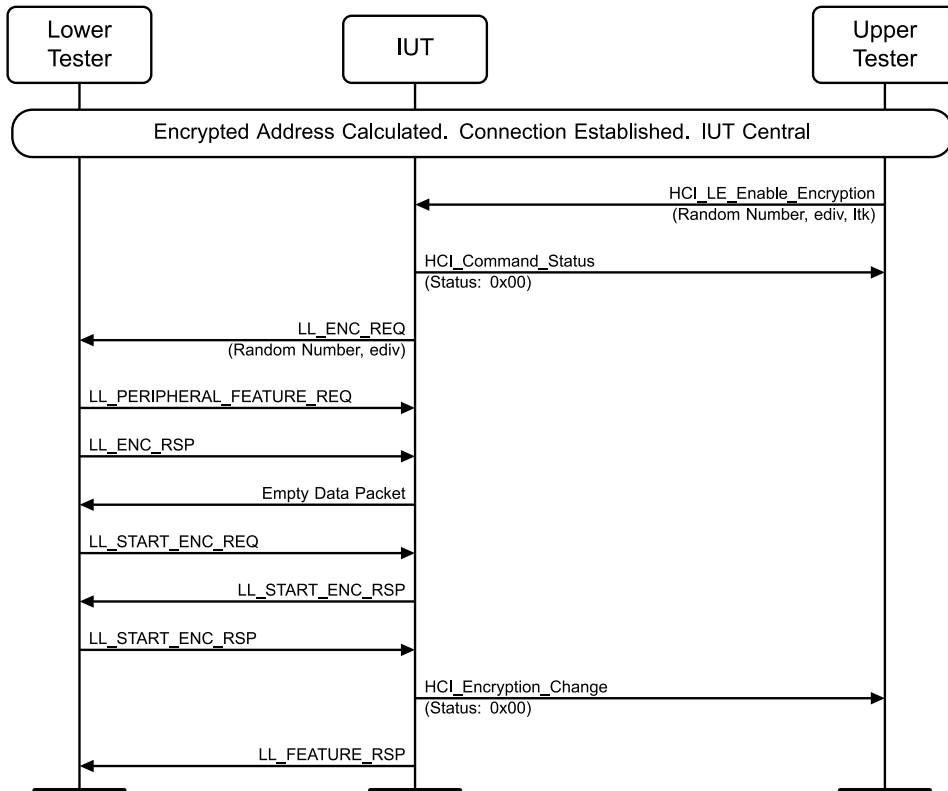
Figure 4.8-52: LL/SEC/CEN/BV-13-C [Central Start Encryption: Overlapping Procedure] MSC
