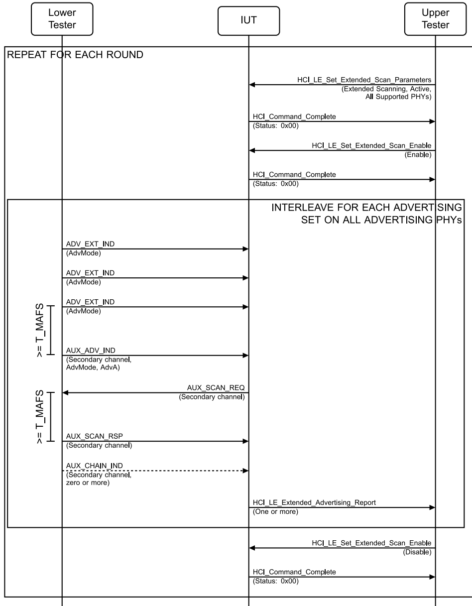
Figure 4.2-97: Extended Scanning, Multiple Sets, Active, Multiple PHYs (All Supported PHYs) MSC
