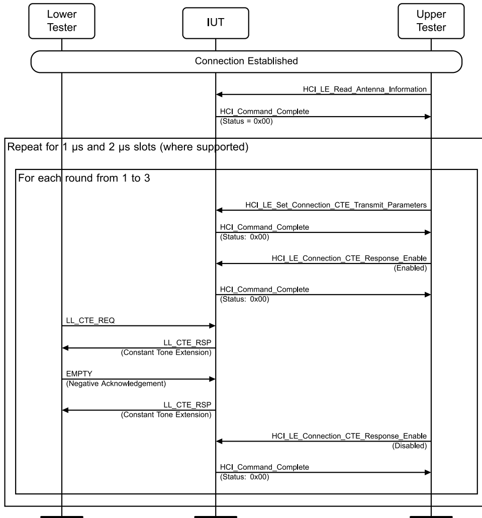
Figure 4.3-240: Constant Tone Extension Request Procedure, IUT Responding, AoD MSC
