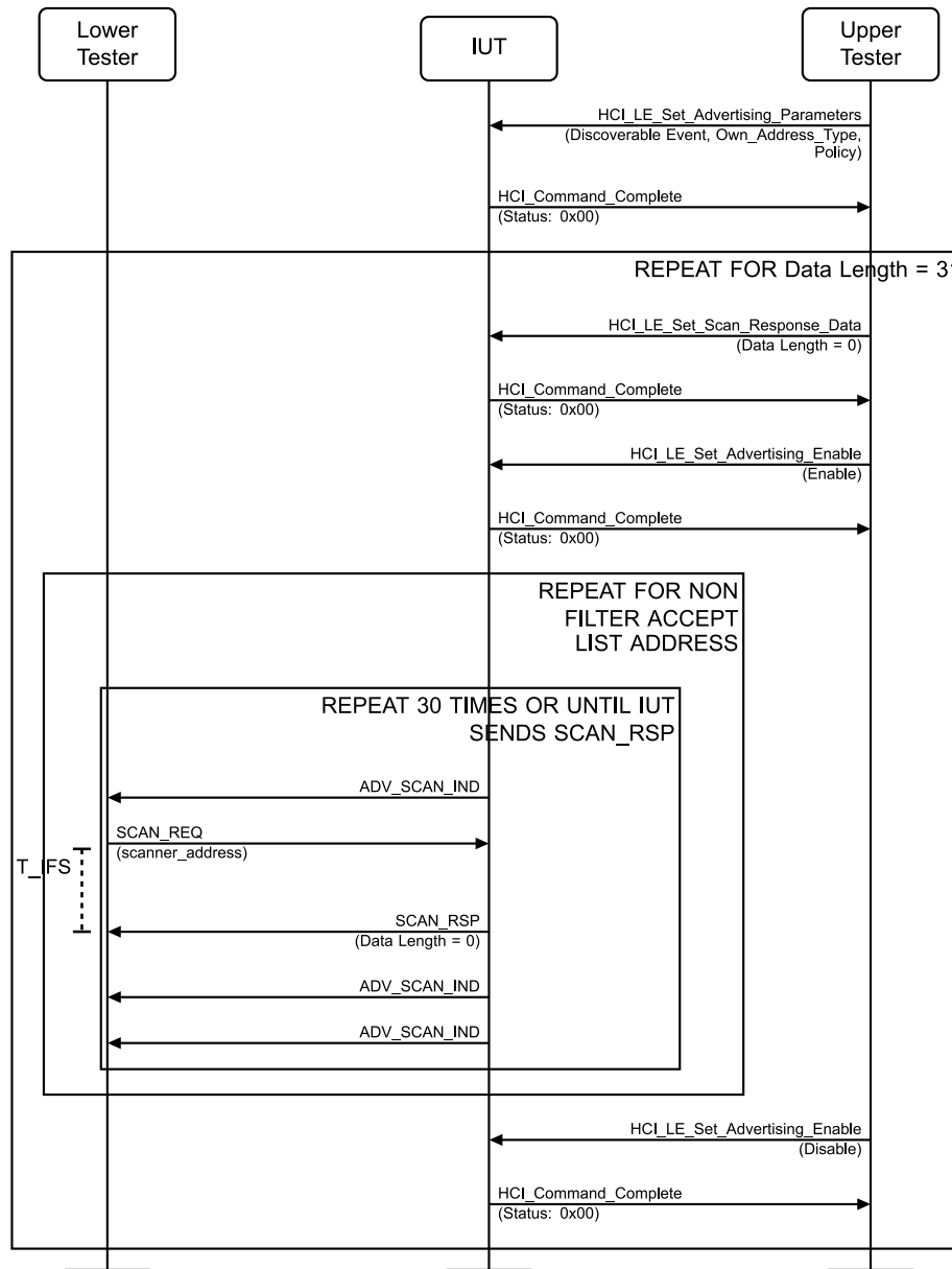
Figure 4.2-11: LL/DDI/ADV/BV-17-C [Scan Request: Discoverable] MSC
