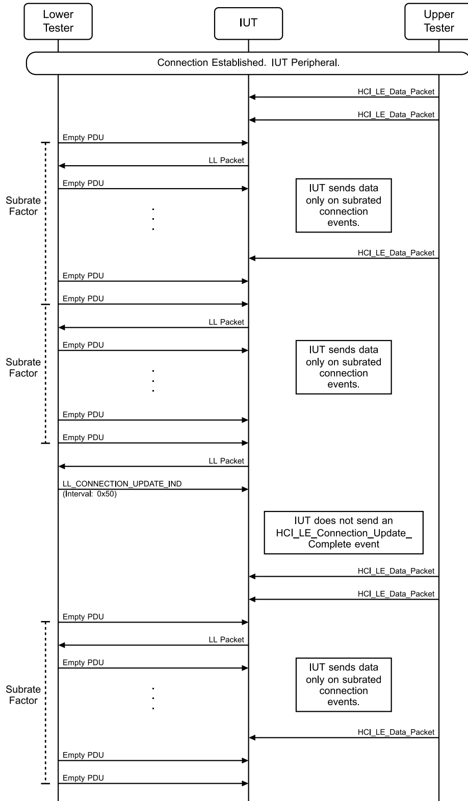
Figure 4.3-114: LL/CON/PER/BV-139-C [Subrate Factor set to 1 and Continuation Number set to 0 on Connection Interval change] MSC – Page 1 of 2
