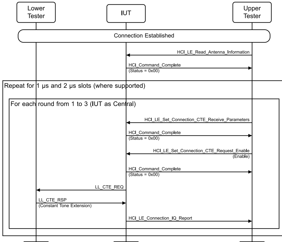
Figure 4.3-233: Constant Tone Extension Request Procedure, IUT Initiated, AoA MSC
