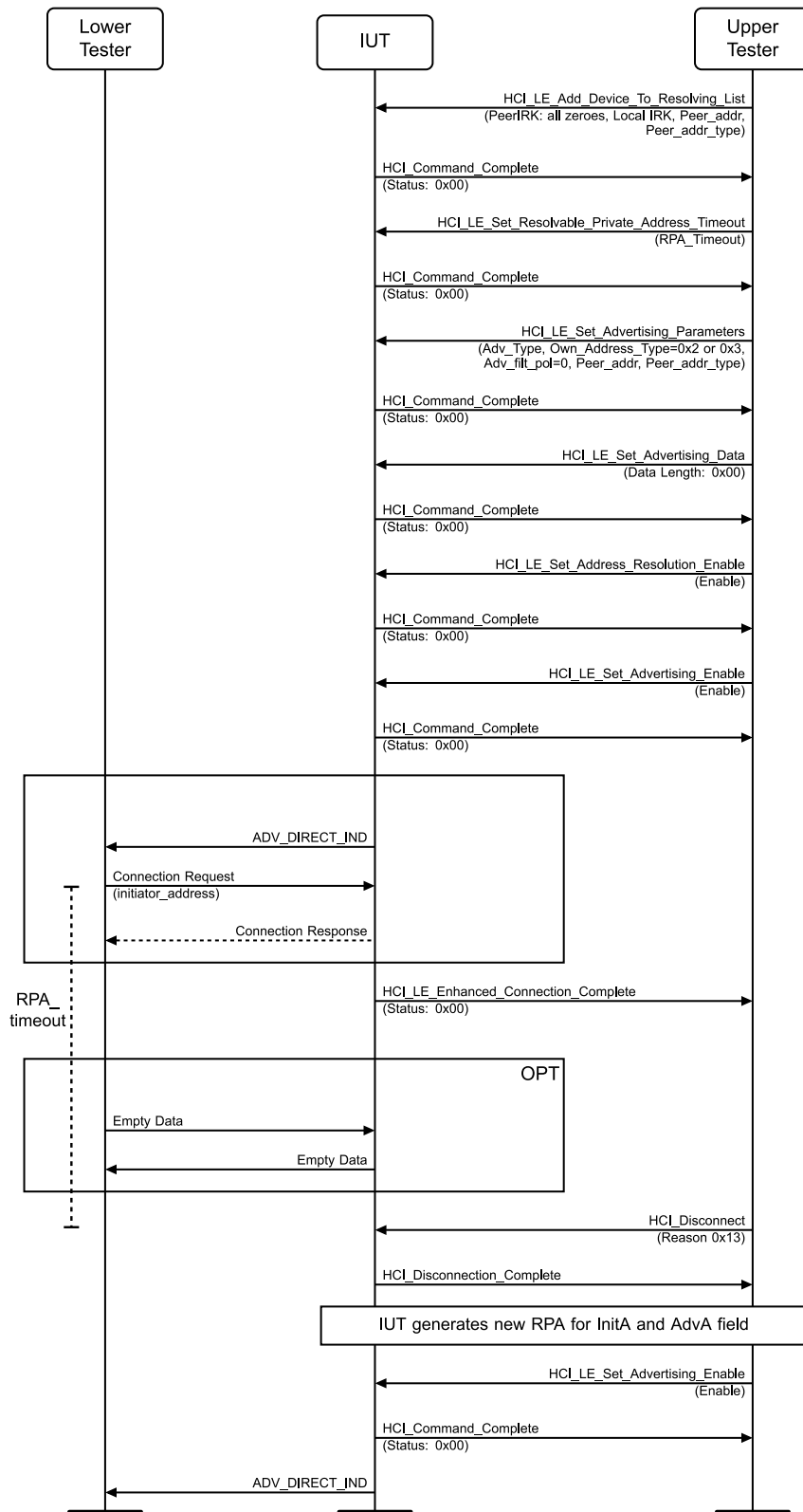
Figure 4.8-12: Network Privacy - Directed Connectable Advertising with local IRK but without remote IRK MSC
