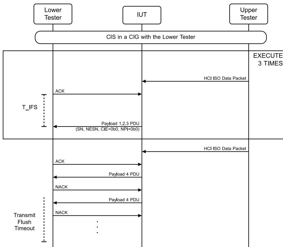
Figure 4.10-33: Acknowledgement Scheme, Peripheral MSC
