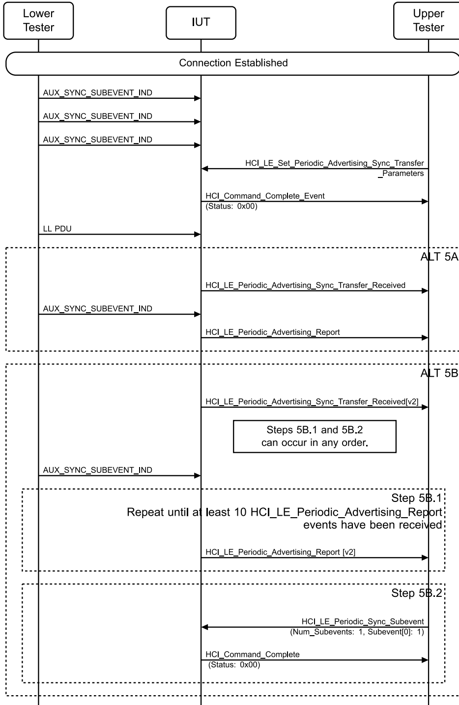
Figure 4.3-218: Periodic Advertising Sync Transfer Procedure, Accepting – Already Synchronized MSC – Page 1 of 2
