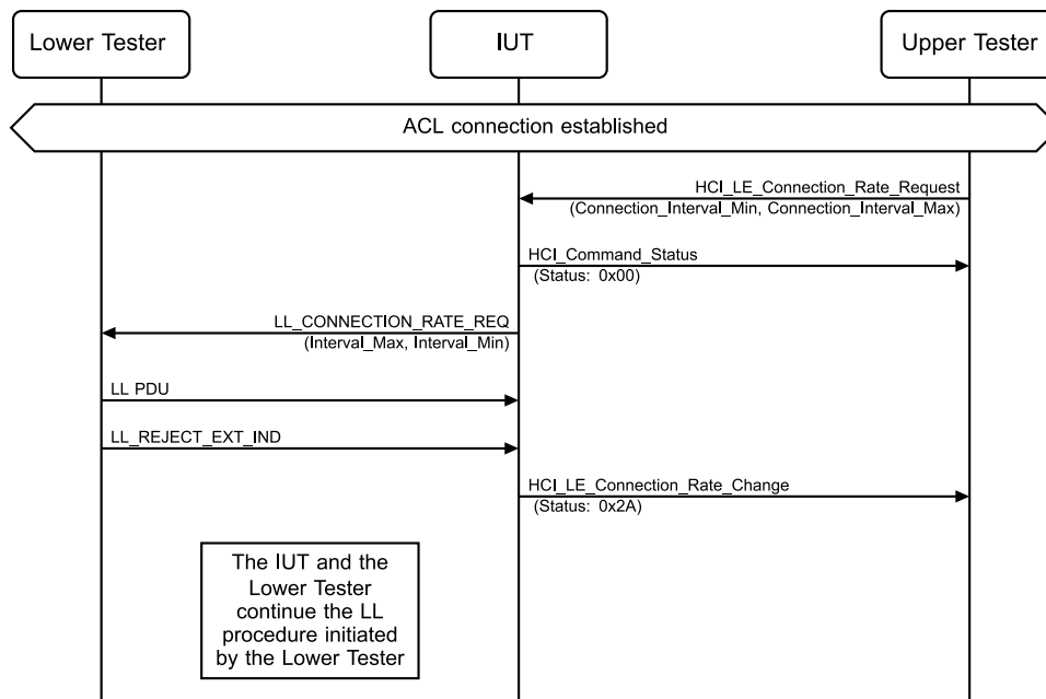
Figure 4.3-132: Reject Connection Rate Request procedure, LL procedure in progress, Peripheral MSC
