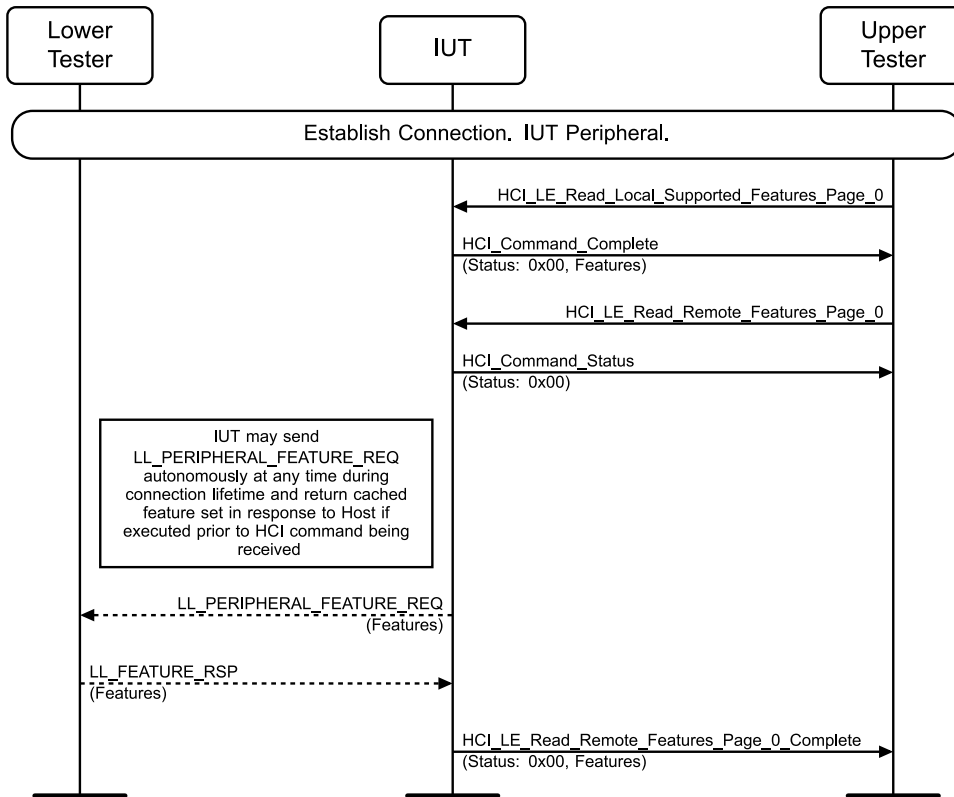
Figure 4.3-64: LL/CON/PER/BV-22-C [Initiate Feature Exchange] MSC
