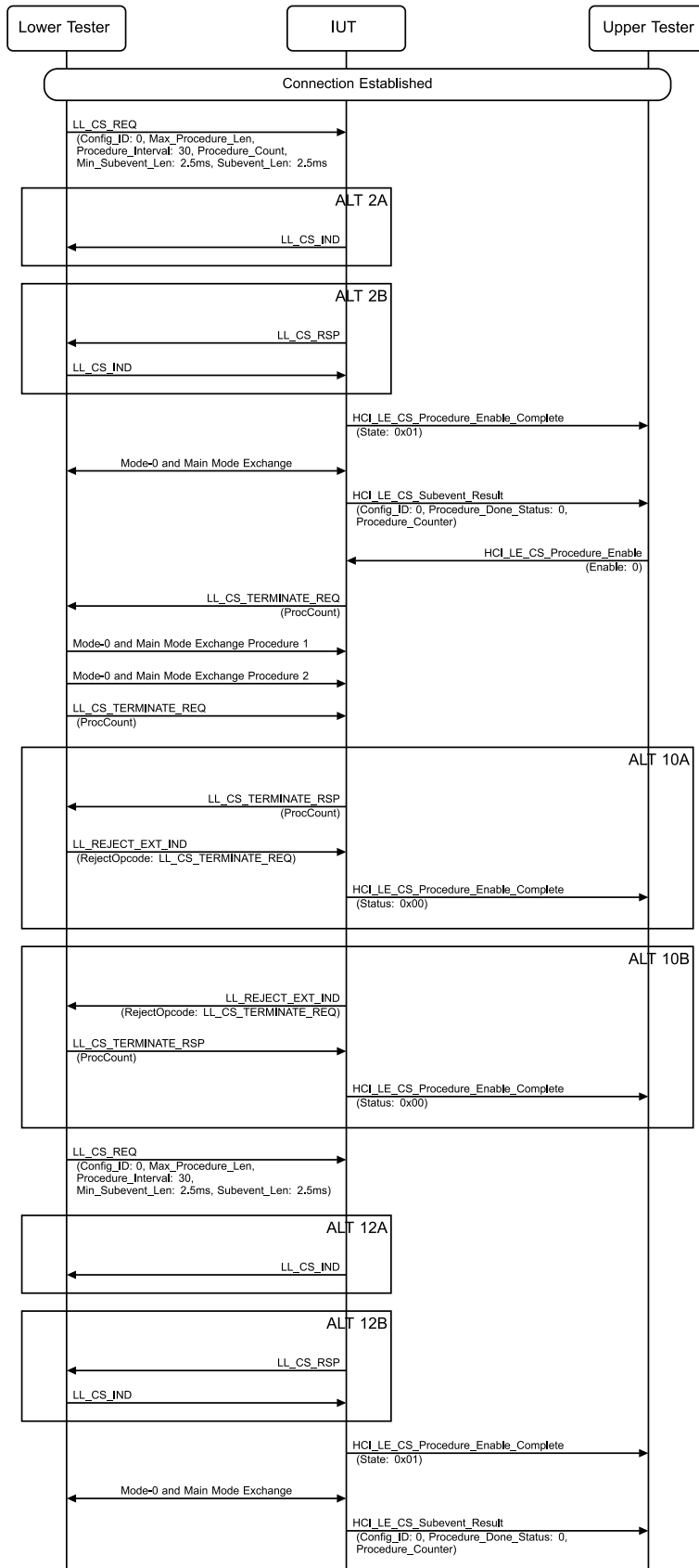
Figure 4.14-63: CS Procedure, Receive Repeat Termination, Verify ProcCount Difference MSC
