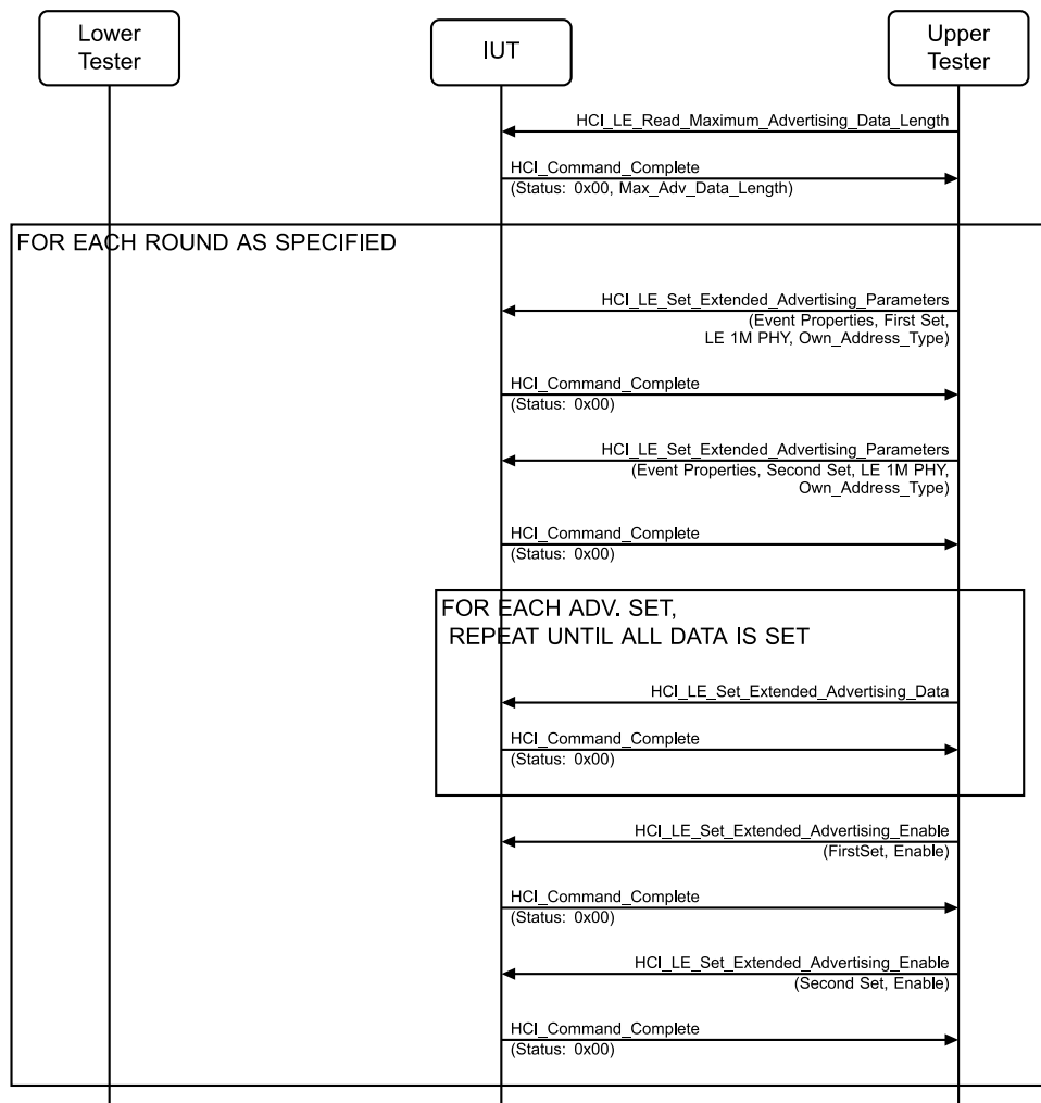
Figure 4.2-29: Extended Advertising, Multiple Sets, Legacy and Extended MSC – Page 1 of 2
