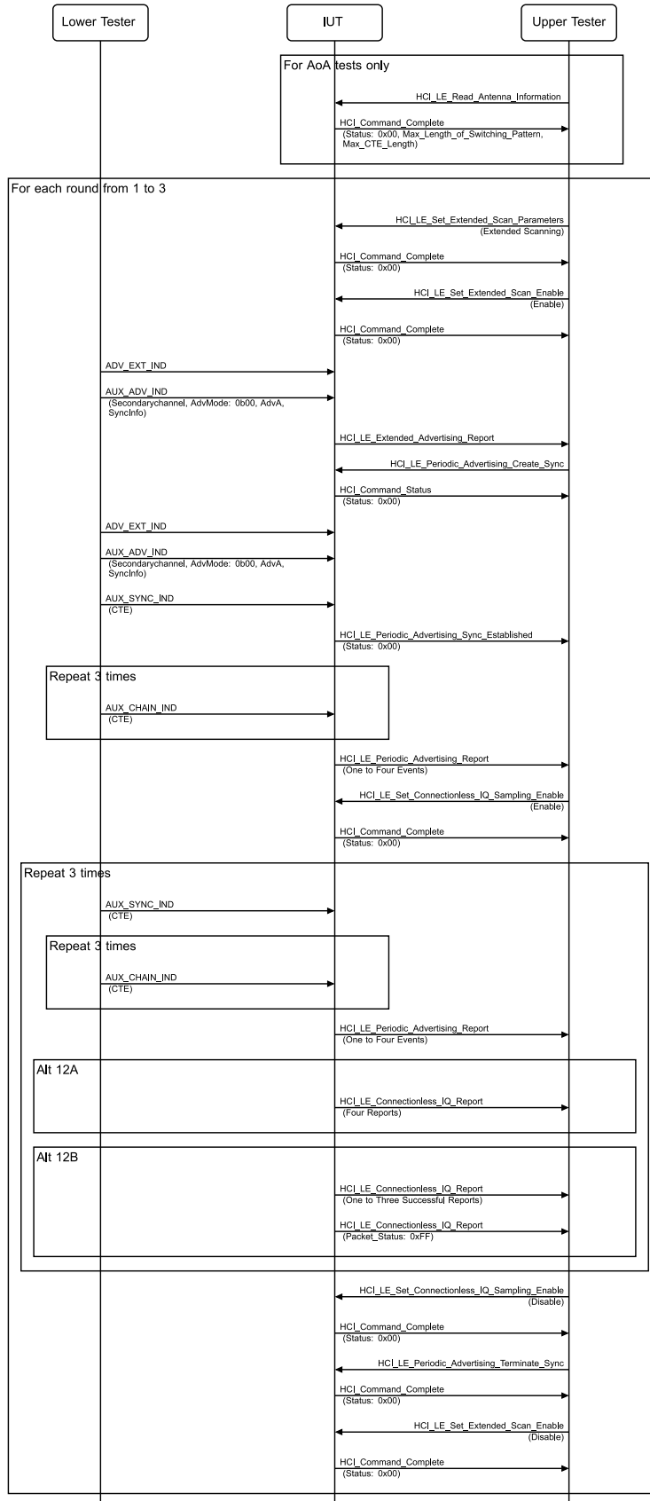
Figure 4.2-100: Connectionless CTE Scanning MSC
