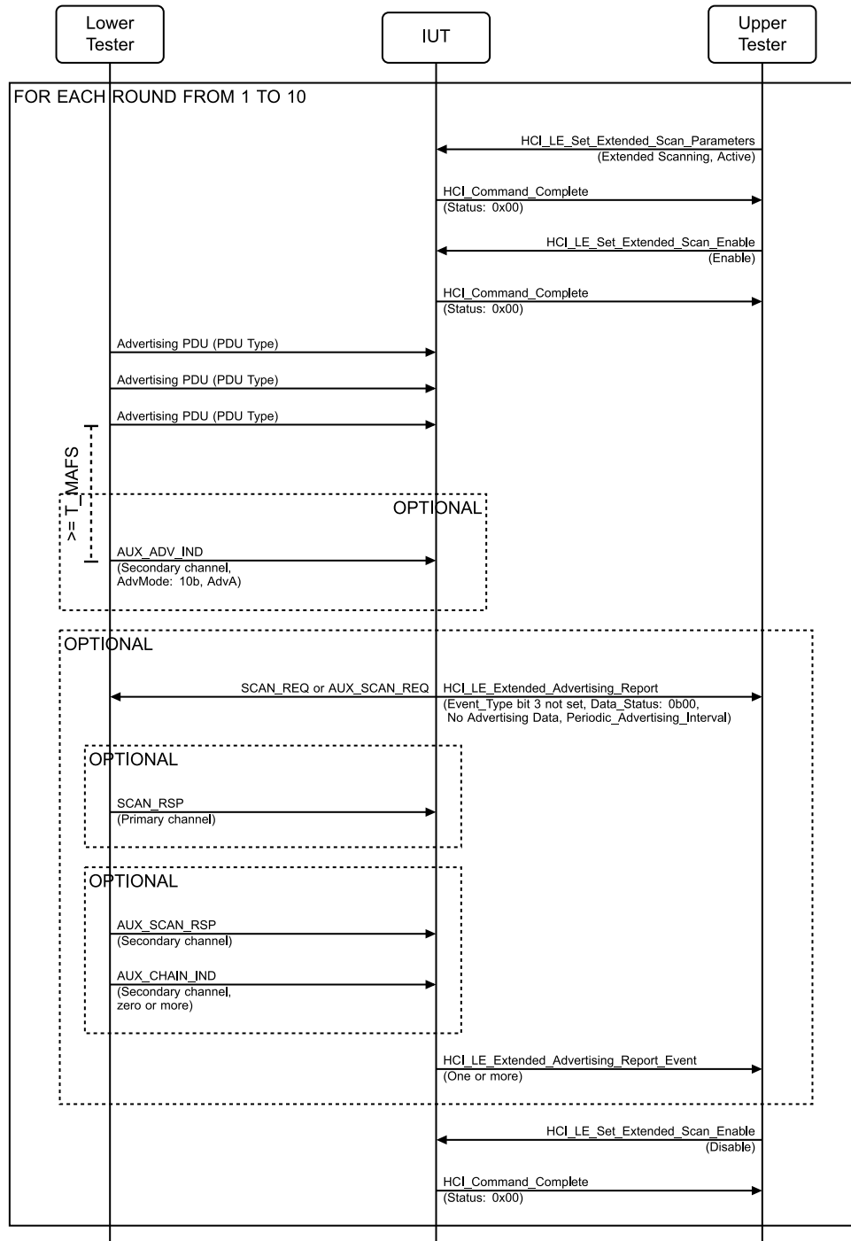
Figure 4.2-89: Extended Scanning, Active MSC
