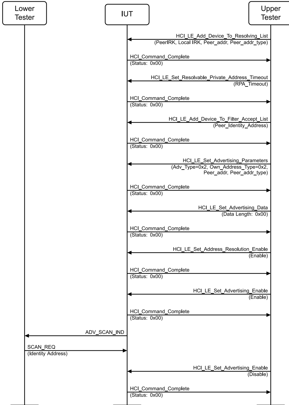
Figure 4.8-15: LL/SEC/ADV/BV-15-C [Network Privacy - Scannable Advertising, resolvable private address, Ignore Identity Address] MSC
