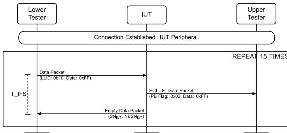
Figure 4.3-63: LL/CON/PER/BV-21-C [Peripheral Acknowledgement Scheme] MSC
