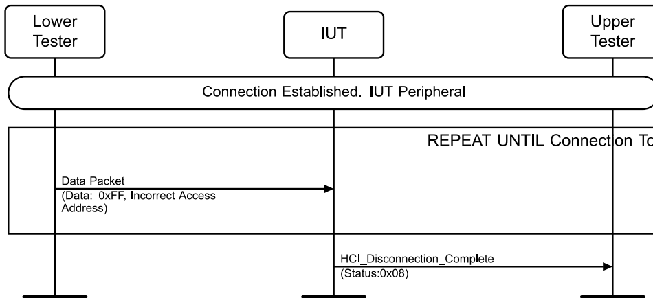
Figure 4.5-6: LL/ENC/PER/BI-01-C [Packets to another Peripheral] MSC
