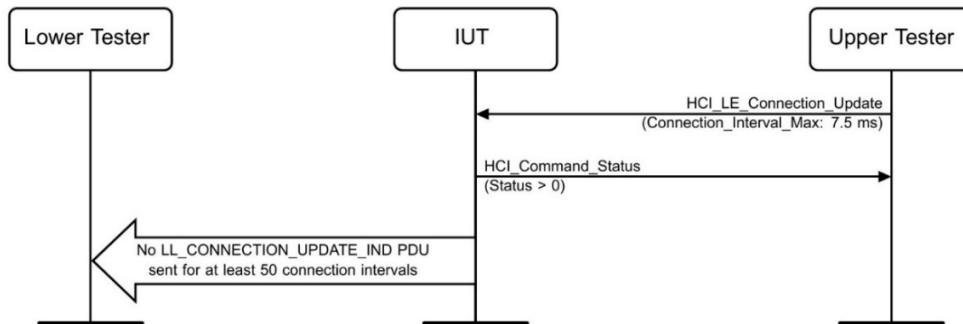
Figure 4.4-43: Frame Space Change, Connection Update, insufficient time MSC
