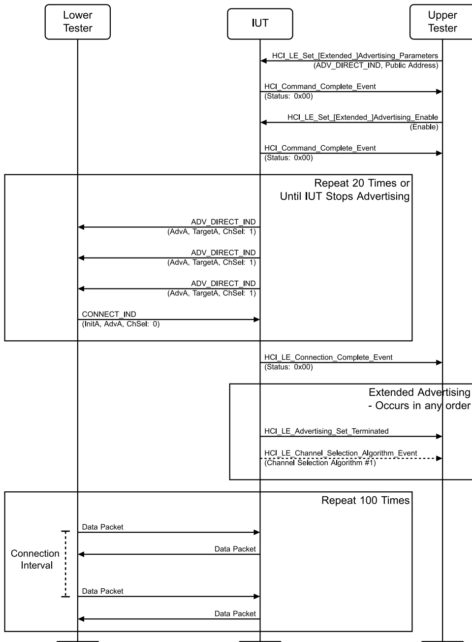
Figure 4.3-10: Directed Advertising Connection, Channel Selection Algorithm #1 MSC
