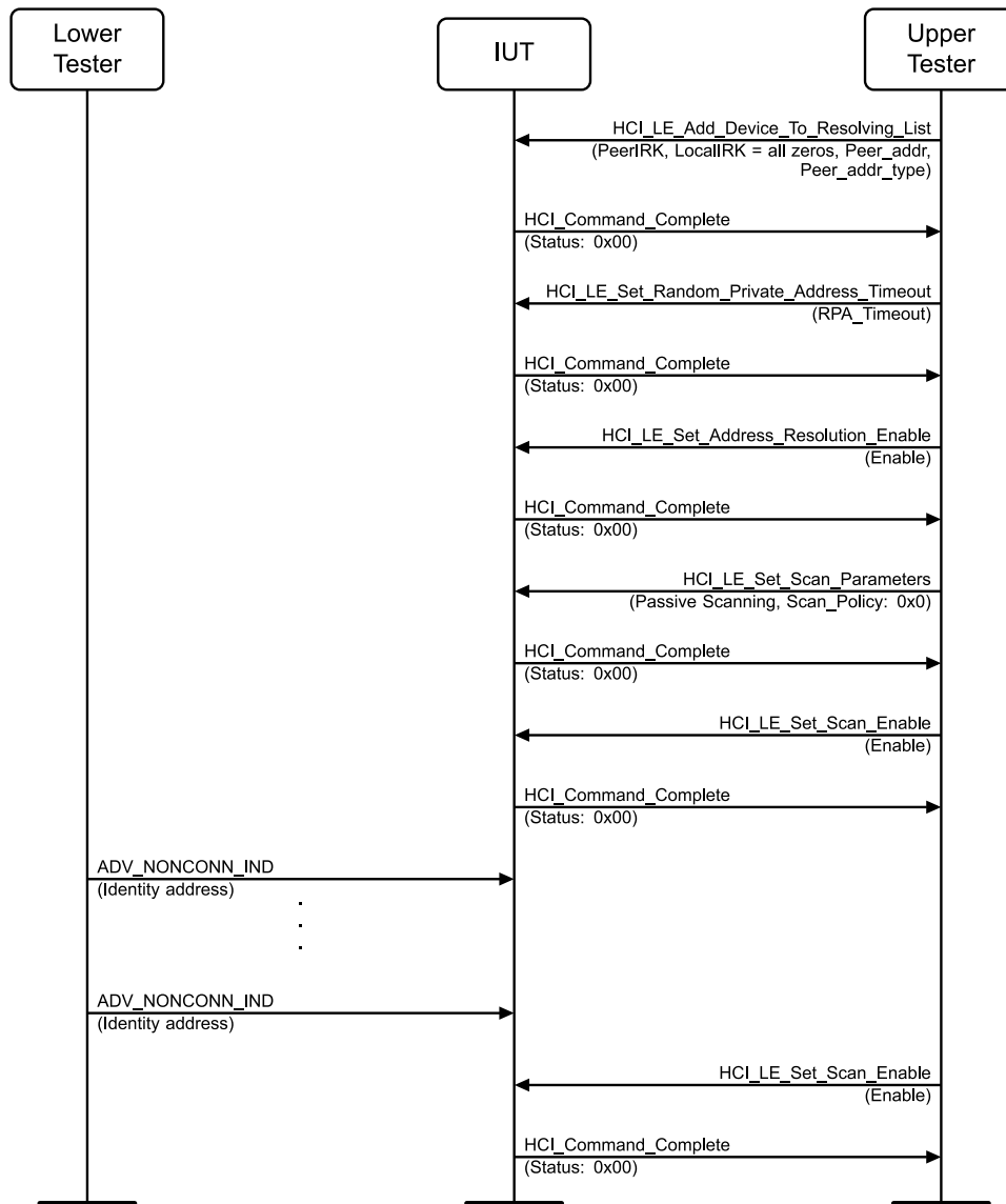
Figure 4.2-99: Network Privacy – Passive Scanning, Peer IRK MSC
