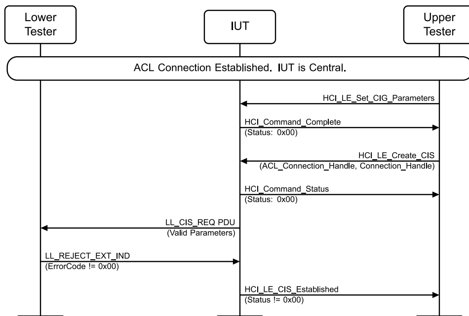
Figure 4.10-3: LL/CIS/CEN/BV-03-C [CIS Setup Procedure, Central Initiated, Rejected] MSC
