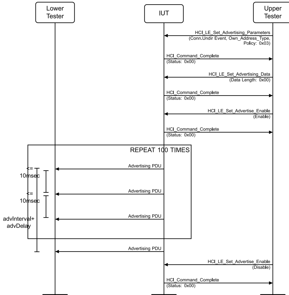
Figure 4.2-1: Non-Connectable or Undirected Advertising Events MSC
