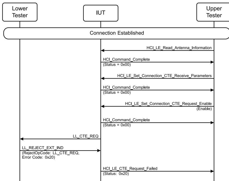
Figure 4.3-235: Constant Tone Extension Request Procedure, IUT Initiated, Responses Disabled MSC
