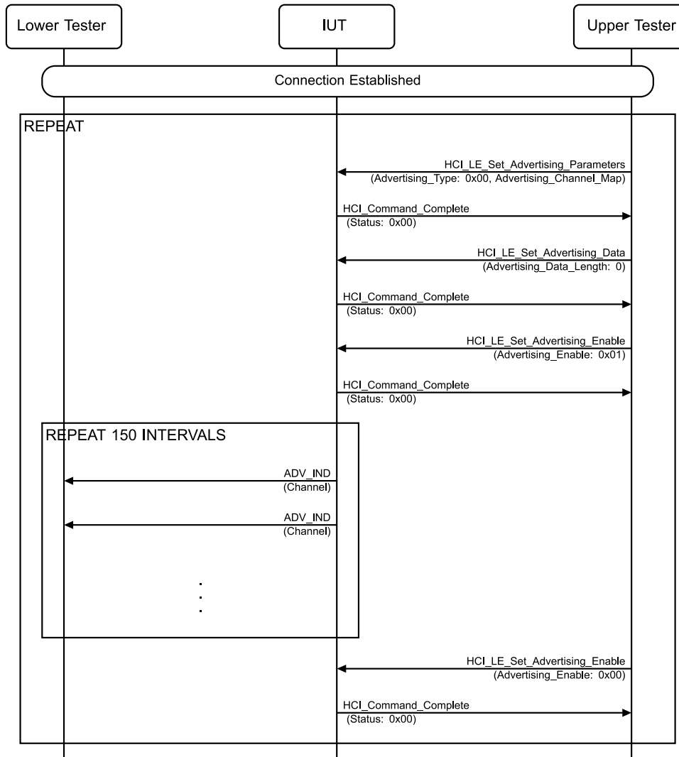
Figure 4.2-75: LL/DDI/ADV/BV-106-C [Advertising on Selected Channels] MSC
