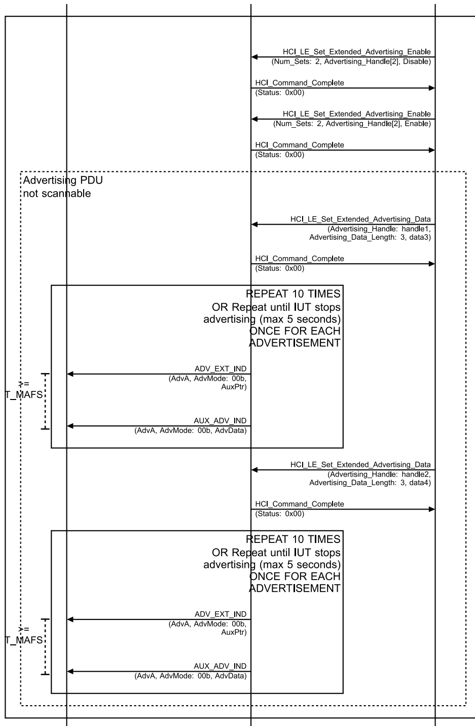
Figure 4.2-58: Extended Advertising, Multiple Sets, New RPA on AdvData Change MSC – Page 3 of 4
