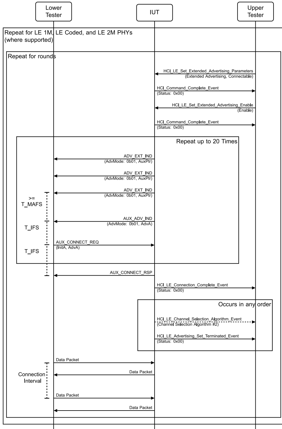
Figure 4.3-15: Extended Advertising, Accepting Connections MSC – Page 1 of 2
