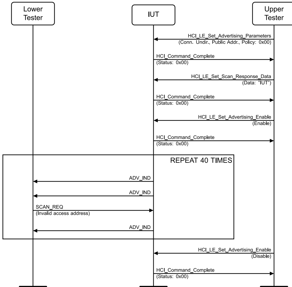
Figure 4.5-1: LL/ENC/ADV/BI-01-C [Scan Request Invalid Address] MSC
