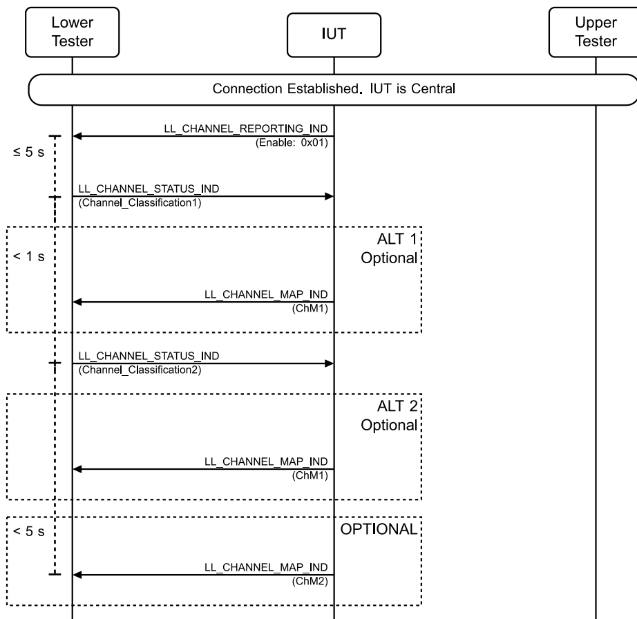
Figure 4.6-9: LL/FRH/CEN/BI-02-C [Channel Classification Enabled, Packets Received Less than Min_Spacing] MSC
