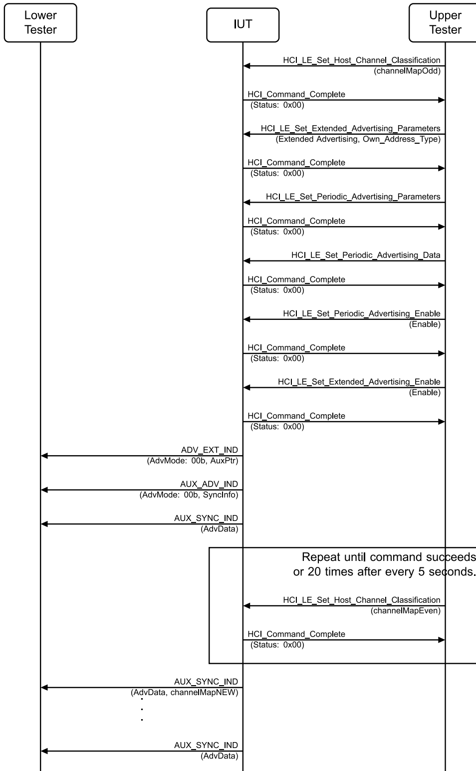
Figure 4.2-45: LL/DDI/ADV/BV-62-C [Periodic Advertising, Channel Map Update] MSC
