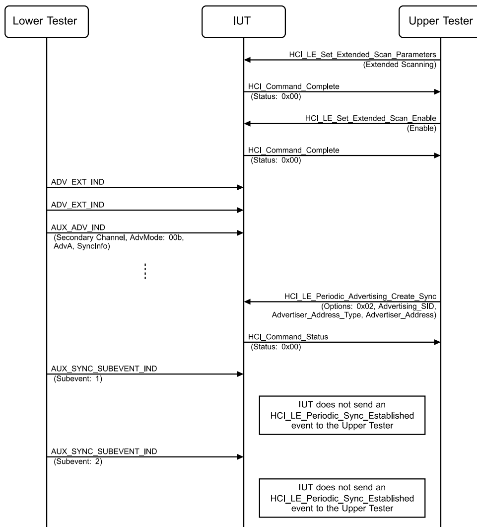
Figure 4.2-135: Ignore a Connection Request, Periodic Advertising with Responses Not Supported MSC – Page 1 of 2
