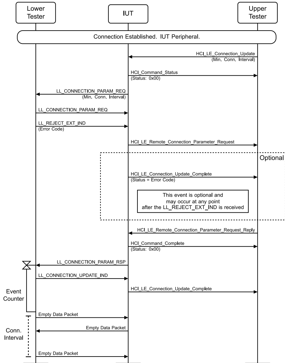
Figure 4.3-68: LL/CON/PER/BV-26-C [Initiating Connection Parameter Request – same procedure collision] MSC
