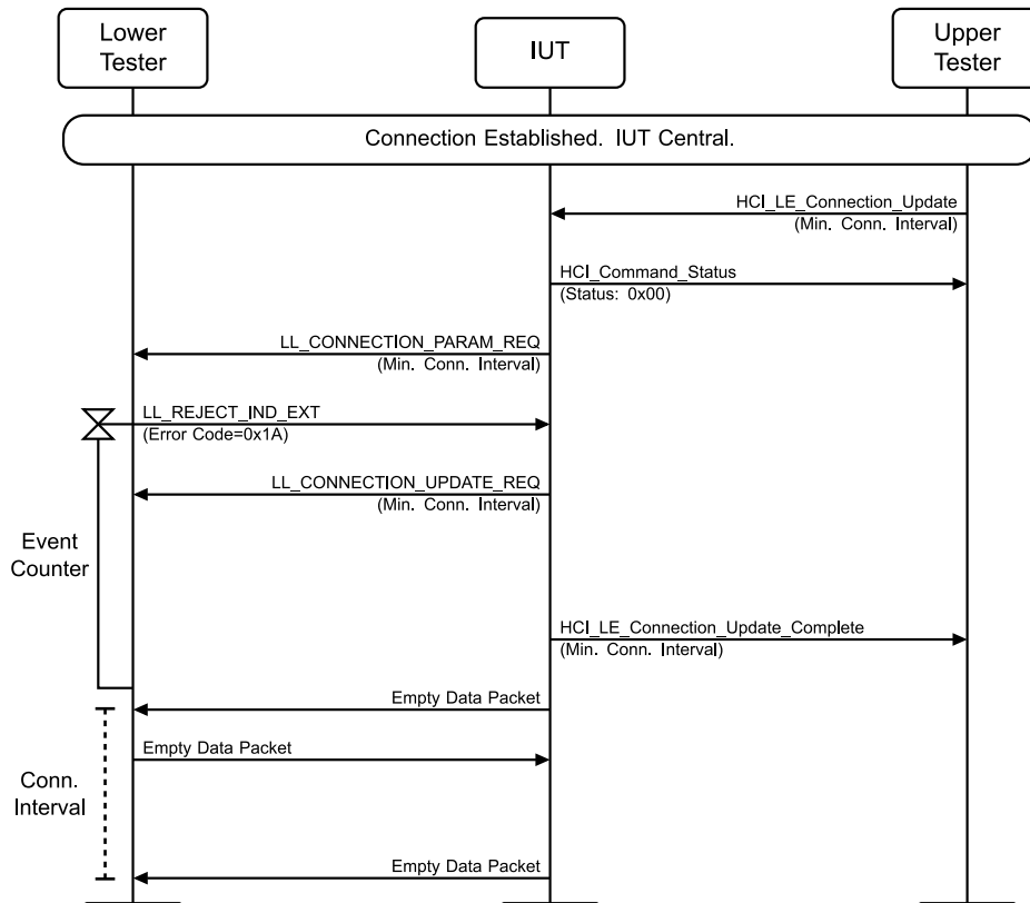
Figure 4.3-159: LL/CON/CEN/BV-29-C [Initiating Connection Parameter Request – remote legacy Host] MSC
