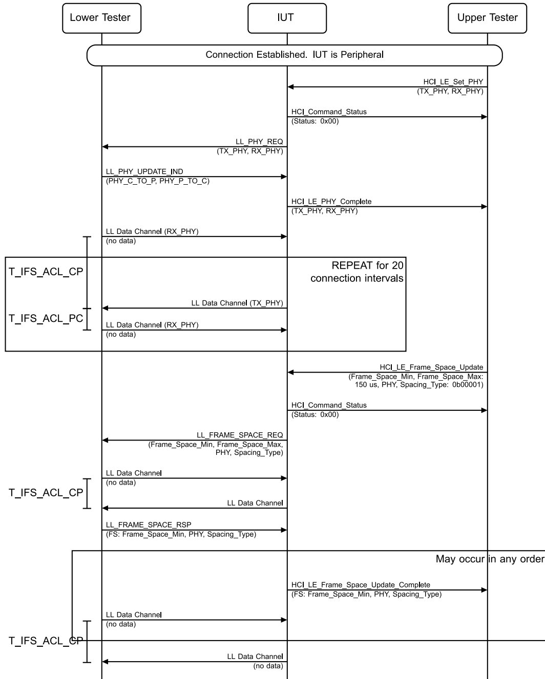
Figure 4.4-15: Initiate Inter Frame Space Change in the current ACL connection, Asymmetric PHYs, Peripheral MSC – Page 1 of 2
