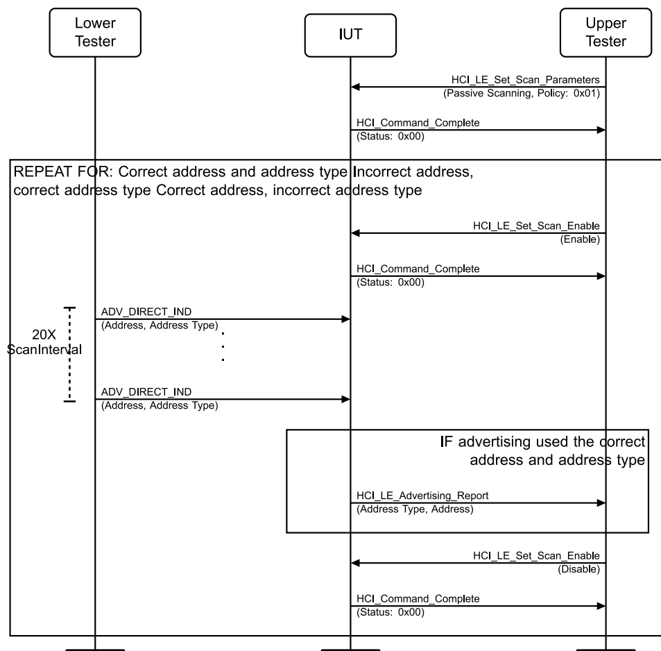
Figure 4.2-82: LL/DDI/SCN/BV-11-C [Passive Scanning: Directed events] MSC
