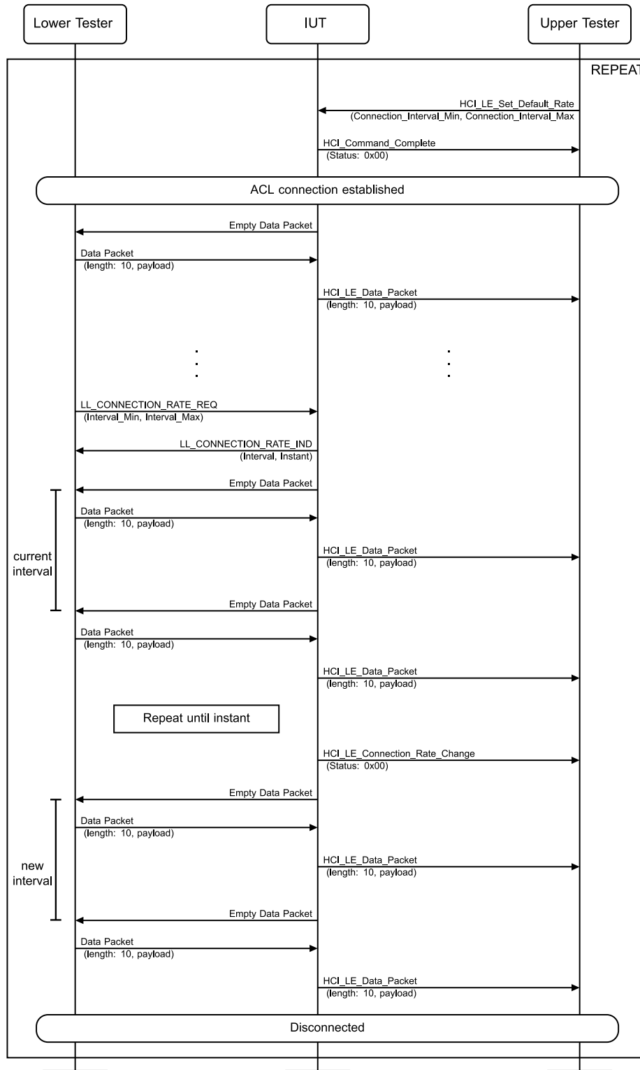
Figure 4.3-209: LL/CON/CEN/BV-175-C [Connection Rate Update, Central, Peer initiated] MSC
