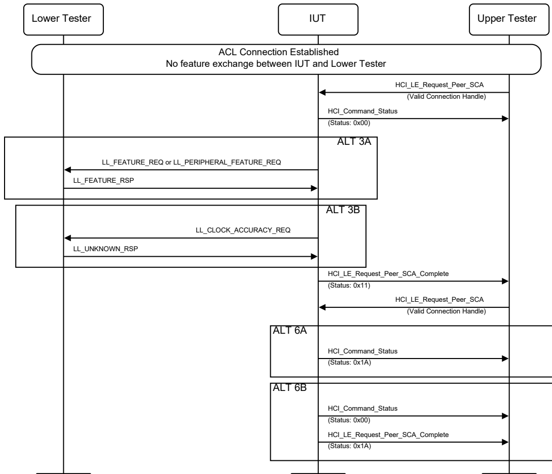
Figure 4.10-55: Error Updating Peer_Clock_Accuracy MSC
