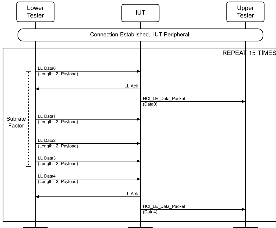
Figure 4.3-124: LL/CON/PER/BV-142-C [Listen for Data on Subrated events] MSC
