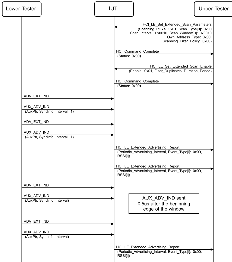
Figure 4.2-154: Extended Scanning, Passive, Periodic Advertising Report, Window Widening – Page 1 of 2
