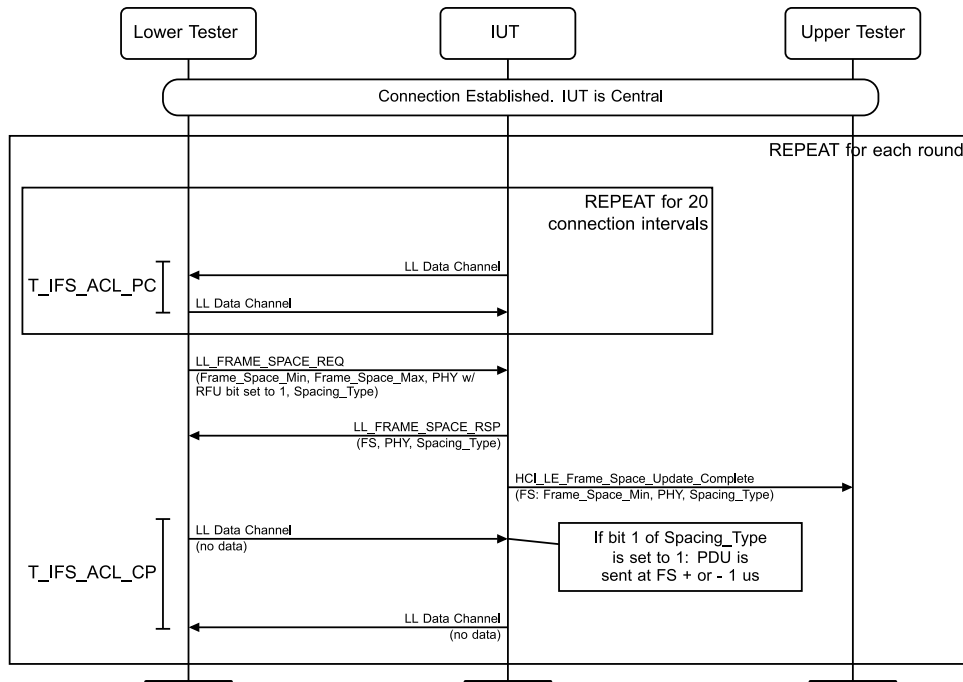
Figure 4.4-35: Respond to Inter Frame Space Change Request in the current ACL connection, Central MSC
