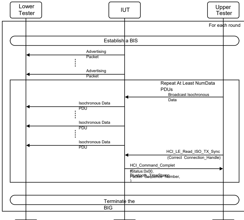
Figure 4.11-4: LL/BIS/BRD/BV-08-C [Pre-transmissions in Broadcast Isochronous Stream] MSC
