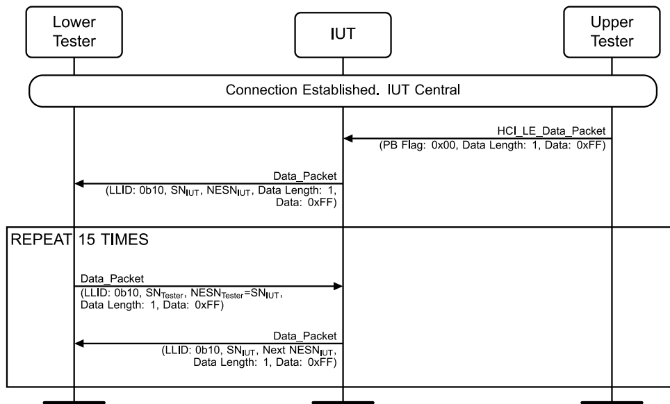
Figure 4.3-144: LL/CON/CEN/BV-15-C [Central Retransmission] MSC
