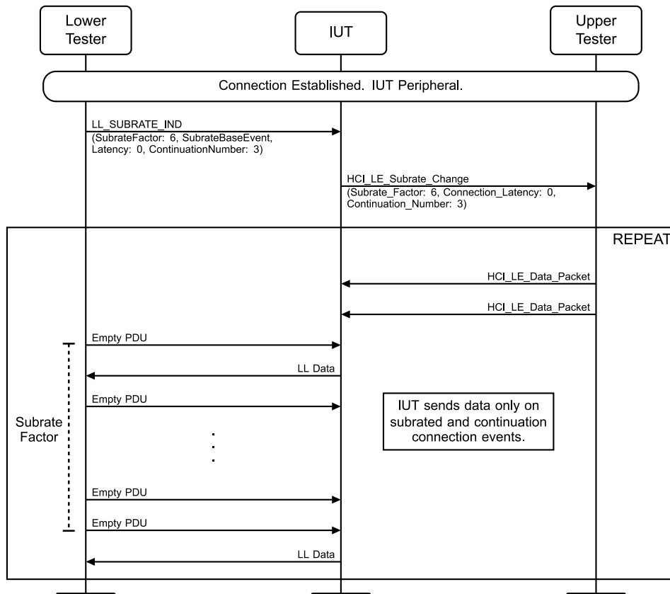
Figure 4.3-117: LL/CON/PER/BV-141-C [Subrate Change, Verify Continuation Number events] MSC
