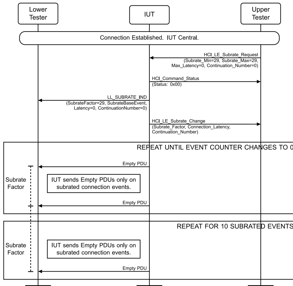
Figure 4.3-203: LL/CON/CEN/BV-141-C [Subrate Factor, Event Counter Wrapping] MSC
