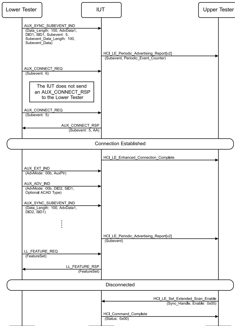
Figure 4.2-128: Synchronized Device Reconnects with an Advertiser using Periodic Advertising with Responses MSC – Page 2 of 2
