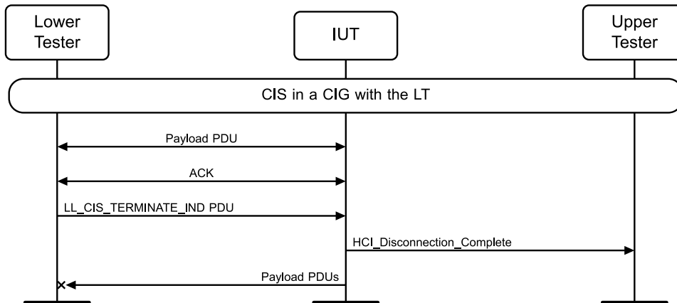
Figure 4.10-53: CIS Terminate Procedure, Accepting MSC
