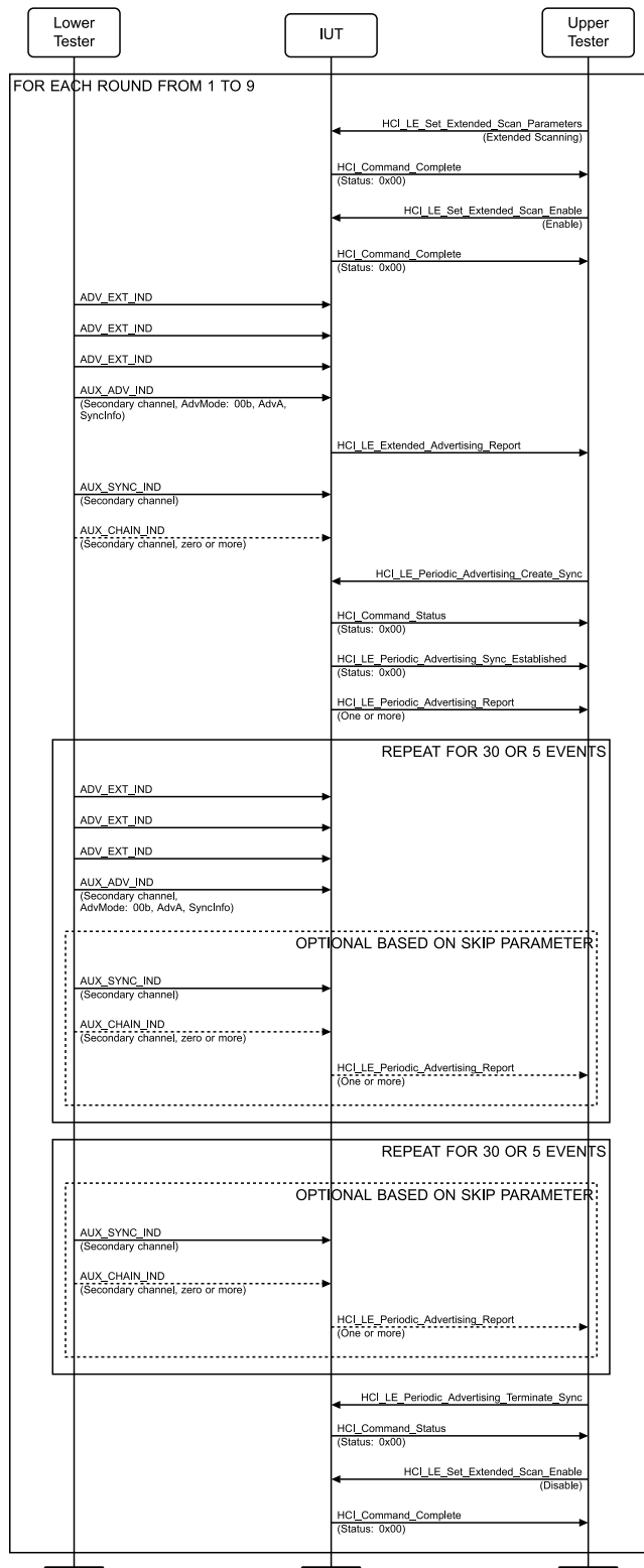
Figure 4.2-95: Extended Scanning, Periodic Advertising Reception MSC
