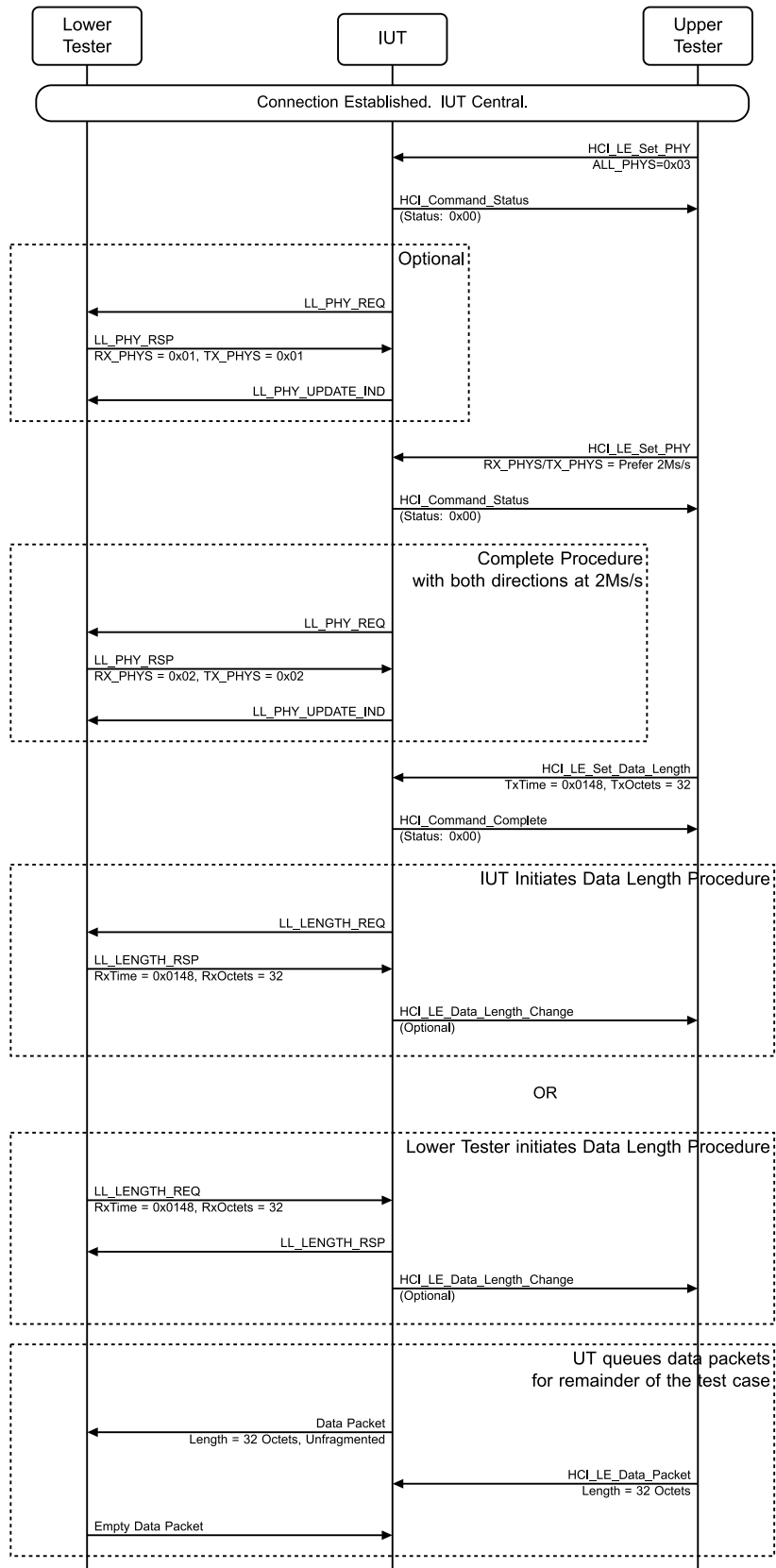
Figure 4.3-173: LL/CON/CEN/BV-50-C [Responding to PHY Update Procedure – Packet Time Restrictions] MSC – Page 1 of 2
