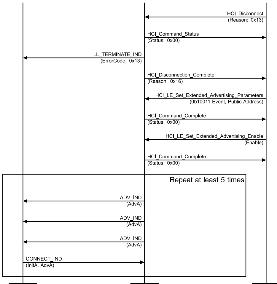
Figure 4.3-8: LL/CON/ADV/BV-06-C [Extended Advertising, Legacy PDUs, Accepting Connections] MSC – Page 2 of 2
