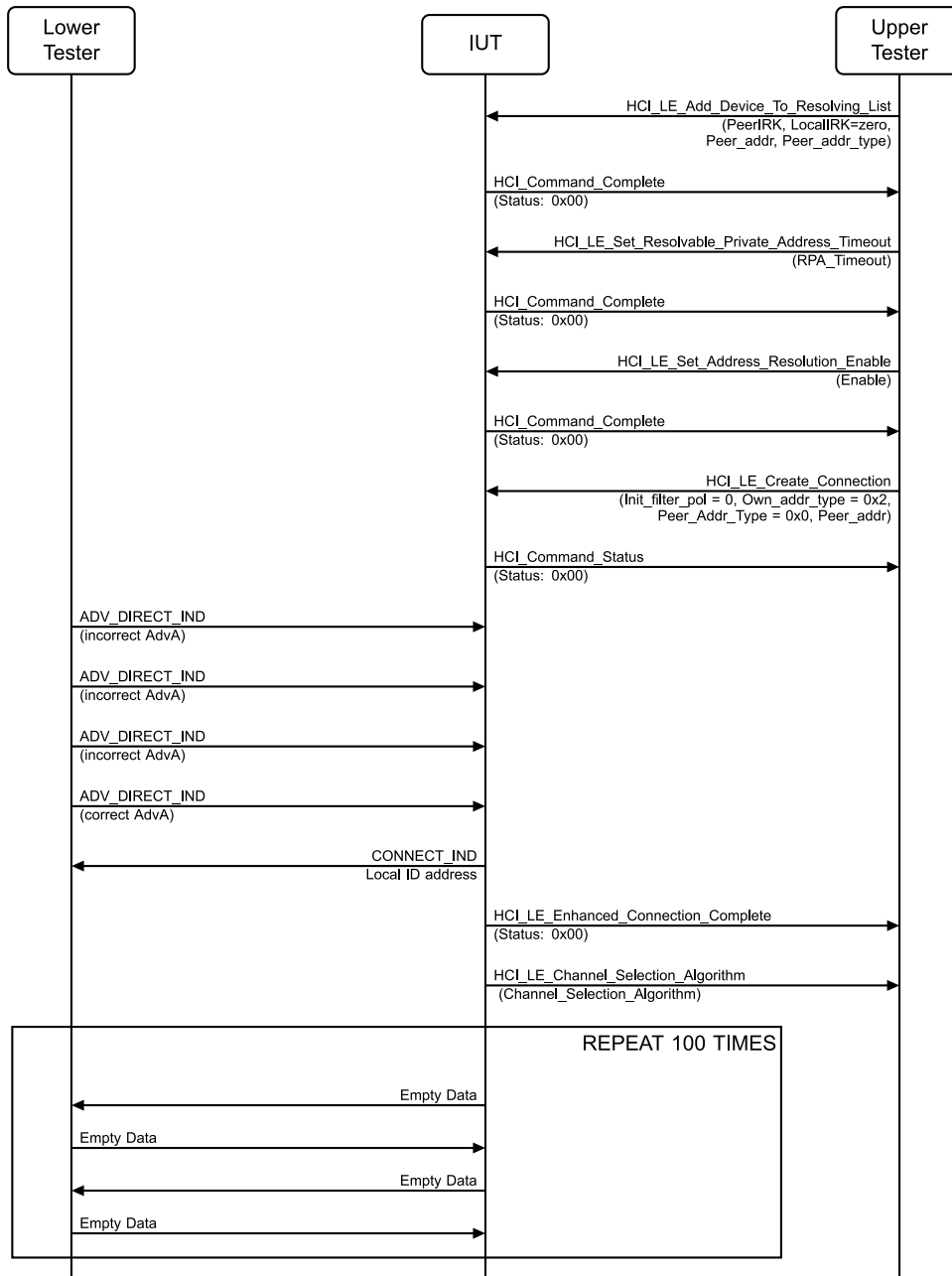
Figure 4.3-28: Network Privacy – Connection Establishment using directed advertising and resolving list, Initiator MSC
