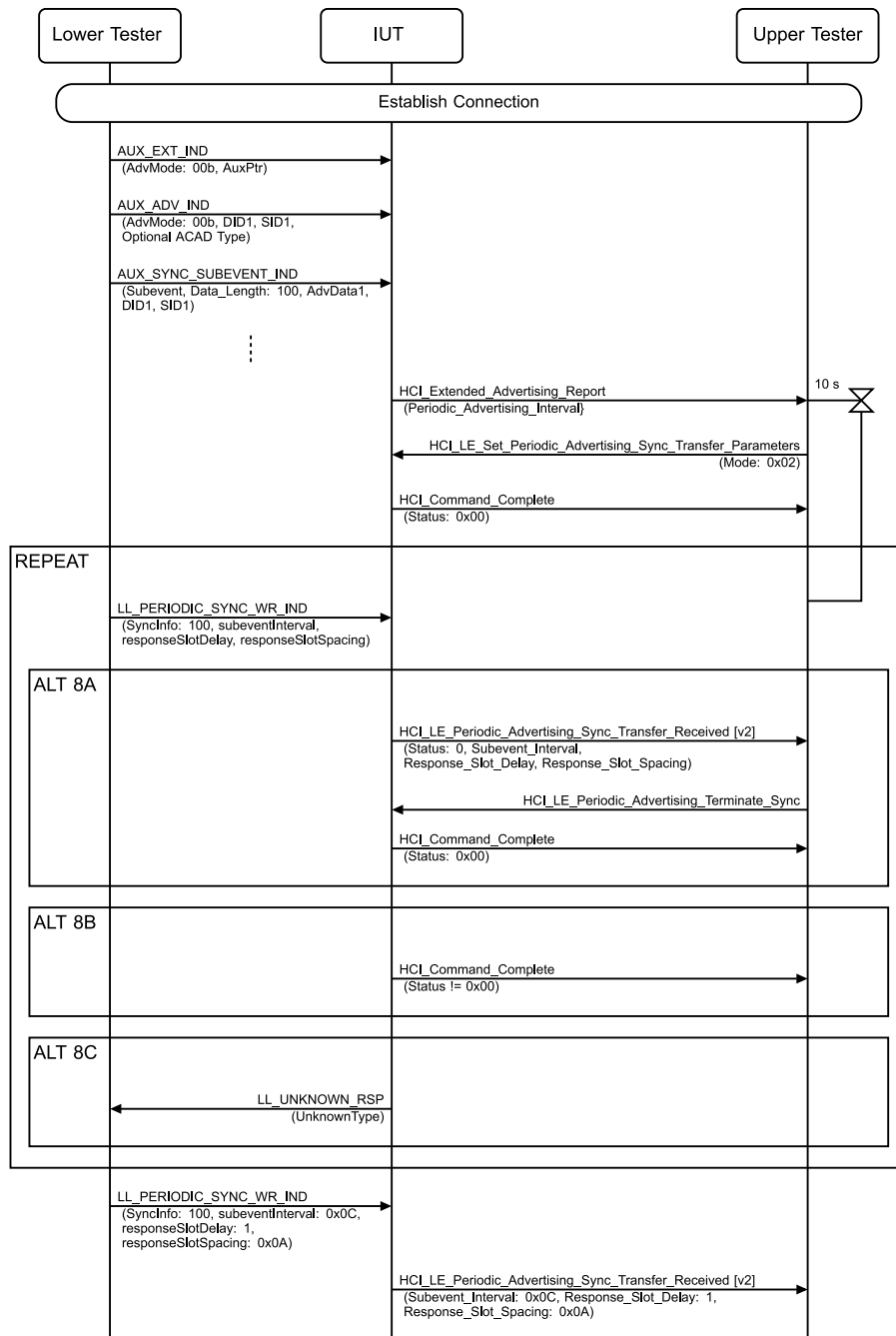
Figure 4.2-130: Periodic Advertising with Responses, Invalid Parameters MSC
