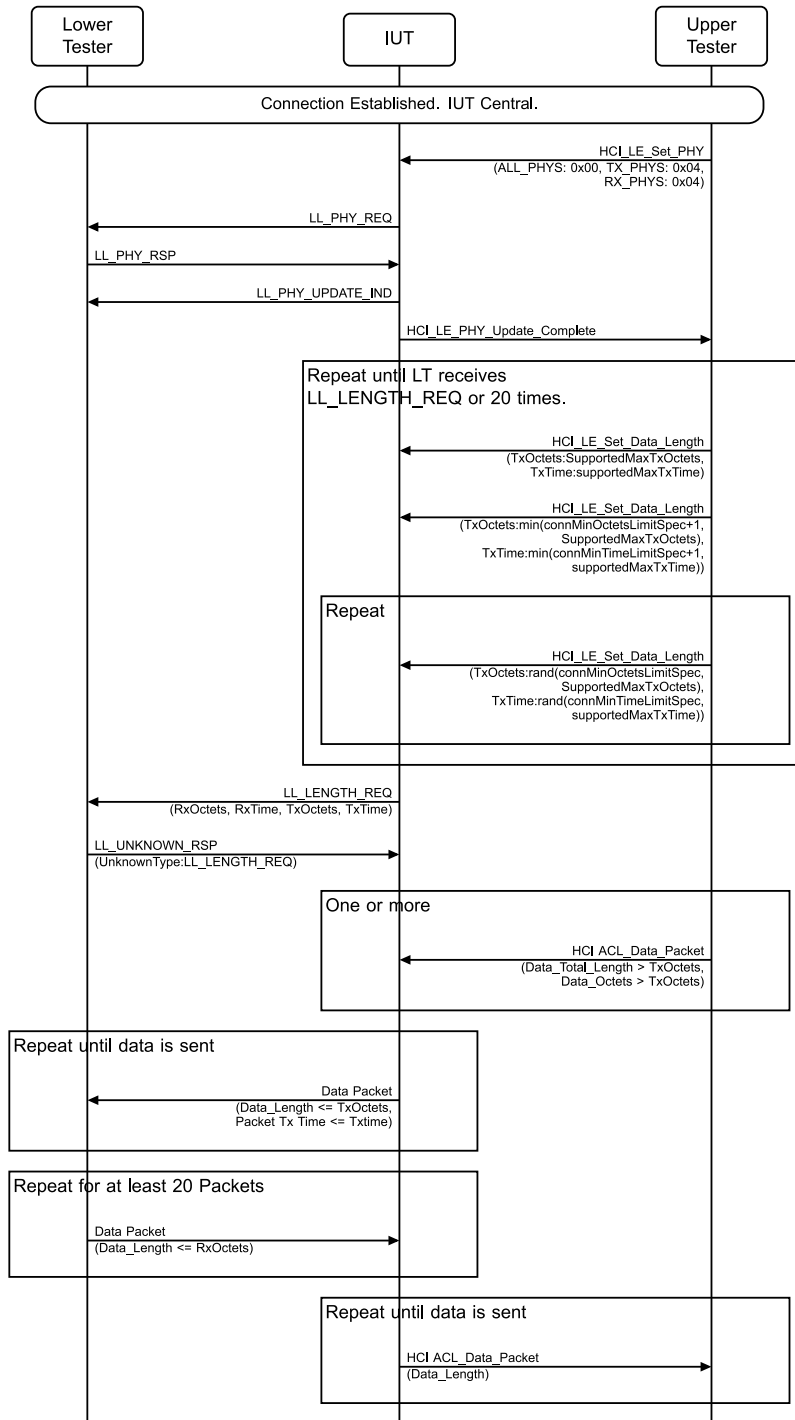
Figure 4.3-186: LL/CON/CEN/BV-80-C [Central Data Length Update – Peripheral does not support; LE Coded PHY] MSC
