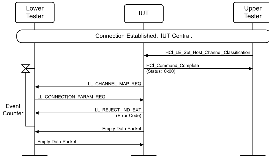
Figure 4.3-157: LL/CON/CEN/BV-27-C [Initiating Connection Parameter Request – different procedure collision – channel map update] MSC
