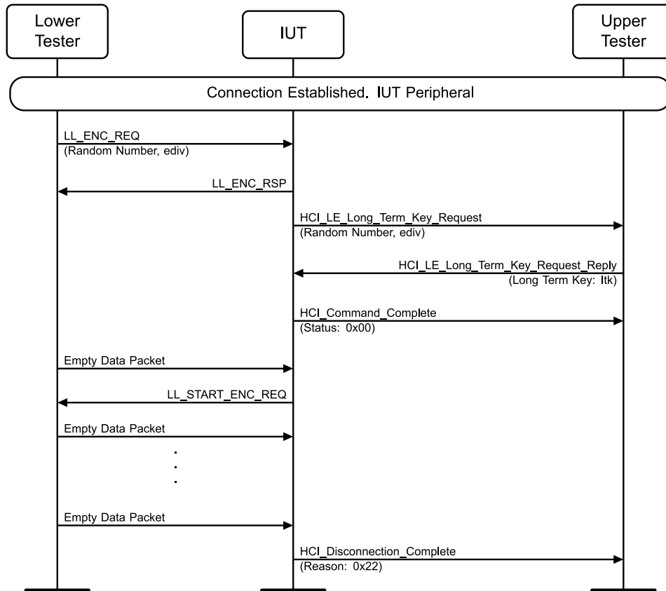
Figure 4.8-38: LL/SEC/PER/BI-01-C [Peripheral Encryption Setup: Missing Response] MSC
