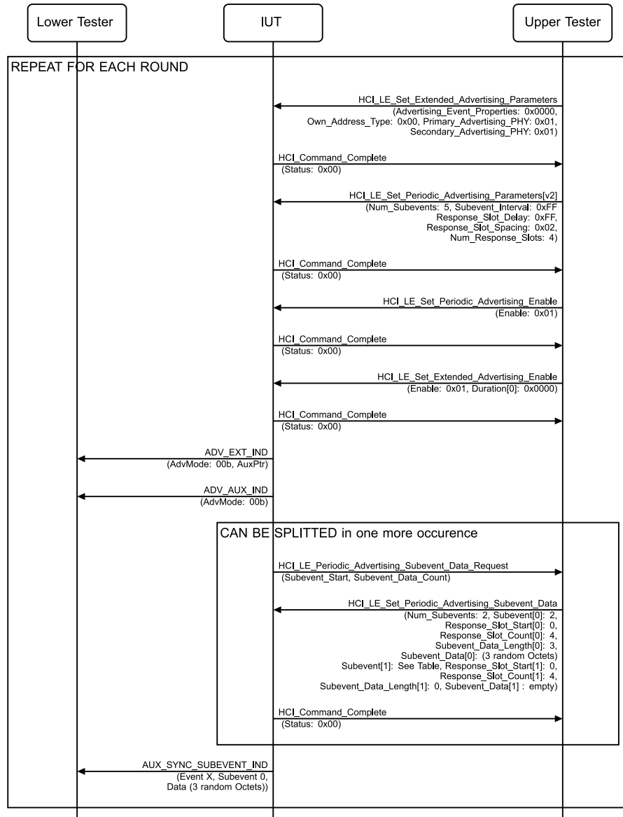
Figure 4.2-70: Receive Subevent Response Data in Future Subevent, Advertiser MSC – Page 1 of 2
