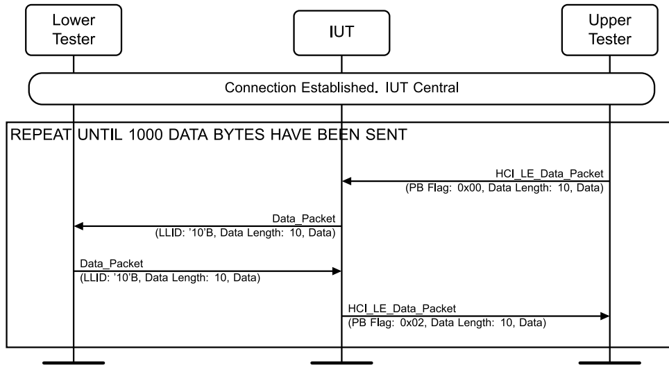
Figure 4.3-137: LL/CON/CEN/BV-05-C [Central Sending and Receiving Data] MSC
