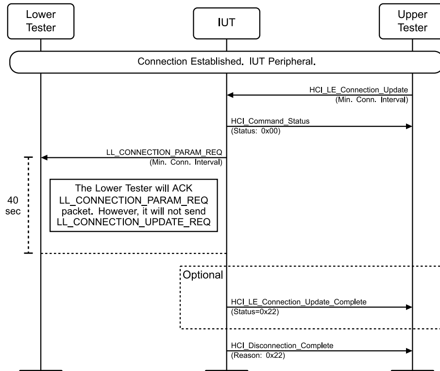
Figure 4.3-109: LL/CON/PER/BI-07-C [Initiating Connection Parameter Request – Timeout] MSC
