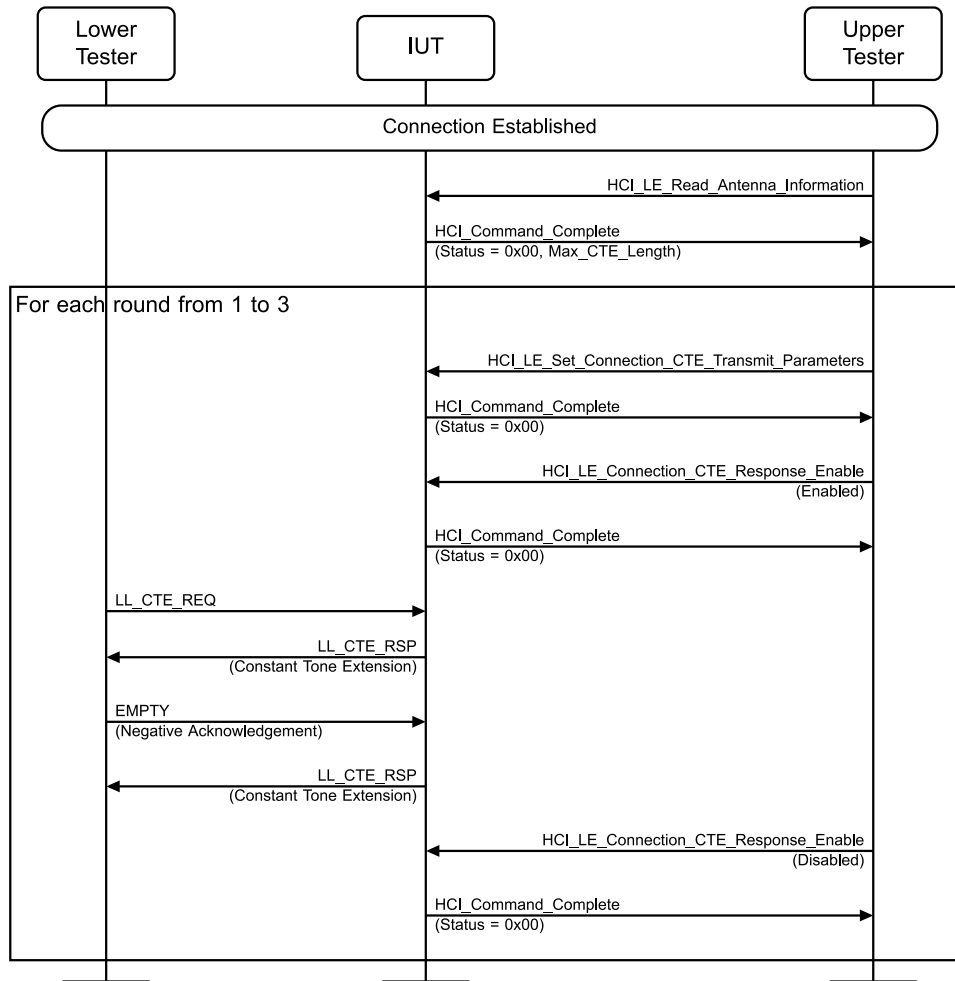
Figure 4.3-237: Constant Tone Extension Request Procedure, IUT Responding, AoA MSC
