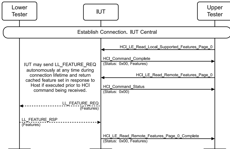
Figure 4.3-142: LL/CON/CEN/BV-13-C [Feature Setup Request] MSC
