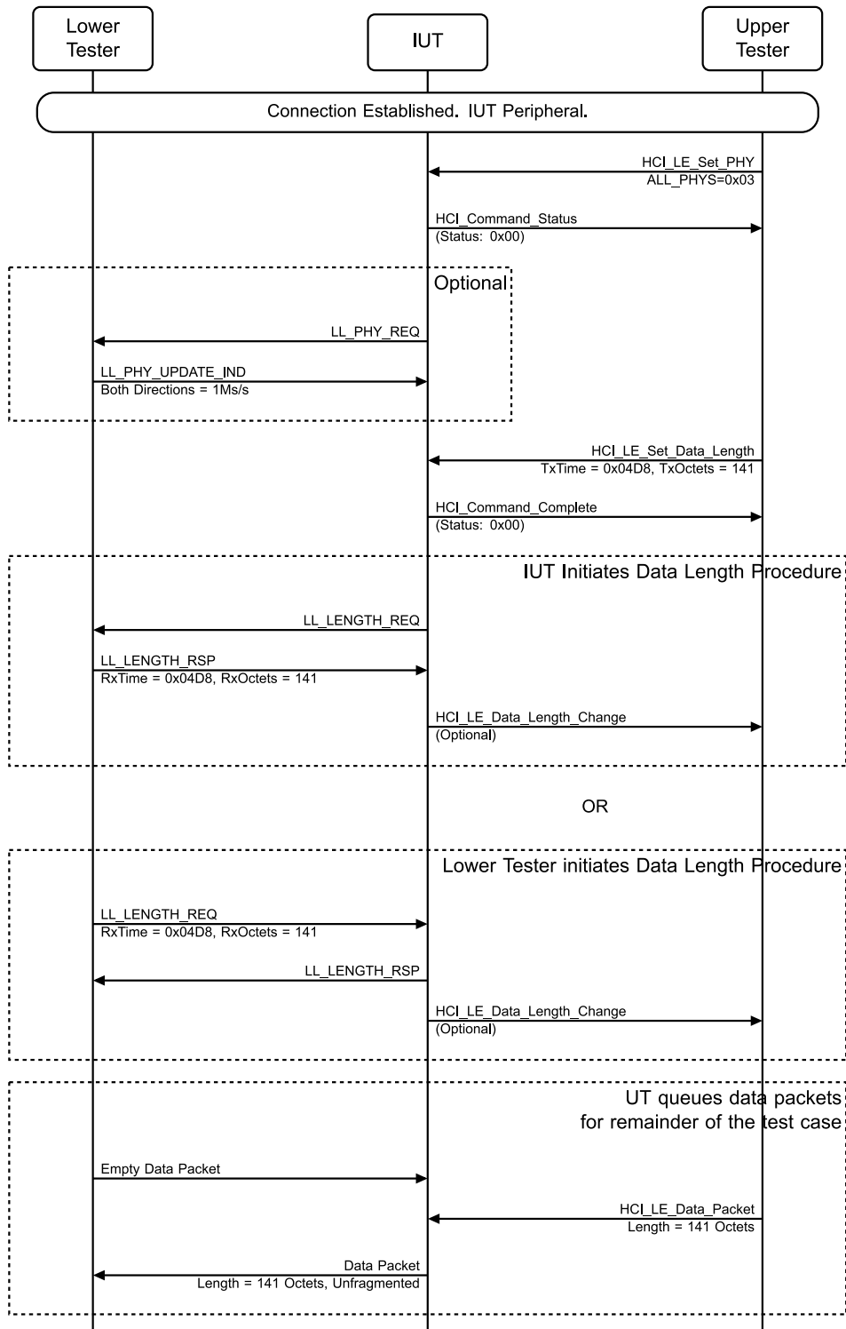
Figure 4.3-99: LL/CON/PER/BV-58-C [Initiating PHY Update Procedure – Packet Time Restrictions, No Change, LE Coded] MSC – Page 1 of 2
