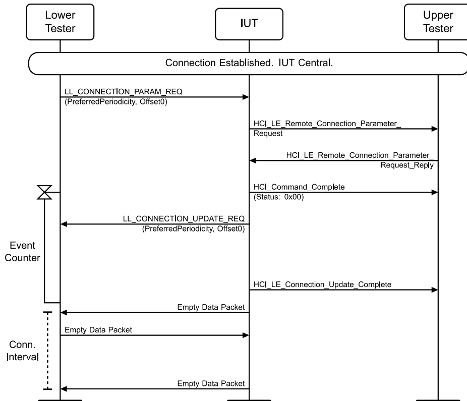
Figure 4.3-162: Accepting Connection Parameter MSC
