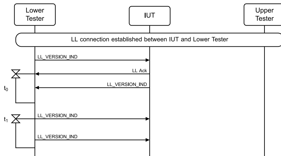
Figure 4.3-254: Version Exchange, IUT Responding MSC
