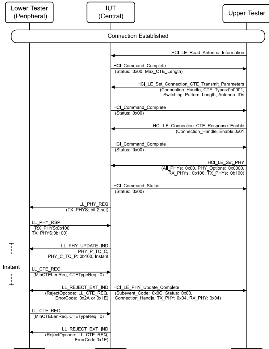
Figure 4.3-207: LL/CON/CEN/BV-150-C [Reject Constant Tone Extension Request Procedure for LE Coded PHY, IUT Responding, AoA, Central] MSC
