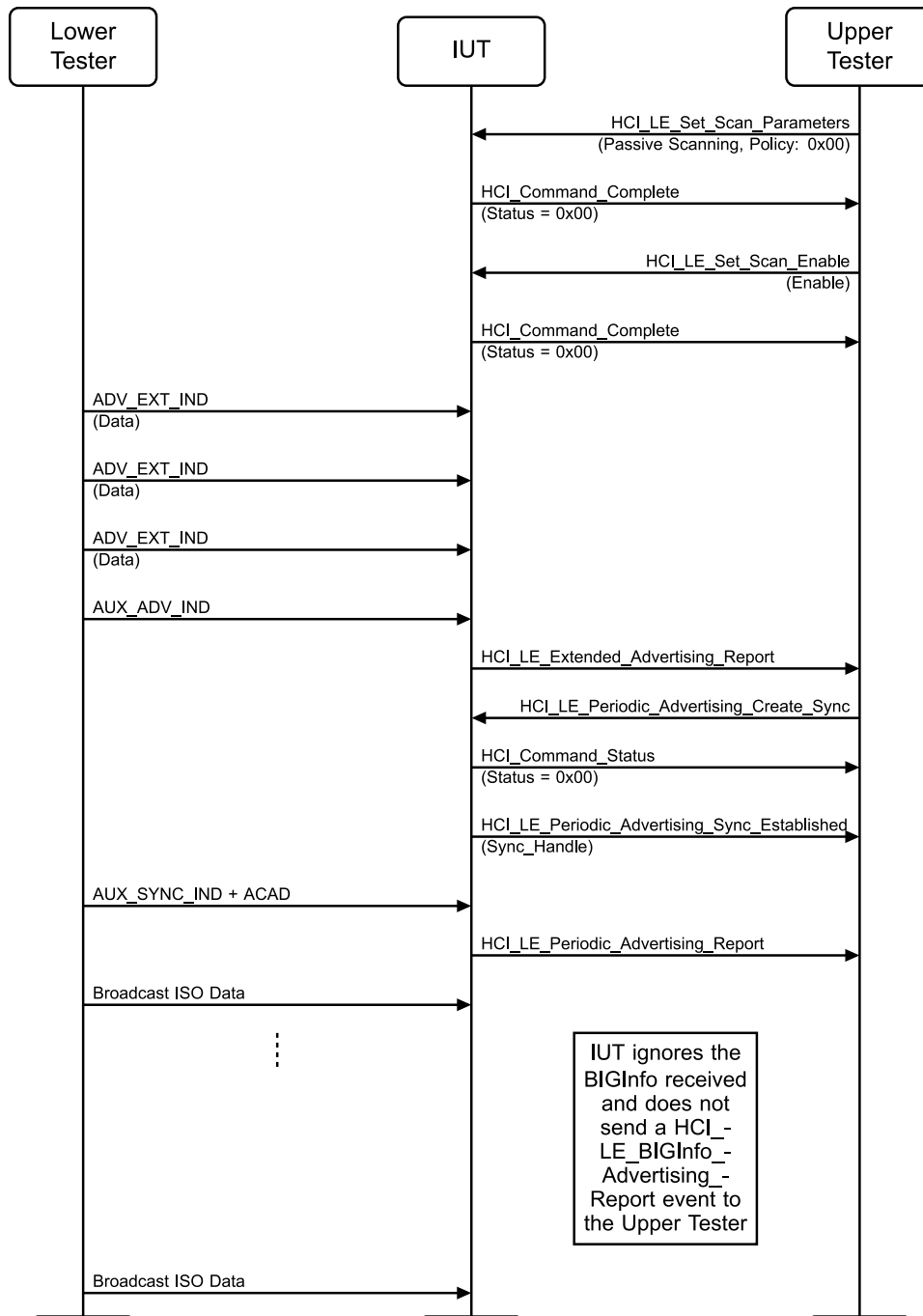
Figure 4.11-23: Broadcast Isochronous Stream Synchronization, Unsupported Features MSC
