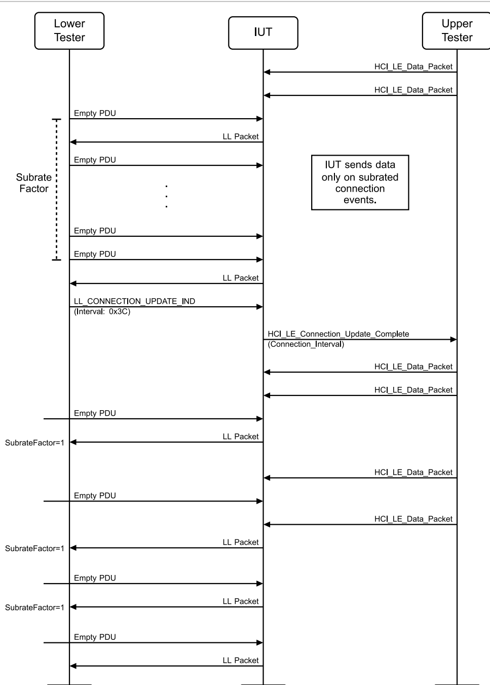
Figure 4.3-115: LL/CON/PER/BV-139-C [Subrate set to 1 and Continuation Number set to 0 on Connection Interval change] MSC – Page 2 of 2
