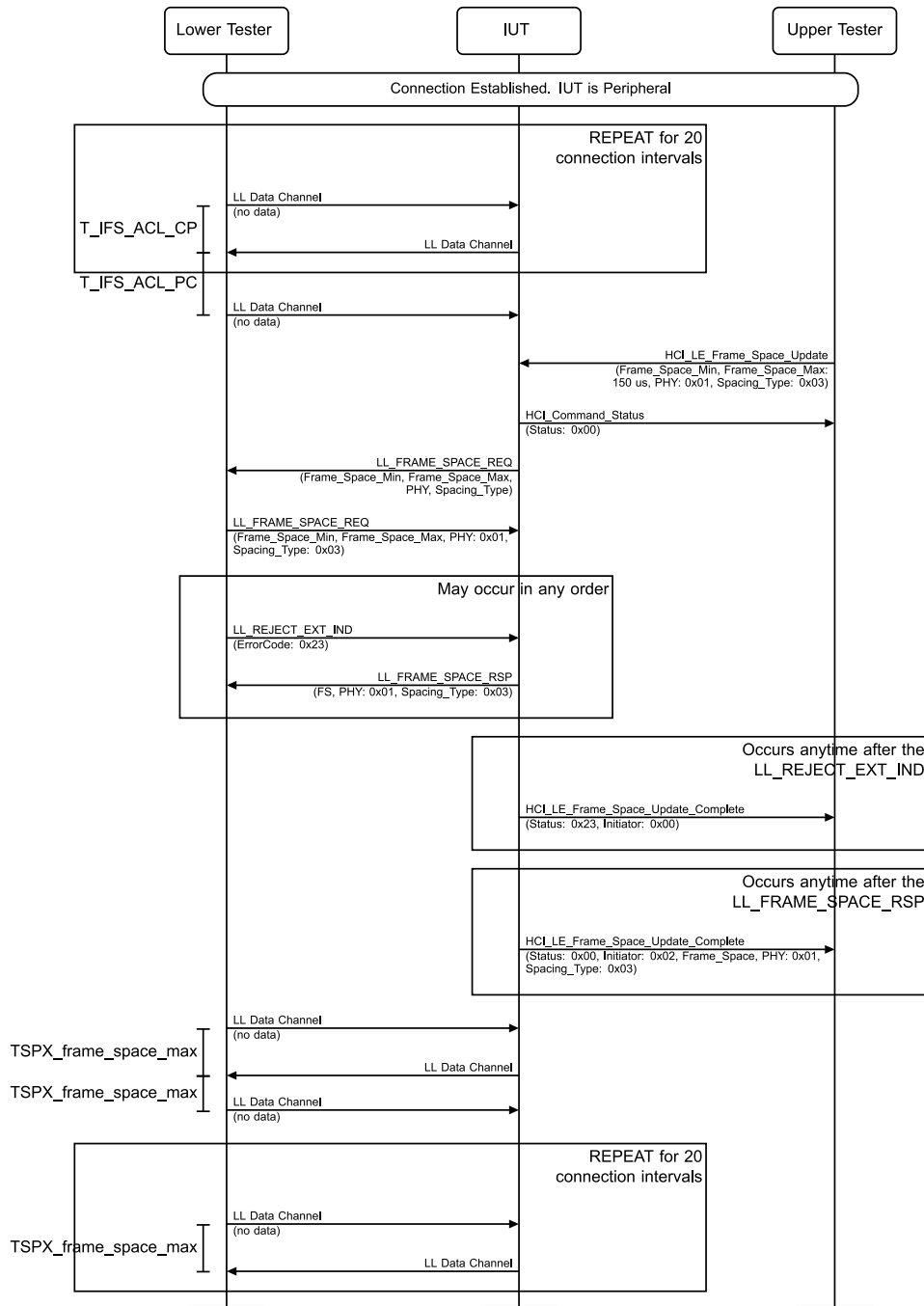
Figure 4.4-18: LL/TIM/PER/BV-27-C [Handling Frame Space Request Collision – Same Procedure, Peripheral] MSC
