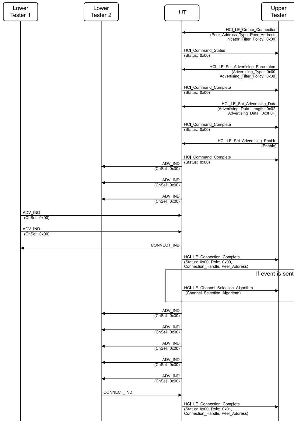
Figure 4.3-43: Parallel connection requests, outgoing connection request first MSC
