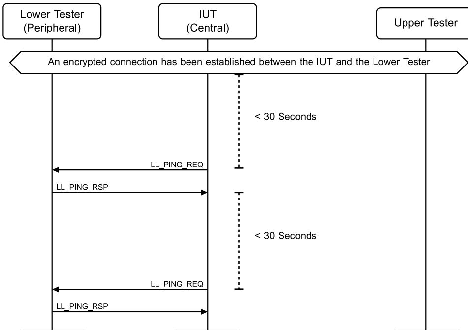
Figure 4.8-45: LL/SEC/CEN/BV-06-C [Initiate LE Ping procedure when encryption is enabled] MSC
