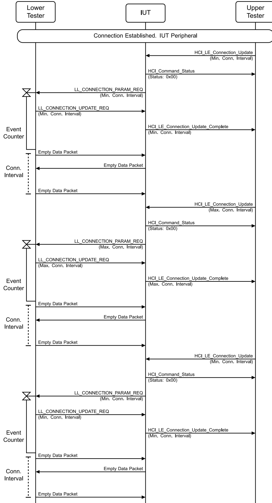
Figure 4.3-66: LL/CON/PER/BV-24-C [Initiating Connection Parameter Request – Accept] MSC
