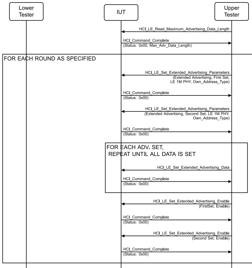
Figure 4.2-25: Extended Advertising, Multiple Sets, Single PHY, LE 1M PHY MSC – Page 1 of 2
