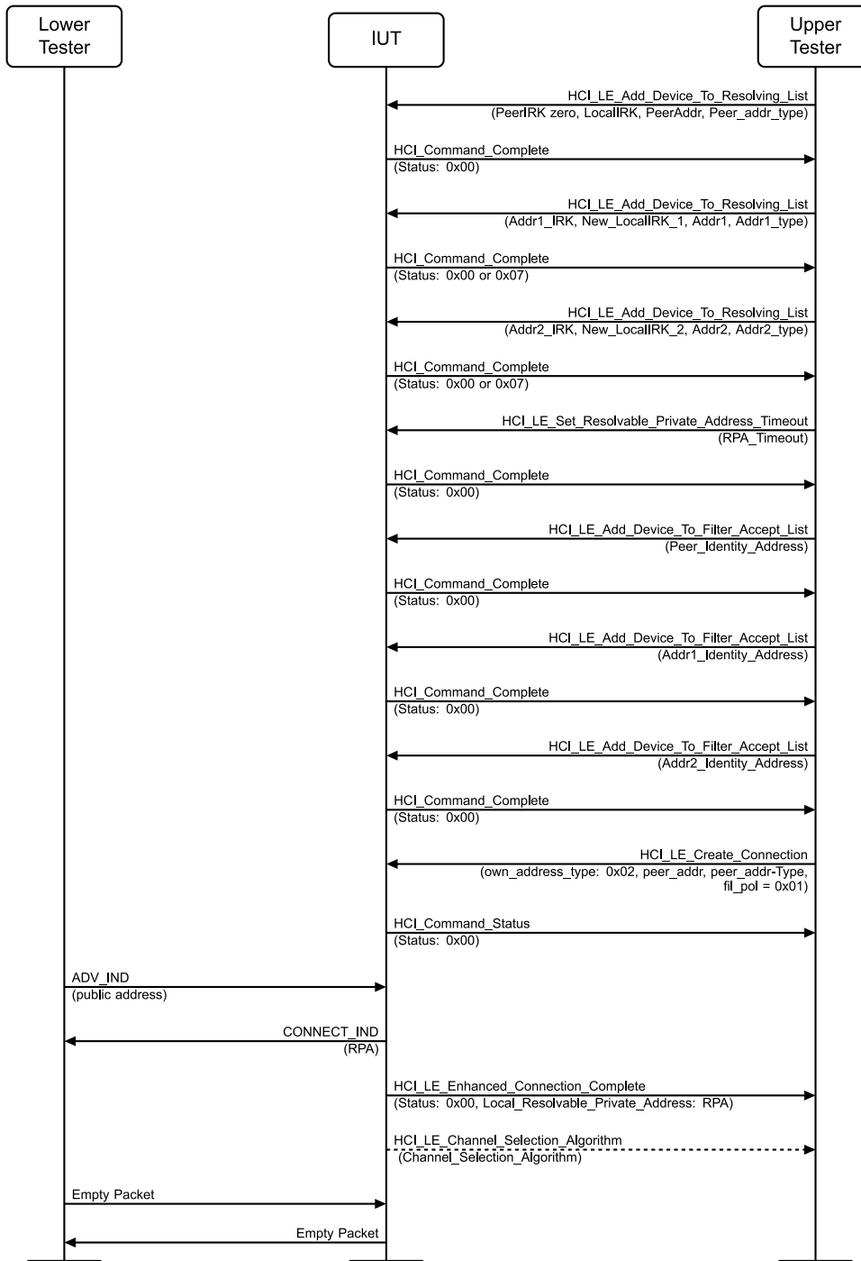
Figure 4.3-40: Network Privacy – Connection Establishment using Filter Accept List and resolving list with address resolution disabled MSC
