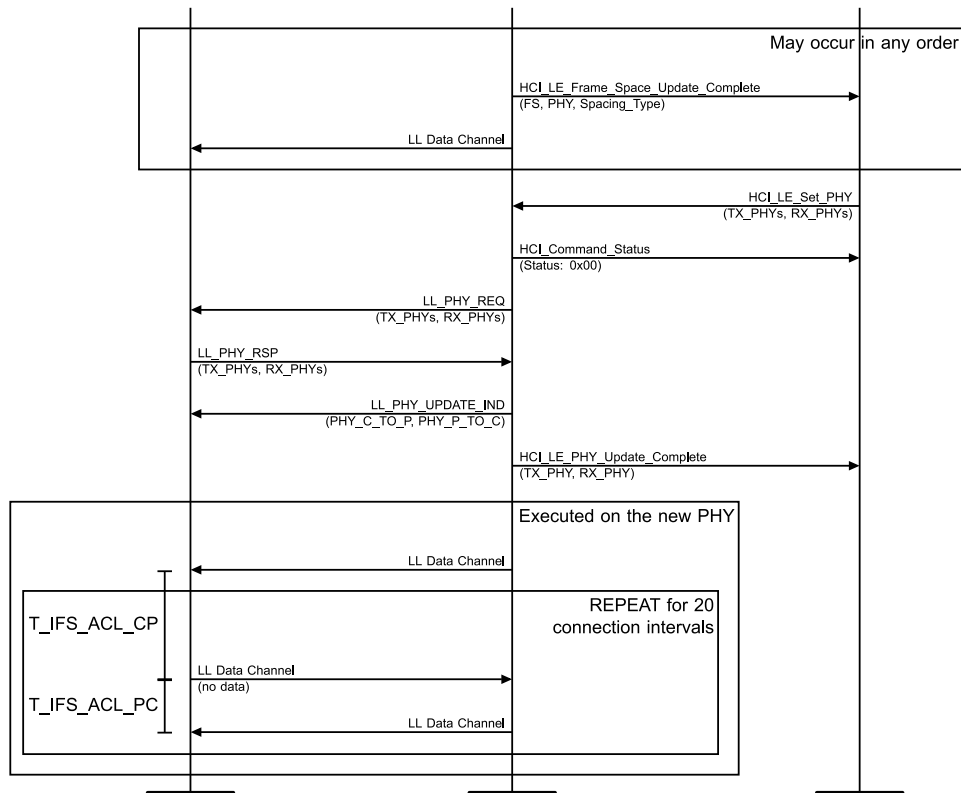
Figure 4.4-38: Initiate Inter Frame Space Change on a Different PHY, Central MSC – Page 2 of 2
