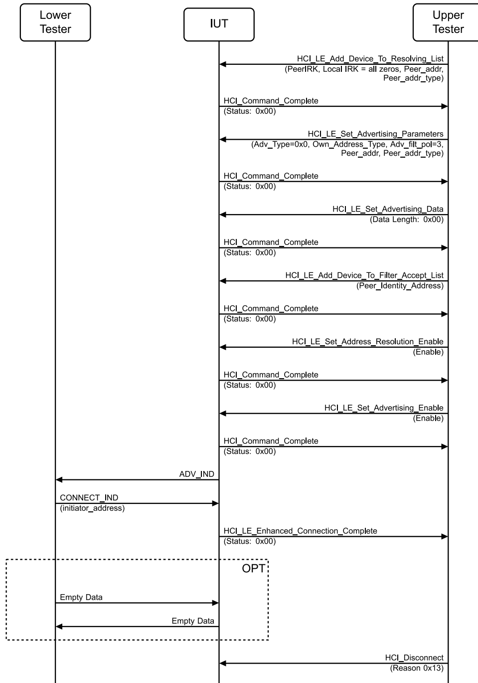
Figure 4.8-9: LL/SEC/ADV/BV-09-C [Network Privacy - Undirected Connectable Advertising without Local IRK and with peer IRK] MSC
