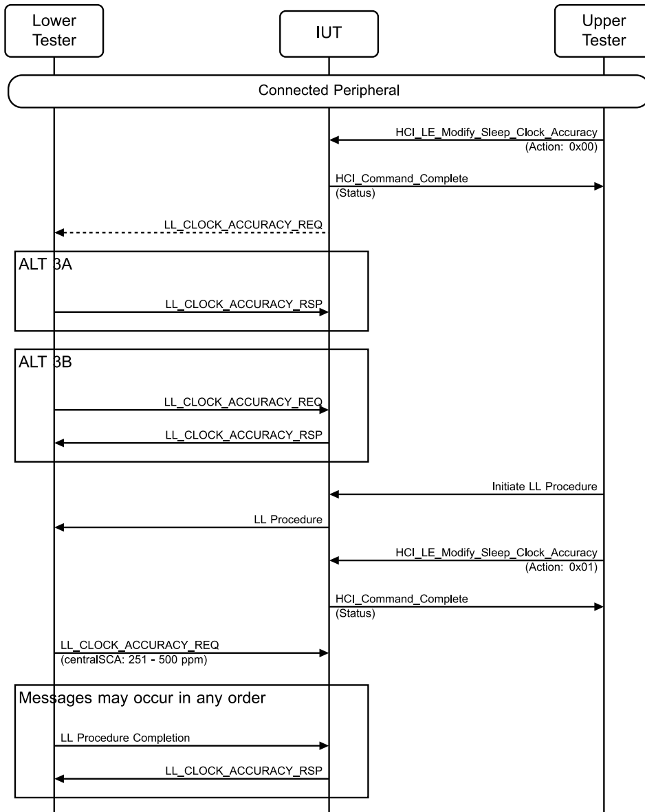
Figure 4.4-12: LL/TIM/PER/BV-10-C [Response without Reducing the Sleep Clock Accuracy] MSC
