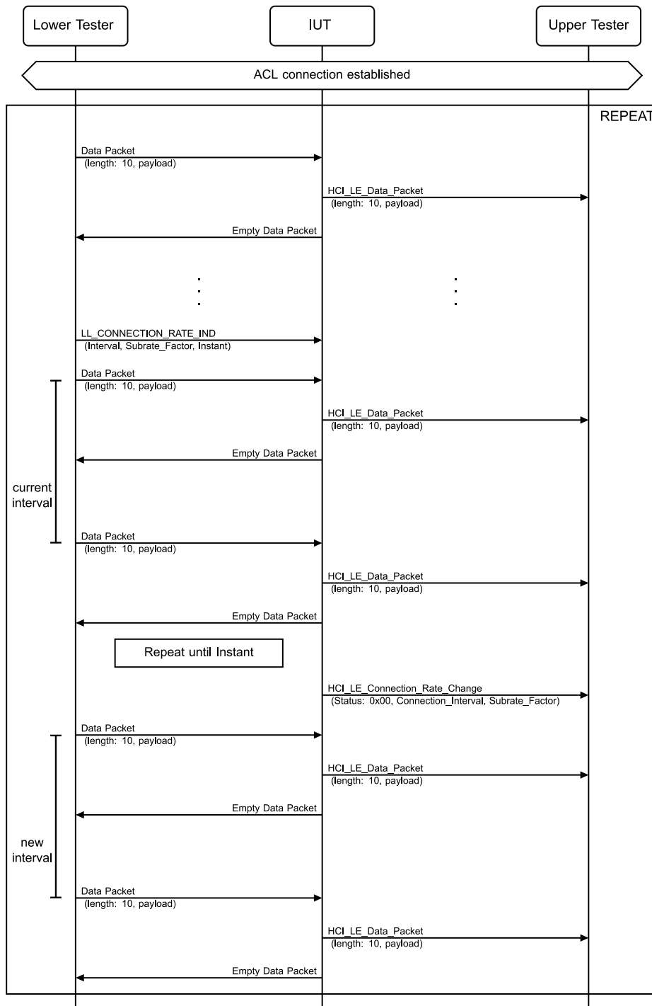
Figure 4.3-131: LL/CON/PER/BV-179-C [Connection Rate Update, Peripheral, Peer Initiated] MSC
