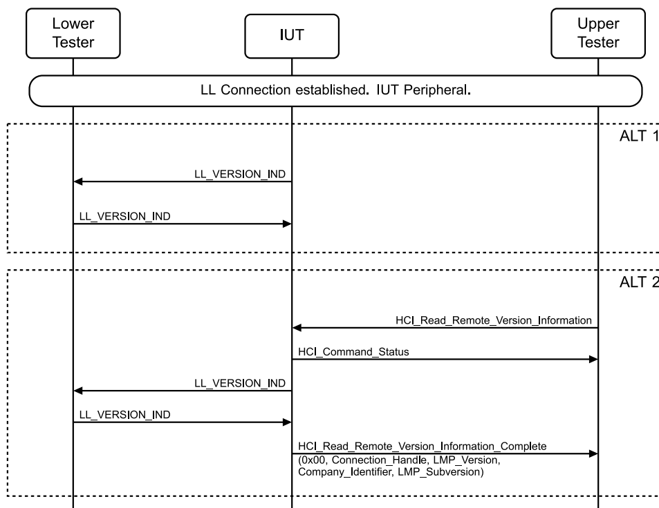
Figure 4.3-61: LL/CON/PER/BV-19-C [Peripheral Request Version] MSC
