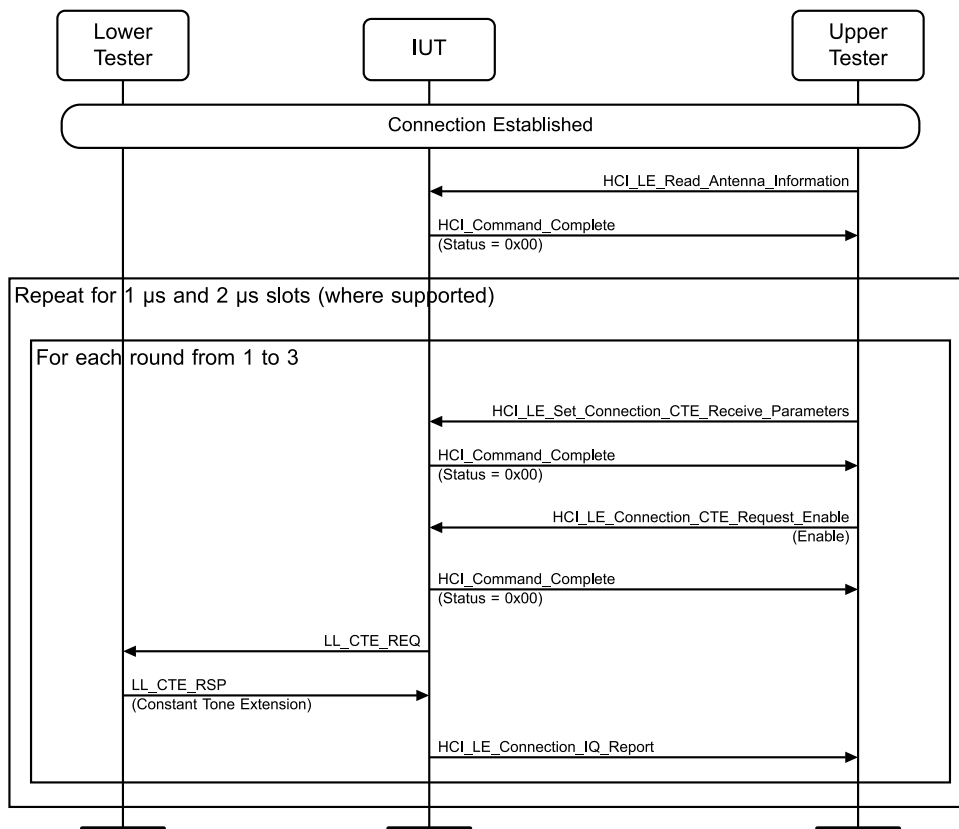
Figure 4.3-239: Constant Tone Extension Request Procedure, IUT Initiated, AoD MSC
