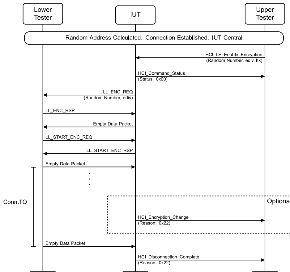
Figure 4.8-56: LL/SEC/CEN/BI-04-C [Central Encryption Setup: Missing Acknowledgement] MSC
