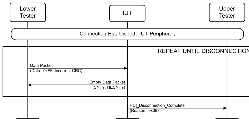
Figure 4.3-105: LL/CON/PER/BI-01-C [Invalid CRC Anchor Point] MSC
