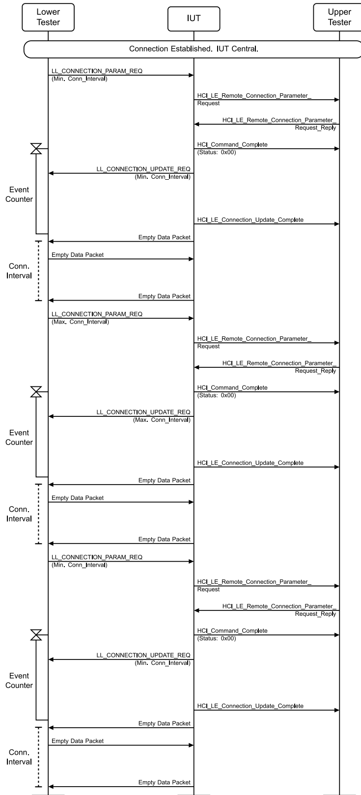
Figure 4.3-160: LL/CON/CEN/BV-30-C [Accepting Connection Parameter Request – no Preferred_Periodicity] MSC
