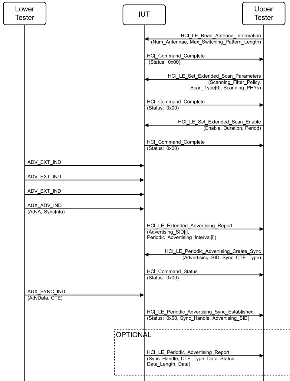
Figure 4.2-93: Connectionless CTE Scanning, Connectionless IQ Report MSC – Page 1 of 2
