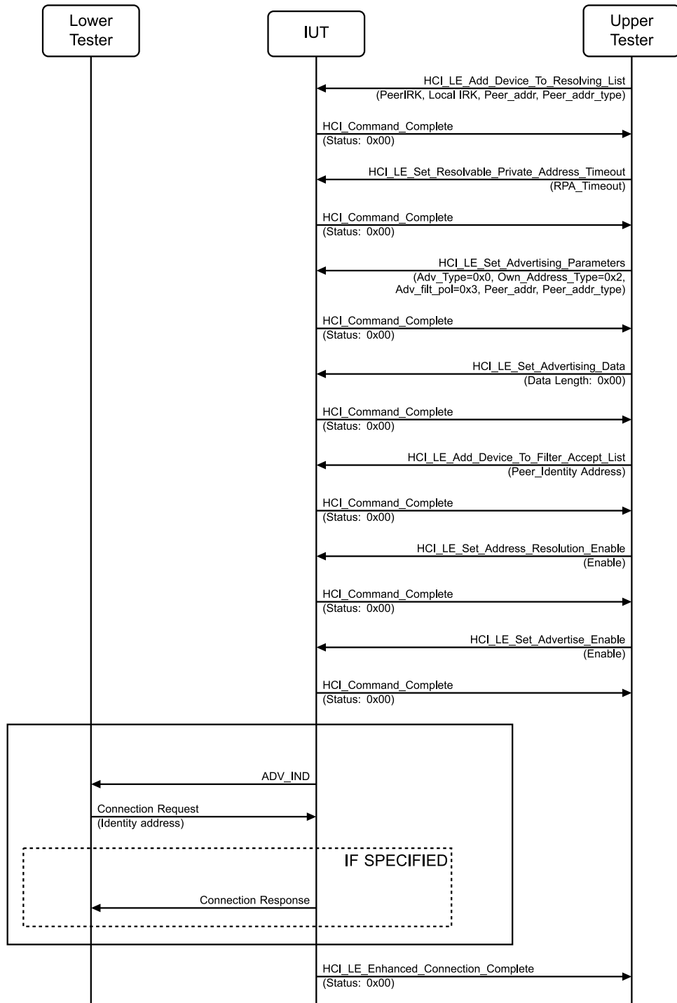
Figure 4.8-7: Network Privacy - Undirected Connectable Advertising with Local IRK and Peer IRK MSC – Page 1 of 2
