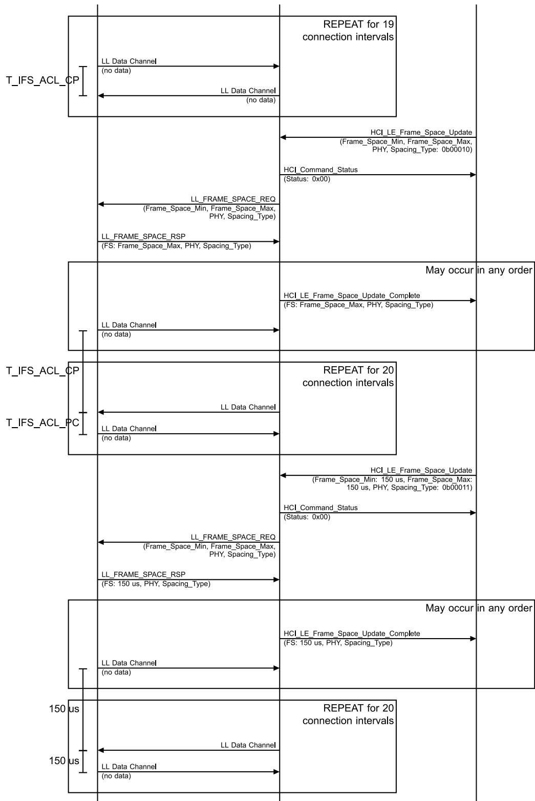
Figure 4.4-16: Initiate Inter Frame Space Change in the current ACL connection, Asymmetric PHYs, Peripheral MSC – Page 2 of 2
