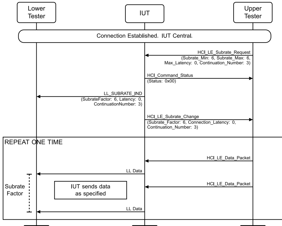
Figure 4.3-204: LL/CON/CEN/BV-142-C [Change the Subrate of an Existing Connection, Verify Sending Data, Continuation Number events] MSC
