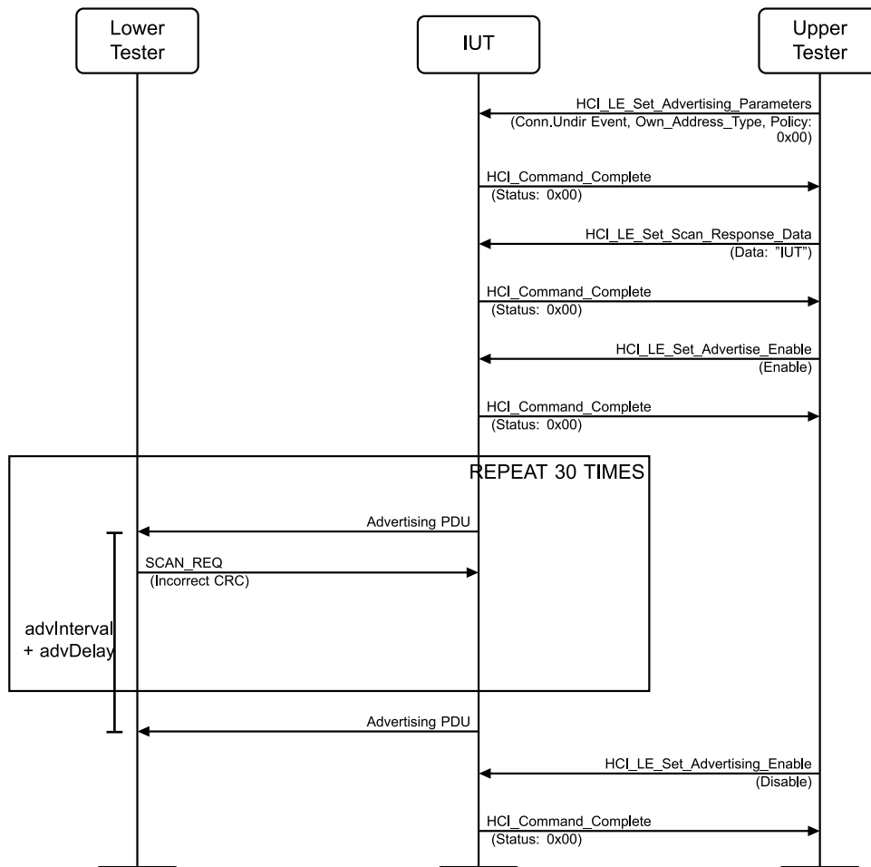
Figure 4.2-13: Scan Request Invalid CRC MSC
