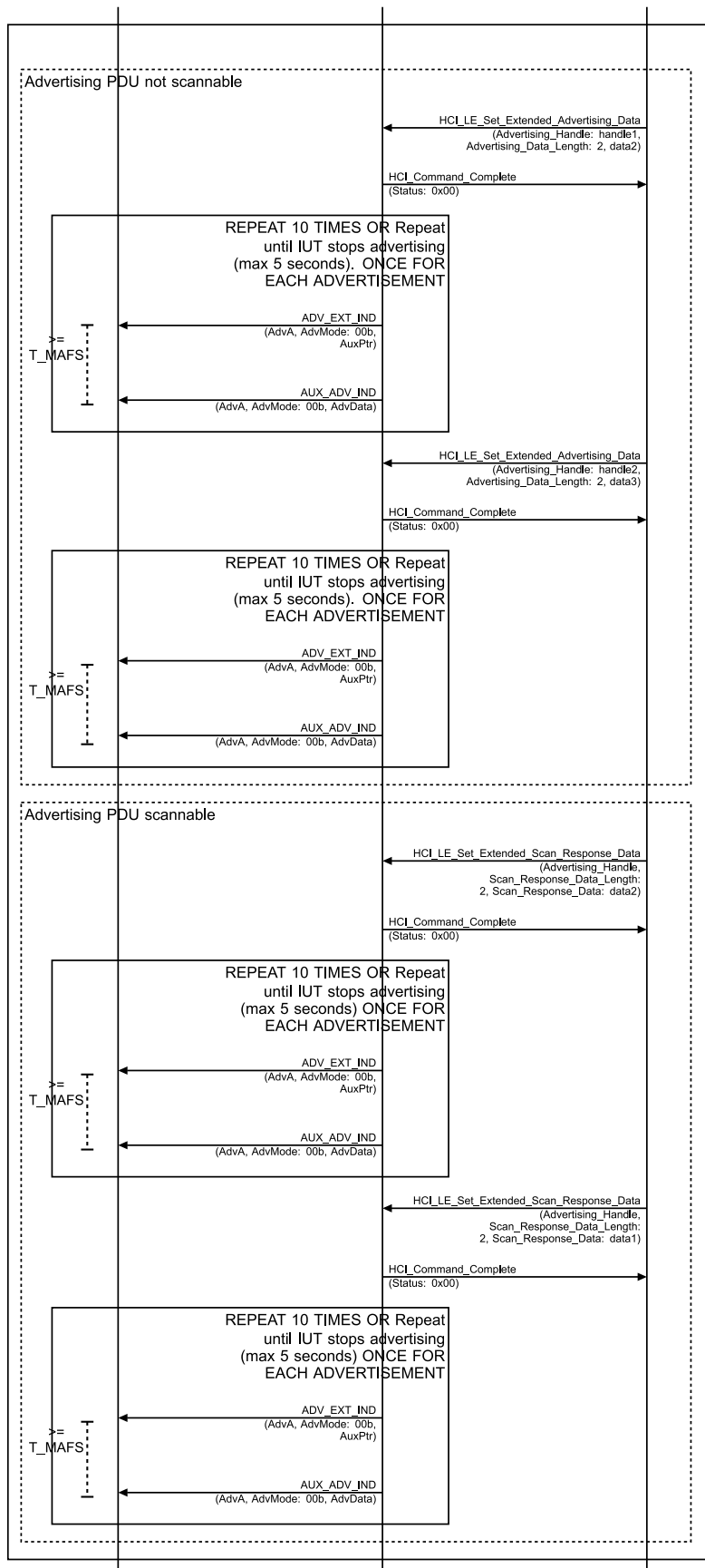
Figure 4.2-57: Extended Advertising, Multiple Sets, New RPA on AdvData Change MSC – Page 2 of 4
