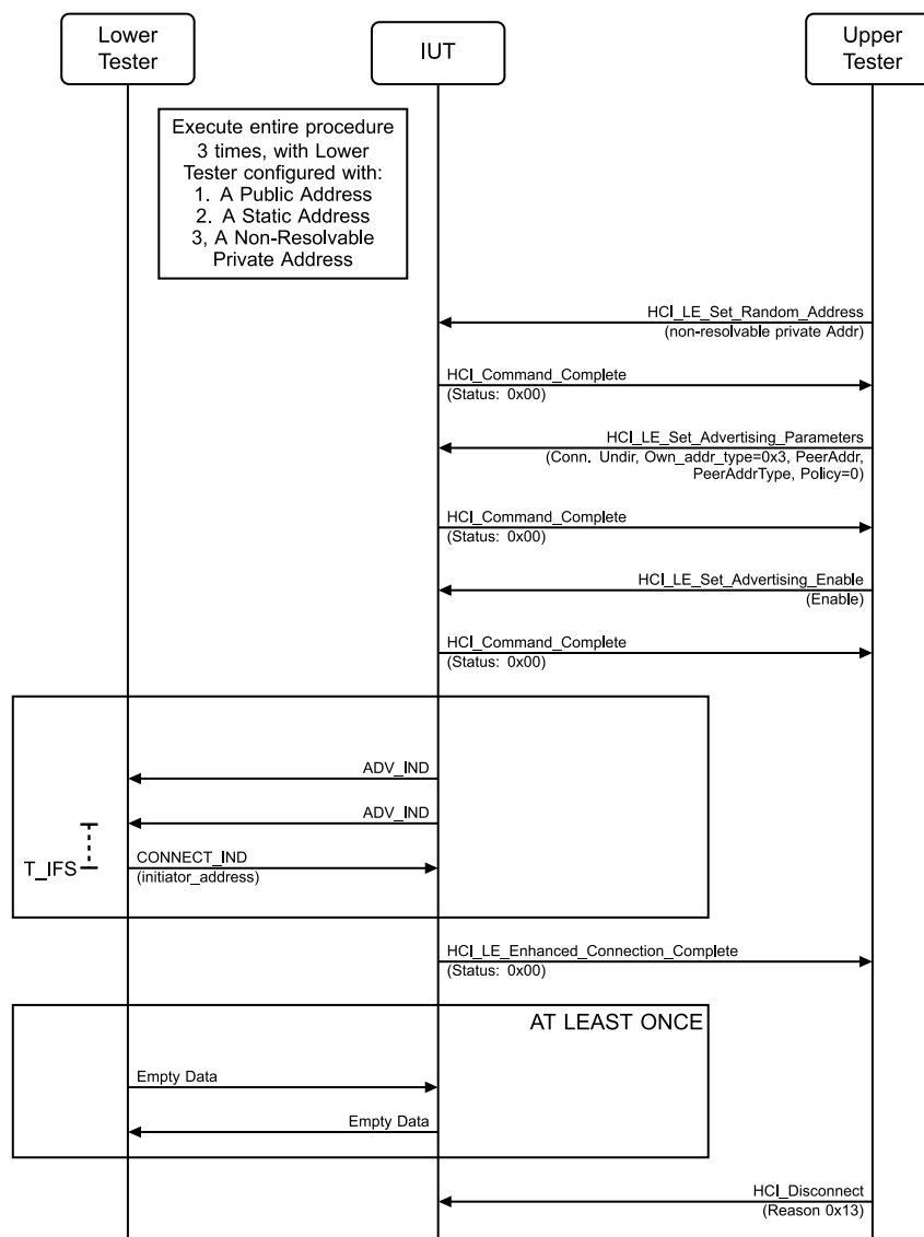
Figure 4.8-5: LL/SEC/ADV/BV-06-C [Network Privacy - Undirected Connectable Advertising no Local IRK, no peer IRK] MSC
