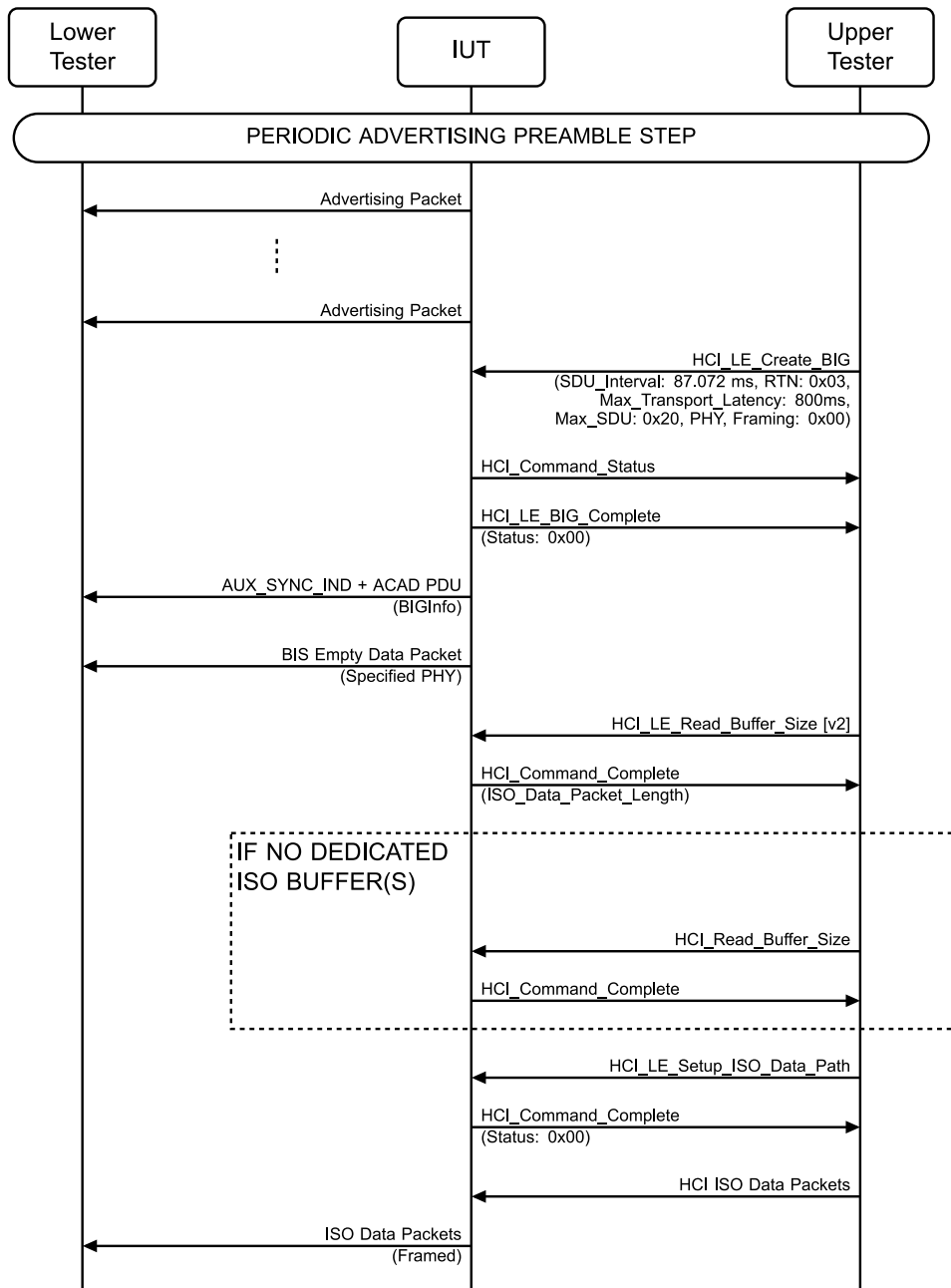
Figure 4.11-10: Broadcast Isochronous Stream Setup, Force Framed PDUs MSC
