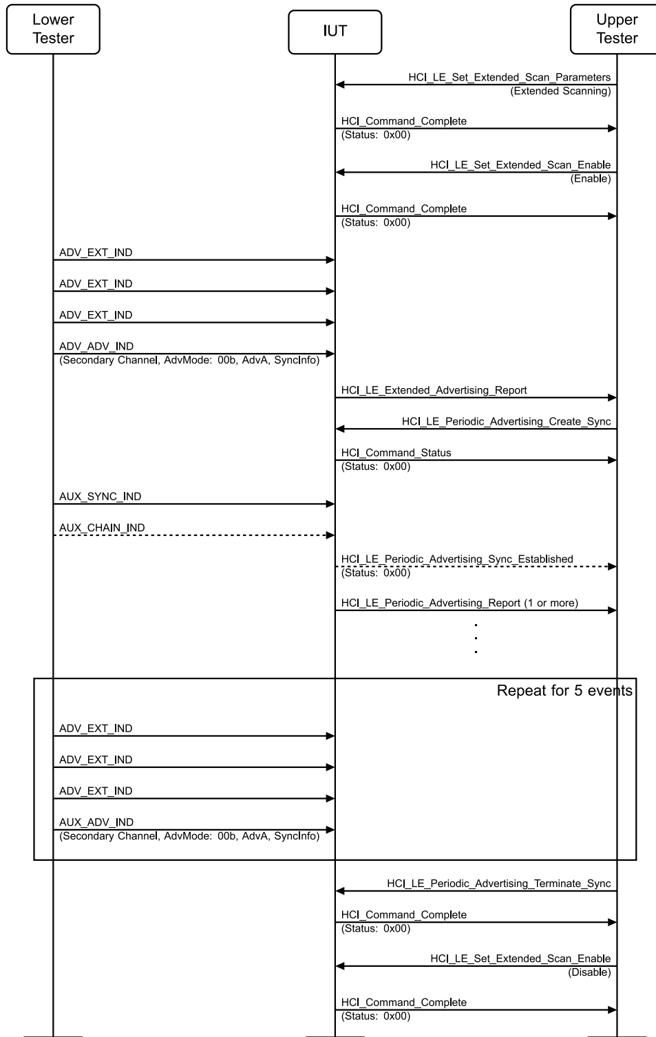
Figure 4.2-124: LL/DDI/SCN/BV-89-C [Extended Scanning, Periodic Advertising, Properly Ignore RFU Fields] MSC
