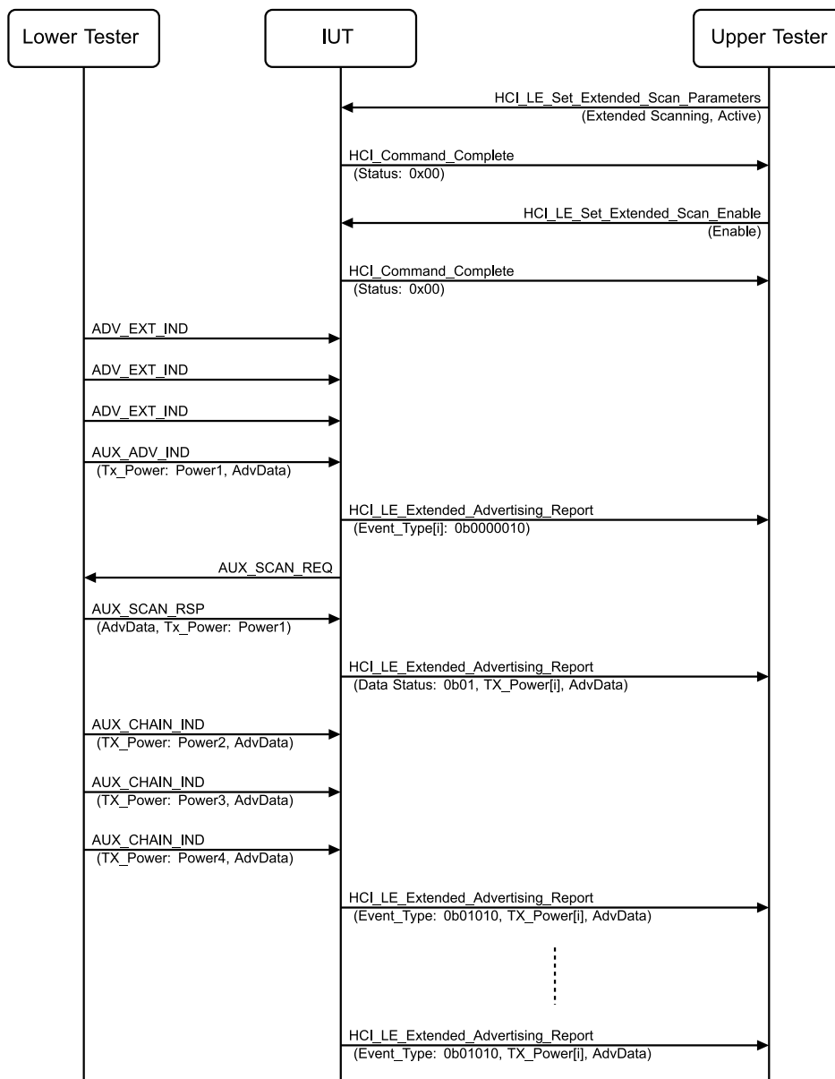
Figure 4.2-91: Extended Scanning, Active, Reporting TX Power MSC
