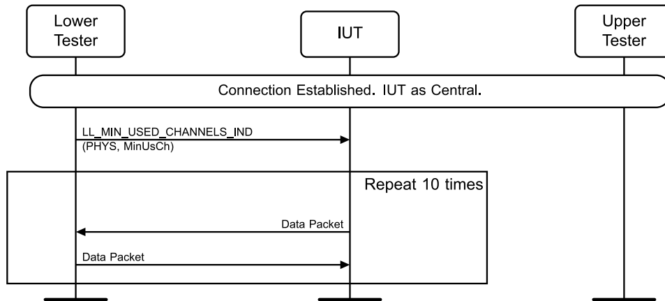
Figure 4.6-7: LL/FRH/CEN/BV-03-C [Accepting Minimum Number of Used Channels] MSC
