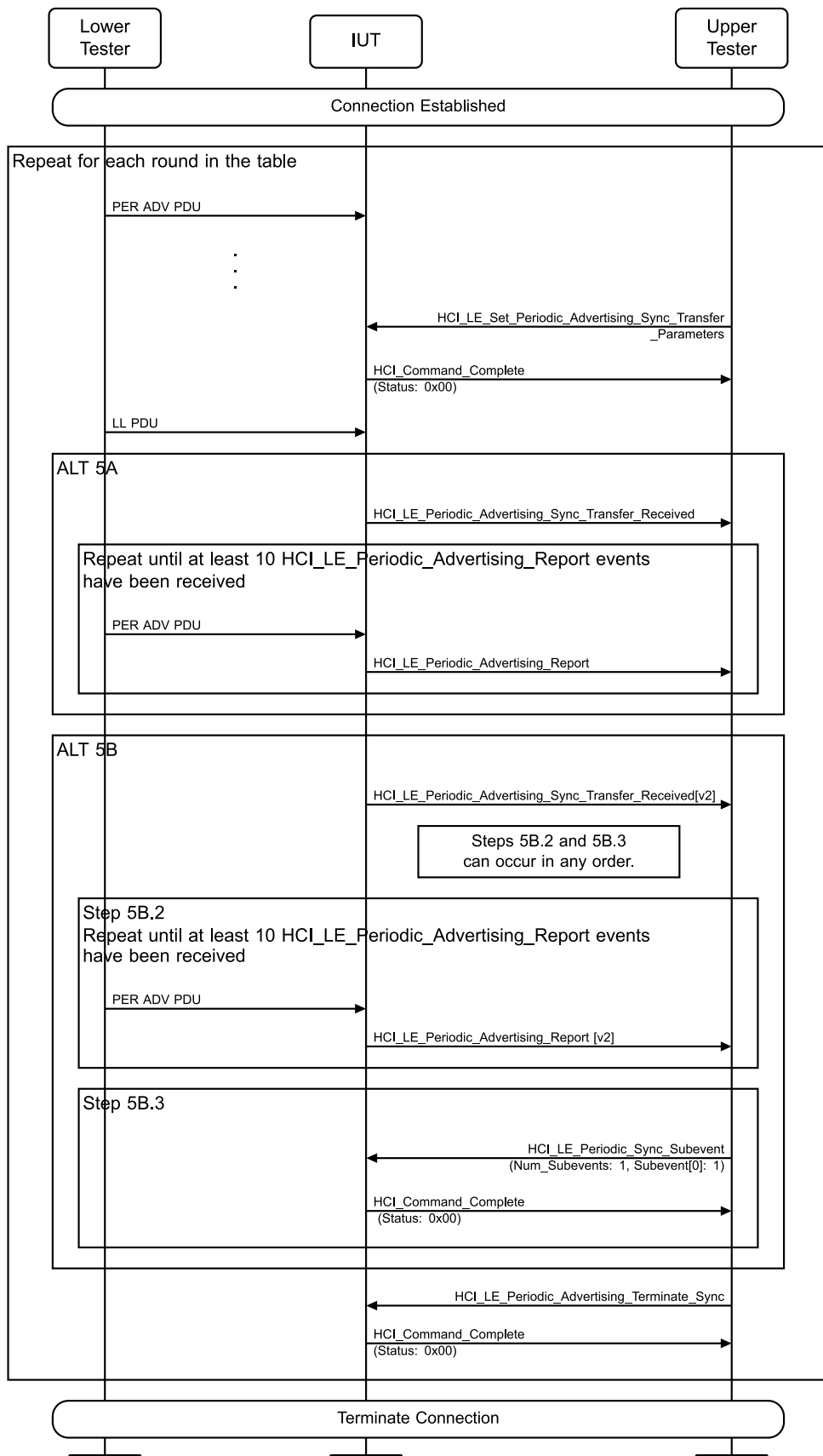
Figure 4.3-216: Periodic Advertising Sync Transfer Procedure, Accepting – Different PHYs MSC
