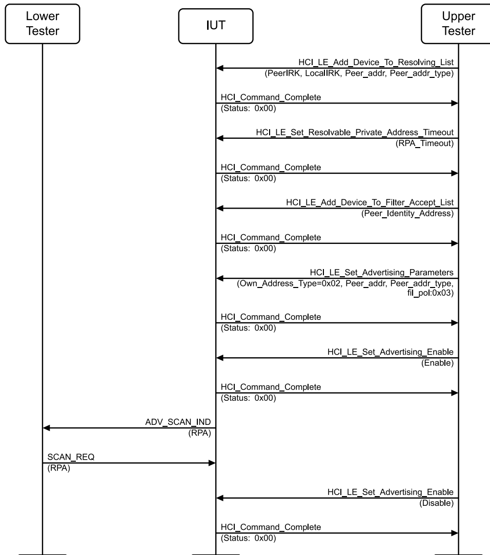
Figure 4.8-21: LL/SEC/ADV/BV-21-C [Network Privacy - Scannable Advertising, resolvable private address, Ignore scanner RPA] MSC
