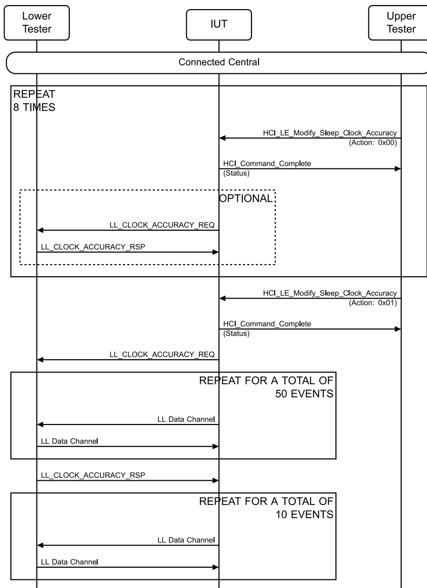
Figure 4.4-30: LL/TIM/CEN/BV-06-C [Change Accuracy after Update] MSC
