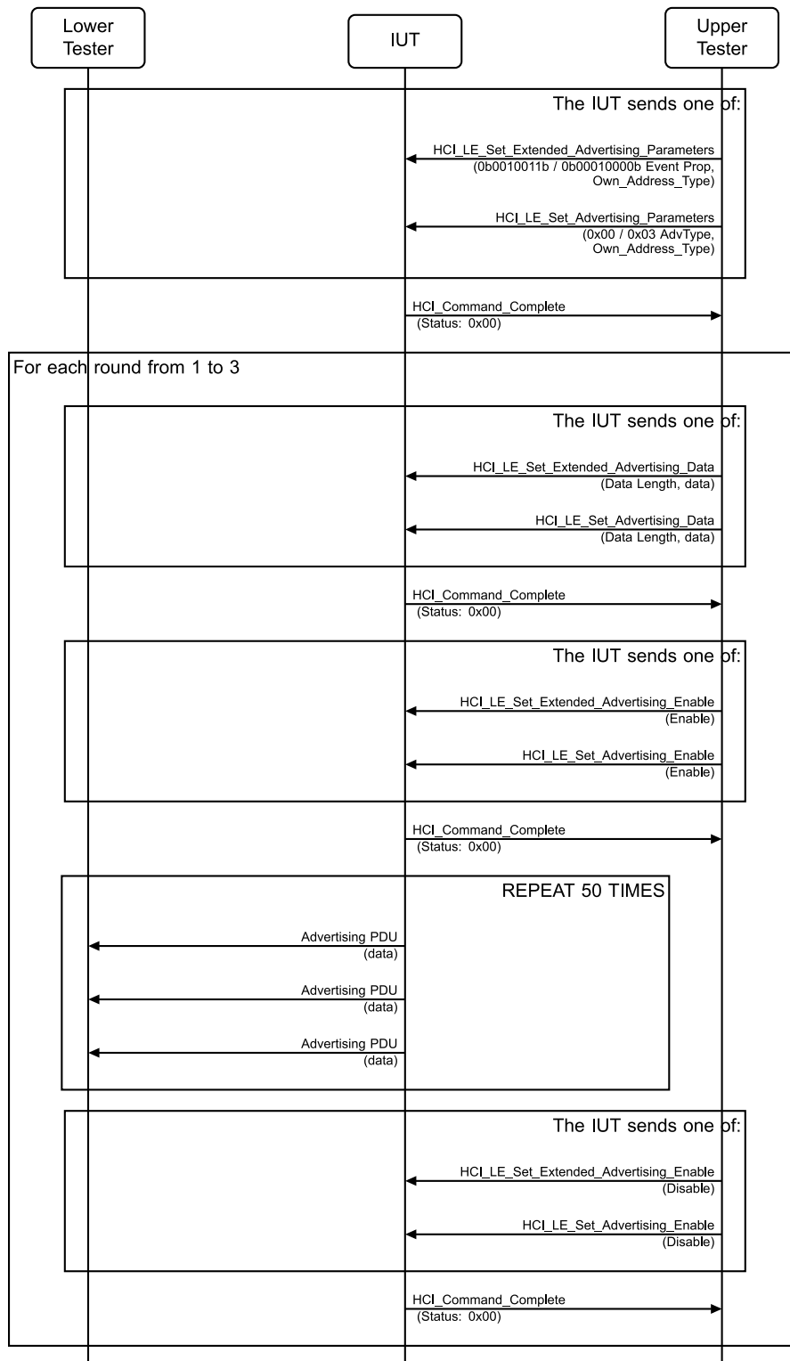
Figure 4.2-18: Extended Advertising, Legacy PDUs, Undirected MSC
