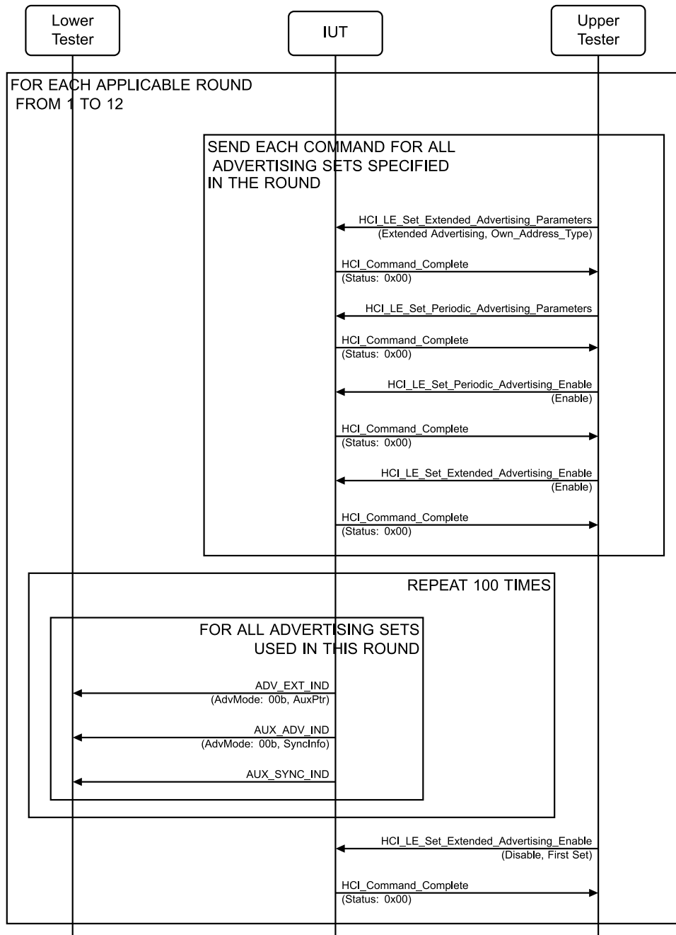
Figure 4.2-31: LL/DDI/ADV/BV-33-C [Extended Advertising, Periodic Advertising, Multiple Sets, Multiple PHYs (All Supported PHYs)] MSC – Page 1 of 2
