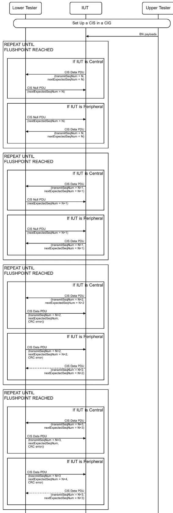
Figure 4.10-60: transmitSeqNum Increments at Flushpoint in Bidirectional CIS MSC
