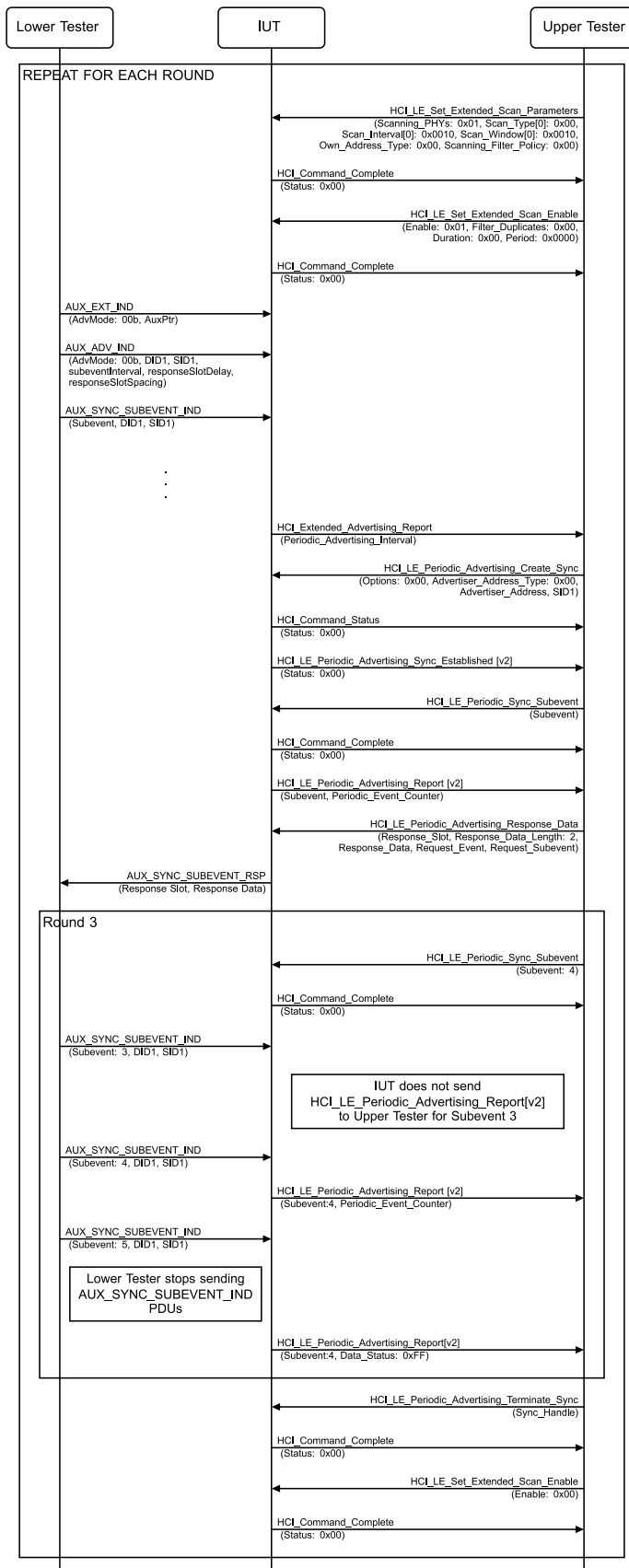
Figure 4.2-126: Sync with a Periodic Advertiser and Listen for the Assigned Subevent MSC
