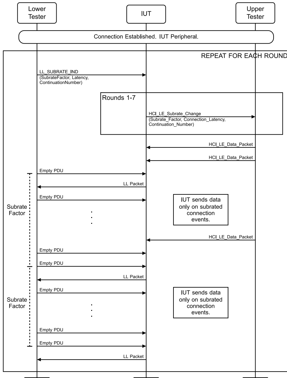
Figure 4.3-112: LL/CON/PER/BV-137-C [Respond to a Subrate Change] MSC
