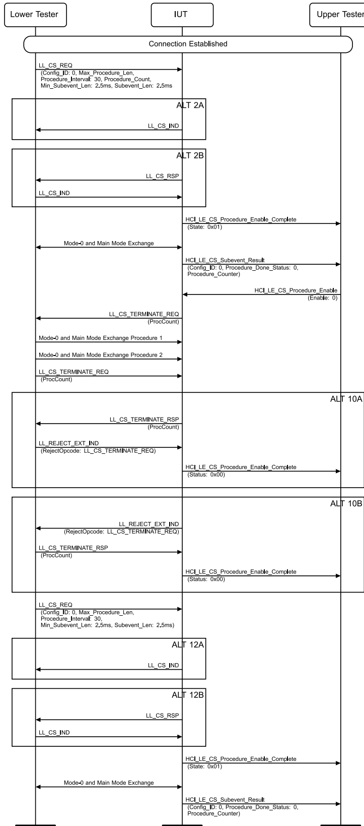
Figure 4.14-62: CS Procedure, Initiate Repeat Termination, Verify ProcCount Difference MSC
