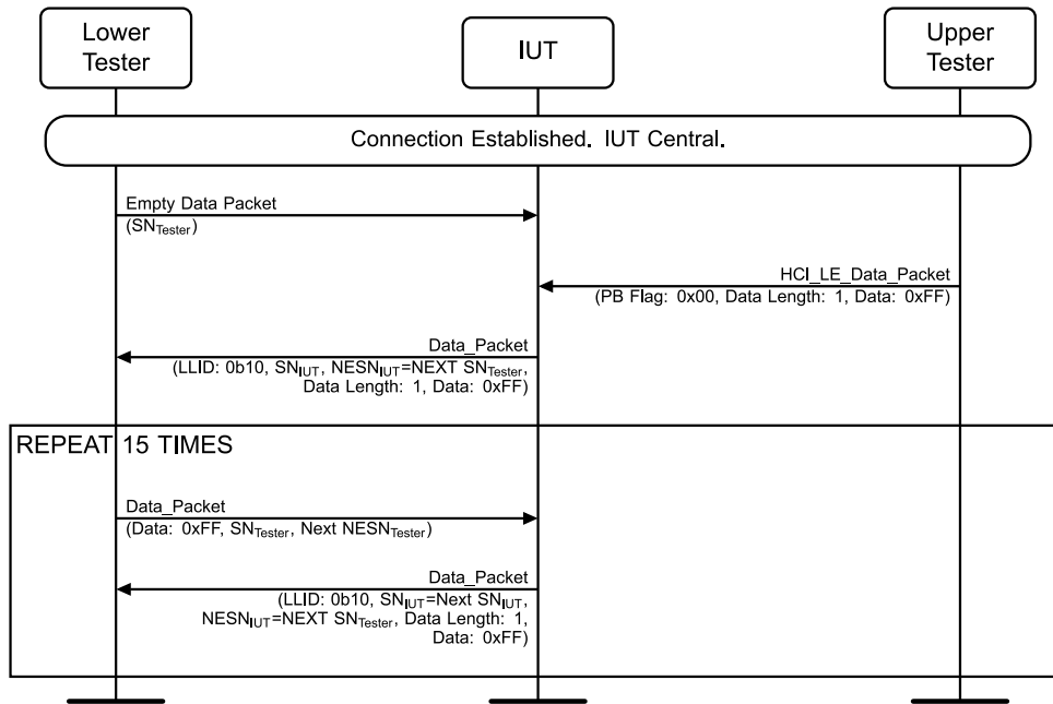
Figure 4.3-145: LL/CON/CEN/BV-16-C [Central Acknowledgement Repetition] MSC
