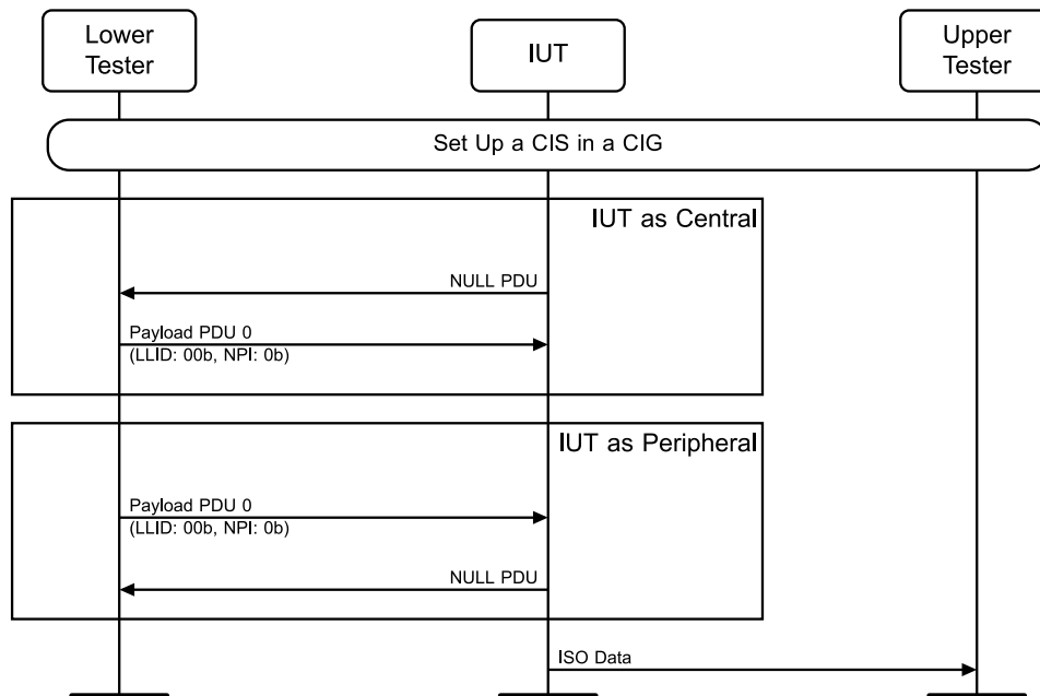
Figure 4.10-58: Receiving Data in Unidirectional CIS MSC
