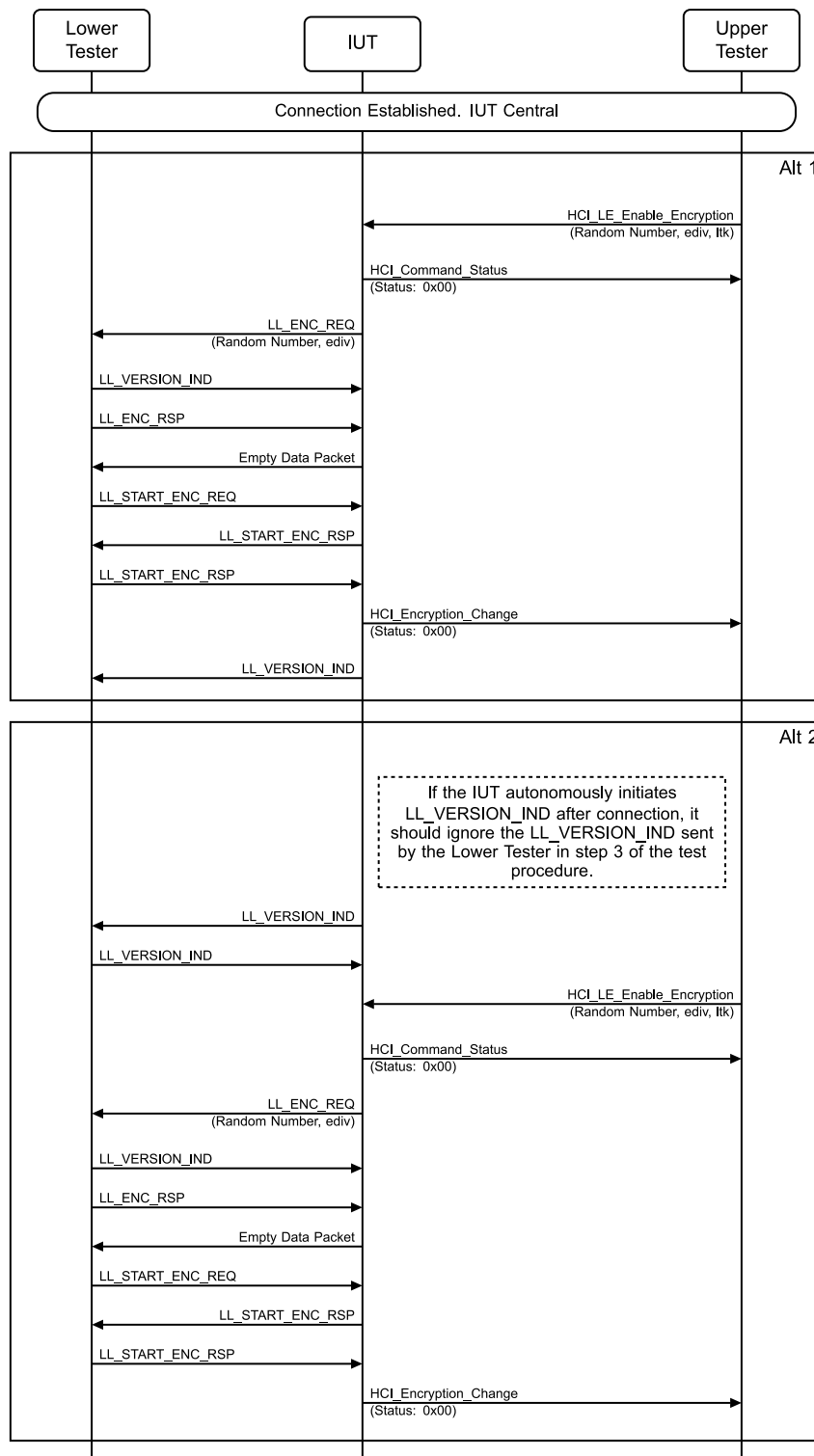
Figure 4.8-51: LL/SEC/CEN/BV-12-C [Central Start Encryption: Overlapping Procedure] MSC
