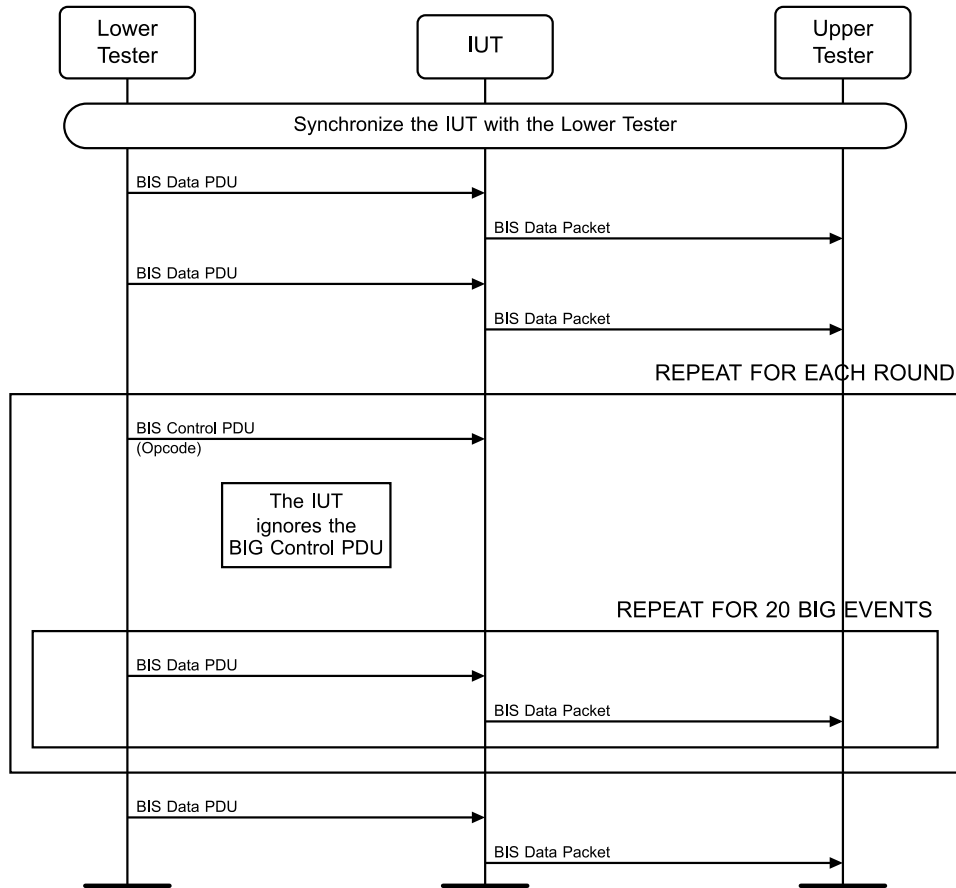
Figure 4.11-24: LL/BIS/SNC/BI-04-C [Ignores Restricted for Future Use Opcodes, BIS] MSC
