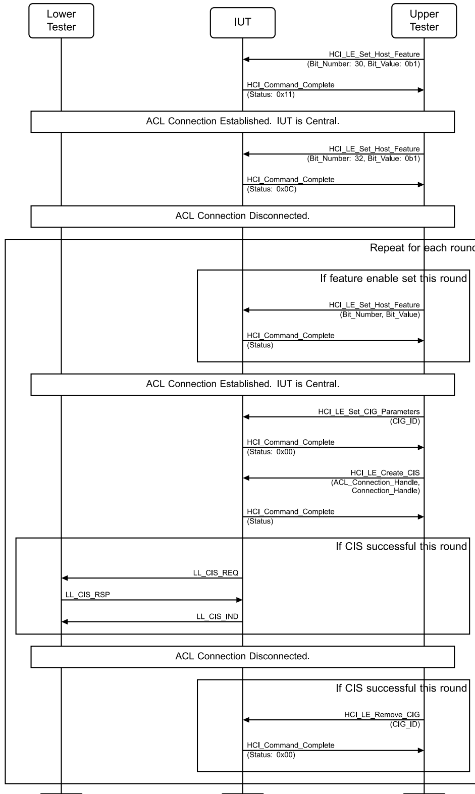
Figure 4.10-9: LL/CIS/CEN/BV-30-C [Isochronous Channels Host Support Feature Bit] MSC
