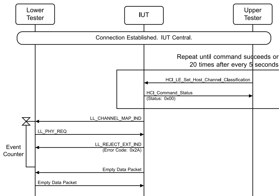
Figure 4.3-169: LL/CON/CEN/BV-47-C [Handling Protocol Collision – Different Procedure – Channel Map] MSC
