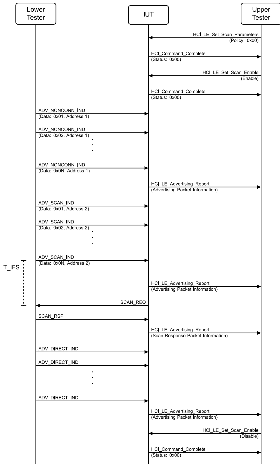
Figure 4.2-81: LL/DDI/SCN/BV-05-C [Scanning for Advertising types] MSC
