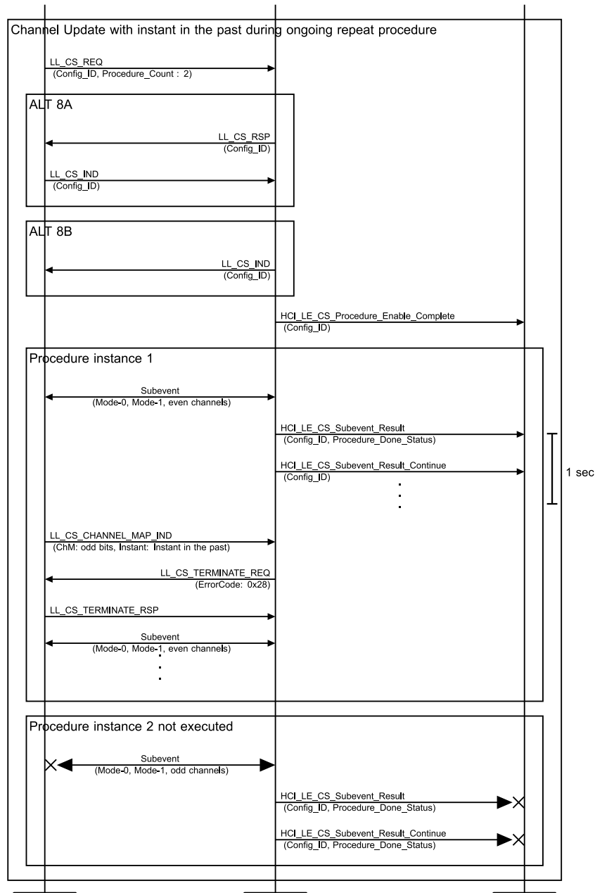
Figure 4.14-40: Channel Sounding Procedure Terminate, Channel Map Update in the Past, Responding CS Procedure MSC – Page 4 of 4
