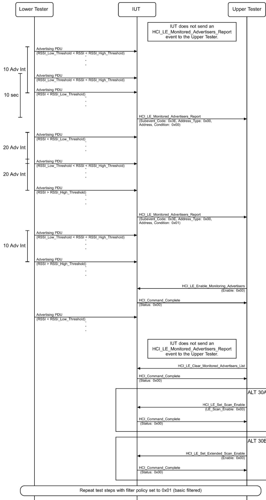
Figure 4.2-148: Monitoring Advertisers MSC – Page 2 of 2
