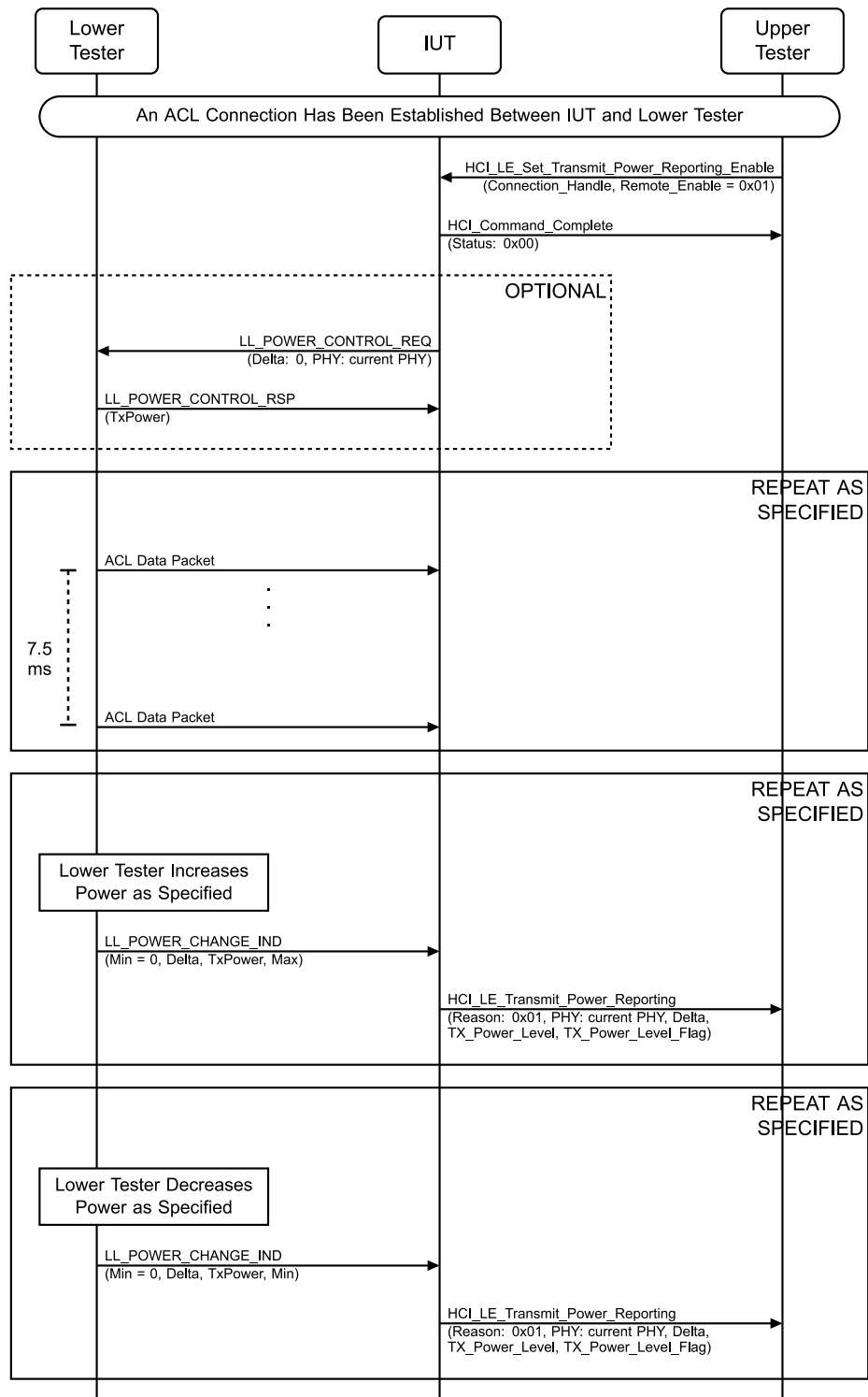
Figure 4.13-5: Power Configuration Response, Min and Max Power Level Reached MSC
