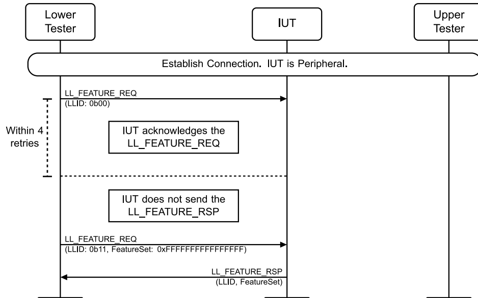
Figure 4.3-123: LL/CON/PER/BI-17-C [Invalid LLID] MSC
