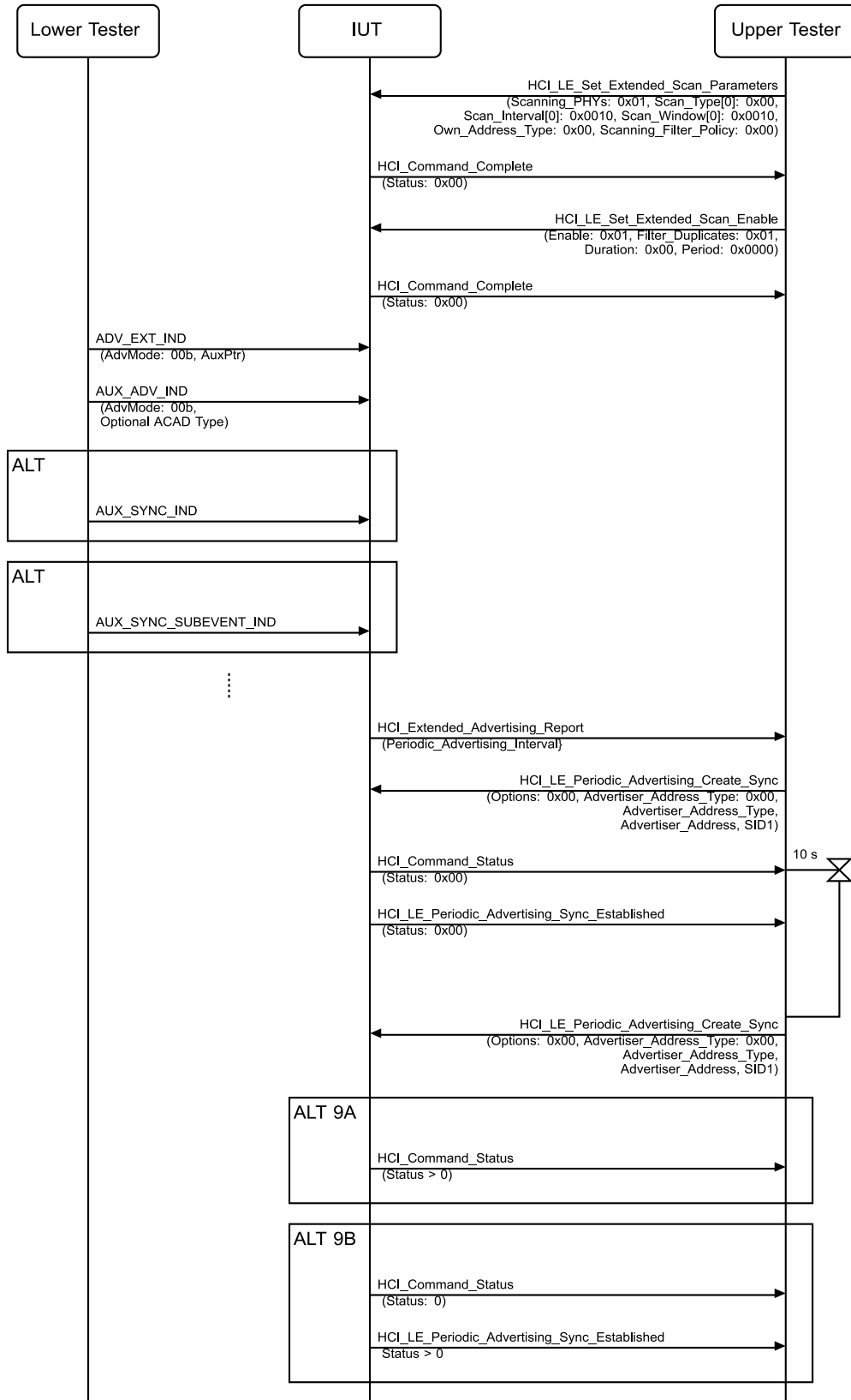
Figure 4.2-131: Periodic Advertising with Responses Trains, Do Not Synchronize with Same Address, Address Type, Advertising SID MSC
