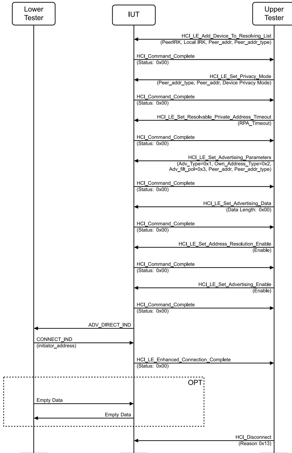
Figure 4.8-20: LL/SEC/ADV/BV-20-C [Device Privacy - Directed Connectable Advertising using local and remote IRK, Accept Identity Address] MSC
