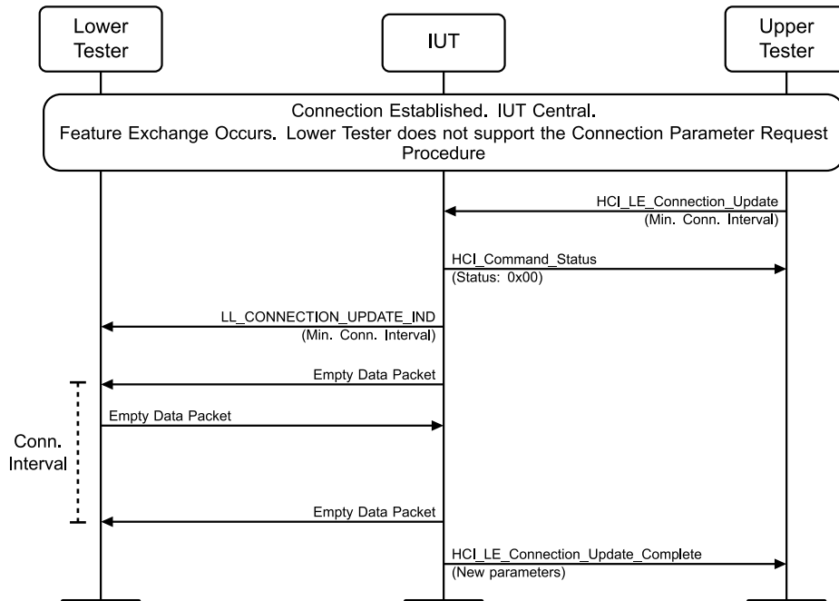
Figure 4.3-188: LL/CON/CEN/BV-82-C [Initiating Connection Parameter Request – Unsupported With Feature Exchange] MSC
