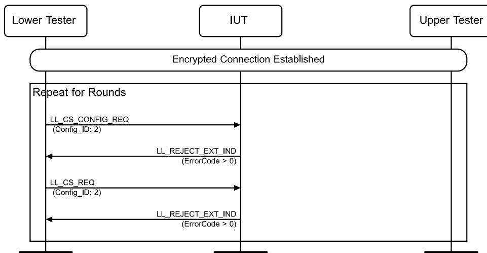
Figure 4.14-16: Reject Invalid Configuration Parameters MSC
