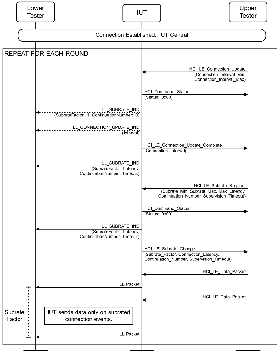
Figure 4.3-194: LL/CON/CEN/BV-134-C [Change the Subrate of an Existing Connection] MSC
