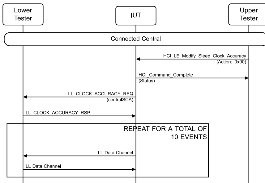
Figure 4.4-27: LL/TIM/CEN/BV-03-C [Initiate Sleep Clock Accuracy Update] MSC
