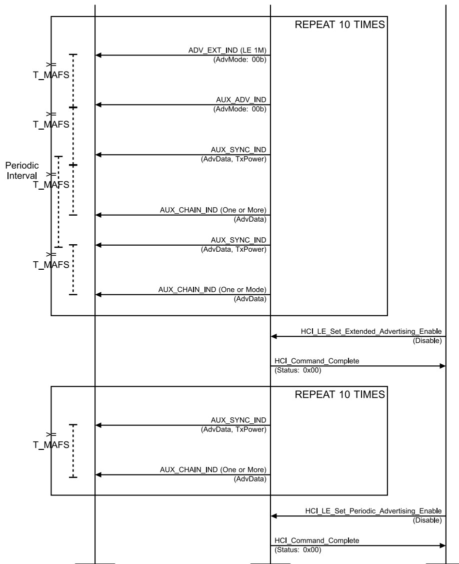
Figure 4.2-44: LL/DDI/ADV/BV-61-C [Extended Advertising, Periodic Advertising with TxPower] MSC – Page 2 of 2
