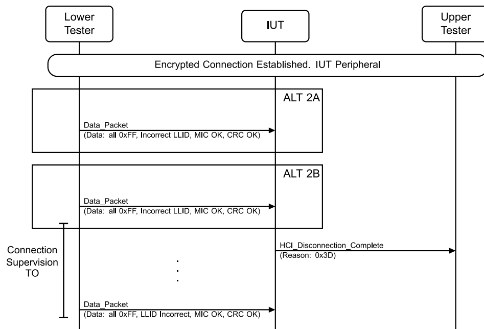
Figure 4.8-39: LL/SEC/PER/BI-03-C [Peripheral MIC Failure: Corrupted MIC] MSC
