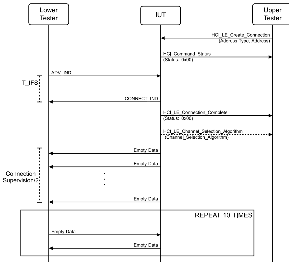
Figure 4.3-23: Connection Initiation Missed Replies MSC
