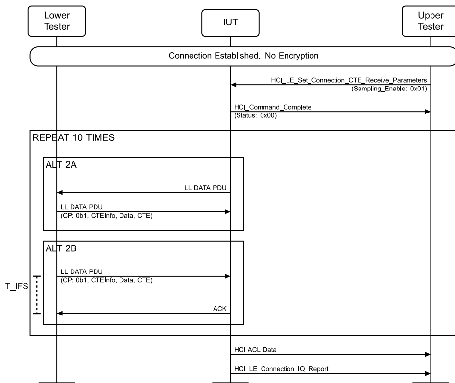
Figure 4.3-259: LL Data PDU size with Constant Tone Extension MSC
