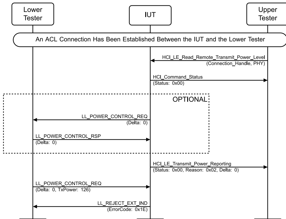
Figure 4.13-11: Remote Transmit Power Level Request MSC
