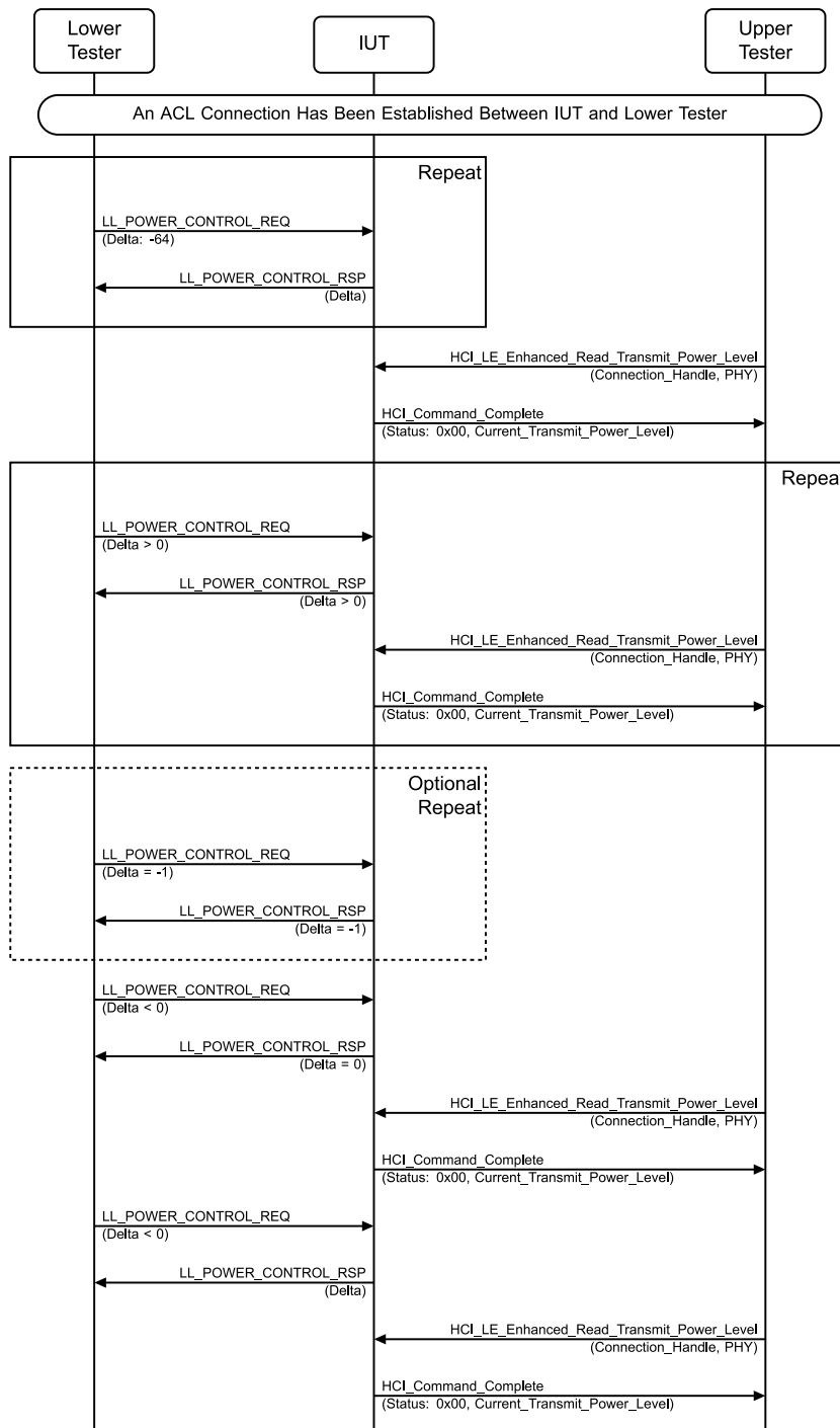
Figure 4.13-4: Power Control Response MSC
