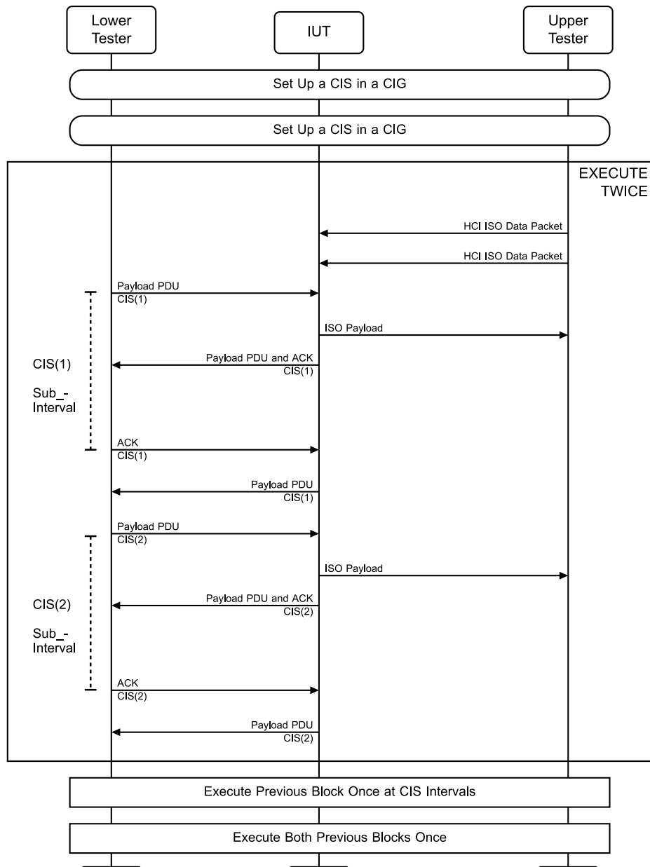
Figure 4.10-32: LL/CIS/PER/BV-08-C [Sending and Receiving Data in Multiple CISes, Single CIG, Single Connection, Sequential, Peripheral] MSC
