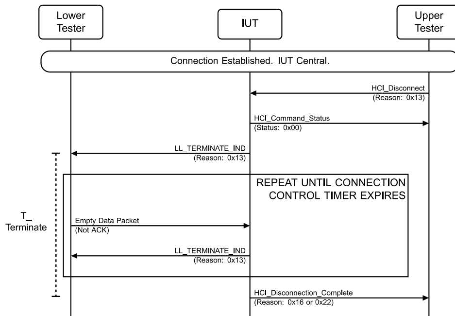
Figure 4.3-190: LL/CON/CEN/BI-02-C [Central T_Terminate Timer] MSC
