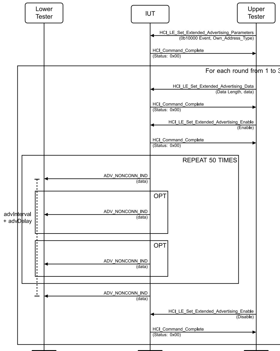
Figure 4.2-17: LL/DDI/ADV/BV-21-C [Extended Advertising, Legacy PDUs, Non-Connectable] MSC
