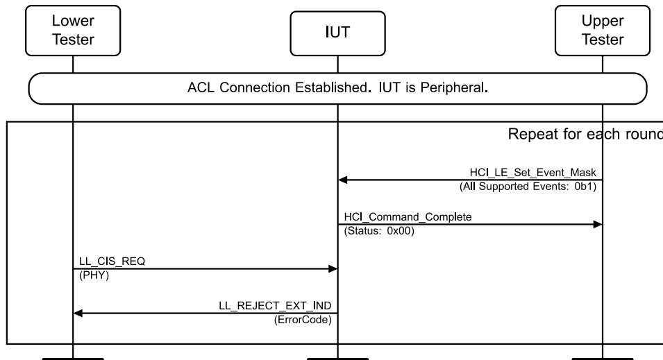
Figure 4.10-42: CIS Setup Response Procedure, Peripheral, Invalid or Unsupported PHY MSC
