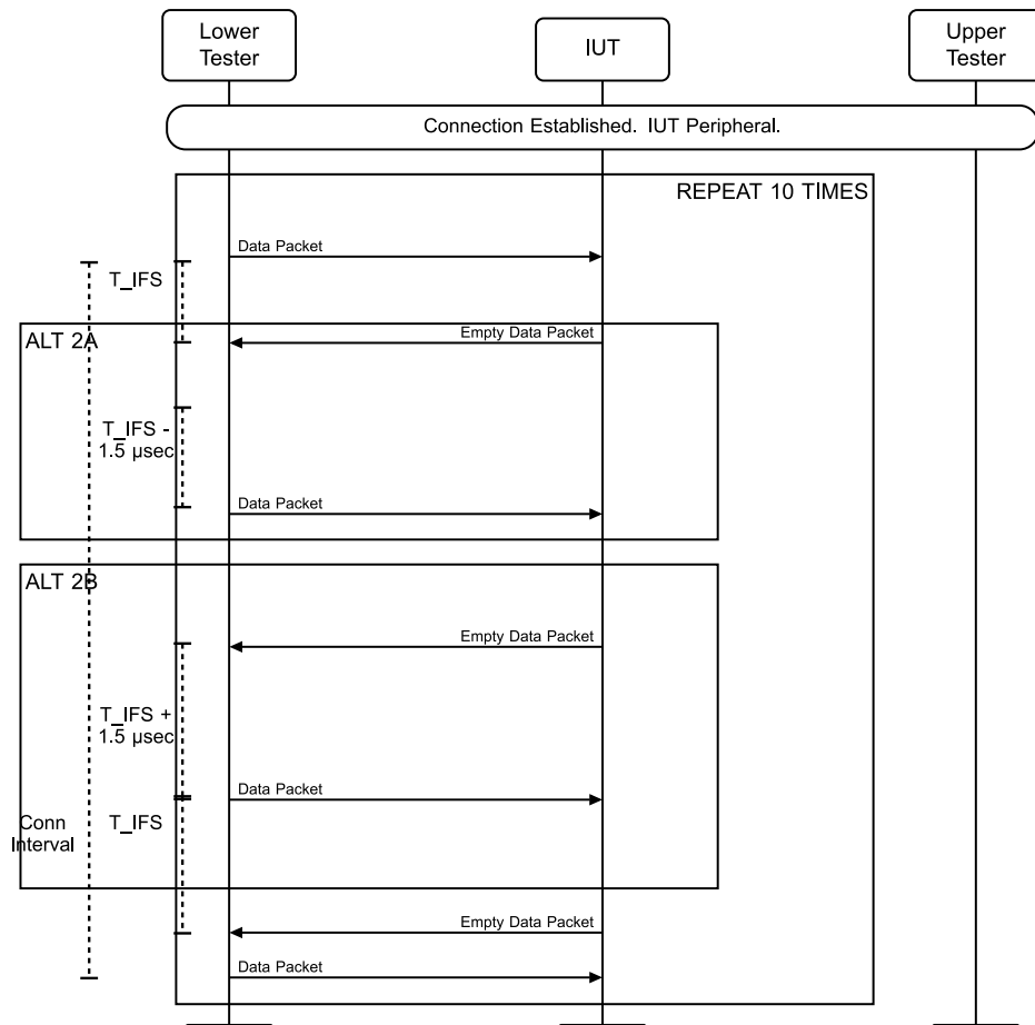
Figure 4.4-9: Earliest/Latest Transmissions to Peripheral MSC
