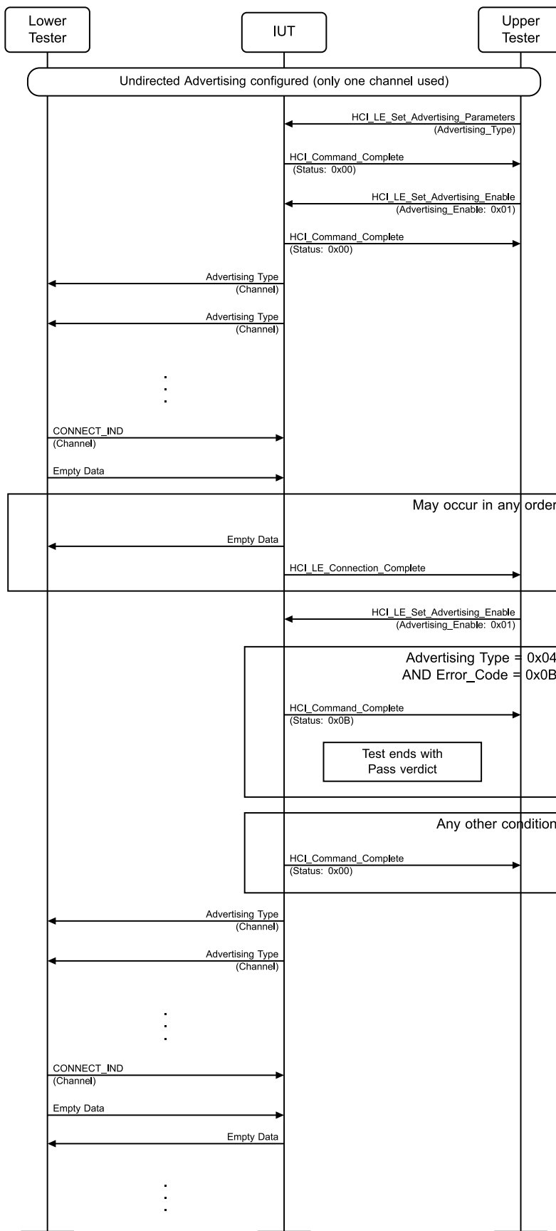
Figure 4.3-18: Reject Connection Request when Connected to the Peer, Legacy Advertising MSC
