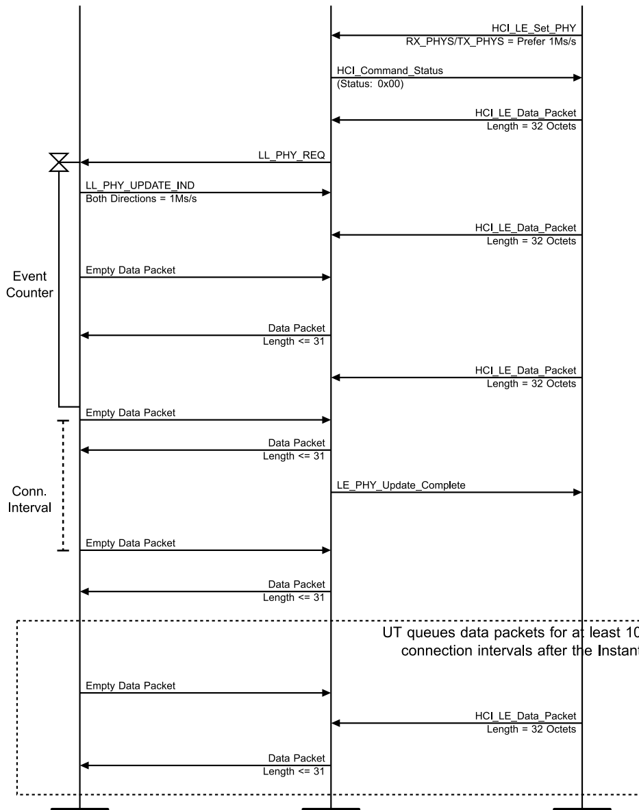
Figure 4.3-84: LL/CON/PER/BV-49-C [Initiating PHY Update Procedure – Packet Time Restrictions] MSC – Page 2 of 2
