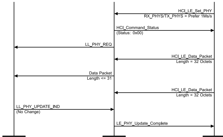
Figure 4.3-89: LL/CON/PER/BV-52-C [Initiating PHY Update Procedure – Packet Time Restrictions, No Change] MSC – Page 2 of 2
