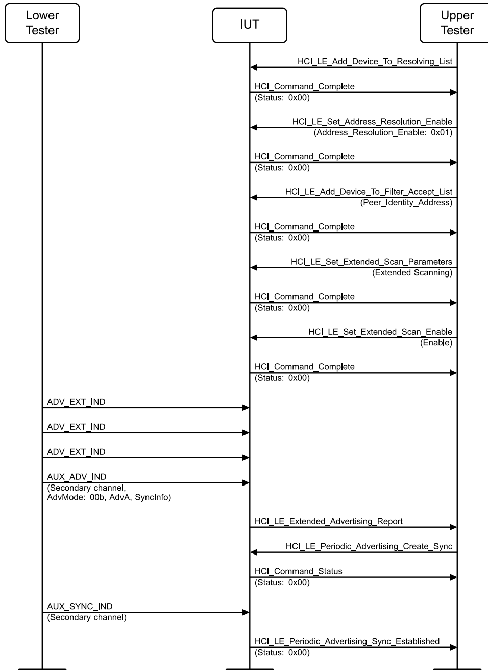
Figure 4.2-119: Extended Scanning, Periodic Advertising Reception, Identity Address MSC
