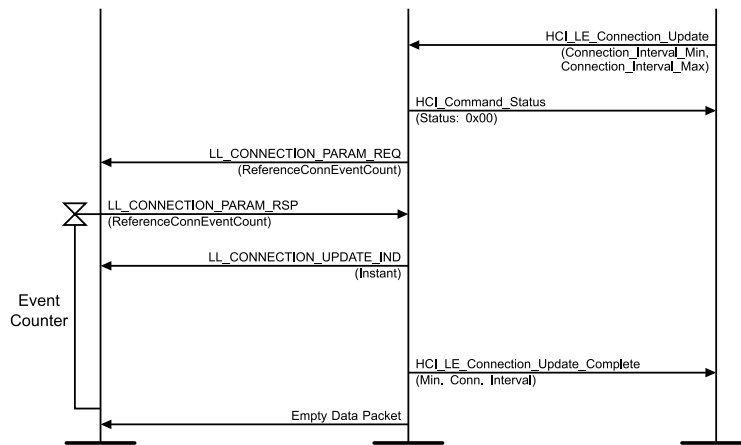
Figure 4.3-154: LL/CON/CEN/BV-24-C [Initiating Connection Parameter Request – Accept] MSC – Page 2 of 2
