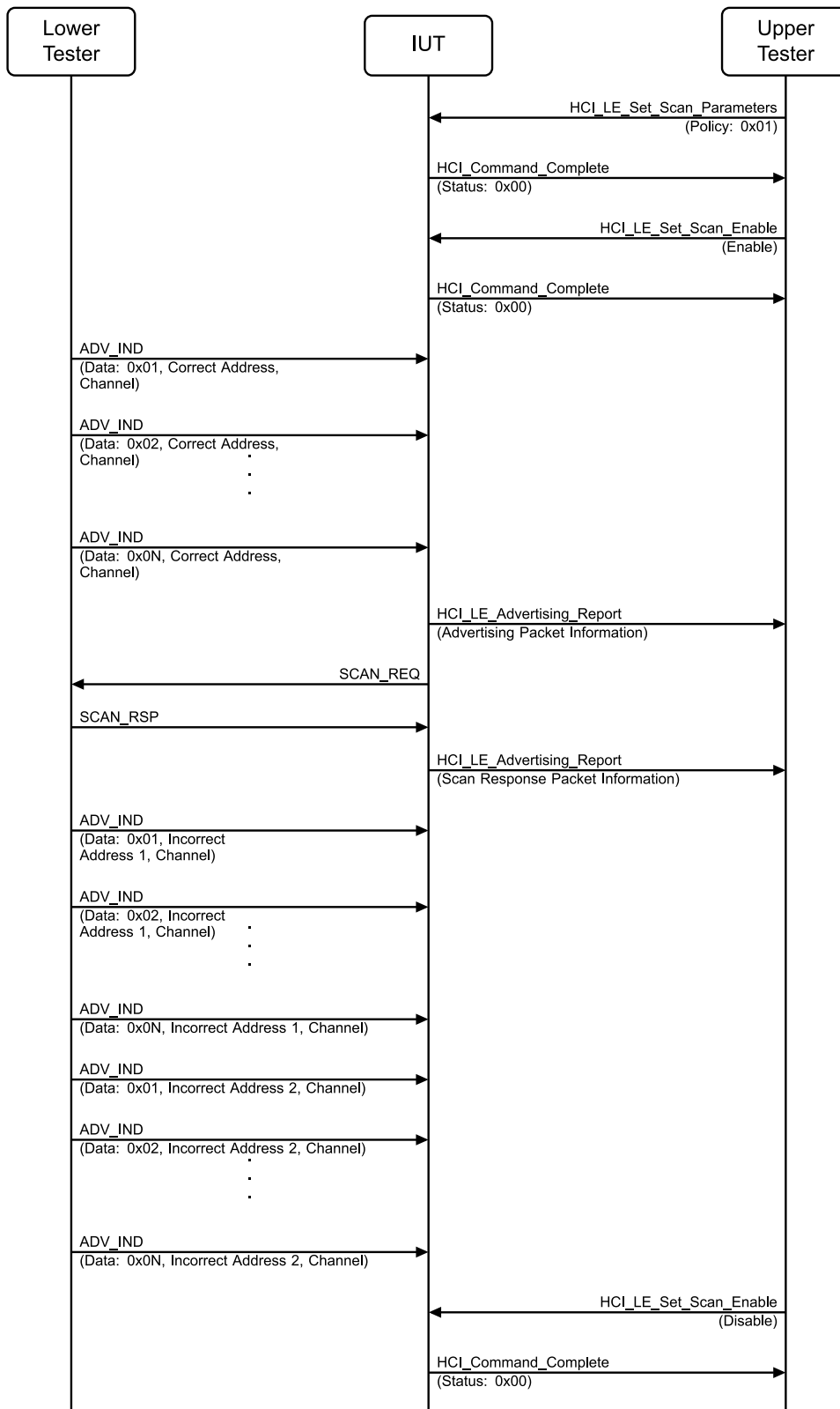
Figure 4.2-80: LL/DDI/SCN/BV-04-C [Active Scanning: Device Filtering] MSC
