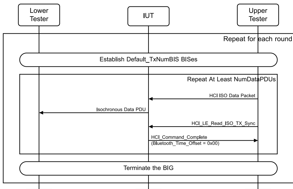
Figure 4.11-3: LL/BIS/BRD/BV-07-C [Bursting of Packets in Broadcast Isochronous Stream] MSC
