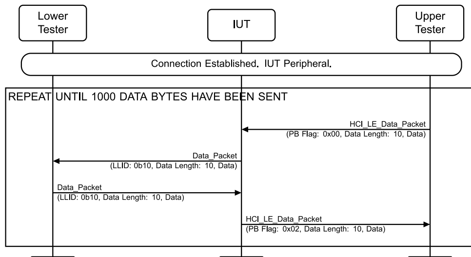
Figure 4.3-50: LL/CON/PER/BV-06-C [Peripheral receiving data and receiving data] MSC
