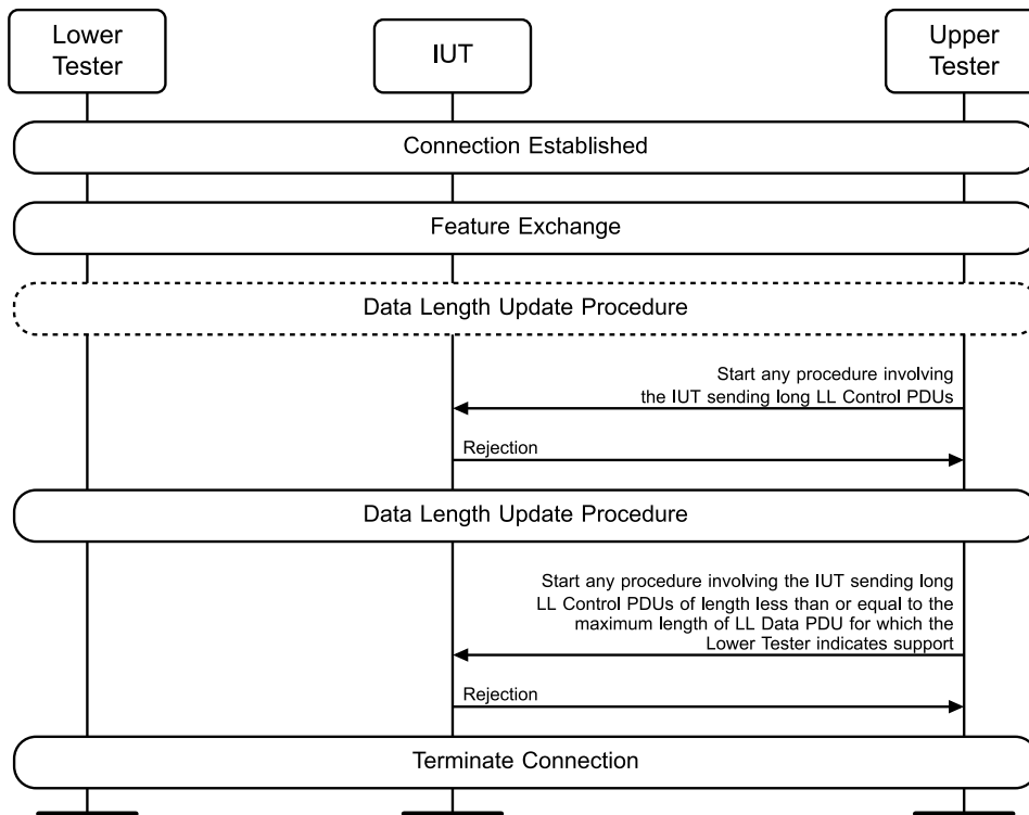
Figure 4.3-229: Rejecting Request to Send Long Control PDUs after Feature Exchange MSC
