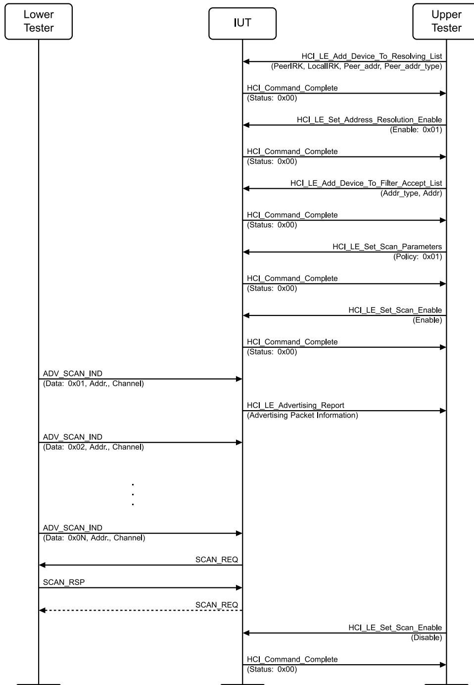
Figure 4.2-110: LL/DDI/SCN/BI-03-C [Privacy – Active Scanning, Local IRK, Peer IRK] MSC
