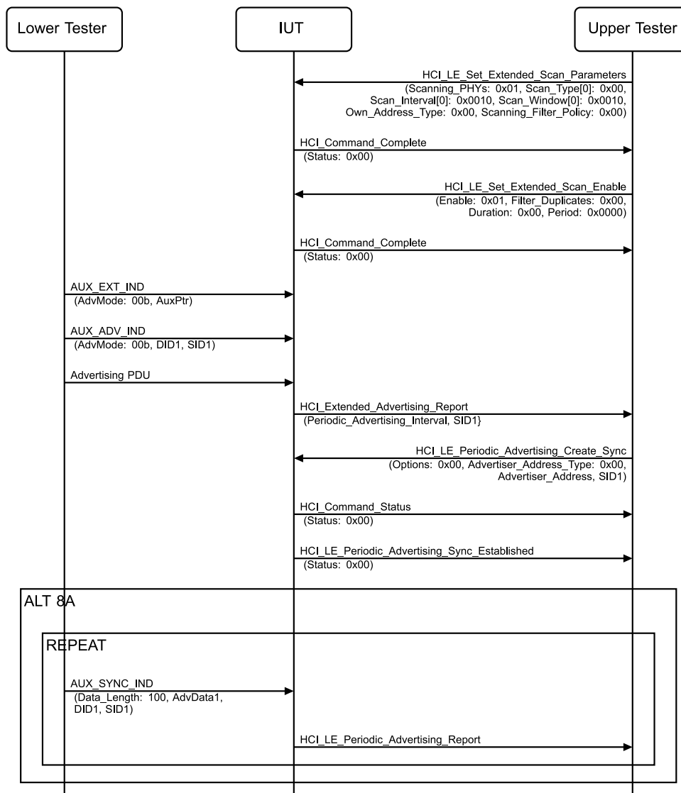
Figure 4.2-112: Scanner not supporting Periodic Advertising ADI accepts Advertising PDU with ADI Set MSC – Page 1 of 2
