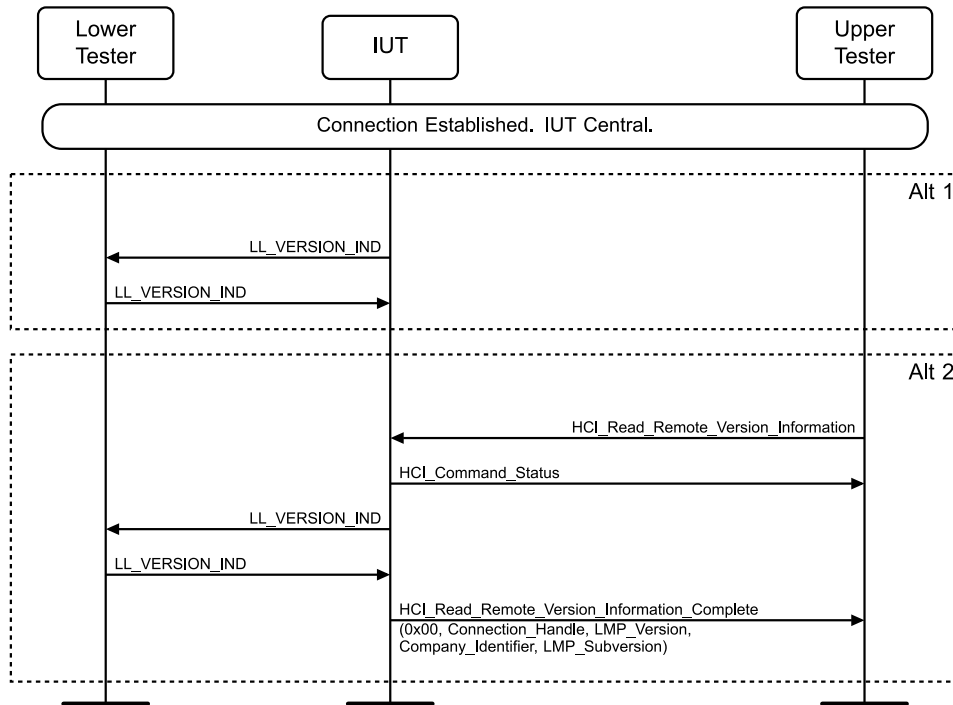
Figure 4.3-149: LL/CON/CEN/BV-20-C [Central Request Version] MSC
