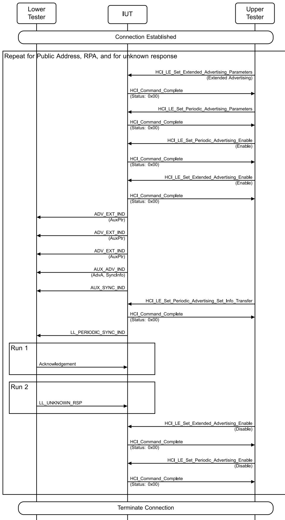
Figure 4.3-214: Periodic Advertising Sync Transfer Procedure, Advertising IUT Initiated MSC
