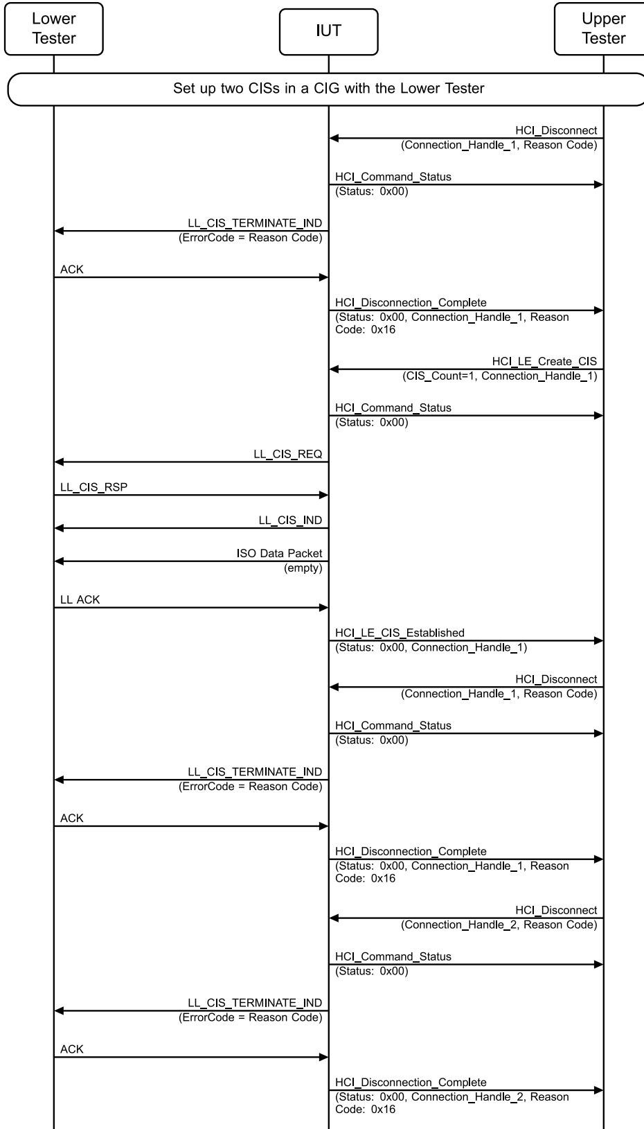
Figure 4.10-21: LL/CIS/CEN/BV-51-C [CIS Setup Procedure, Central Initiated, CIG ID Reuse] MSC – Page 1 of 2
