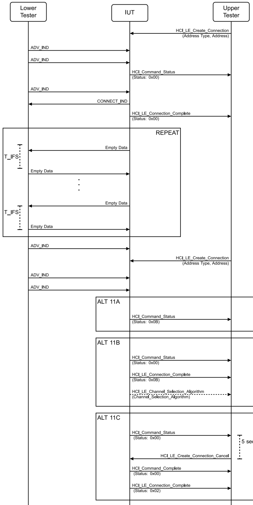
Figure 4.3-44: Duplicate Connection Request MSC
