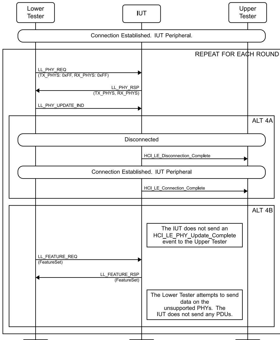
Figure 4.3-125: Responding to PHY Update Procedure, Invalid or Unsupported PHY, Central Initiated MSC
