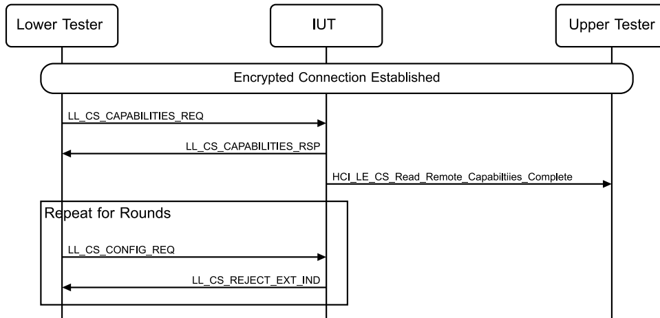
Figure 4.14-18: Reject Remote CS Configuration Procedure request with invalid Capability Exchange parameters MSC
