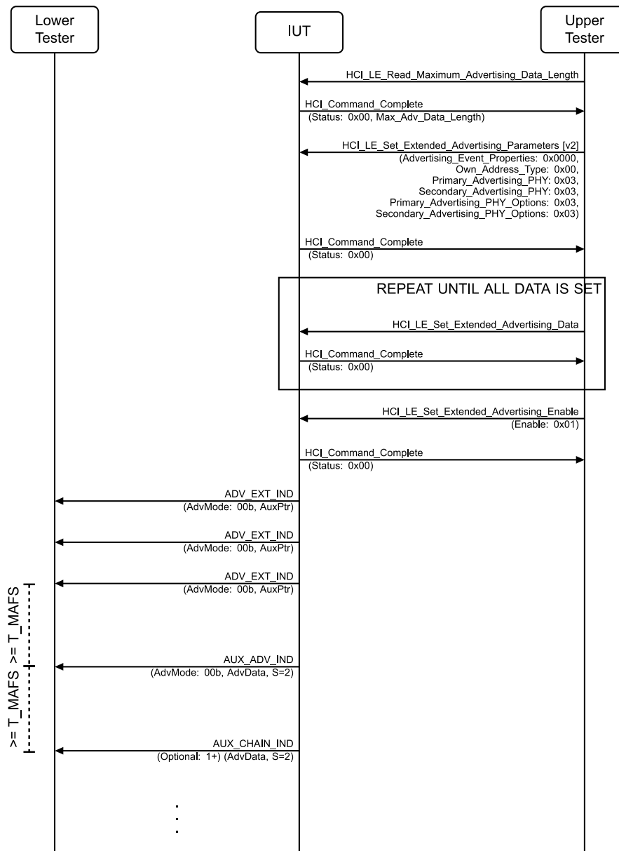
Figure 4.2-61: Extended Advertising, Non-Connectable, Advertising Coding Selection MSC – Page 1 of 2
