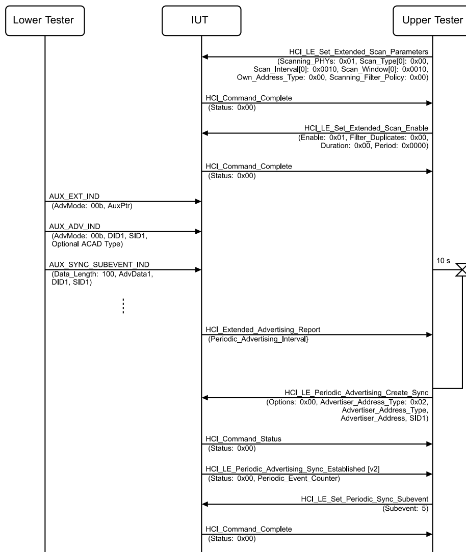
Figure 4.2-127: Synchronized Device Reconnects with an Advertiser using Periodic Advertising with Responses MSC – Page 1 of 2
