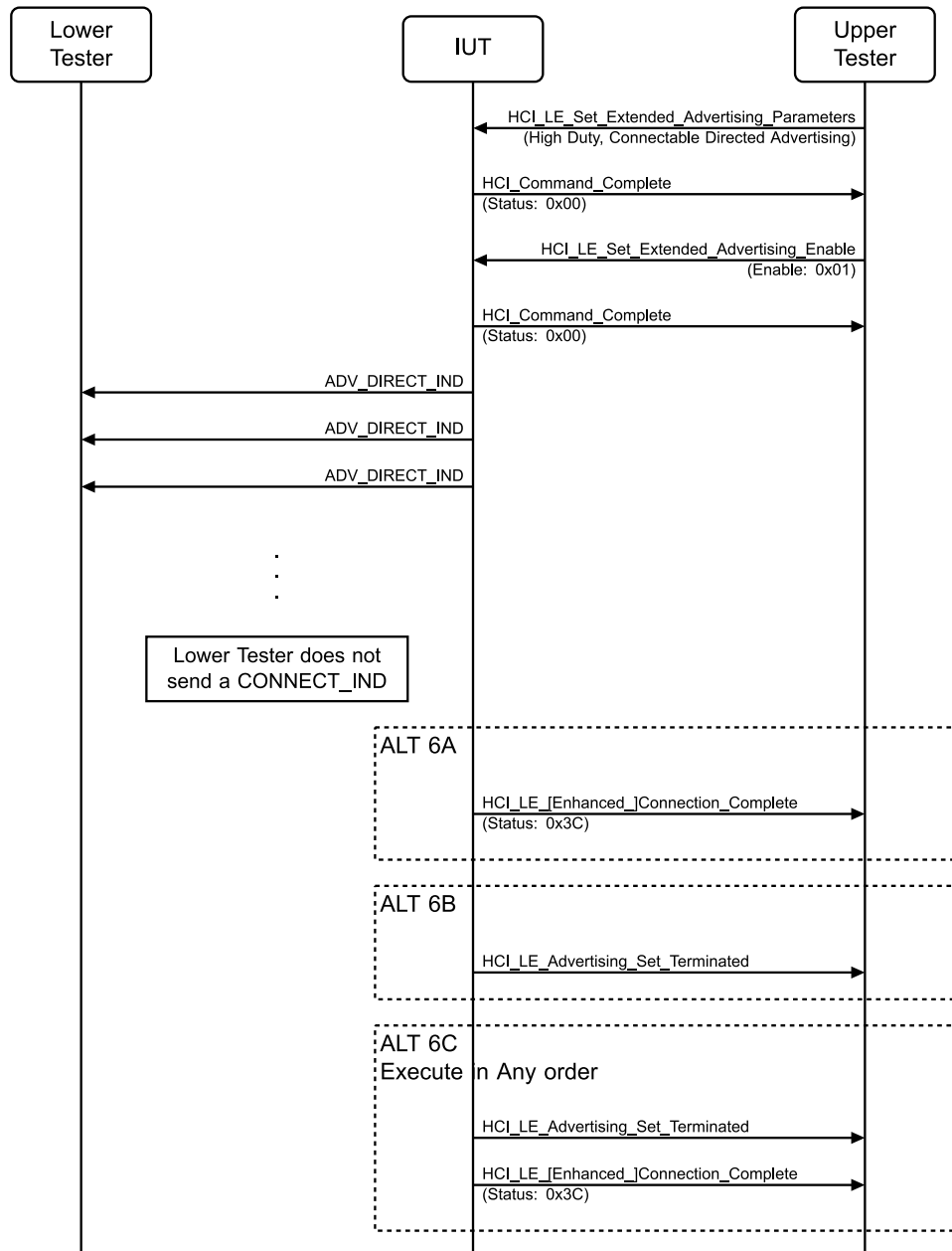
Figure 4.2-60: LL/DDI/ADV/BV-80-C [High Duty Cycle Connectable Directed Advertising, No Connection] MSC
