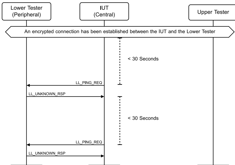
Figure 4.8-49: LL/SEC/CEN/BV-10-C [Initiate LE Ping procedure when the other side does not support the procedure] MSC
