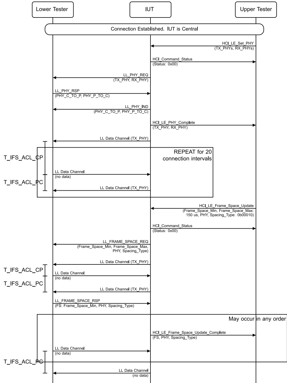
Figure 4.4-33: Initiate Inter Frame Space Change Request in the current ACL connection, Asymmetric PHYs, Peripheral Transmit, Central MSC – Page 1 of 2
