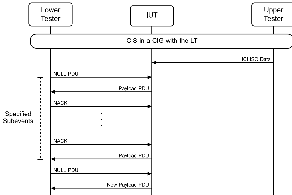
Figure 4.10-34: LL/CIS/PER/BV-14-C [Flushing of Packets in CIS, Peripheral] MSC
