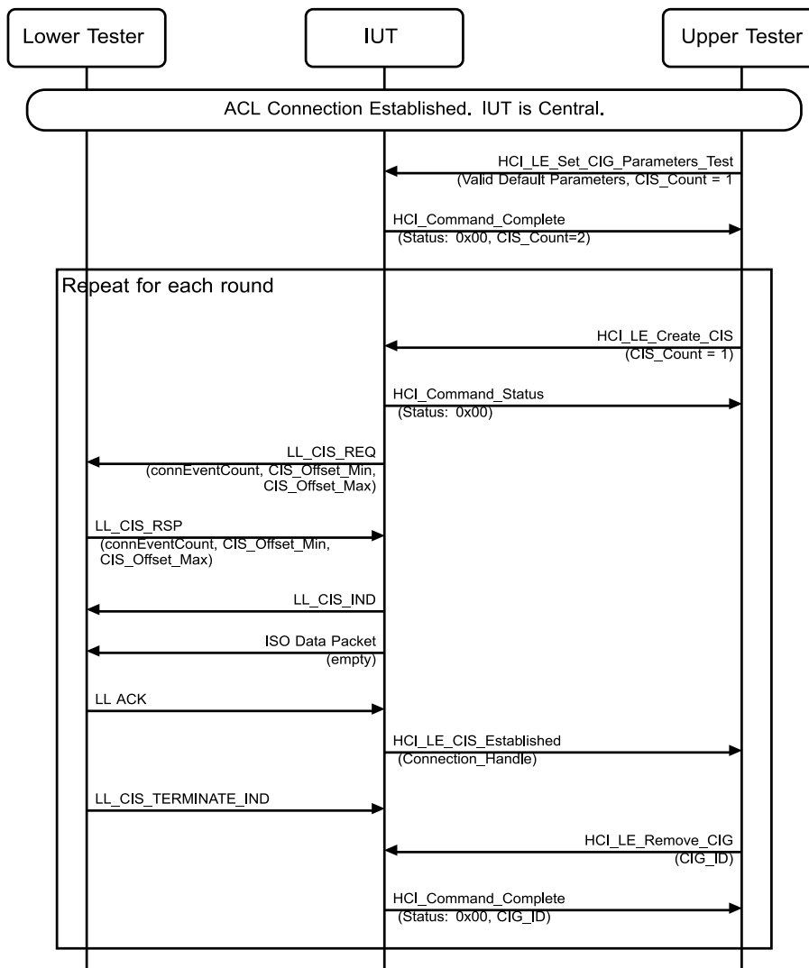
Figure 4.10-20: LL/CIS/CEN/BV-50-C [Connected Isochronous Stream, Central, CIS Offset] MSC
