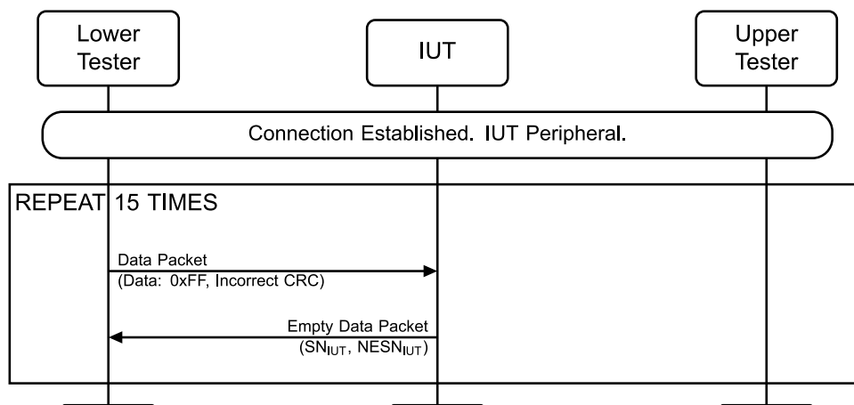
Figure 4.3-57: LL/CON/PER/BV-15-C [Peripheral retransmission request] MSC
