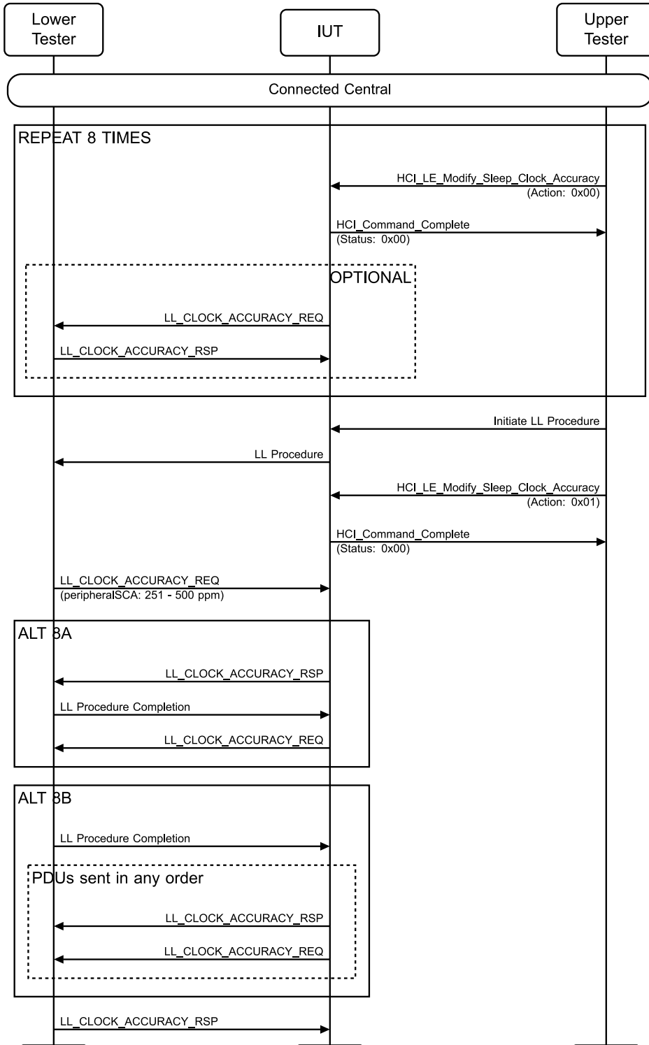
Figure 4.4-29: LL/TIM/CEN/BV-05-C [Response without Reducing the Sleep Clock Accuracy] MSC
