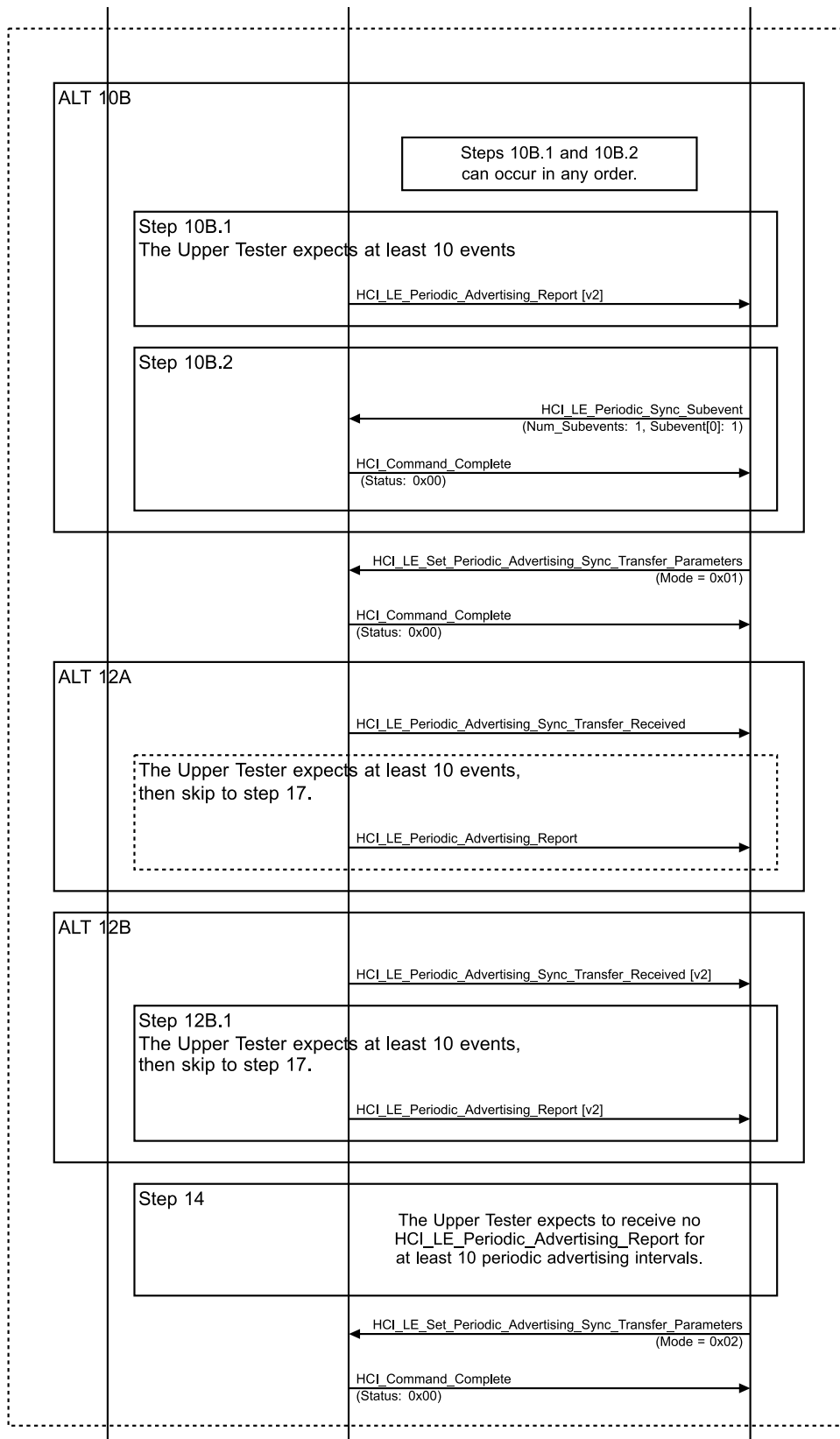
Figure 4.3-223: Periodic Advertising Sync Transfer Procedure, Accepting – Different Modes and Addresses MSC – Page 2 of 3
