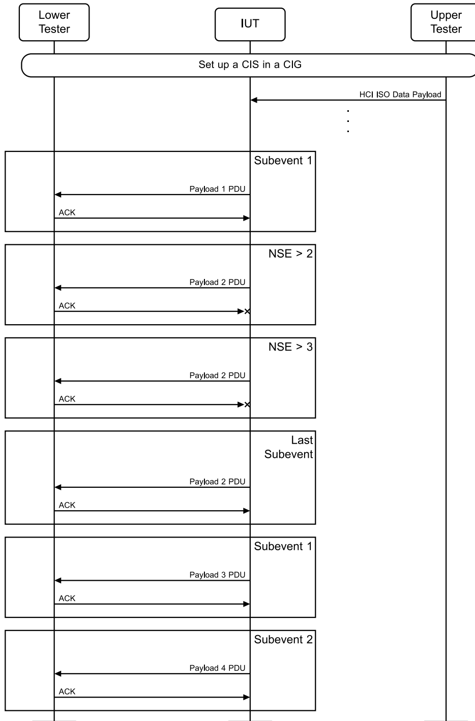
Figure 4.10-14: LL/CIS/CEN/BV-18-C [Bursting of Payloads in CIS, Central] MSC
