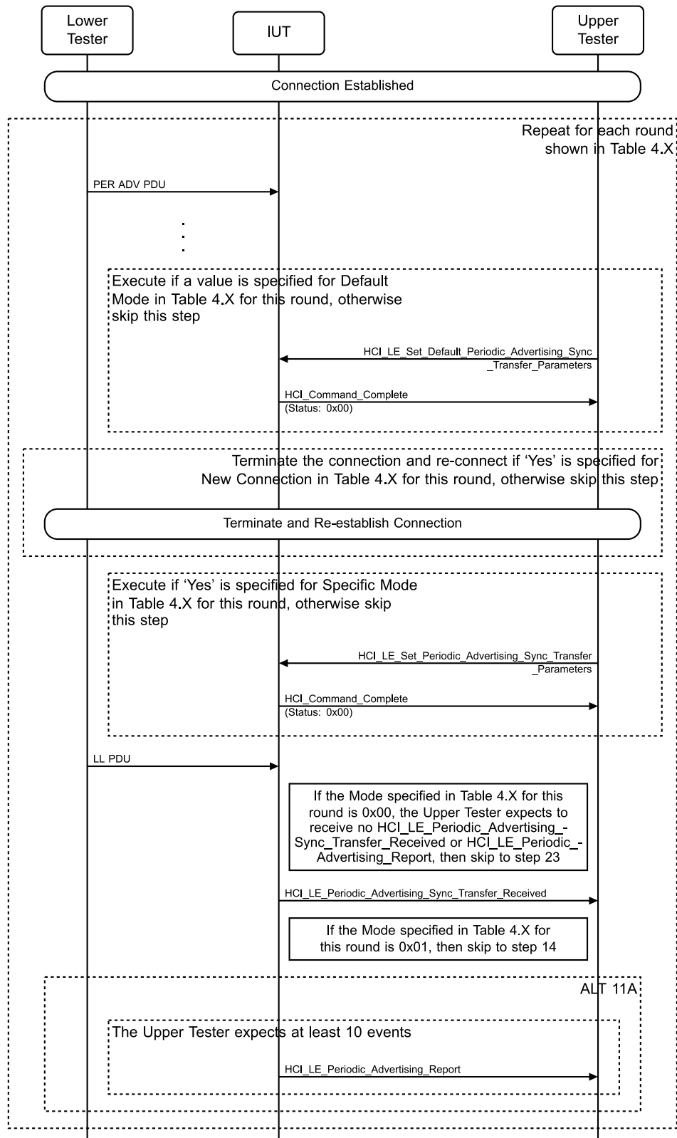
Figure 4.3-222: Periodic Advertising Sync Transfer Procedure, Accepting – Different Modes and Addresses MSC – Page 1 of 3
