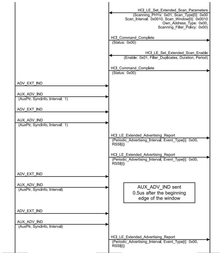
Figure 4.2-155: Extended Scanning, Passive, Periodic Advertising Report, Window Widening – Page 2 of 2
