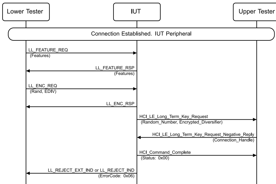
Figure 4.8-37: LL/SEC/PER/BV-11-C [Peripheral Sending LL_REJECT_EXT_IND] MSC
