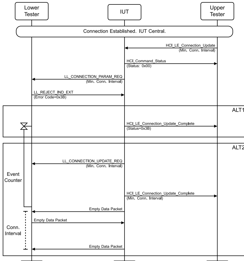
Figure 4.3-155: LL/CON/CEN/BV-25-C [Initiating Connection Parameter Request – Reject] MSC
