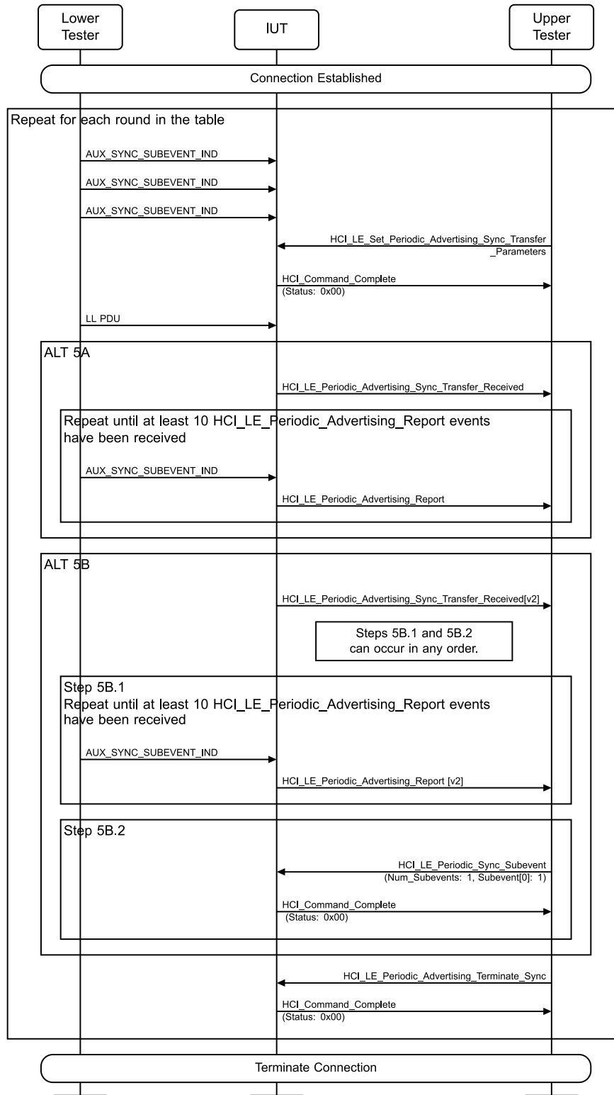
Figure 4.3-220: Periodic Advertising Sync Transfer Procedure, Accepting – Extreme Timings MSC
