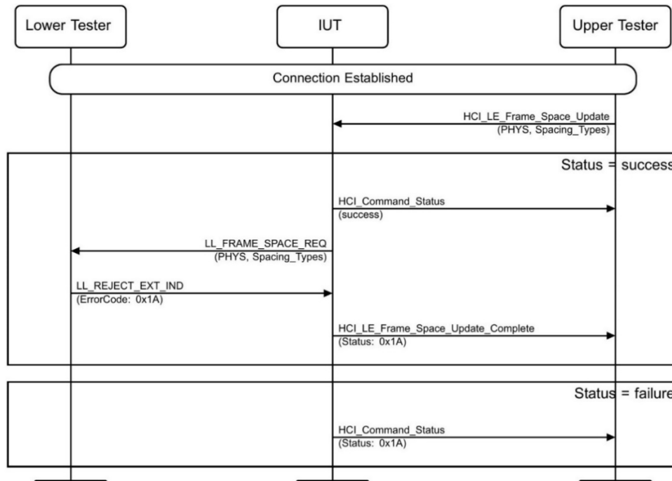
Figure 4.4-51: Frame Space Change, remote device does not support MSC
