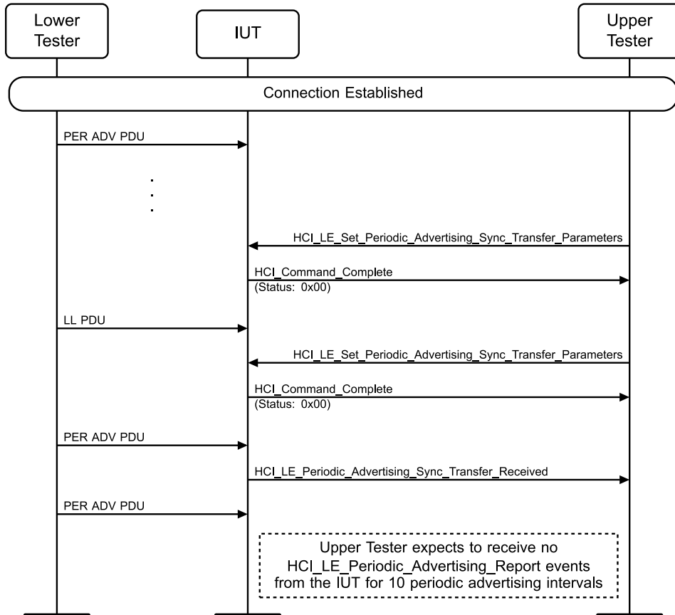
Figure 4.3-225: Periodic Advertising Sync Transfer Procedure, Accepting, Changing Transfer Mode during Synchronization MSC
