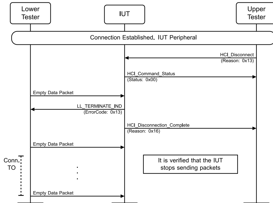
Figure 4.3-53: LL/CON/PER/BV-11-C [Peripheral sending termination] MSC
