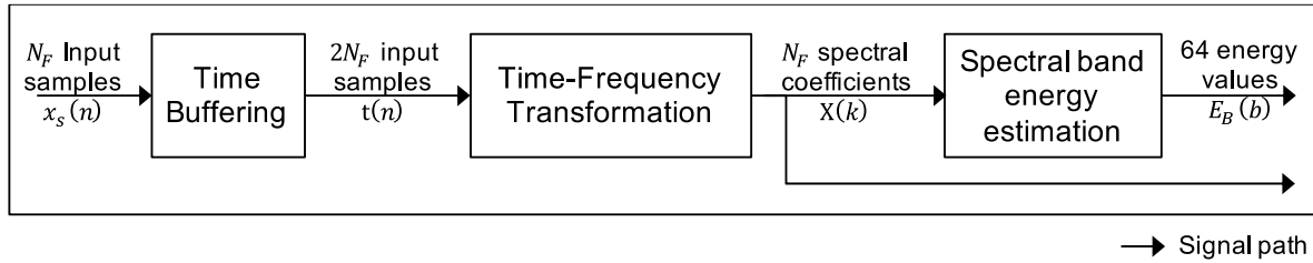
Figure 3.2: LD-MDCT overview
