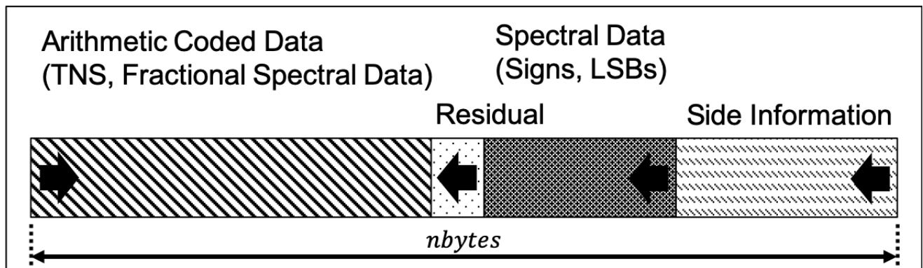
Figure 3.12: Frame structure
