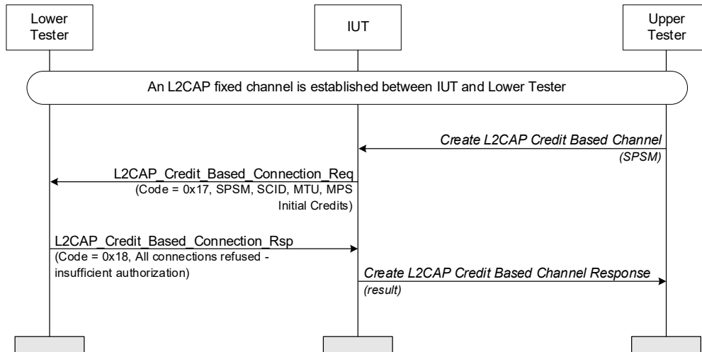
Figure 4.232: Security – Insufficient Authorization – Initiator MSC
