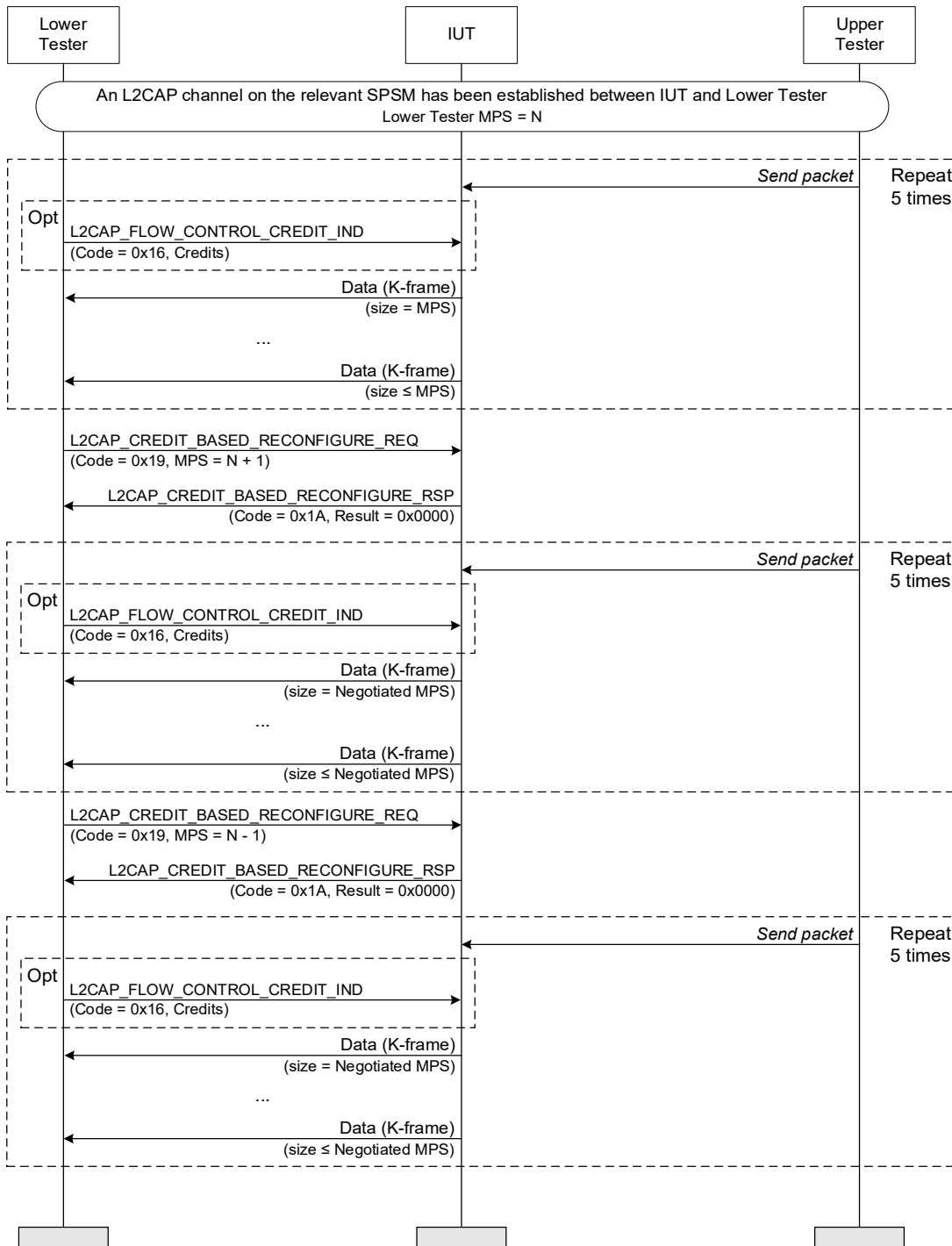
Figure 4.205: Renegotiate MPS – Responder MSC
