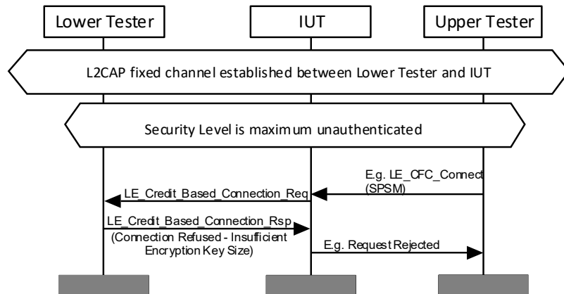
Figure 4.222: L2CAP/LE/CFC/BV-14-C [Security - Insufficient Encryption Key Size – Initiator] MSC
