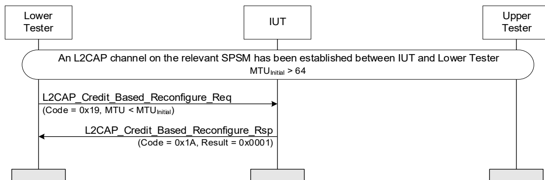
Figure 4.203: Renegotiate MTU – MTU value is decreased MSC
