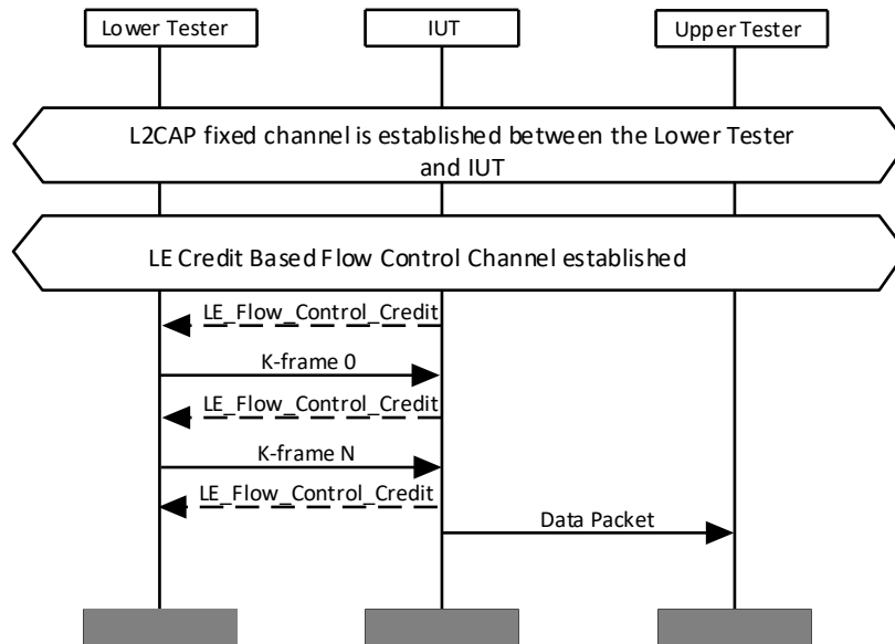
Figure 4.29: L2CAP/COS/CFC/BV-03-C [Reassembling] MSC
