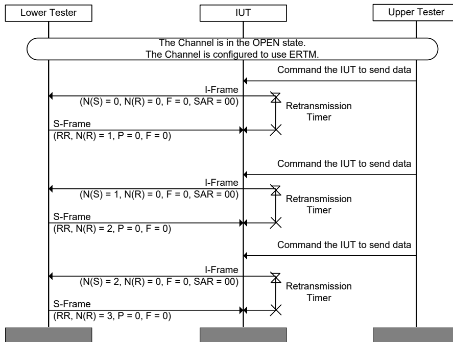
Figure 4.165: L2CAP/ECF/BV-02-C [Transmit I-Frames with Extended Control Field] MSC
