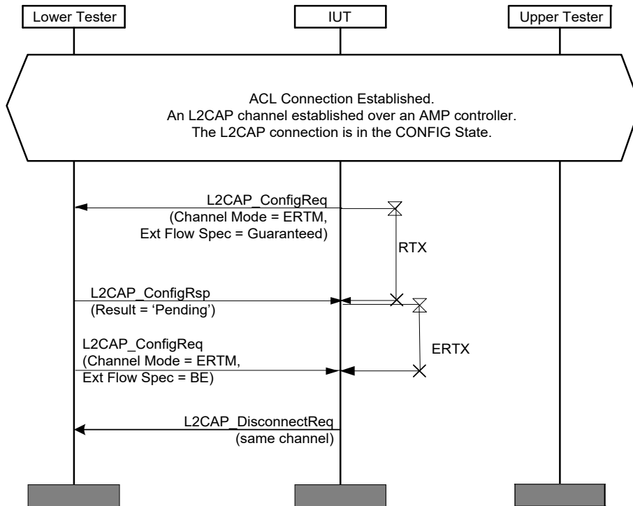
Figure 4.122: L2CAP/LSC/BI-11-C [Mismatched Service Type, Guaranteed, AMP Channel] MSC
