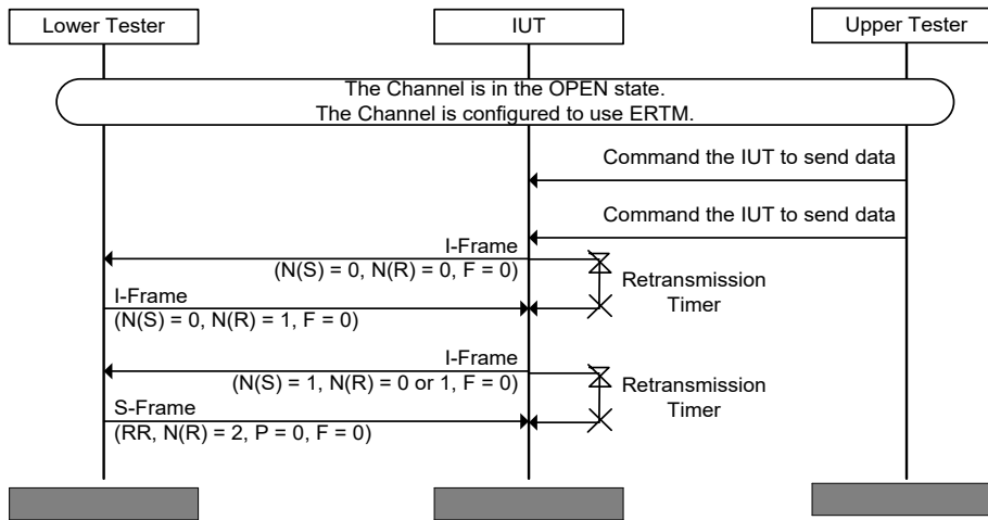
Figure 4.81: L2CAP/ERM/BV-06-C [Resume Transmitting I-Frames when an I-Frame is Received] MSC
