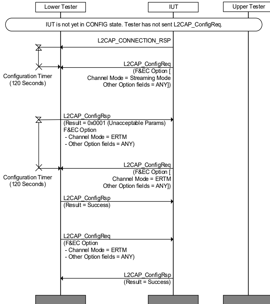
Figure 4.64: L2CAP/CMC/BV-14-C [Failed Configuration of Streaming Mode when use of the mode is optional and ERTM is proposed by the Lower Tester] MSC
