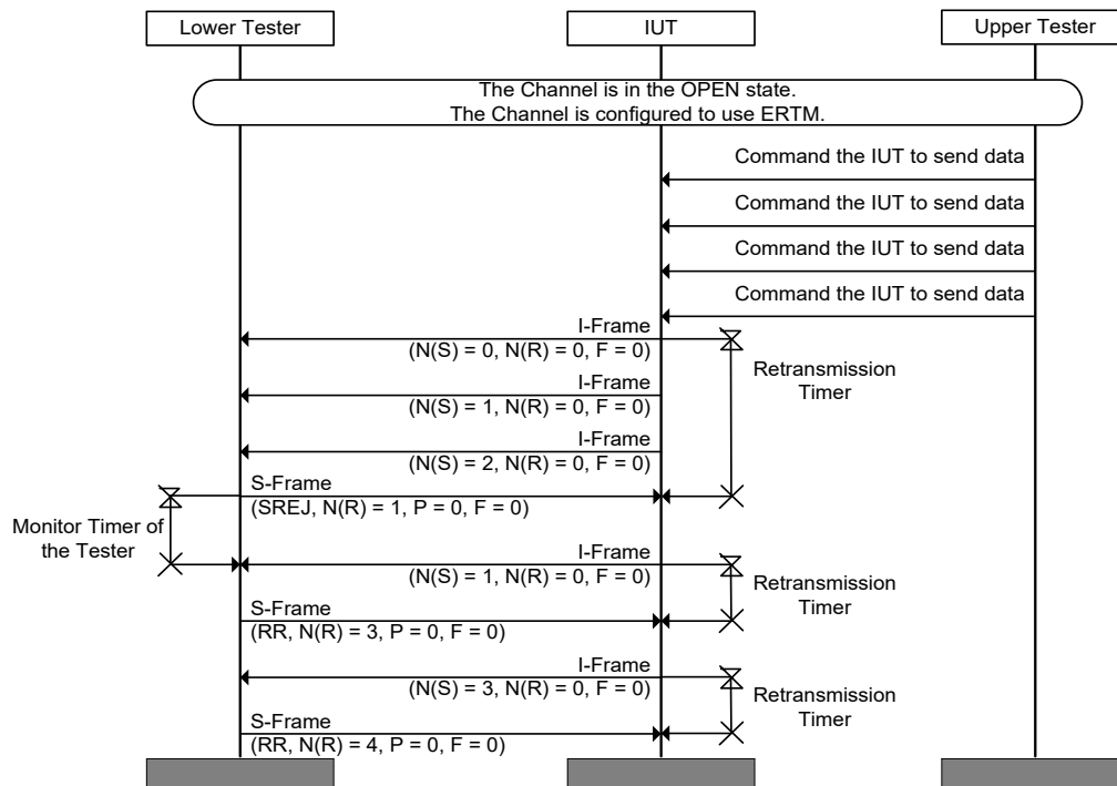
Figure 4.170: L2CAP/ECF/BV-07-C [Respond to S-Frame [SREJ] with Extended Control Field and POLL Bit Clear] MSC
