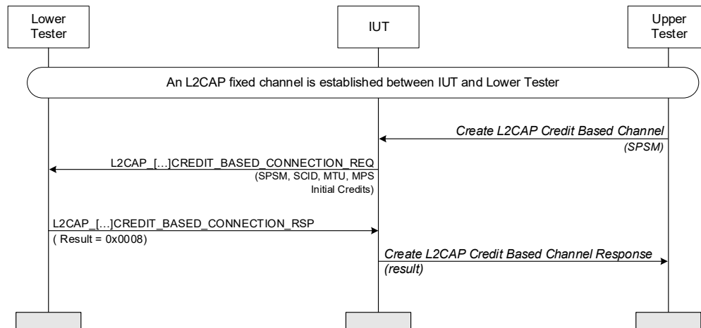
Figure 4.238: Security – Insufficient Encryption – Initiator MSC
