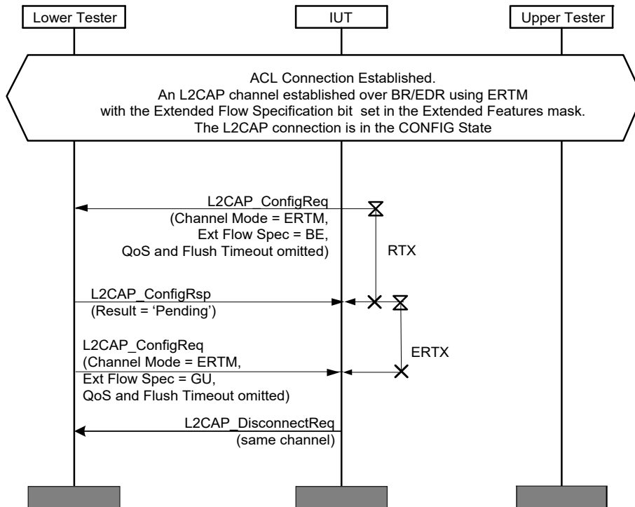
Figure 4.115: L2CAP/LSC/BI-04-C [Mismatched Service Type, Best Effort, BR/EDR ERTM Channel] MSC
