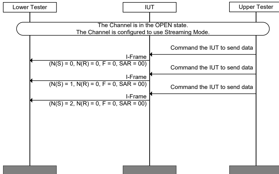
Figure 4.103: L2CAP/STM/BV-01-C [Streaming Mode Source] MSC
