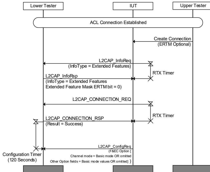
Figure 4.60: L2CAP/CMC/BV-10-C [ERTM Not Supported by Lower Tester for Optional ERTM Channel] MSC
