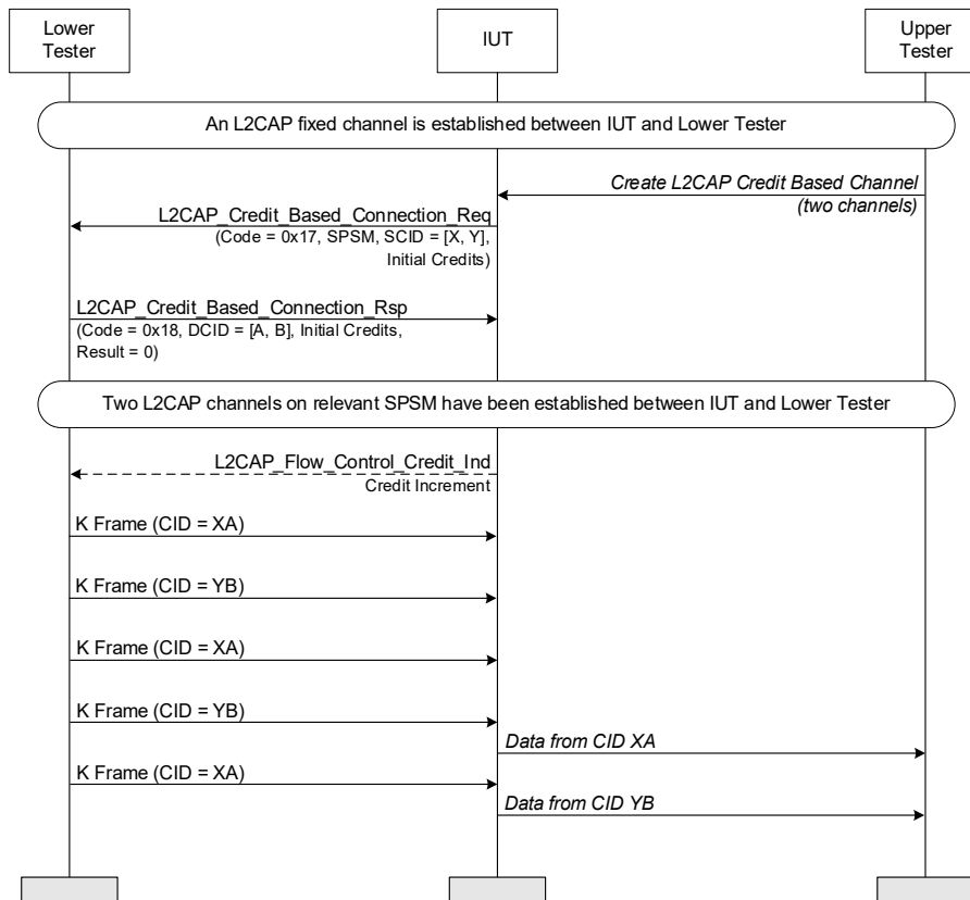
Figure 4.35: Multiple Channels with Interleaved Data Streams MSC
