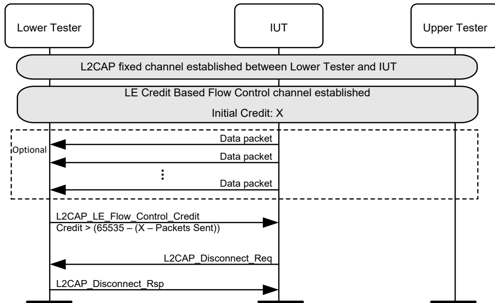
Figure 4.220: L2CAP/LE/CFC/BI-01-C [Credit Exchange – Exceed Initial Credits] MSC
