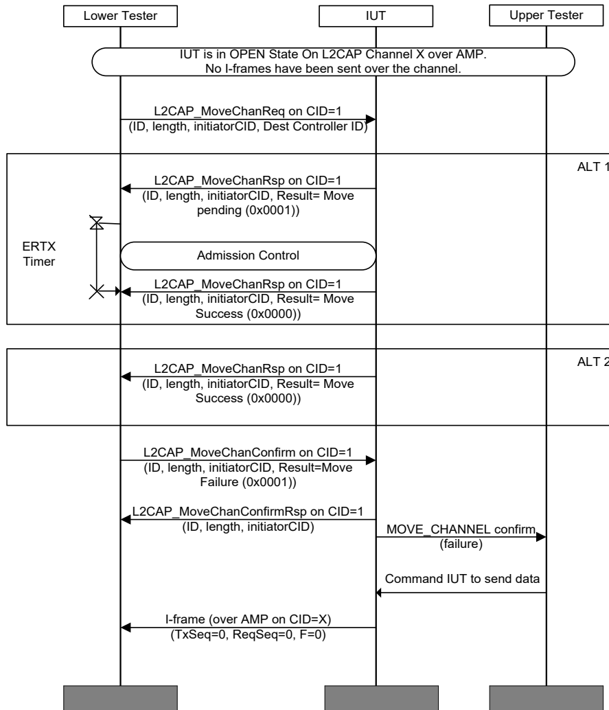
Figure 4.160: L2CAP/MCH/BV-33-C [Move Channel Response for AMP to BR/EDR (STM Source) – Failed] MSC
