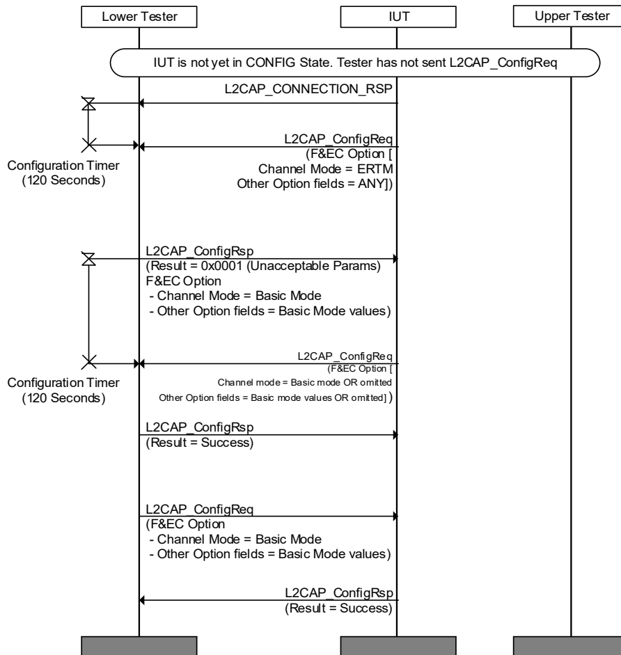
Figure 4.47: L2CAP/CMC/BV-03-C [Failed Configuration of Enhanced Retransmission Mode when use of the Mode is Optional] MSC
