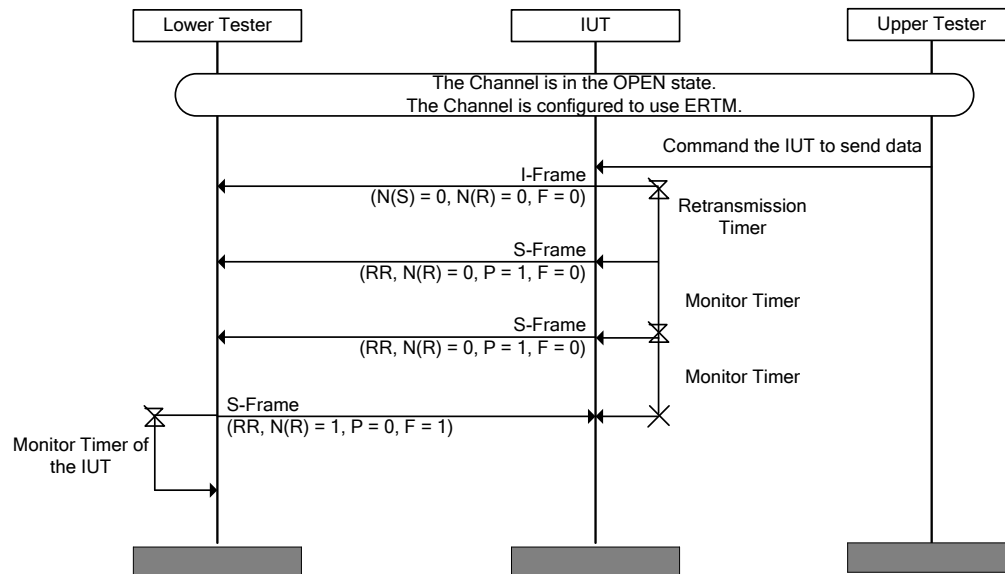
Figure 4.85: L2CAP/ERM/BV-10-C [Retransmit S-Frame [RR] with Poll Bit Set] MSC
