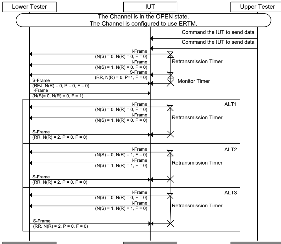
Figure 4.102: L2CAP/ERM/BI-05-C [Handle receipt of S-Frame [REJ] and I-Frame [F=1] that Both Require Retransmission of the Same I-Frames] MSC
