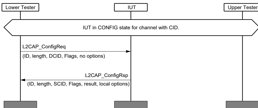
Figure 4.14: L2CAP/COS/CFD/BV-03-C [Send Requested Options] MSC
