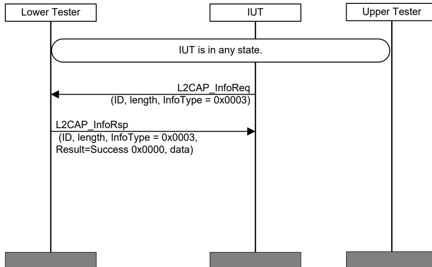
Figure 4.106: L2CAP/FIX/BV-01-C [Fixed Channels Supported Information Request] MSC
