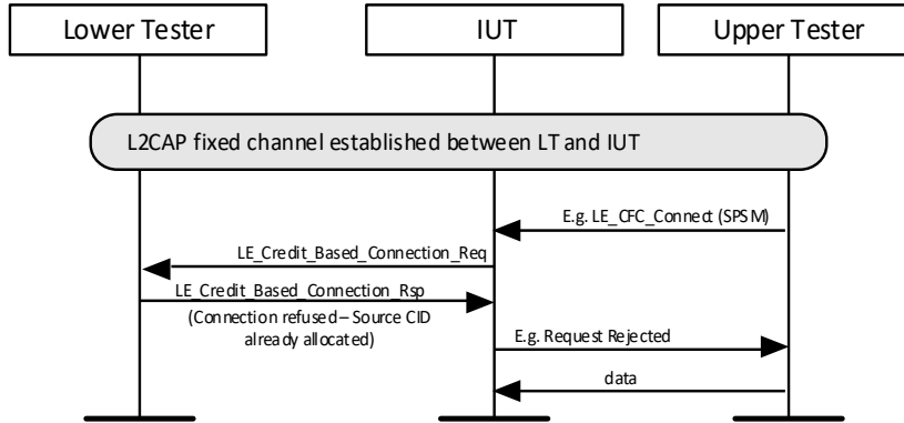
Figure 4.225: L2CAP/LE/CFC/BV-19-C [LE Credit Based Connection Request - refused due to source CID already allocated - Initiator] MSC
