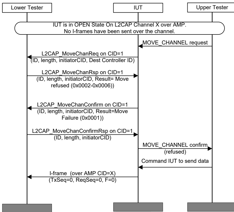
Figure 4.150: L2CAP/MCH/BV-23-C [Move Channel Request for AMP to BR/EDR (STM Source) – Refused] MSC
