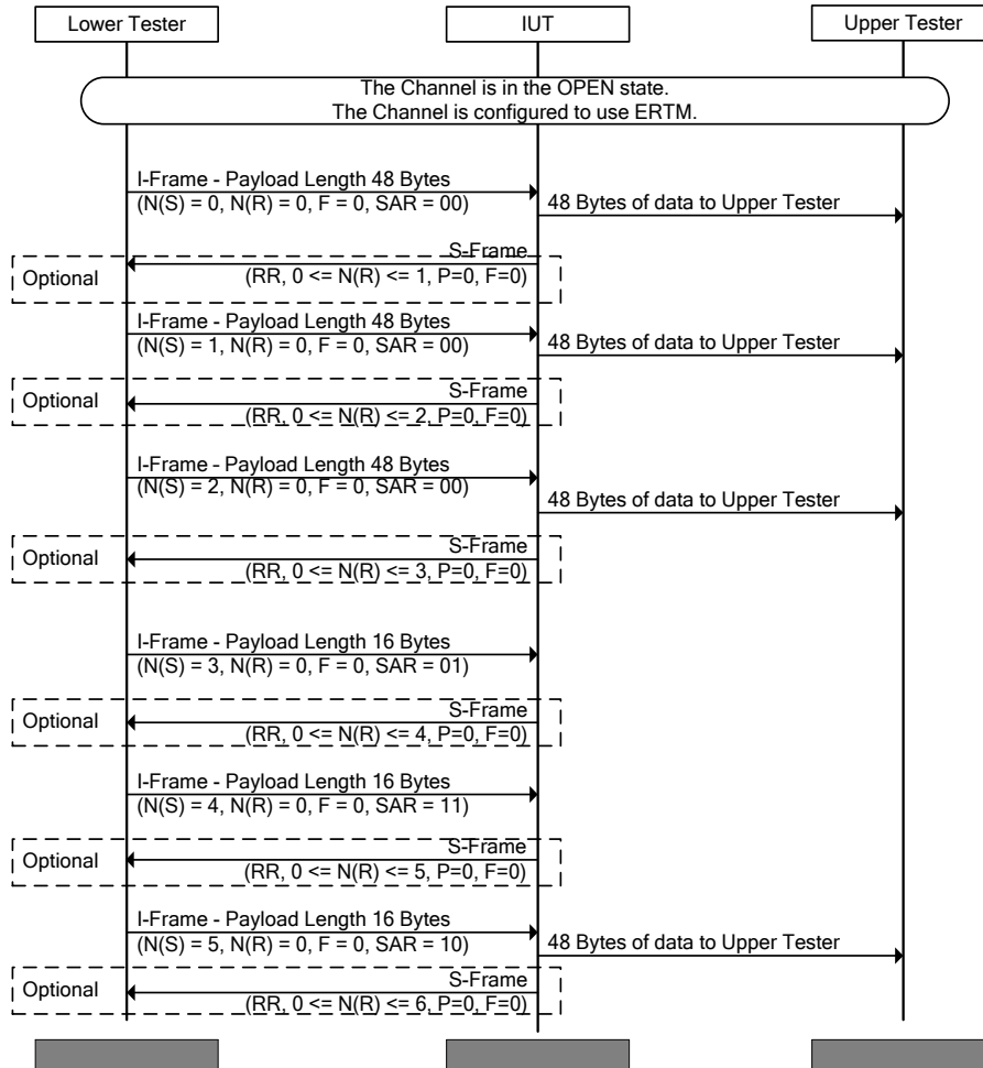
Figure 4.78: L2CAP/ERM/BV-02-C [Receive I-Frames] MSC
