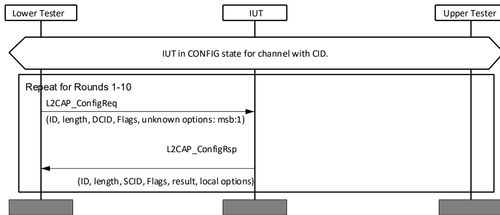
Figure 4.19: L2CAP/COS/CFD/BV-12-C [Unknown Option Response] MSC
