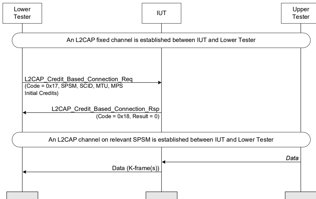
Figure 4.188: L2CAP Credit Based Connection Response on Supported PSM MSC
