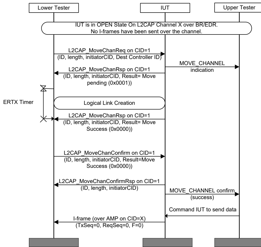
Figure 4.154: L2CAP/MCH/BV-27-C [Move Channel Response for BR/EDR to AMP (STM Source) – Success] MSC
