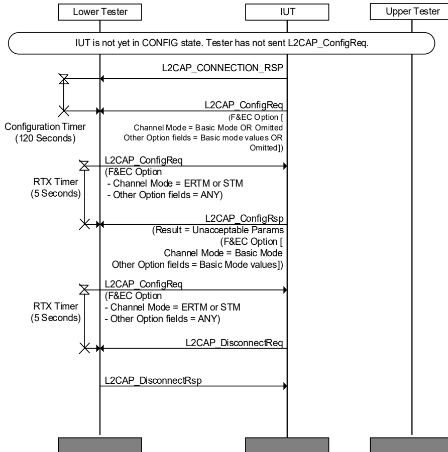
Figure 4.58: L2CAP/CMC/BI-05-C [Failed Configuration to Basic Mode by the IUT] MSC
