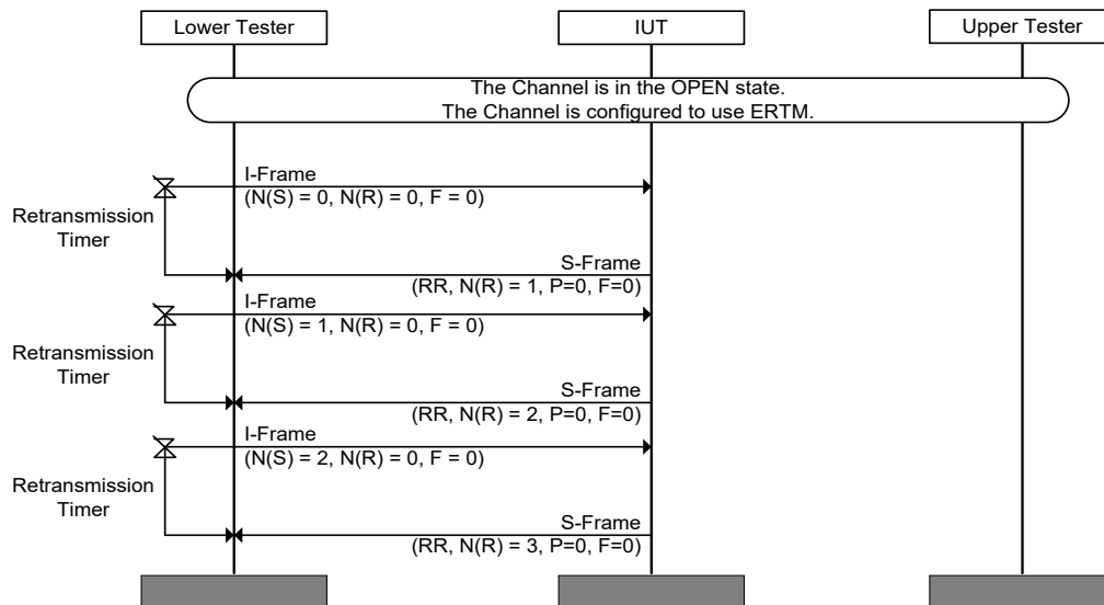
Figure 4.166: L2CAP/ECF/BV-03-C [Acknowledging Received I-Frames with Extended Control Field] MSC
