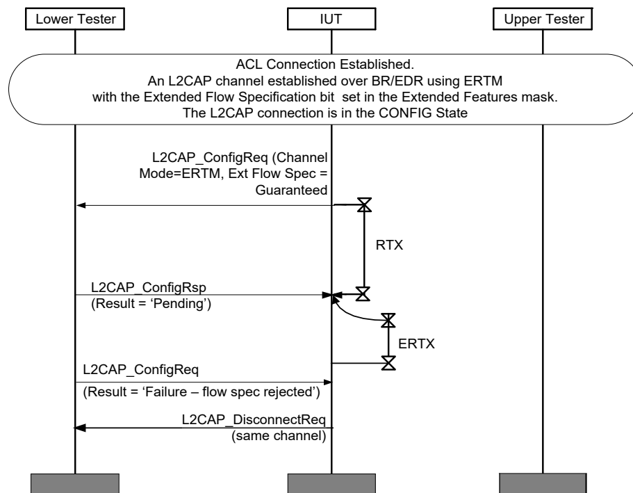
Figure 4.117: L2CAP/LSC/BV-06-C [Remote Failed on Guaranteed, BR/EDR ERTM Channel] MSC
