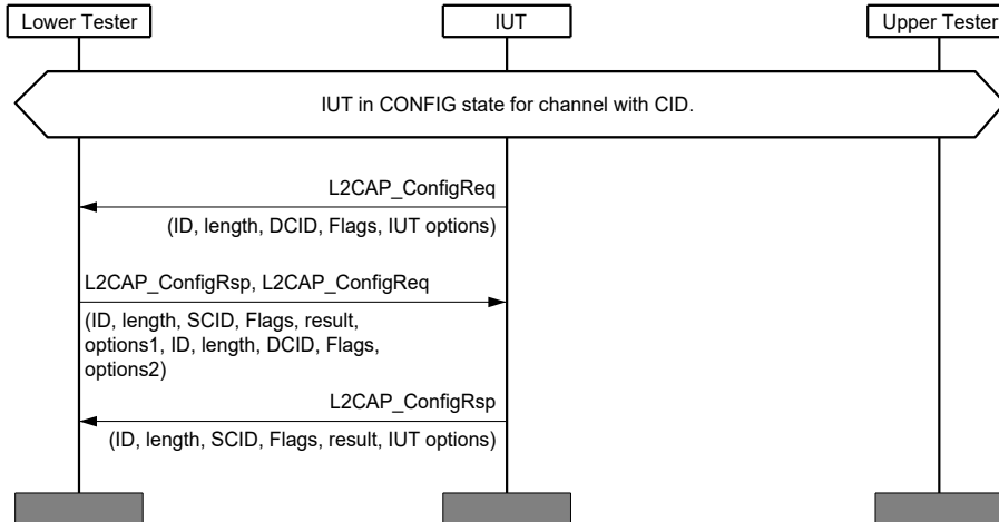
Figure 4.20: L2CAP/COS/CFD/BV-13-C [Flow Control Mode Negotiation] MSC
