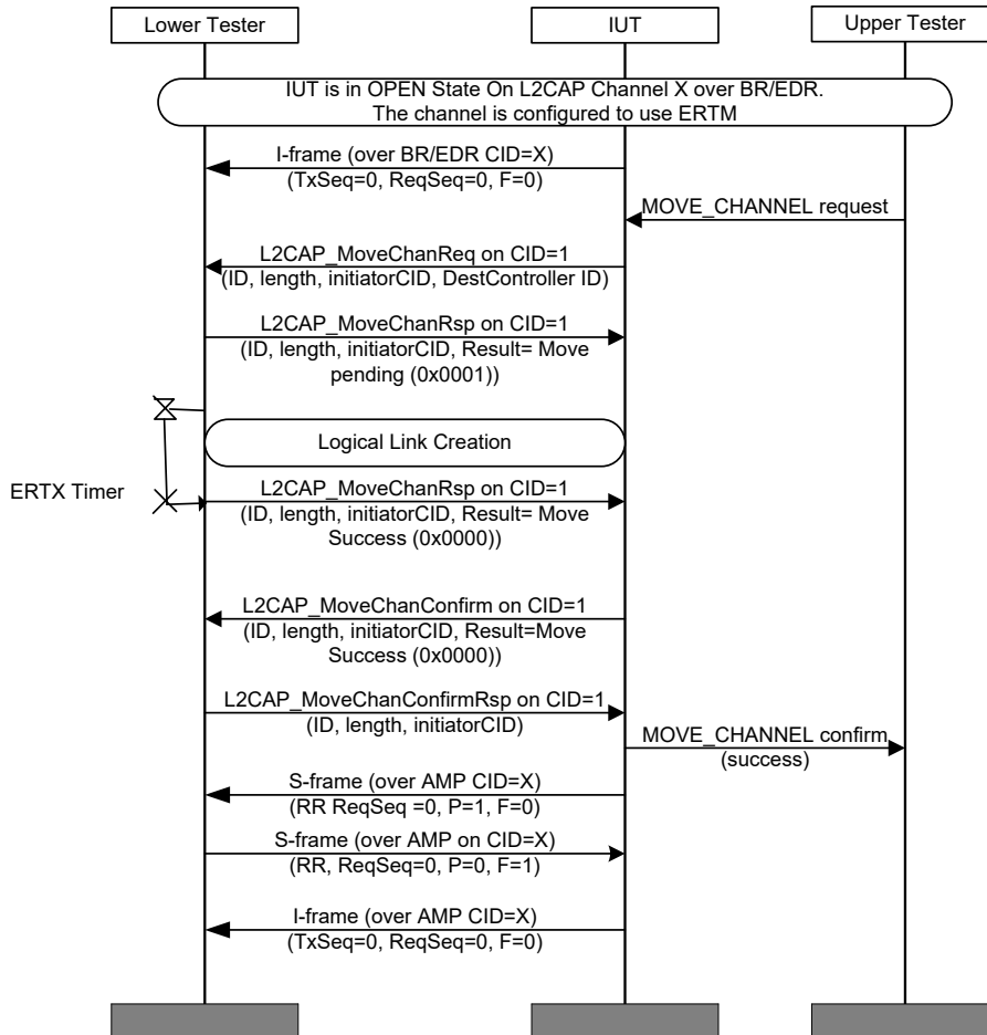
Figure 4.138: L2CAP/MCH/BV-11-C [Data Transfer while Moving ERTM Channel from BR/EDR to AMP – Unacknowledged Data] MSC
