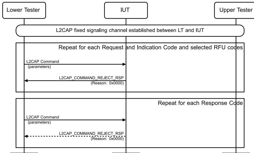
Figure 4.179: Reject Unknown Command MSC
