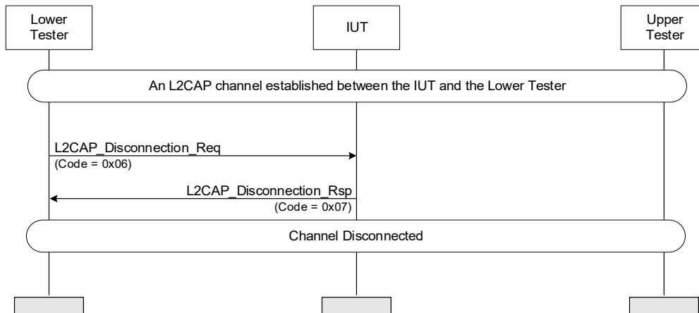
Figure 4.230: Disconnect Response MSC
