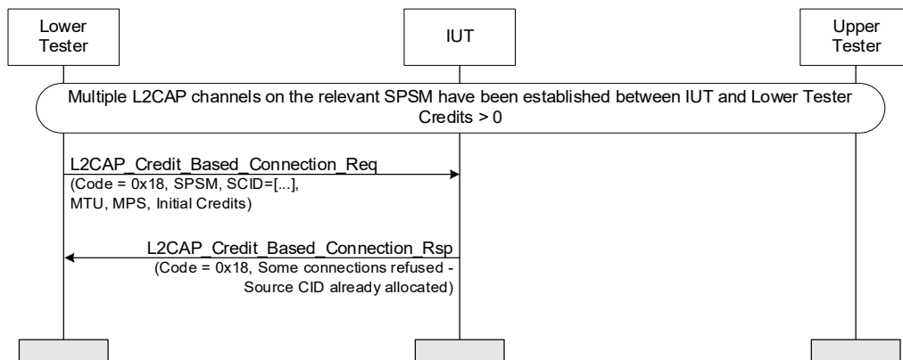
Figure 4.199: L2CAP Credit Based Connection Response – refused due to Source CID already allocated MSC
