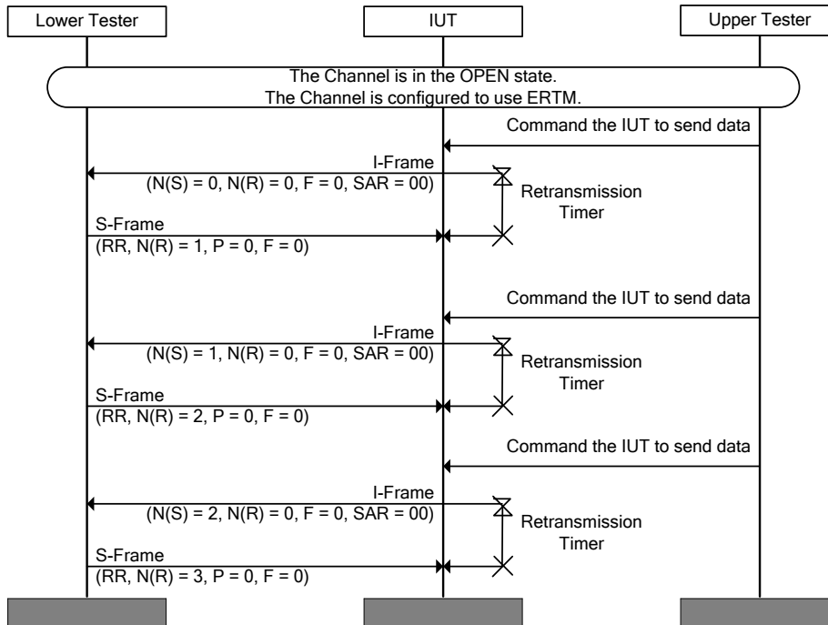
Figure 4.77: L2CAP/ERM/BV-01-C [Transmit I-frames] MSC
