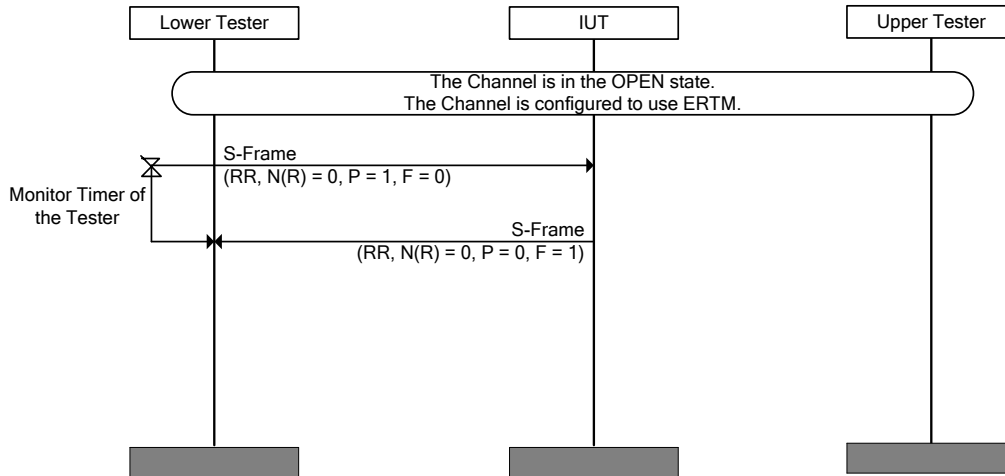
Figure 4.84: L2CAP/ERM/BV-09-C [Send S-frame [RR] with Final Bit Set] MSC
