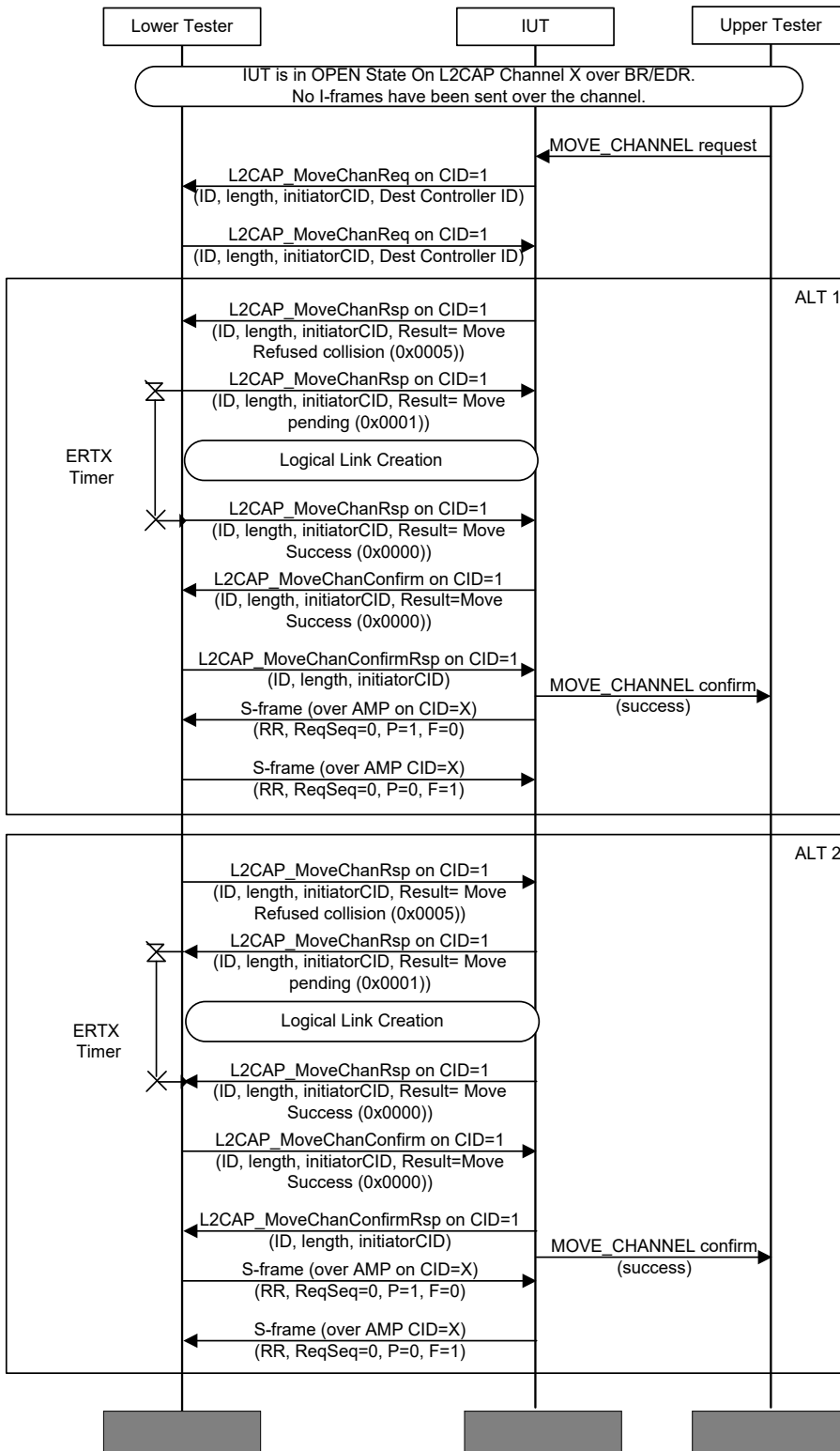
Figure 4.141: L2CAP/MCH/BV-14-C [Move Collision – ERTM] MSC
