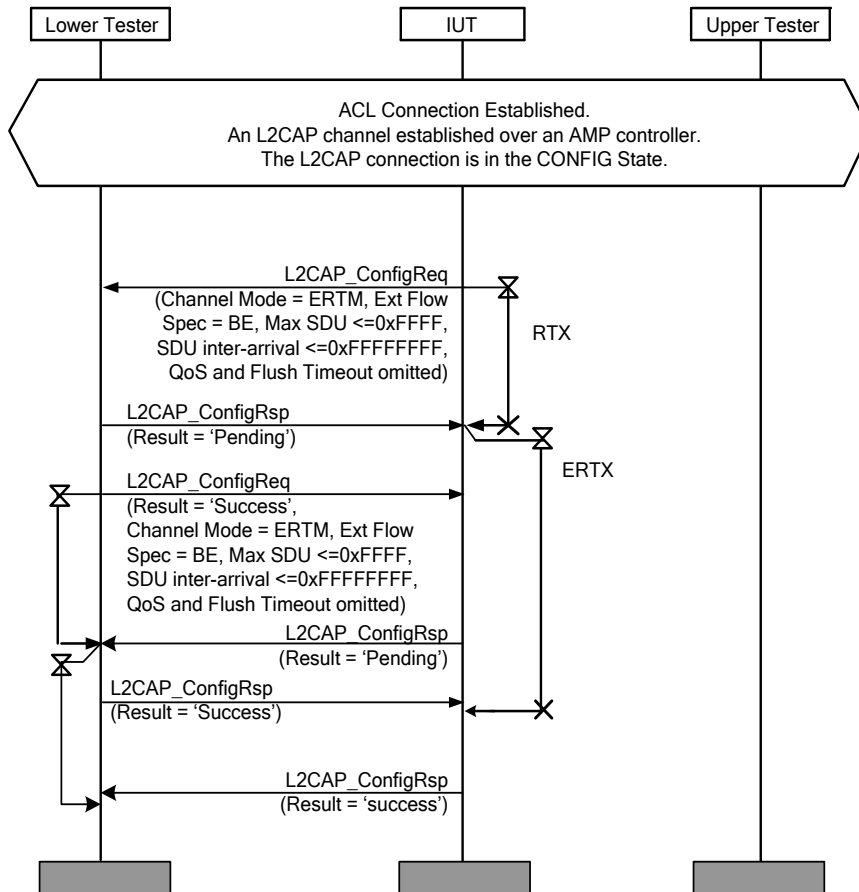
Figure 4.118: L2CAP/LSC/BV-07-C [Normal Lock Step Configuration Process for Best Effort, AMP Channel] MSC
