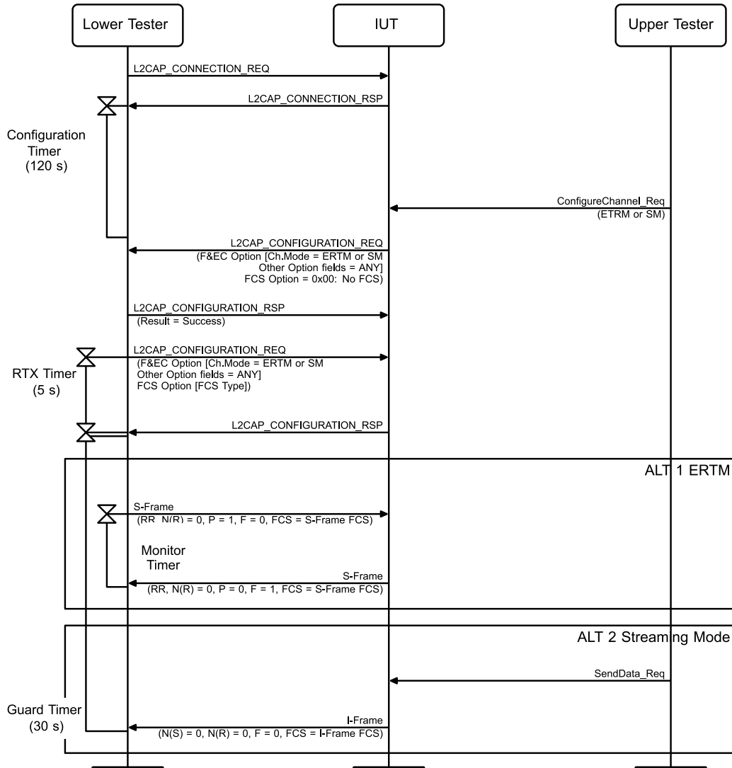
Figure 4.66: IUT Initiated Configuration of the FCS Option, IUT No FCS MSC
