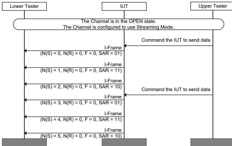
Figure 4.174: L2CAP/STM/BV-13-C [Streaming Mode Source using Extended Control Field and SAR] MSC
