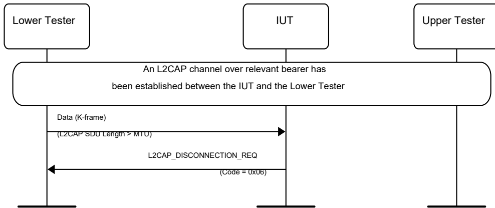
Figure 4.240: K-frame - SDU length greater than MTU of IUT MSC
