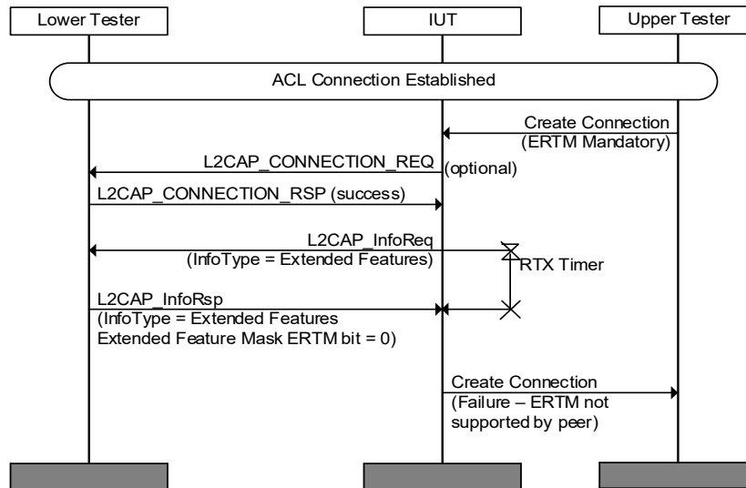
Figure 4.62: L2CAP/CMC/BV-12-C [ERTM Not Supported by Lower Tester for Mandatory ERTM channel] MSC
