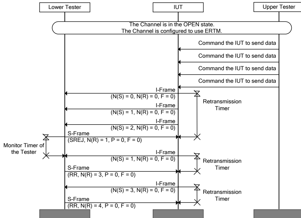
Figure 4.90: L2CAP/ERM/BV-15-C [Respond to S-Frame [SREJ] POLL bit clear] MSC
