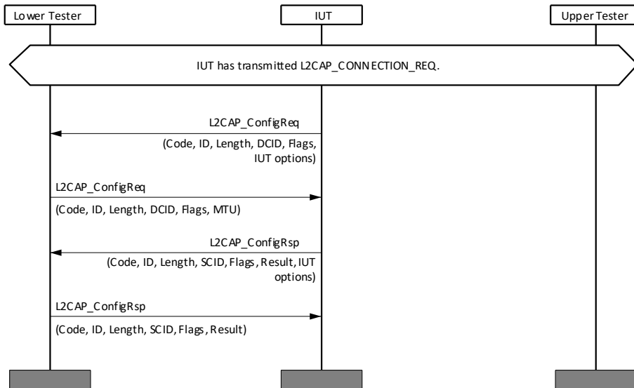
Figure 4.15: L2CAP/COS/CFD/BV-08-C [Non-blocking Config Response] MSC
