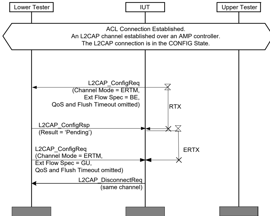
Figure 4.121: L2CAP/LSC/BV-10-I [Mismatched Service Type, Best Effort, AMP Channel] MSC
