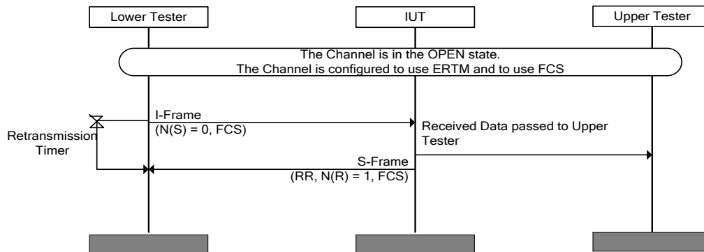
Figure 4.74: L2CAP/OFS/BV-06-C [Receiving Frames with FCS for ERTM] MSC
