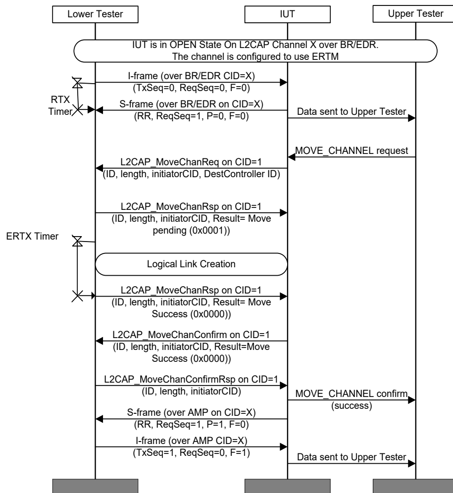
Figure 4.137: L2CAP/MCH/BV-10-C [Data Transfer while Moving ERTM Channel from BR/EDR to AMP] MSC
