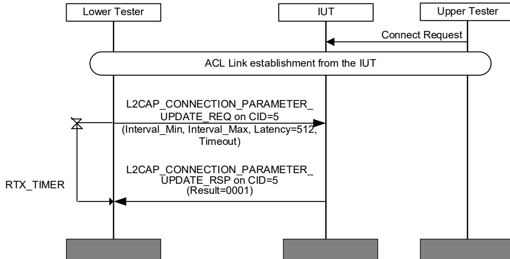
Figure 4.177: L2CAP/LE/CPU/BI-01-C [Reject Connection Parameter Update Parameters] MSC
