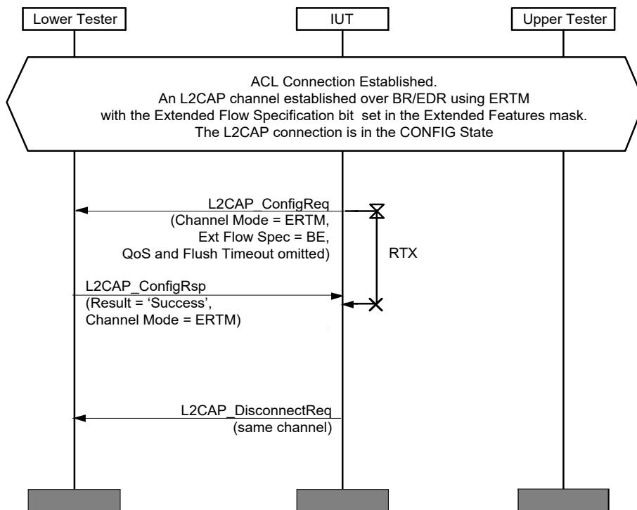
Figure 4.114: L2CAP/LSC/BV-03-C [Premature Success in Configuration Response, BR/EDR ERTM Channel] MSC
