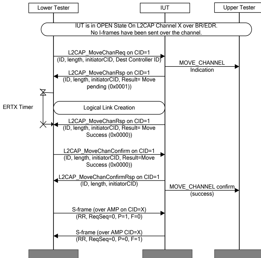
Figure 4.133: L2CAP/MCH/BV-06-C [Move ERTM Channel Response for BR/EDR to AMP – Success] MSC
