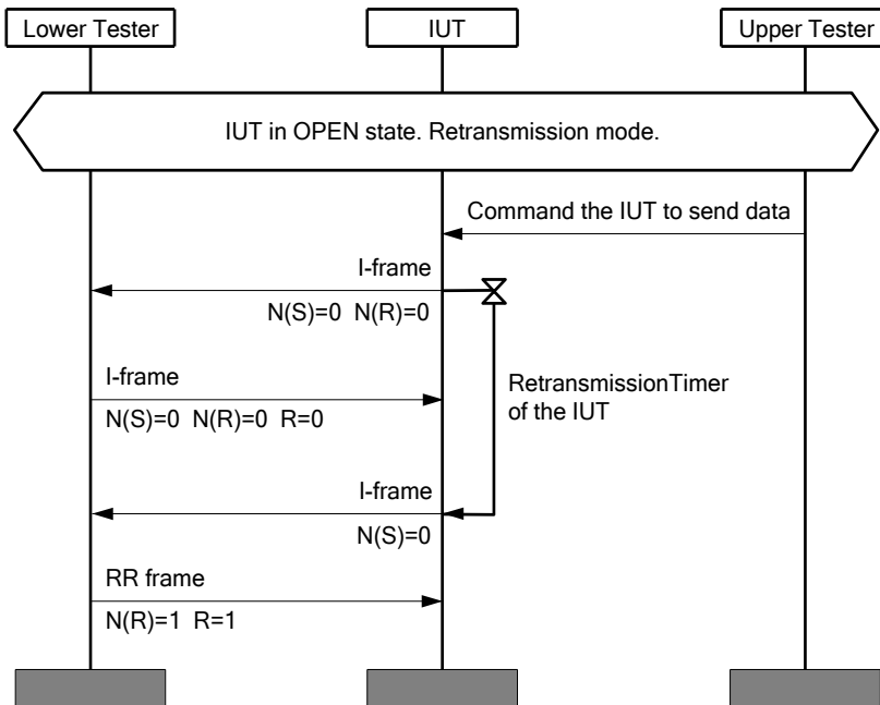
Figure 4.42: L2CAP/COS/RTX/BV-03-C [Retransmission with R=0 in I-frame] MSC
