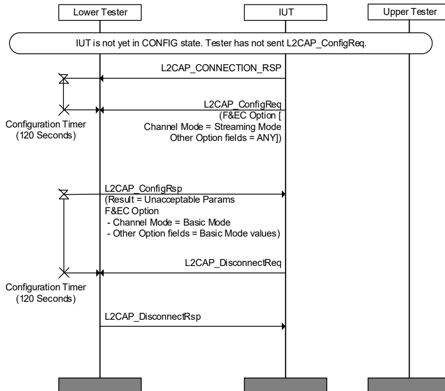
Figure 4.56: L2CAP/CMC/BI-03-C [Failed Configuration of Streaming Mode when use of the Mode is Mandatory] MSC
