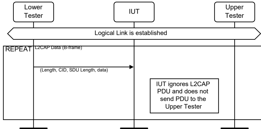
Figure 4.184: Ignore Unsupported CIDs MSC
