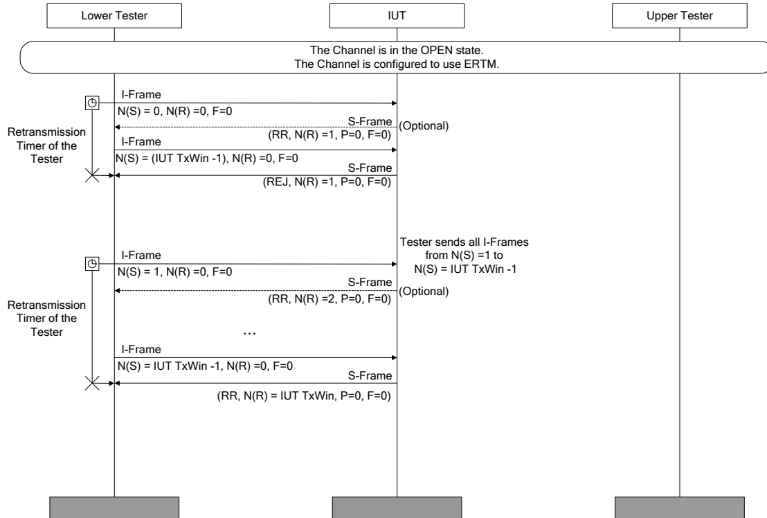
Figure 4.91: L2CAP/ERM/BV-16-C [Send S-Frame [REJ]] MSC
