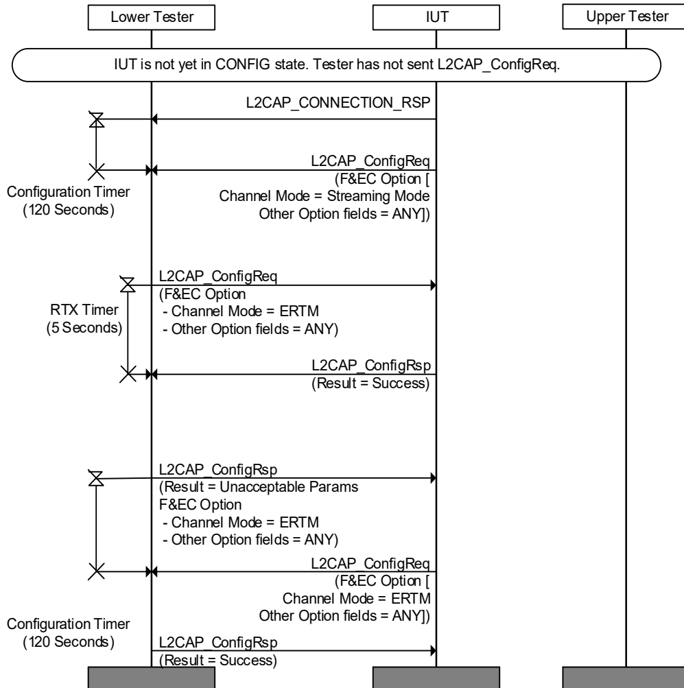
Figure 4.65: L2CAP/CMC/BV-15-C [Configuration Mode Mismatch when use of Streaming Mode is Optional and ERTM is proposed by the Lower Tester] MSC
