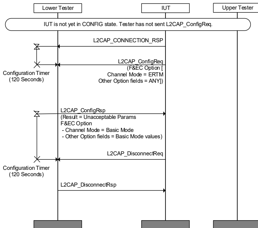
Figure 4.54: L2CAP/CMC/BI-01-C [Failed Configuration of Enhanced Retransmission Mode when use of the Mode is Mandatory] MSC
