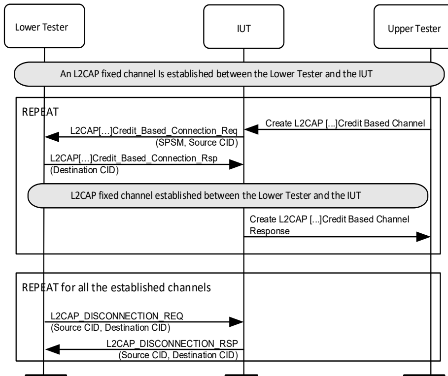
Figure 4.228: Credit Based Connection Request Dynamically Allocated Source CID MSC
