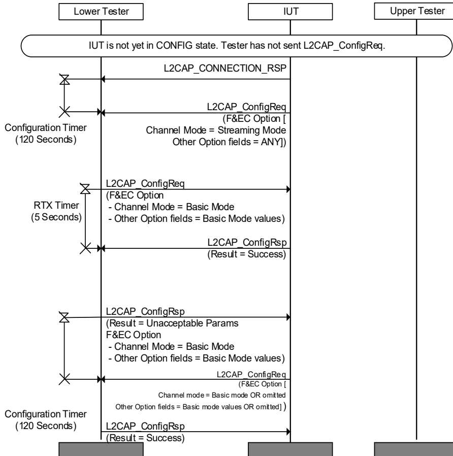
Figure 4.52: L2CAP/CMC/BV-08-C [Configuration Mode Mismatch when use of Streaming Mode is Optional] MSC
