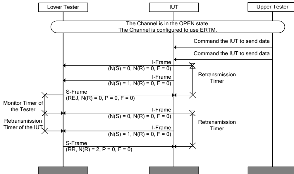
Figure 4.88: L2CAP/ERM/BV-13-C [Respond to S-Frame [REJ]] MSC
