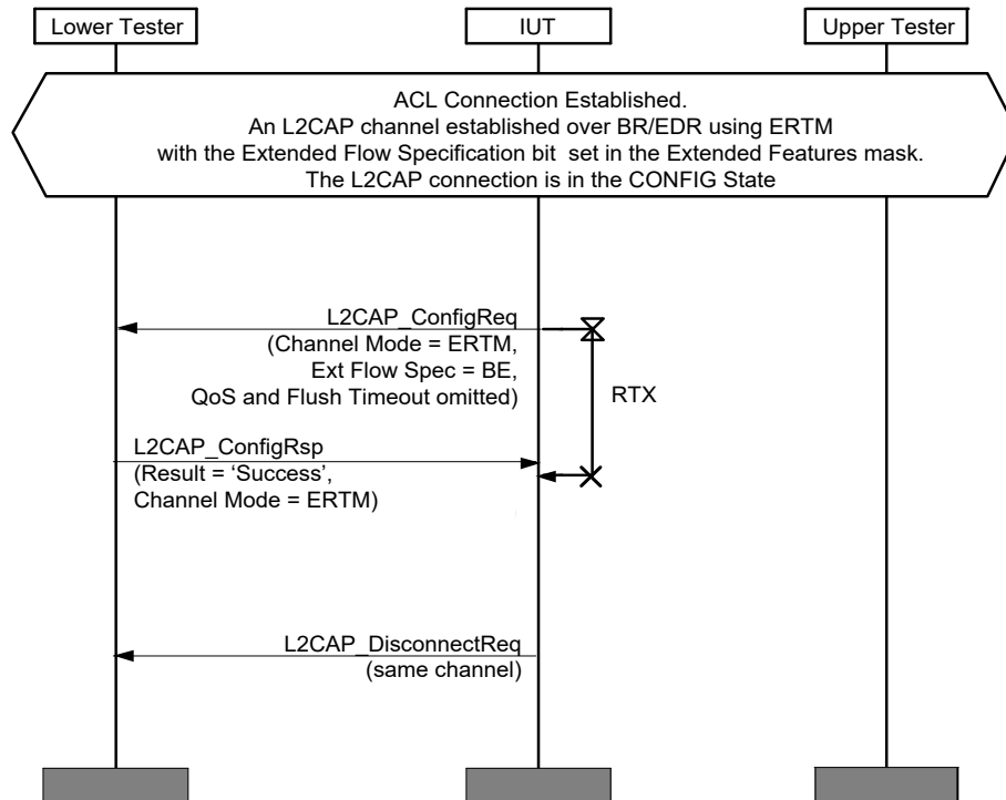
Figure 4.112: L2CAP/LSC/BV-01-C [Normal Lock Step Configuration Process for Best Effort, BR/EDR ERTM Channel] MSC
