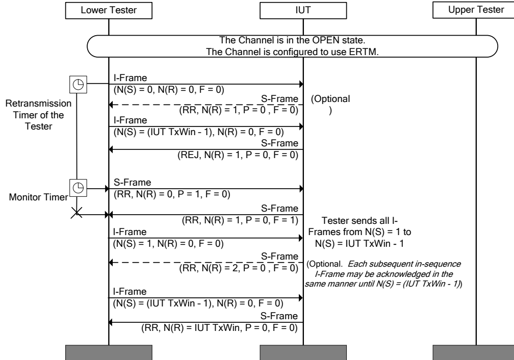
Figure 4.98: L2CAP/ERM/BI-01-C [S-Frame [REJ] Lost or Corrupted] MSC
