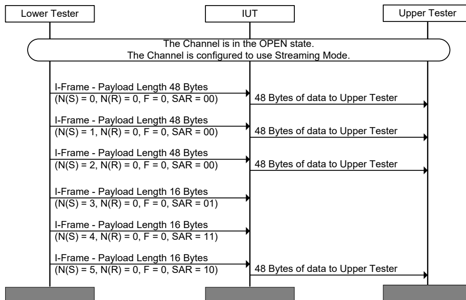
Figure 4.173: L2CAP/STM/BV-02-C [Streaming Mode Sink with Extended Control Field] MSC
