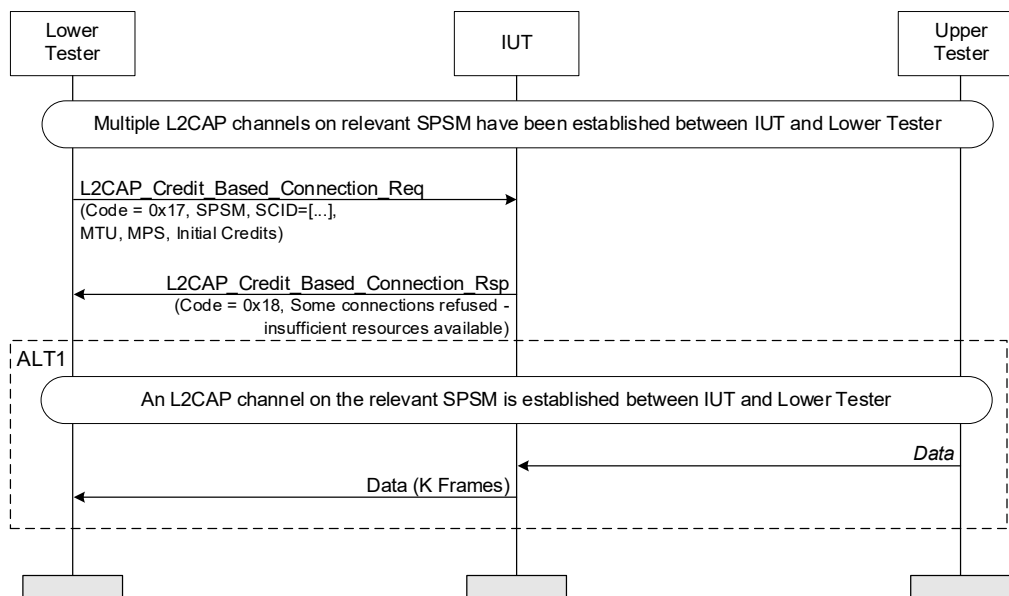
Figure 4.196: L2CAP Credit Based Connection Response – refused due to insufficient resources MSC
