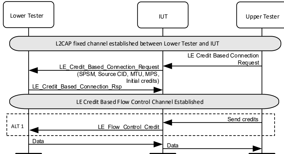
Figure 4.214: L2CAP/LE/CFC/BV-02-C [LE Credit Based Connection Request on Supported SPSM] MSC
