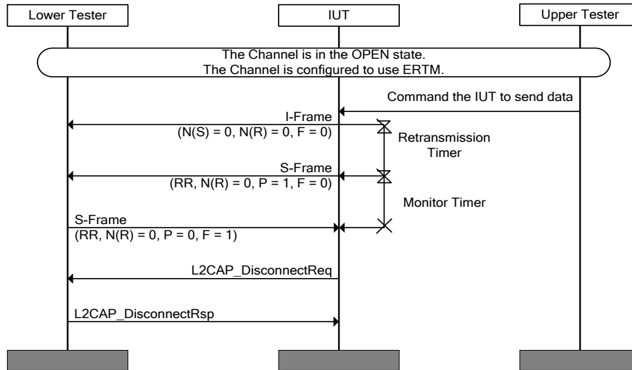
Figure 4.87: L2CAP/ERM/BV-12-C [I-Frame Transmissions Exceed MaxTransmit] MSC
