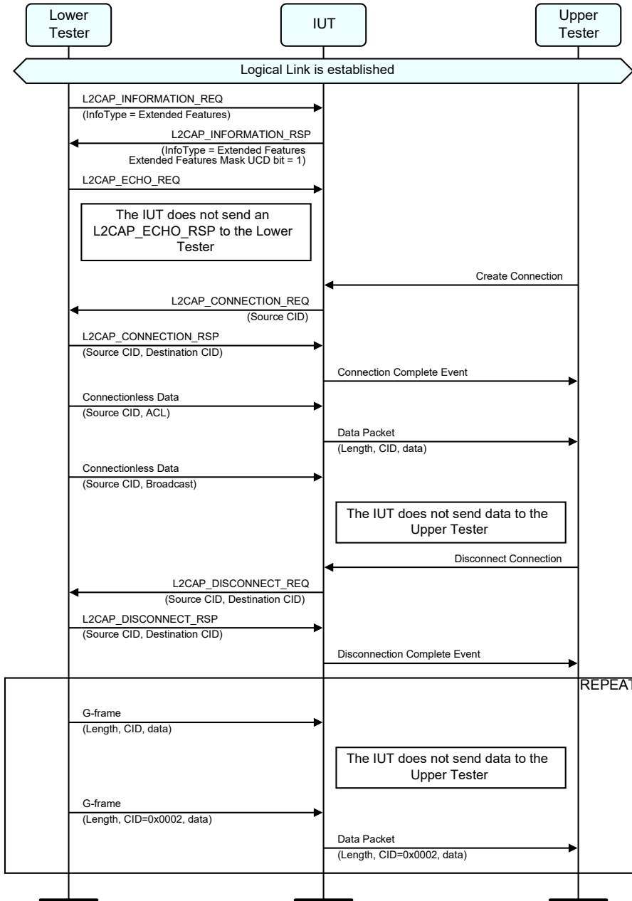
Figure 4.185: L2CAP/CLS/CID/BV-01-C [Ignore Unsupported CIDs, APB] MSC
