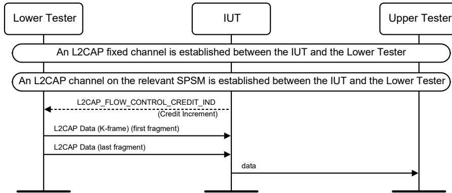
Figure 4.33: Recombination of Data Packets MSC
