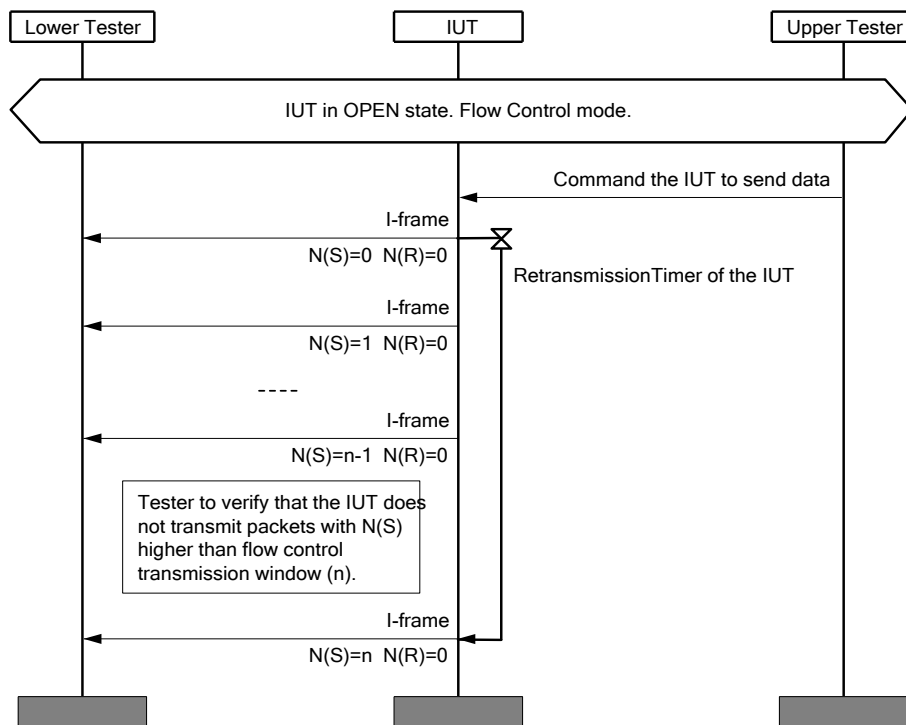
Figure 4.36: L2CAP/COS/FLC/BV-01-C [Flow Control without Acks] MSC
