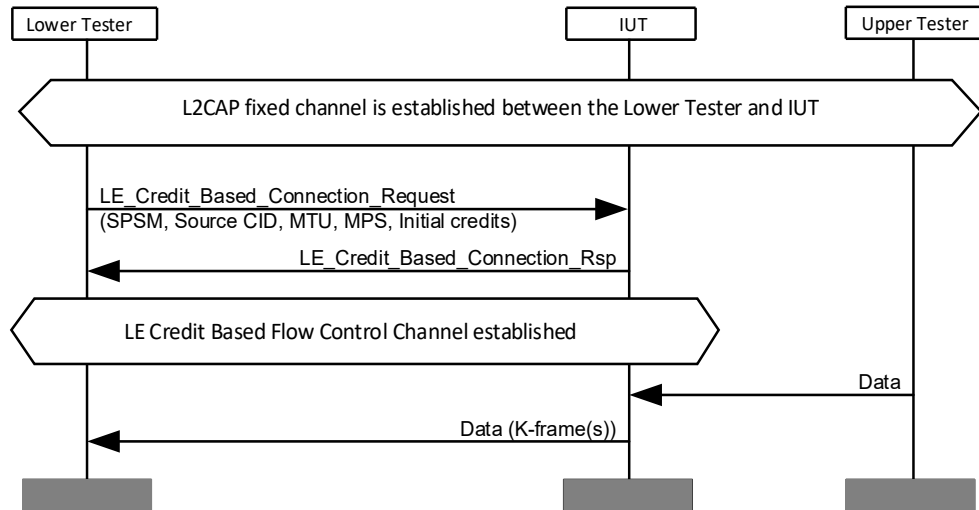
Figure 4.215: L2CAP/LE/CFC/BV-03-C [LE Credit Based Connection Response on Supported SPSM] MSC
