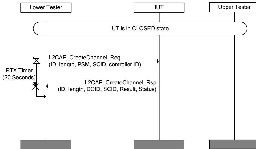
Figure 4.127: L2CAP/CCH/BV-04-C [Create Channel Response for an AMP Physical Link] MSC
