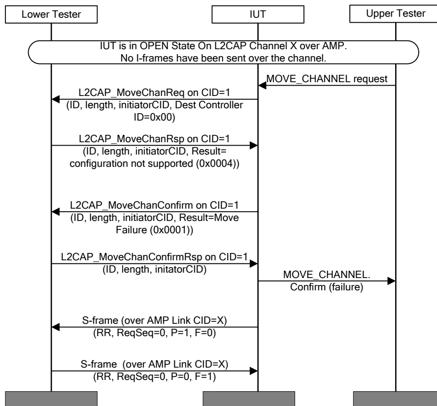
Figure 4.132: L2CAP/MCH/BV-05-C [Move ERTM Channel Request for AMP to BR/EDR – Refused] MSC
