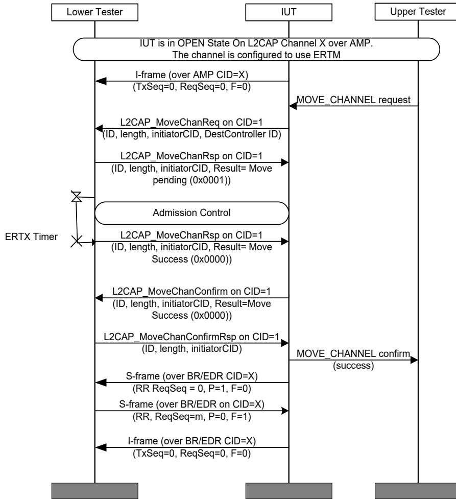
Figure 4.140: L2CAP/MCH/BV-13-C [Data Transfer while Moving ERTM Channel from AMP to BR/EDR – Unacknowledged Data] MSC
