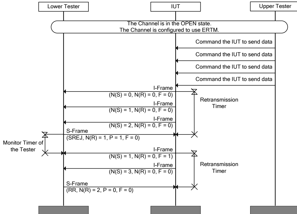
Figure 4.89: L2CAP/ERM/BV-14-C [Respond to S-Frame [SREJ] POLL Bit Set] MSC
