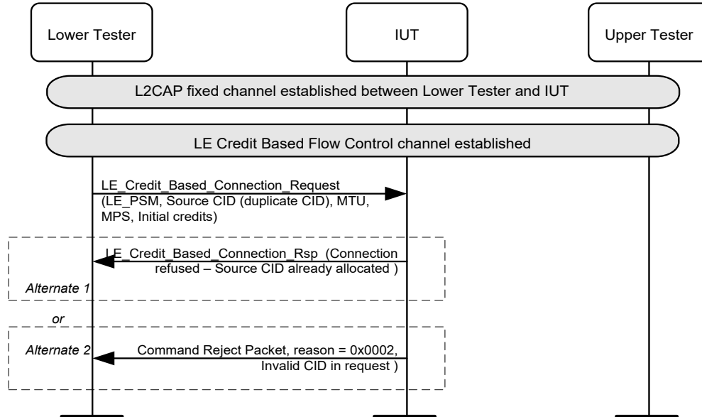
Figure 4.226: L2CAP/LE/CFC/BV-20-C [LE Credit Based Connection Response - refused due to Source CID already allocated - Responder] MSC
