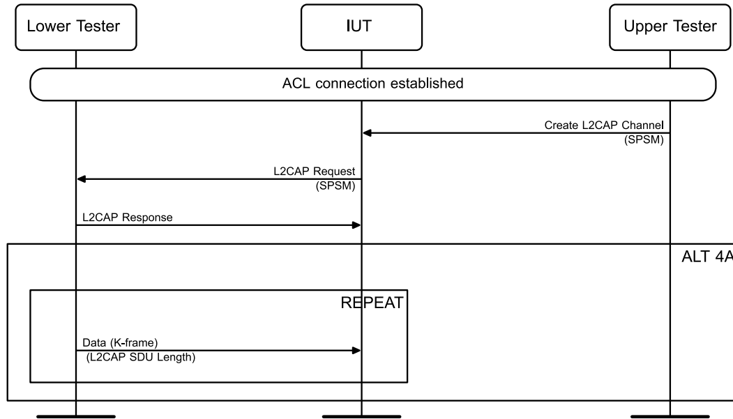
Figure 4.242: K-frame – SDU length = MPS MSC
