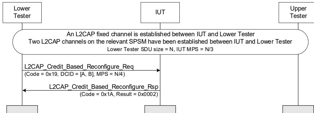
Figure 4.206: Renegotiate MPS – MPS value is decreased MSC
