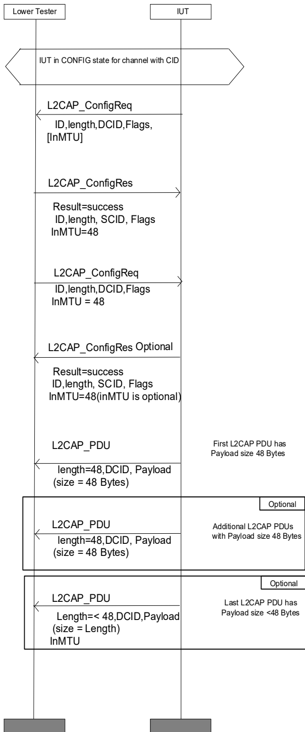
Figure 4.16: L2CAP/COS/CFD/BV-09-C [Mandatory 48 Byte MTU] MSC
