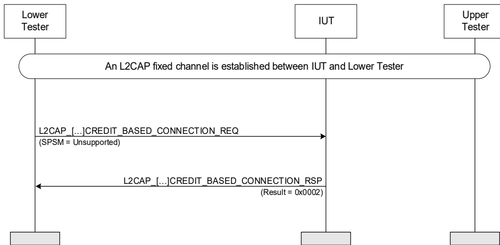
Figure 4.236: L2CAP Credit Based Connection Response on Unsupported SPSM MSC
