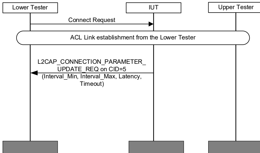
Figure 4.175: L2CAP/LE/CPU/BV-01-C [Send Connection Parameter Update Request] MSC
