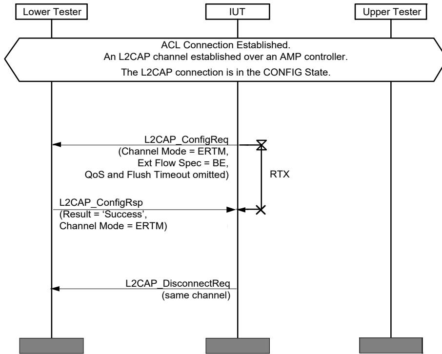
Figure 4.120: L2CAP/LSC/BV-09-C [Premature Success in Configuration Response, AMP Channel] MSC
