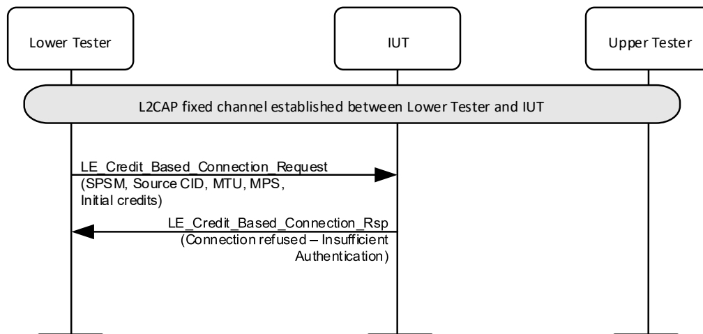
Figure 4.221: L2CAP/LE/CFC/BV-11-C [Security - Insufficient Authentication – Responder] MSC
