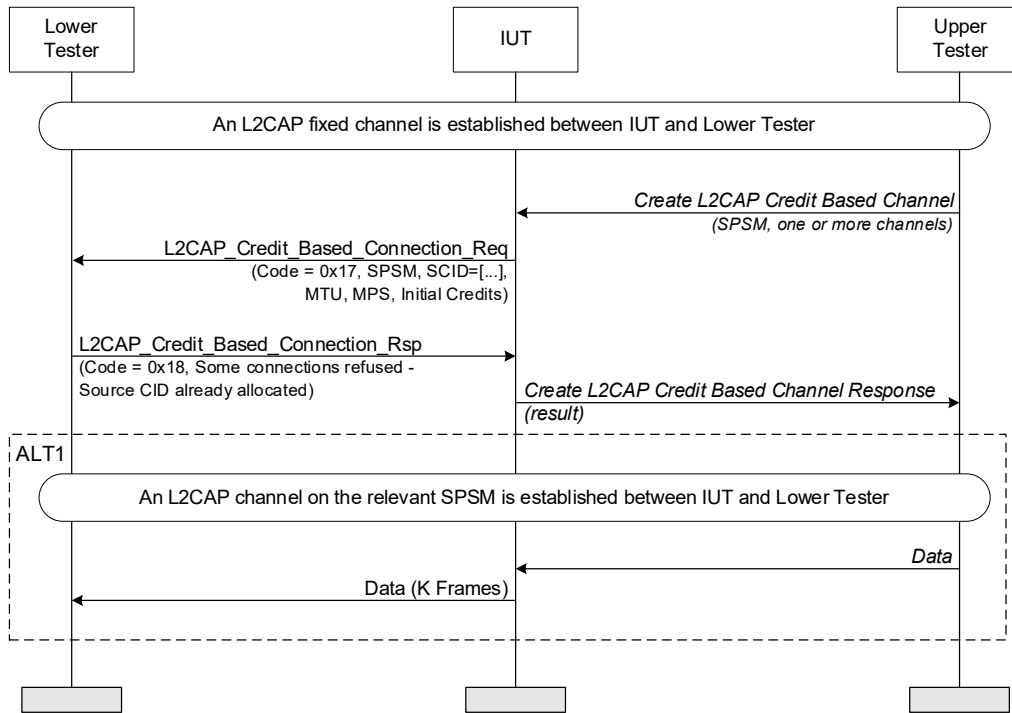
Figure 4.198: L2CAP Credit Based Connection Request – refused due to Source CID already allocated MSC
