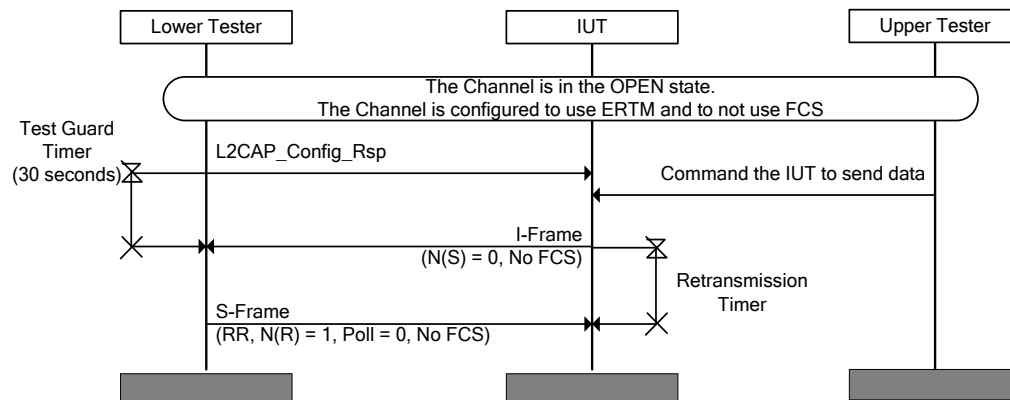
Figure 4.69: L2CAP/OFS/BV-01-C [Sending I-Frames without FCS for ERTM] MSC
