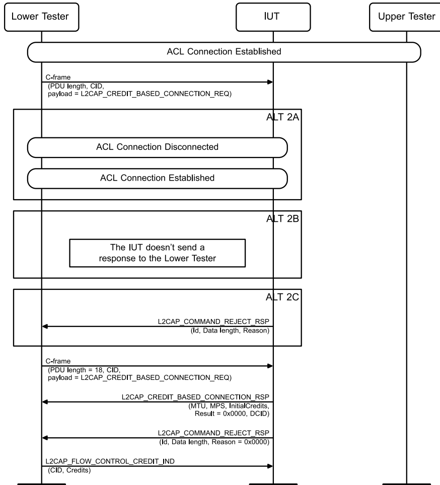
Figure 4.34: L2CAP/ECFC/BI-09-C [Incorrect Size Signaling Packets] MSC
