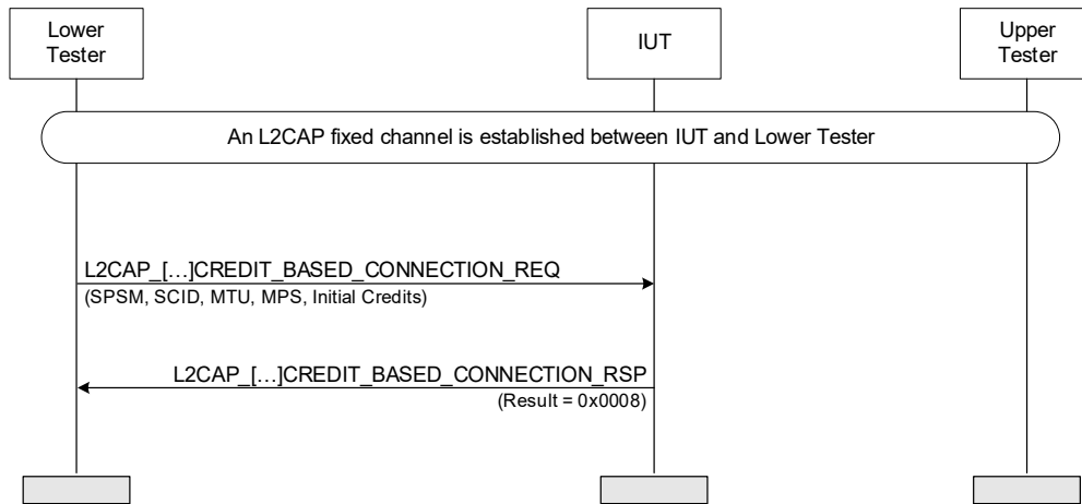
Figure 4.239: Security – Insufficient Encryption – Responder MSC
