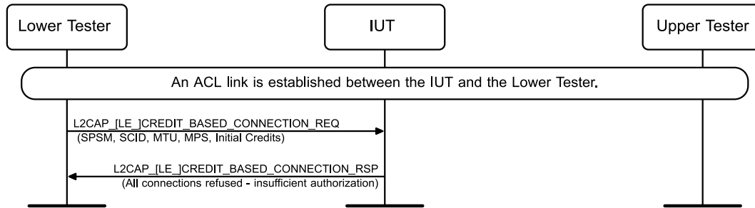
Figure 4.233: Security – Insufficient Authorization – Responder MSC
