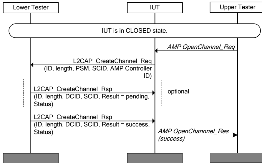
Figure 4.124: L2CAP/CCH/BV-01-C [Create Channel Request for an AMP Physical Link] MSC
