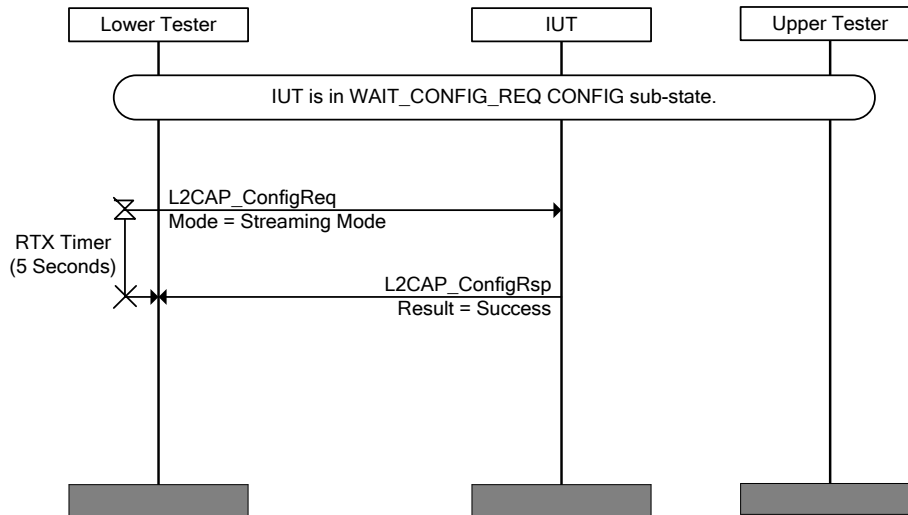
Figure 4.49: L2CAP/CMC/BV-05-C [Lower Tester Initiated Configuration of Streaming Mode] MSC
