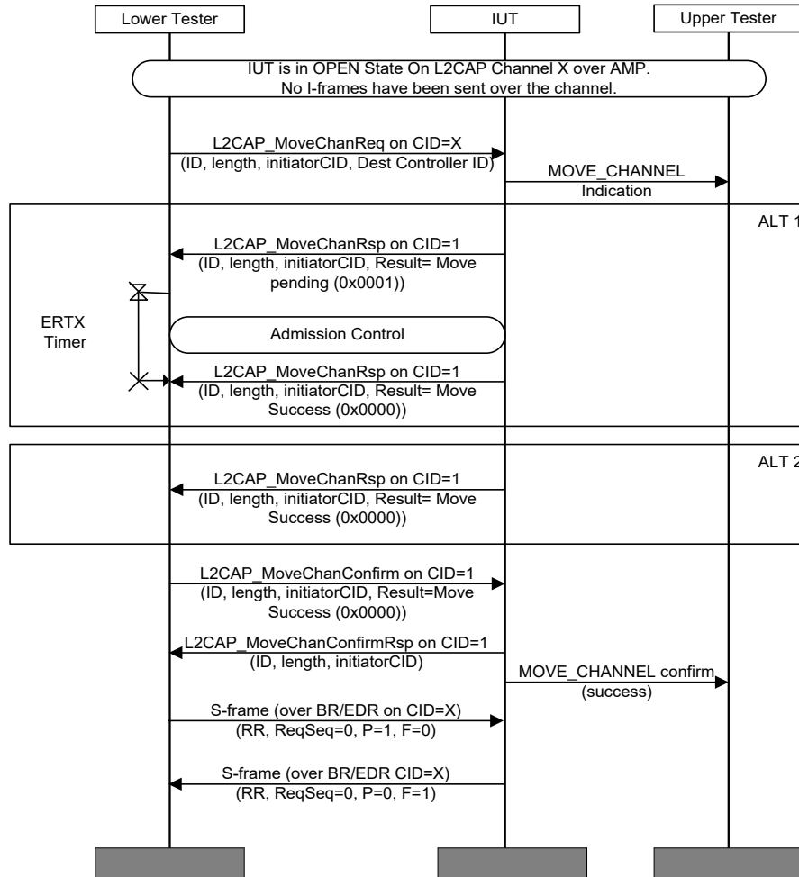
Figure 4.135: L2CAP/MCH/BV-08-C [Move ERTM Channel Response for AMP to BR/EDR – Success] MSC
