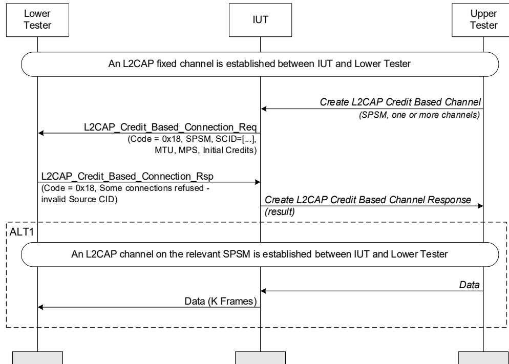
Figure 4.197: L2CAP Credit Based Connection Request – refused due to Invalid Source CID MSC
