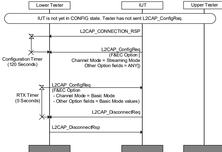
Figure 4.57: L2CAP/CMC/BI-04-C [Configuration Mode mismatch when use of Streaming Mode is Mandatory] MSC
