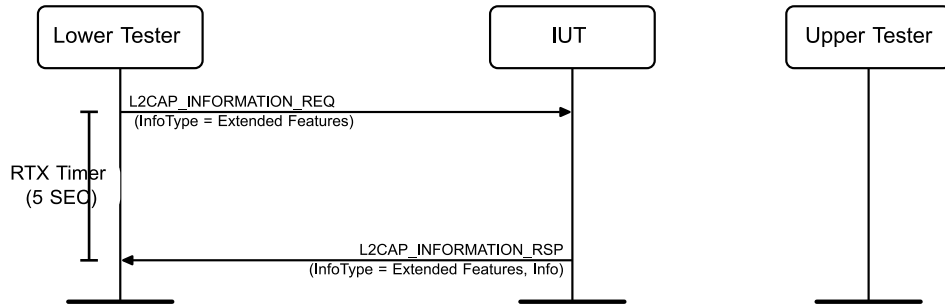
Figure 4.43: L2CAP/EXF/BV-07-C [Extended Features Information Response] MSC
