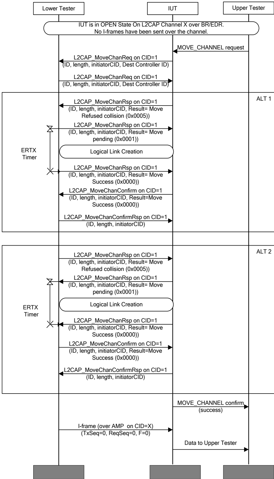
Figure 4.163: L2CAP/MCH/BV-36-C [Move Collision – STM Sink] MSC
