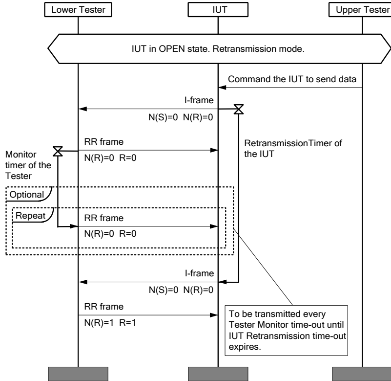
Figure 4.41: L2CAP/COS/RTX/BV-02-C [Retransmission with R=0 in RR frame] MSC
