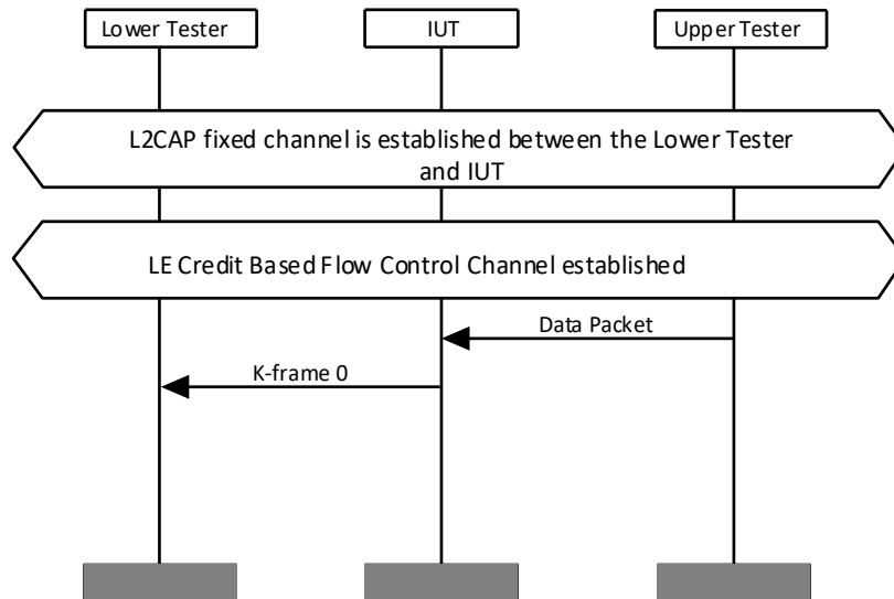
Figure 4.28: L2CAP/COS/CFC/BV-02-C [No Segmentation] MSC
