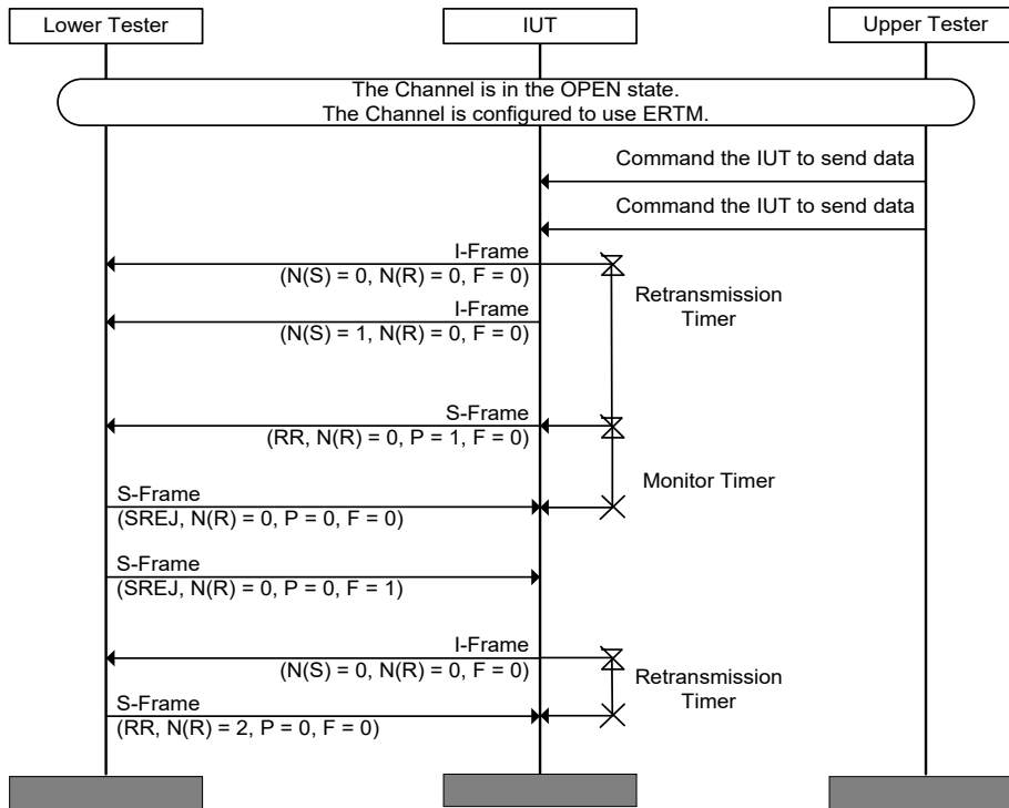
Figure 4.100: L2CAP/ERM/BI-03-C [Handle Duplicate S-Frame [SREJ]] MSC
