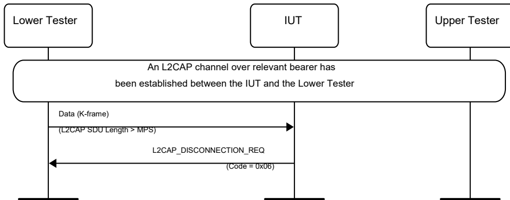
Figure 4.241: K-frame – Information Payload length greater than MPS of IUT MSC
