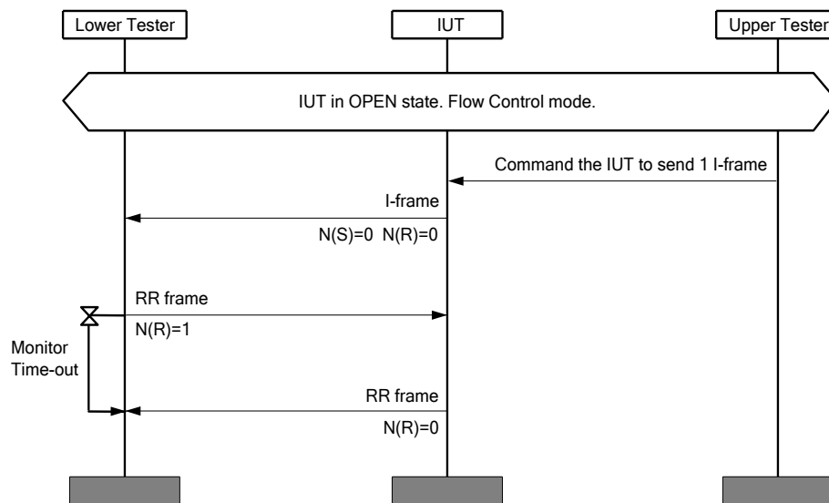
Figure 4.39: L2CAP/COS/FLC/BV-04-C [Transmit RR Frame on Monitor Timeout] MSC
