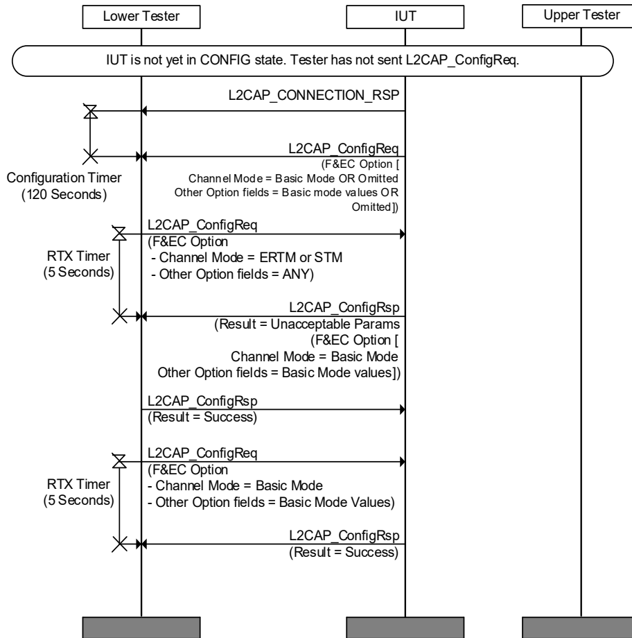
Figure 4.53: L2CAP/CMC/BV-09-C [Configuration to Basic Mode by the IUT] MSC
