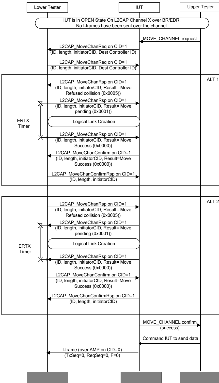
Figure 4.162: L2CAP/MCH/BV-35-C [Move Collision – STM Source] MSC
