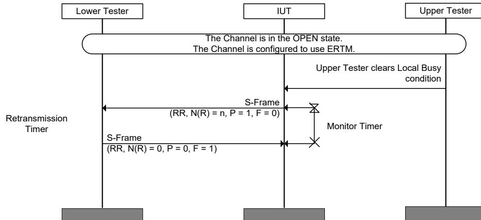
Figure 4.96: L2CAP/ERM/BV-22-C [Exit Local Busy Condition] MSC
