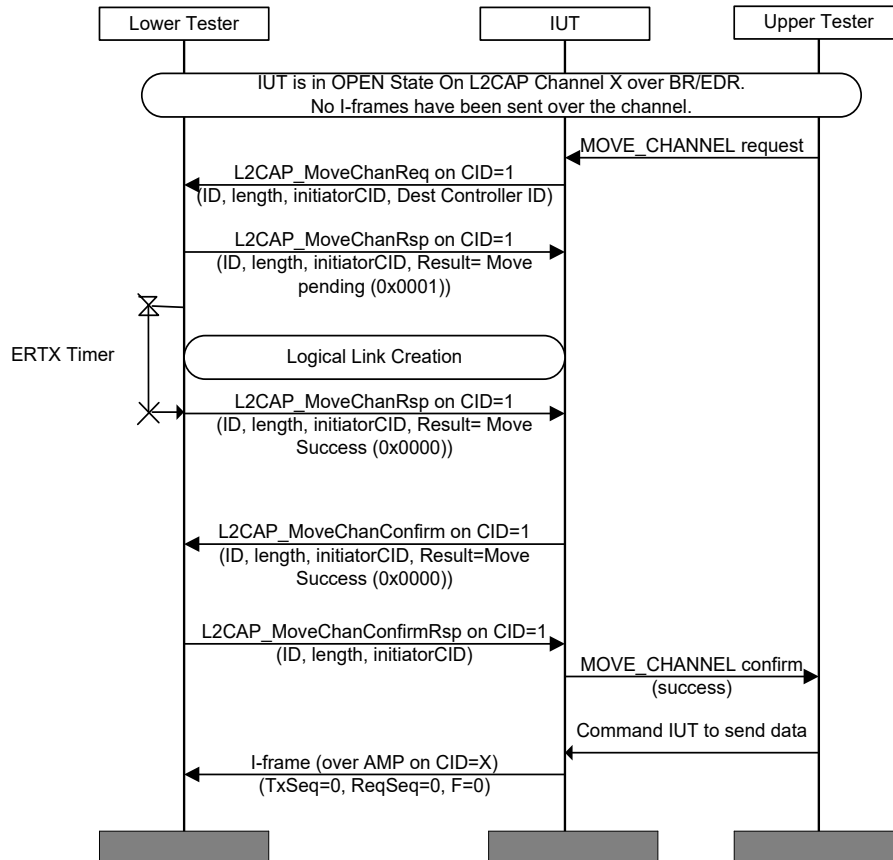
Figure 4.142: L2CAP/MCH/BV-15-C [Move Channel Request for BR/EDR to AMP (STM Source) – Success] MSC
