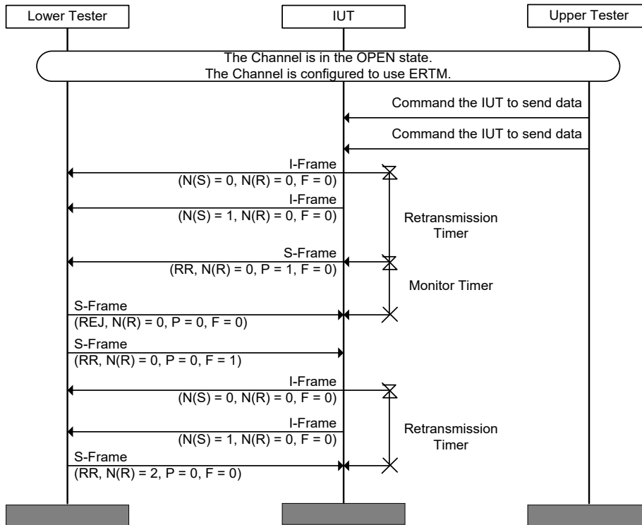
Figure 4.101: L2CAP/ERM/BI-04-C [Handle Receipt of S-Frame [REJ] and S-Frame [RR, F=1] that Both Require Retransmission of the Same I-Frames] MSC
