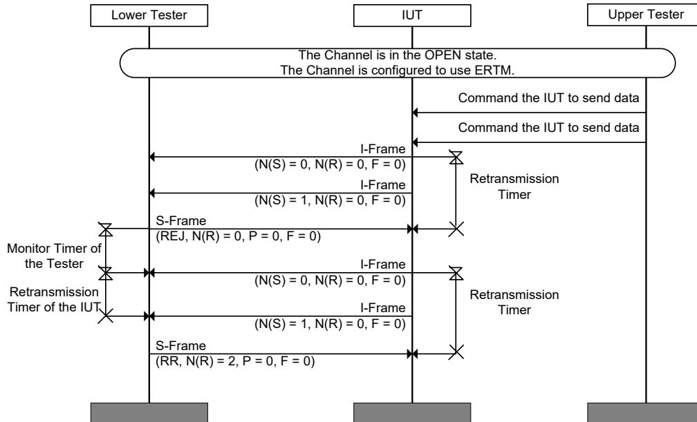
Figure 4.168: L2CAP/ECF/BV-05-C [Respond to S-Frame [REJ] with Extended Control Field] MSC
