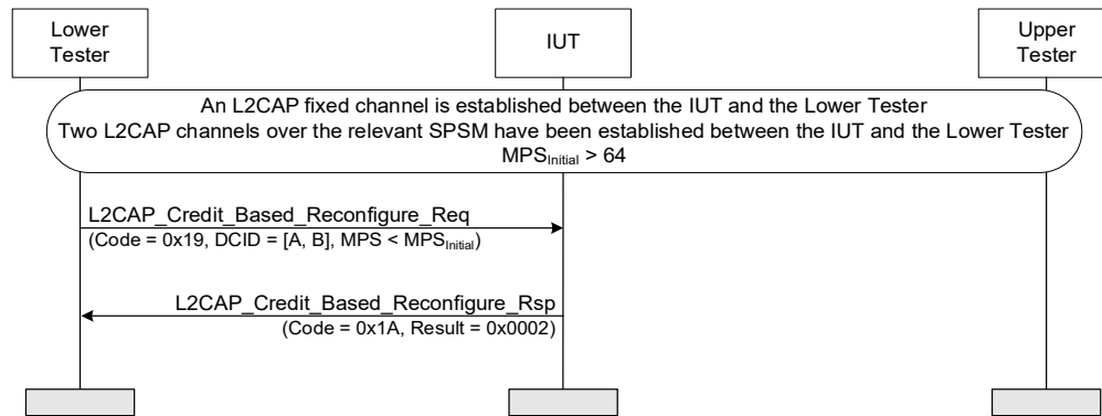
Figure 4.212: Renegotiate MPS – MPS value is decreased, Multiple Channels MSC
