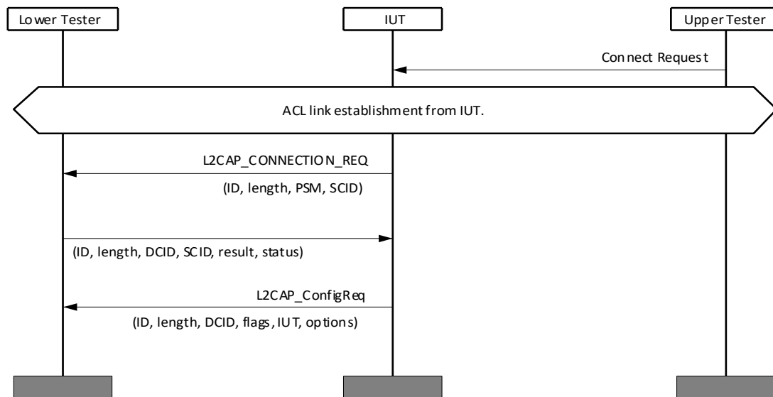
Figure 4.1: L2CAP/COS/CED/BV-01-C [Request Connection] MSC
