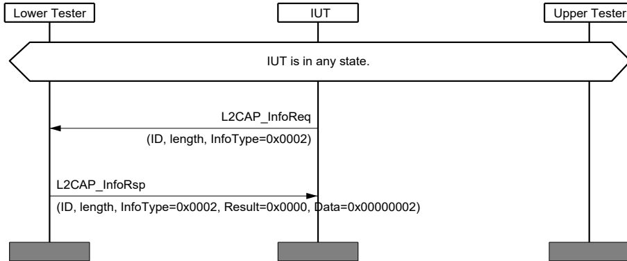
Figure 4.22: L2CAP/COS/IEX/BV-01-C [Query for 1.2 Features] MSC
