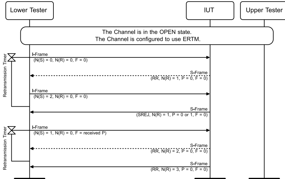
Figure 4.92: L2CAP/ERM/BV-17-C [Send S-Frame [SREJ]] MSC
