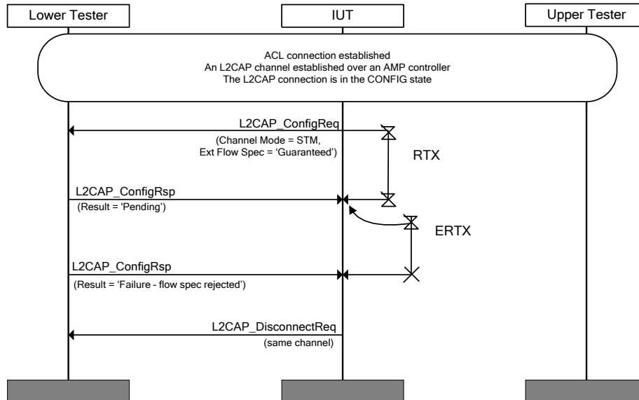
Figure 4.123: L2CAP/LSC/BV-12-C [Remote Failed on Guaranteed, AMP Channel] MSC
