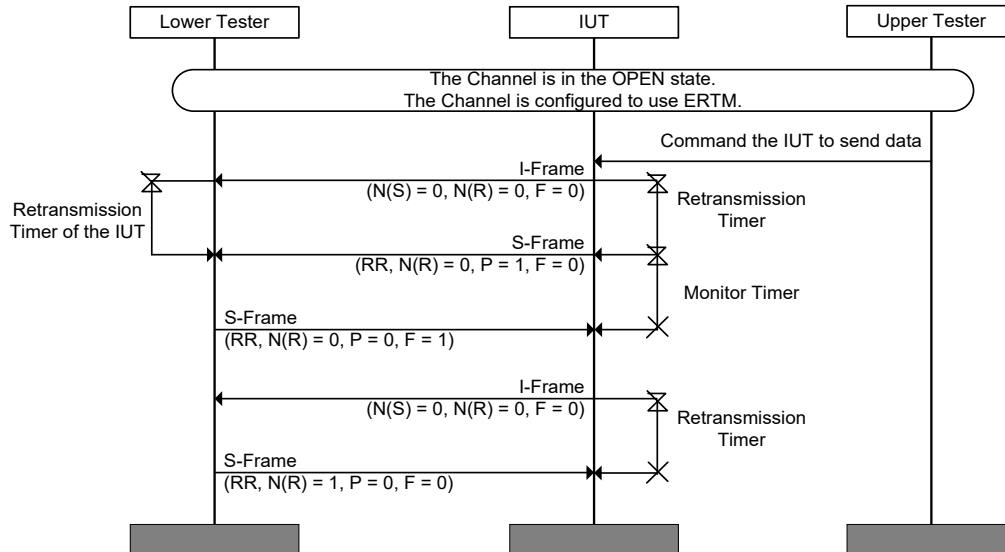
Figure 4.93: L2CAP/ERM/BV-18-C [Receive S-Frame [RR] Final Bit = 1] MSC
