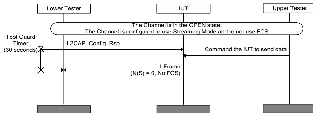
Figure 4.71: L2CAP/OFS/BV-03-C [Sending I-Frames without FCS for Streaming Mode] MSC
