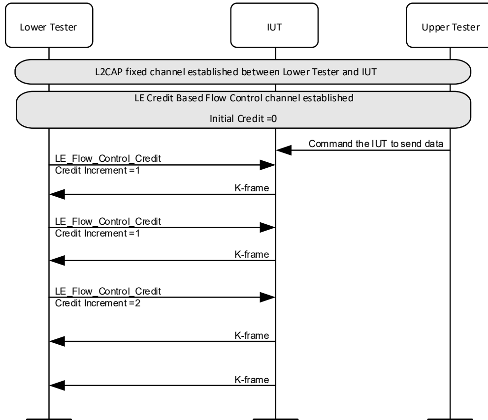
Figure 4.218: L2CAP/LE/CFC/BV-06-C [Credit Exchange – Receiving Incremental Credits] MSC
