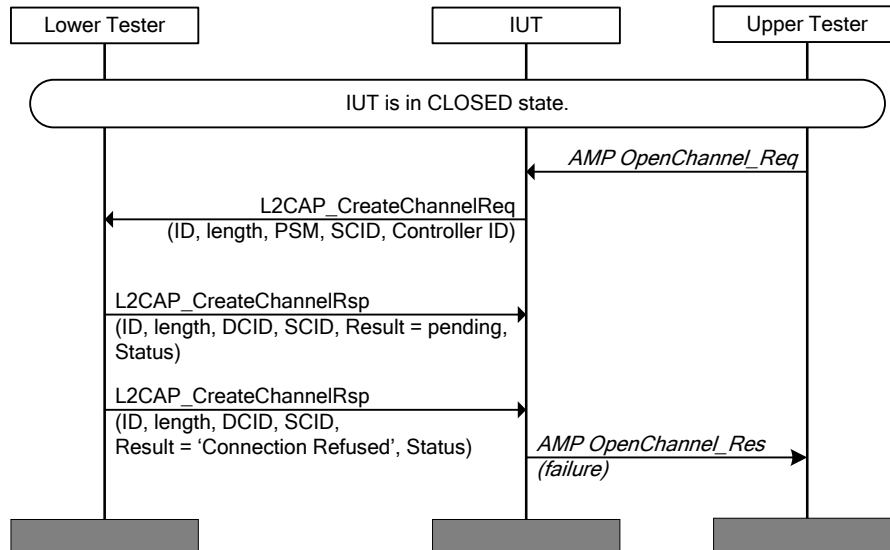
Figure 4.126: L2CAP/CCH/BV-03-C [Create Channel Request for an AMP Physical Link – Failed] MSC
