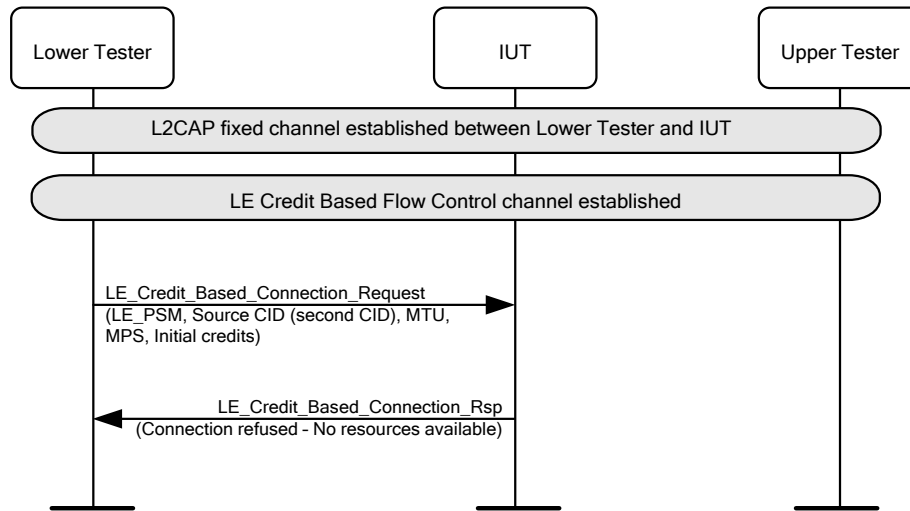
Figure 4.223: L2CAP/LE/CFC/BV-17-C [LE Credit Based Connection Response - refused due to insufficient resources - Responder] MSC
