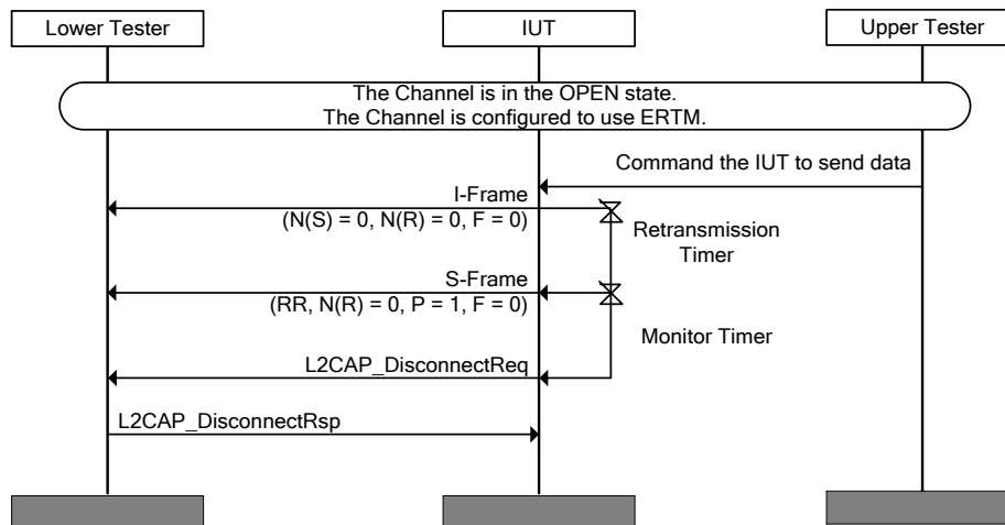
Figure 4.86: L2CAP/ERM/BV-11-C [S-Frame Transmissions Exceed MaxTransmit] MSC
