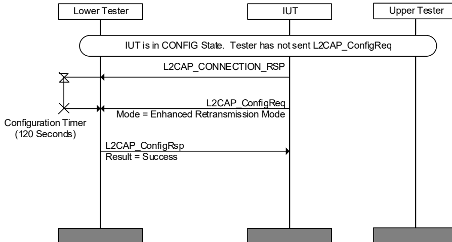
Figure 4.45: L2CAP/CMC/BV-01-C [IUT Initiated Configuration of Enhanced Retransmission Mode] MSC
