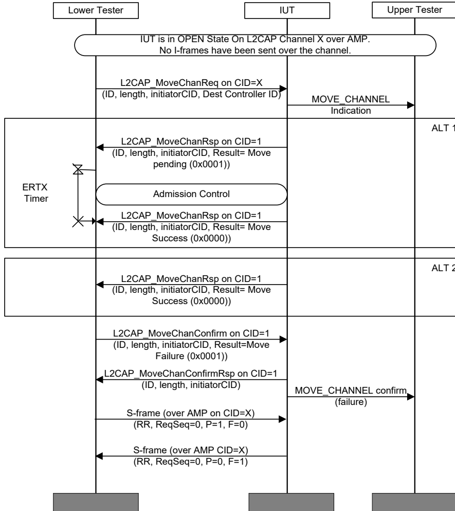
Figure 4.136: L2CAP/MCH/BV-09-C [Move ERTM Channel Response for AMP to BR/EDR – Failure] MSC
