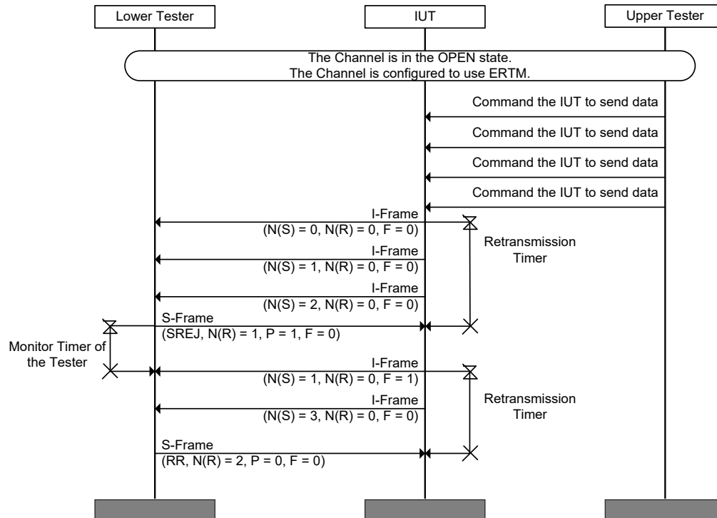
Figure 4.169: L2CAP/ECF/BV-06-C [Respond to S-Frame [SREJ] with Extended Control Field and POLL bit Set] MSC
