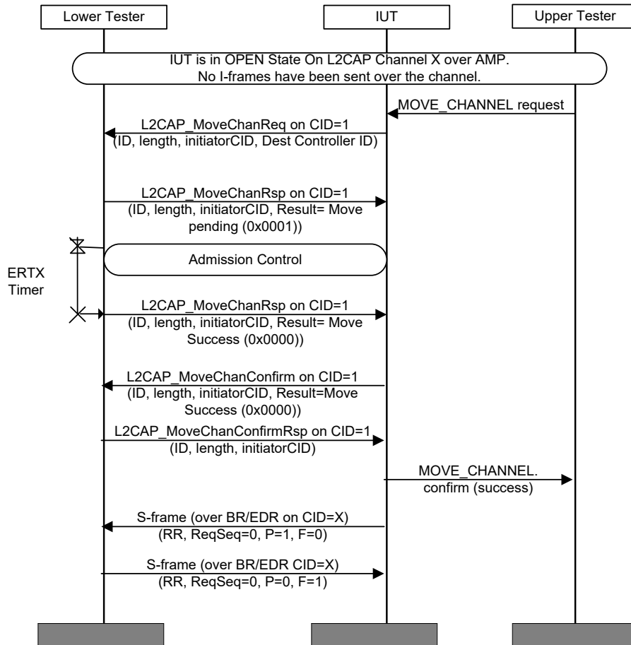
Figure 4.131: L2CAP/MCH/BV-04-C [Move ERTM Channel Request for AMP to BR/EDR – Success] MSC
