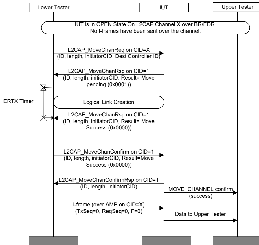
Figure 4.155: L2CAP/MCH/BV-28-C [Move Channel Response for BR/EDR to AMP (STM Sink) – Success] MSC
