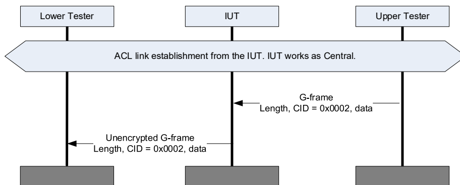
Figure 4.182: L2CAP/CLS/UCD/BV-02-C [Unencrypted data transmission over unicast connectionless channel] MSC
