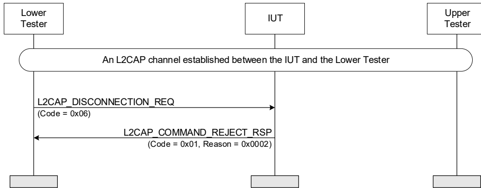
Figure 4.237: Disconnect Request – DCID not recognized or fixed channel MSC
