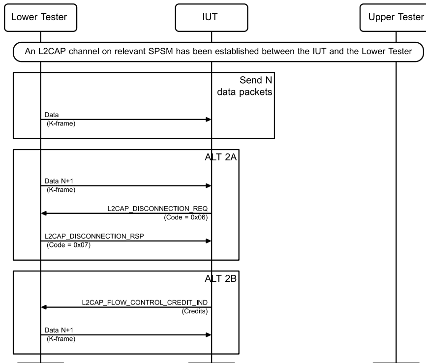
Figure 4.193: Credit Exchange – No Credits MSC
