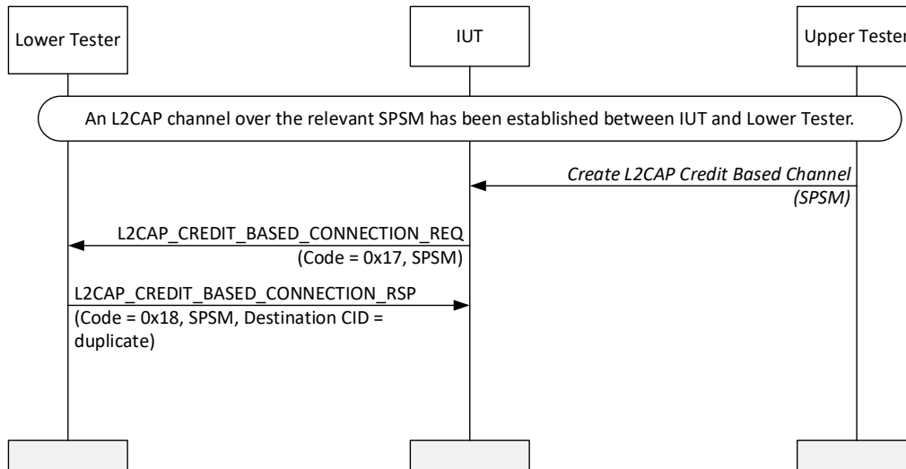
Figure 4.211: L2CAP Credit Based Connection Response – Duplicate DCID MSC
