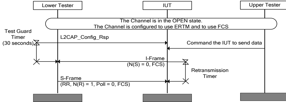
Figure 4.73: L2CAP/OFS/BV-05-C [Sending I-Frames with FCS for ERTM] MSC
