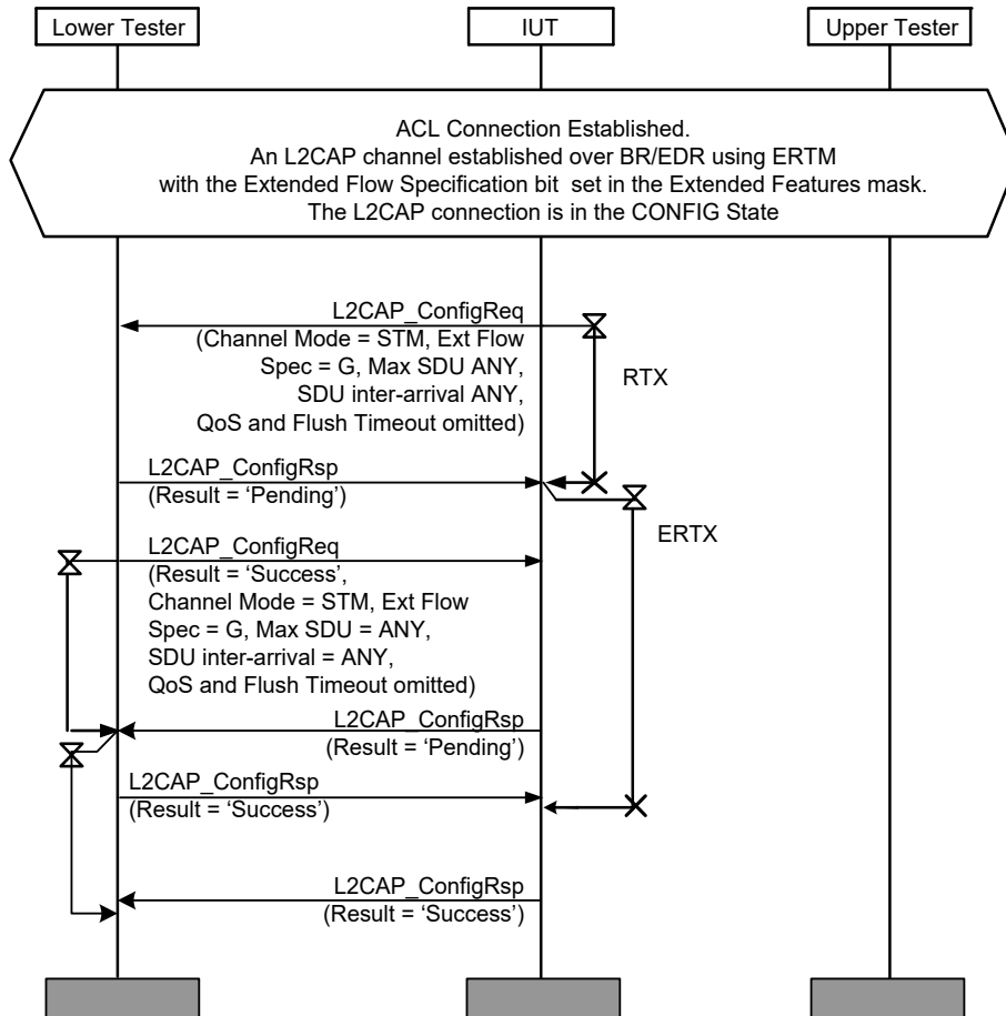
Figure 4.113: L2CAP/LSC/BV-02-C [Normal Lock Step Configuration Process for Guaranteed, BR/EDR ERTM Channel] MSC
