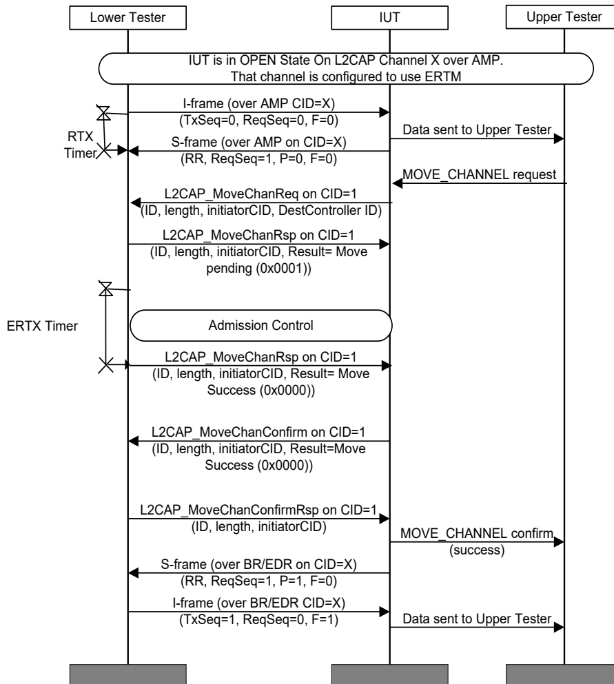
Figure 4.139: L2CAP/MCH/BV-12-C [Data Transfer while Moving ERTM Channel from AMP to BR/EDR] MSC
