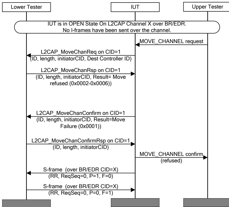
Figure 4.129: L2CAP/MCH/BV-02-C [Move ERTM Channel Request for BR/EDR to AMP – Refused] MSC
