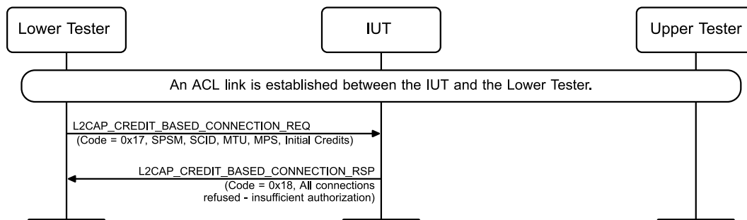
Figure 4.194: Security – Insufficient Authentication – Responder, LE MSC
