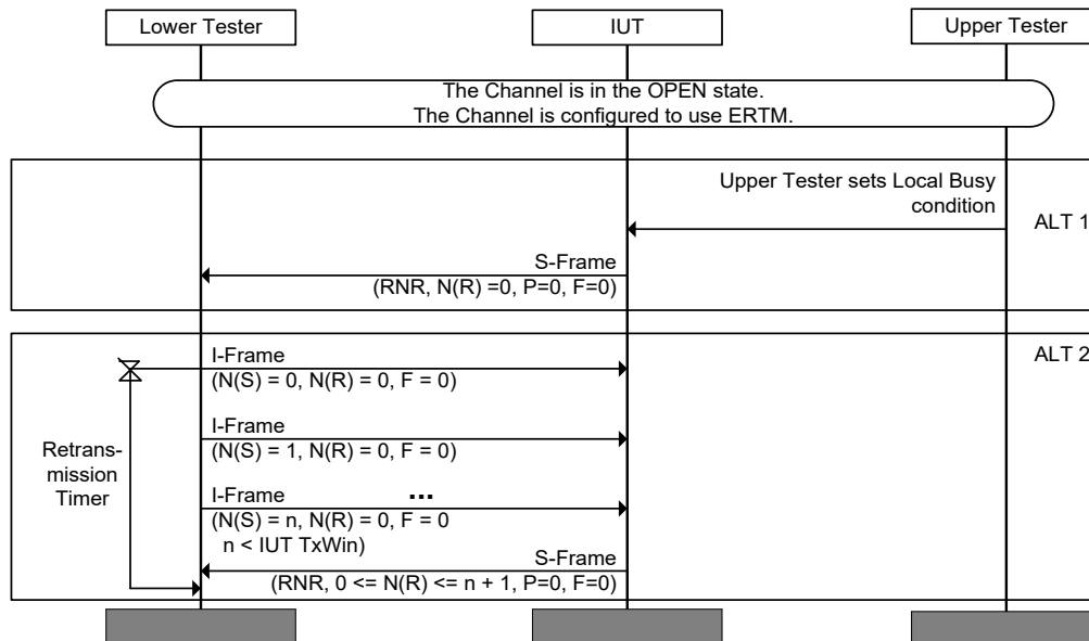
Figure 4.82: L2CAP/ERM/BV-07-C [Send S-Frame [RNR]] MSC
