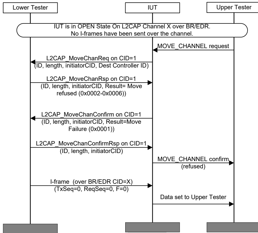
Figure 4.145: L2CAP/MCH/BV-18-C [Move Channel Request for BR/EDR to AMP (STM Sink) – Refused] MSC
