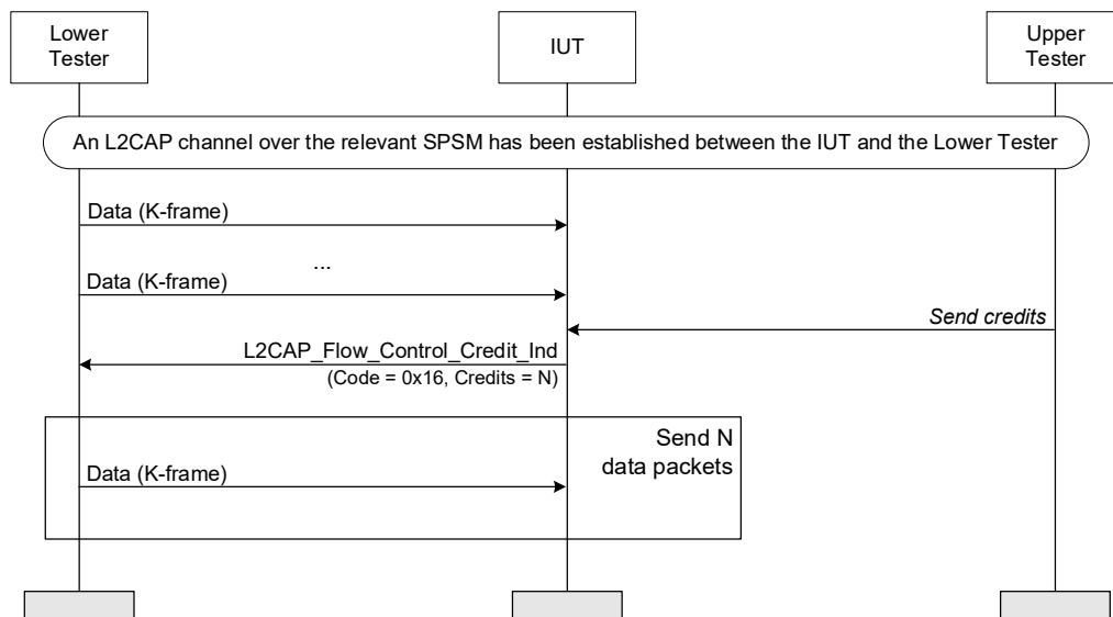
Figure 4.191: Credit Exchange – Sending Credits MSC
