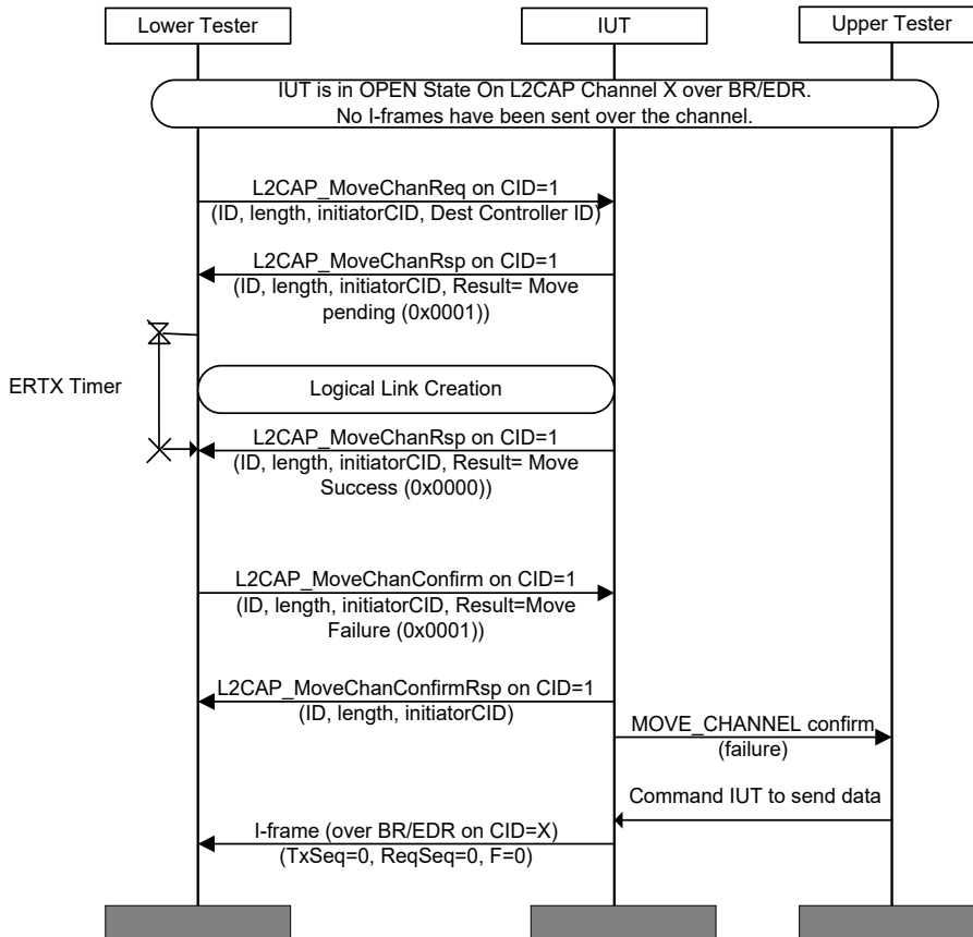
Figure 4.158: L2CAP/MCH/BV-31-C [Move Channel Response for BR/EDR to AMP (STM Source) – Failed] MSC
