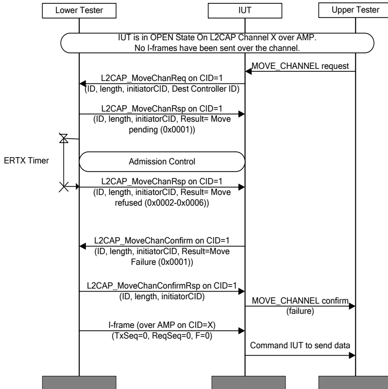
Figure 4.153: L2CAP/MCH/BV-26-C [Move Channel Request for AMP to BR/EDR (STM Sink) – AMP Failed] MSC
