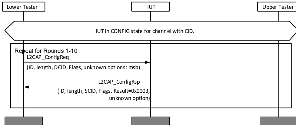
Figure 4.21: L2CAP/COS/CFD/BV-14-C [Unknown Mandatory Options Request] MSC
