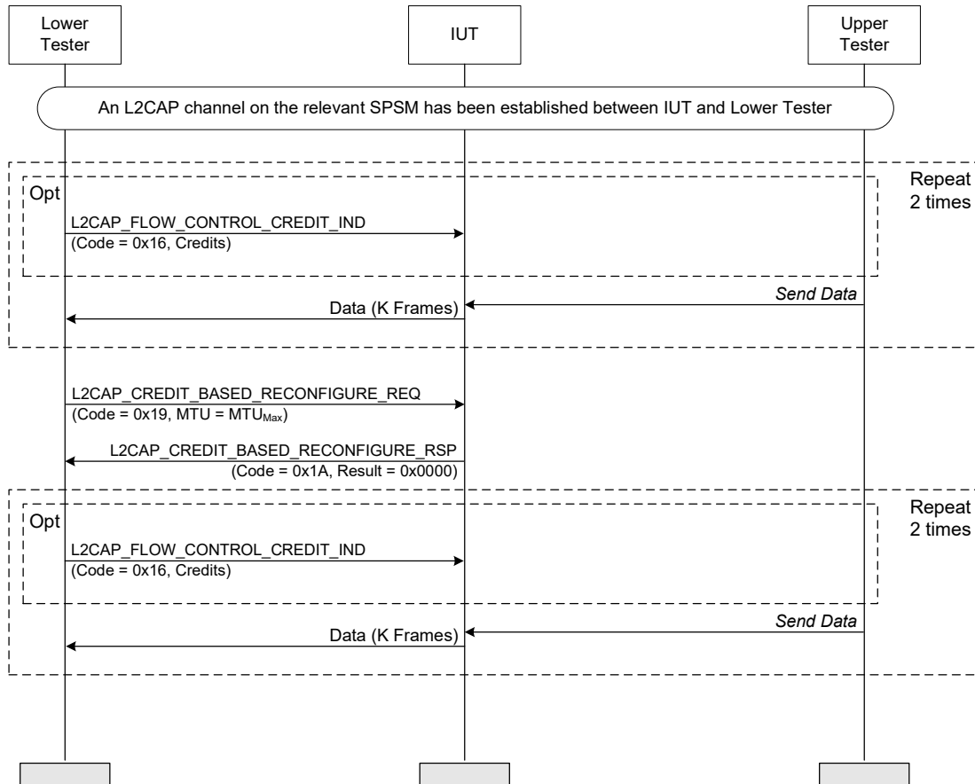
Figure 4.202: Renegotiate MTU – Responder MSC
