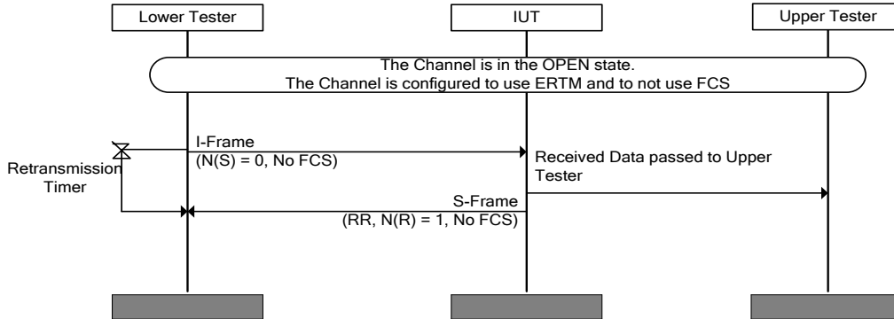
Figure 4.70: L2CAP/OFS/BV-02-C [Receiving Frames without FCS for ERTM] MSC
