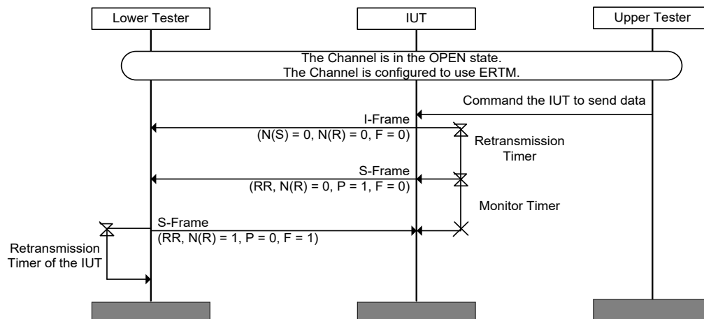
Figure 4.167: L2CAP/ECF/BV-04-C [Send S-Frame [RR] with Extended Control Field and Poll Bit Set] MSC
