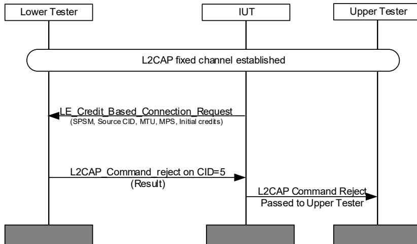
Figure 4.213: L2CAP/LE/CFC/BV-01-C [LE Credit Based Connection Request - Legacy Peer] MSC
