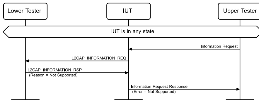
Figure 4.24: L2CAP/COS/IEX/BI-01-C [Accept Reject of Information Request, Peer Older Than v3.0] MSC
