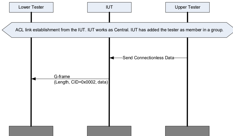
Figure 4.180: L2CAP/CLS/CLR/BV-01-C [Data Over Connectionless Channel] MSC
