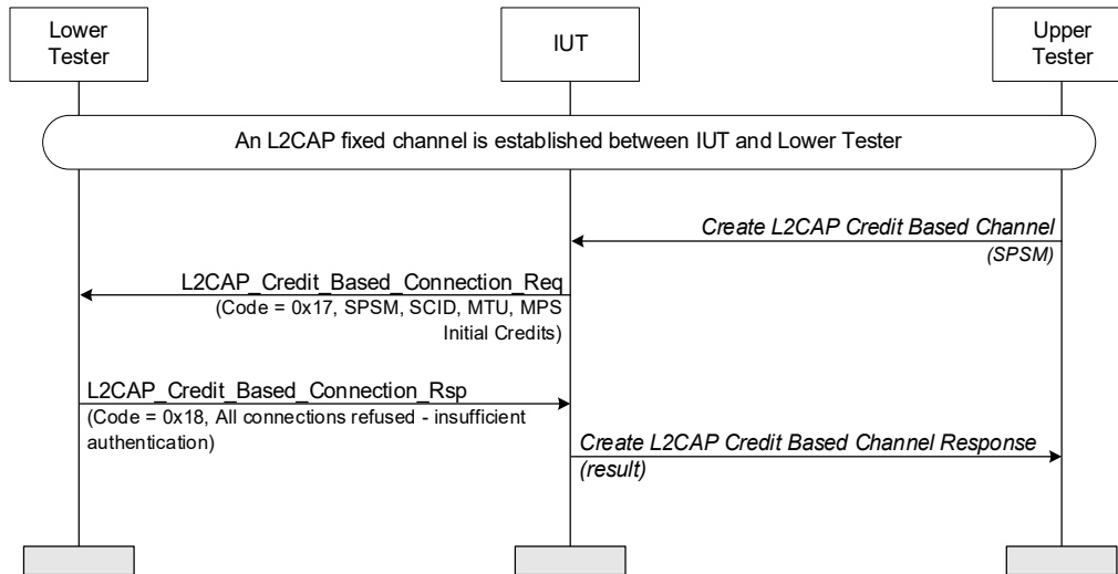
Figure 4.231: Security – Insufficient Authentication – Initiator MSC
