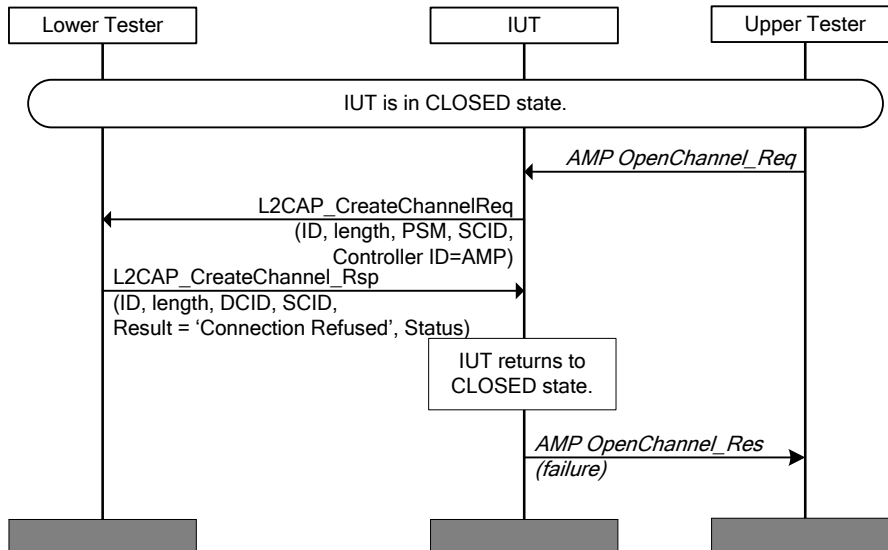
Figure 4.125: L2CAP/CCH/BV-02-C [Create Channel Request for an AMP Physical Link – Refused] MSC
