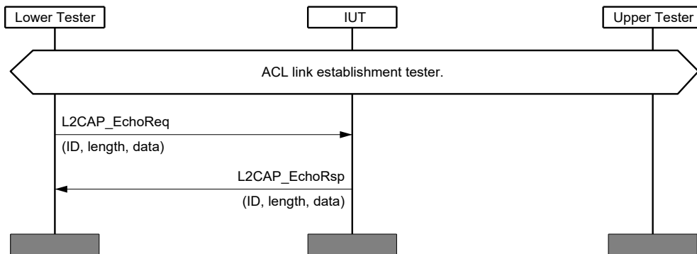
Figure 4.25: L2CAP/COS/ECH/BV-01-C [Respond to Echo Request] MSC
