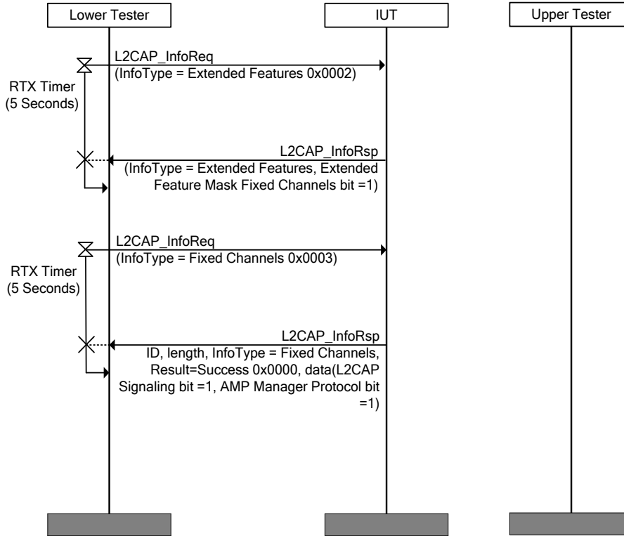
Figure 4.107: L2CAP/FIX/BV-02-C [AMP Manager Channel Supported] MSC
