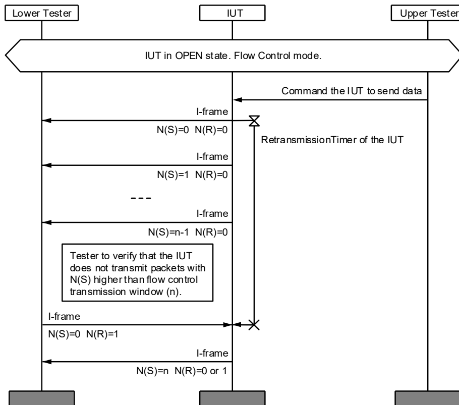
Figure 4.38: L2CAP/COS/FLC/BV-03-C [Resume Flow on I-frame Ack] MSC
