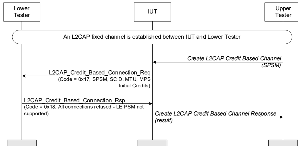
Figure 4.189: L2CAP Credit Based Connection Request on an Unsupported PSM MSC
