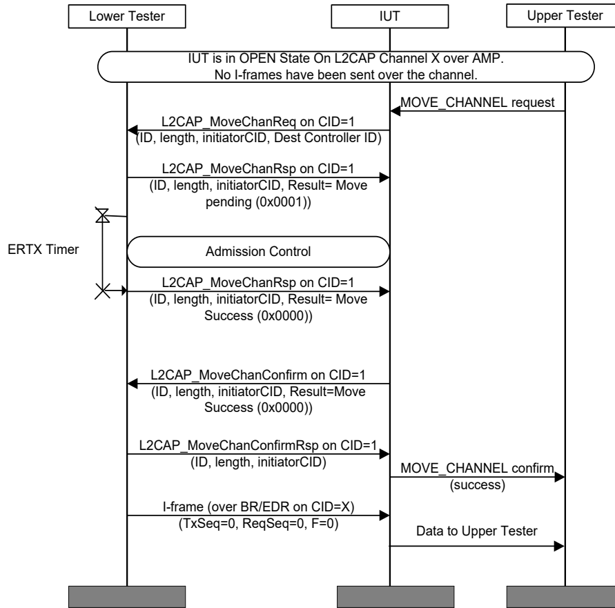
Figure 4.149: L2CAP/MCH/BV-22-C [Move Channel Request for AMP to BR/EDR (STM Sink) – Success] MSC
