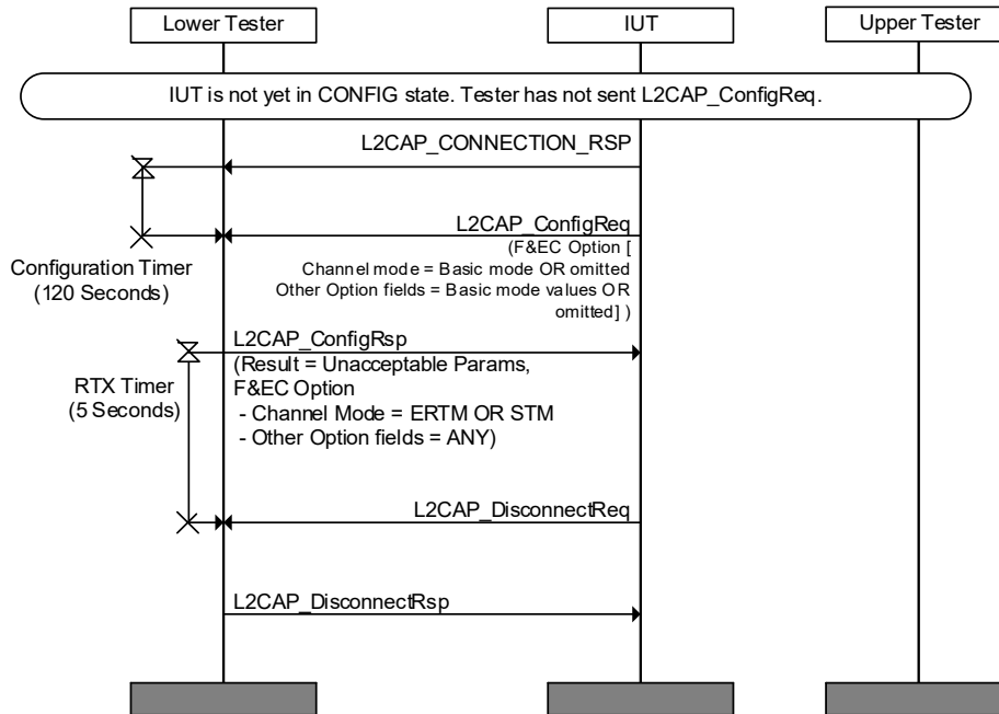
Figure 4.59: L2CAP/CMC/BI-06-C [Configuration to Basic Mode Rejected by the Lower Tester] MSC
