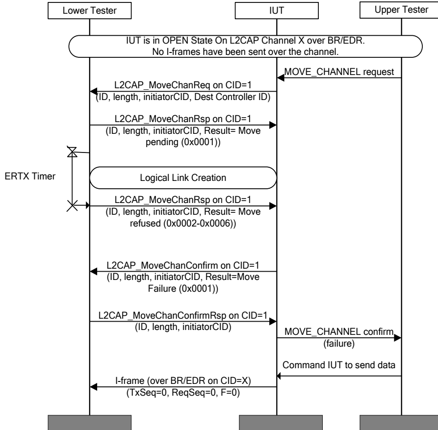
Figure 4.146: L2CAP/MCH/BV-19-C [Move Channel Request for BR/EDR to AMP (STM Source) – AMP Fail] MSC
