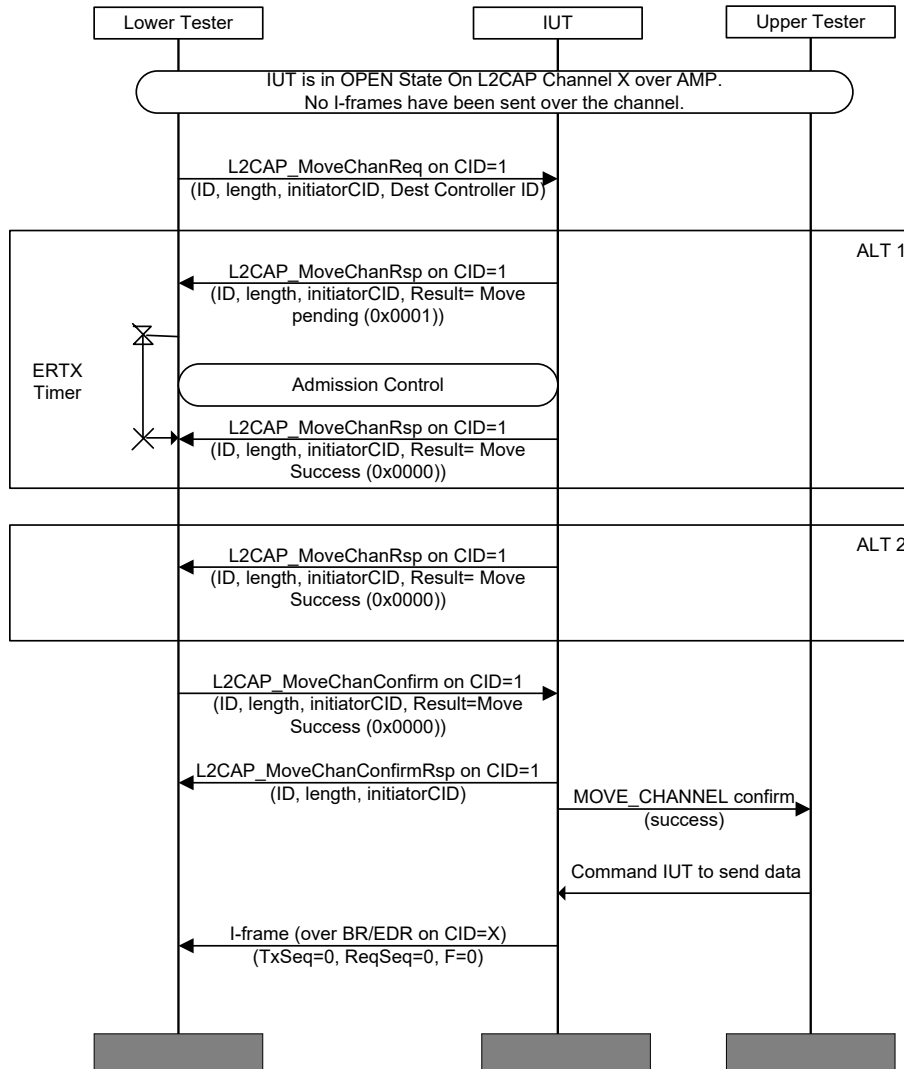
Figure 4.156: L2CAP/MCH/BV-29-C [Move Channel Response for AMP to BR/EDR (STM Source) – Success] MSC
