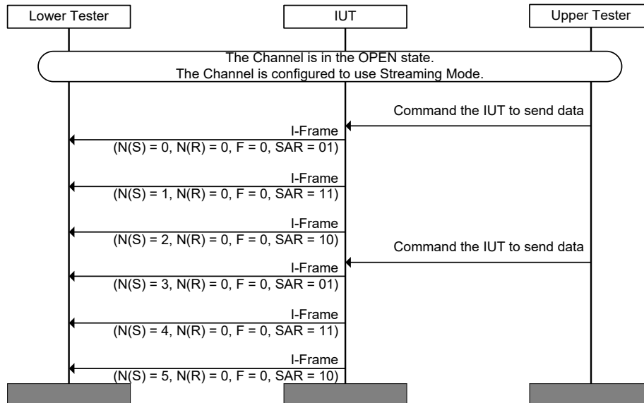
Figure 4.105: L2CAP/STM/BV-03-C [Streaming Mode Source using SAR] MSC
