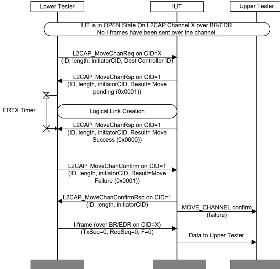
Figure 4.159: L2CAP/MCH/BV-32-C [Move Channel Response for BR/EDR to AMP (STM Sink) – Failed] MSC
