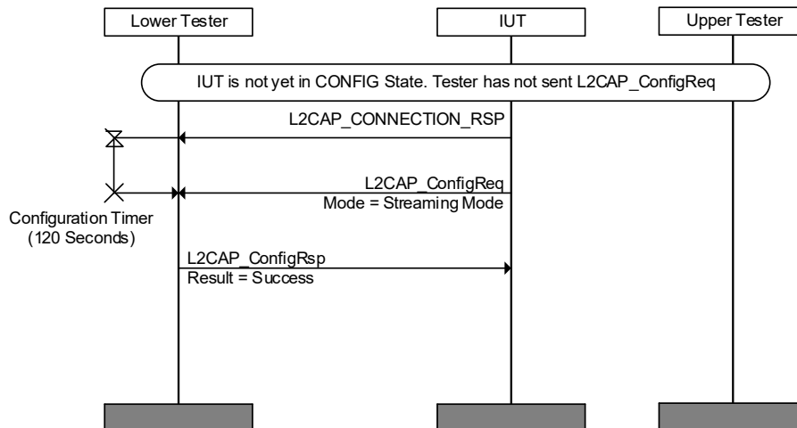
Figure 4.48: L2CAP/CMC/BV-04-C [IUT Initiated Configuration of Streaming Mode] MSC
