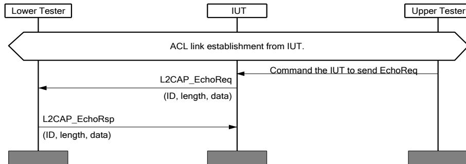
Figure 4.26: L2CAP/COS/ECH/BV-02-C [Send Echo Request] MSC
