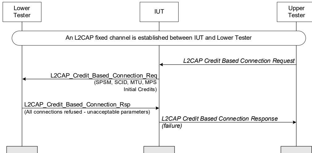
Figure 4.200: L2CAP Credit Based Connection Request – refused due to Unacceptable Parameters MSC
