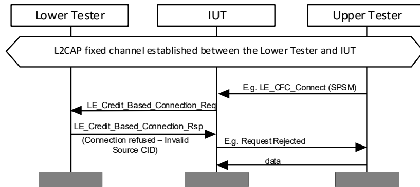
Figure 4.224: L2CAP/LE/CFC/BV-18-C [LE Credit Based Connection Request - refused due to Invalid Source CID - Initiator] MSC
