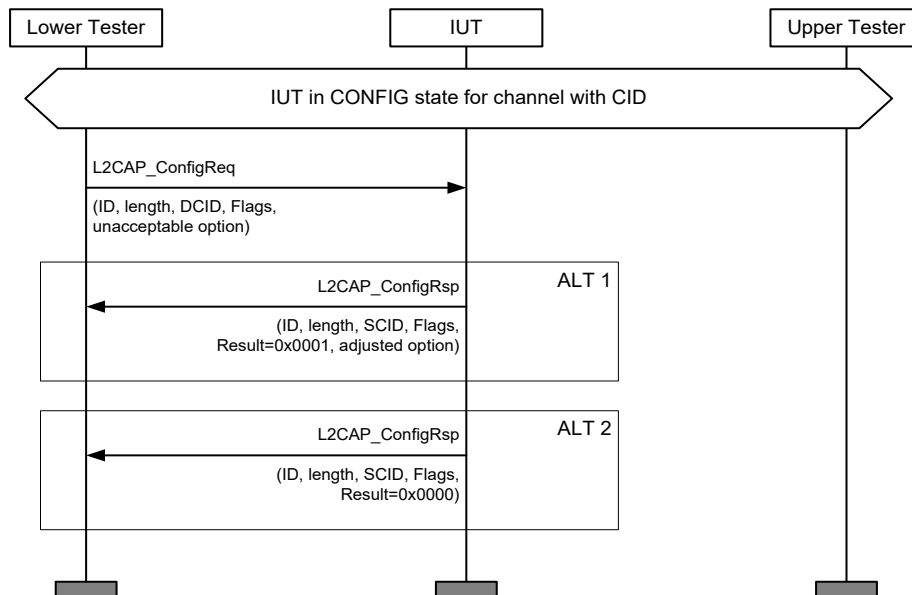
Figure 4.18: L2CAP/COS/CFD/BV-11-C [Negotiation of Unsupported Parameter] MSC
