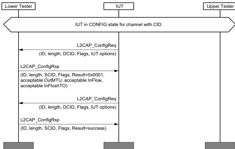
Figure 4.13: L2CAP/COS/CFD/BV-02-C [Negotiation with Reject] MSC
