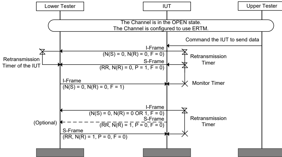
Figure 4.94: L2CAP/ERM/BV-19-C [Receive I-Frame Final Bit = 1] MSC
