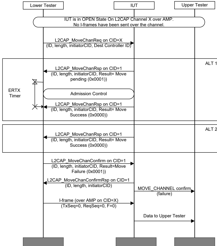
Figure 4.161: L2CAP/MCH/BV-34-C [Move Channel Response for AMP to BR/EDR (STM Sink) – Failed] MSC
