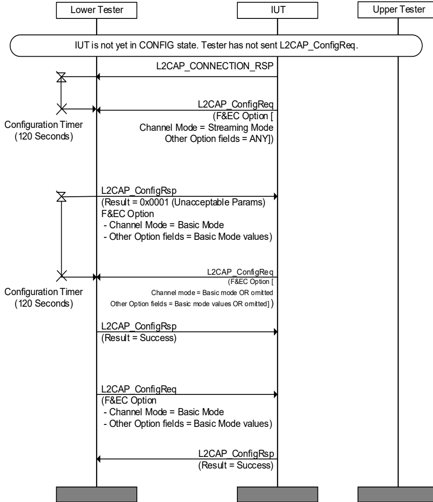
Figure 4.50: L2CAP/CMC/BV-06-C [Failed Configuration of Streaming Mode when use of the Mode is Optional] MSC
