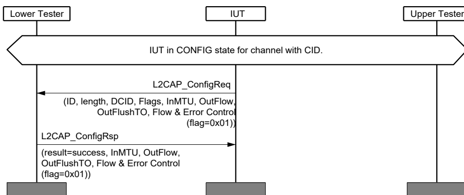
Figure 4.17: L2CAP/COS/CFD/BV-10-C [Retransmission Mode Negotiation] MSC
