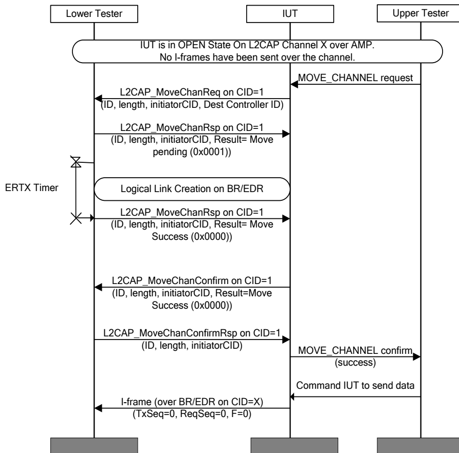
Figure 4.148: L2CAP/MCH/BV-21-C [Move Channel Request for AMP to BR/EDR (STM Source) – Success] MSC
