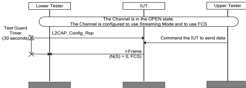
Figure 4.75: L2CAP/OFS/BV-07-C [Sending I-Frames with FCS for Streaming Mode] MSC
