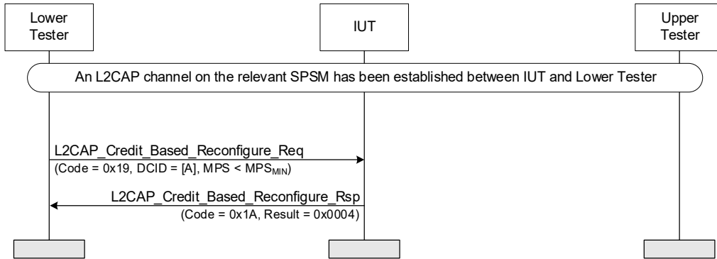
Figure 4.210: Reconfigure – other unacceptable parameters MSC
