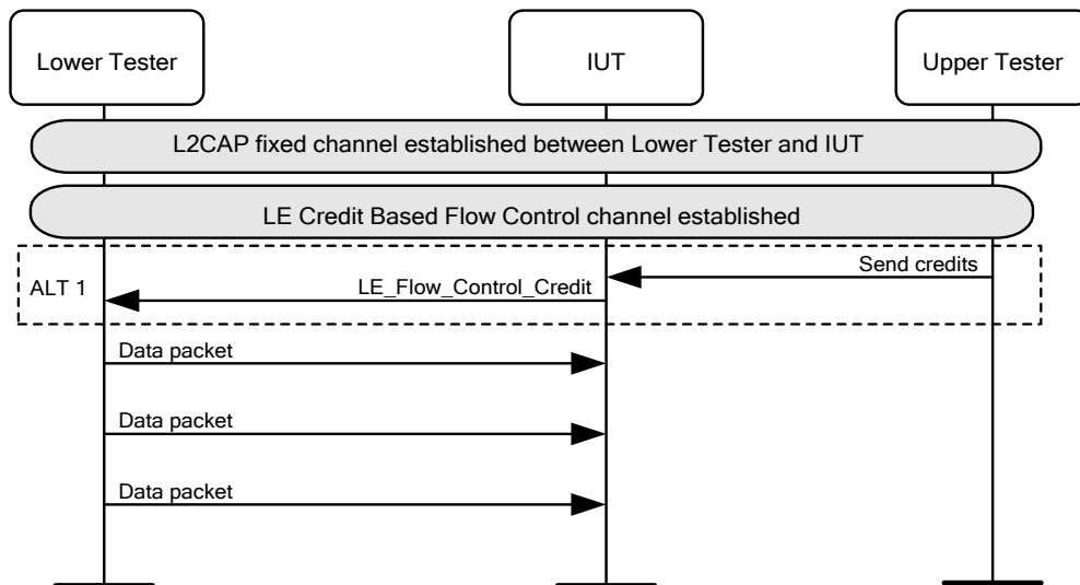
Figure 4.219: L2CAP/LE/CFC/BV-07-C [Credit Exchange – Sending Credits] MSC
