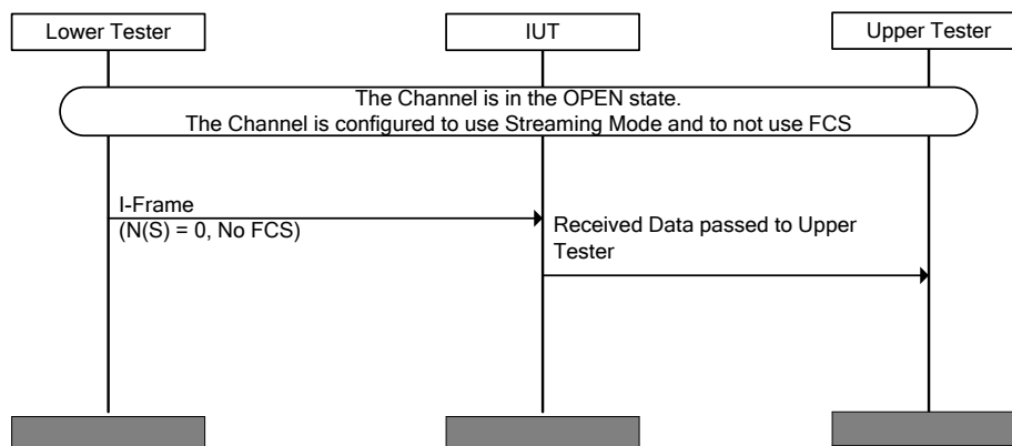
Figure 4.72: L2CAP/OFS/BV-04-C [Receiving Frames without FCS for Streaming Mode] MSC
