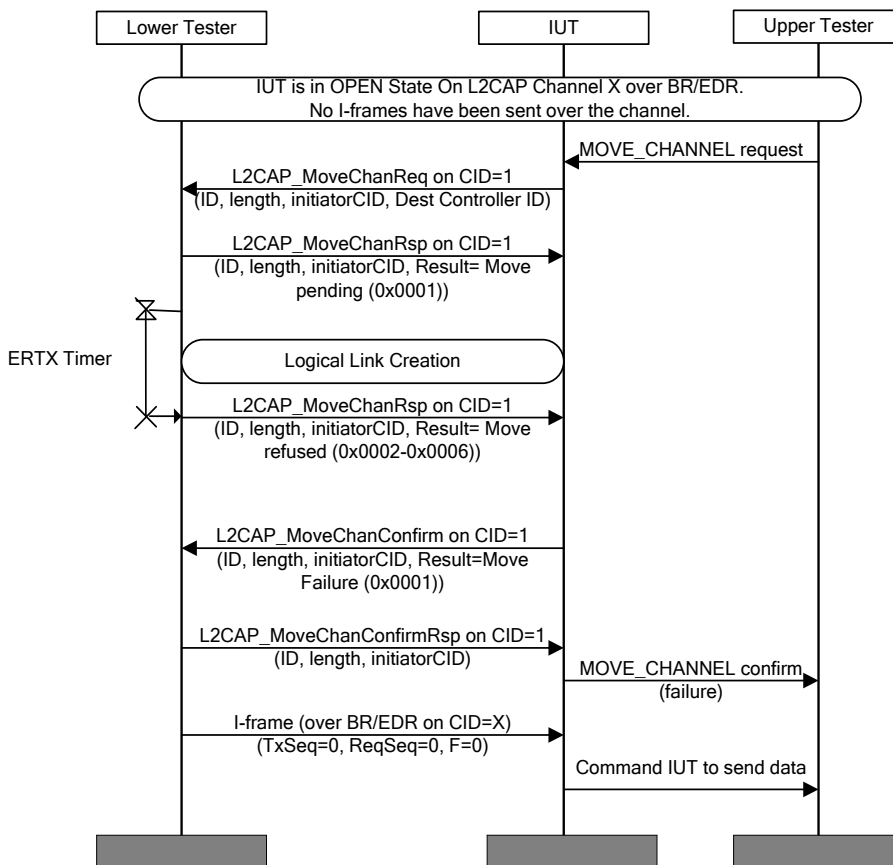
Figure 4.147: L2CAP/MCH/BV-20-C [Move Channel Request for BR/EDR to AMP (STM Sink) – AMP Failed] MSC
