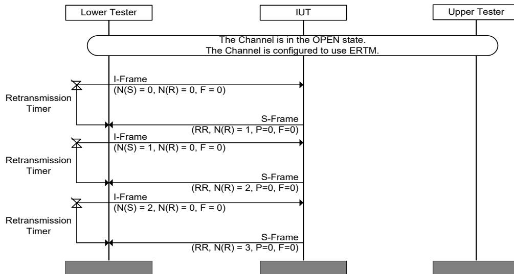
Figure 4.79: L2CAP/ERM/BV-03-C [Acknowledging Received I-Frames] MSC
