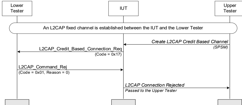
Figure 4.186: L2CAP Credit Based Connection Request – Legacy Peer MSC
