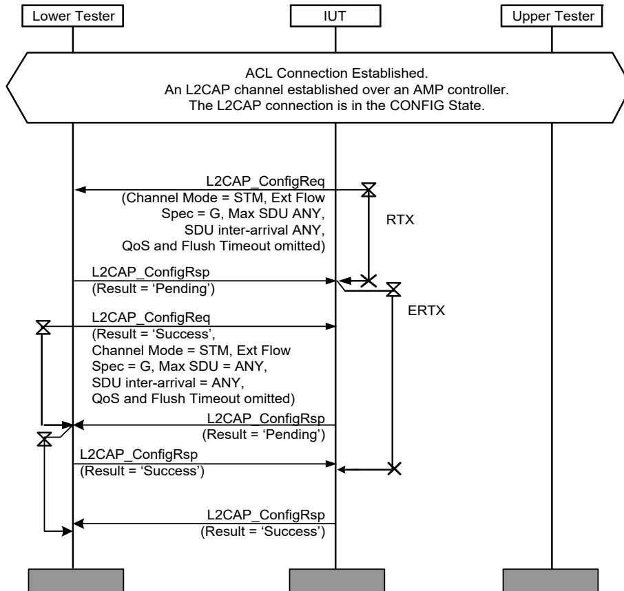
Figure 4.119: L2CAP/LSC/BV-08-C [Normal Lock Step Configuration Process for Guaranteed, AMP Channel] MSC
