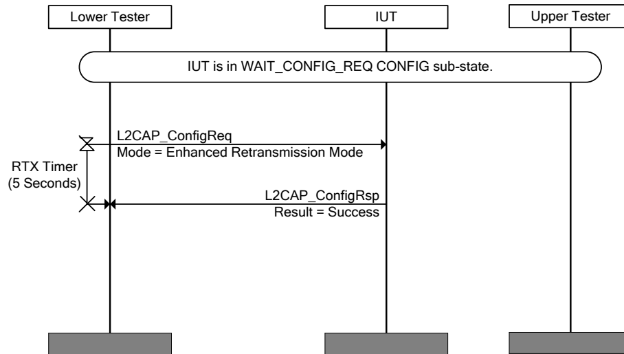
Figure 4.46: L2CAP/CMC/BV-02-C [Lower Tester Initiated Configuration of Enhanced Retransmission Mode] MSC
