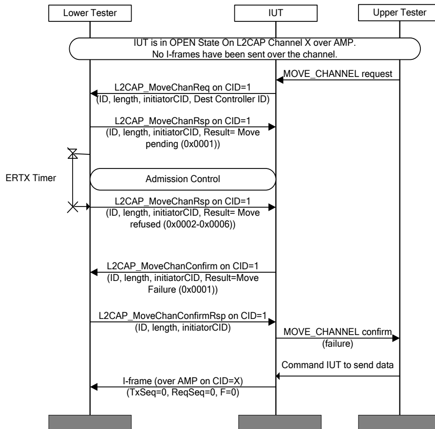
Figure 4.152: L2CAP/MCH/BV-25-C [Move Channel Request for AMP to BR/EDR (STM Source) – AMP Fail] MSC
