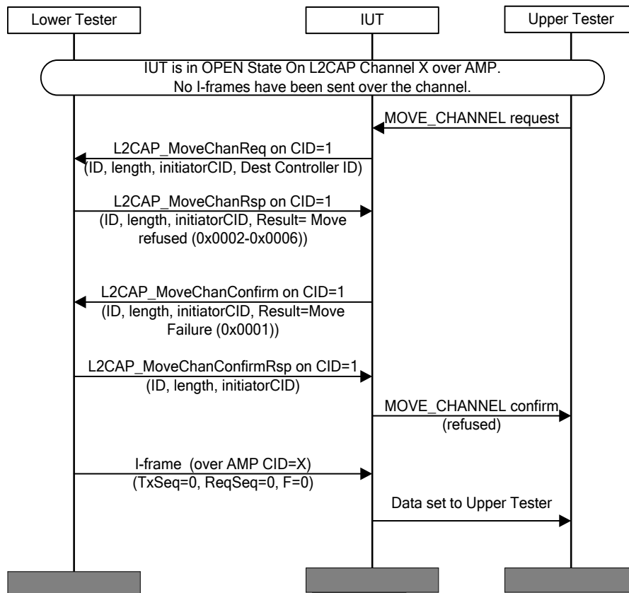
Figure 4.151: L2CAP/MCH/BV-24-C [Move Channel Request for AMP to BR/EDR (STM Sink) – Refused] MSC
