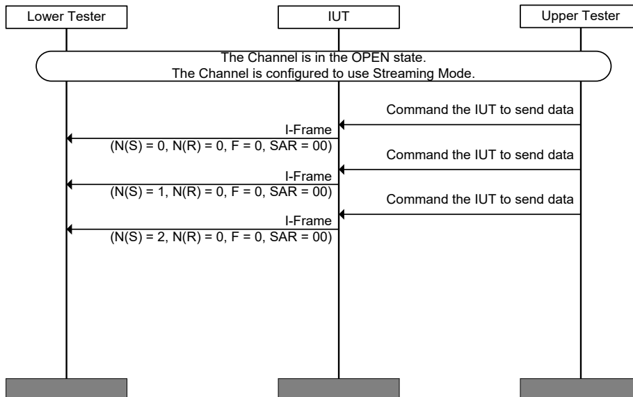
Figure 4.172: L2CAP/STM/BV-01-C [Streaming Mode Source with Extended Control Field] MSC
