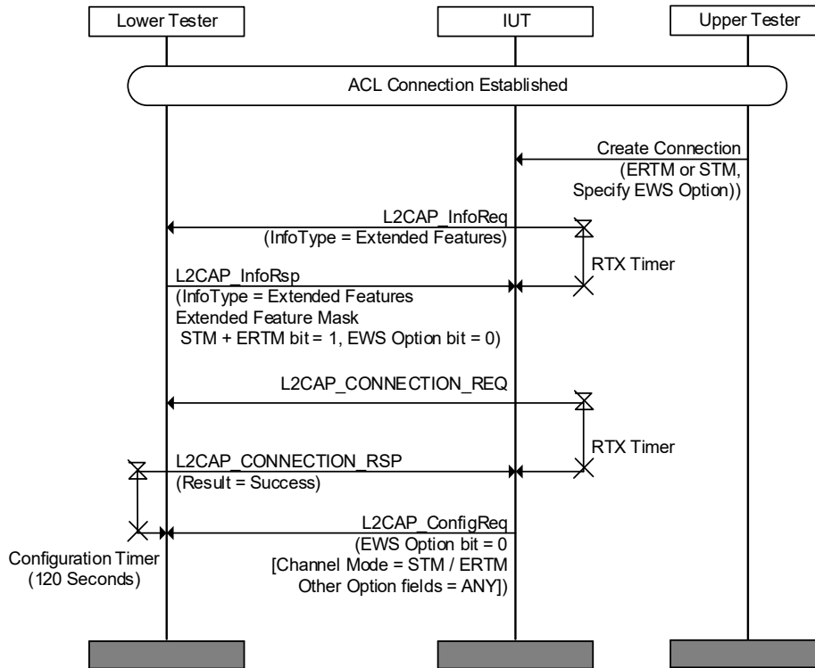
Figure 4.111: L2CAP/EWC/BV-03-C [Extended Window Size Option Not Supported by Lower Tester] MSC
