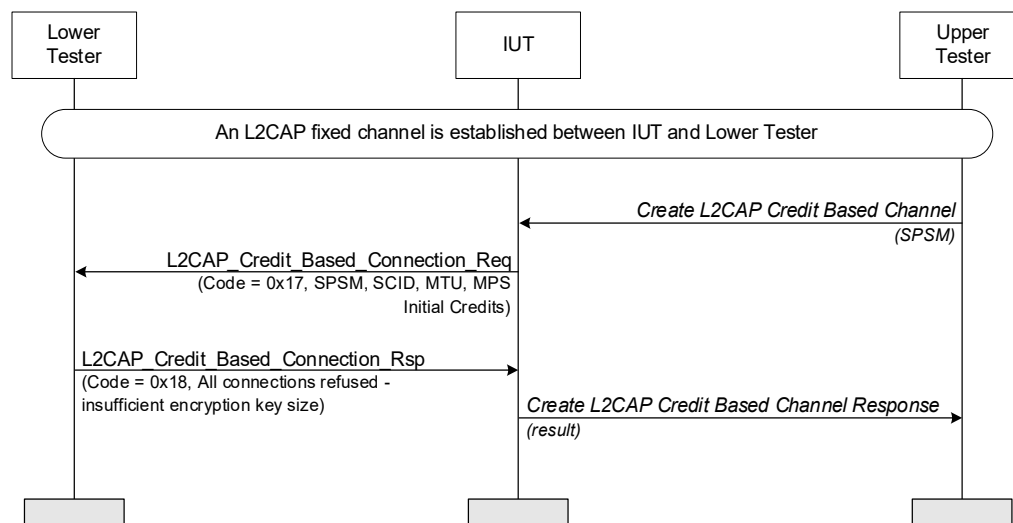
Figure 4.195: Security – Insufficient Encryption Key Size – Initiator MSC
