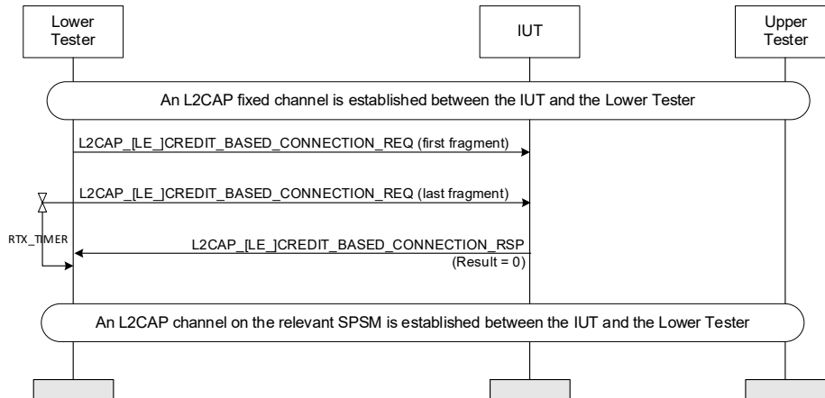
Figure 4.32: Recombination of Signaling Packets MSC
