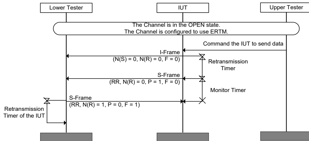
Figure 4.83: L2CAP/ERM/BV-08-C [Send S-Frame [RR] with Poll Bit Set] MSC
