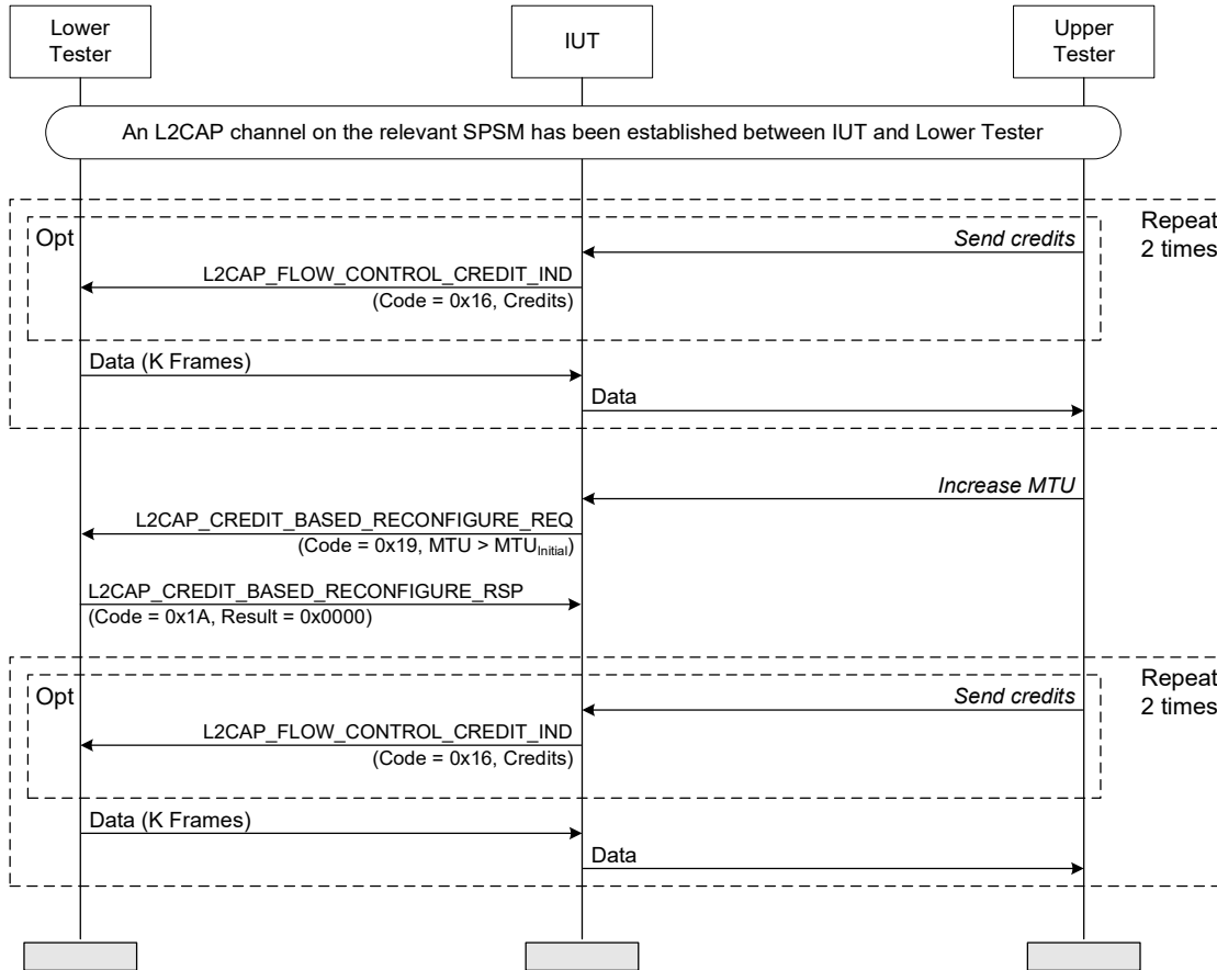
Figure 4.201: Renegotiate MTU – Initiator MSC
