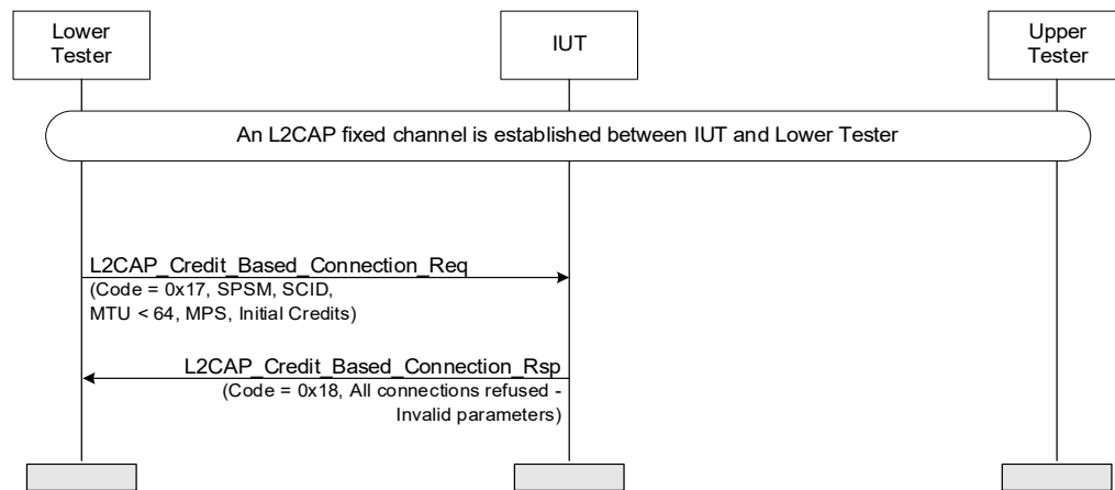
Figure 4.207: L2CAP Credit Based Connection Response – refused due to Invalid Parameters MSC
