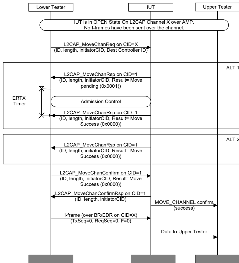
Figure 4.157: L2CAP/MCH/BV-30-C [Move Channel Response for AMP to BR/EDR (STM Sink) – Success] MSC
