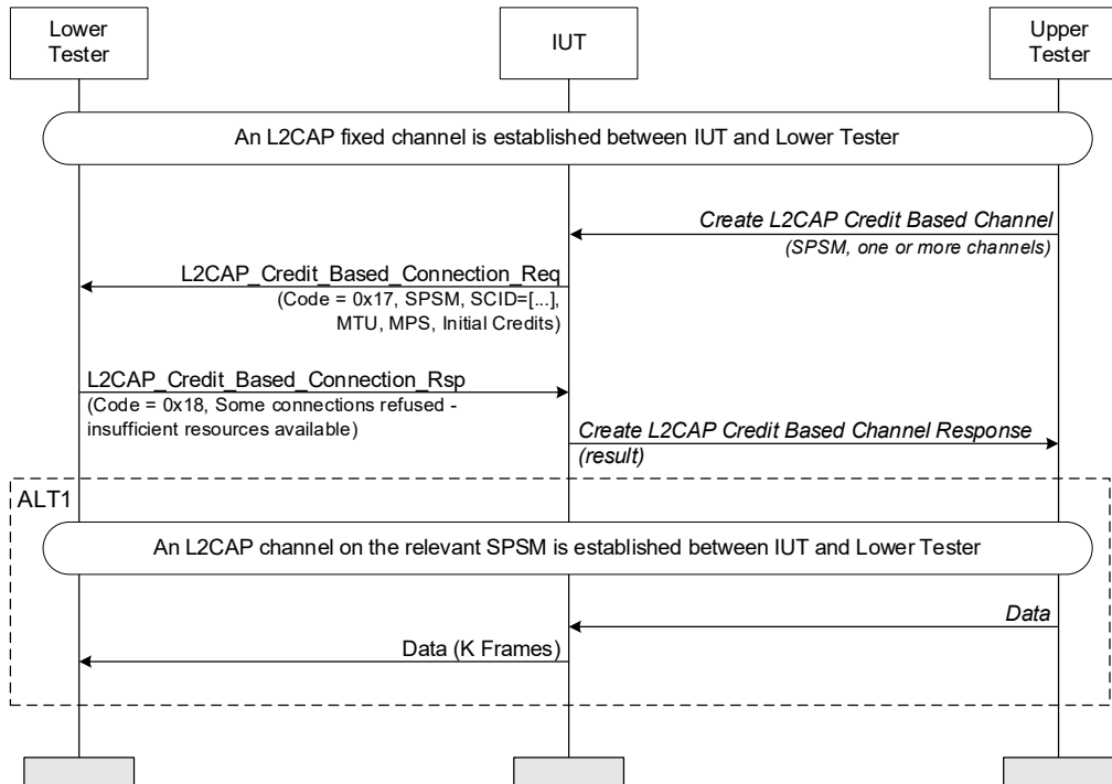
Figure 4.235: L2CAP Credit Based Connection Request – refused due to insufficient resources MSC
