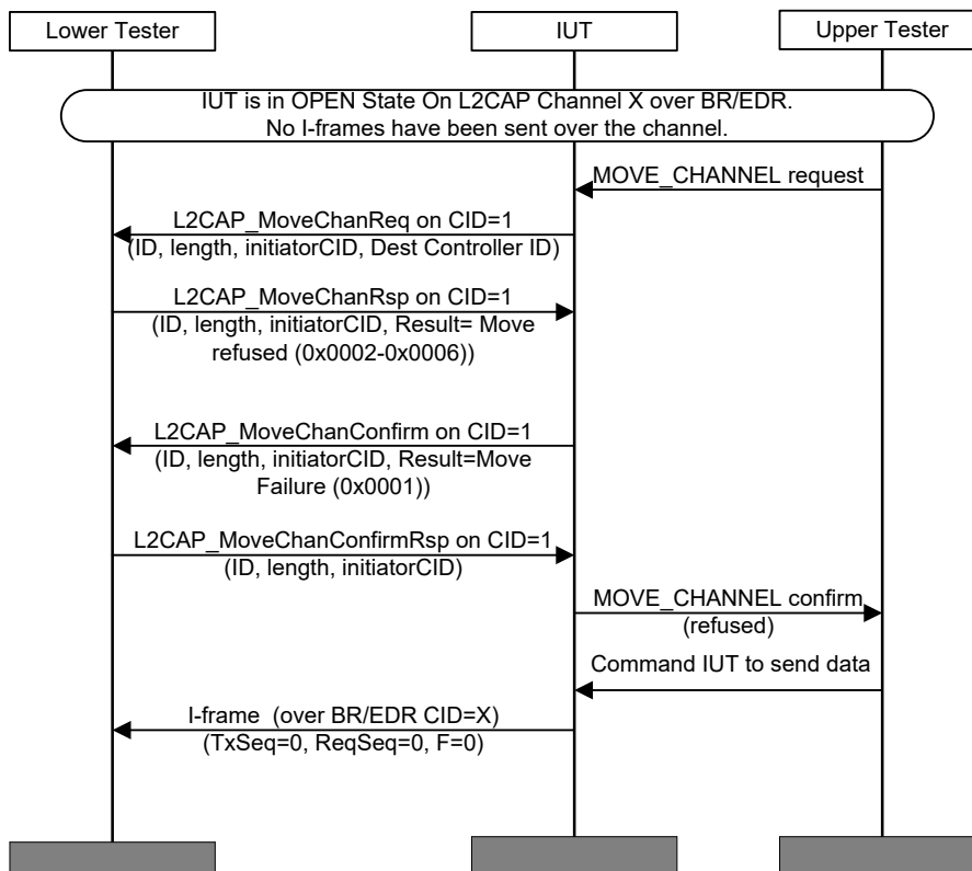
Figure 4.144: L2CAP/MCH/BV-17-C [Move Channel Request for BR/EDR to AMP (STM Source) – Refused] MSC
