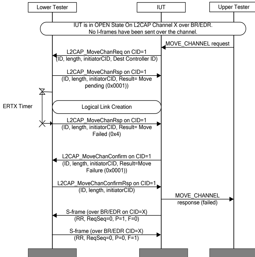
Figure 4.130: L2CAP/MCH/BV-03-C [Move ERTM Channel Request for BR/EDR to AMP – AMP Fail] MSC
