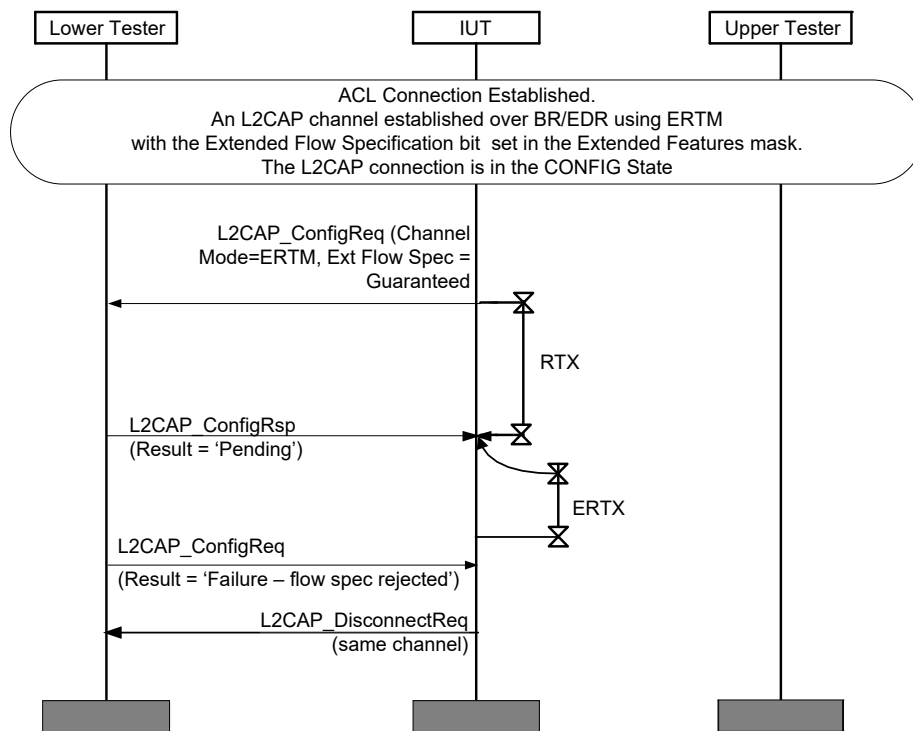
Figure 4.116: L2CAP/LSC/BI-05-C [Mismatched Service Type, Guaranteed, BR/EDR ERTM Channel] MSC
