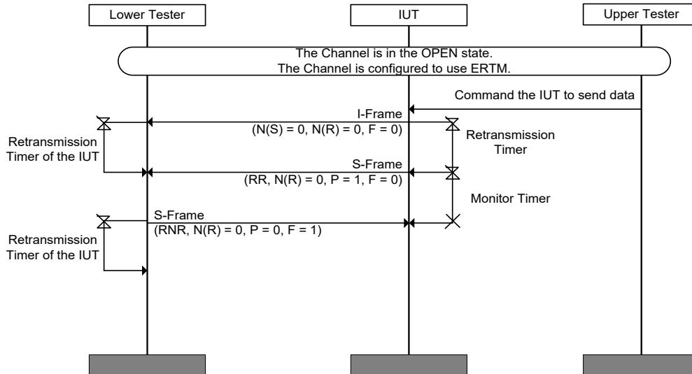
Figure 4.95: L2CAP/ERM/BV-20-C [Enter Remote Busy Condition] MSC
