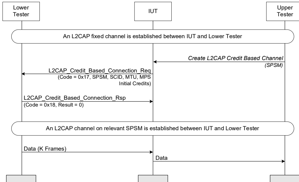
Figure 4.187: L2CAP Credit Based Connection Request on Supported PSM MSC
