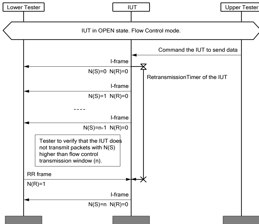
Figure 4.37: L2CAP/COS/FLC/BV-02-C [Resume Flow on RR Frame Ack] MSC
