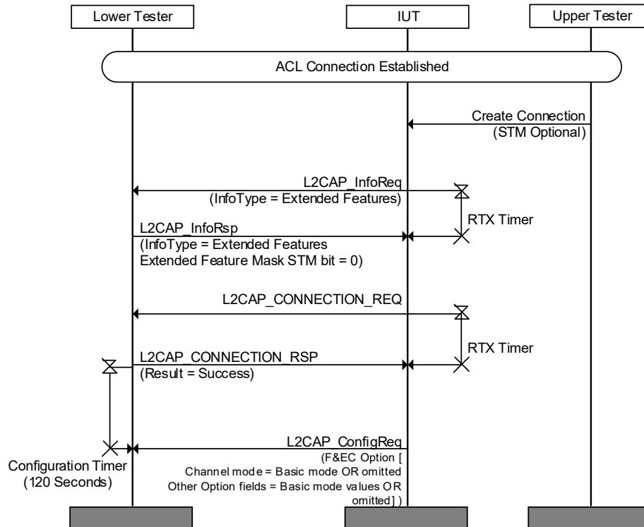
Figure 4.61: L2CAP/CMC/BV-11-C [Streaming Mode not supported by Lower Tester for Optional Streaming Mode Channel] MSC
