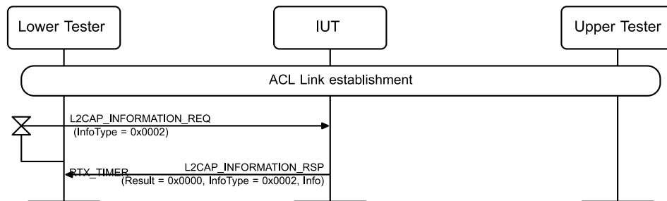
Figure 4.44: L2CAP/EXF/BV-08-C [Information Request, Extended Features] MSC
