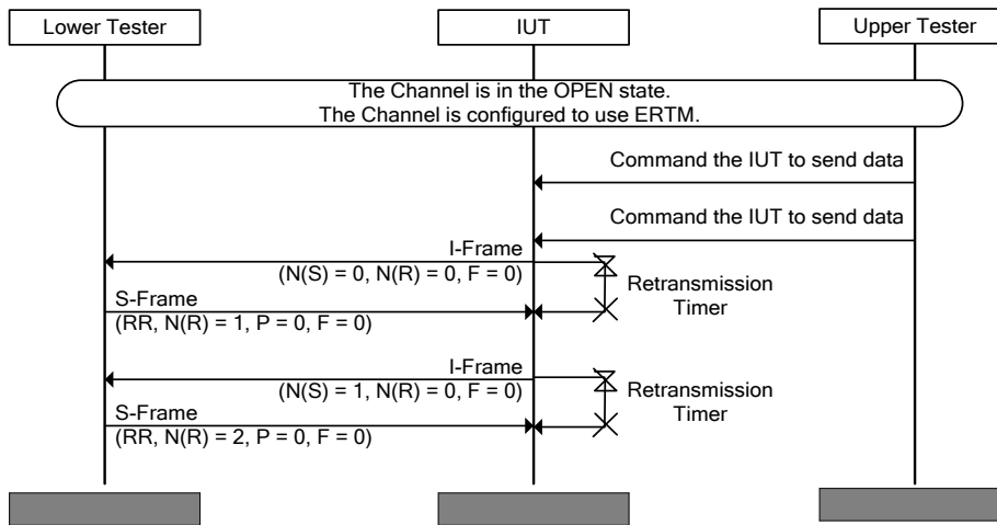
Figure 4.80: L2CAP/ERM/BV-05-C [Resume Transmitting I-Frames when an S-Frame [RR] is Received] MSC
