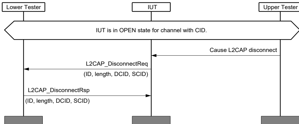
Figure 4.3: L2CAP/COS/CED/BV-04-C [Disconnect] MSC
