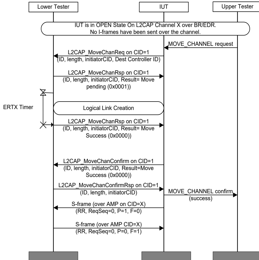
Figure 4.128: L2CAP/MCH/BV-01-C [Move ERTM Channel Request for BR/EDR to AMP – Success] MSC
