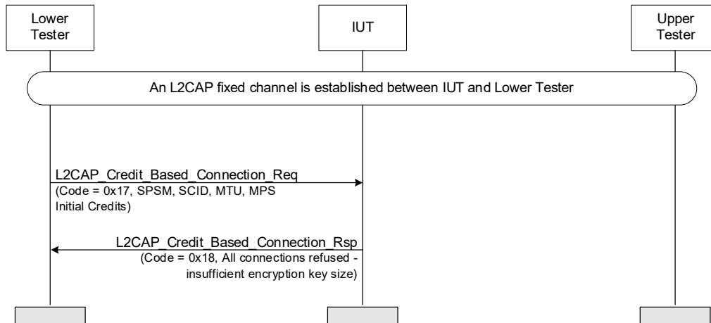
Figure 4.234: Security – Insufficient Encryption Key Size – Responder MSC
