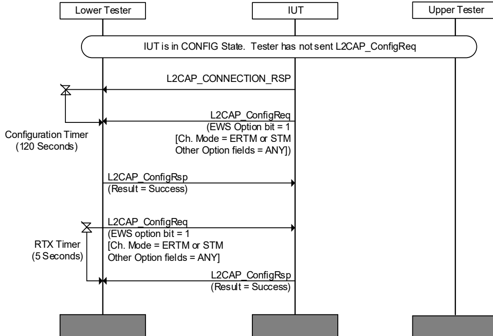
Figure 4.109: L2CAP/EWC/BV-01-C [IUT Initiated Extended Window Size Option] MSC
