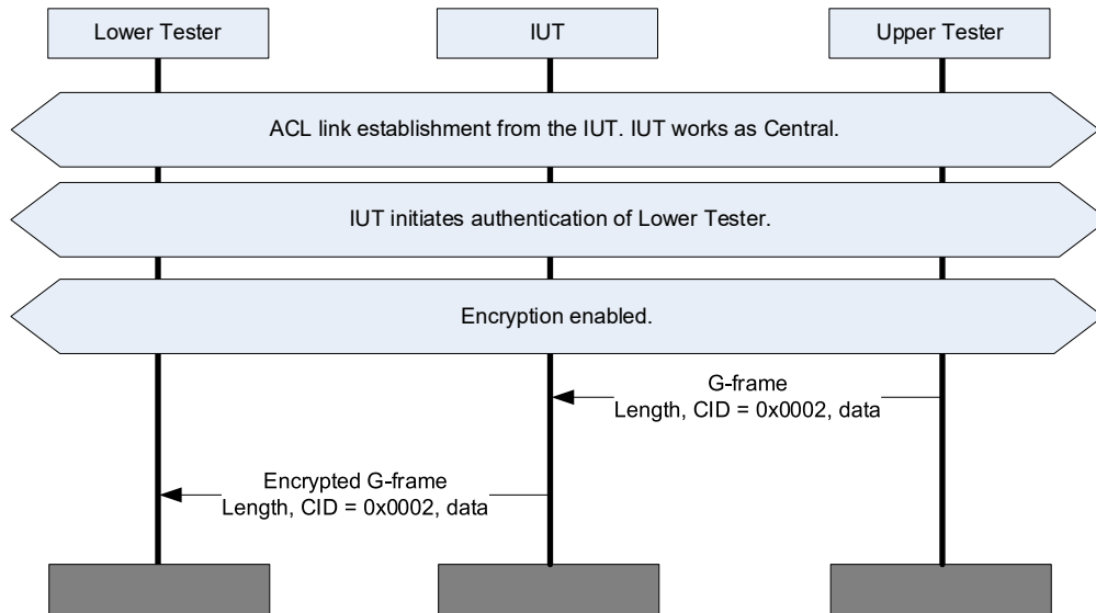
Figure 4.183: L2CAP/CLS/UCD/BV-03-C [Encrypted Data Transmission over Unicast Connectionless Channel] MSC
