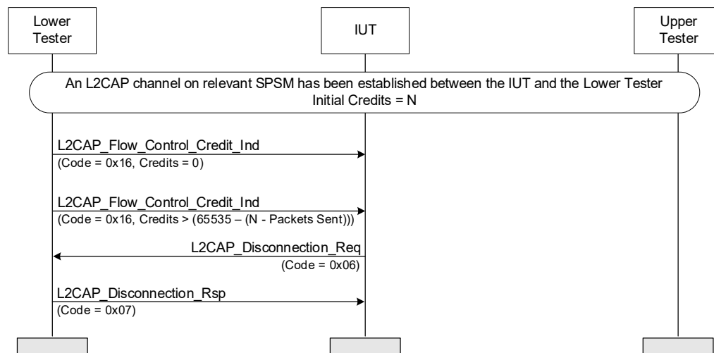
Figure 4.192: Credit Exchange – Zero Credits and Exceed Maximum Credits MSC
