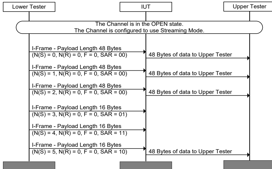
Figure 4.104: L2CAP/STM/BV-02-C [Streaming Mode Sink] MSC
