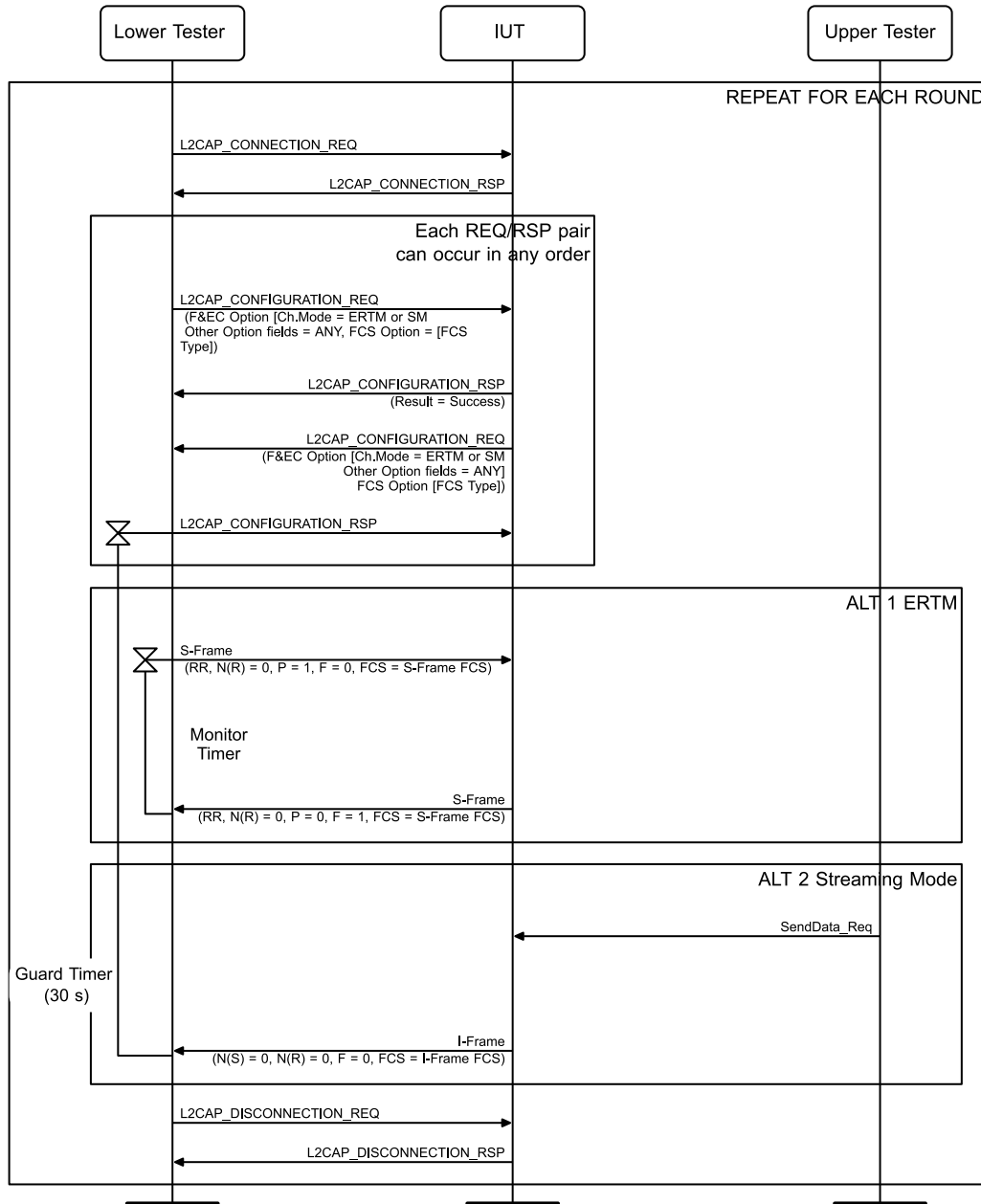
Figure 4.68: IUT Responder, Configuration of the FCS Option MSC
