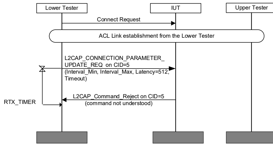
Figure 4.178: L2CAP/LE/CPU/BI-02-C [Reject Connection Parameter Update Request] MSC
