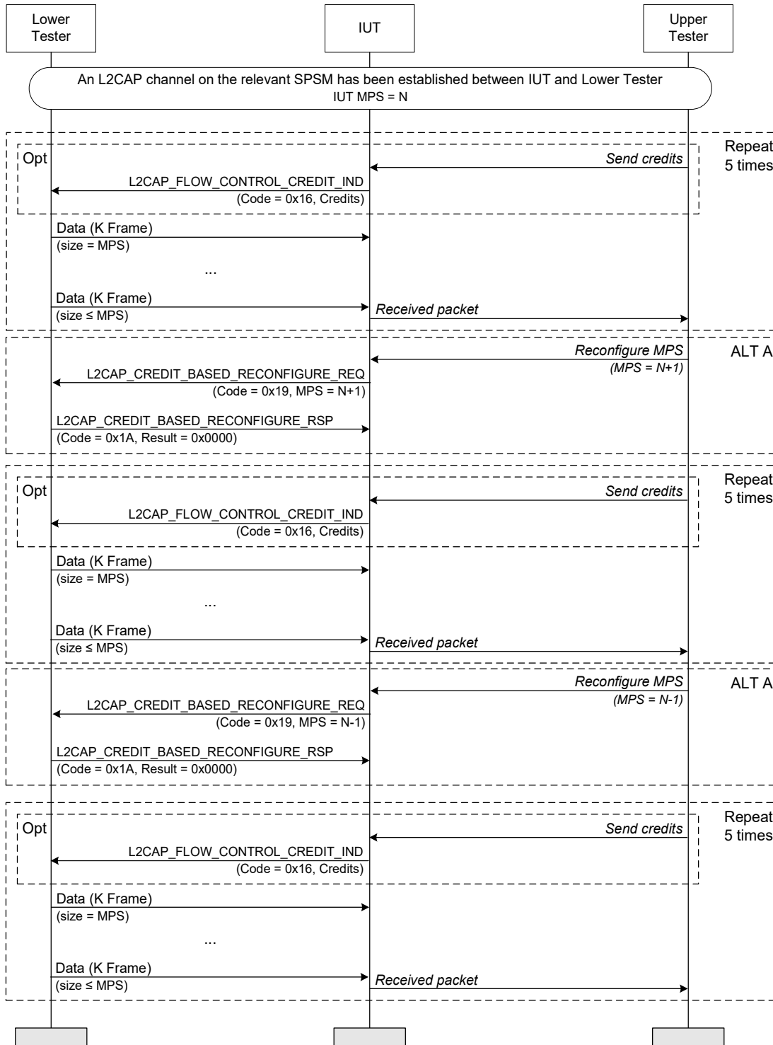
Figure 4.204: Renegotiate MPS – Initiator MSC
