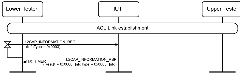
Figure 4.108: L2CAP/FIX/BV-03-C [Information Request, Fixed Channels Supported] MSC
