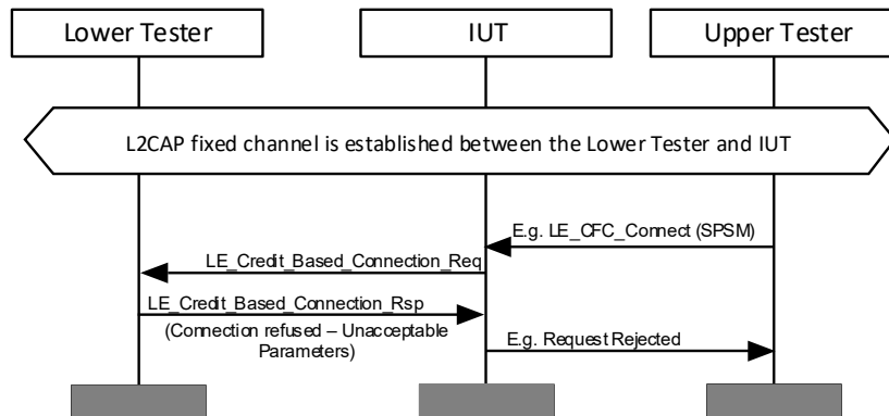
Figure 4.227: L2CAP/LE/CFC/BV-21-C [LE Credit Based Connection Request - refused due to Unacceptable Parameters - Initiator] MSC
