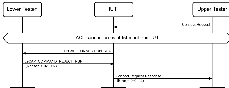
Figure 4.10: L2CAP/COS/CED/BI-30-C [Accept Reject of Connection Request, Peer Older Than v4.2] MSC
