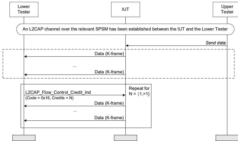
Figure 4.190: Credit Exchange – Receiving Incremental Credits MSC
