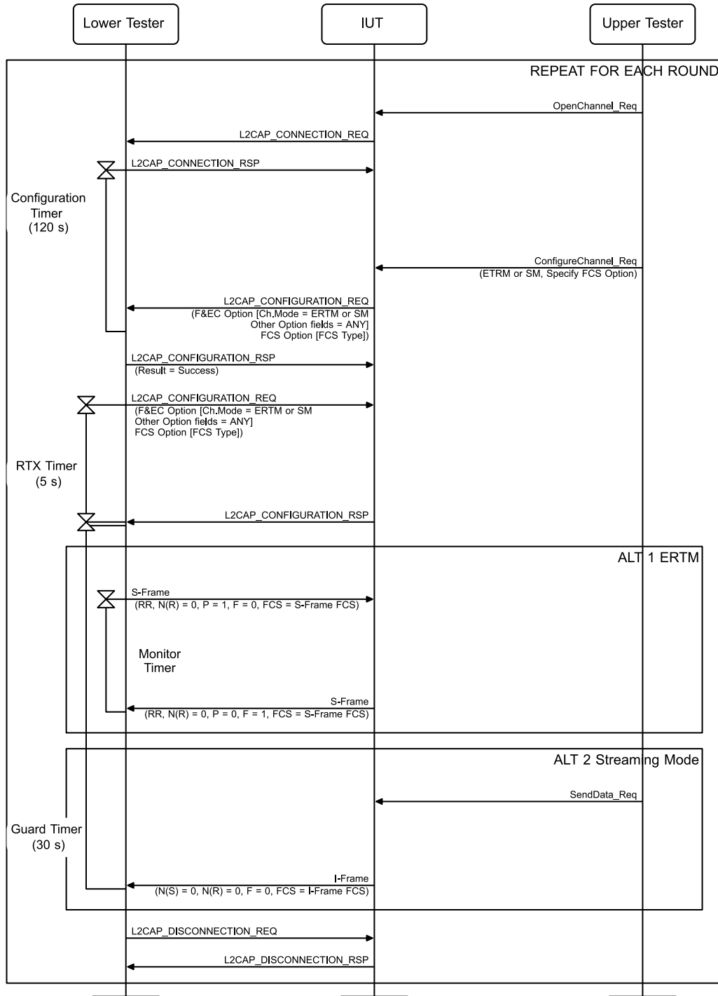
Figure 4.67: IUT Initiated Configuration of the FCS Option, IUT FCS or Omitted MSC
