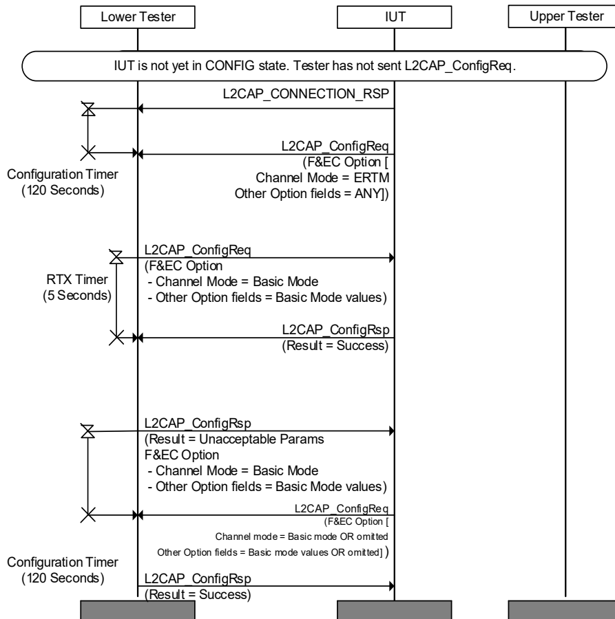
Figure 4.51: L2CAP/CMC/BV-07-C [Configuration Mode mismatch when use of Enhanced Retransmission Mode is Optional] MSC
