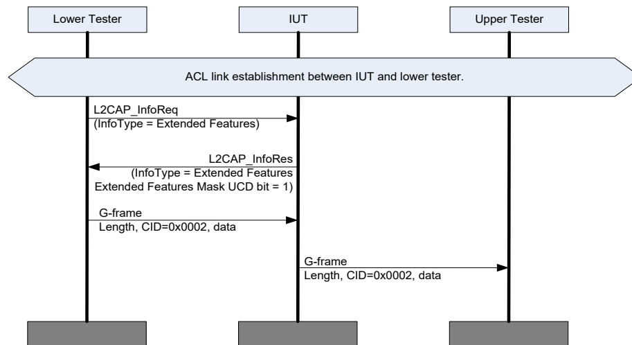
Figure 4.181: L2CAP/CLS/UCD/BV-01-C [Data Reception over Unicast Connectionless Channel] MSC
