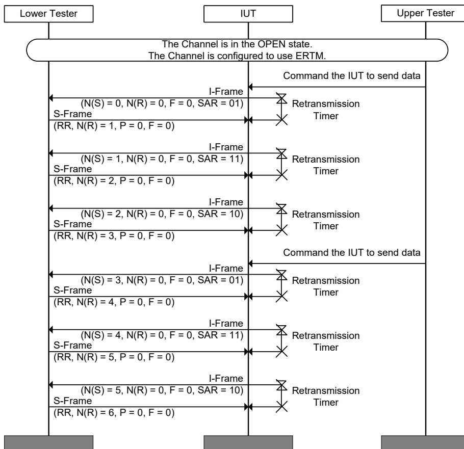
Figure 4.171: L2CAP/ECF/BV-08-C [Transmit I-Frames using Extended Control Field and SAR] MSC
