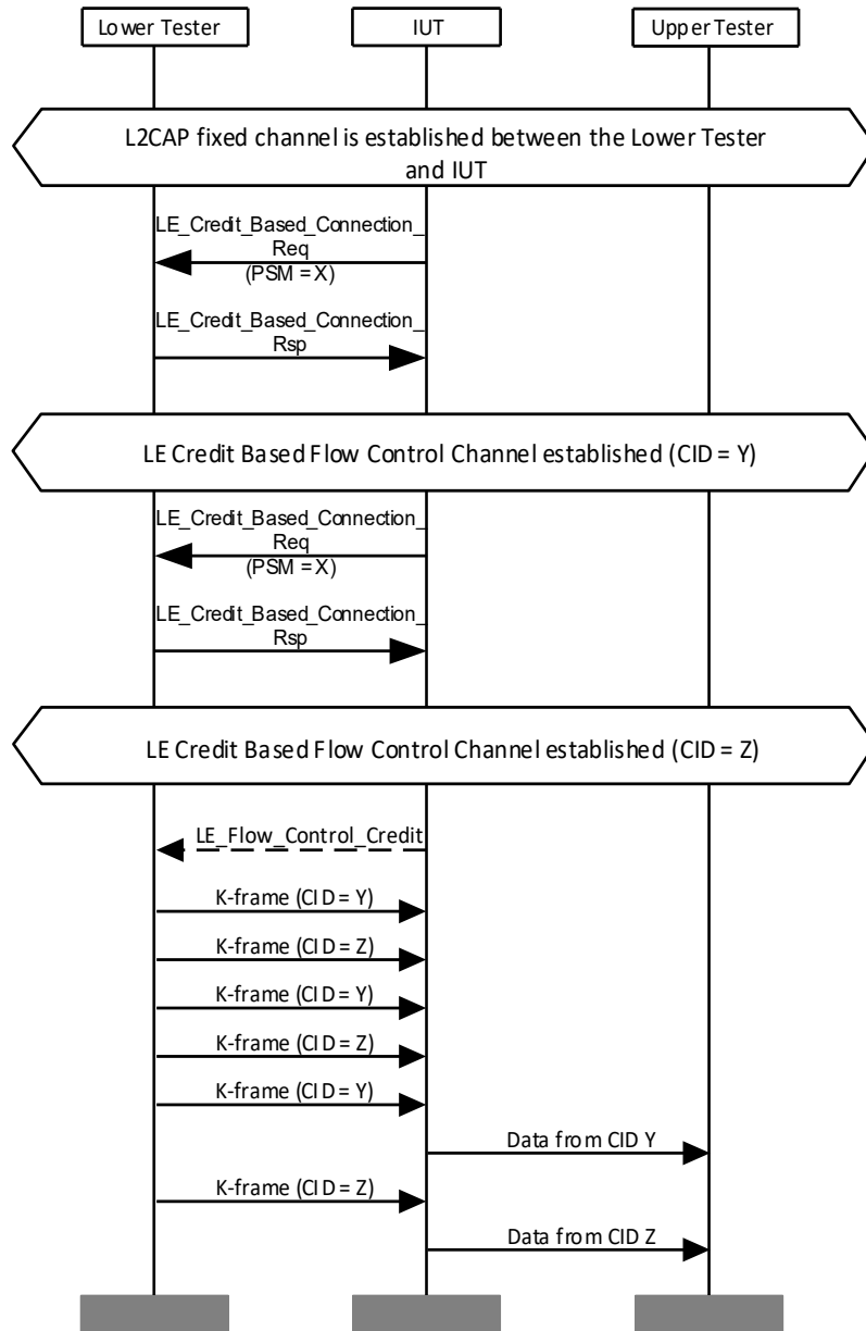
Figure 4.31: L2CAP/COS/CFC/BV-05-C [Multiple Channels with Interleaved Data Streams] MSC
