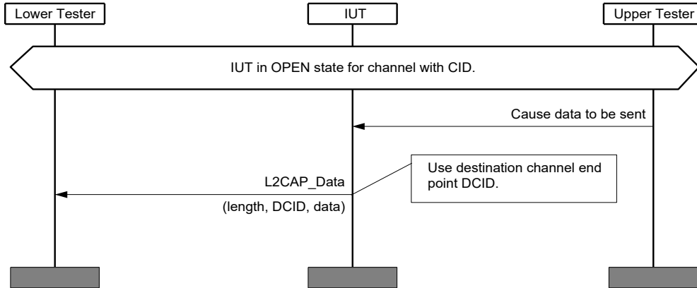
Figure 4.2: L2CAP/COS/CED/BV-03-C [Send Data] MSC
