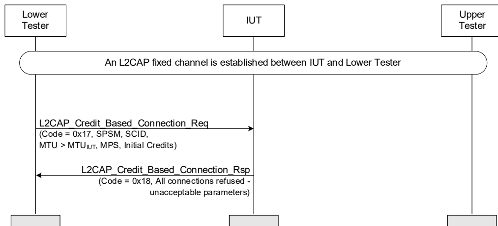
Figure 4.208: L2CAP Credit Based Connection Response – refused due to Unacceptable Parameters MSC
