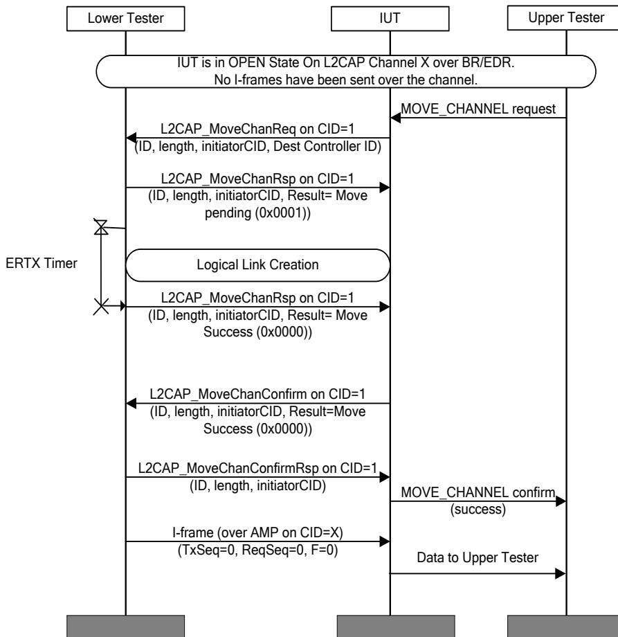
Figure 4.143: L2CAP/MCH/BV-16-C [Move Channel Request for BR/EDR to AMP (STM Sink) – Success] MSC
