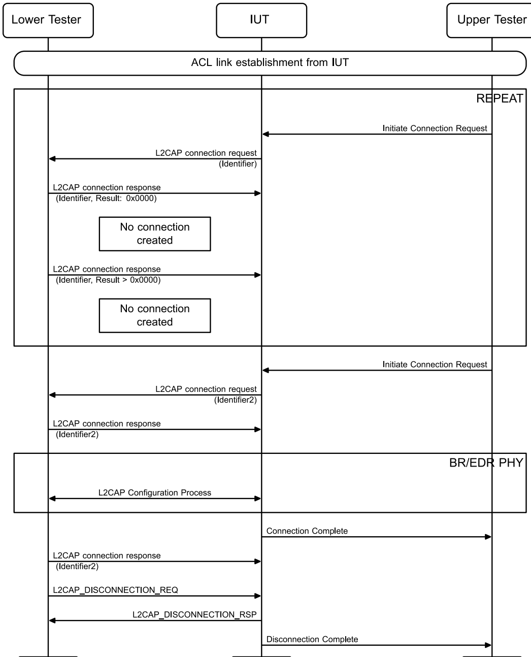
Figure 4.11: Ignore Command Response with Invalid ID or Duplicate Response MSC
