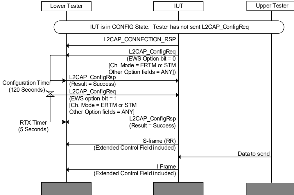
Figure 4.110: L2CAP/EWC/BV-02-C [Lower Tester Requests Extended Window Size] MSC
