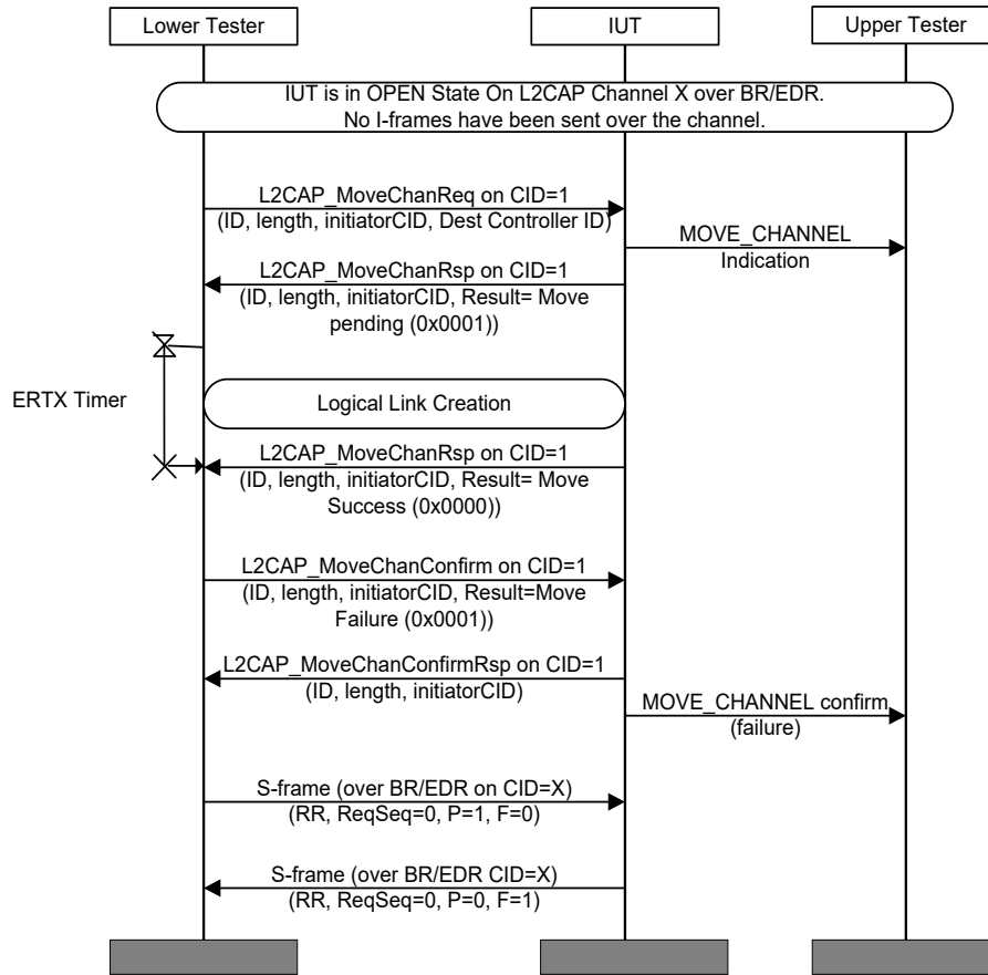
Figure 4.134: L2CAP/MCH/BV-07-C [Move ERTM Channel Response for BR/EDR to AMP – Failure] MSC
