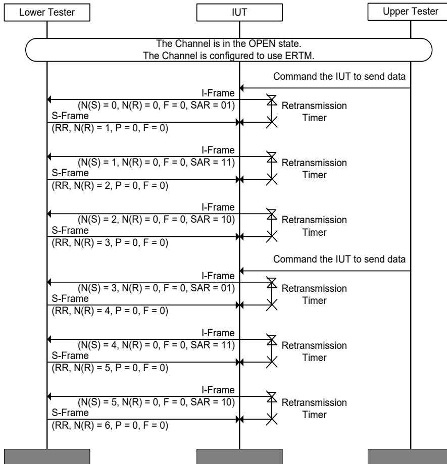
Figure 4.97: L2CAP/ERM/BV-23-C [Transmit I-Frames using SAR] MSC
