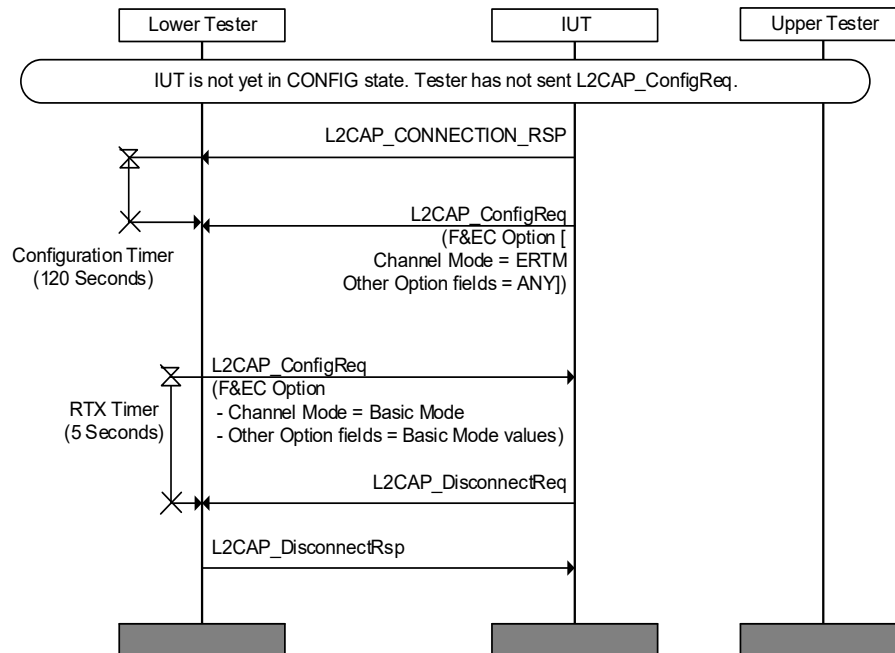
Figure 4.55: L2CAP/CMC/BI-02-C [Configuration Mode mismatch when use of Enhanced Retransmission Mode is Mandatory] MSC
