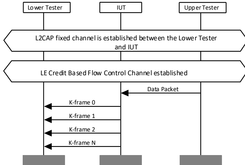
Figure 4.27: L2CAP/COS/CFC/BV-01-C [Segmentation] MSC
