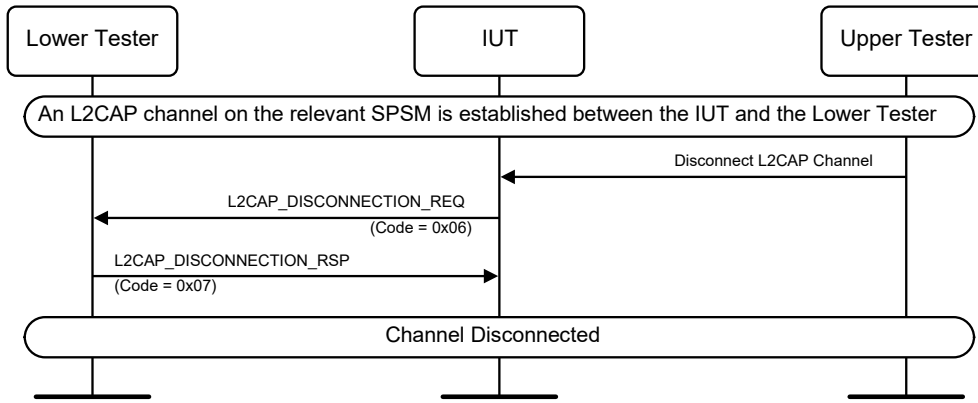
Figure 4.229: Disconnection Request MSC
