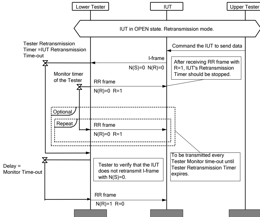
Figure 4.40: L2CAP/COS/RTX/BV-01-C [No Retransmission with R=1] MSC
