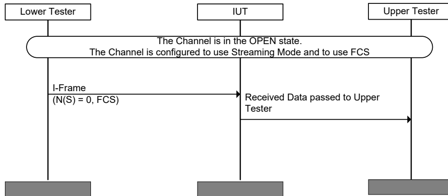
Figure 4.76: L2CAP/OFS/BV-08-C [Receiving Frames with FCS for Streaming Mode] MSC
