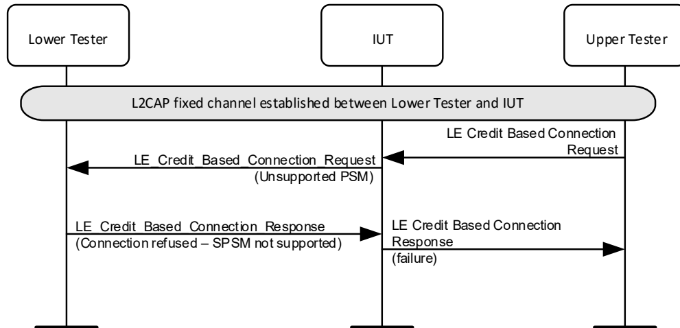
Figure 4.216: L2CAP/LE/CFC/BV-04-C [LE Credit Based Connection Request on an unsupported SPSM] MSC
