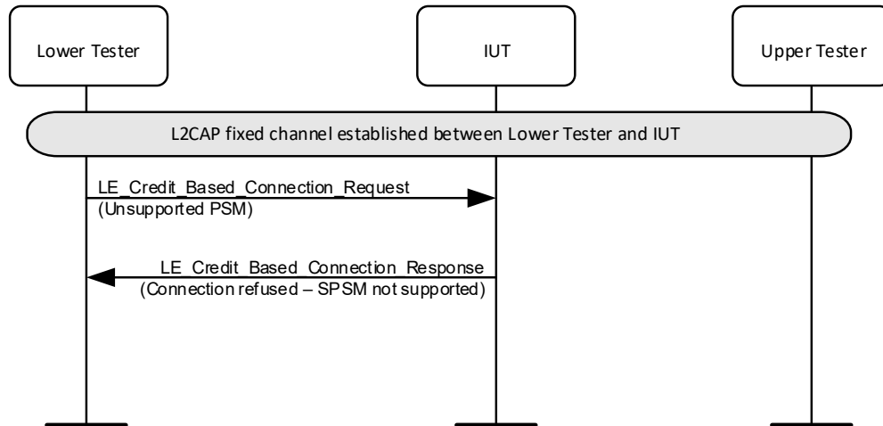
Figure 4.217: L2CAP/LE/CFC/BV-05-C [LE Credit Based Connection Request - unsupported SPSM] MSC
