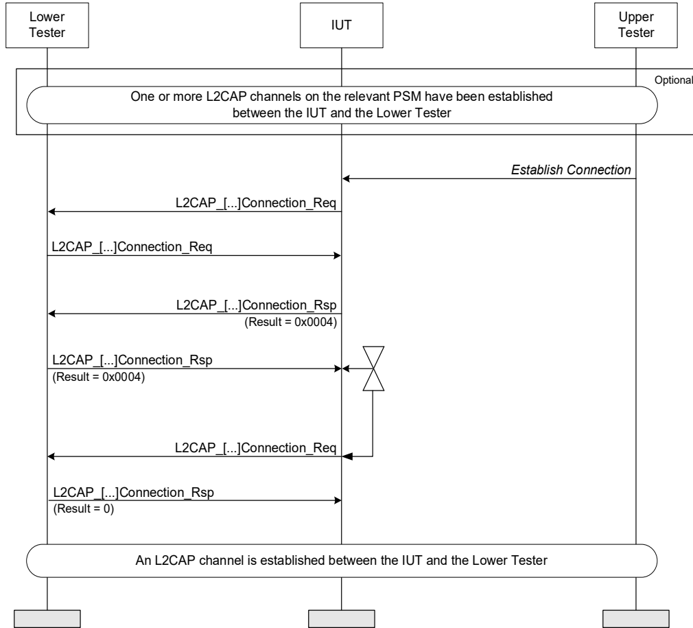
Figure 4.243: Back-off on Connection Request Collision MSC
