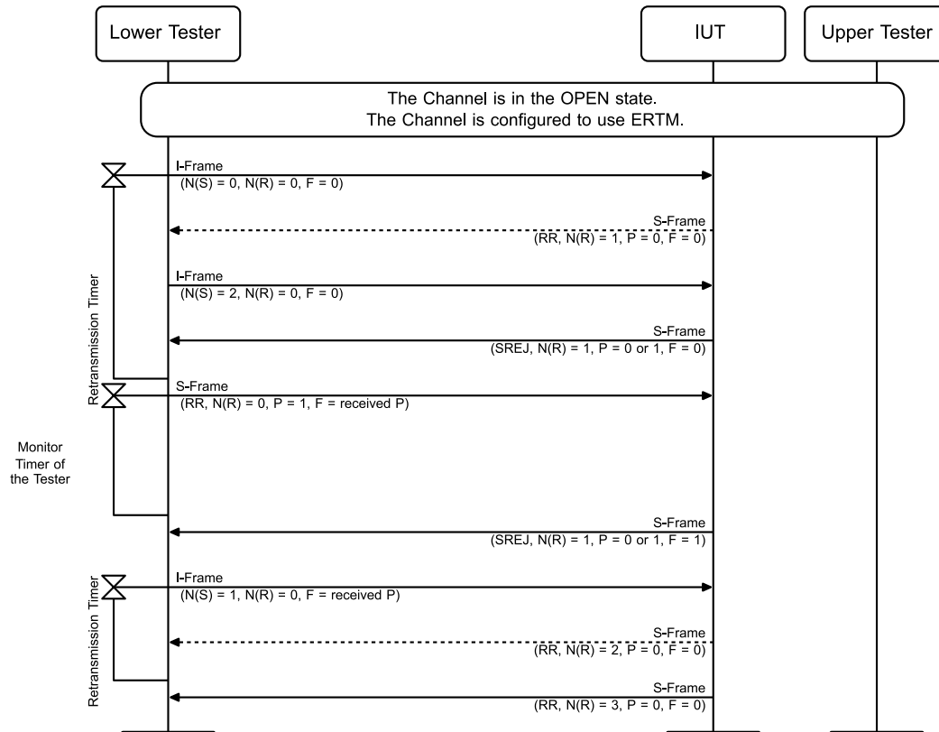
Figure 4.99: L2CAP/ERM/BI-02-C [S-Frame [SREJ] Lost or Corrupted] MSC
