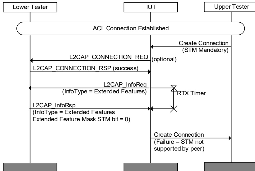
Figure 4.63: L2CAP/CMC/BV-13-C [Streaming Mode not supported by Lower Tester for Mandatory Streaming Mode Channel] MSC
