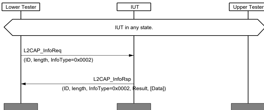
Figure 4.23: L2CAP/COS/IEX/BV-02-C [Respond with 1.2 Features] MSC
