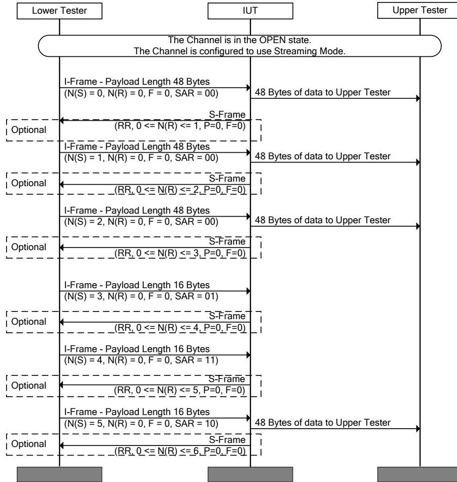
Figure 4.164: L2CAP/ECF/BV-01-C [Receive I-Frames with Extended Control Field] MSC
