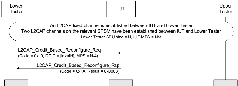
Figure 4.209: Reconfigure – refused due to invalid Destination CID MSC
