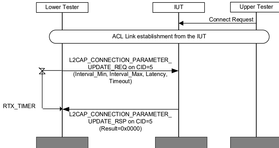
Figure 4.176: L2CAP/LE/CPU/BV-02-C [Accept Connection Parameter Update Request] MSC
