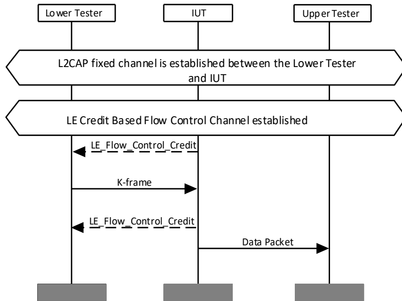
Figure 4.30: L2CAP/COS/CFC/BV-04-C [Data Receiving] MSC
