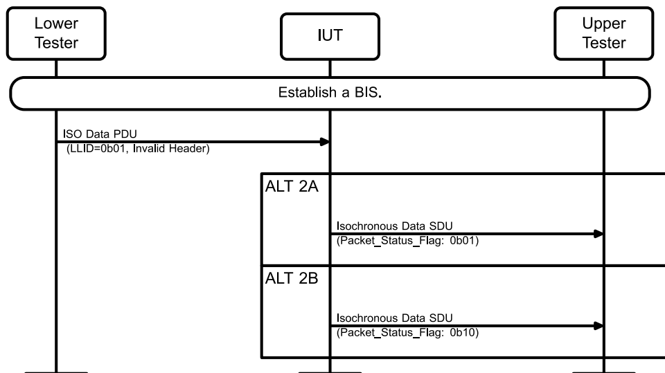
Figure 4.36: IAL/BIS/FRA/SNC/BI-02-C [SDU Reporting, BIS, BN = 1, NSE = 1, Framed PDU] MSC
