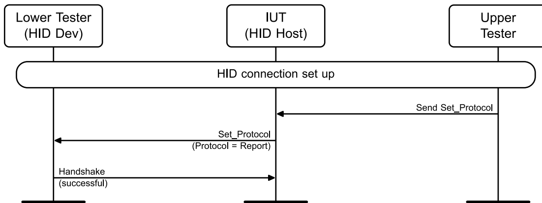
Figure 4.5: HID11/HOS/HCT/BV-05-C [Set_Protocol]
