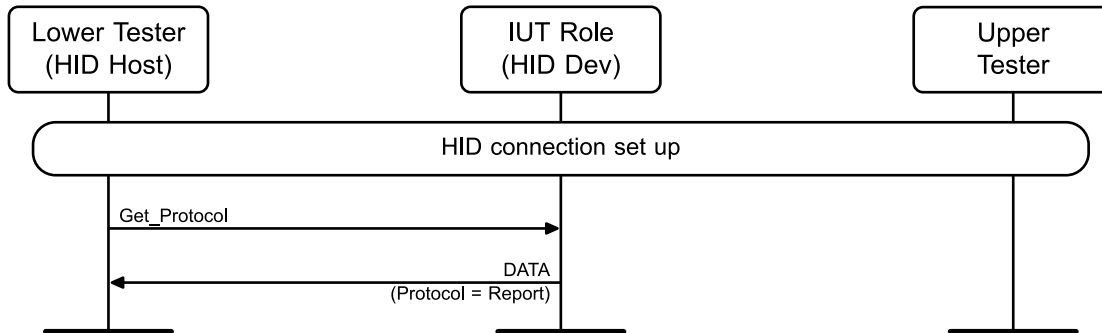
Figure 4.21: HID11/DEV/DCT/BV-03-C [Get_Protocol]
