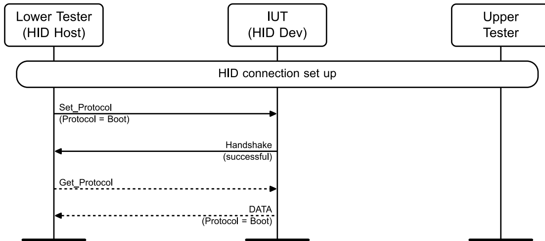
Figure 4.22: HID11/DEV/DCT/BV-04-C [Set_Protocol]
