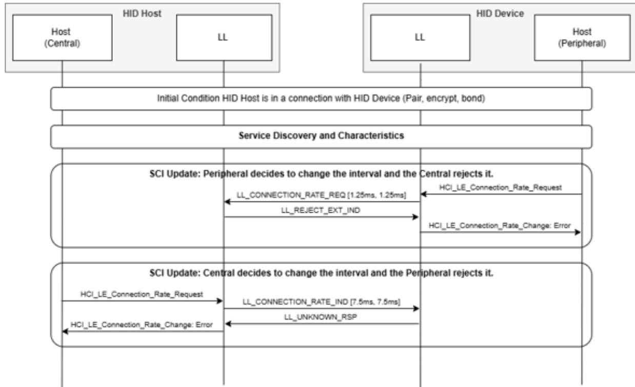
Figure 7.3: Example of HID Control Point characteristic usage with rejected changes (not all messages are shown)
