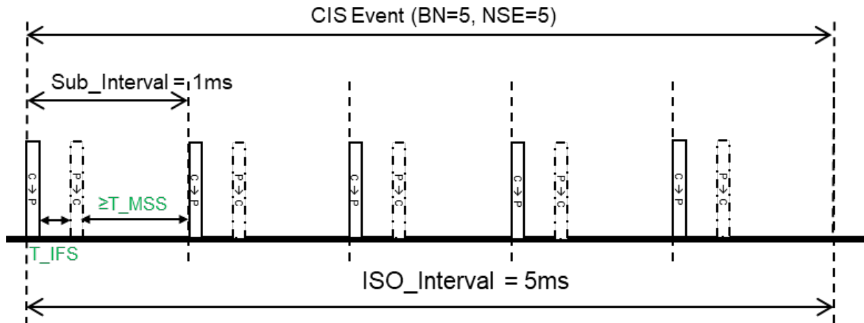
Figure C.1: Timing diagram of 1 ms report interval
