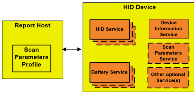
Figure 2.2: Report Host and HID Device Roles/Service Relationships
