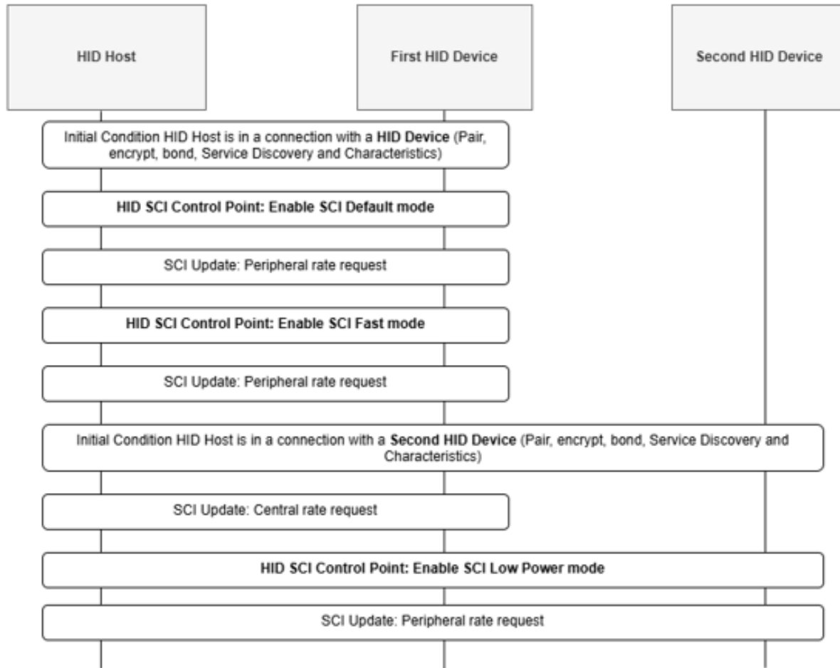
Figure 7.2: Example of HID Control Point characteristic usage with multiple devices in different HID SCI modes (not all messages are shown)
