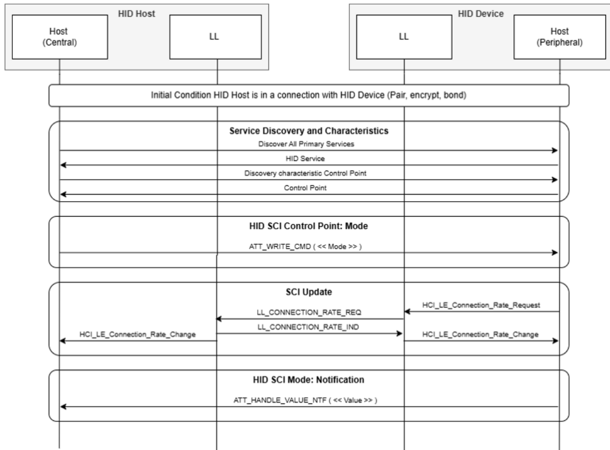
Figure 7.1: Example of initial discovery and configuration of SCI conveying information related to SCI (not all messages are shown)
