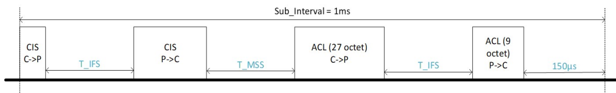
Figure C.2: One sub-interval with ACL event
