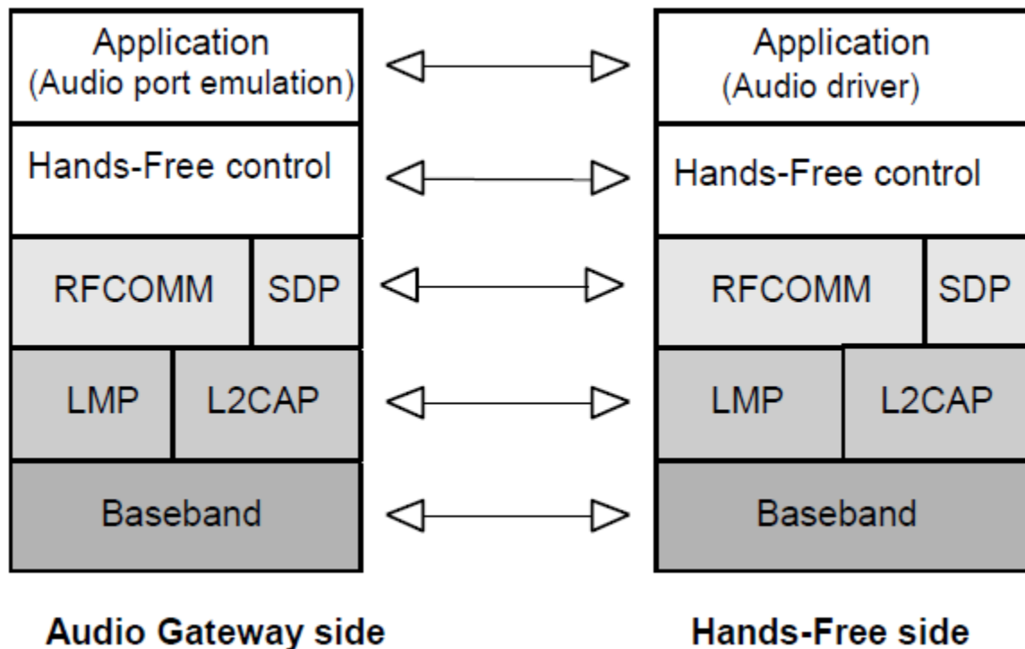
Figure 2.1: Protocol stack
