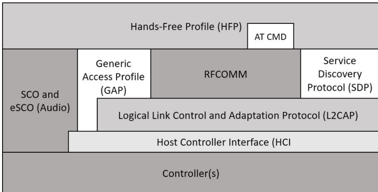
Figure 1.1: Bluetooth Profiles
