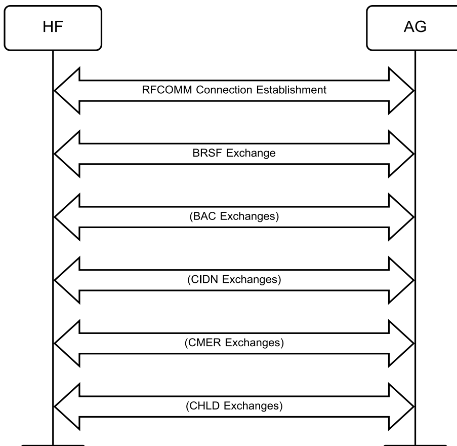
Figure 4.7: SLC, IUT supports HF Indicators, Lower Tester does not MSC
