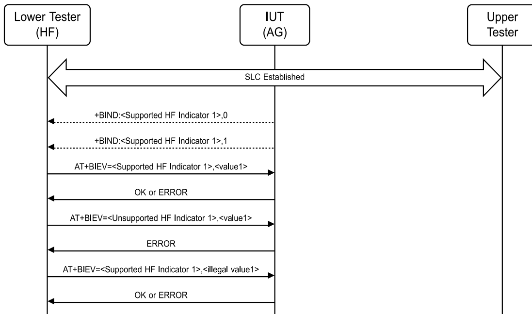
Figure 4.23: HFP/AG/HFI/BI-03-C [AG receives invalid HF Indicator values] MSC
