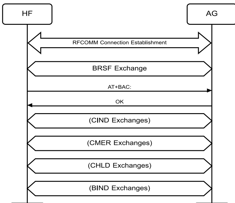
Figure 4.3: HF Initiates SLC with Codec Negotiation MSC
