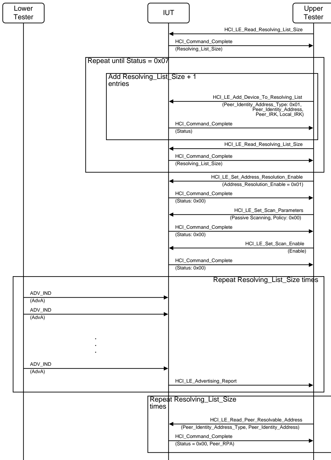
Figure 4.107: HCL/CCO/BI-50-C [LE Add Device To Resolving List – No Space Available] MSC
