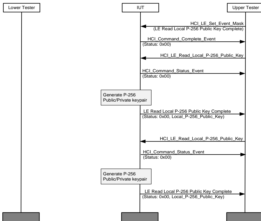
Figure 4.75: HCI/AEN/BV-06-C [Public Keys] MSC
