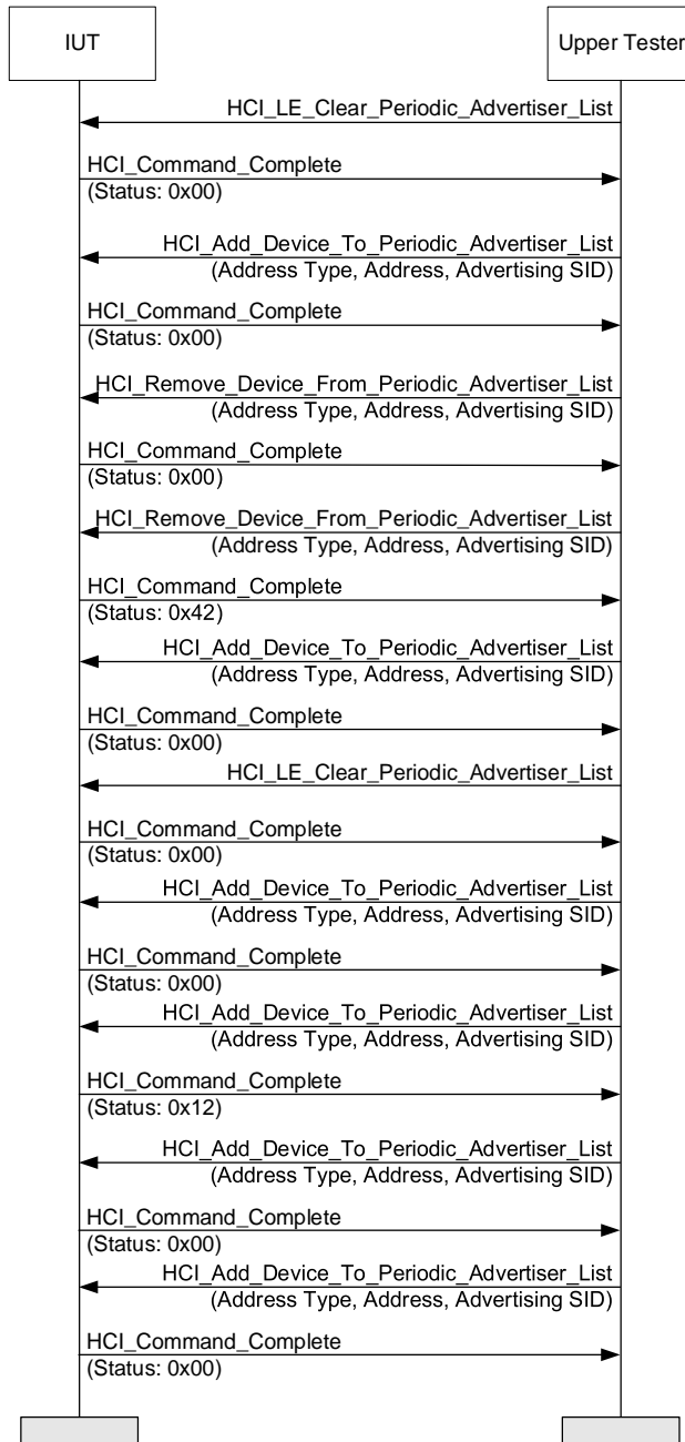
Figure 4.91: HCI/CCO/BV-17-C [LE Add/Remove/Clear Periodic Advertiser List Commands] MSC
