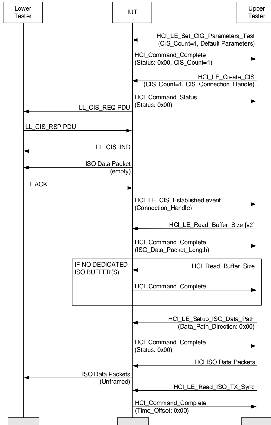
Figure 4.151: HCI/CIS/BV-06-C [Connected Isochronous Stream Using Test Command, Central Initiated, Time_Offset] MSC
