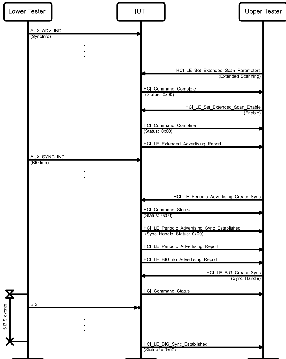
Figure 4.161: HCI/BIS/BI-16-C [Reporting Failure to Sync to BIS] MSC
