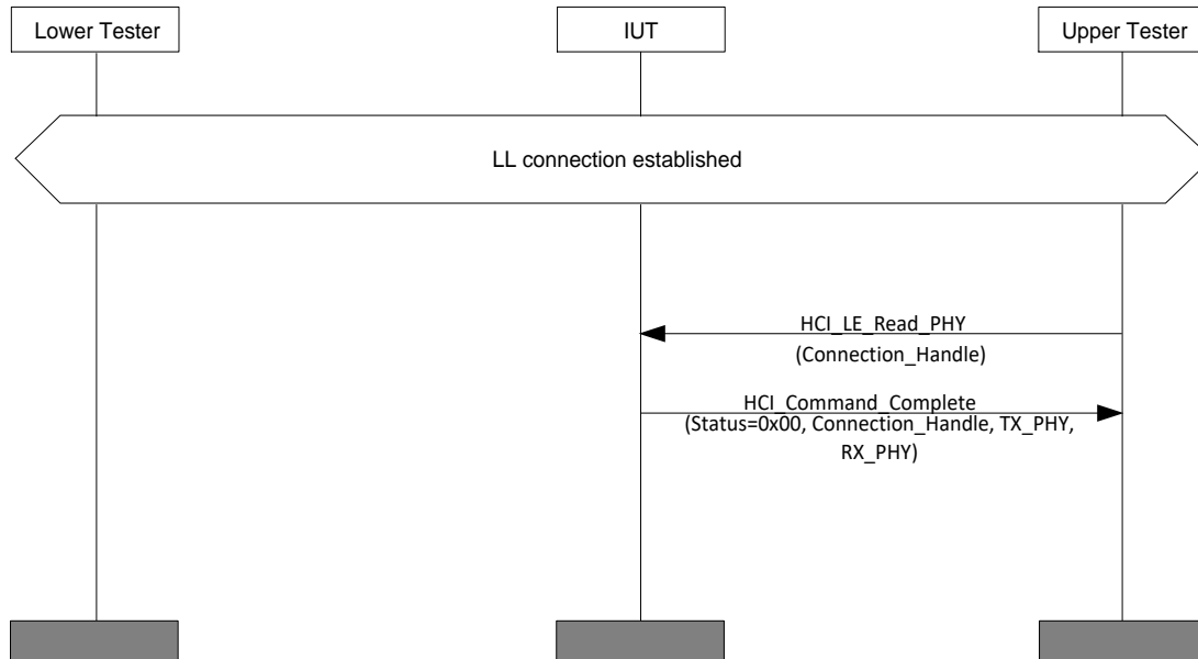
Figure 4.132: HCI/CM/BV-03-C [LE Read PHY Command] MSC
