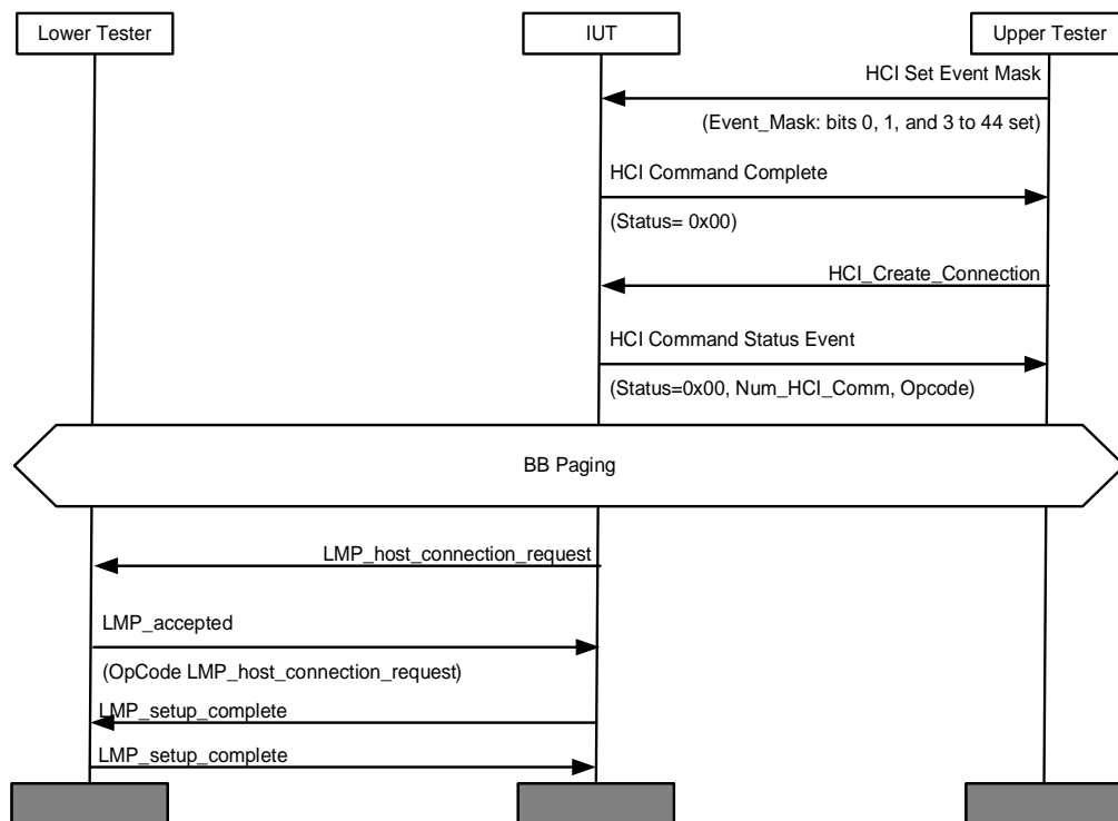
Figure 4.53: HCI/HFC/BV-01-C [Set_Event_Mask Command] MSC
