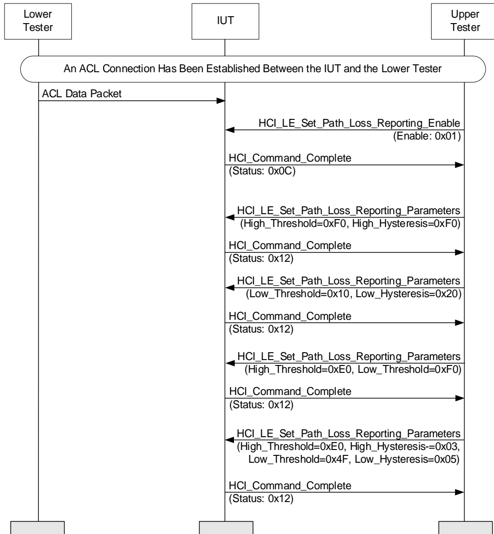
Figure 4.99: HCI/CCO/BI-13-C [Invalid Path Loss Monitoring Parameters] MSC
