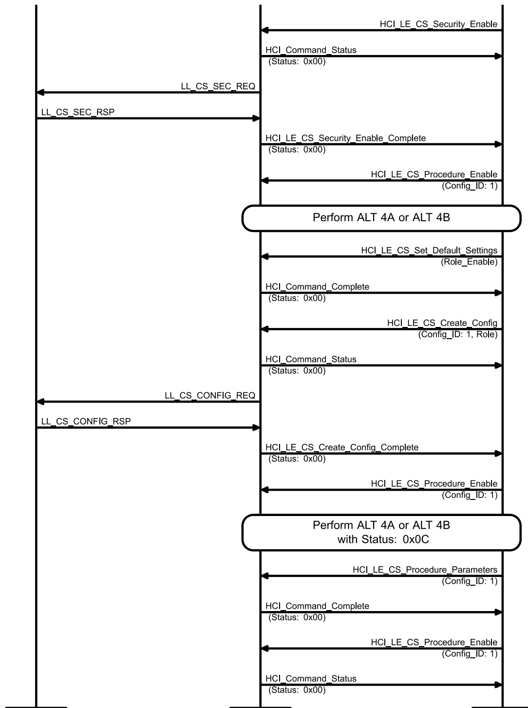
Figure 4.115: Reject CS Start Procedure when IUT Configuration has not completed MSC – Page 2 of 2
