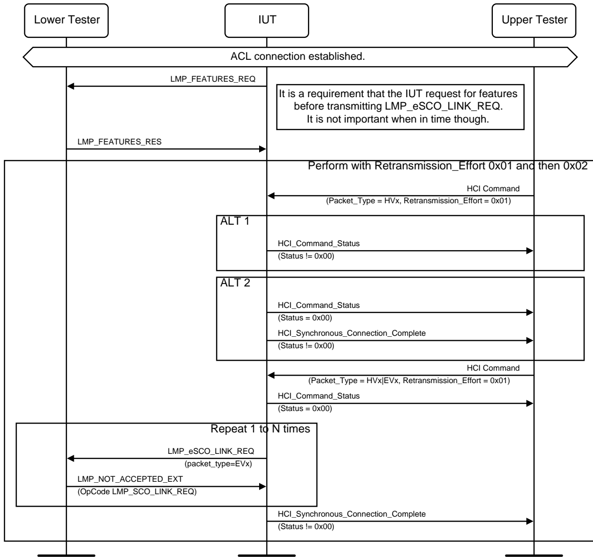
Figure 4.171: Do Not Establish a SCO Connection When Retransmission is Specified MSC
