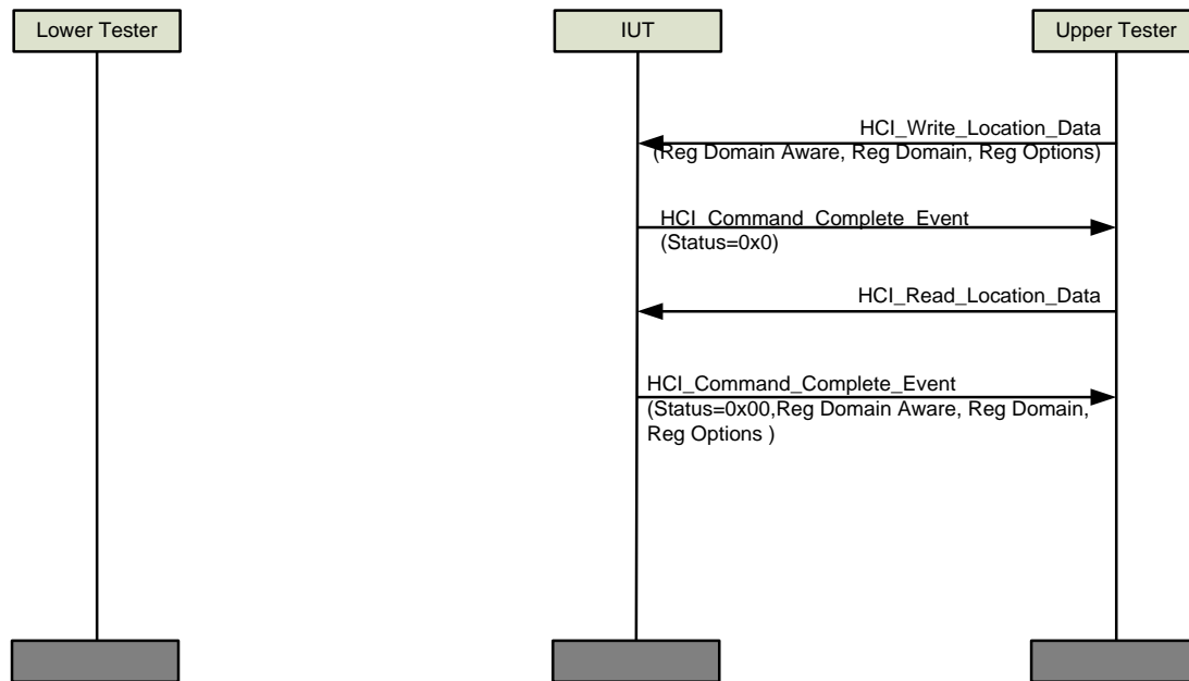
Figure 4.79: HCI/CCO/BV-01-C [Write Location Data Command/ Read Location Data Command] MSC
