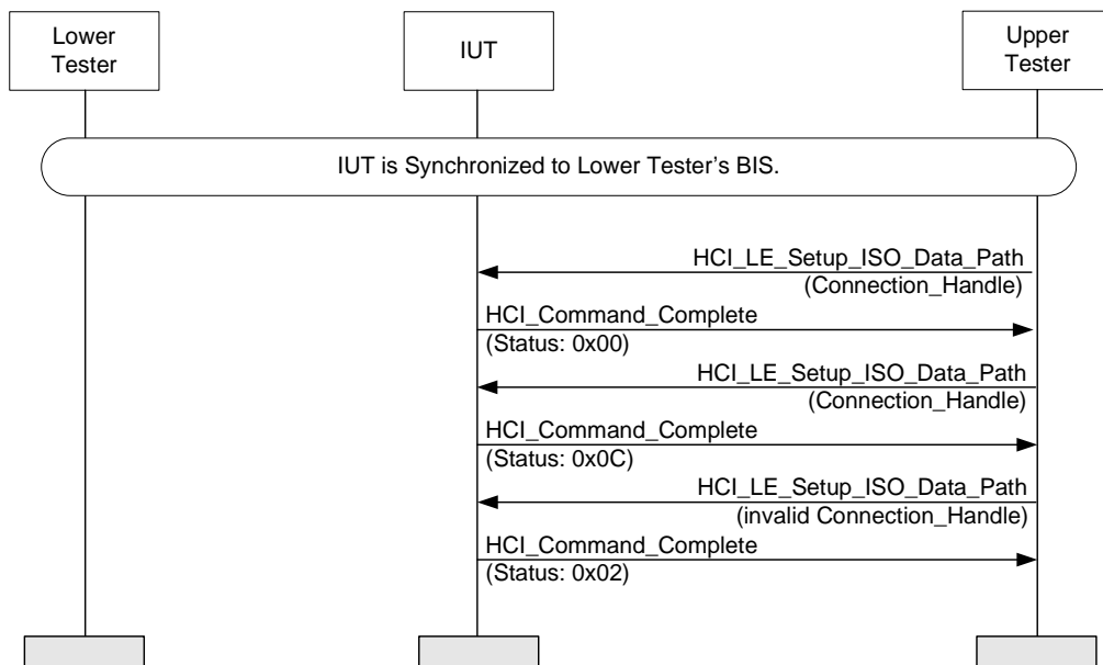
Figure 4.166: HCI/BIS/BI-02-C [Broadcast Isochronous Stream, Synchronized Receiver, Reject Invalid Commands] MSC
