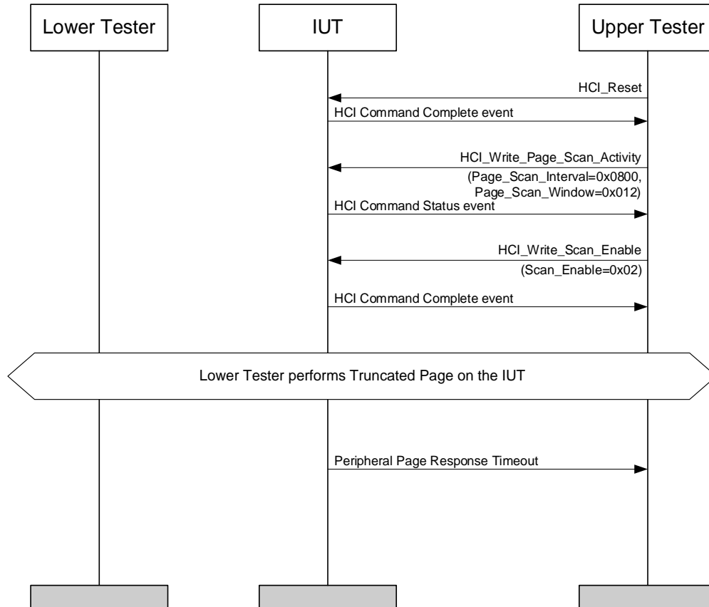
Figure 4.122: HCI/CSE/BV-07-C [Page Response Timeout Detection] MSC
