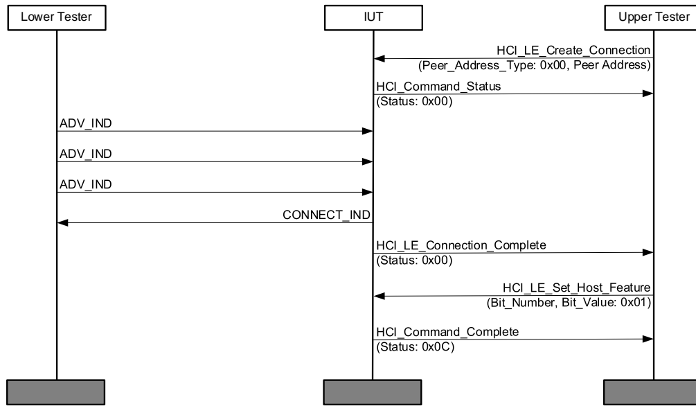
Figure 4.123: HCI/CSE/BV-08-C [LE Set Host Feature Command During Connection, Initiator] MSC
