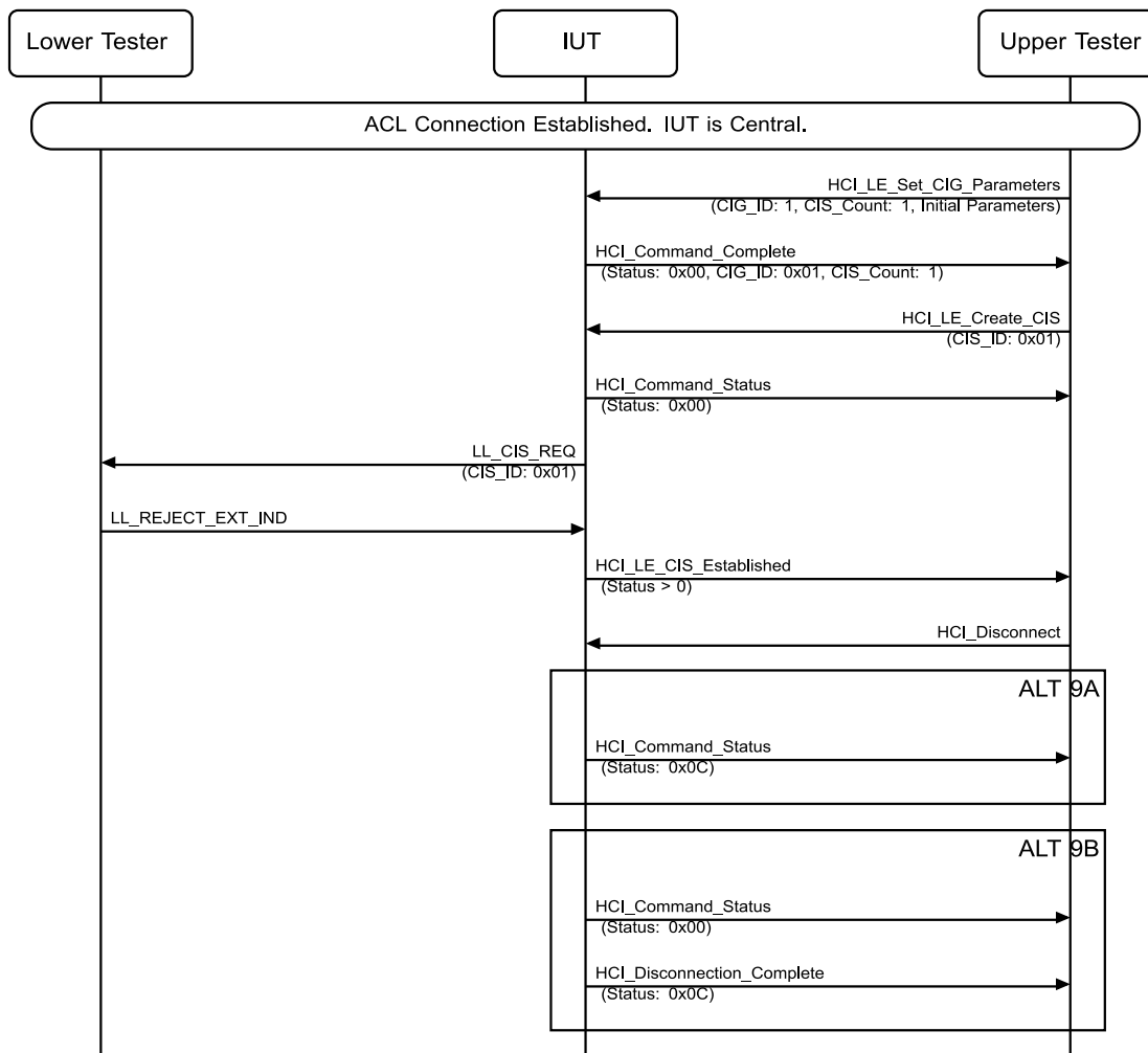
Figure 4.159: HCI/CIS/BI-16-C [Disconnecting Immediately After a Failed Create CIS Attempt] MSC
