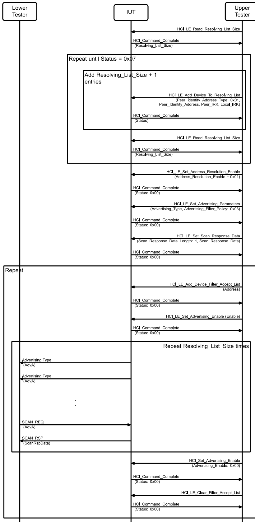
Figure 4.108: LE Add Device To Resolving List – No Space Available, Advertiser MSC
