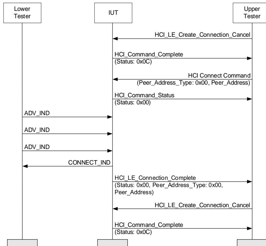
Figure 4.138: LE Create Connection Cancel, Command Disallowed MSC
