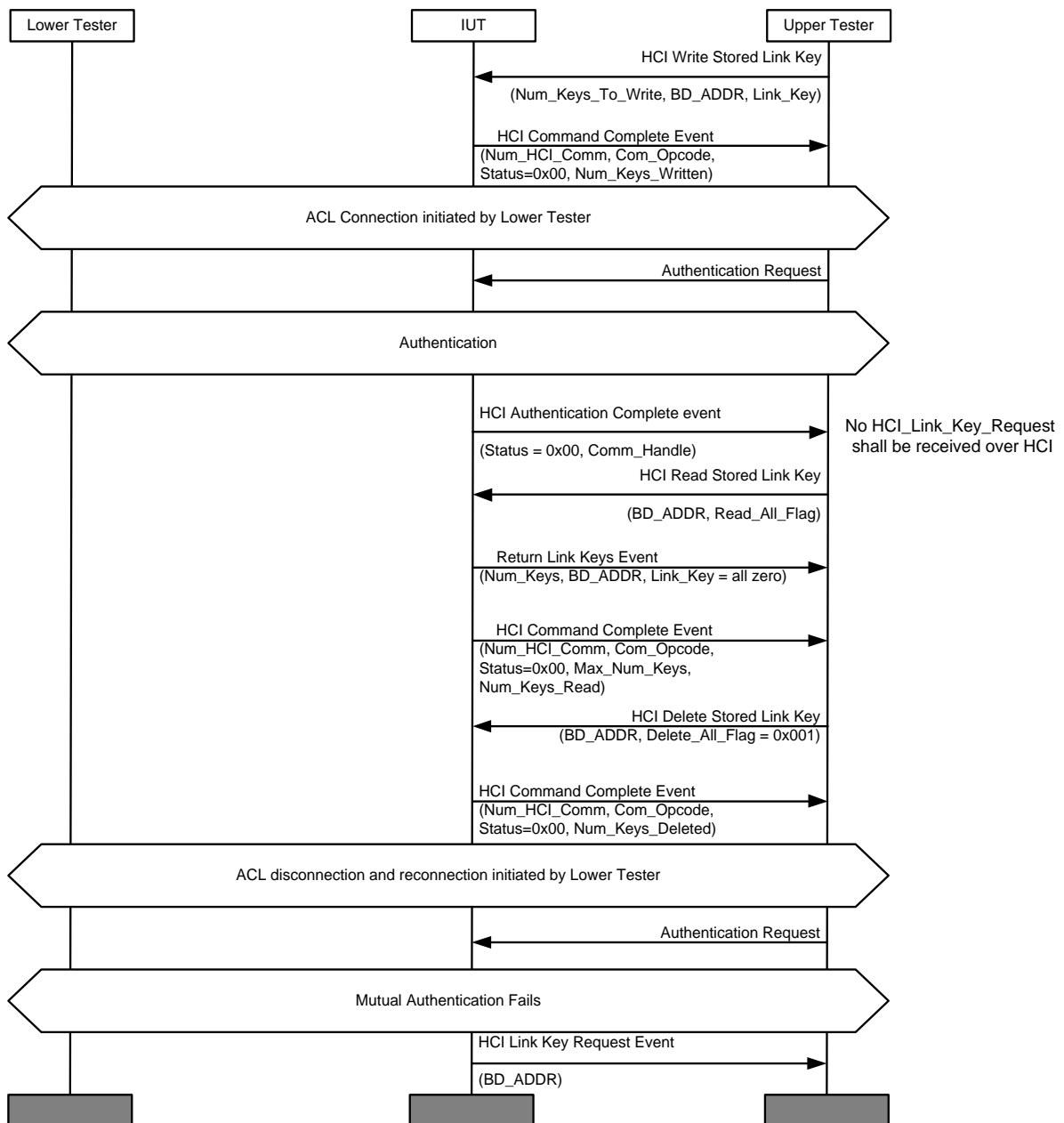
Figure 4.73: HCI/AEN/BV-04-C [Link Key Commands – IUT Returns All Zero Link Key] MSC
