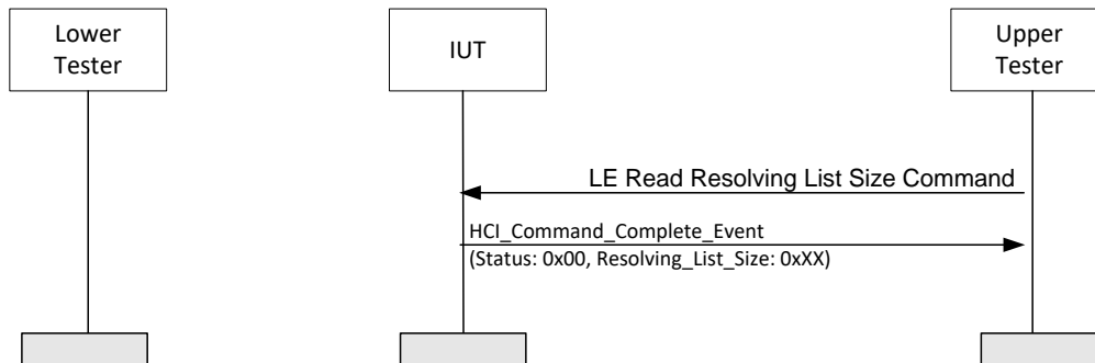
Figure 4.88: HCI/CCO/BV-14-C [LE Read Resolving List Size Command] MSC
