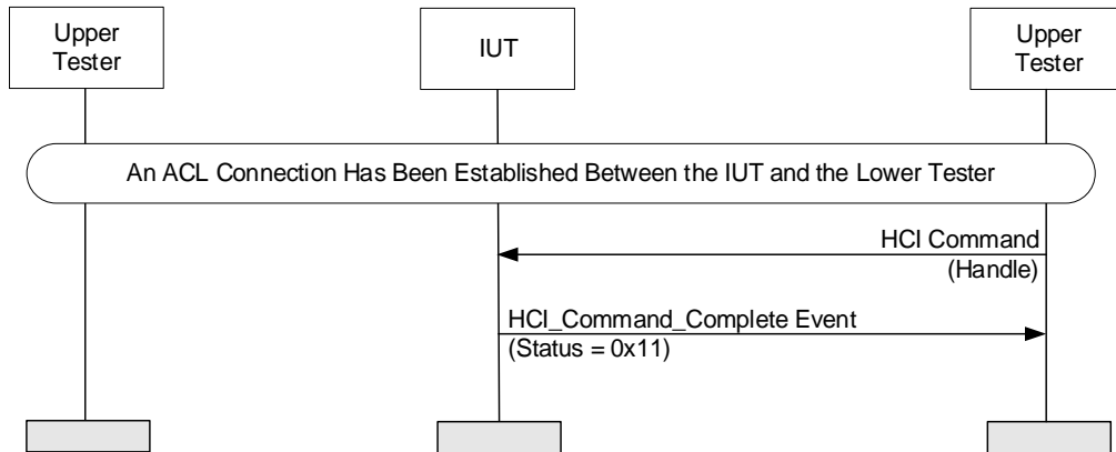
Figure 4.101: Error Response for Unsupported Commands on Transports MSC
