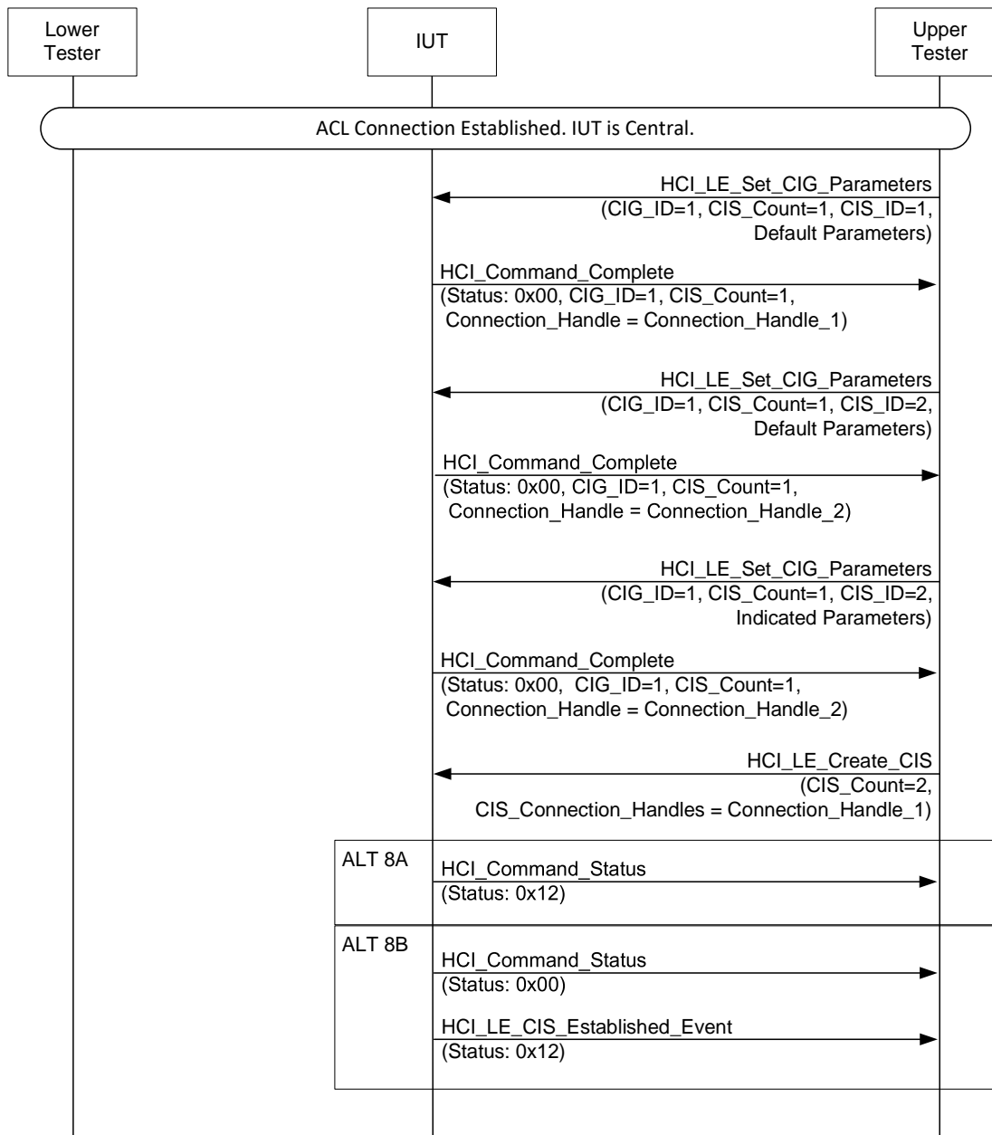
Figure 4.148: HCI/CIS/BV-05-C [Connected Isochronous Stream, Central Initiated, Add or Modify CIS] MSC – Page 1 of 2
