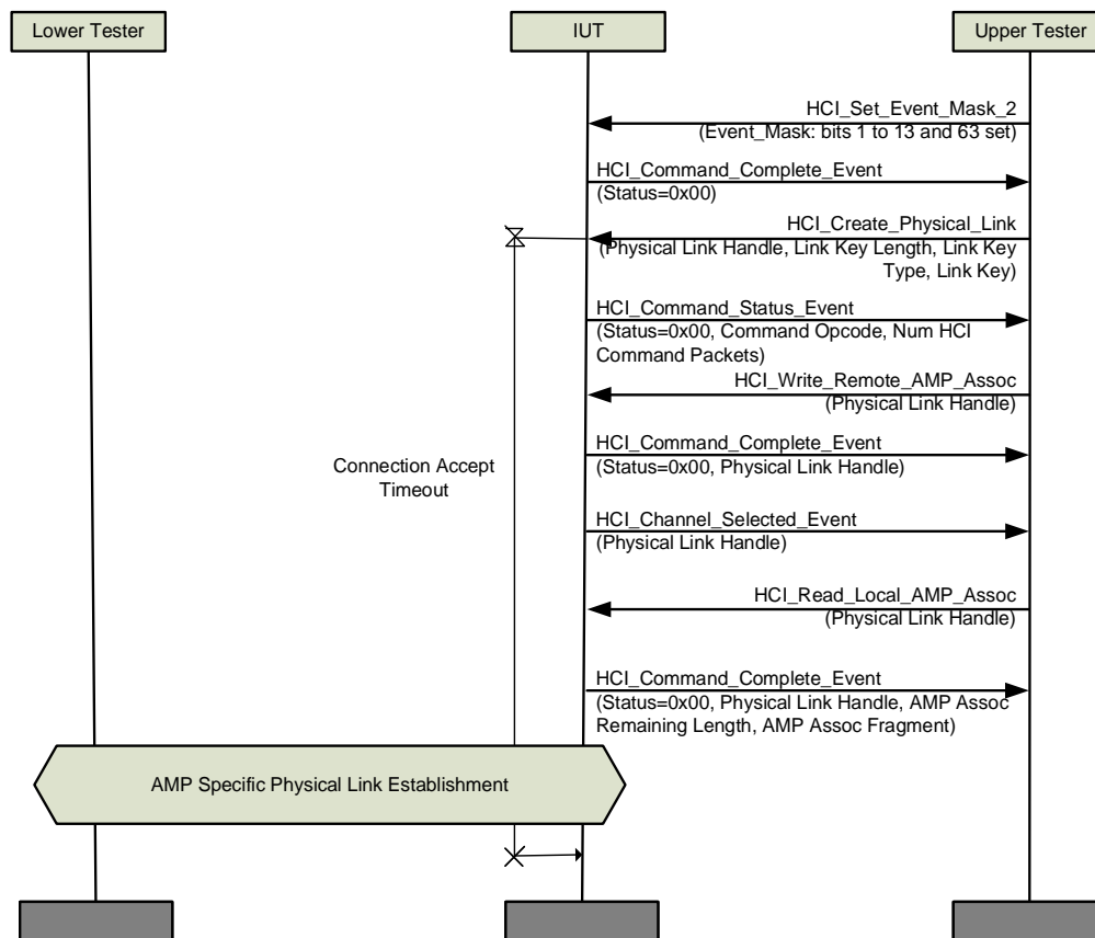
Figure 4.55: HCI/HFC/BV-03-C [Set_Event_Mask_2 Command] MSC
