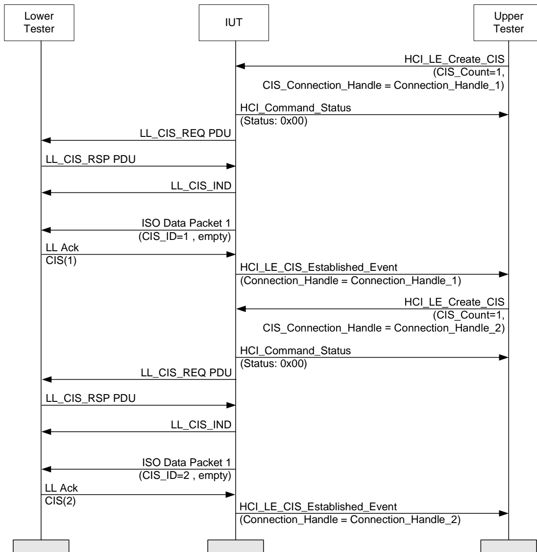
Figure 4.149: HCI/CIS/BV-05-C [Connected Isochronous Stream, Central Initiated, Add or Modify CIS] MSC – Page 2 of 2
