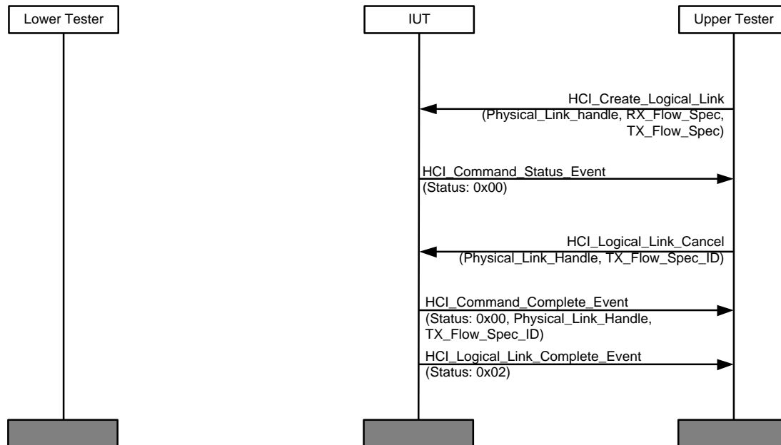
Figure 4.116: HCI/CSE/BV-01-C [Logical Link Cancel Command] MSC
