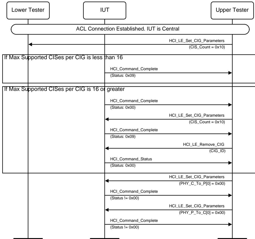
Figure 4.141: Connected Isochronous Stream Using Non-Test Command, Central Initiated MSC – Page 1 of 4
