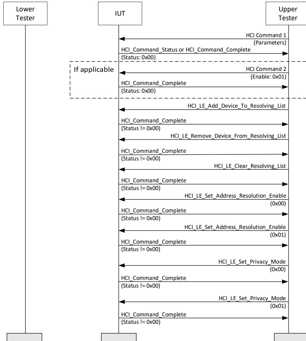
Figure 4.97: Resolving List Commands fail when list in use MSC
