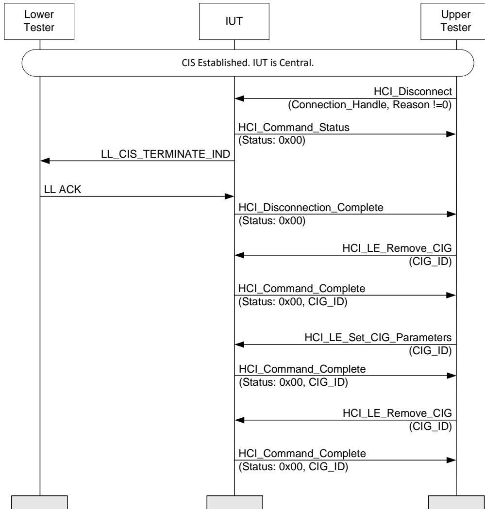
Figure 4.157: HCI/CIS/BV-13-C [Connected Isochronous Stream, Central, Removal of Configurable and Inactive CIG] MSC
