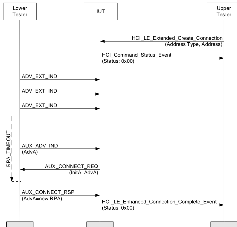
Figure 4.133: HCI/CM/BV-04-C [Extended Scanning with Device Privacy, RPA Timeout During Connection Initiation] MSC
