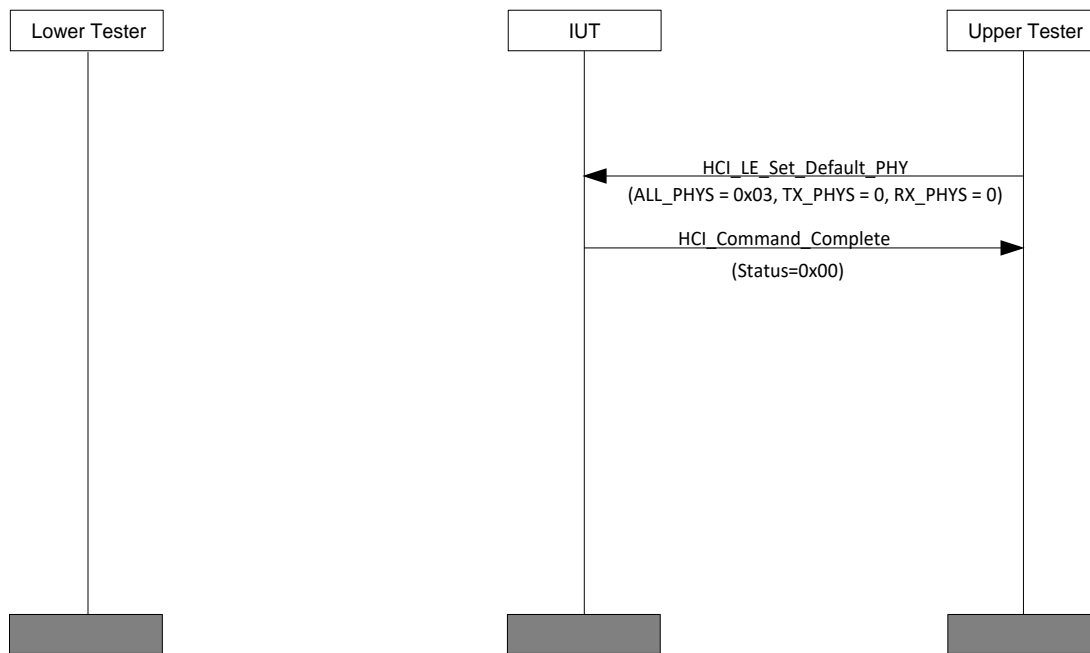
Figure 4.89: HCI/CCO/BV-15-C [LE Set Default PHY Command] MSC
