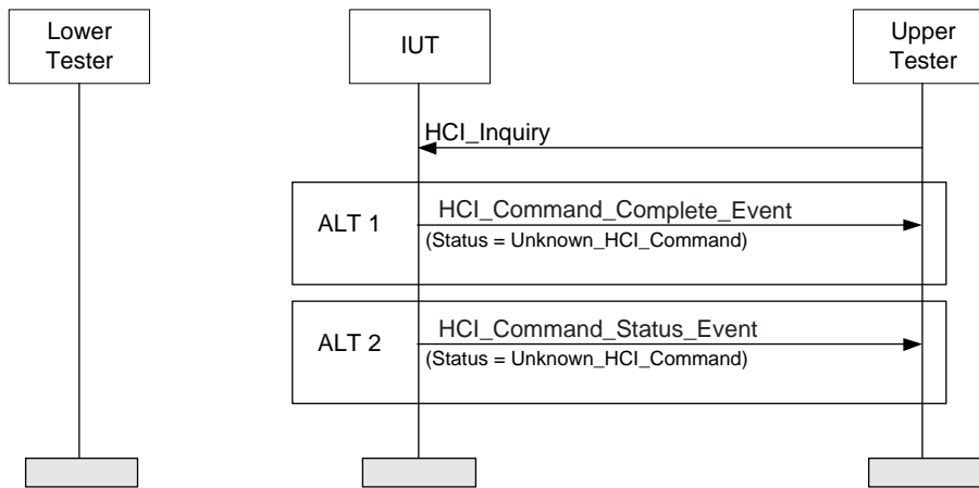
Figure 4.82: HCI/CCO/BV-07-C [BR/EDR Not Supported] MSC
