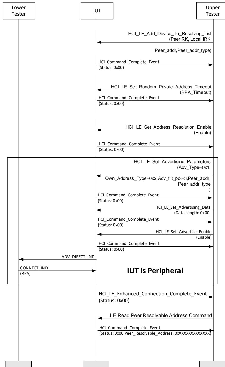
Figure 4.134: HCI/CM/BV-05-C [LE Read Peer Resolvable Address Command – Peripheral] MSC
