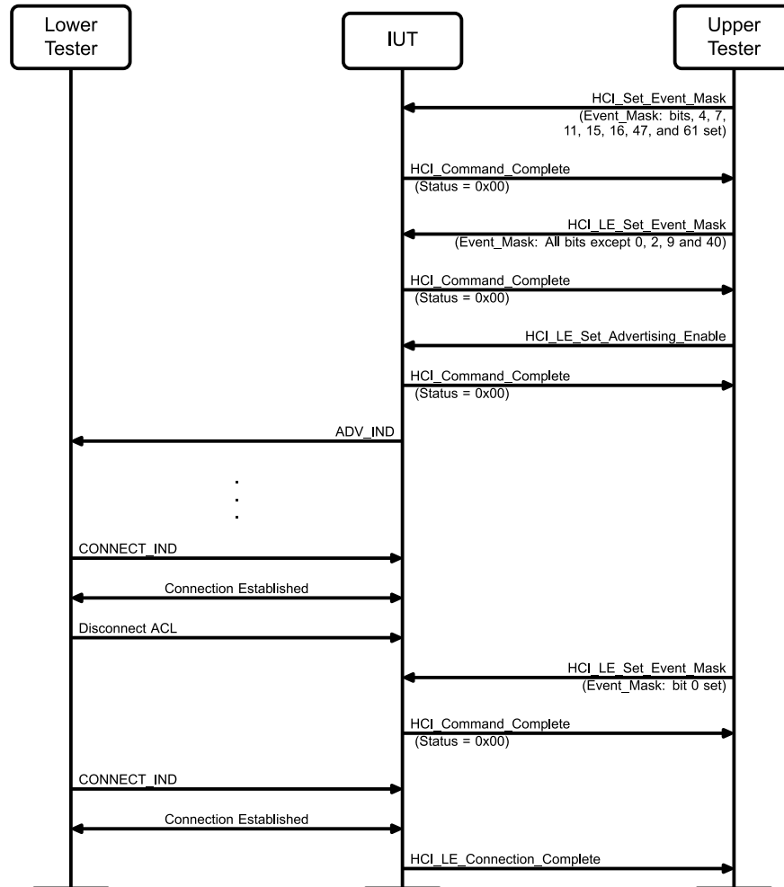
Figure 4.58: HCI/HFC/BV-15-C [LE Set Event Mask – Advertising state and connections supported] MSC
