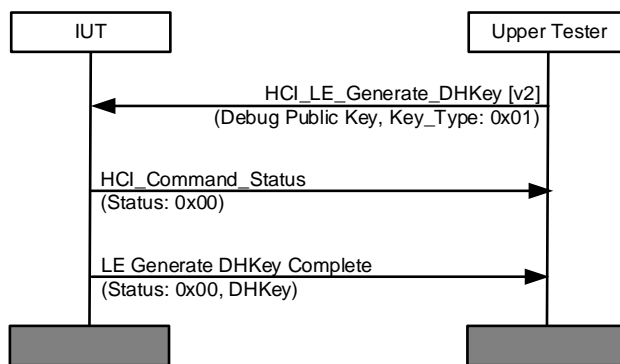
Figure 4.77: HCI/AEN/BV-08-C [Generate Debug Keys] MSC
