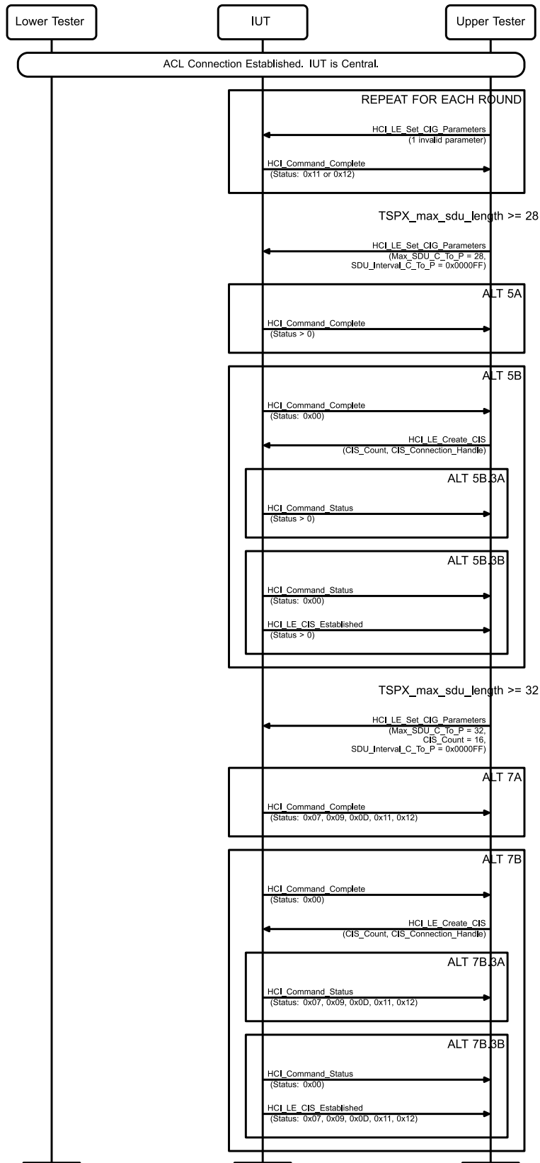
Figure 4.150: HCI/CIS/BI-05-C [Connected Isochronous Stream Using Non-Test Command, Central, Reject Invalid Parameters] MSC
