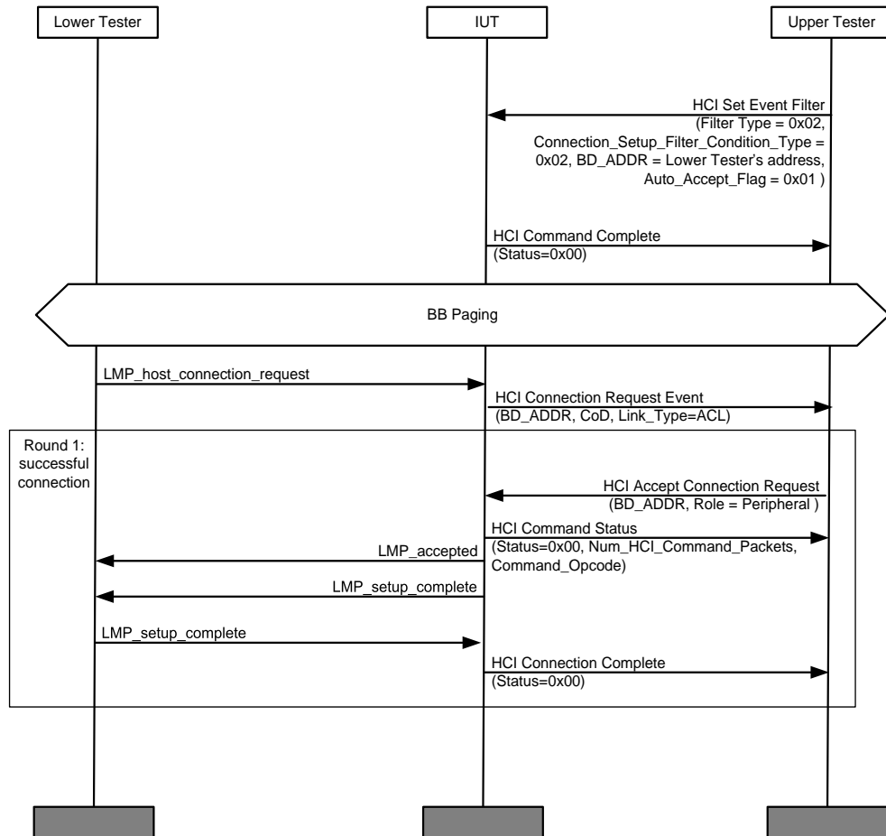
Figure 4.65: HCI/HFC/BV-08-C [Set_Event_Filter Command to controls which events are generated using filters] MSC – Page 1 of 2
