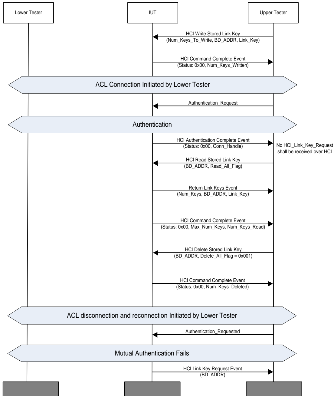
Figure 4.70: HCI/AEN/BV-01-C [Link Key Commands] MSC
