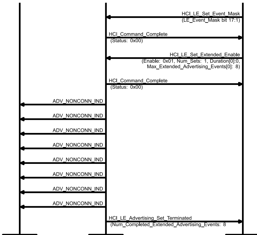
Figure 4.61: HCI/HFC/BV-19-C [LE Set Event Mask – Advertising Set Terminated] MSC – Page 2 of 2
