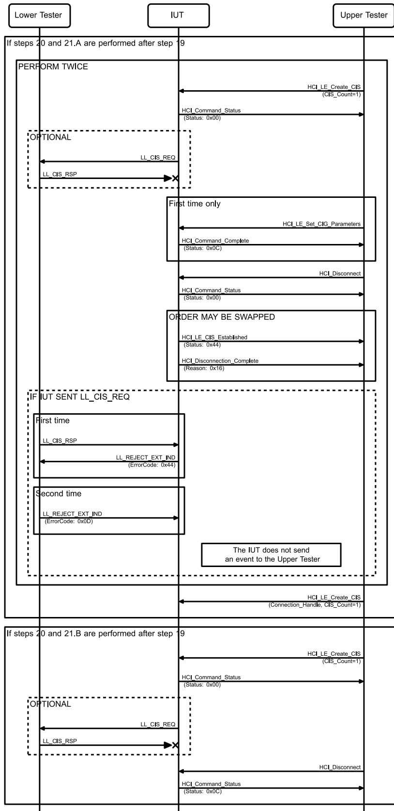
Figure 4.143: Connected Isochronous Stream Using Non-Test Command, Central Initiated MSC – Page 3 of 4
