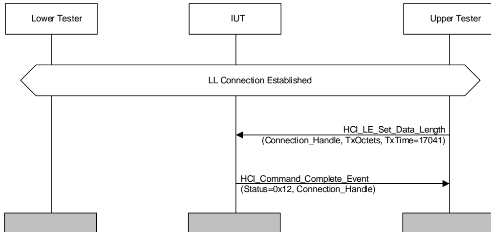
Figure 4.103: HCI/CCO/BI-40-C [LE Set Data Length, Invalid Parameters] MSC
