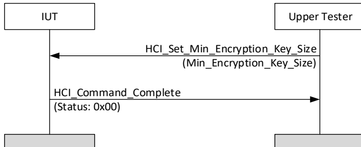
Figure 4.95: HCI/CCO/BV-21-C [Set Minimum Encryption Key Size] MSC
