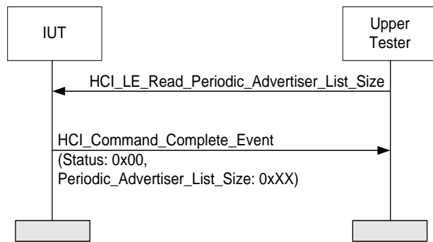
Figure 4.90: HCI/CCO/BV-16-01-C [LE Read Periodic Advertiser List Size Command] MSC
