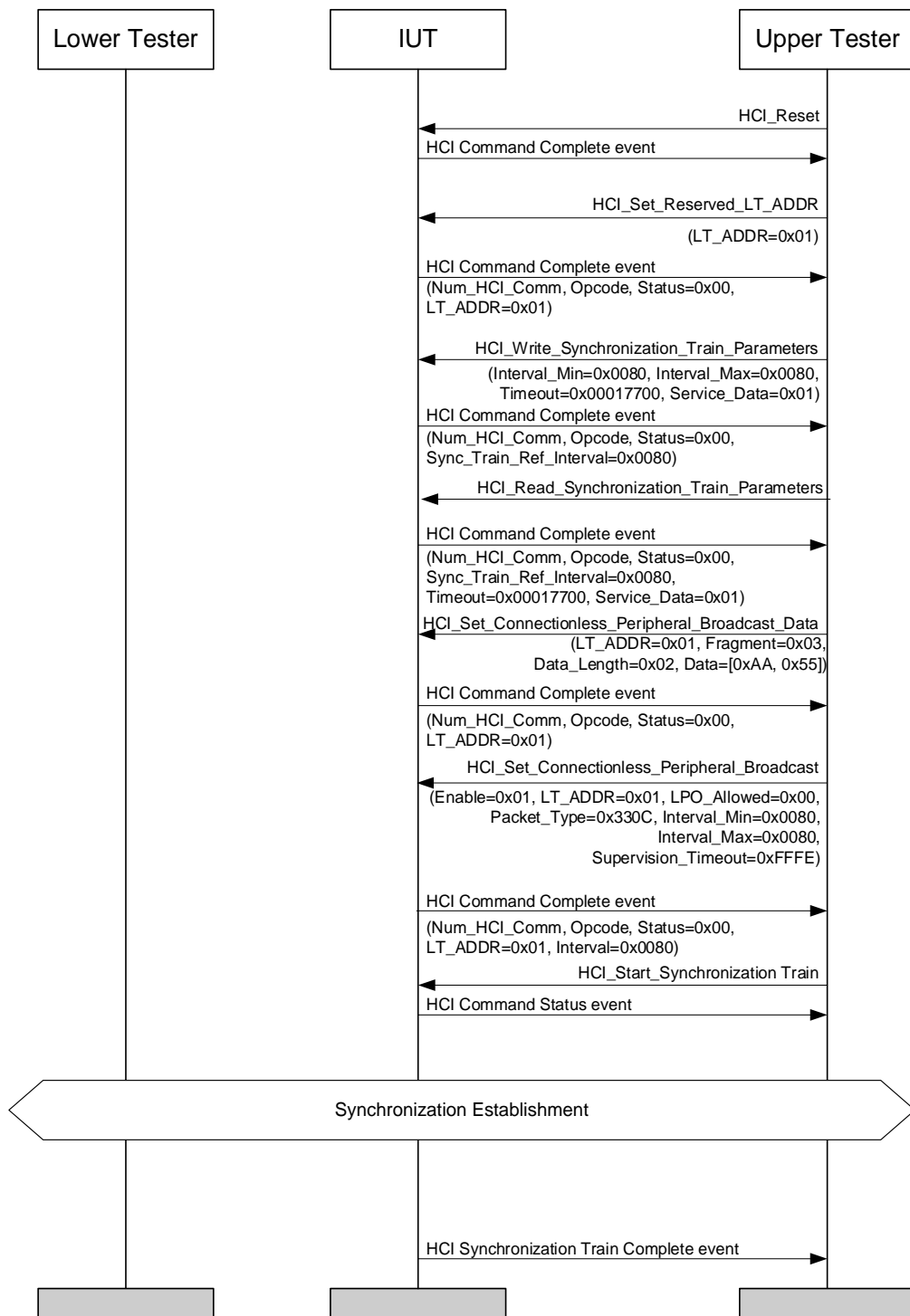
Figure 4.125: HCI/CPB/BV-01-C [Connectionless Peripheral Broadcast Transmission] MSC
