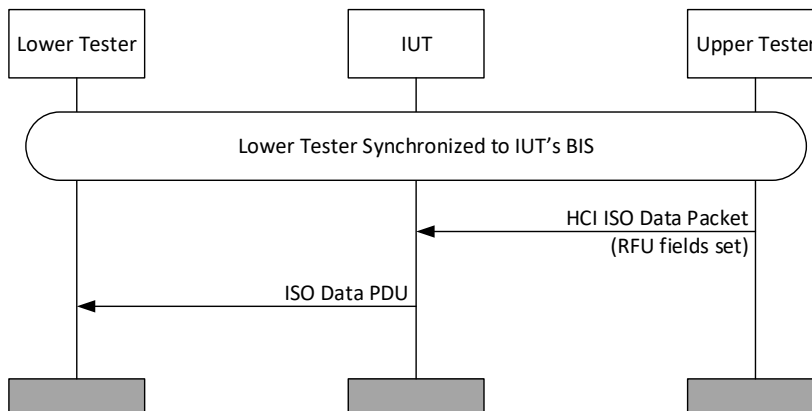
Figure 4.164: HCI/BIS/BI-01-C [Ignoring RFU Bits in HCI ISO Data Packets, BIS] MSC
