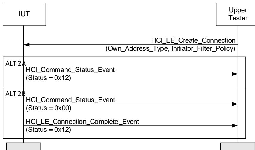
Figure 4.109: Reject Invalid Create Connection Command MSC
