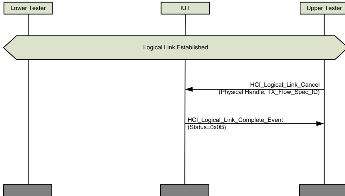
Figure 4.118: HCI/CSE/BI-03-C [Logical Link Cancel Command] MSC
