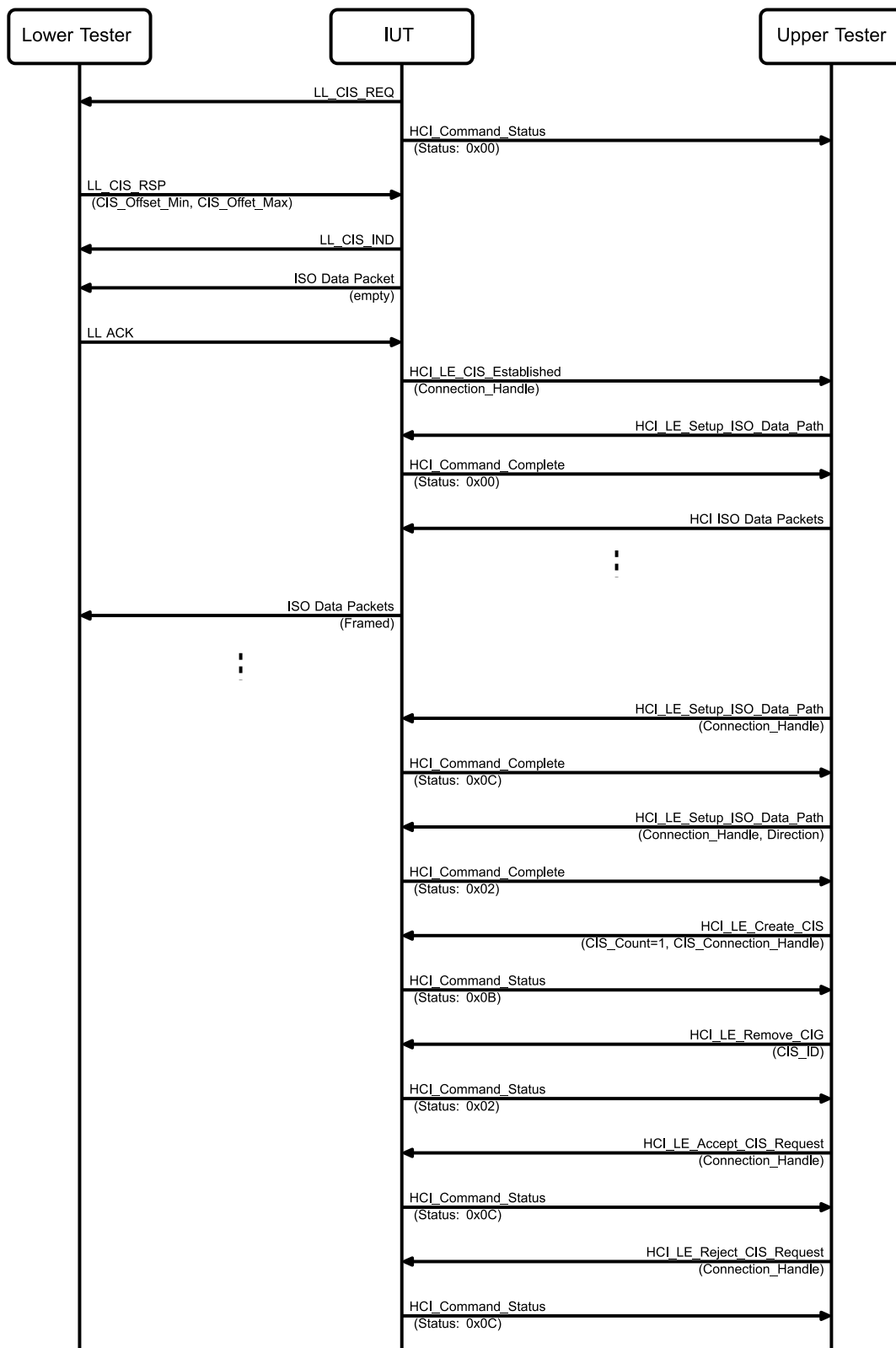
Figure 4.144: Connected Isochronous Stream Using Non-Test Command, Central Initiated MSC – Page 4 of 4
