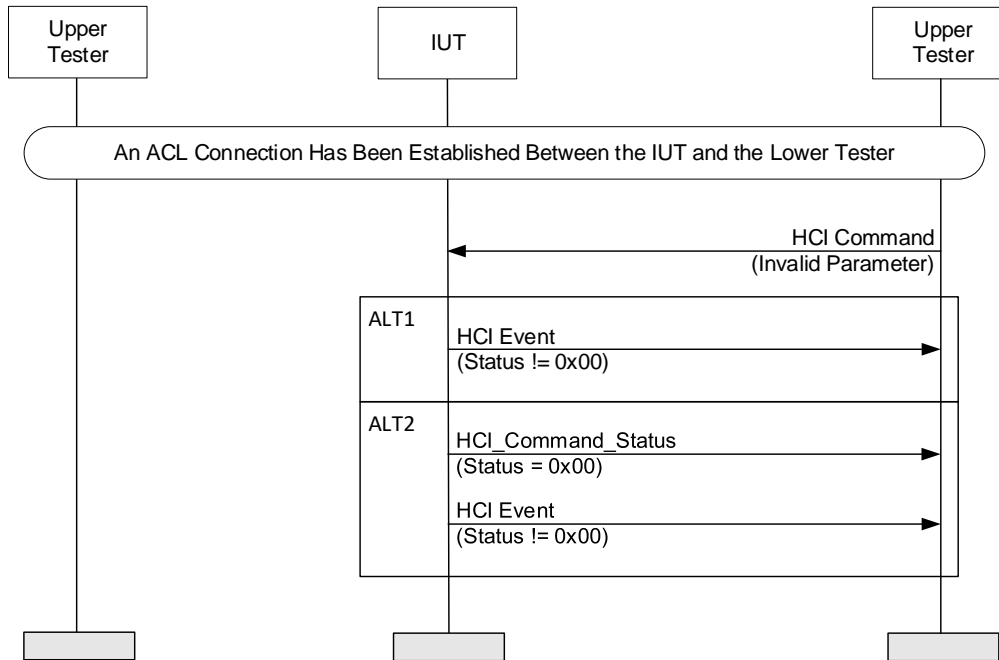
Figure 4.98: Invalid LE Power Control HCI Parameters MSC
