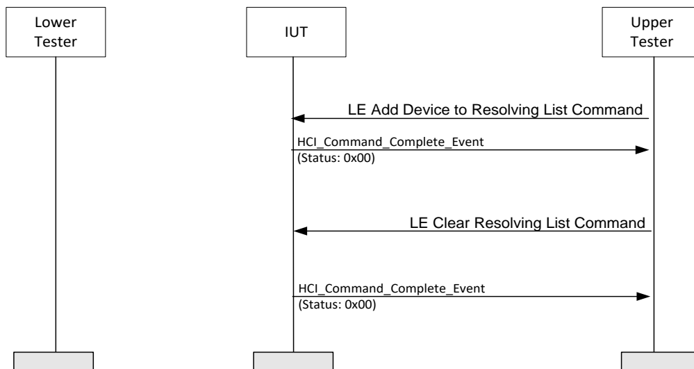
Figure 4.87: HCI/CCO/BV-13-C [LE Clear Resolving List Command] MSC
