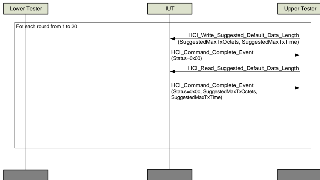
Figure 4.85: HCI/CCO/BV-11-C [LE Write Suggested Default Data Length Command] MSC
