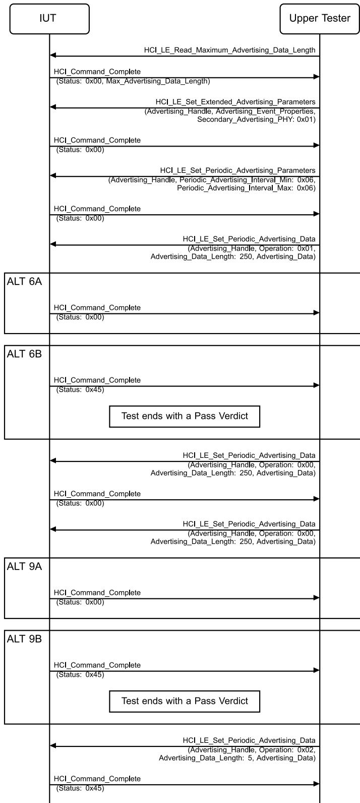
Figure 4.46: HCI/DDI/B1-52-C [Reject Set Periodic Advertising Data Command when Advertising Data Too Long] MSC
