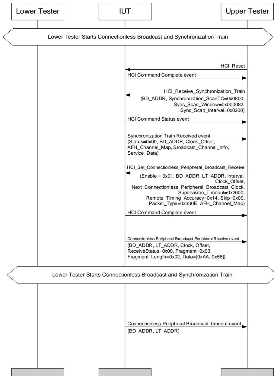
Figure 4.129: HCI/CPB/BV-05-C [Connectionless Peripheral Broadcast Reception Timeout] MSC
