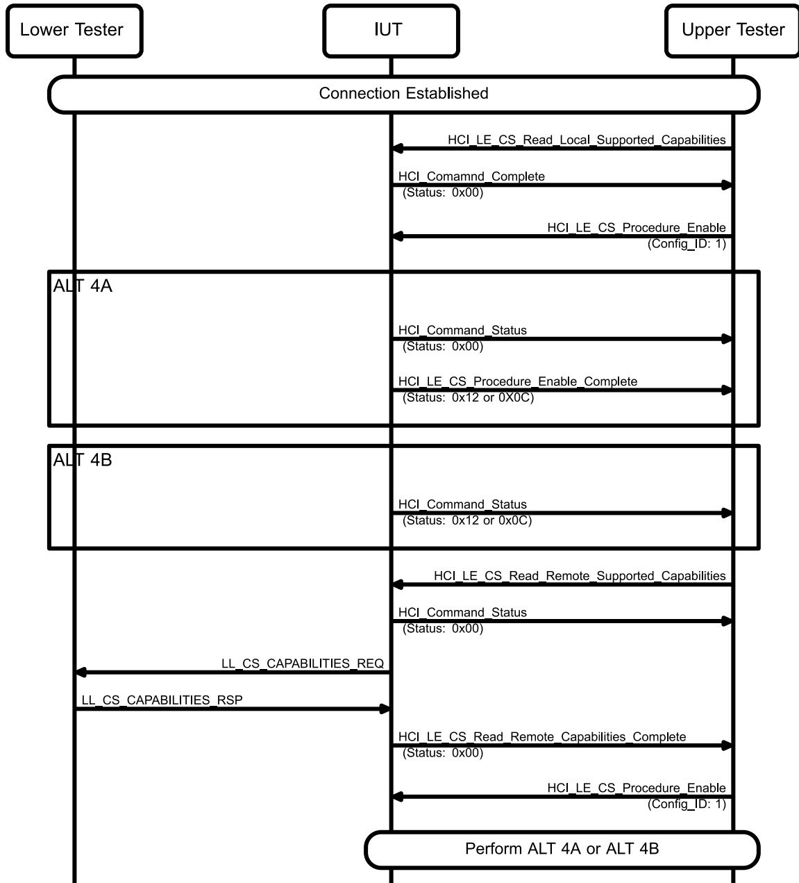
Figure 4.114: Reject CS Start Procedure when IUT Configuration has not completed MSC – Page 1 of 2
