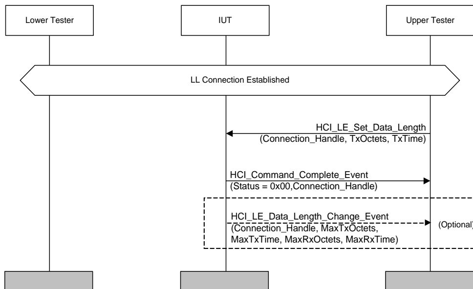
Figure 4.83: HCI/CCO/BV-09-C [LE Set Data Length] MSC
