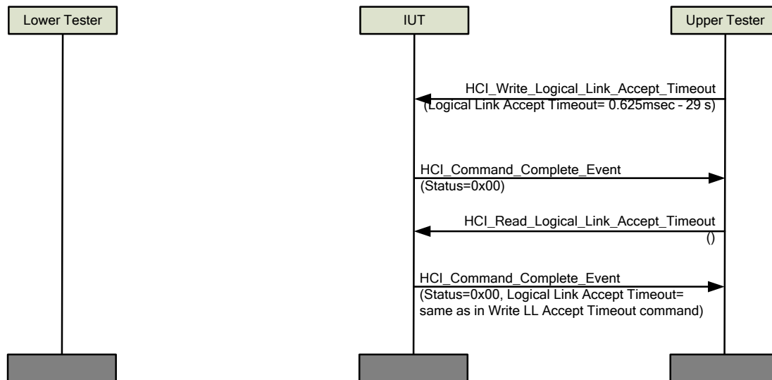
Figure 4.120: HCI/CSE/BV-05-C [Write Logical Link Accept Timeout Command/Read Logical Link Accept Timeout Command] MSC
