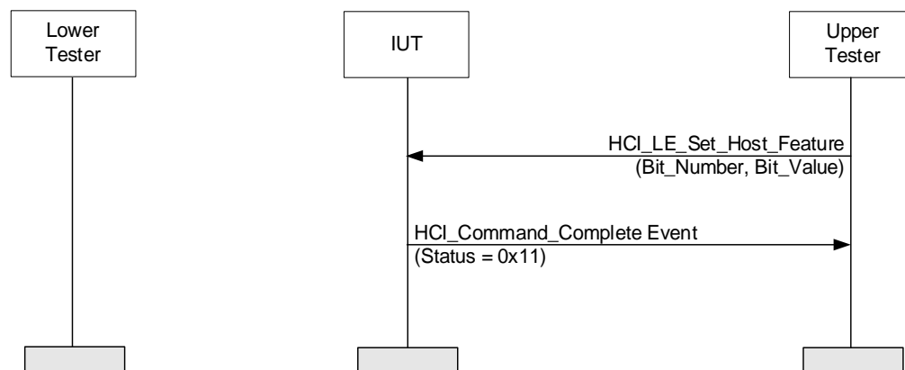
Figure 4.105: Reject Setting Host Controlled FeatureSet Bit, Unsupported Feature on Controller MSC
