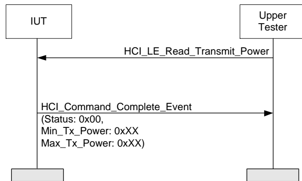
Figure 4.92: HCI/CCO/BV-18-C [LE Read Transmit Power Command] MSC
