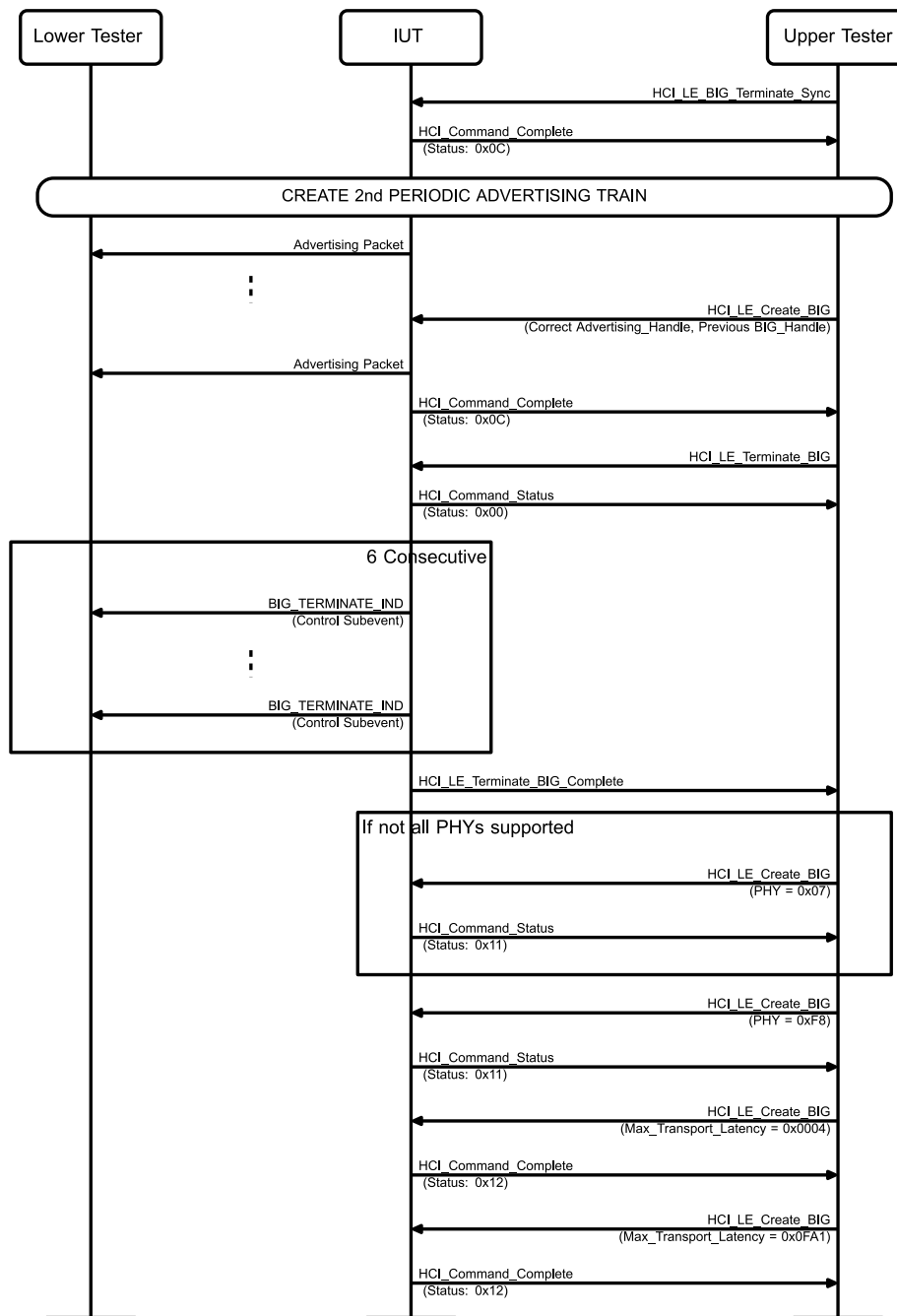
Figure 4.163: Broadcast Isochronous Stream Using Non-Test Command, Isochronous Broadcaster MSC – Page 2 of 2
