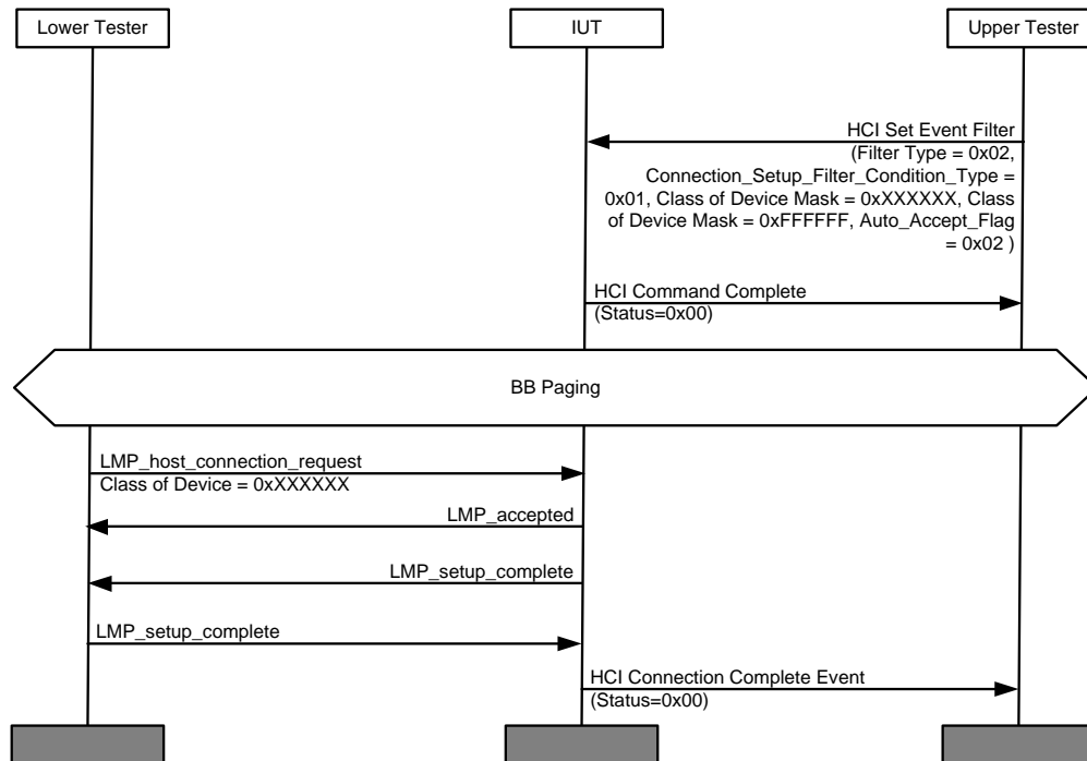
Figure 4.64: HCI/HFC/BV-07-C [Set_Event_Filter Command, Host configures the Controller to Allow Connections, specifying a Class of Device and a Class of Device Mask] MSC
