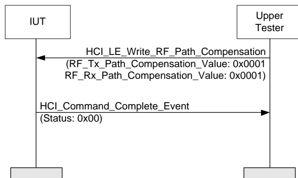
Figure 4.93: HCI/CCO/BV-19-C [LE Write RF Path Compensation Command] MSC
