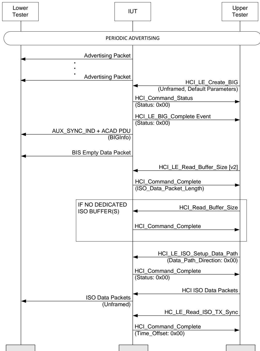
Figure 4.165: HCI/BIS/BV-03-C [Broadcast Isochronous Stream Using Test Command, Time_Offset] MSC
