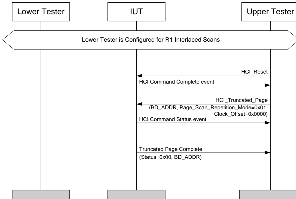
Figure 4.121: HCI/CSE/BV-06-C [Verify Truncated Paging] MSC
