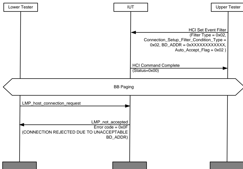
Figure 4.63: HCI/HFC/BV-06-C [Set_Event_Filter Command, connection request rejection] MSC
