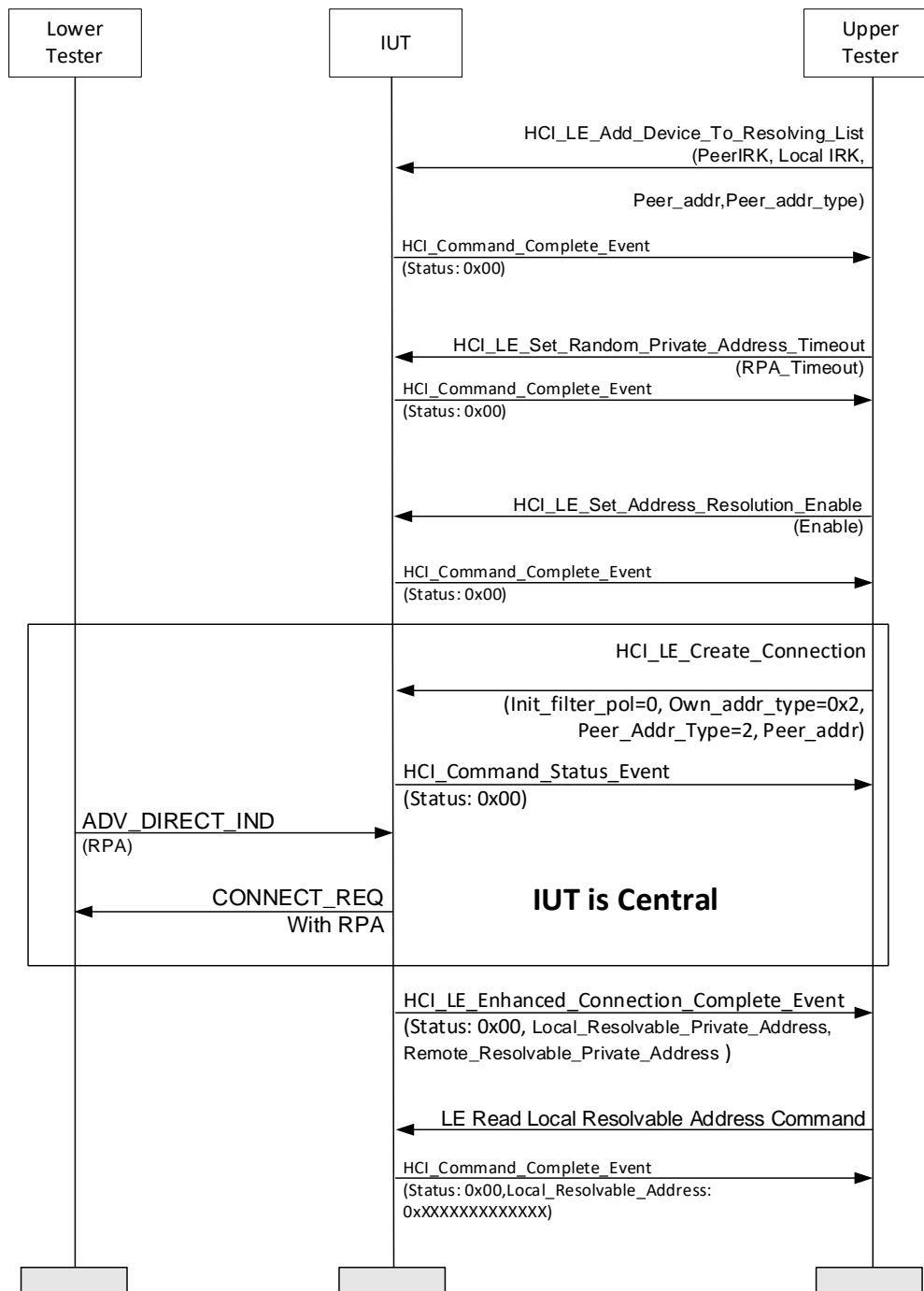
Figure 4.131: HCI/CM/BV-02-C [LE Read Local Resolvable Address Command – Central] MSC
