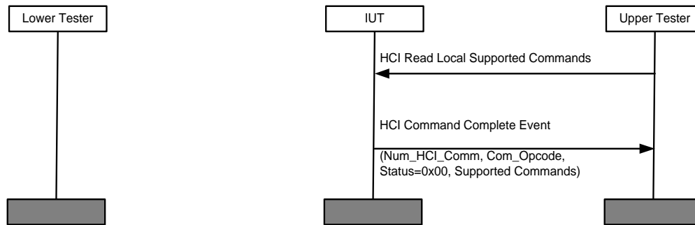
Figure 4.17: HCI/CIN/BV-03-C [Read Local Supported Commands Command] MSC
