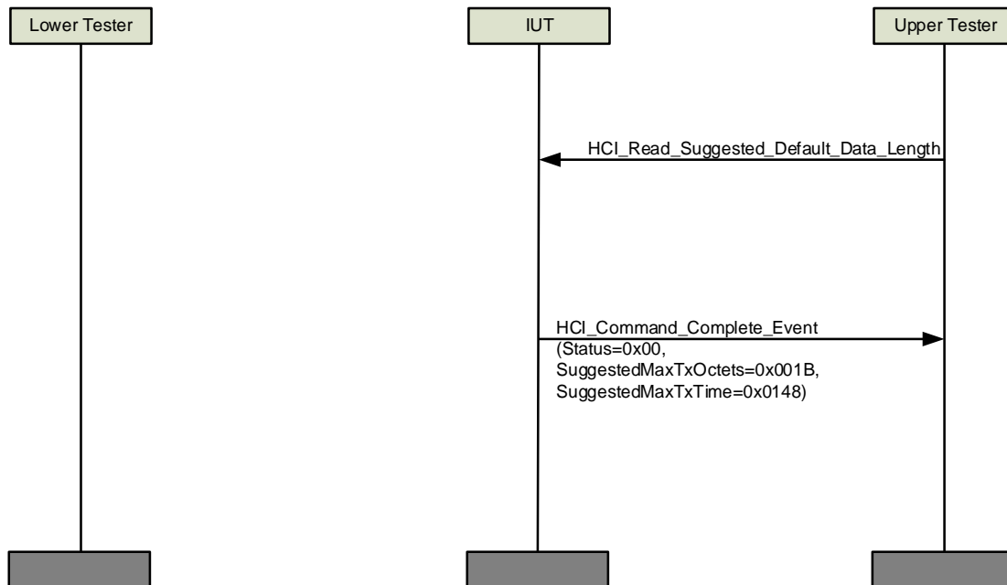
Figure 4.84: HCI/CCO/BV-10-C [LE Read Suggested Default Data Length Command] MSC
