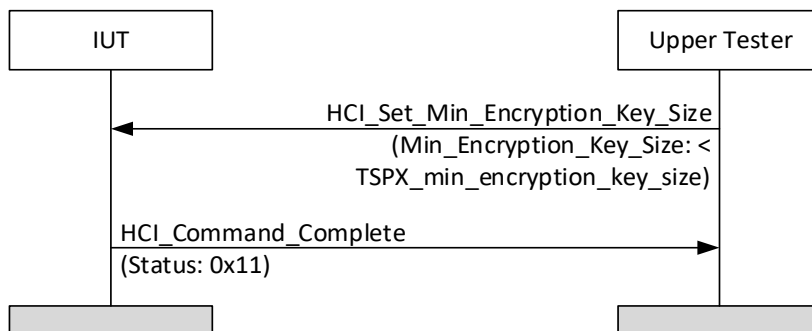
Figure 4.102: HCI/CCO/BI-35-C [Invalid Set Min Encryption Key Size Parameters] MSC
