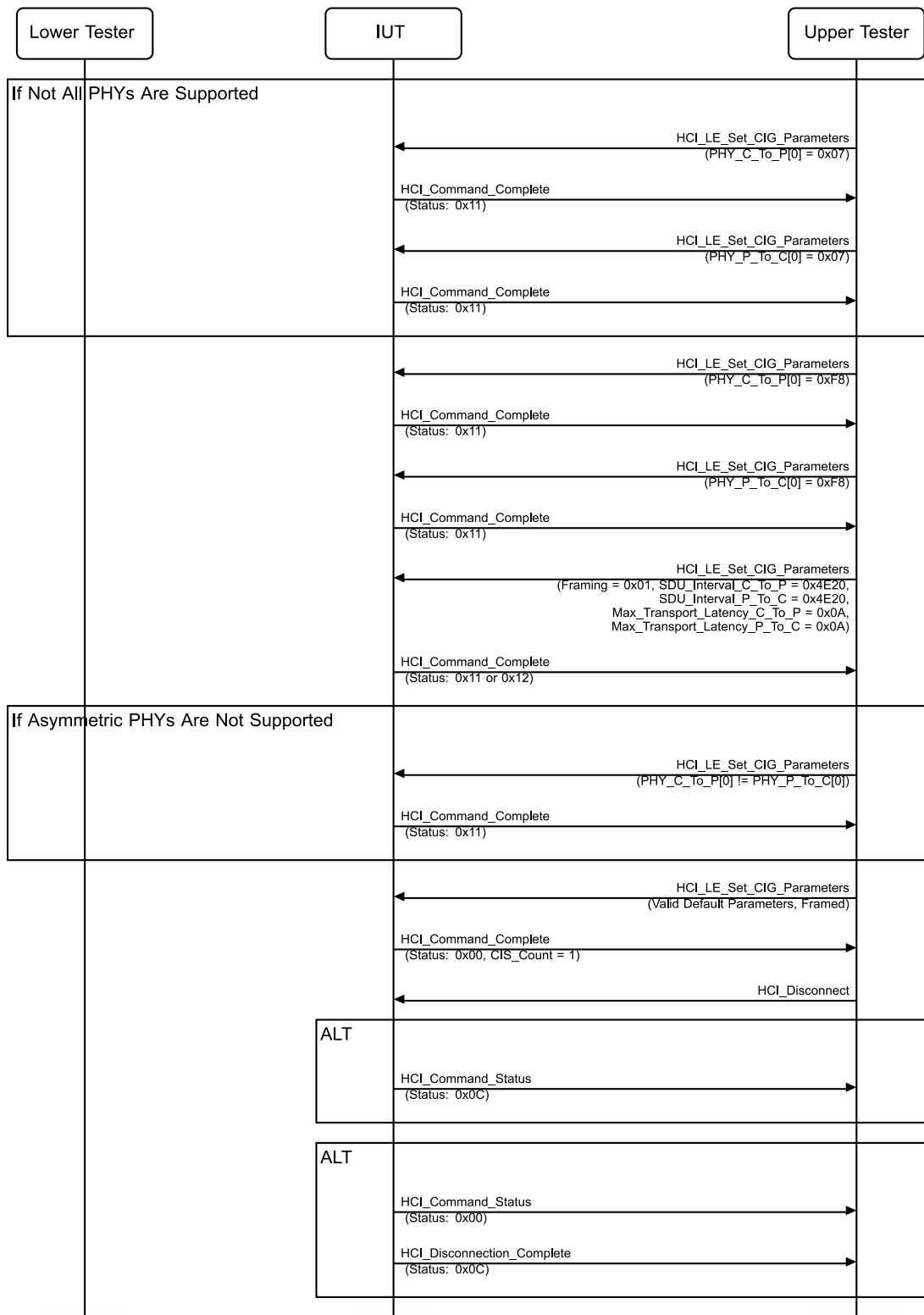
Figure 4.142: Connected Isochronous Stream Using Non-Test Command, Central Initiated MSC – Page 2 of 4
