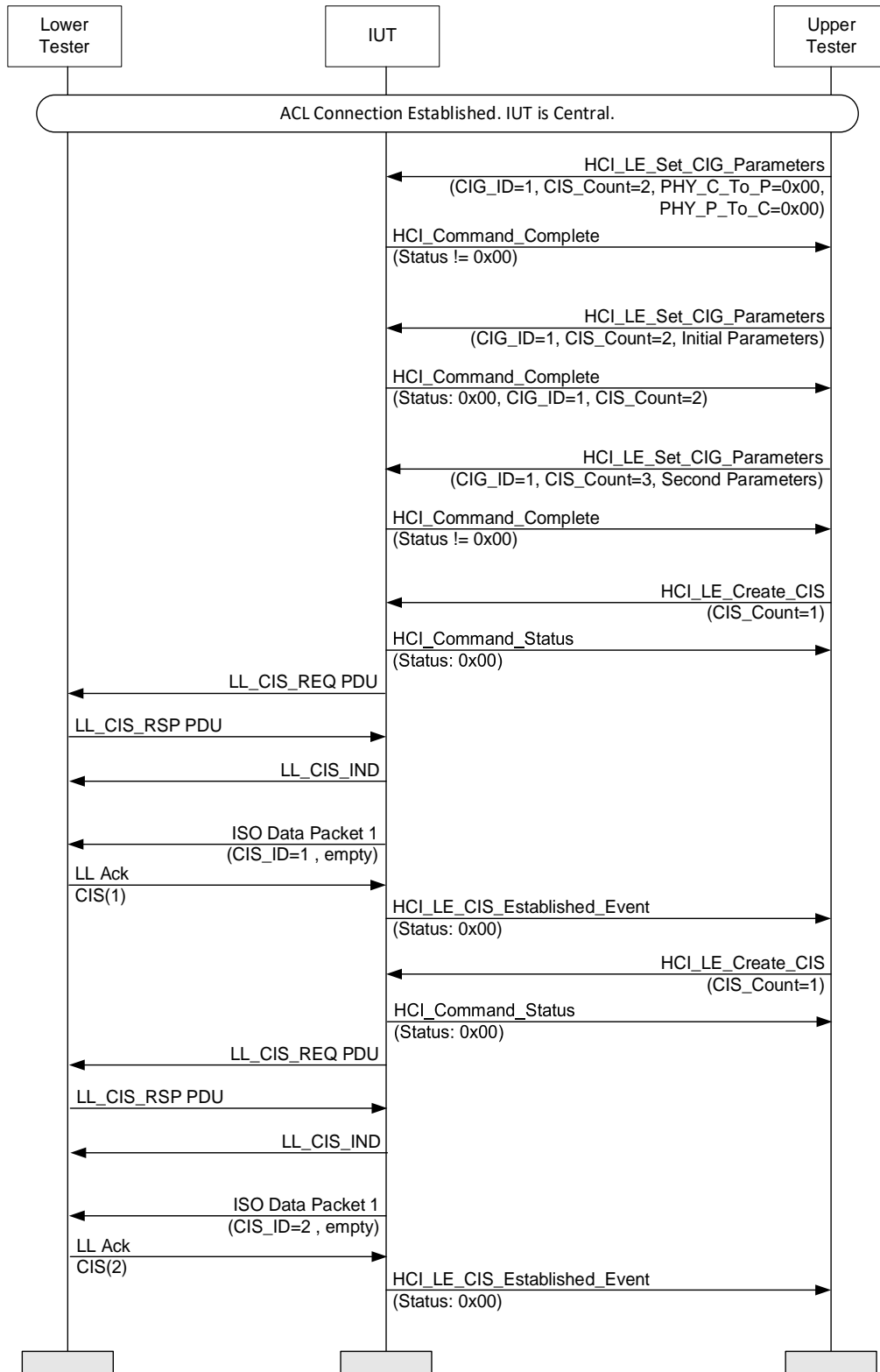
Figure 4.145: HCI/CIS/BI-11-C [Connected Isochronous Stream, Central Initiated, CIG Parameters Failure Behavior] MSC
