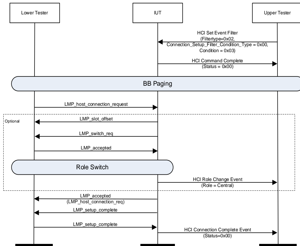
Figure 4.54: HCI/HFC/BV-02-C [Set_Event_Filter Command] MSC
