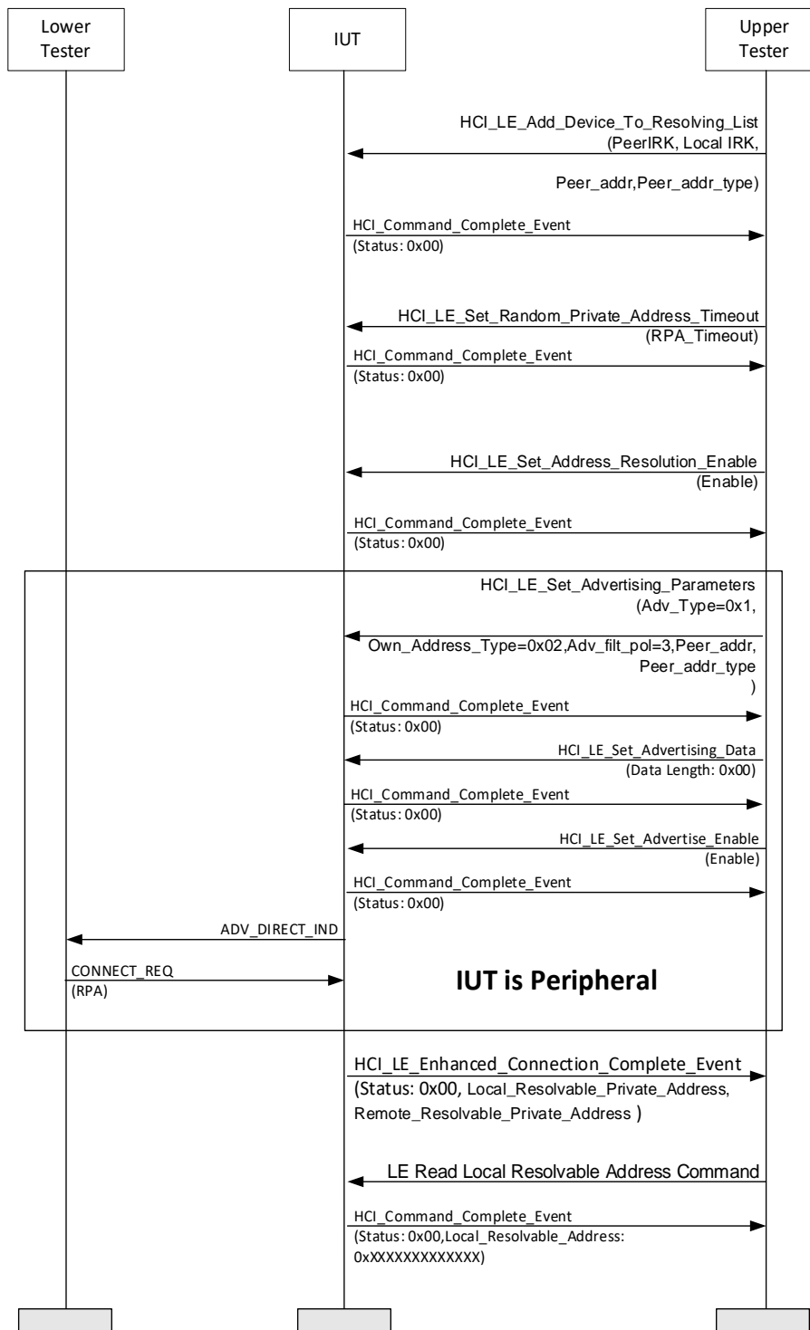
Figure 4.135: HCI/CM/BV-06-C [LE Read Local Resolvable Address Command – Peripheral] MSC
