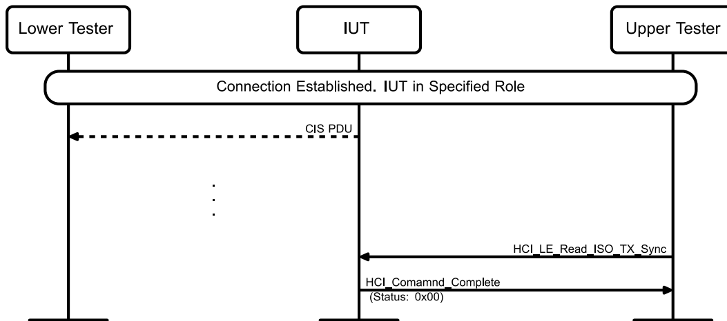
Figure 4.147: Connected Isochronous Stream, Reject Early Read ISO TX Sync MSC
