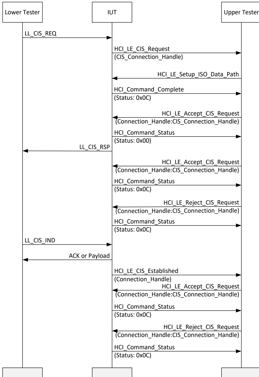
Figure 4.152: HCI/CIS/BI-06-C [Invalid LE Accept or Reject CIS Request, Premature Setup ISO Data Path] MSC
