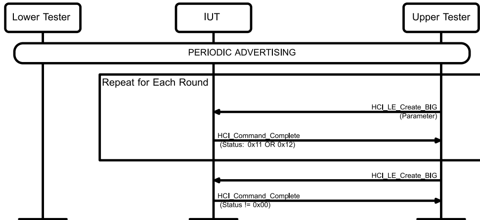
Figure 4.167: HCI/BIS/BI-06-C [Broadcast Isochronous Stream Using Non-Test Command, Invalid BIG Parameters] MSC
