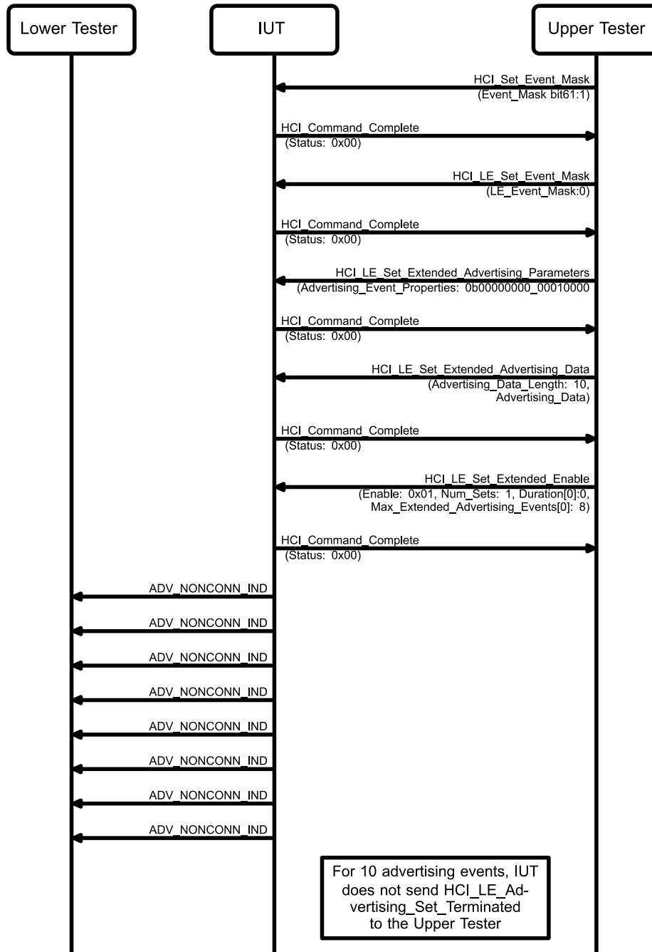
Figure 4.60: HCI/HFC/BV-19-C [LE Set Event Mask – Advertising Set Terminated] MSC – Page 1 of 2
