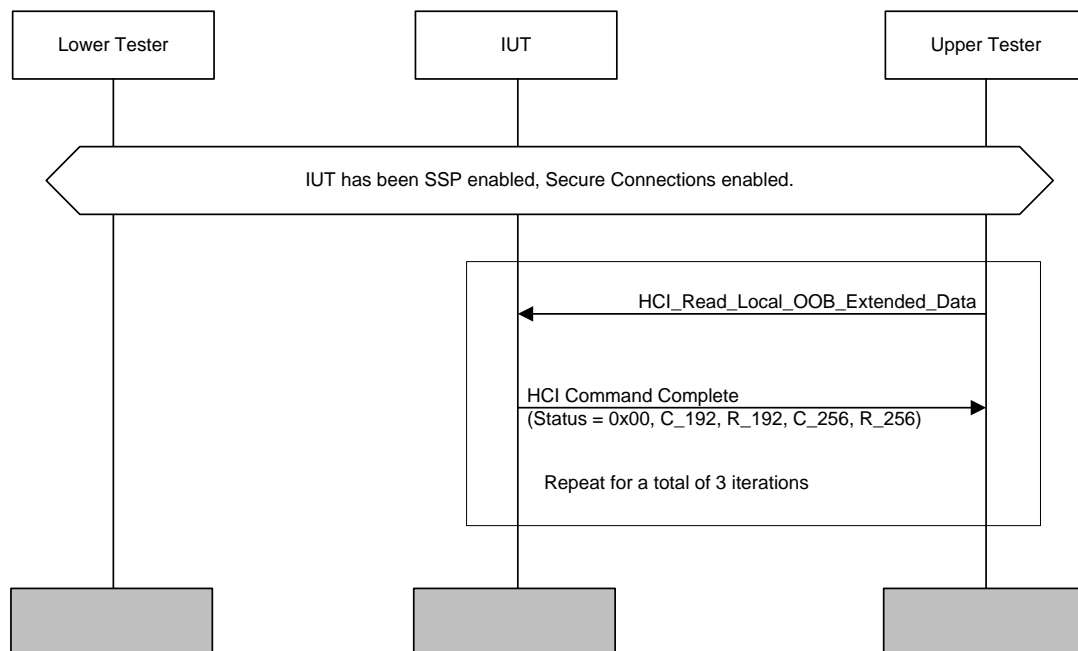
Figure 4.74: HCI/AEN/BV-05-C [Read Local OOB Extended Data Command, test unique values] MSC
