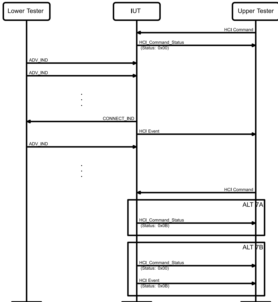
Figure 4.139: Connection Attempt Rejected When Connected to the Peer MSC
