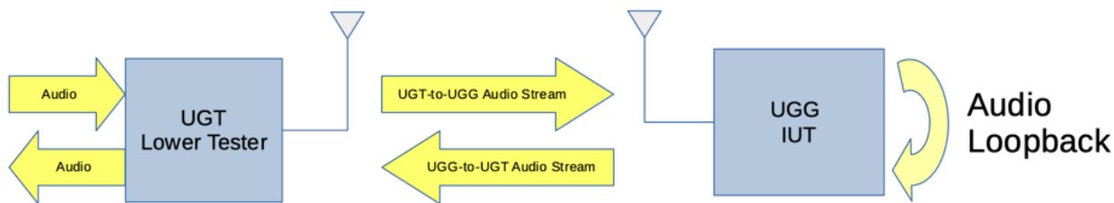
Figure 3.22: UGG audio loopback test configuration
