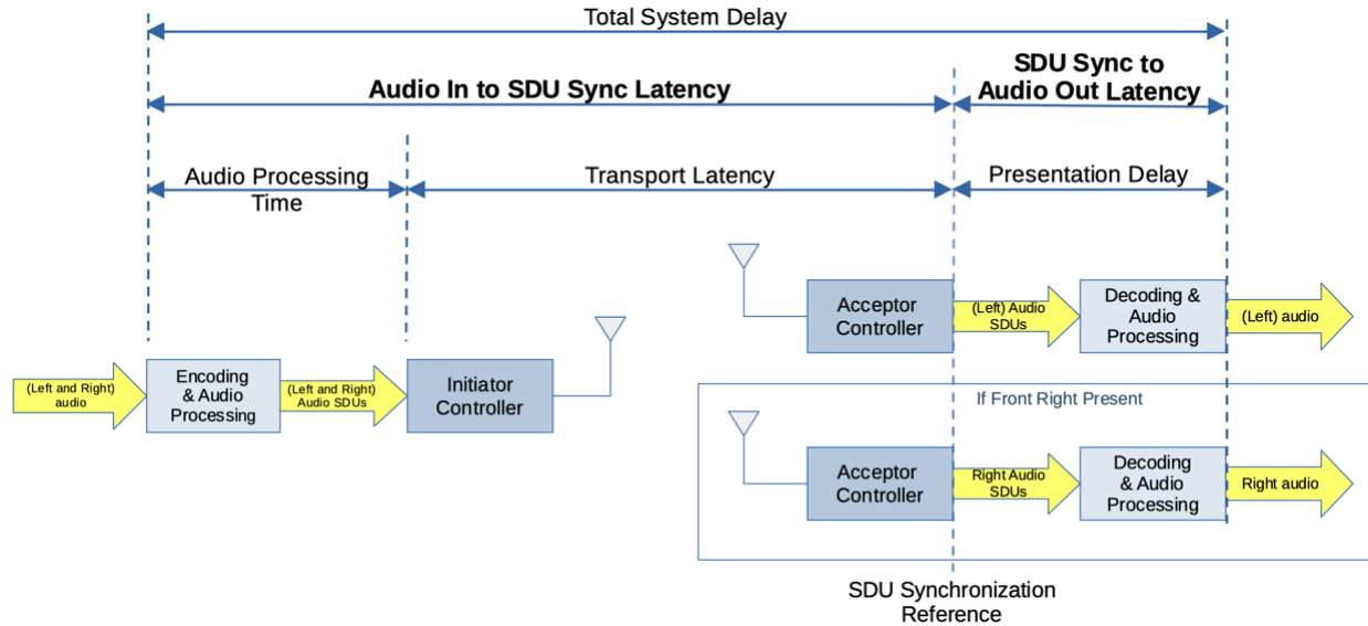
Figure 3.6: Generalized Initiator to Acceptor audio system delays
