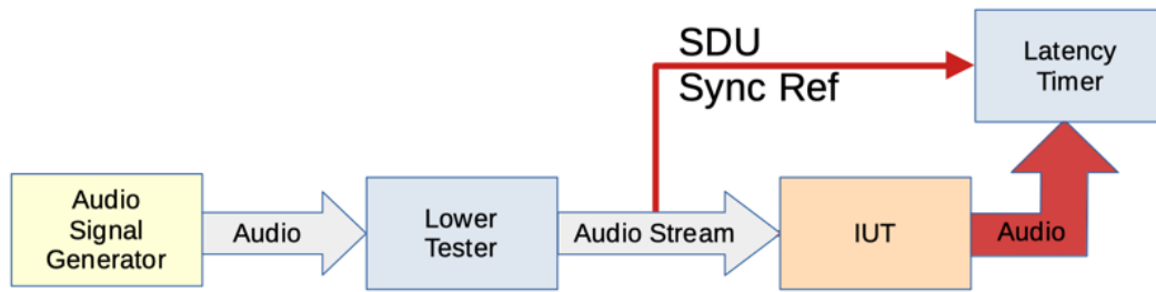
Figure 3.9: Latency testing with an Acceptor IUT, Initiator to Acceptor audio direction
