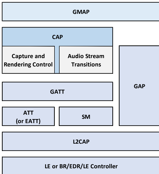
Figure 3.1: GMAP stack
