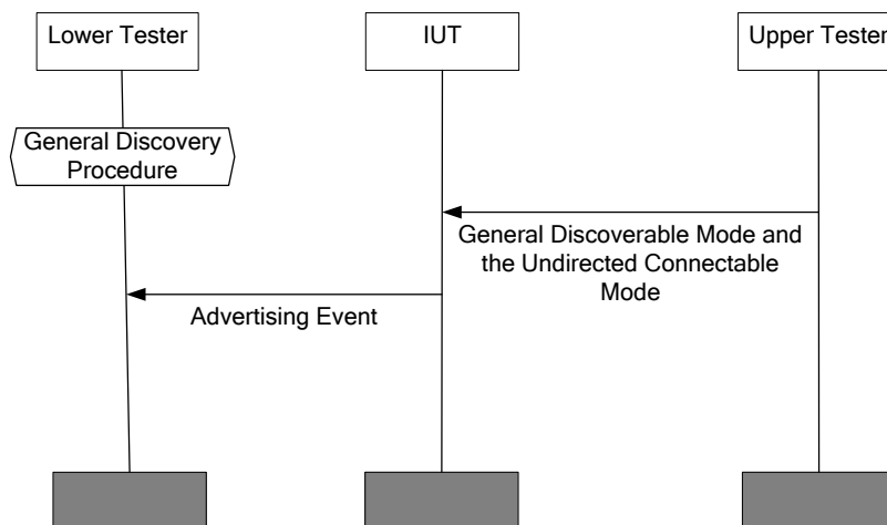
Figure 4.100: GAP/DISC/GENM/BV-04-C [General Discoverable mode, Undirected Connectable mode – LE Only] MSC
