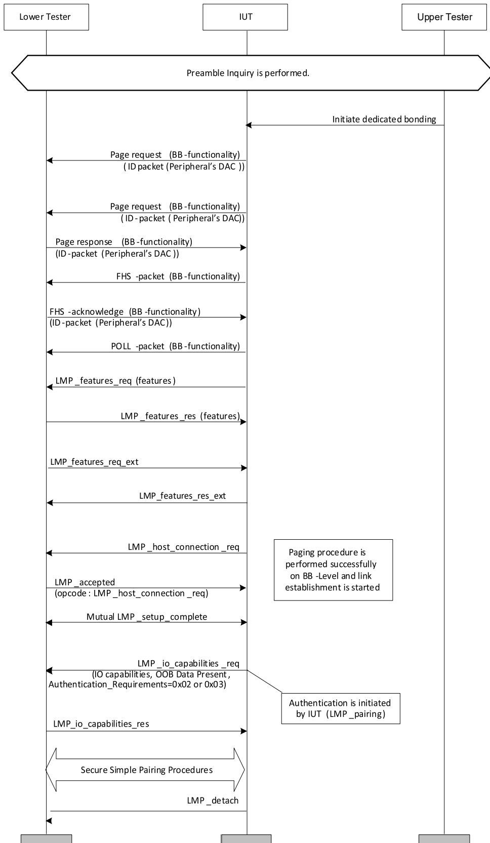
Figure 4.77: GAP/IDLE/BON/BV-03-C [Dedicated Bonding] MSC
