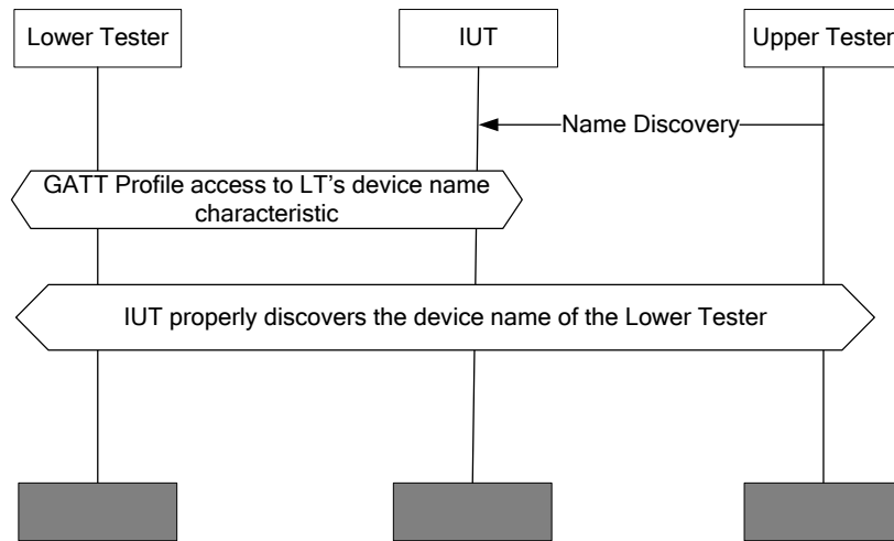
Figure 4.211: GAP/DM/NAD/BV-02-C [LE Name Discovery] MSC
