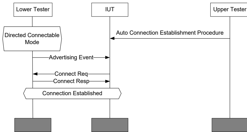
Figure 4.123: GAP/CONN/ACEP/BV-01-C [Auto Connection Establishment procedure, Directed Connectable mode] MSC
