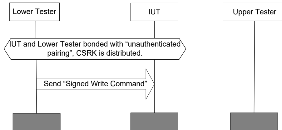
Figure 4.173: GAP/SEC/CSIGN/BI-04-C [Connection Based Signing – Receive, Insufficient Authentication, as Peripheral] MSC
