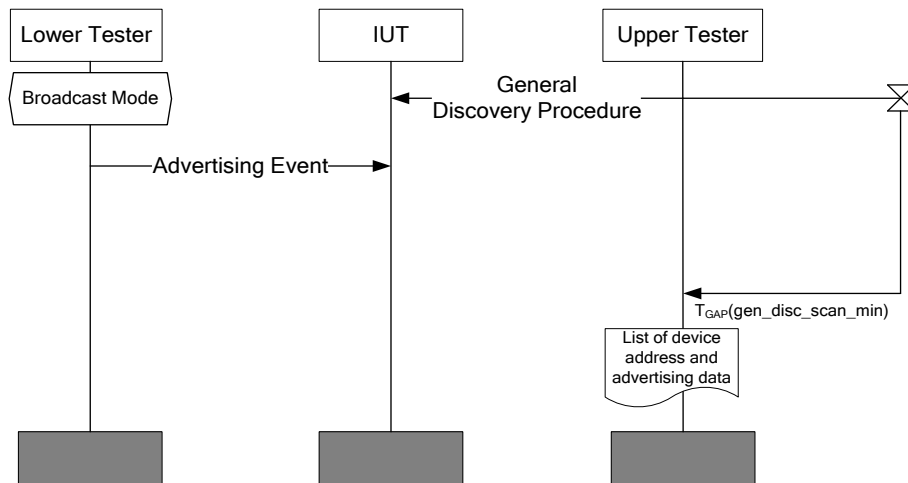
Figure 4.109: GAP/DISC/GENP/BV-04-C [General Discovery procedure does not find Undirected Connectable device] MSC
