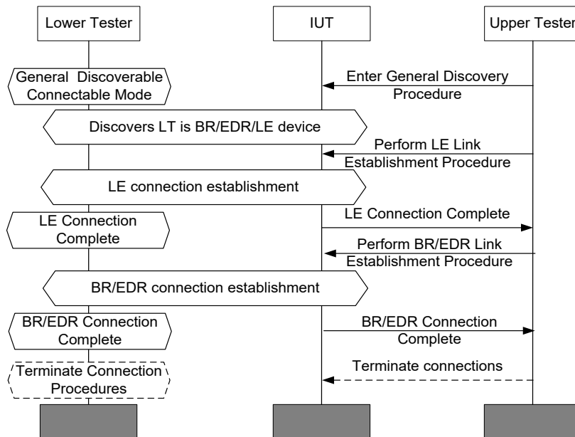
Figure 4.216: GAP/DM/LEP/BV-09-C [BR/EDR/LE and BR/EDR/LE Link Establishment IUT is Central/BR Central – LE and BR/EDR Transports] MSC
