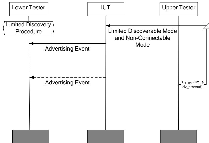
Figure 4.93: GAP/DISC/LIMM/BV-01-C [Limited Discoverable mode, Non-Connectable mode – BR/EDR/LE] MSC
