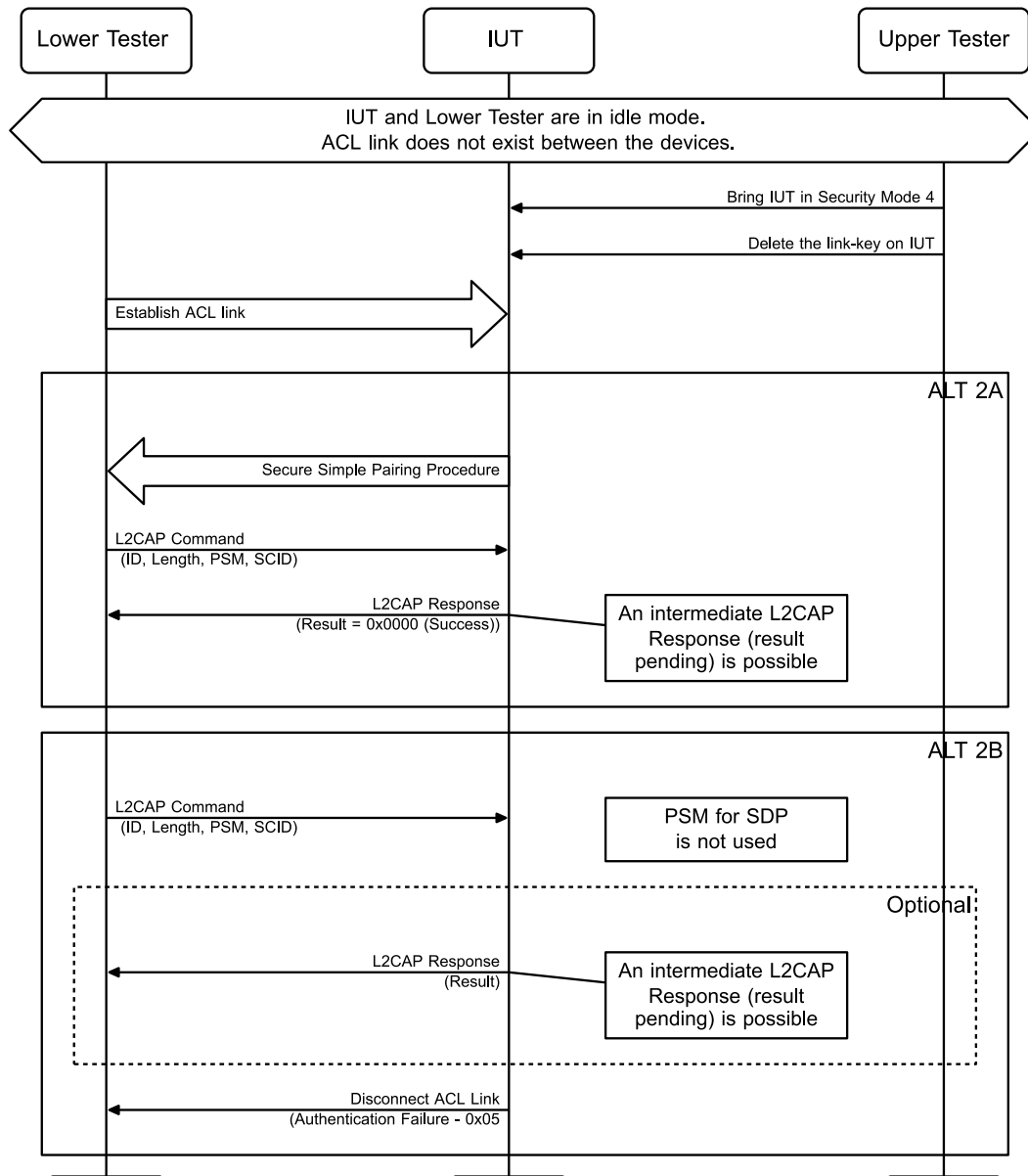
Figure 4.42: Security mode 4 – Responder MSC
