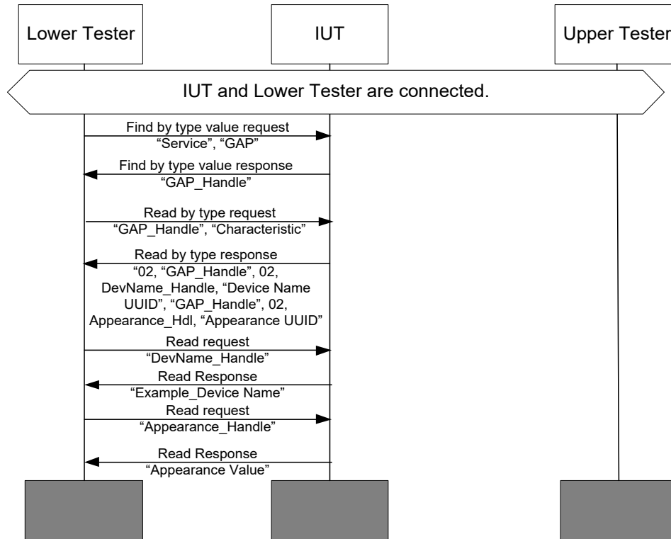
Figure 4.6: GAP Mandatory Characteristics MSC
