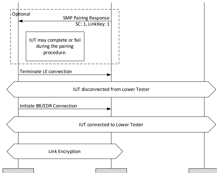
Figure 4.236: Verify that a Weaker LE Key Does Not Overwrite a Stronger Key, as Responder MSC – Page 2 of 2
