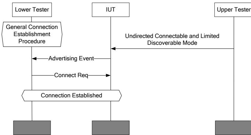
Figure 4.122: GAP/CONN/UCON/BV-03-C [Undirected Connectable mode, Limited Discoverable mode] MSC
