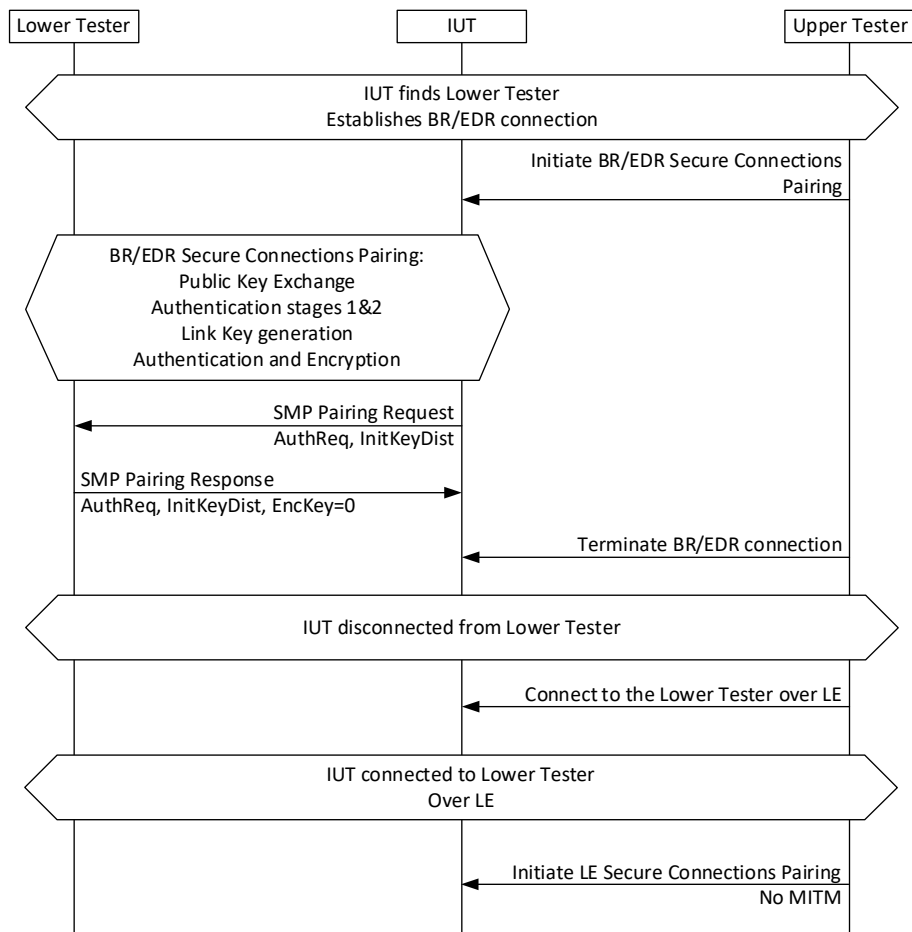
Figure 4.233: Verify that a Weaker LE Key Does Not Overwrite a Stronger Key, as Initiator MSC – Page 1 of 2
