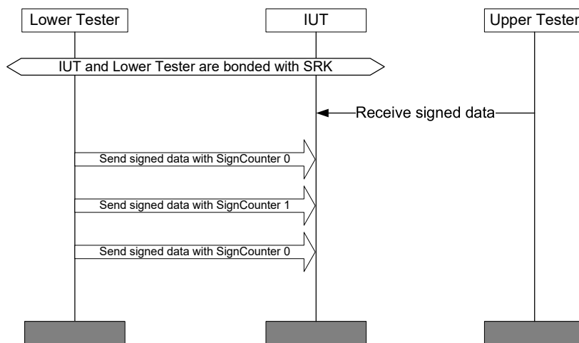
Figure 4.171: GAP/SEC/CSIGN/BI-02-C [Connection Based Signing – Receive Invalid SignCounter] MSC
