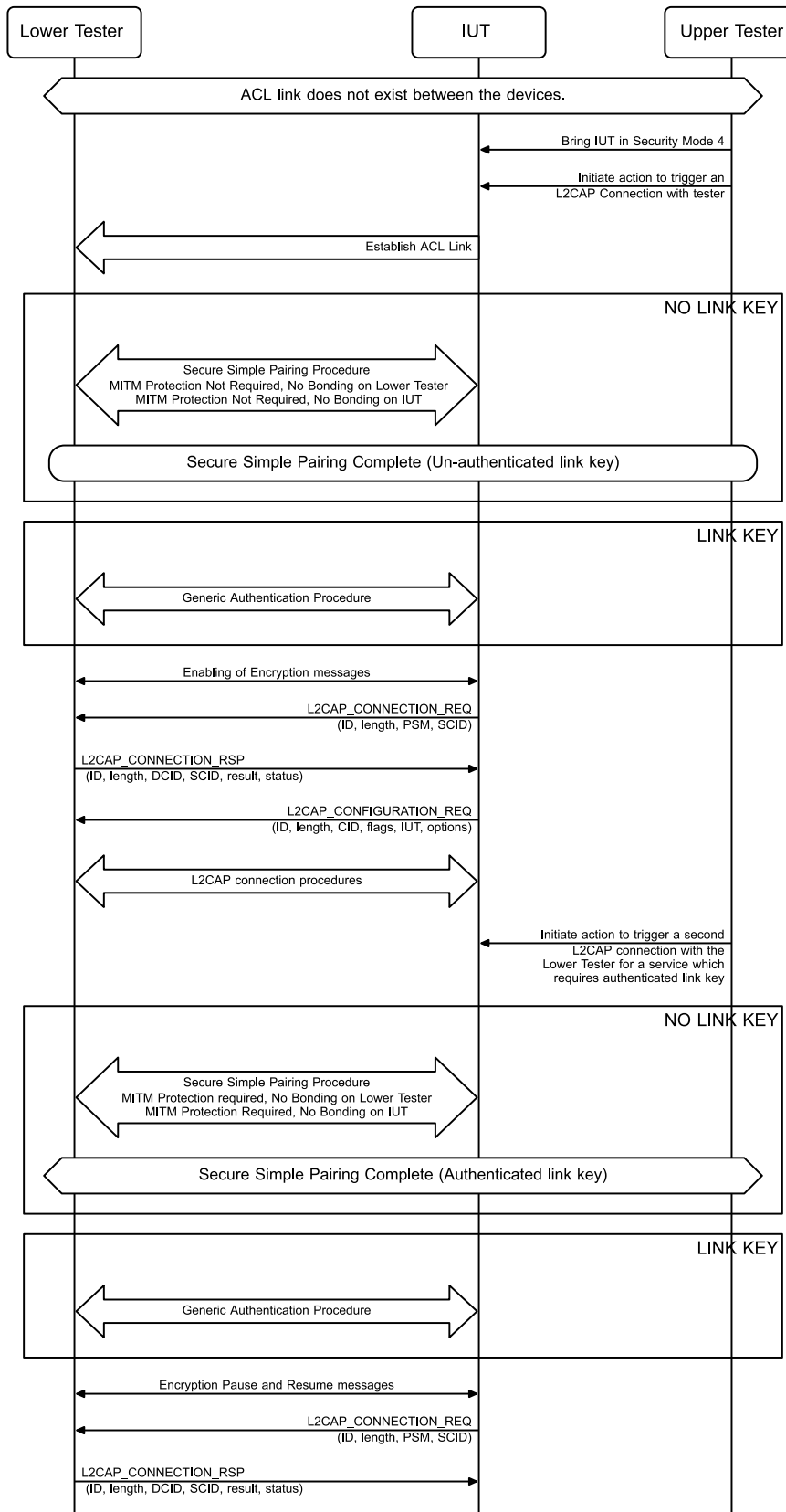
Figure 4.41: Security mode 4 – Link Key Upgrade – Initiator MSC
