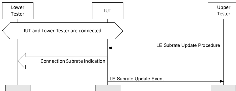
Figure 4.201: GAP/CSUB/CSU/BV-01-C [Connection Subrate Update procedure] MSC
