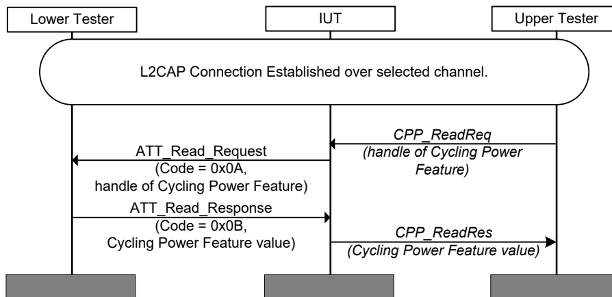
Figure 4.4: Read Cycling Power Feature characteristic with reserved value MSC
