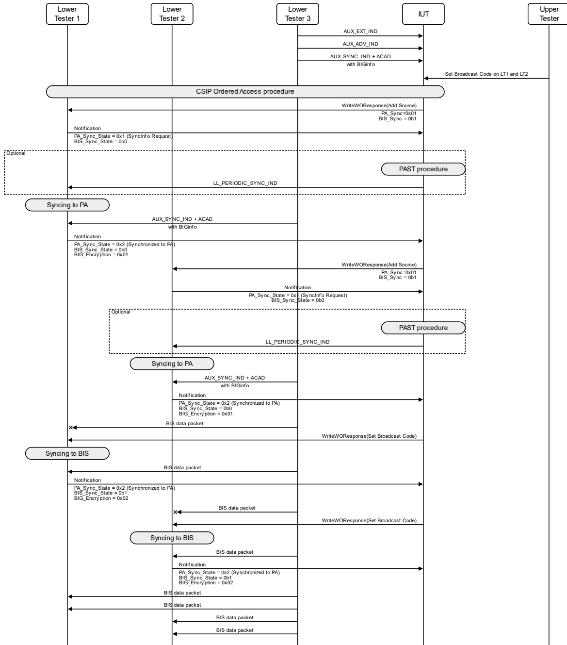
Figure 4.1: Distribute Broadcast Code MSC
