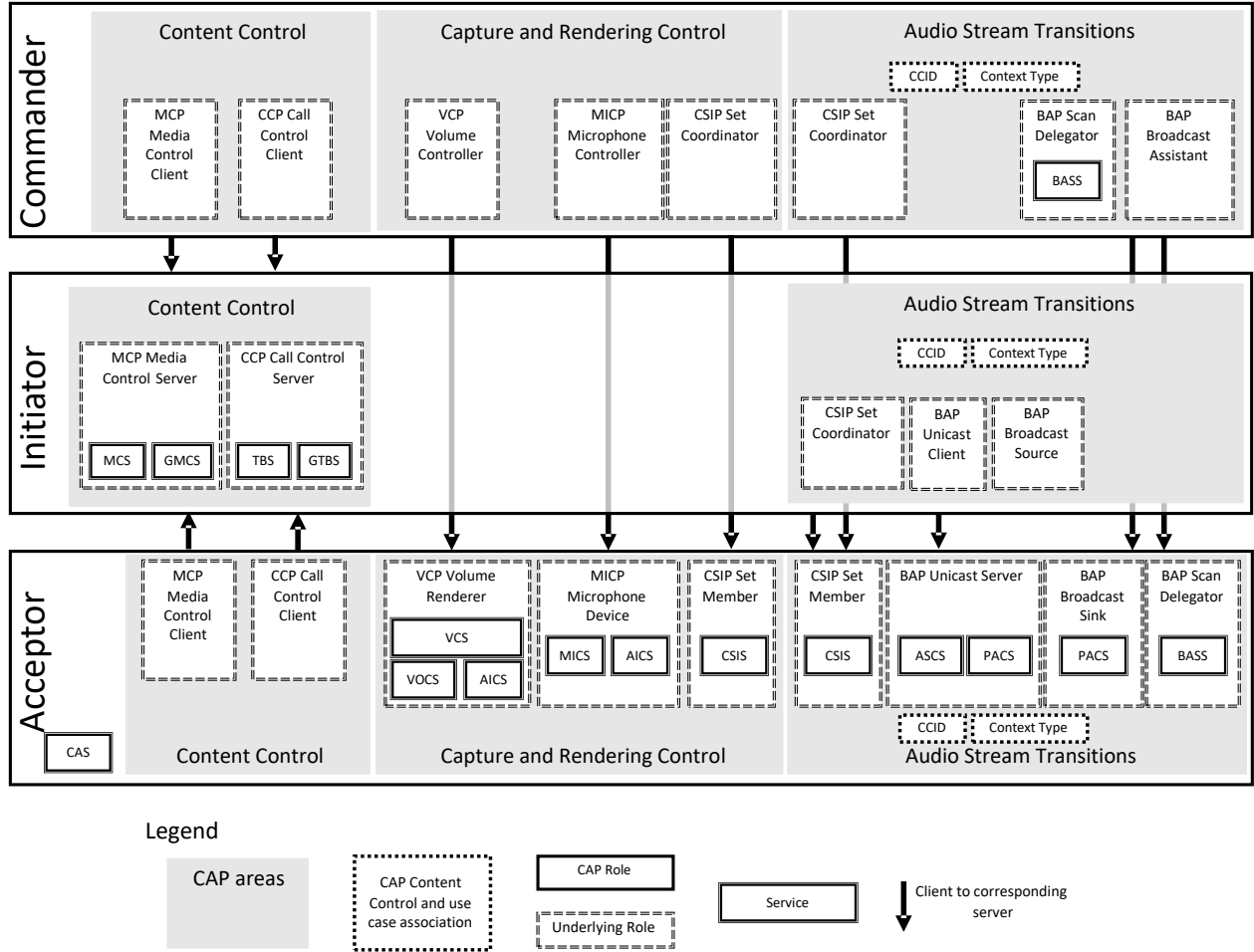
Figure 3.1: Example of the relationship between services and profile roles. The CSIP/CSIS profiles/services implementation is shared between Capture and Rendering Control and Audio Stream Transitions, but it is depicted as two identical roles.
