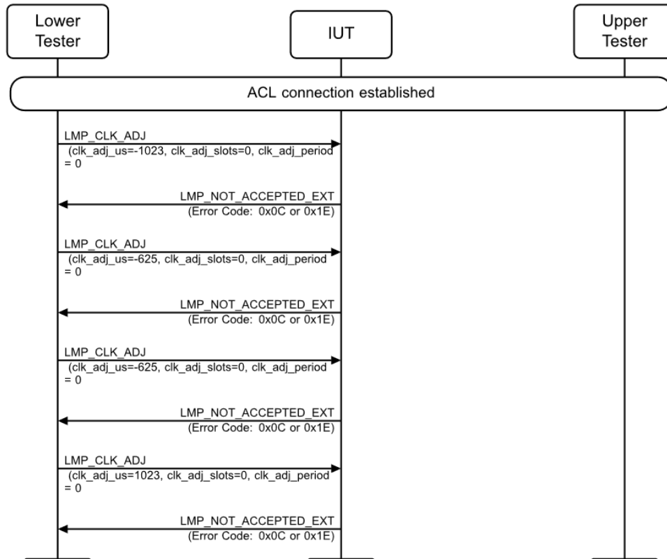
Figure 4.130: BB/XCB/BV-16-C [Central rejection of invalid adjustment requests] MSC
