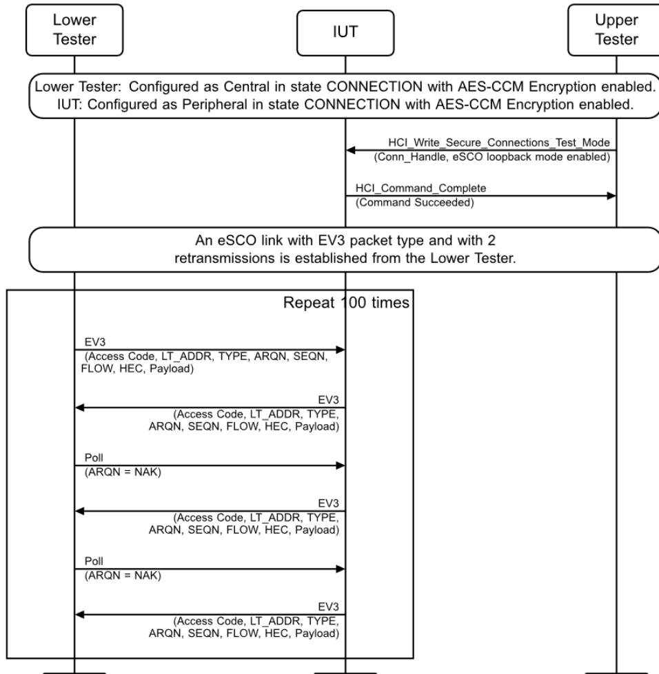
Figure 4.39: BB/PROT/ARQ/BV-40-C [Retransmitting eSCO with AES as Peripheral] MSC
