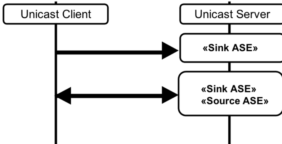
Figure 4.20: Audio Configuration 8(i)
