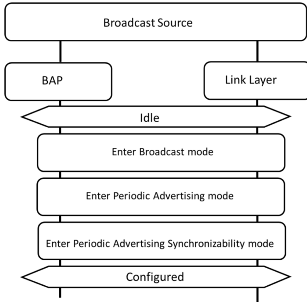
Figure 6.4: Broadcast Audio Stream configuration
