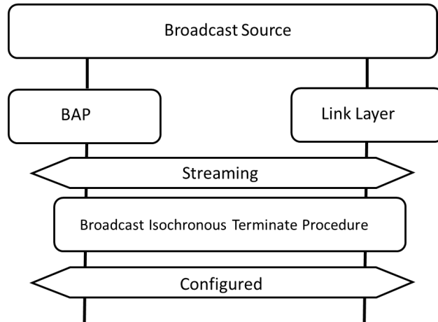
Figure 6.6: Disabling a broadcast Audio Stream
