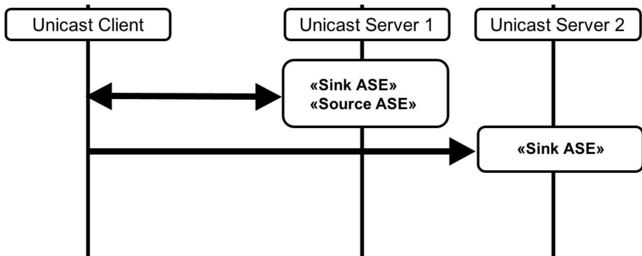
Figure 4.21: Audio Configuration 8(ii)
