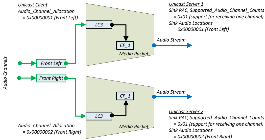
Figure 4.7: Example stereo Audio Stream configured for two Unicast Servers encoded using LC3
