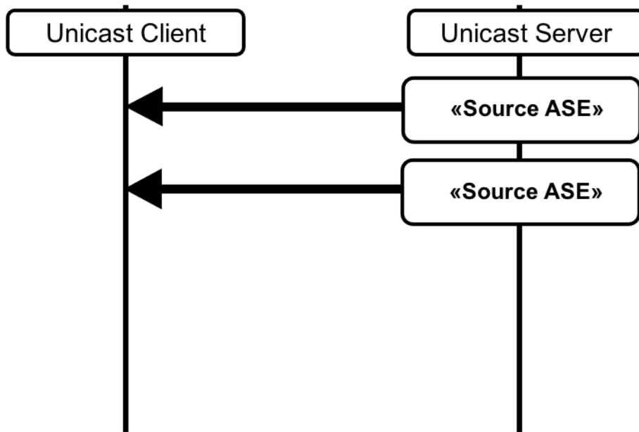
Figure 4.22: Audio Configuration 9(i)
