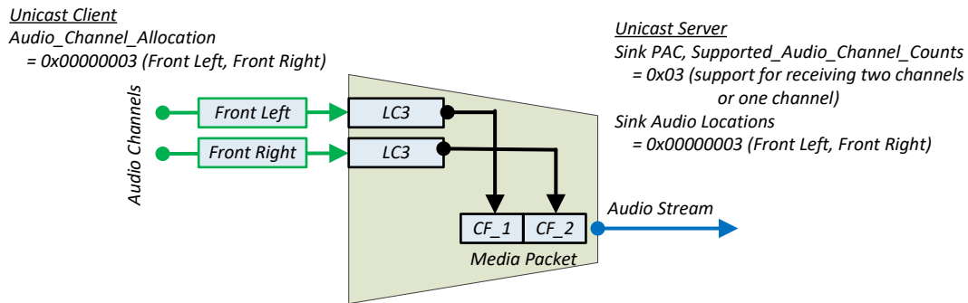
Figure 4.5: Example stereo Audio Stream encoded using multiplexed LC3 codec frames in a single block
