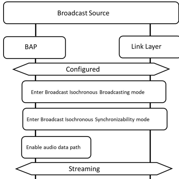
Figure 6.5: Broadcast Audio Stream establishment
