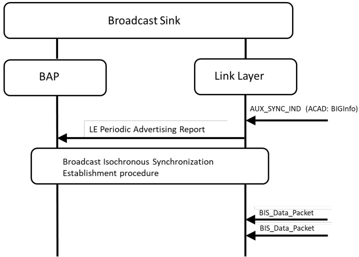
Figure 6.17: Broadcast Audio Stream synchronization
