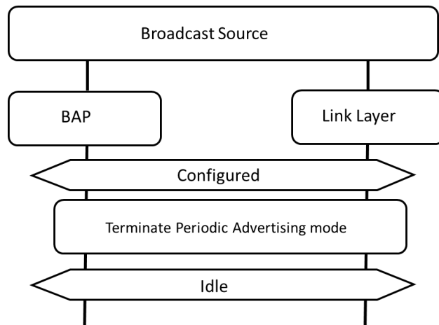
Figure 6.7: Releasing a broadcast Audio Stream
