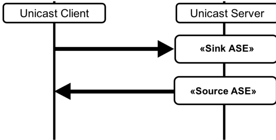
Figure 4.18: Audio Configuration 7(i)
