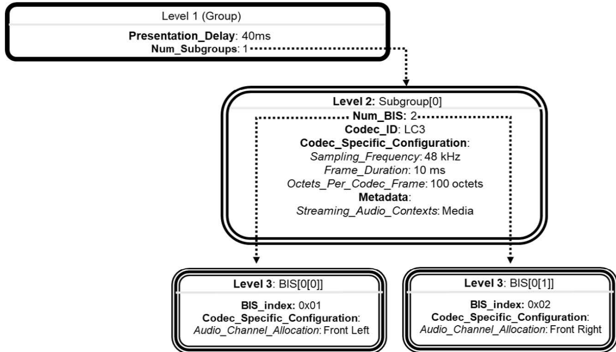
Figure 4.8: Example BASE structure for stereo audio as two streams
