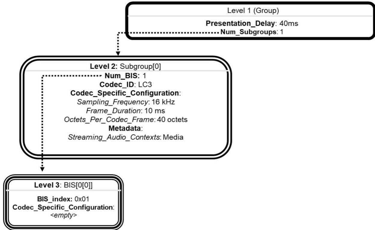
Figure 4.9: Example BASE structure for mono audio
