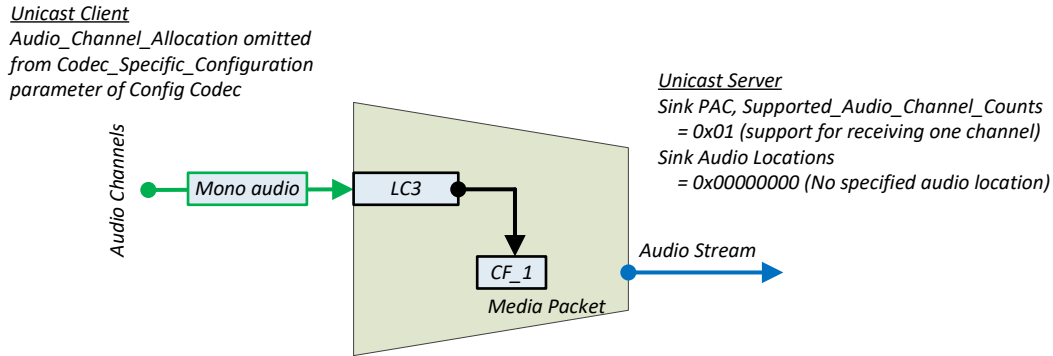
Figure 4.4: Example mono Audio Stream encoded using LC3
