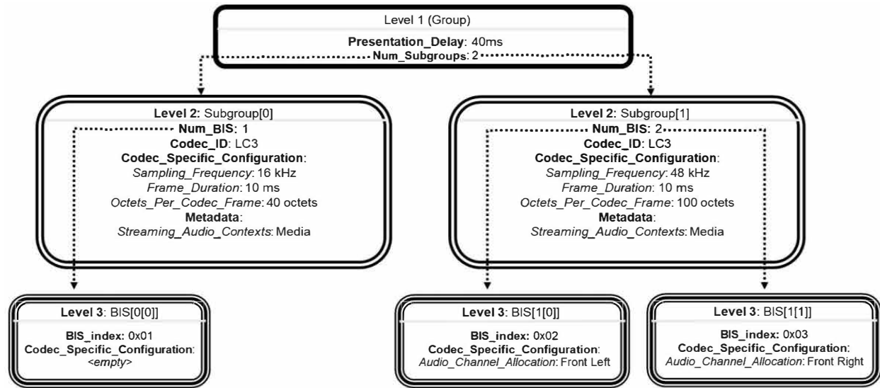
Figure 4.10: Example BASE structure for concurrent mono and stereo broadcast
