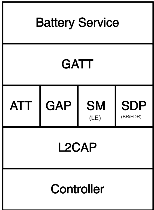
Figure 3.1: Battery Service test model
